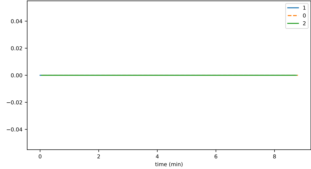
SmartContractService:SystemContractMethodCall_ERC721_failed
