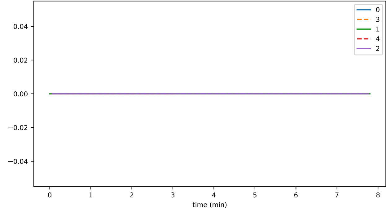
doNotSyncFallenBehind
