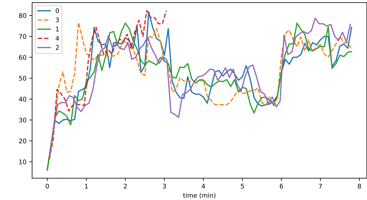
doNotSyncFallenBehind
