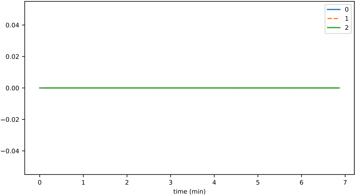
SmartContractService:SystemContractMethodCall_SCHEDULE_failed
