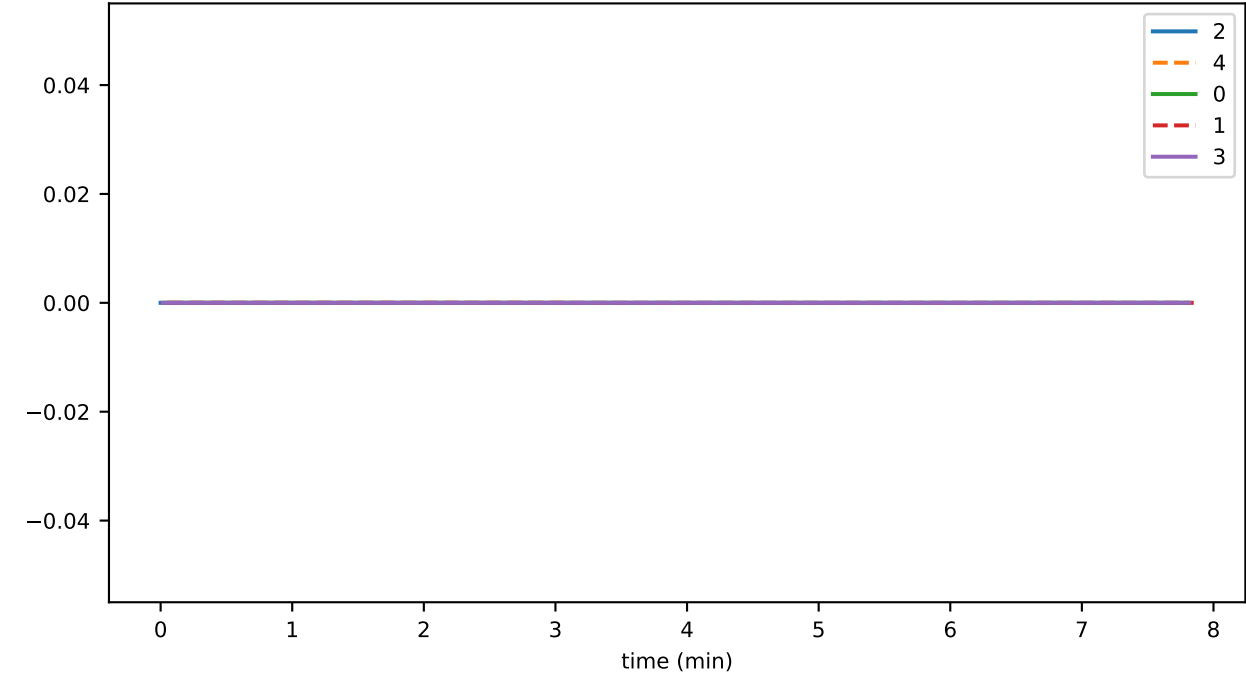
totalNeverSignedStates
