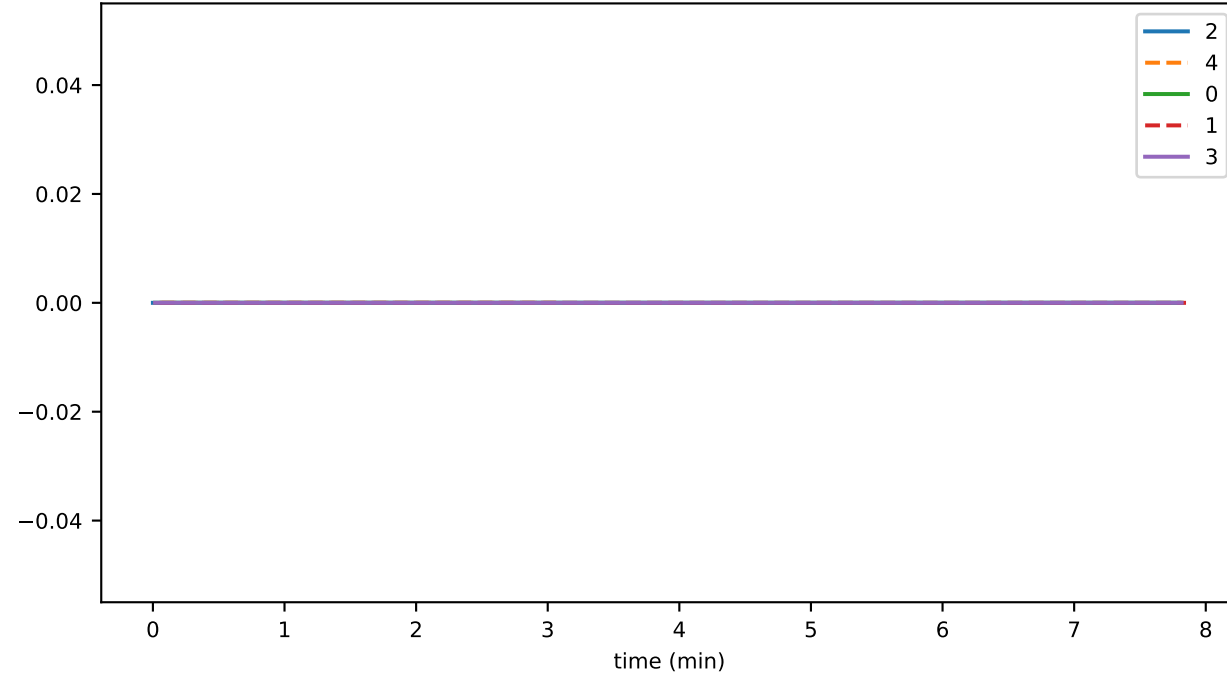
totalNeverSignedDiskStates
