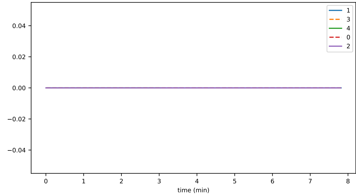
totalNeverSignedStates
