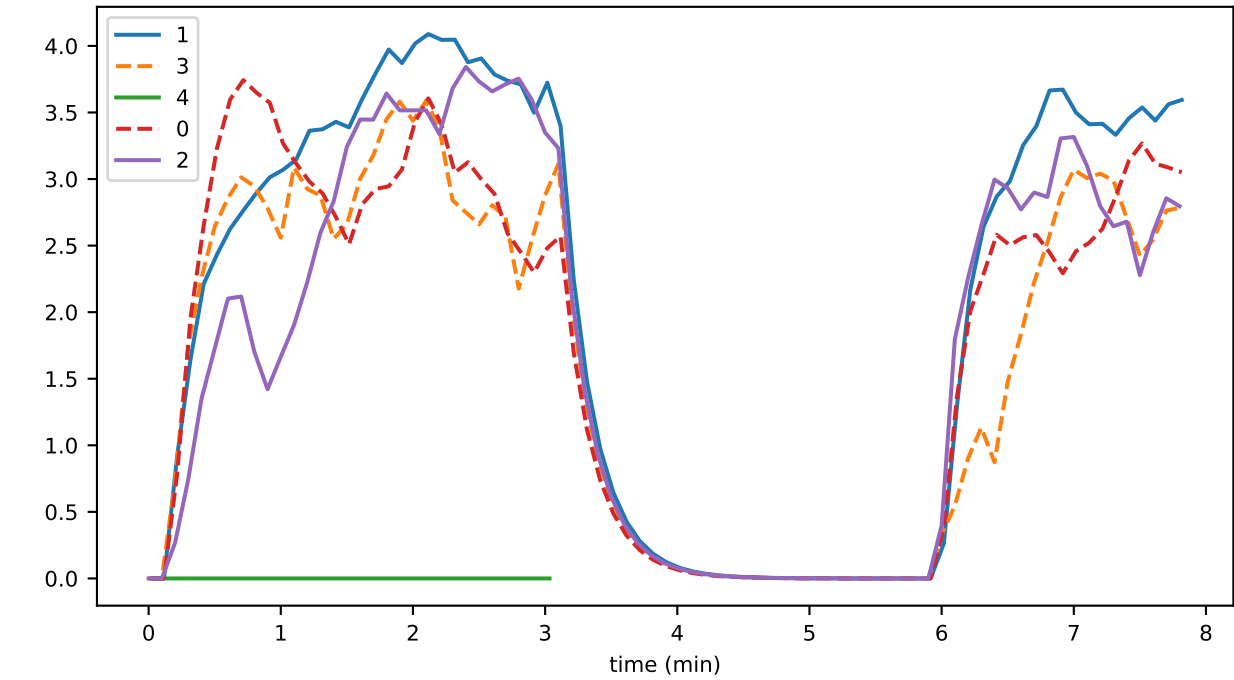
totalNeverSignedStates
