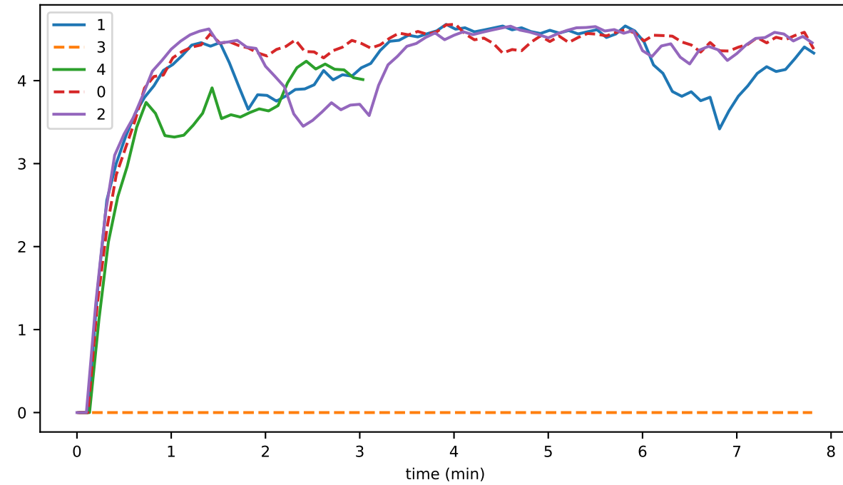
totalNeverSignedDiskStates
