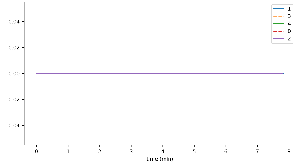
totalNeverSignedDiskStates
