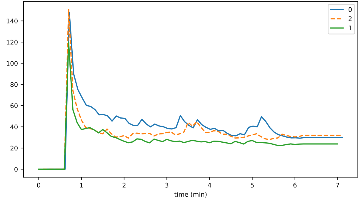
consensus_time_HANDLING_CONSENSUS_ROUND
