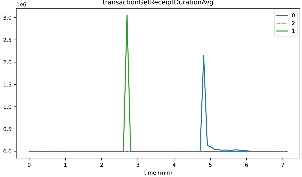
transactionGetReceiptDurationAvg
