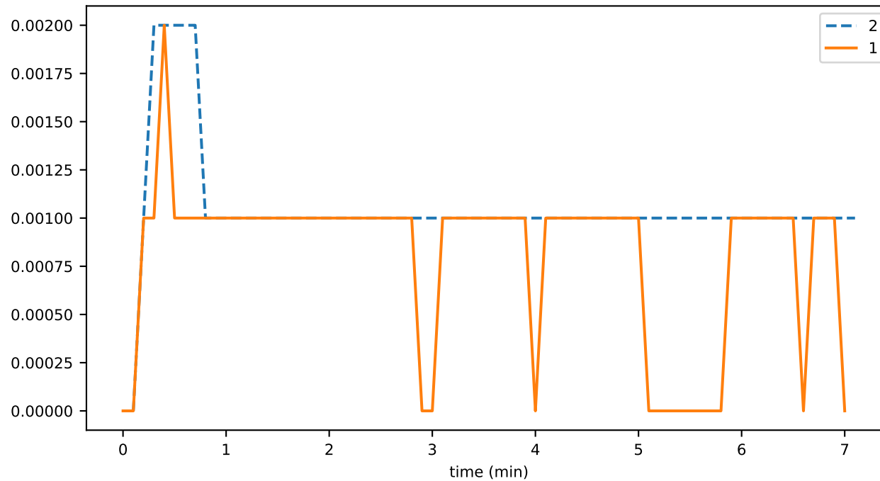
sync_phase_00_fraction_EXCHANGING_EVENTS
