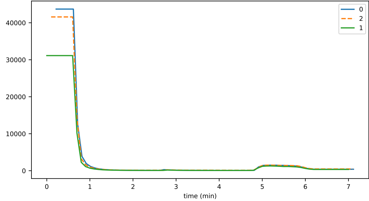
consensus_time_HANDLING_CONSENSUS_ROUND
