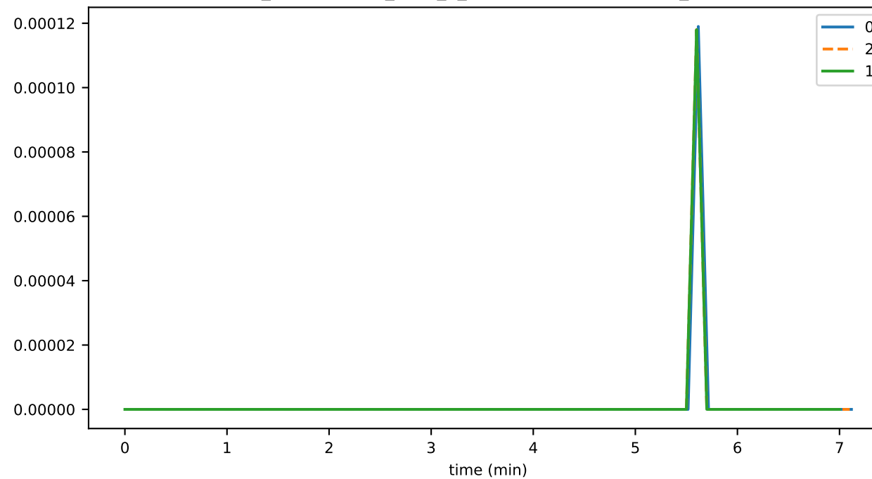
ds_compactions_level_3_leafKeysSavedSpaceMb_state
