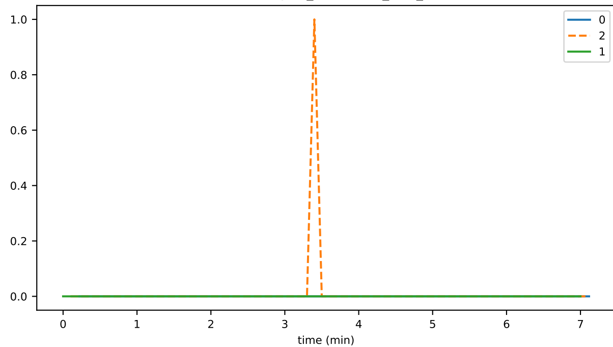
consensusGetTopicInfoDurationMax
