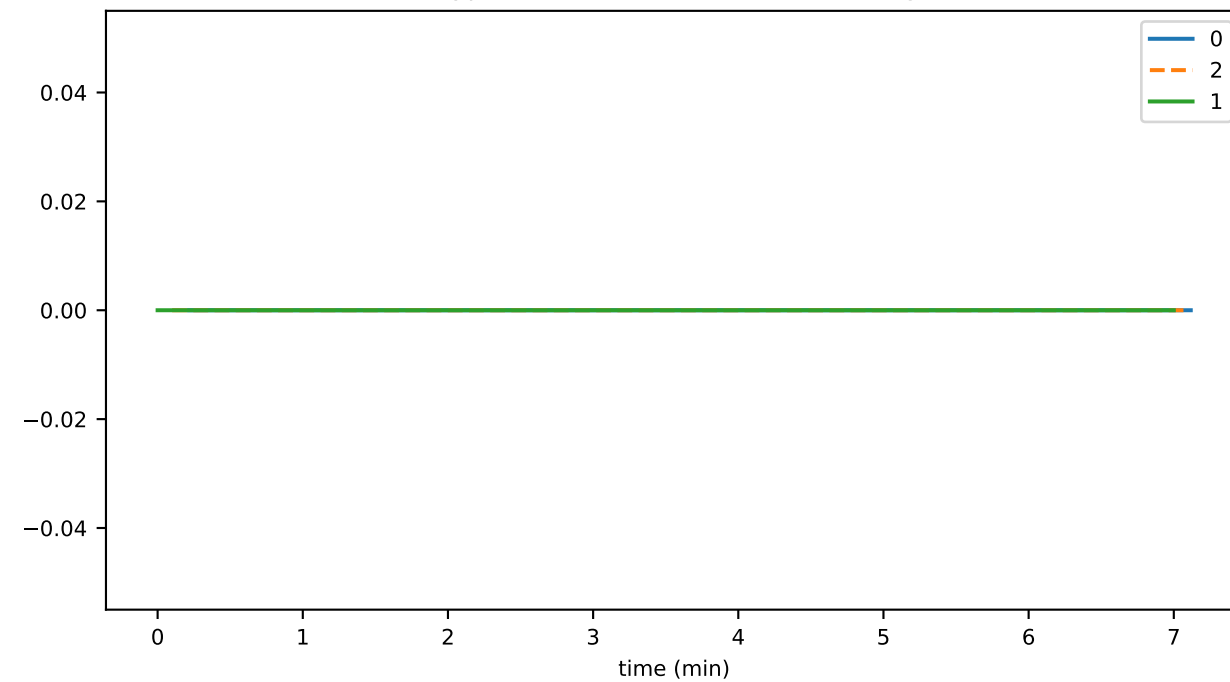
cryptoGetAccountRecordsThrottledTxns
