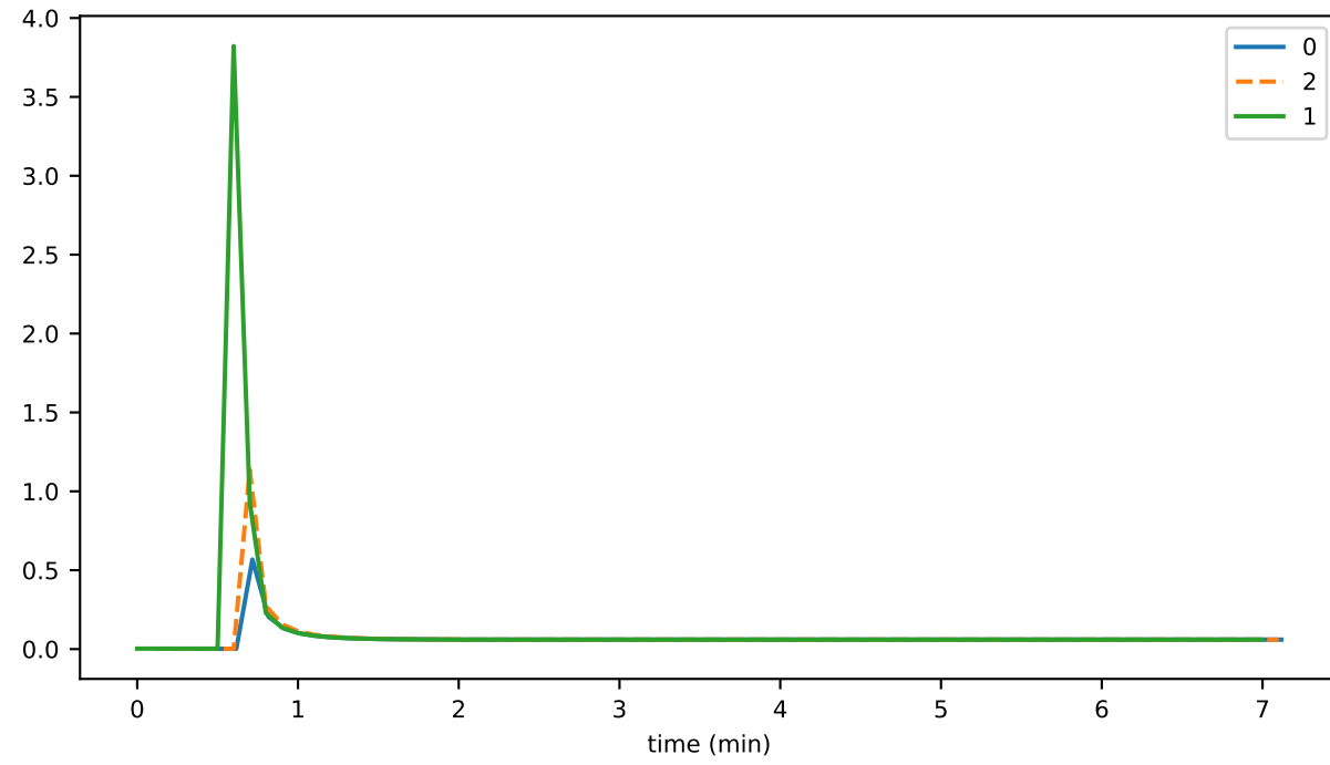
secR2nR
