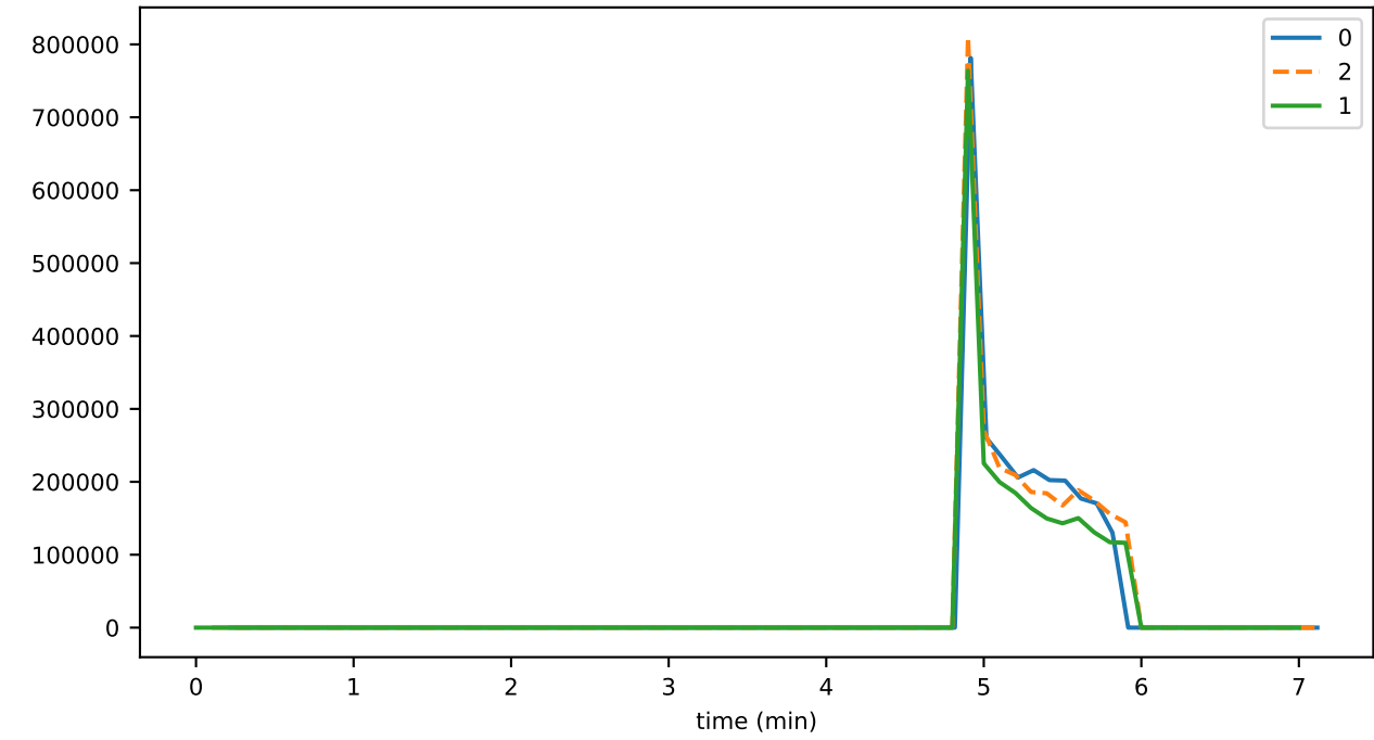
cryptoTransferThrottledTxns
