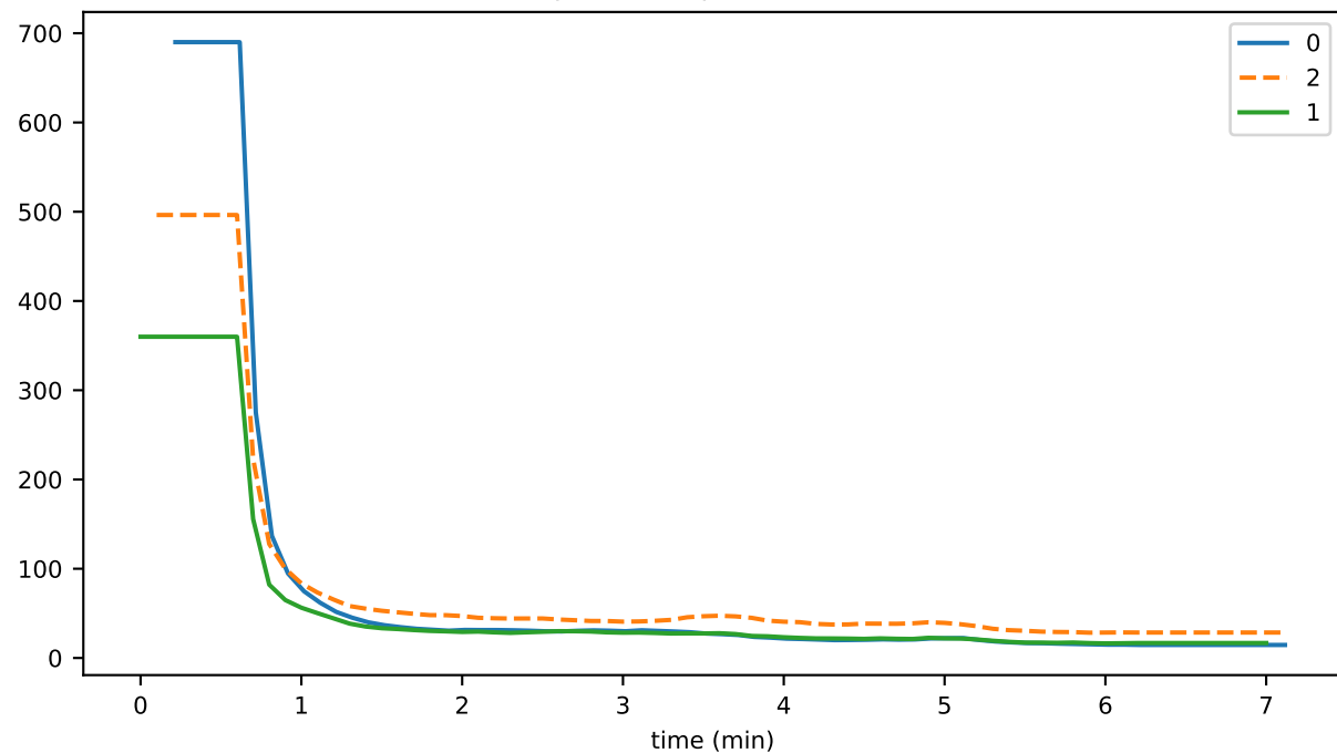
utilPngDurationMax
