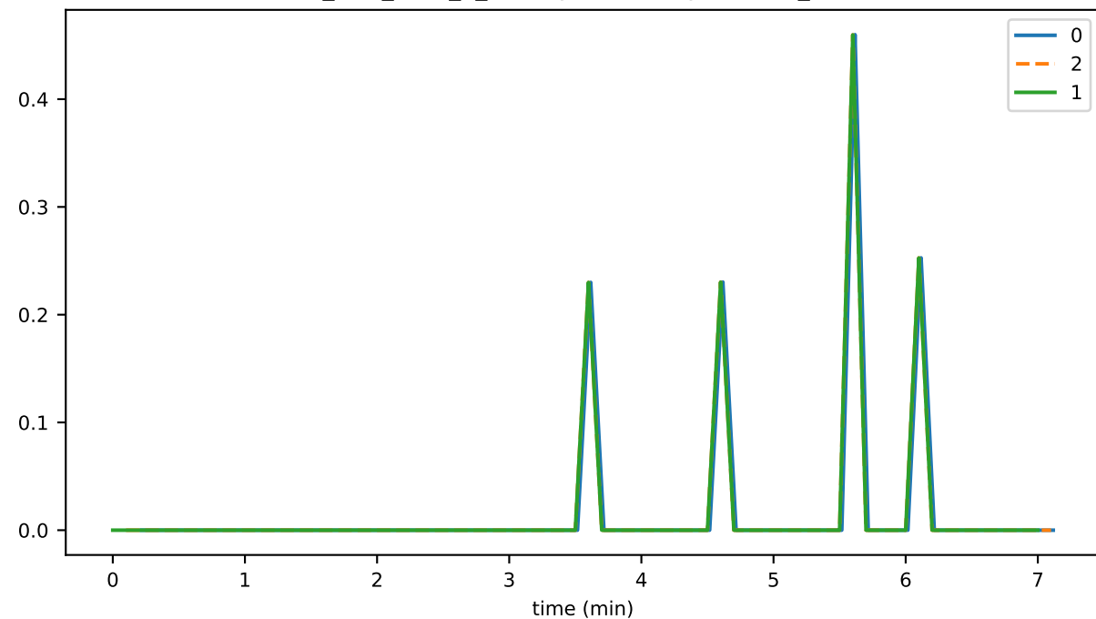
ds_files_level_2_hashesFileSizeByLevelMb_state
