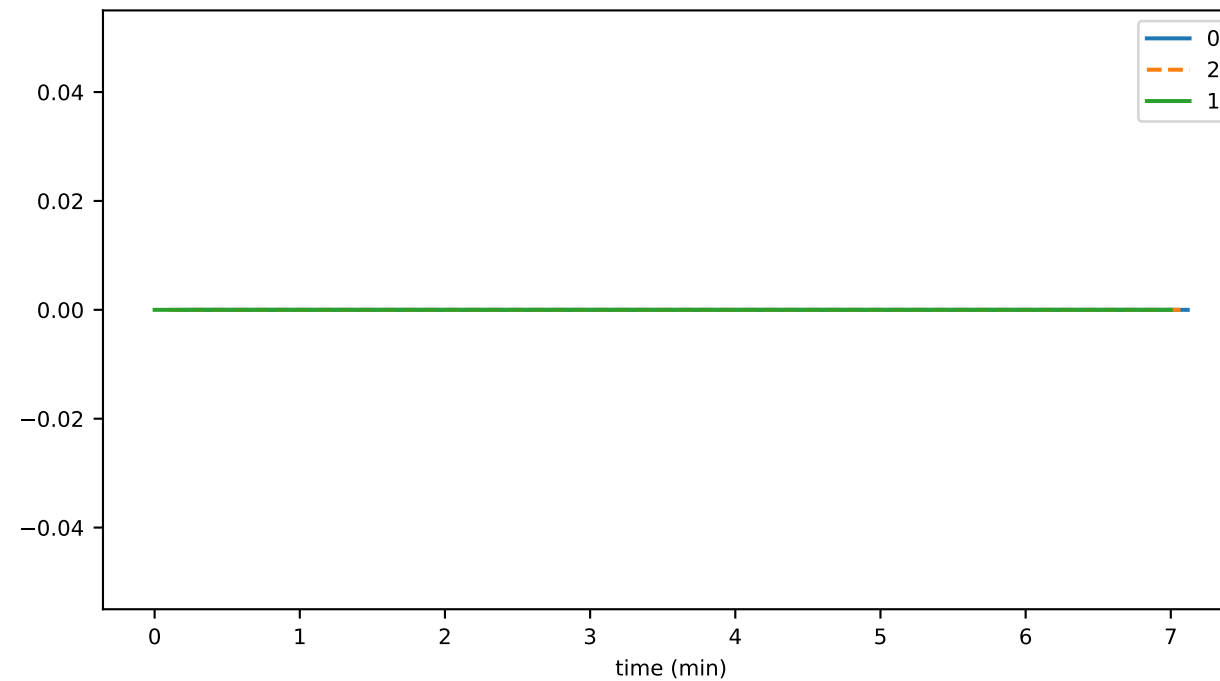
utilPngThrottledTxns
