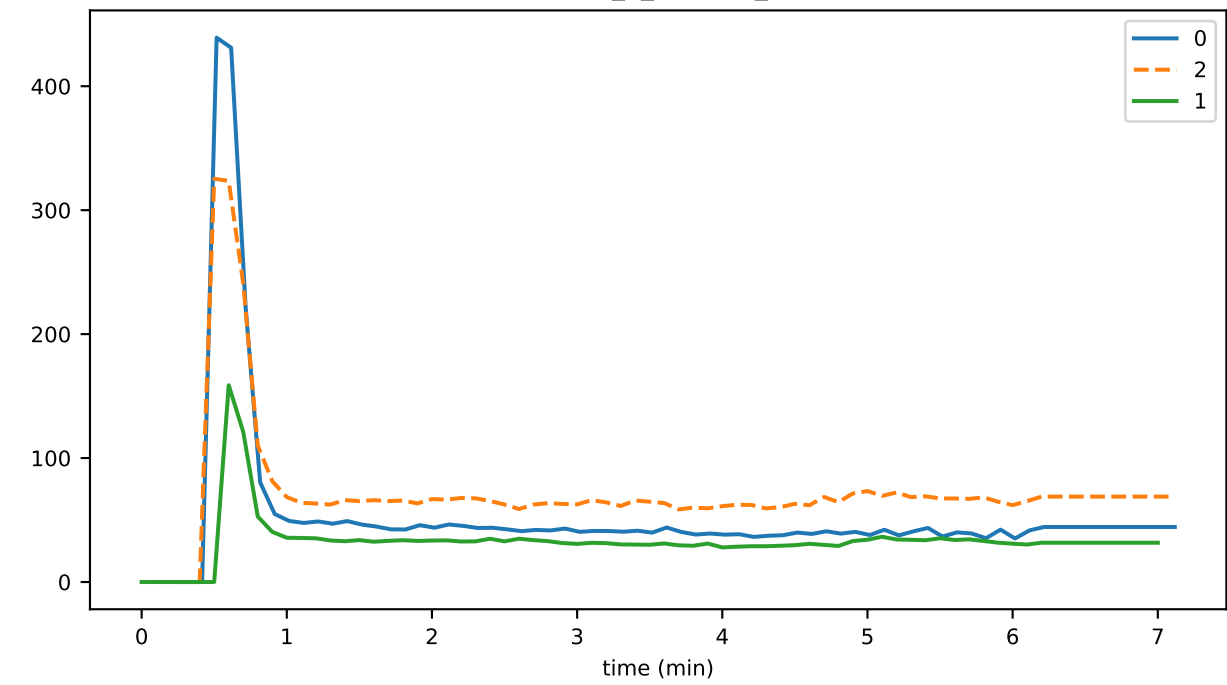
eventDelay_1_hashing_gossip
