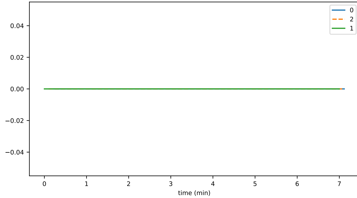
cryptoTransferDurationMax
