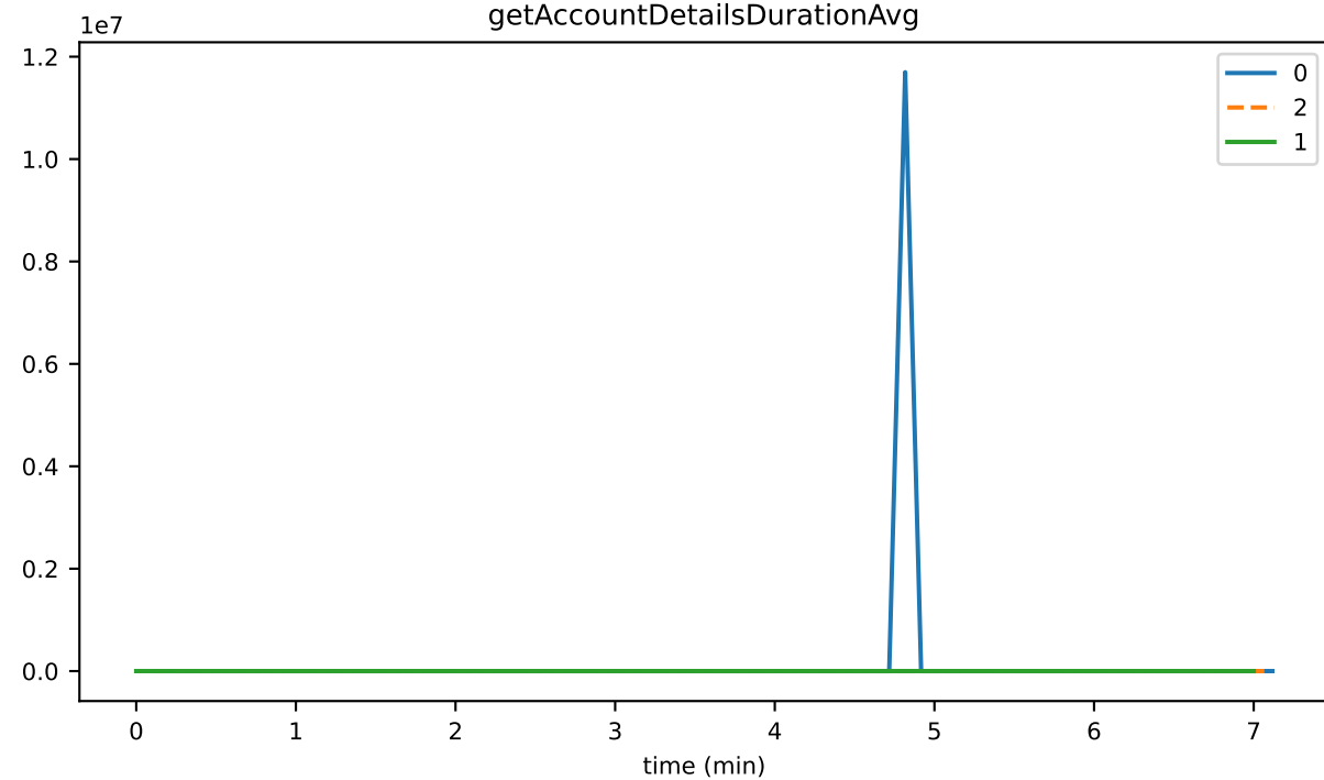
getAccountDetailsDurationAvg
