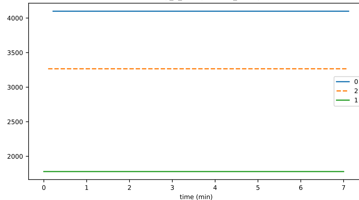
eventDelay_4_verification_gossip
