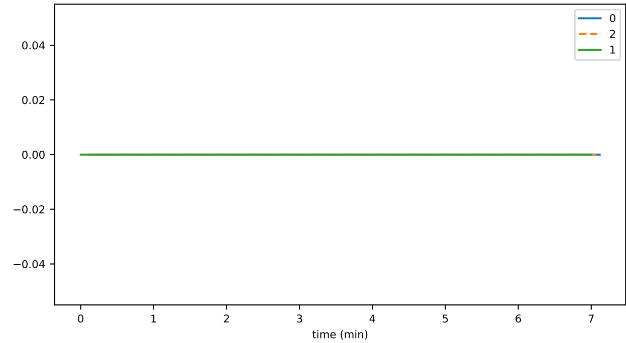
SmartContractService:SystemContractMethodCall_REJECT_failed
