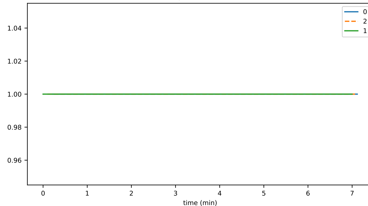
hintsKeyPublicationDurationMax
