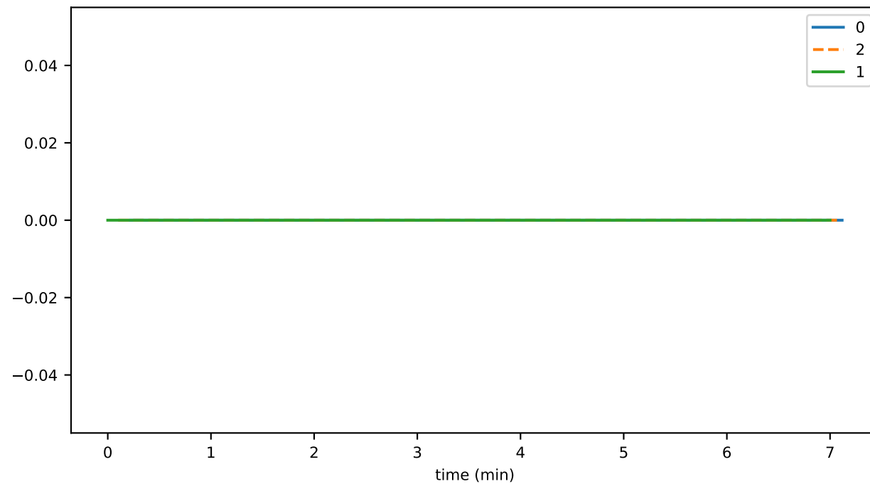
atomicBatchDurationAvg
