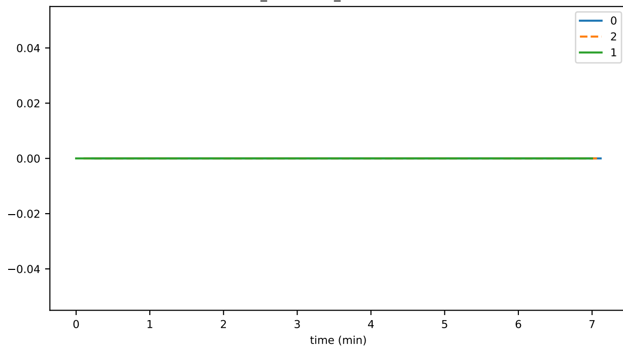
conn_connClose_connectionError
