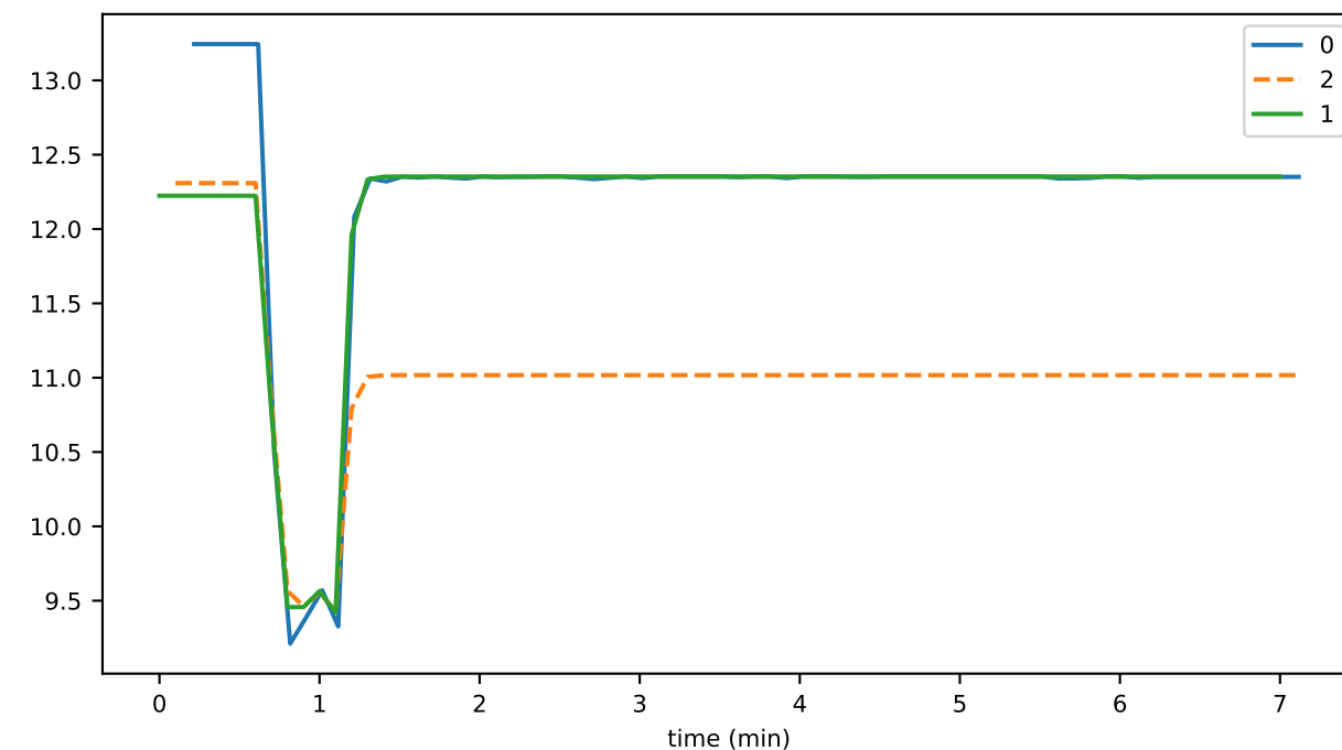
numIndirectProofs
