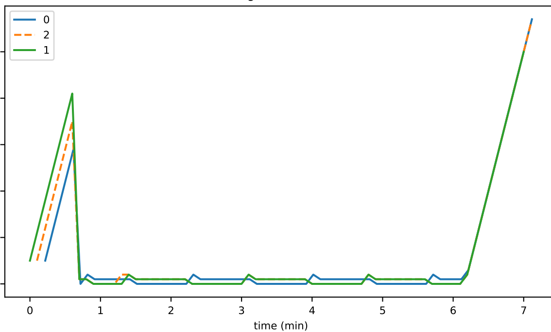
oldestSignedStateSeconds
