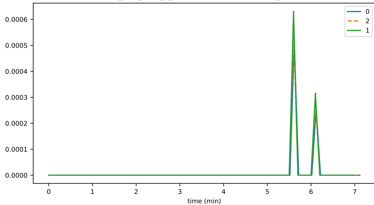
ds_files_level_3_leafKeysFileSizeByLevelMb_state
