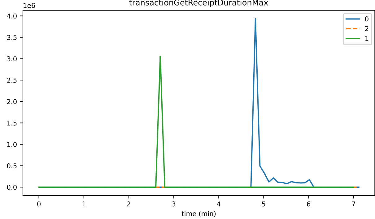
transactionGetReceiptDurationMax
