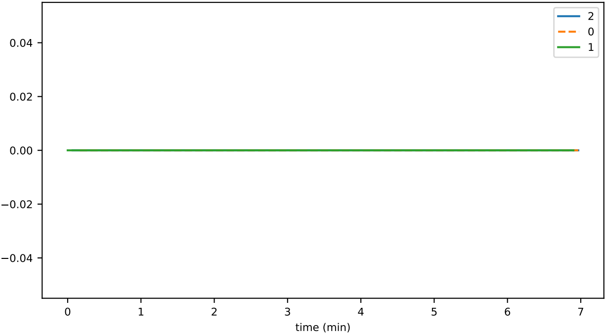
SmartContractService:SystemContractMethodCall_PAUSE_UNPAUSE_failed
