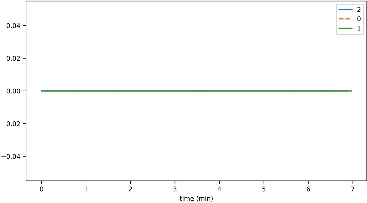
SmartContractService:Rejected_ethType3BlobTransaction_total
