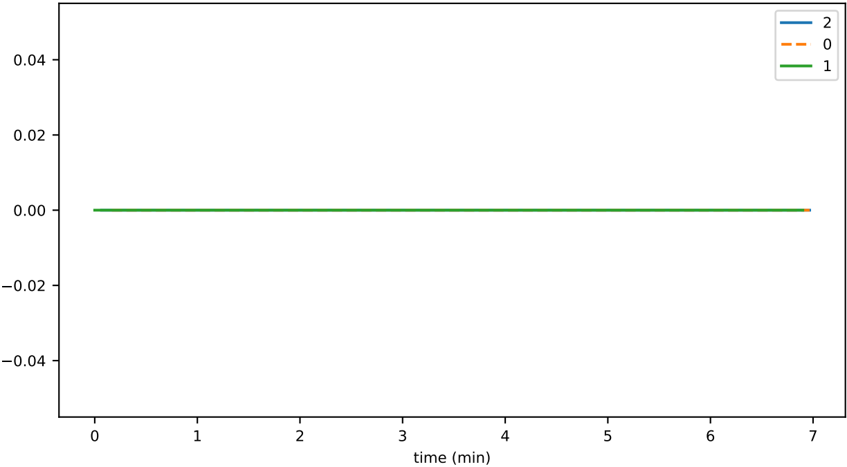
SmartContractService:Rejected_ethereumTxDueToIntrinsicGas_total
