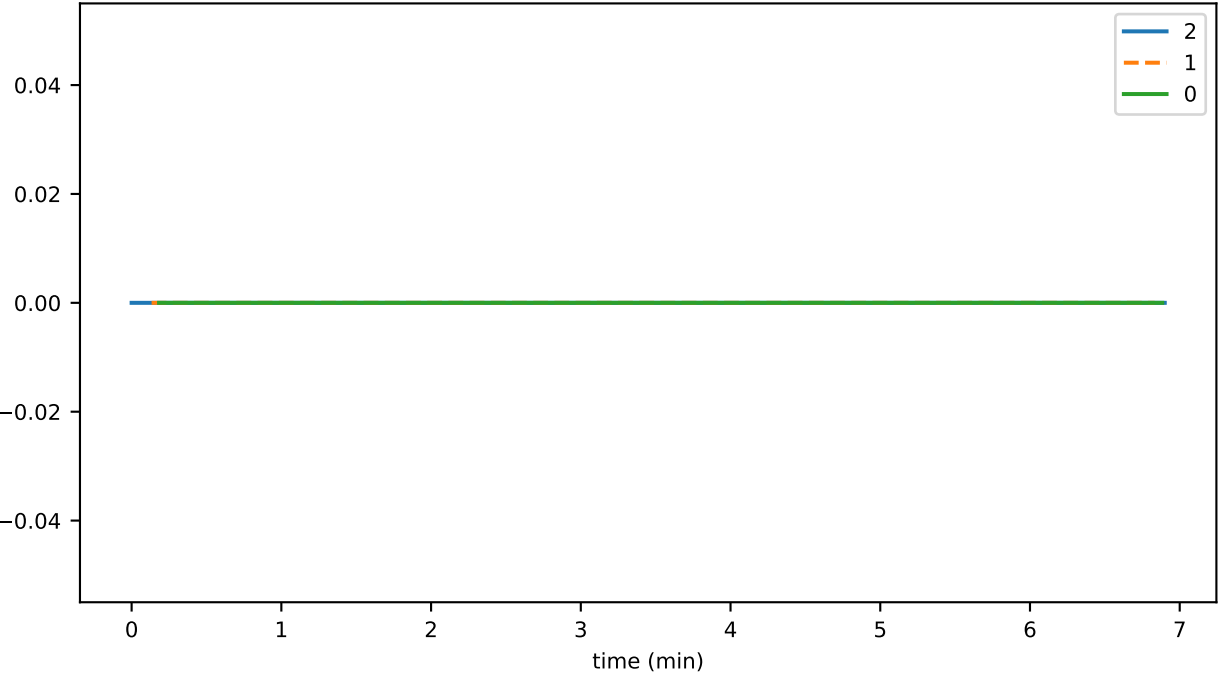
SmartContractService:SystemContractMethodCall_DIRECT_total
