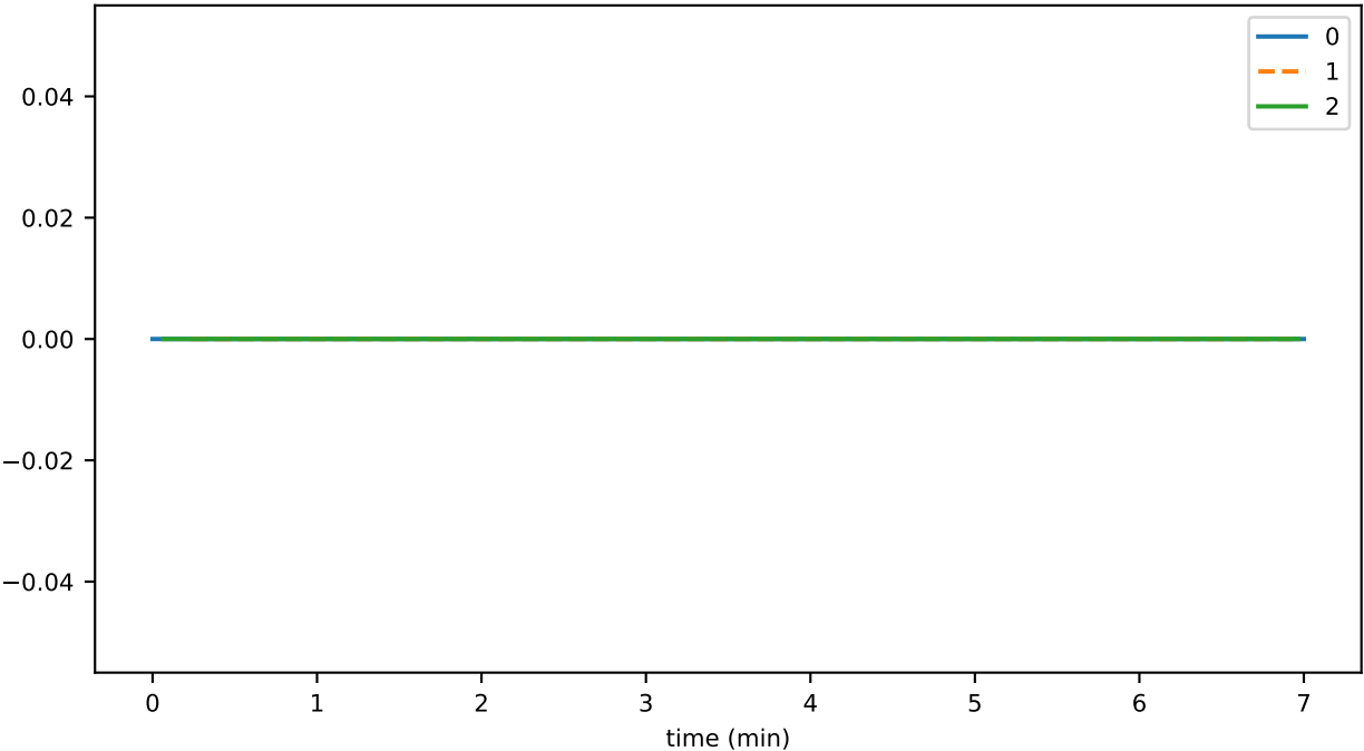
SmartContractService:SystemContractMethodCall_HTS_failed
