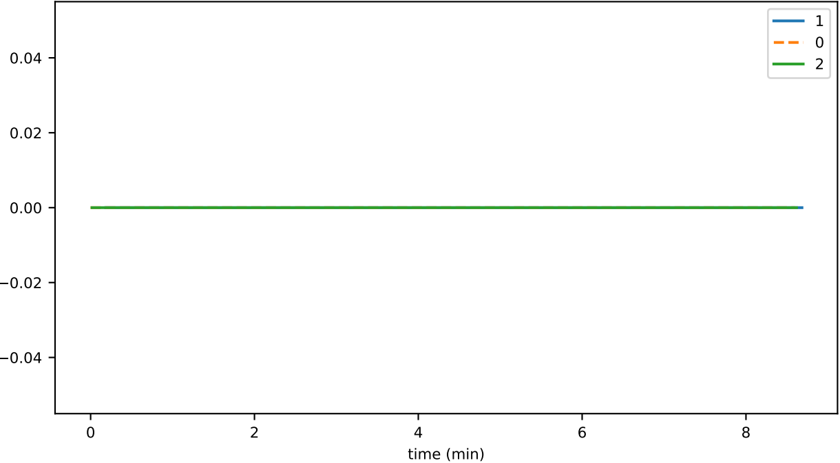
SmartContractService:SystemContractMethodCall_DIRECT_total
