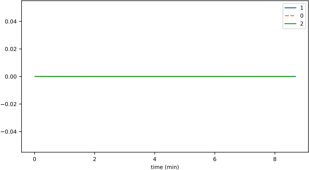
SmartContractService:SystemContractMethodCall_DIRECT_failed
