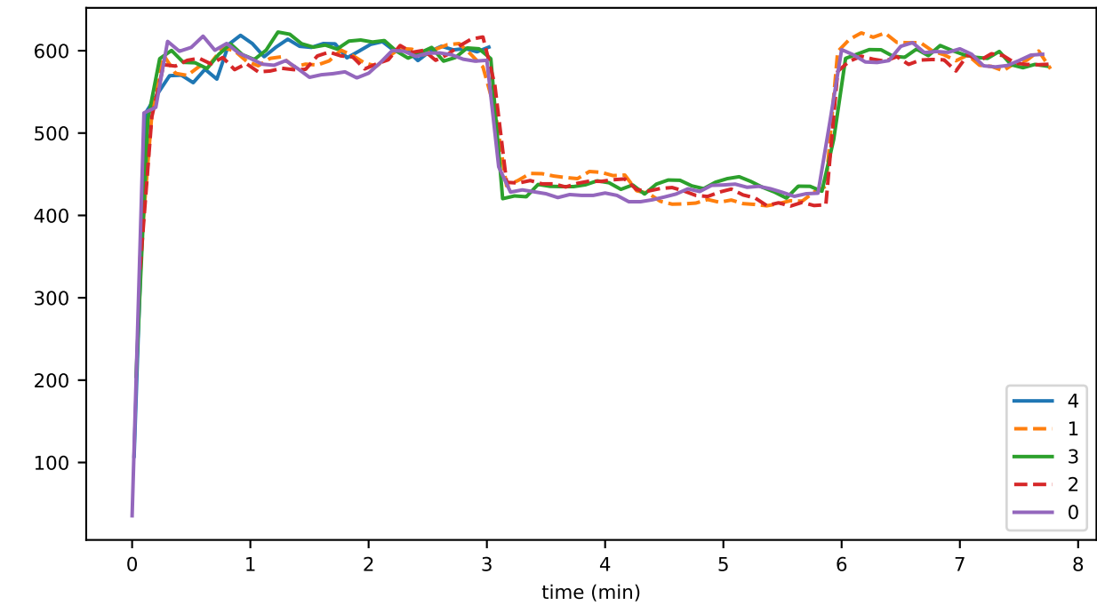
ds_compactions_level_0_hashesTimeMs_state
