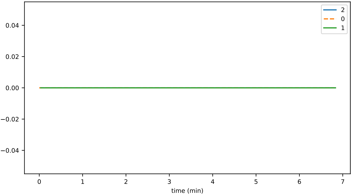
SmartContractService:SuccessfulTransactionDuration_count
