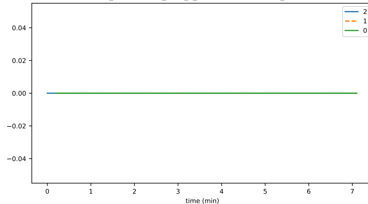
ds_compactions_level_1_hashesSavedSpaceMb_state
