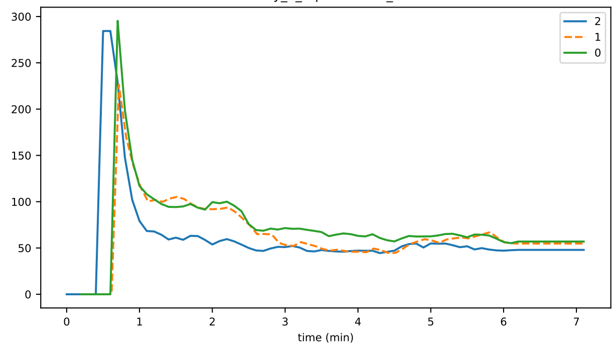
eventDelay_5_orphanBuffer_runtime
