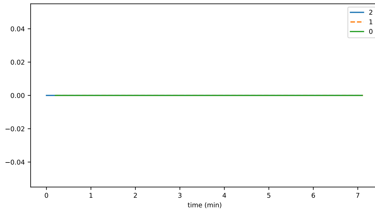
startsReconnectAsReceiver
