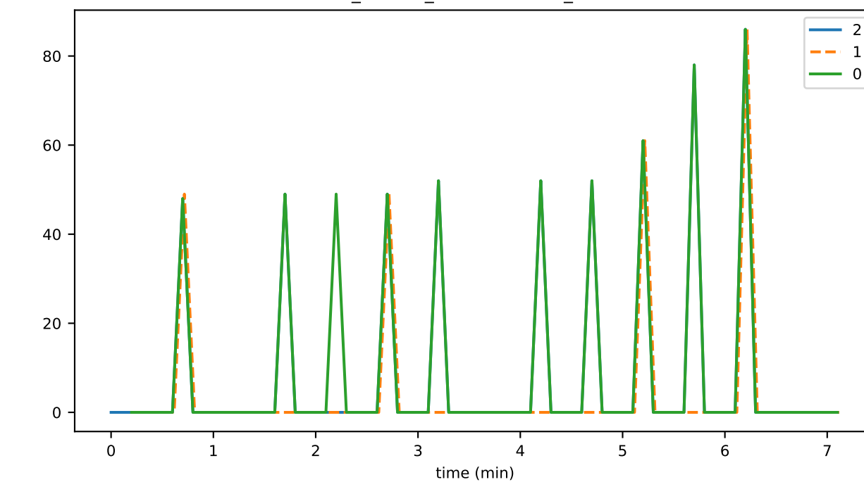
ds_flushes_hashesWritten_state
