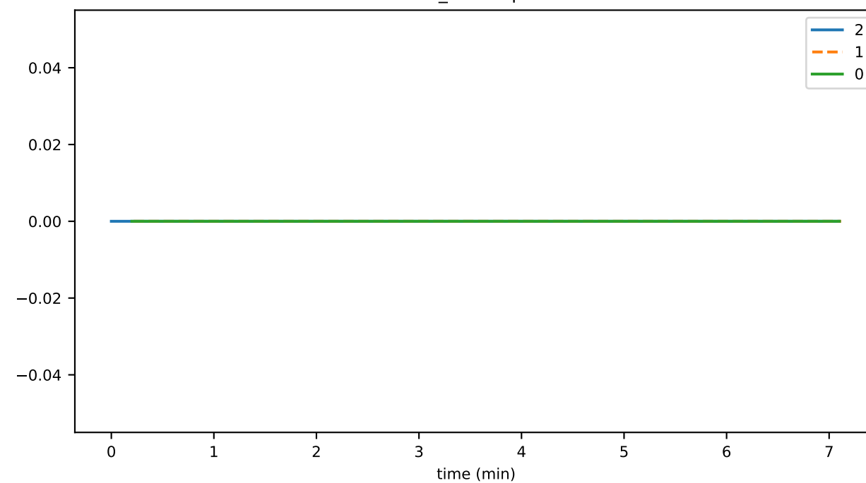
conn_onComplete
