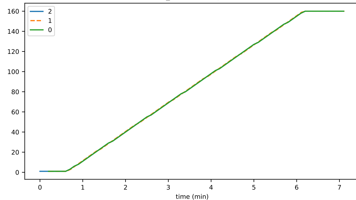
buffer_oldestBlock
