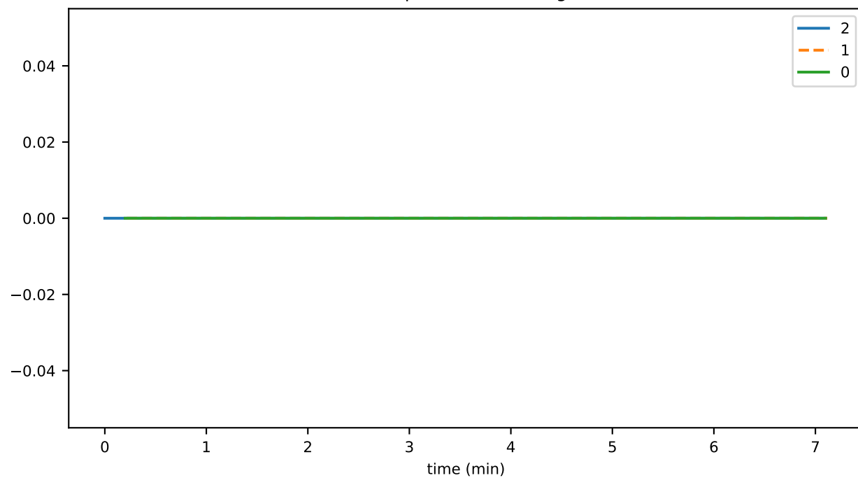
fileUpdateDurationAvg
