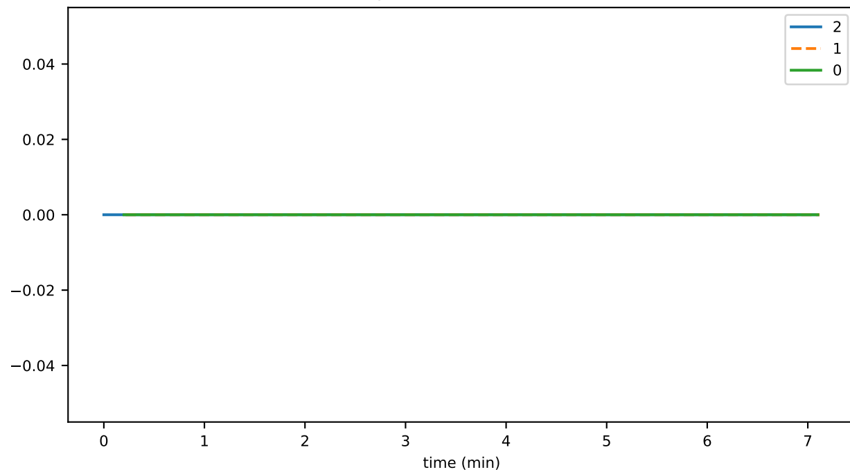
syncPermitsUtilized
