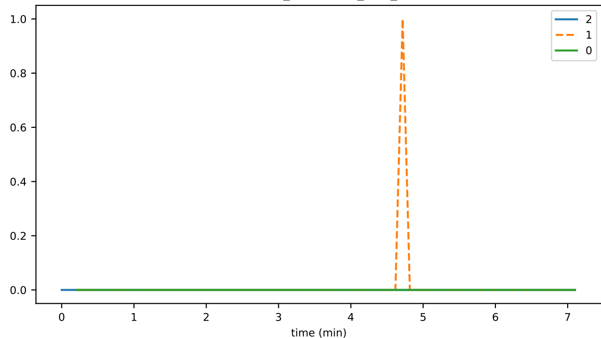
StateSignatureCollector_unhandled_task_count
