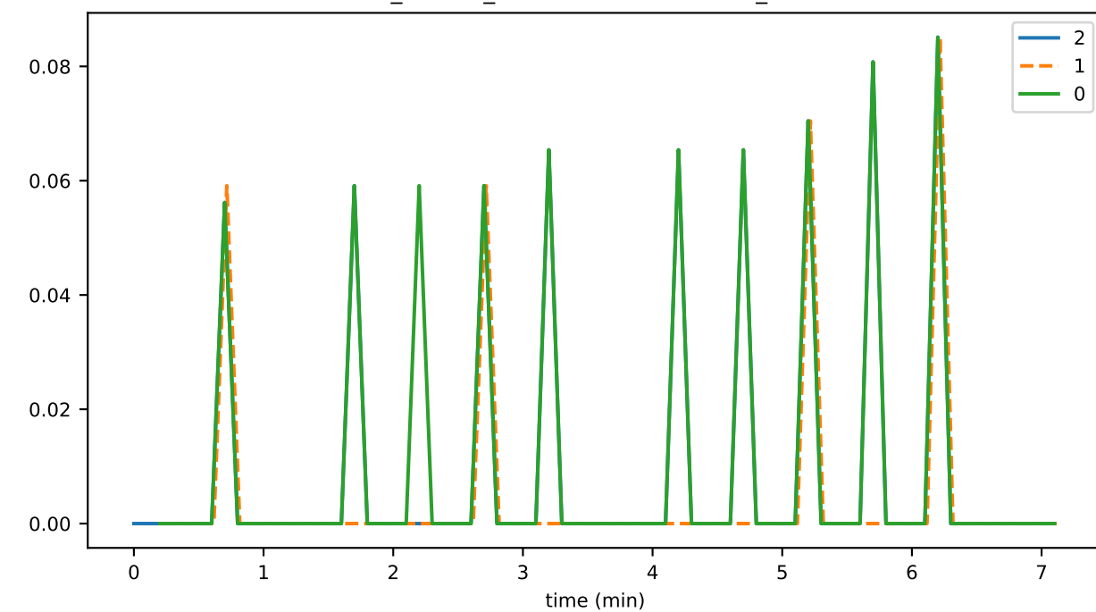
ds_flushes_hashesStoreFileSizeMb_state
