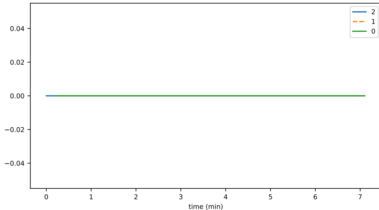
consensusGetTopicInfoDurationAvg
