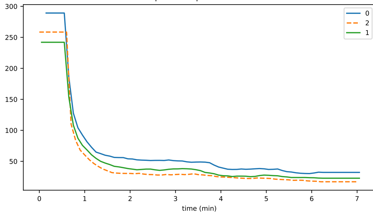
utilPngDurationMax
