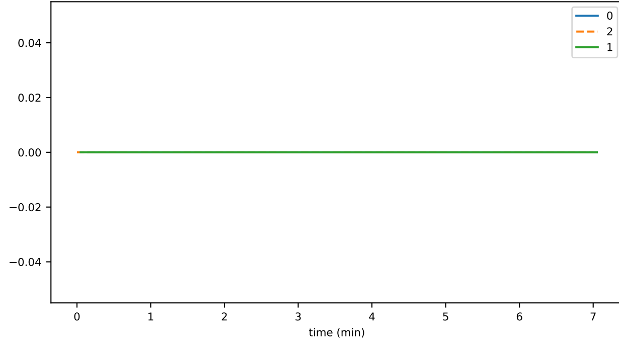
conn_endOfStreamLimitExceeded
