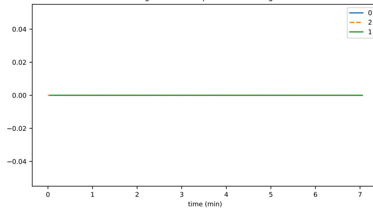
registeredNodeUpdateDurationAvg
