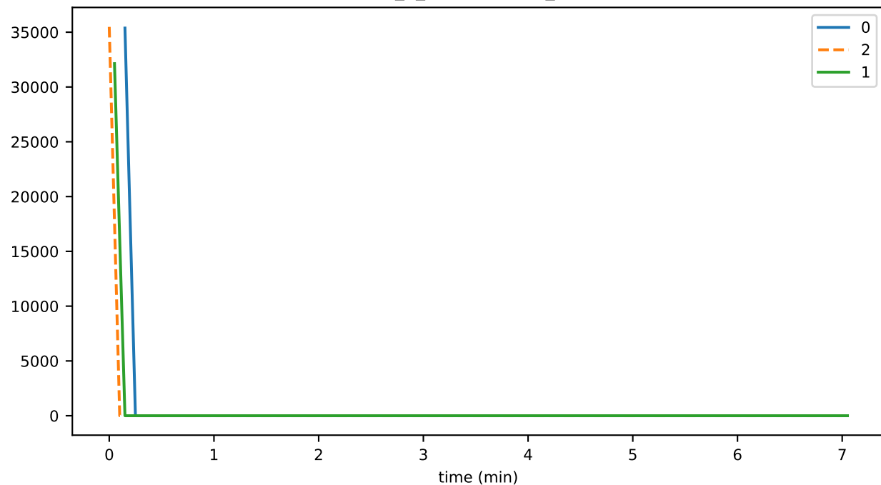
eventDelay_5_orphanBuffer_storageMAX
