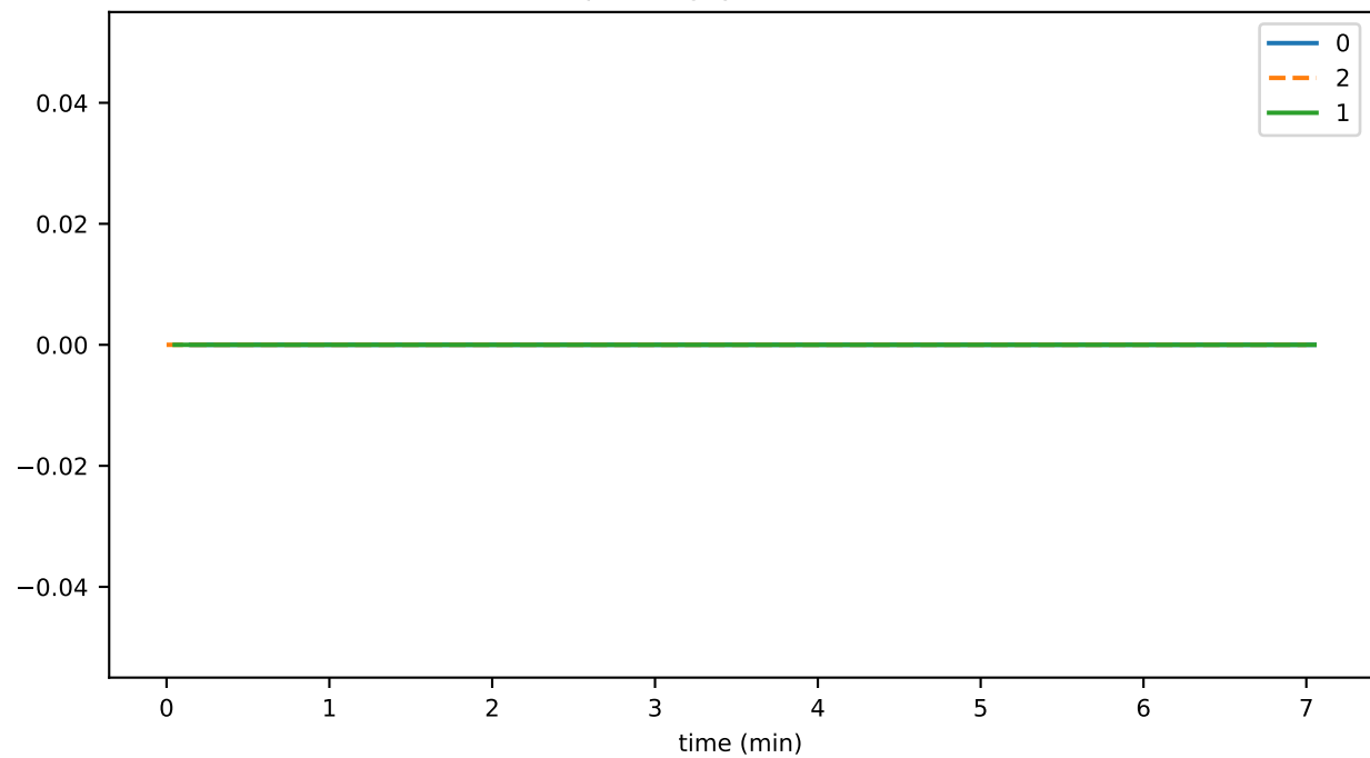
pcesAvgWriteDuration
