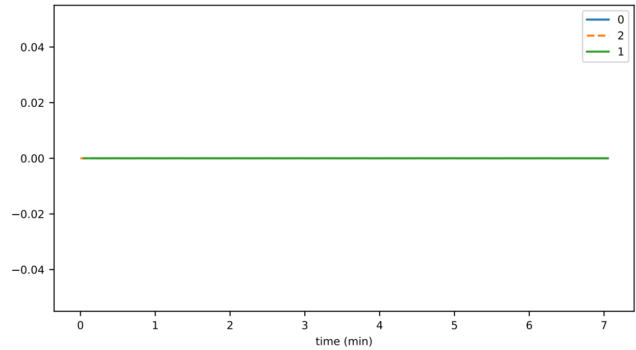
staleTransactions
