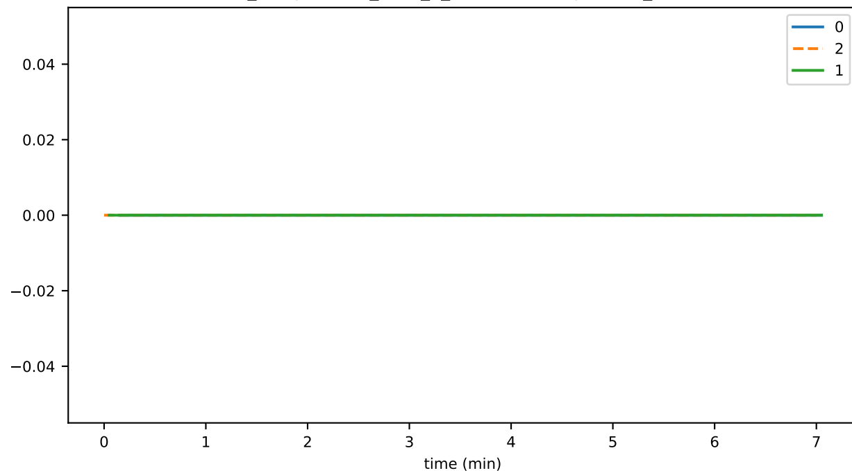
ds_compactions_level_2_hashesSavedSpaceMb_state
