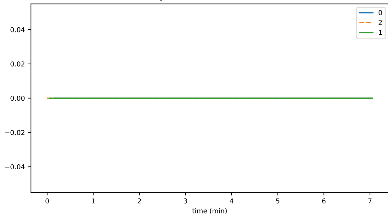
stateSignatureTransactionDurationMax
