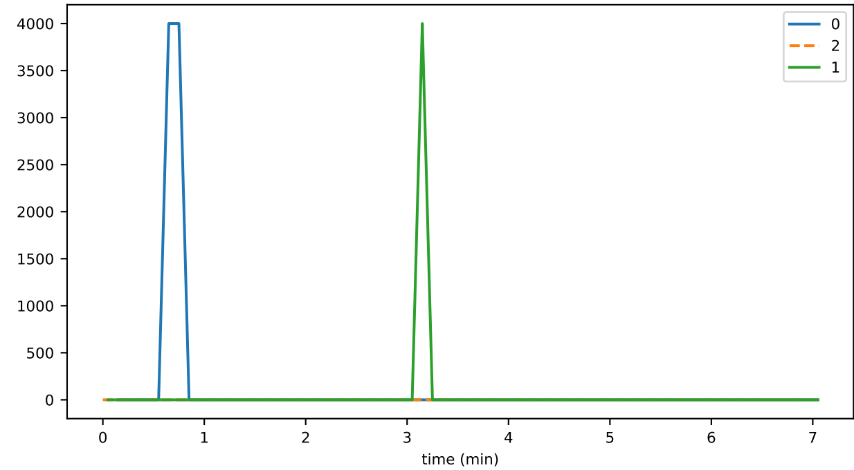
transH_per_sec
