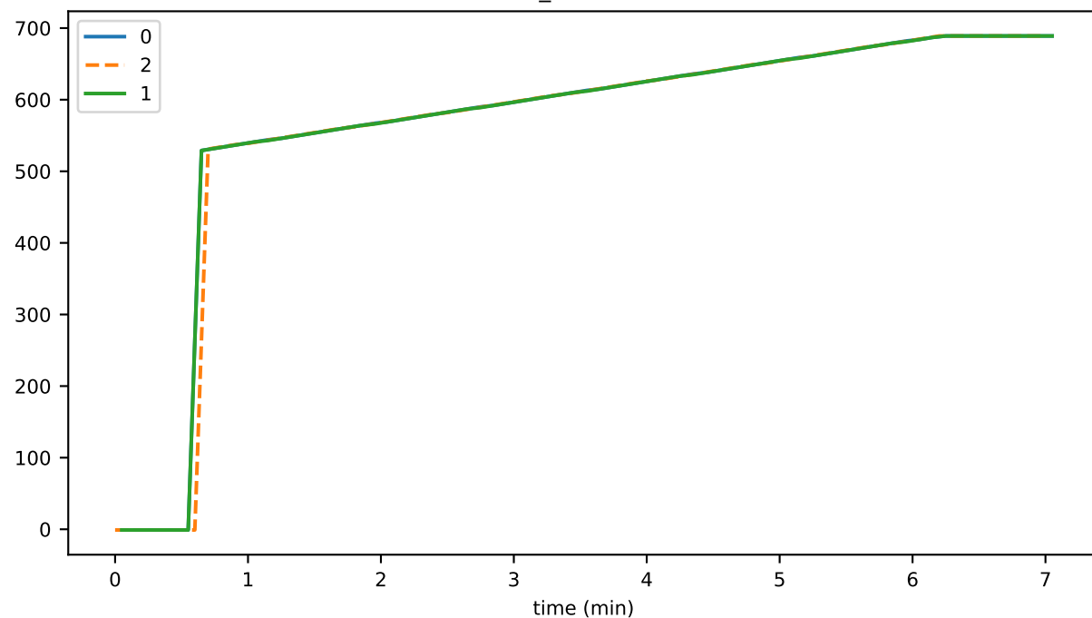
buffer_newestBlock
