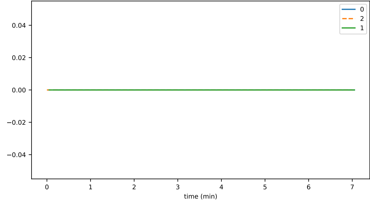
cryptoGetAccountBalanceDurationAvg
