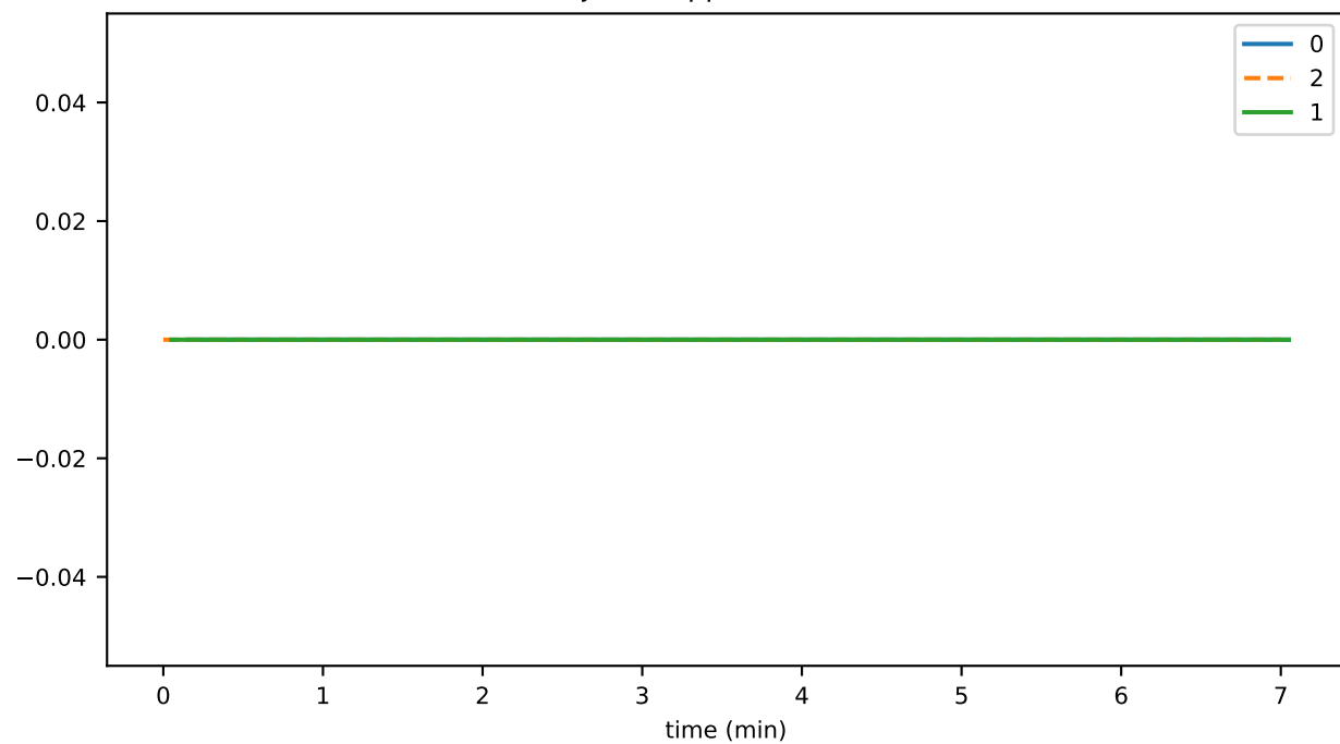
rejectedAppTransactions
