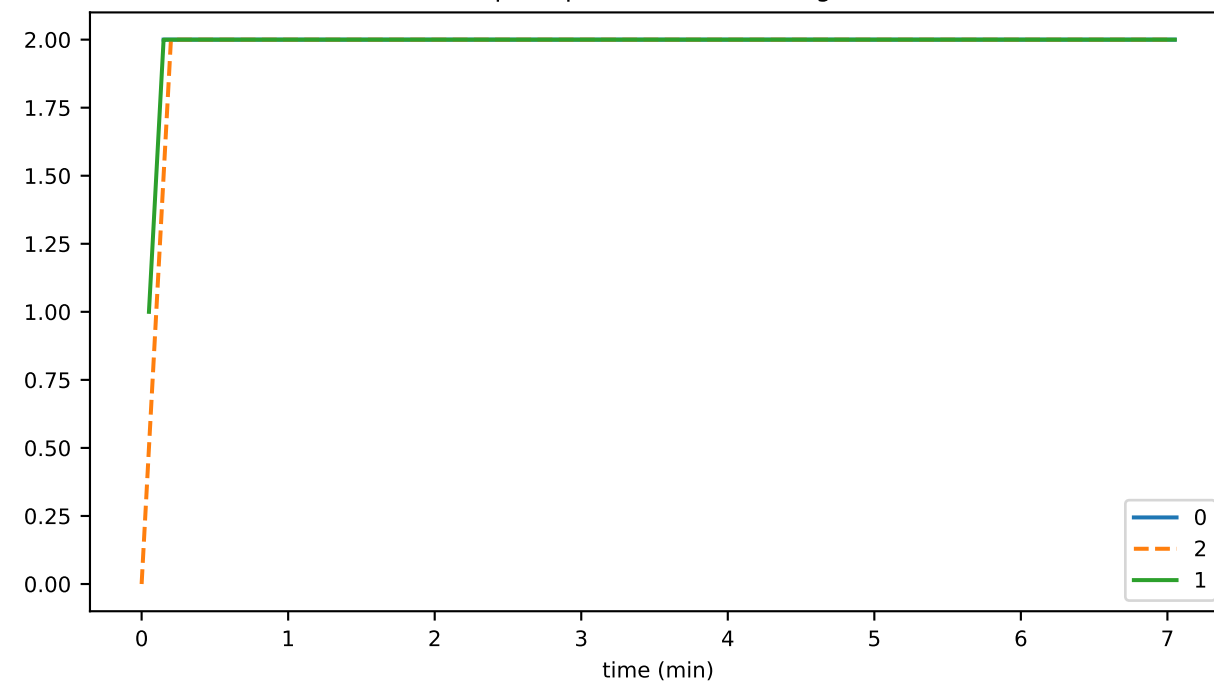
rpcDispatchThreadRunning
