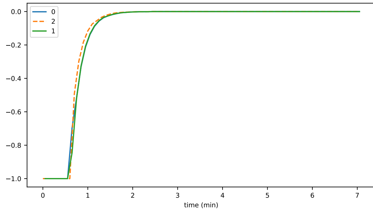
stateSignatureAge
