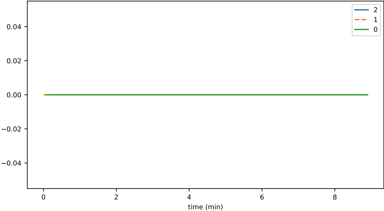
SmartContractService:SystemContractMethodCall_ERC721_failed
