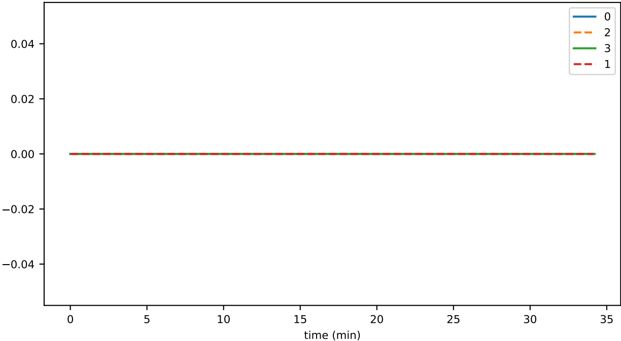
SmartContractService:IgnoredCodeDelegations_avg
