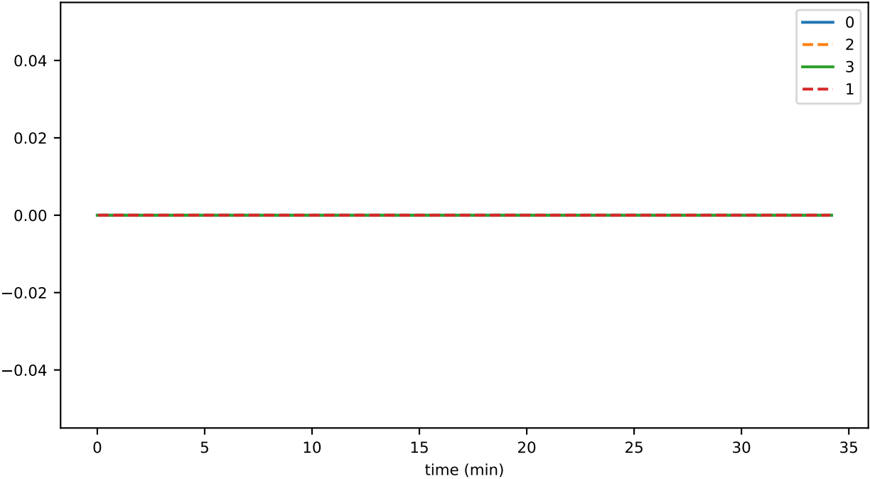
SmartContractService:FailedTransactionDuration_sum
