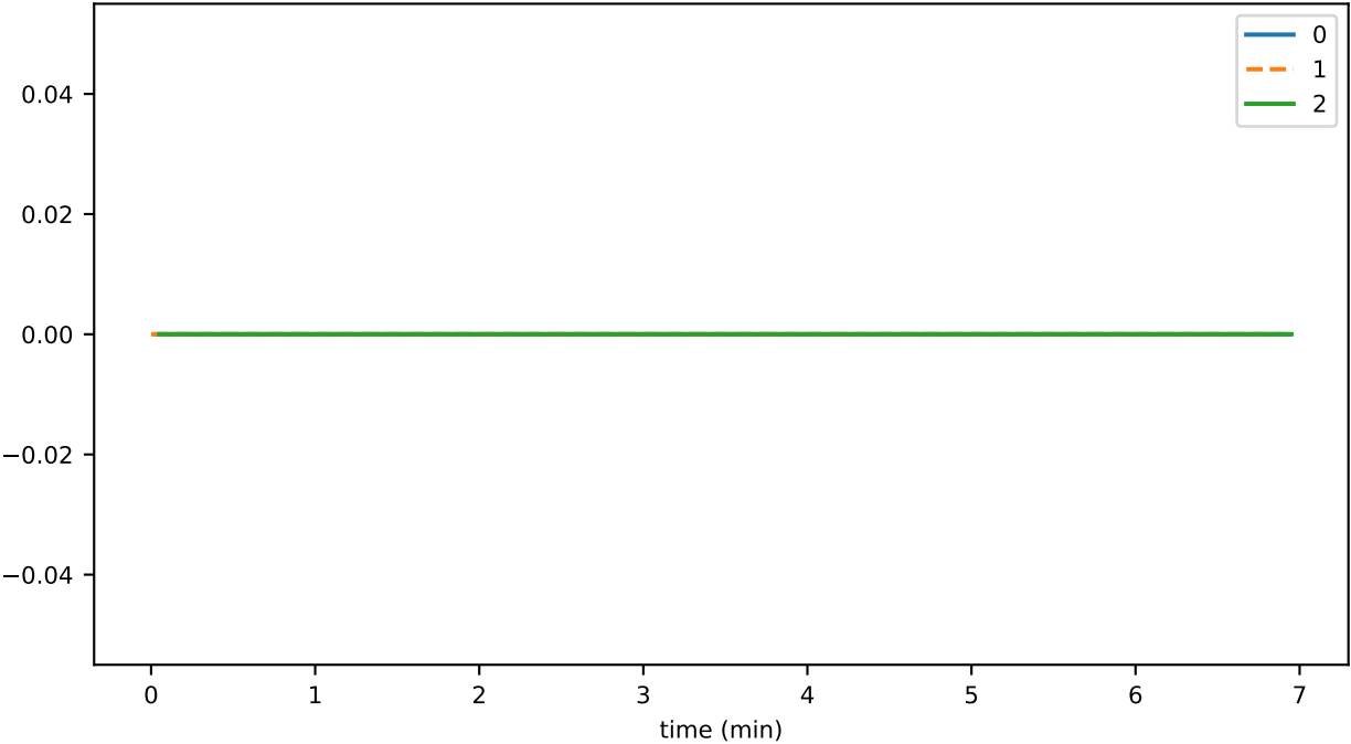
SmartContractService:SystemContractMethodCall_ALLOWANCE_failed
