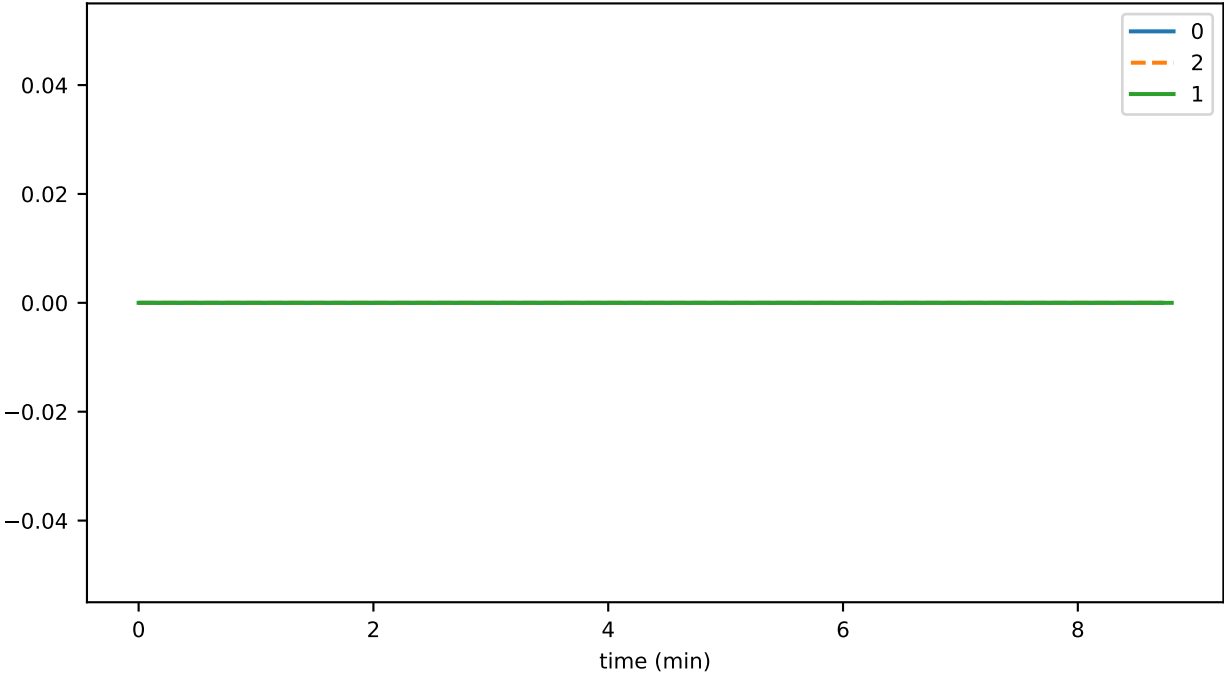
SmartContractService:SuccessfullyProcessedCodeDelegations_sum
