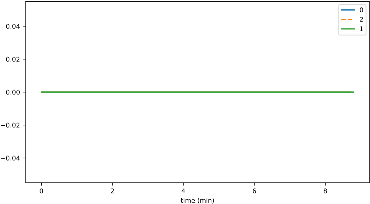
SmartContractService:SuccessfullyProcessedCodeDelegations_count
