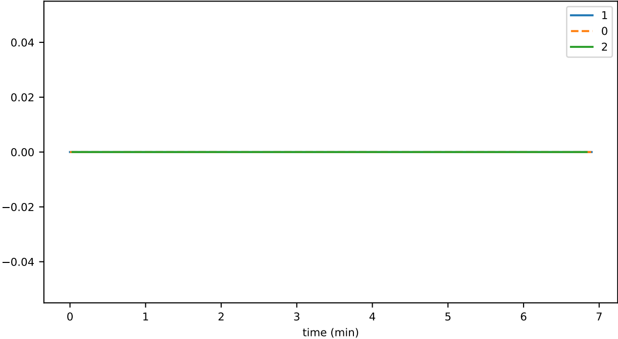
SmartContractService:SystemContractMethodCall_TRANSFER_failed
