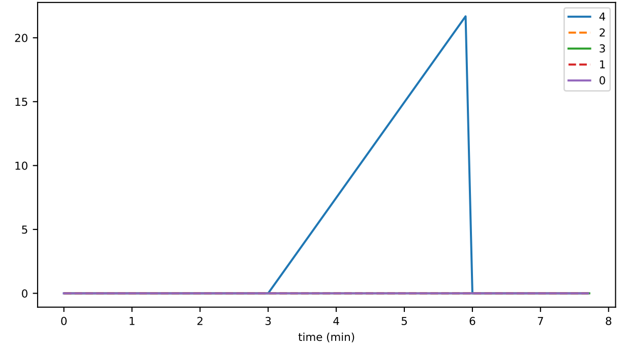
doNotSyncRemoteFallenBehind
