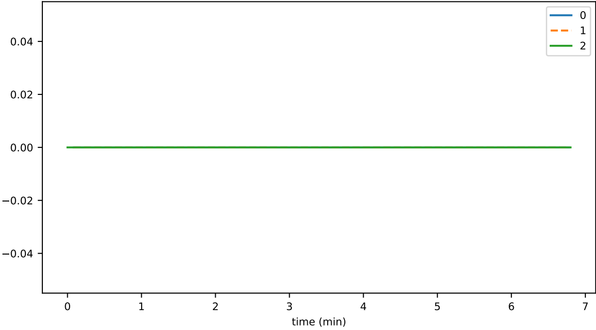
SmartContractService:SystemContractMethodCall_ALIASES_failed
