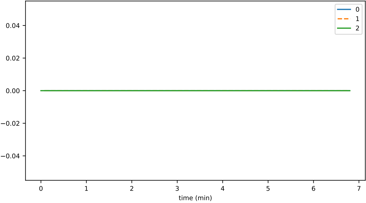
SmartContractService:SystemContractMethodCall_AIRDROP_total
