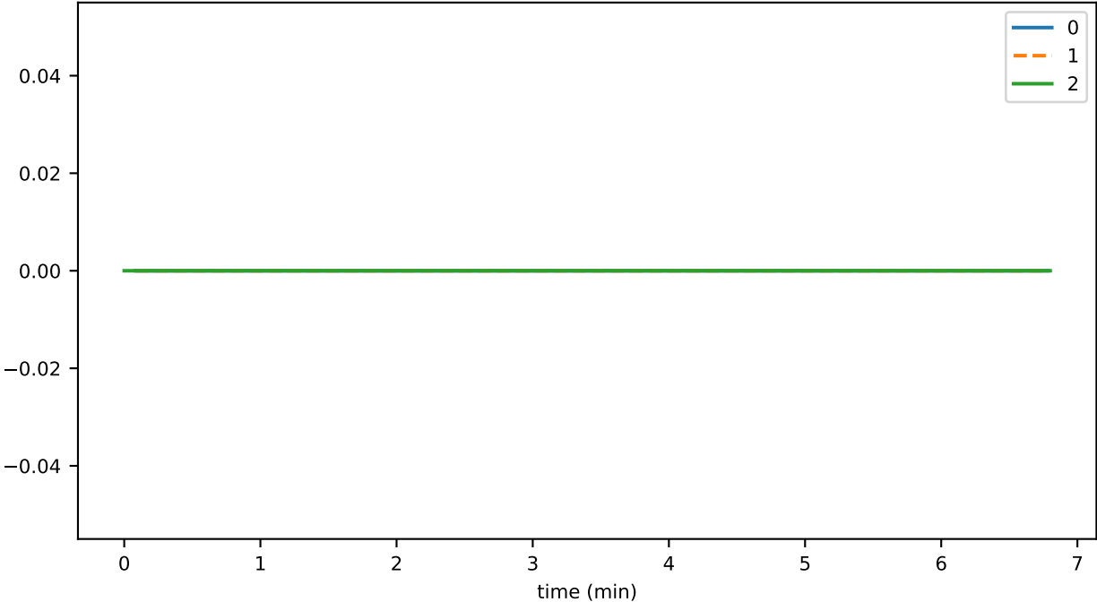
SmartContractService:SystemContractMethodCall_MINT_BURN_failed
