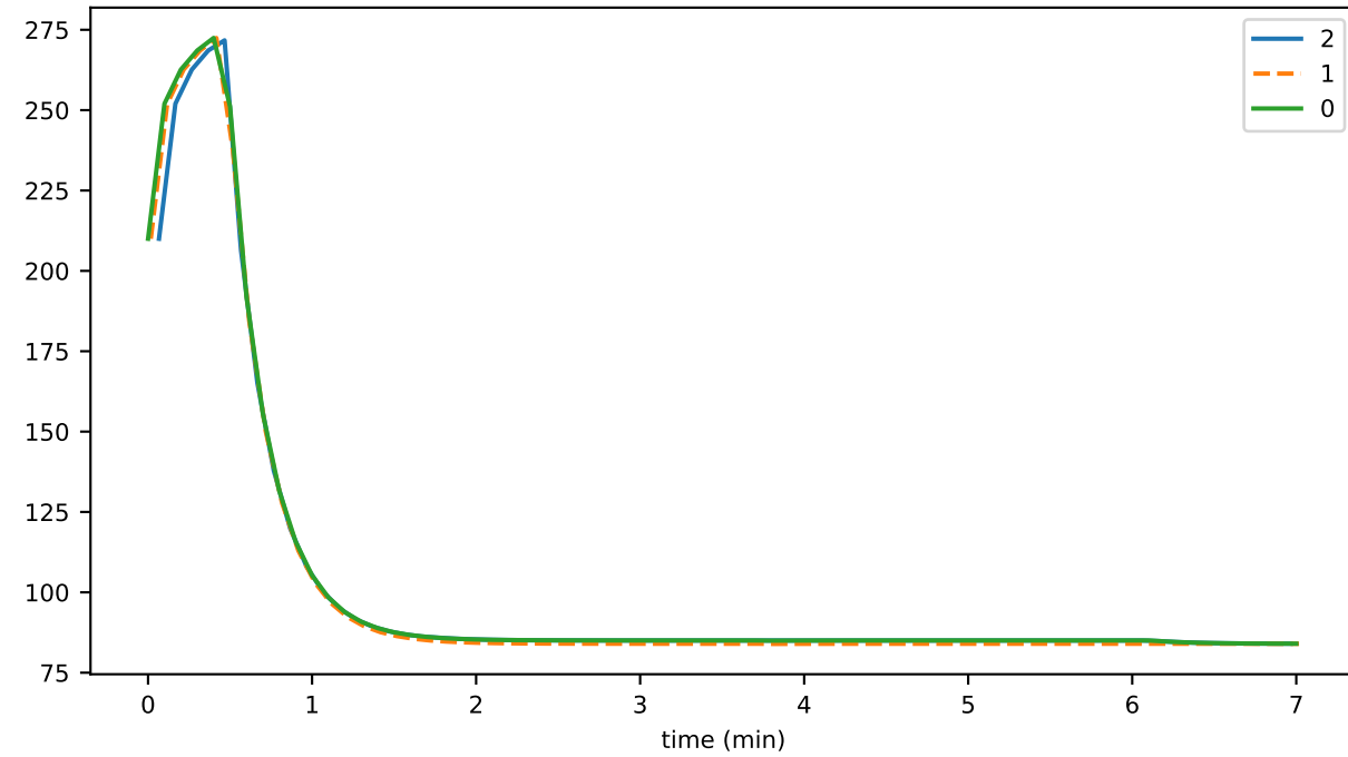
eventStreamQueueSize
