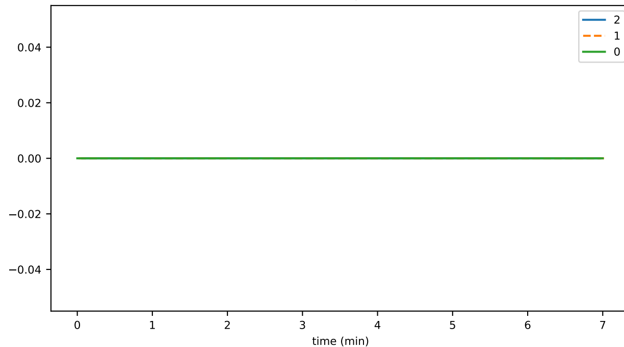
tokenClaimAirdropDurationAvg
