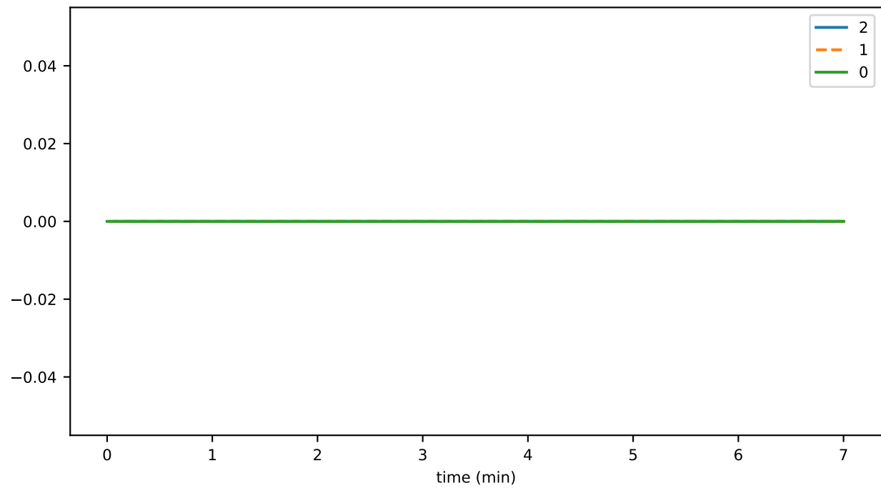
scheduleCreateDurationMax
