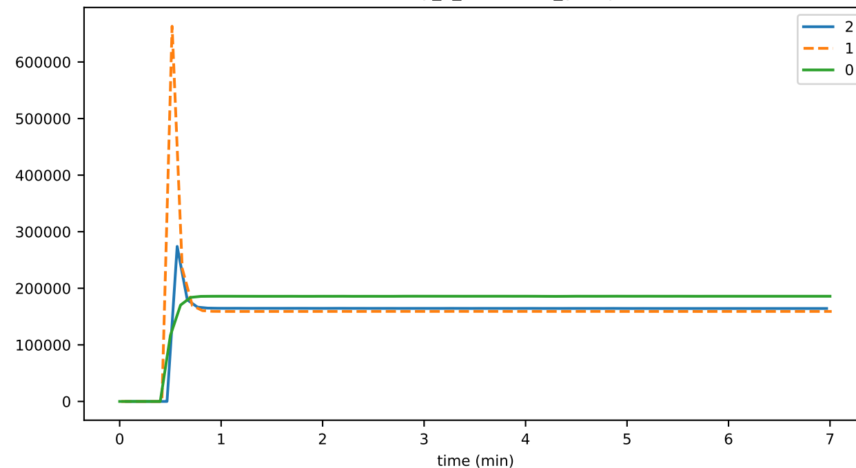
eventDelay_7_consensus_runtime
