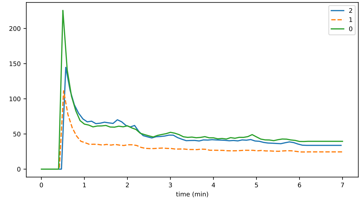
eventDelay_3_deduplication_runtime
