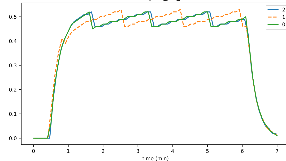
staleTransactions
