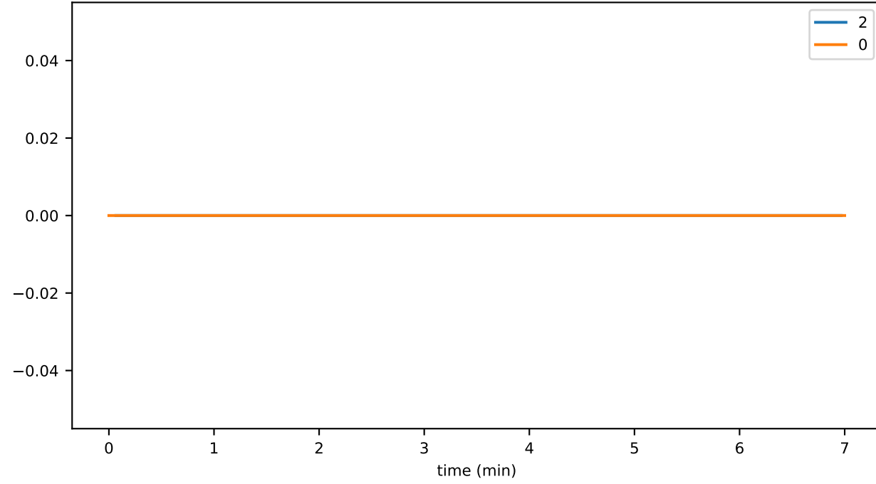
disconnects_per_sec_01
