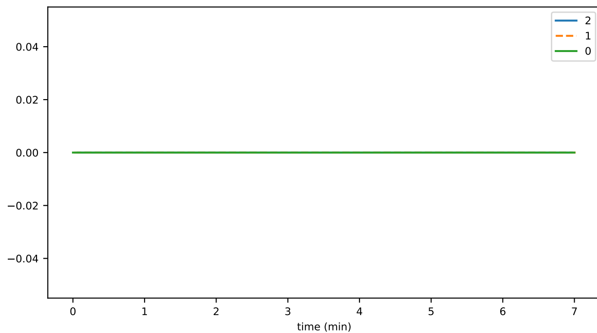
tokenDissociateFromAccountThrottledTxns
