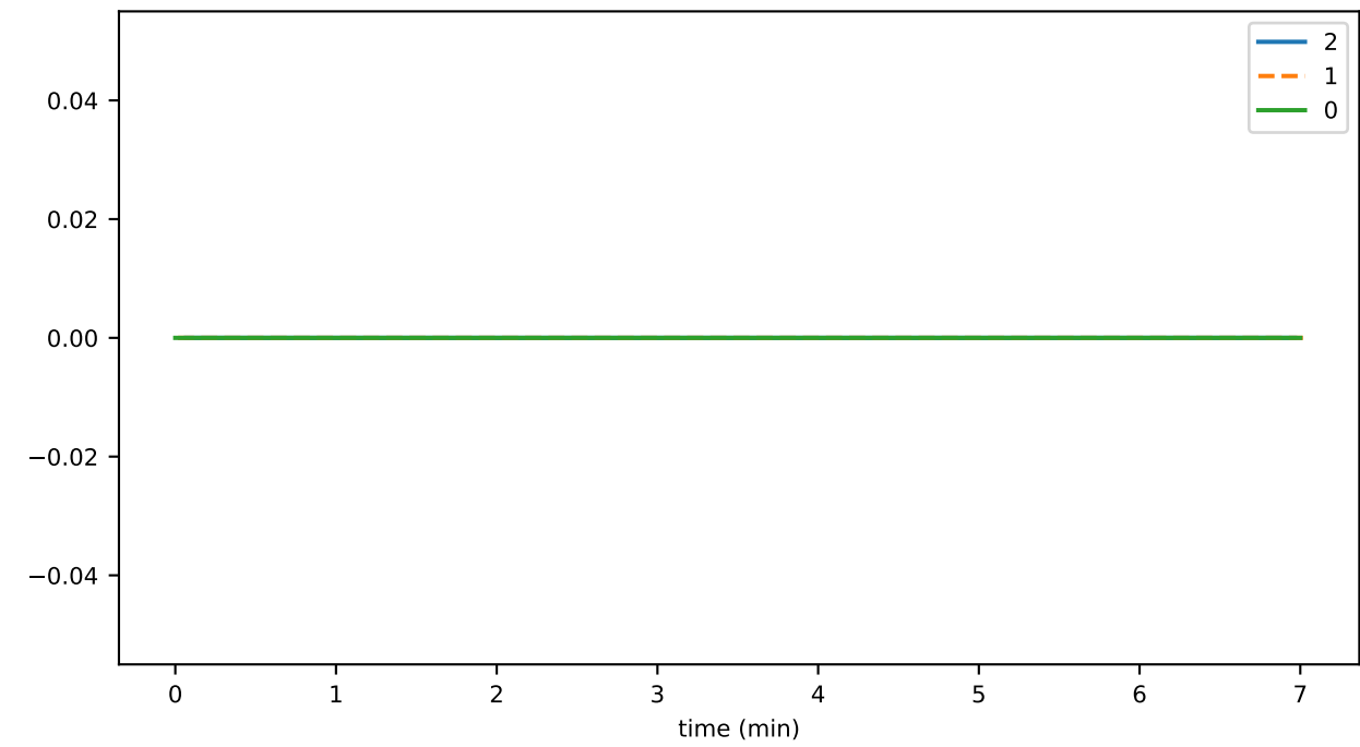
contractDeleteDurationAvg
