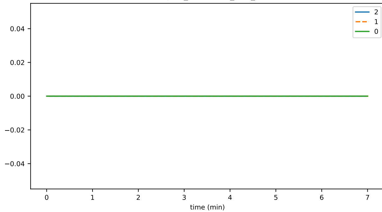
StateSnapshotManager_unhandled_task_count
