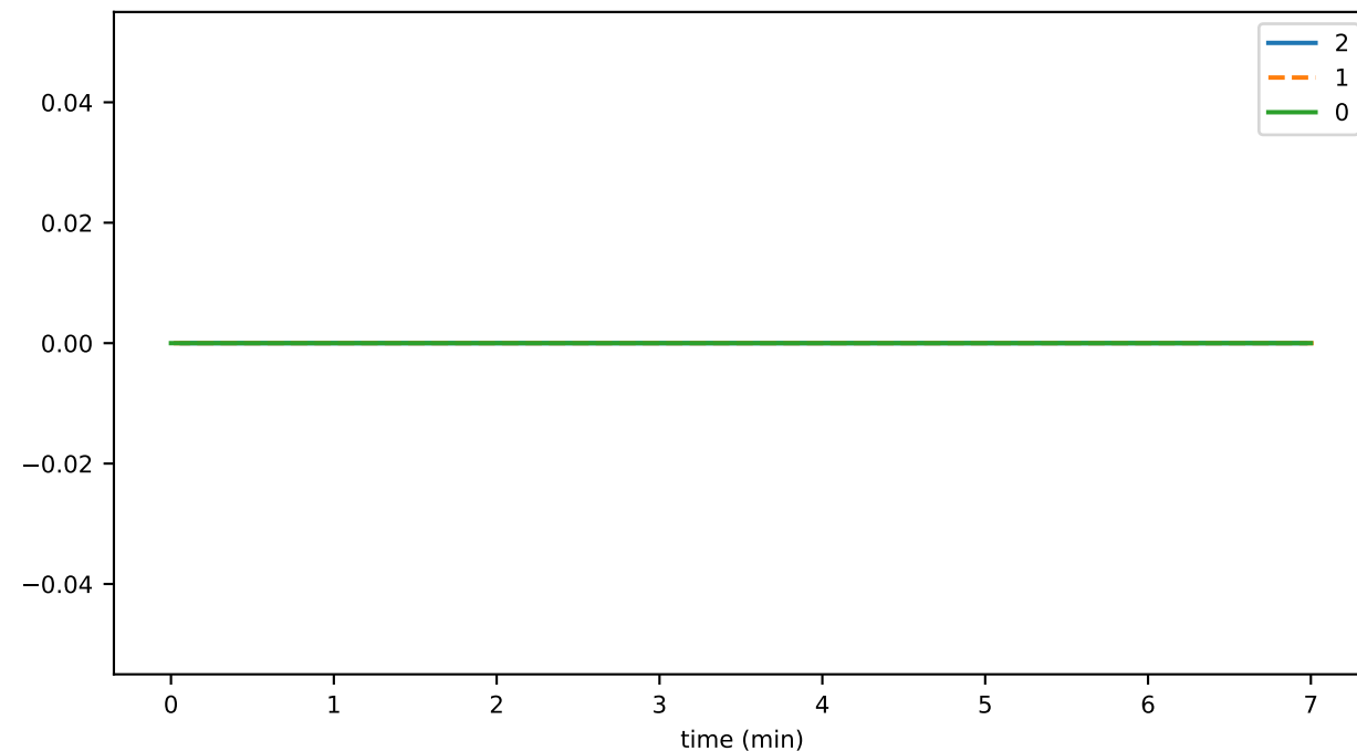
contractsMaxNumber
