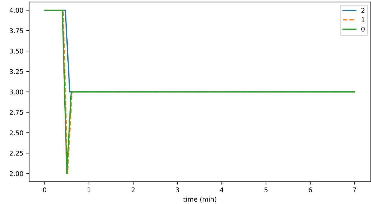
eventsWithDisparateSignature
