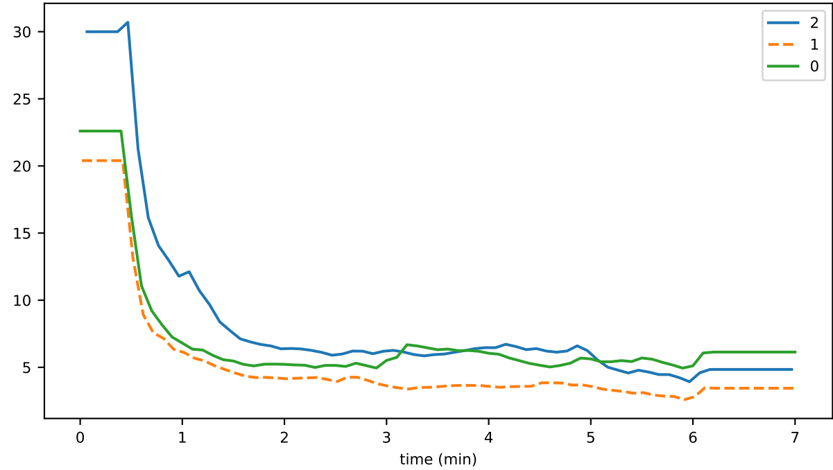
consensus_time_UPDATING_PLATFORM_STATE_RUNNING_HASH
