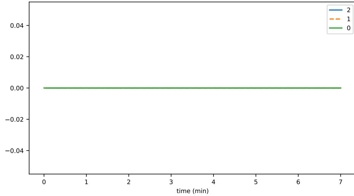
connRecv_acknowledgement
