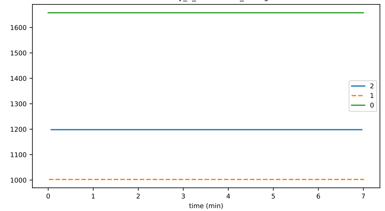
eventDelay_4_verification_storage
