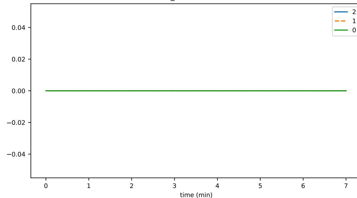
connSend_requestBlockItemCount
