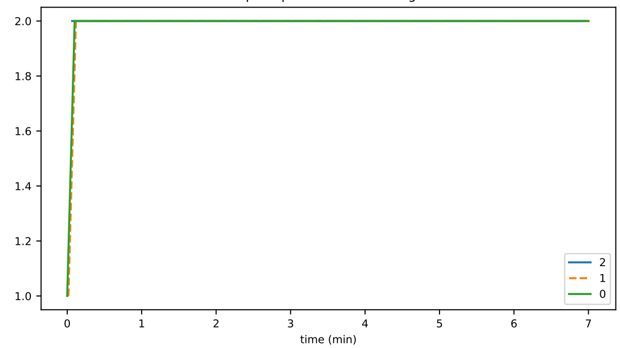
rpcDispatchThreadRunning
