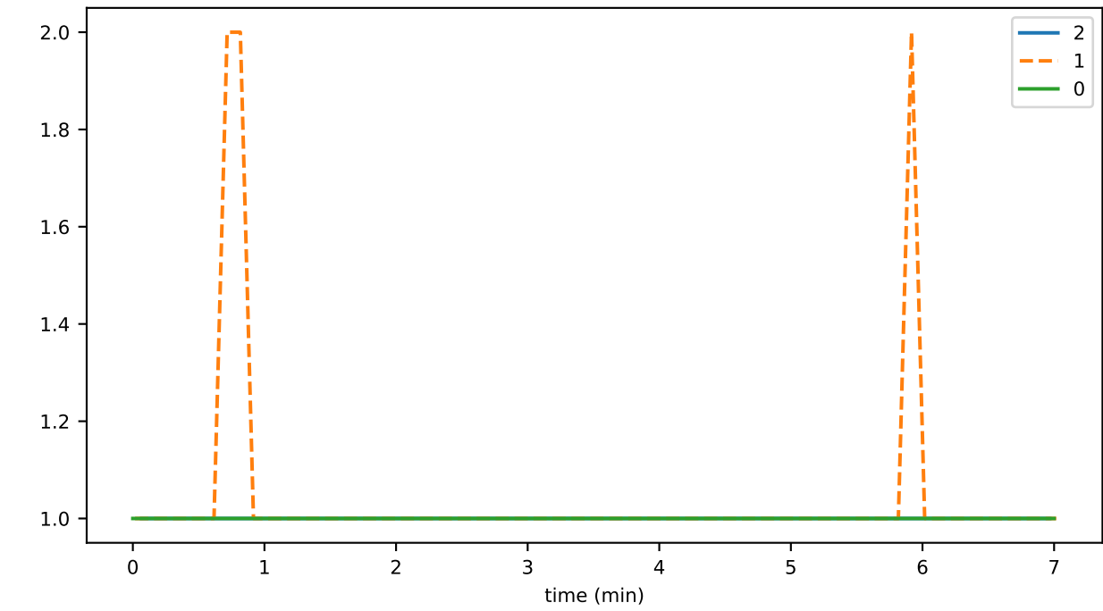
createTransactionRecordDurationAvg
