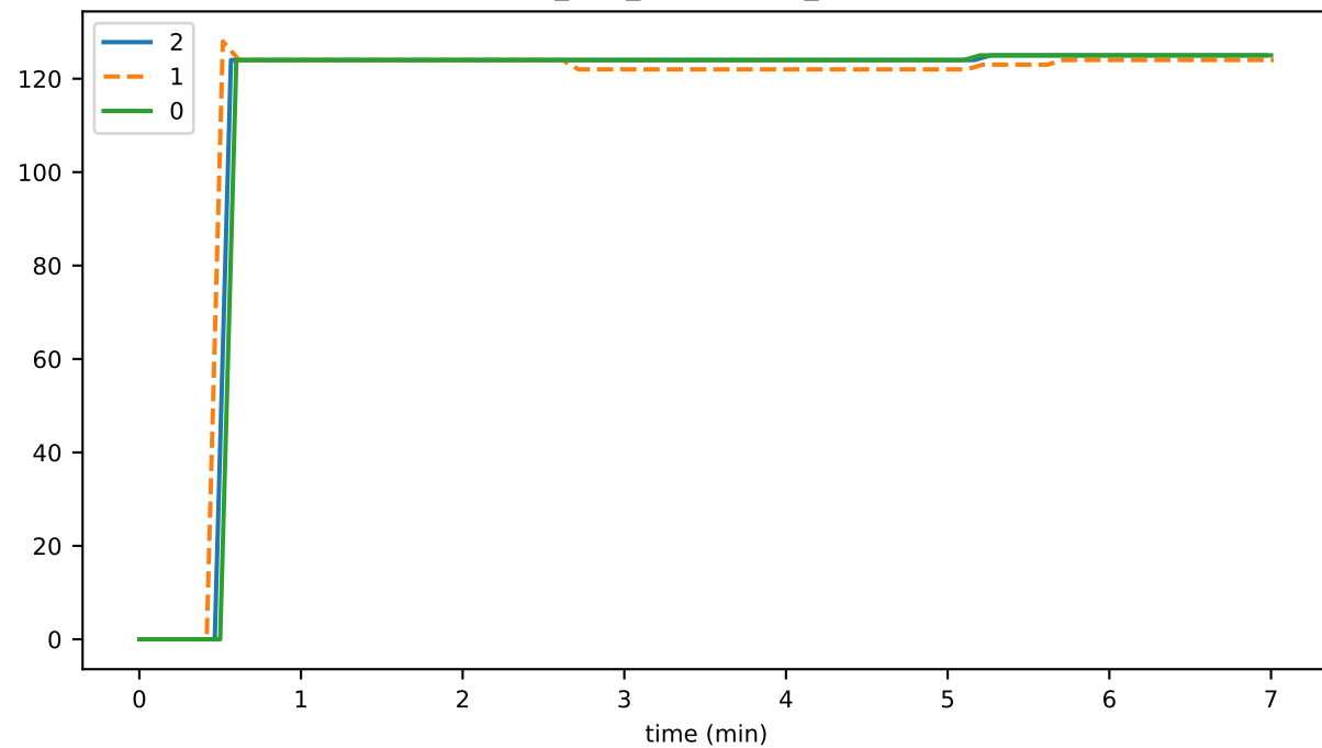
ds_files_totalSizeMb_state
