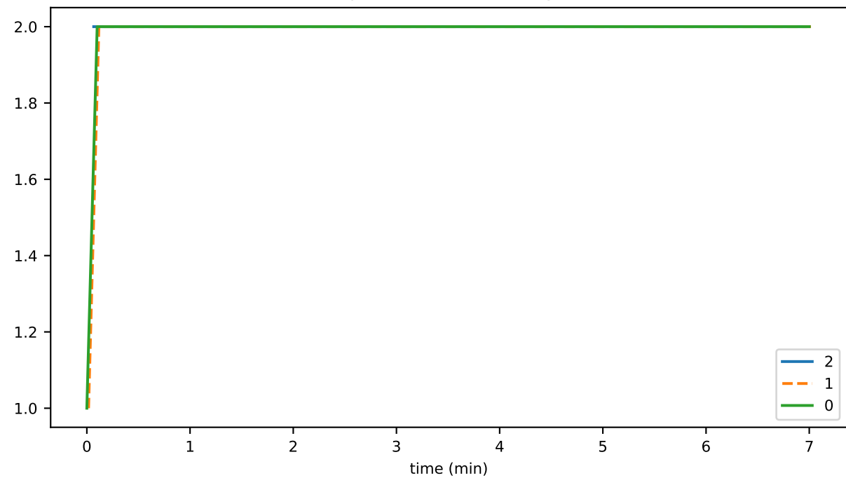
scheduleCreateDurationMax
