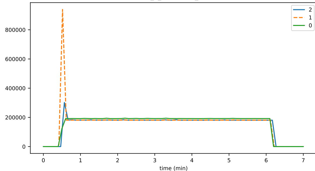
eventDelay_7_consensus_gossipMAX
