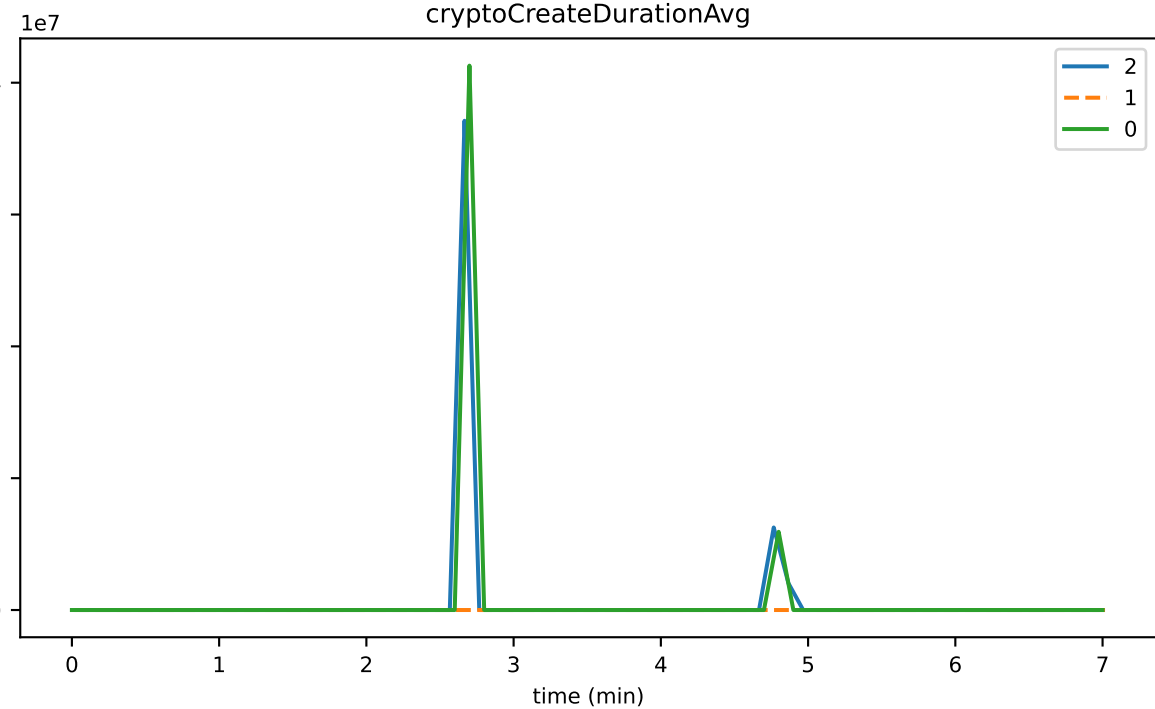
cryptoCreateDurationAvg
