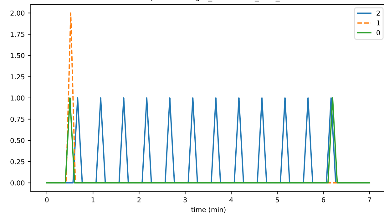
StateSnapshotManager_unhandled_task_count
