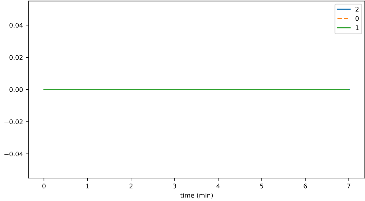
historyProofTransWMetaToFailCnt
