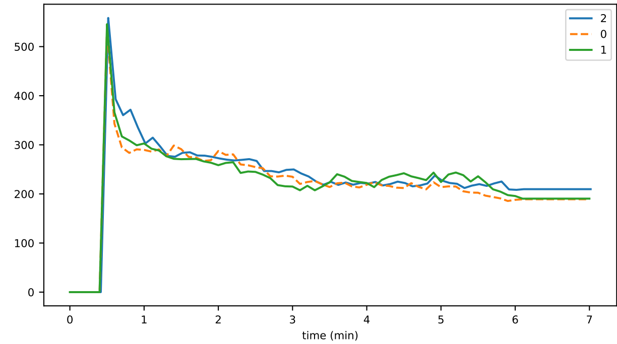
eventDelay_4_verification_gossip
