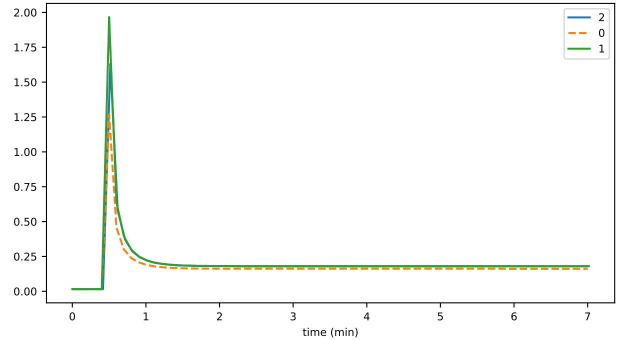
memFree
