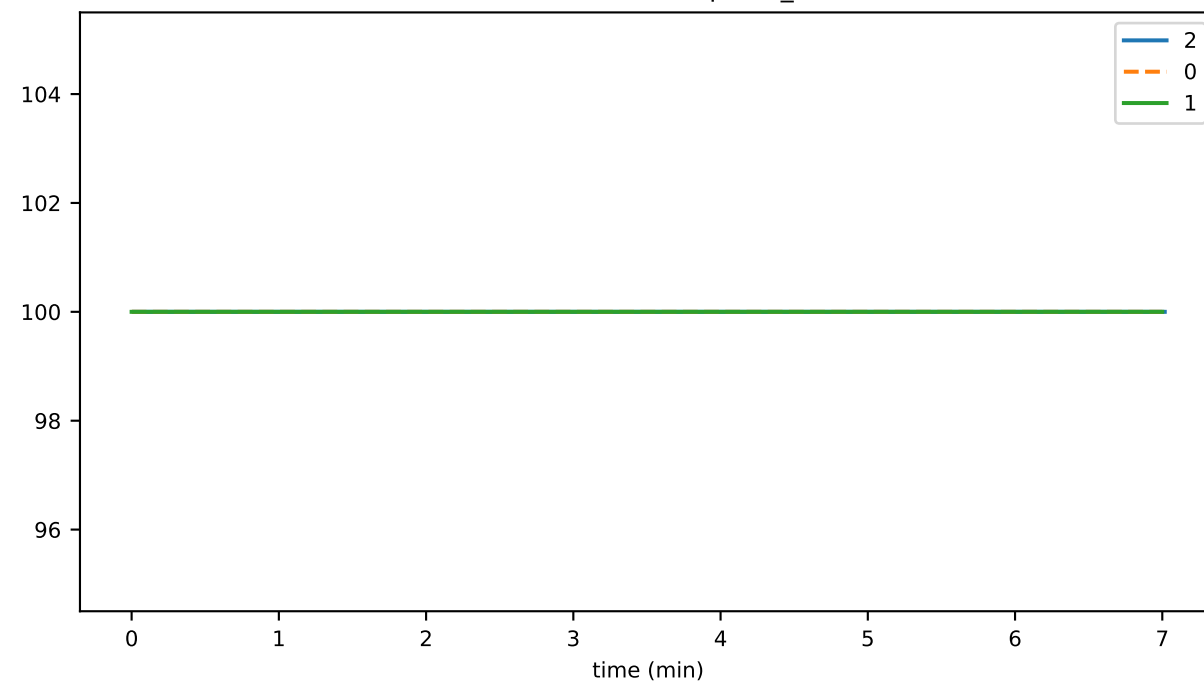
nodeActivePercentSnapshot_node0
