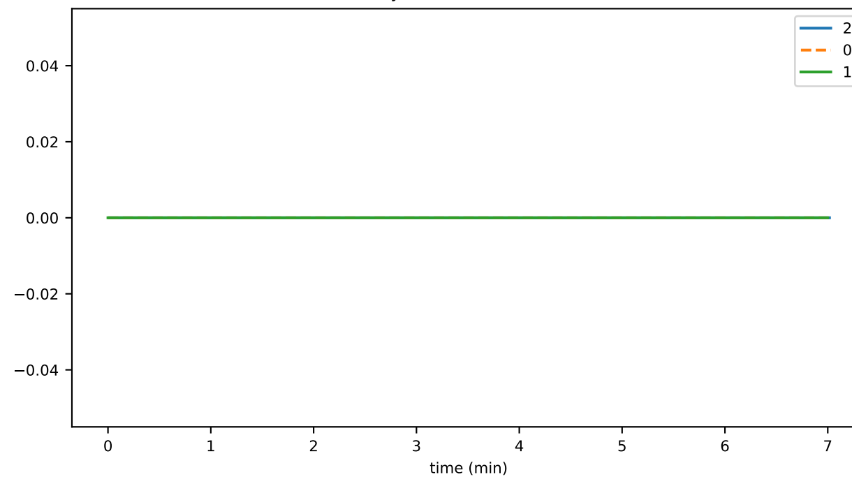
historyProofTransR2ToFailCnt
