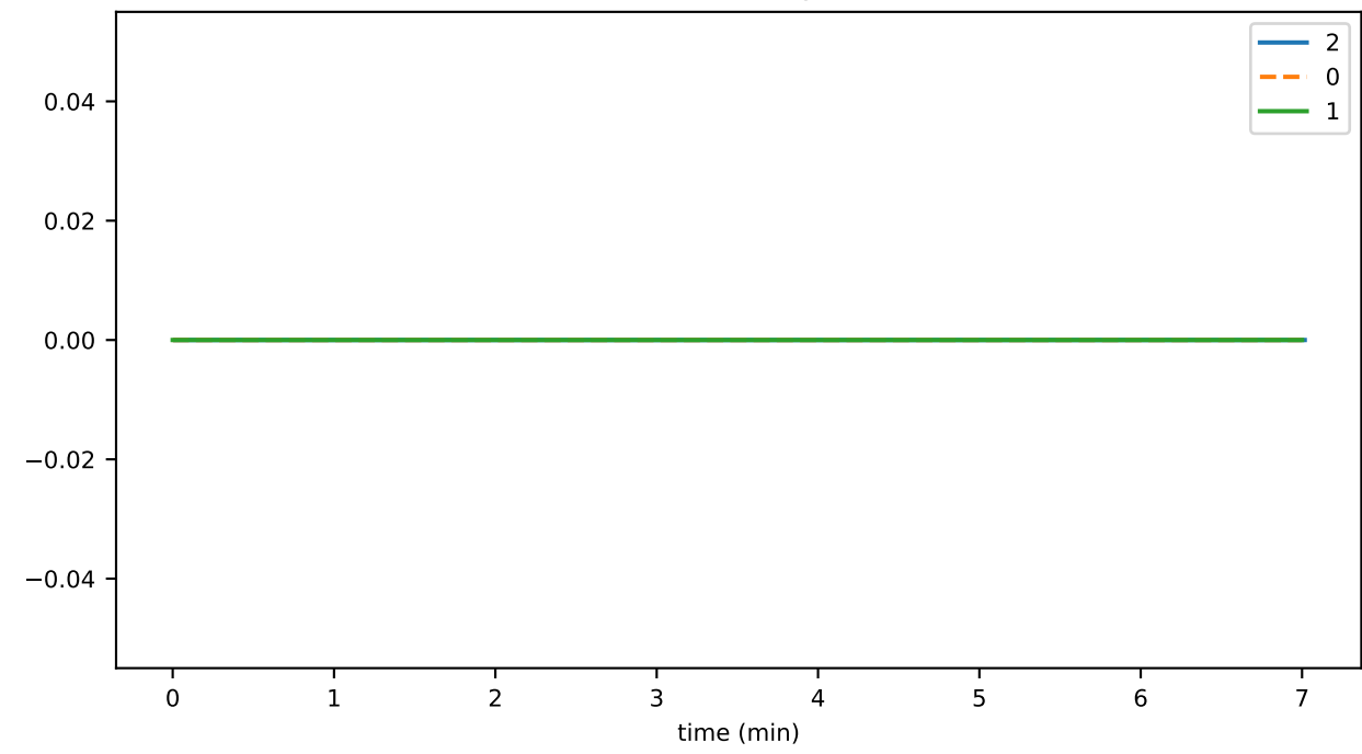
consensusTime
