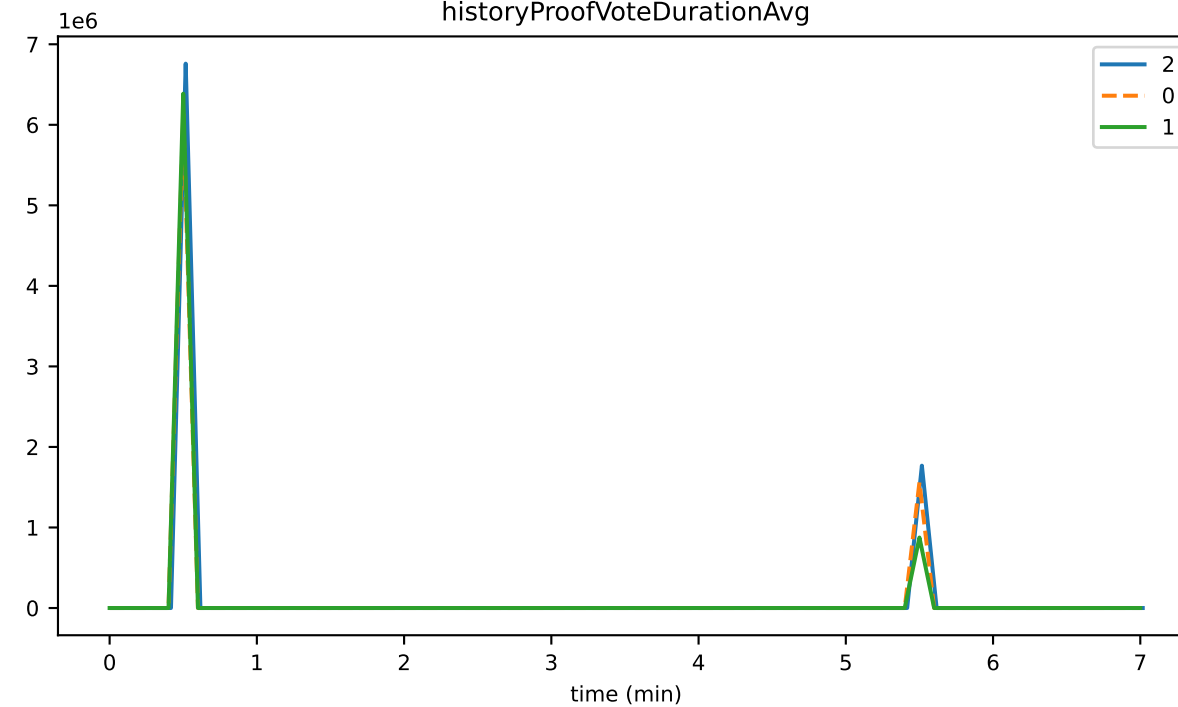
historyProofVoteDurationAvg
