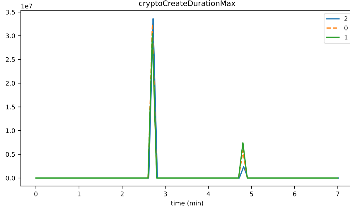
cryptoCreateDurationMax
