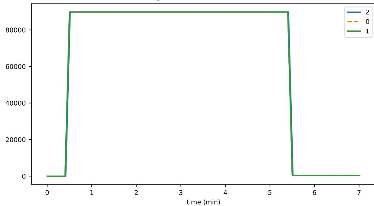
historyProofTransWMetaToWasmMs
