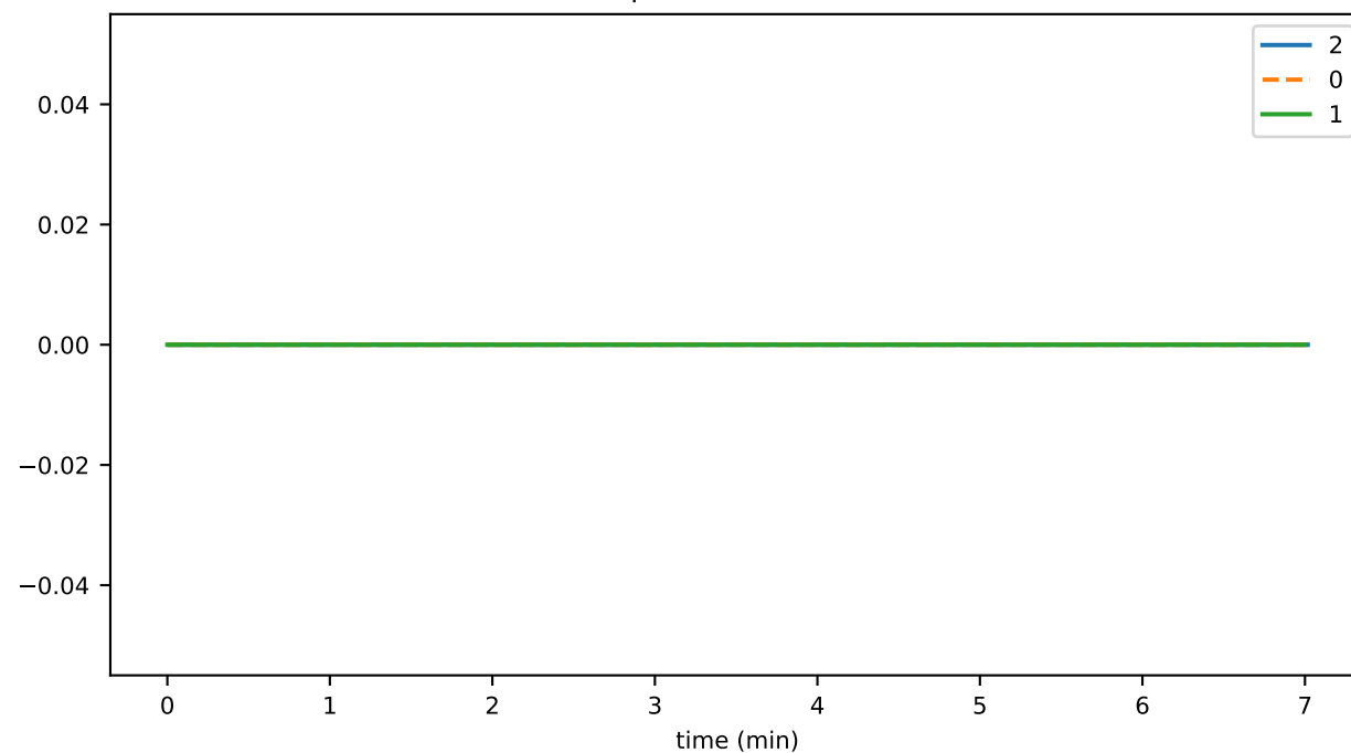
freezeDurationMax
