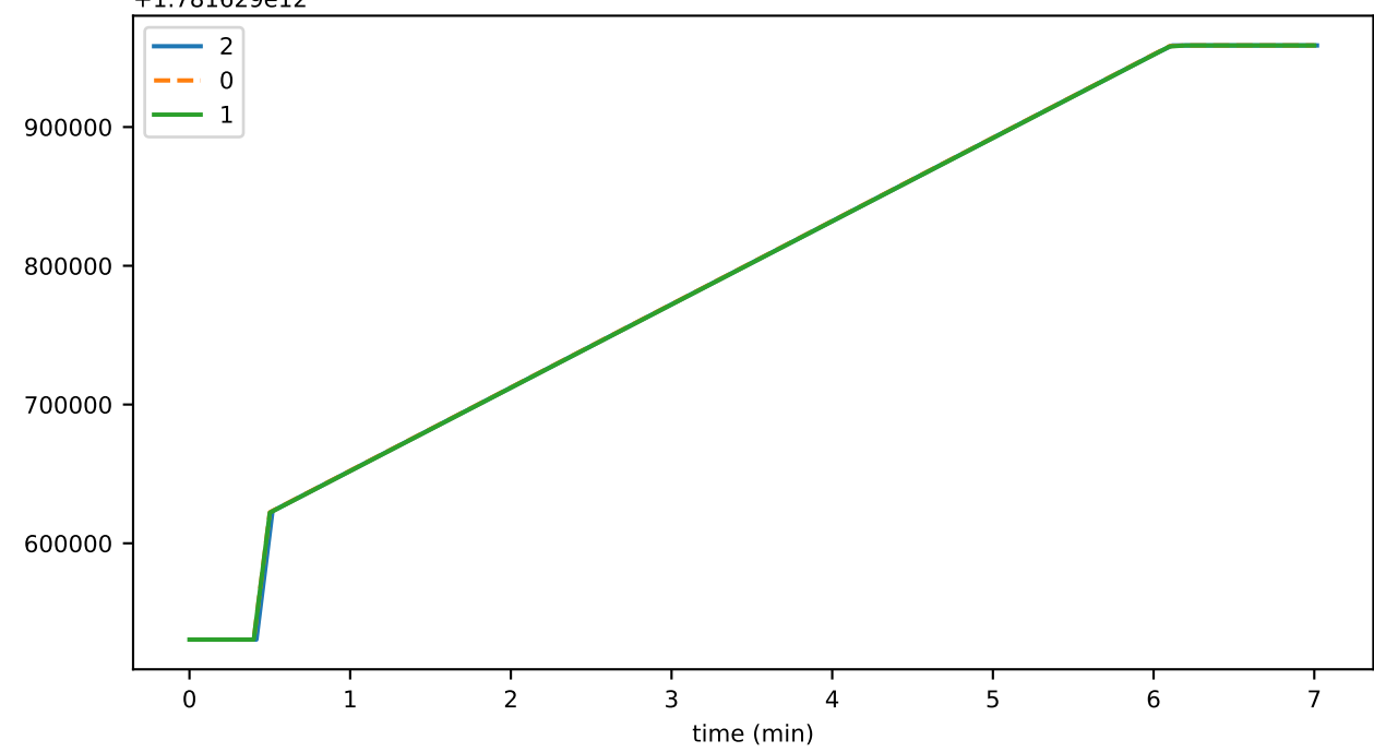
consensusTime
