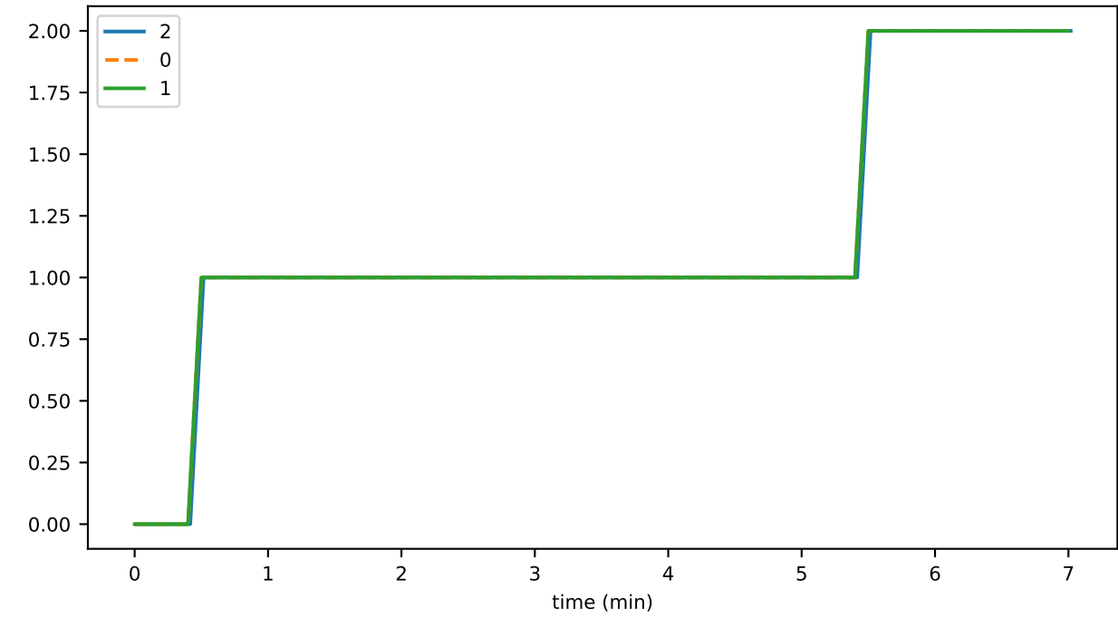
historyProofTransWMetaToFailCnt
