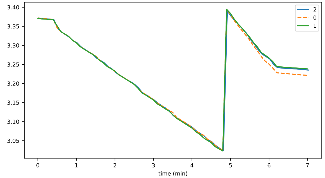
memFree
