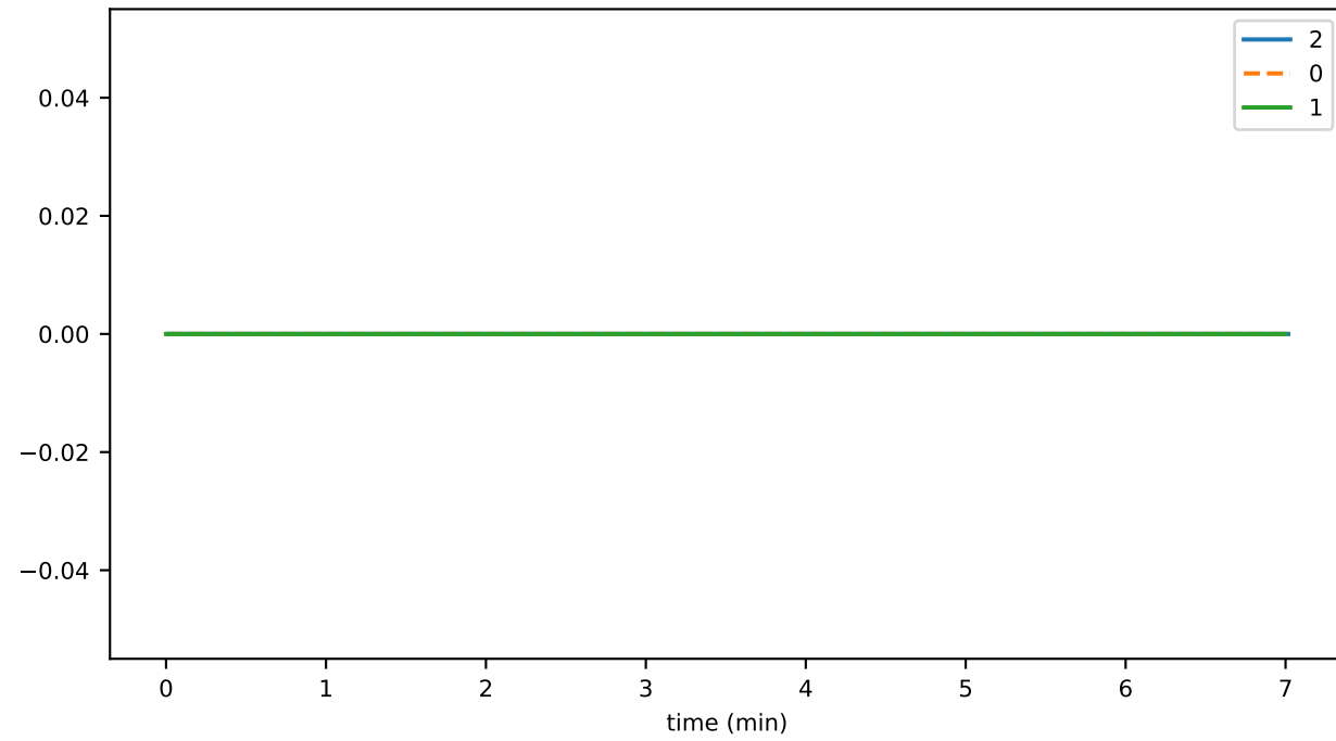
ds_compactions_level_2_leafKeysTimeMs_state
