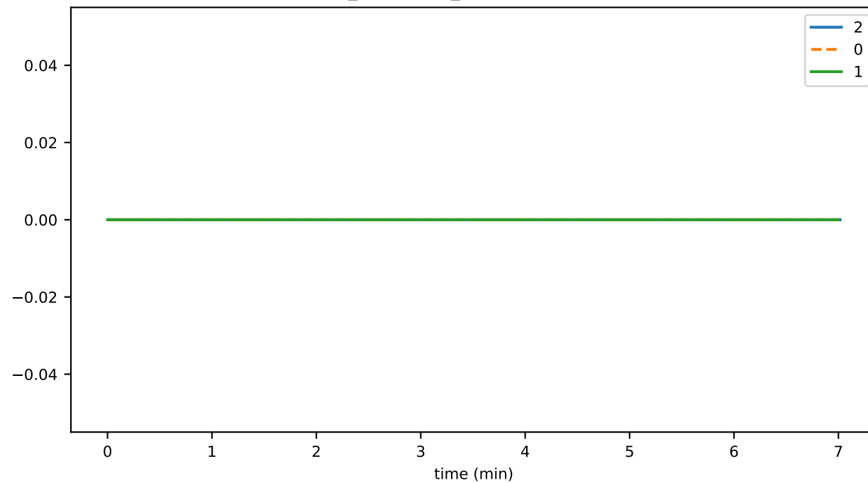
conn_connClose_endStreamReceived
