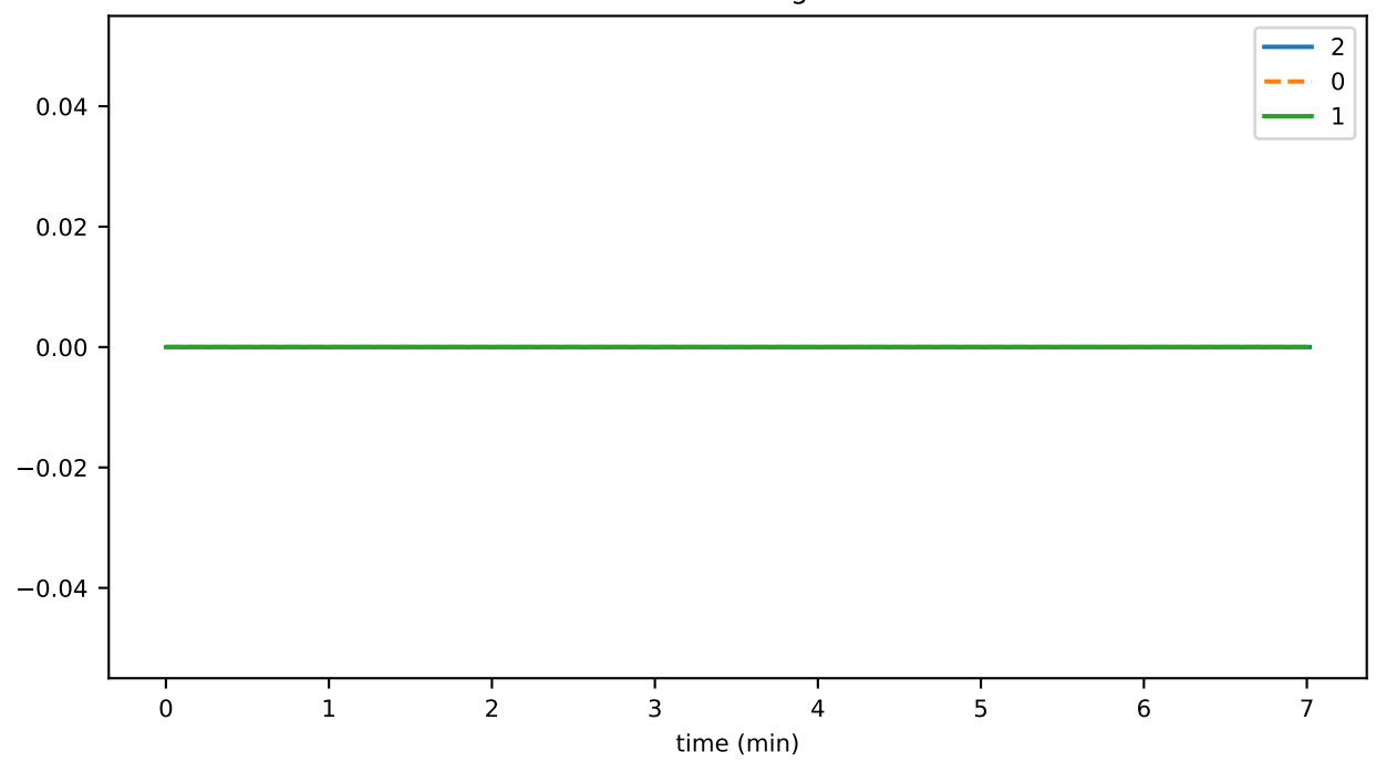
consensusSubmitMessageThrottledTxns
