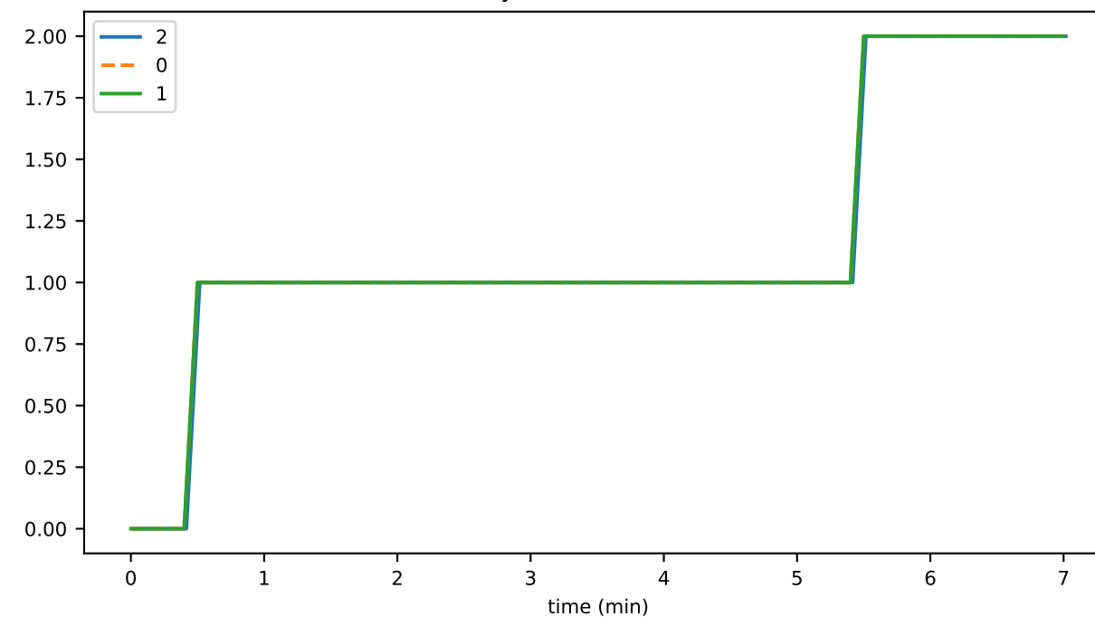
historyProofTransR2ToFailCnt
