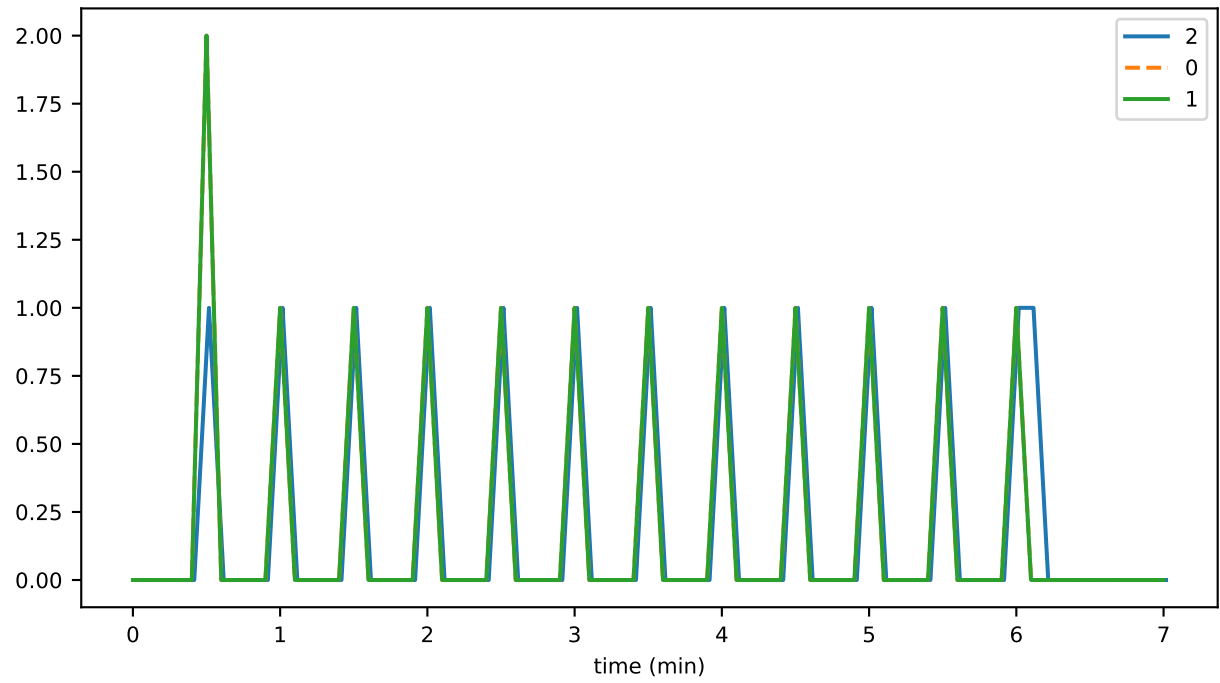
StateSnapshotManager_unhandled_task_count
