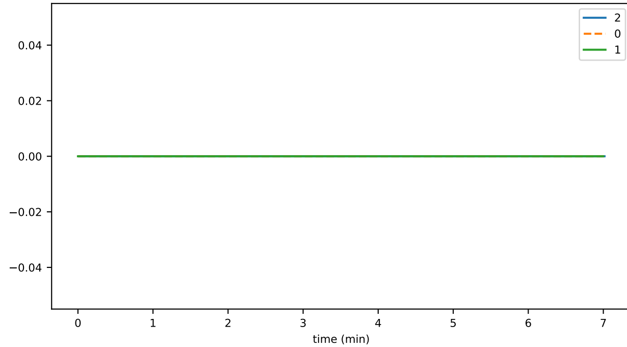
ds_compactions_level_2_leafKeysTimeMs_state
