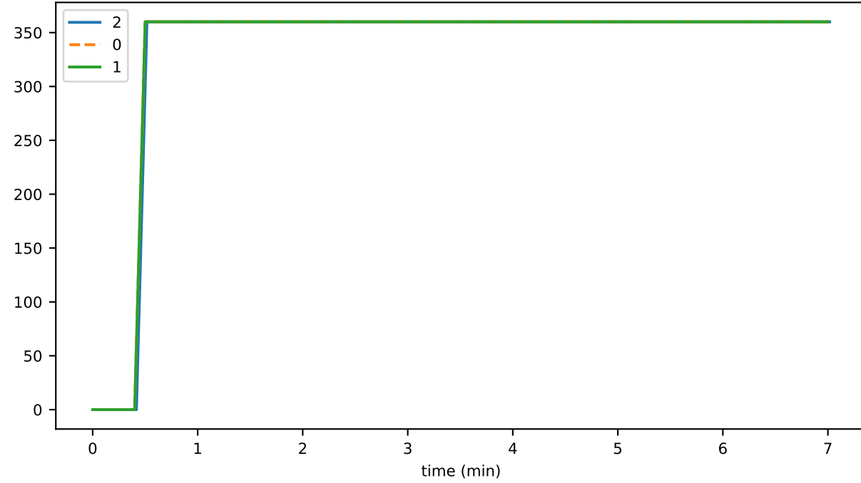
historyProofTransR2ToR3Ms
