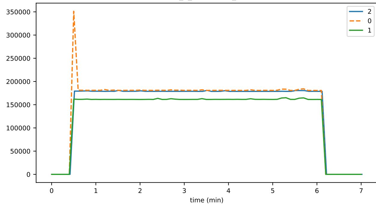
eventDelay_7_consensus_gossipMAX
