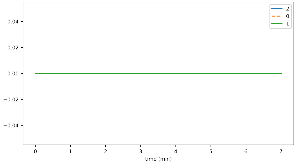
SmartContractService:Rejected_ethType3BlobTransaction_total
