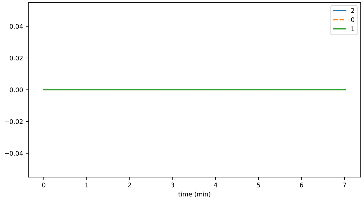
SmartContractService:Rejected_ethereumTxDueToIntrinsicGas_total
