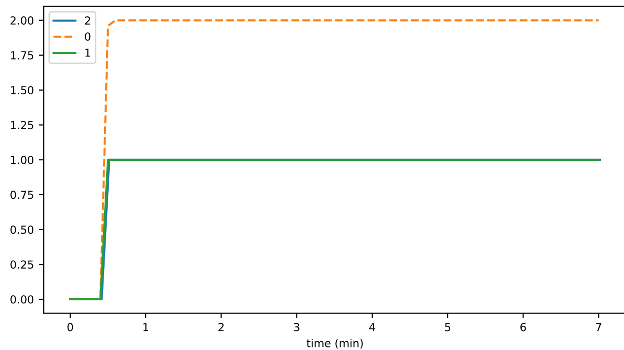
createdEventParents
