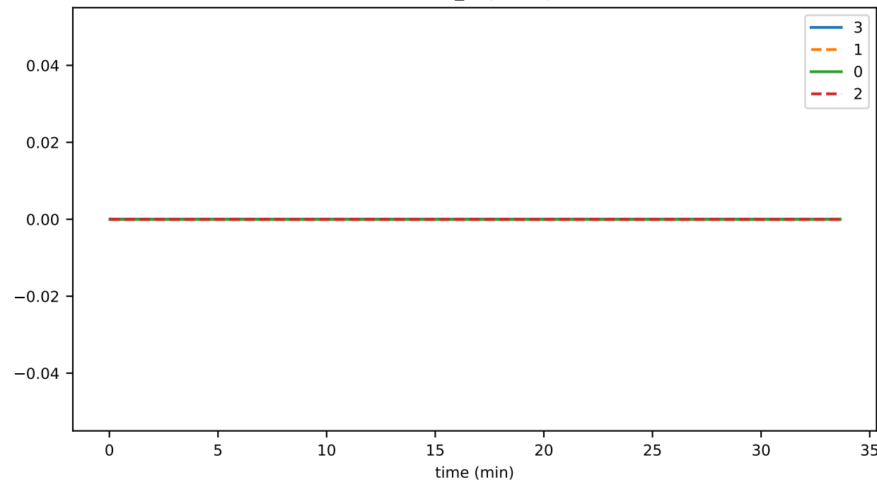
connSend_requestSendLatency
