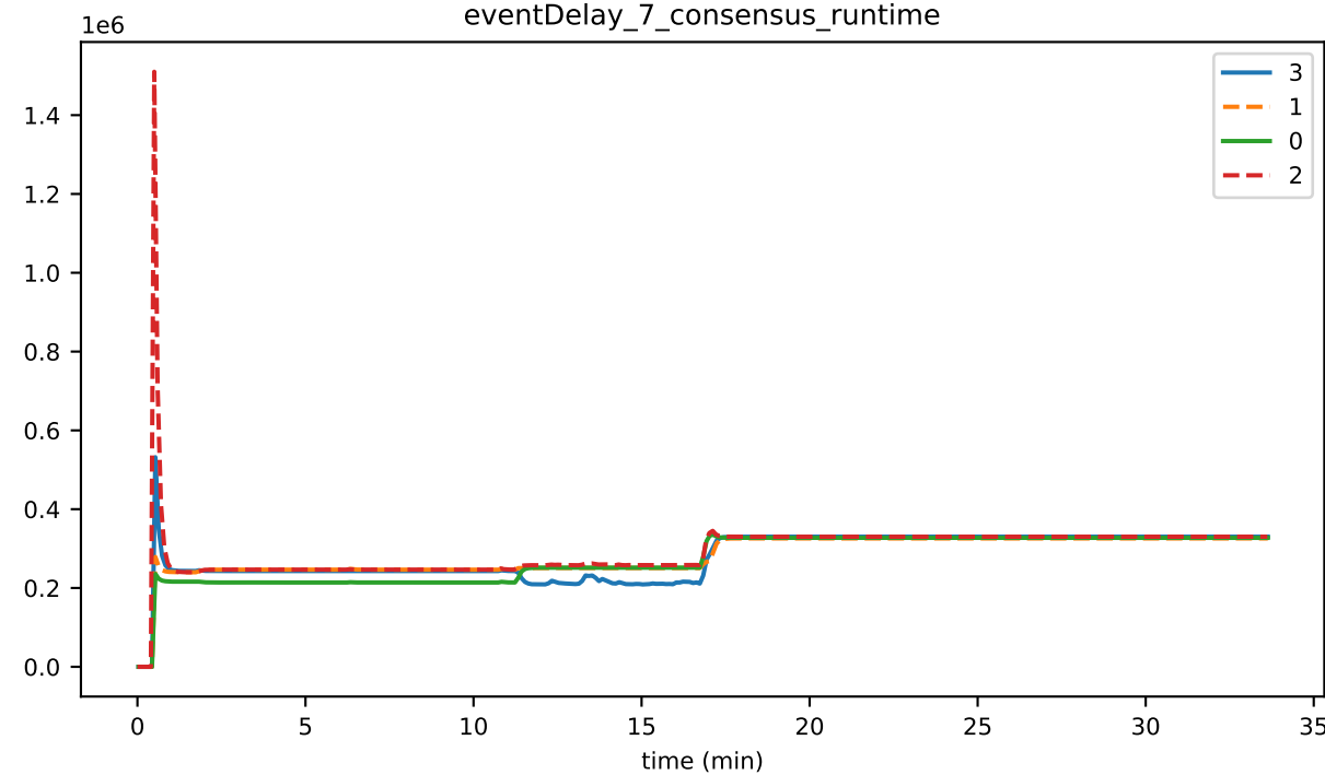
eventDelay_7_consensus_runtime
