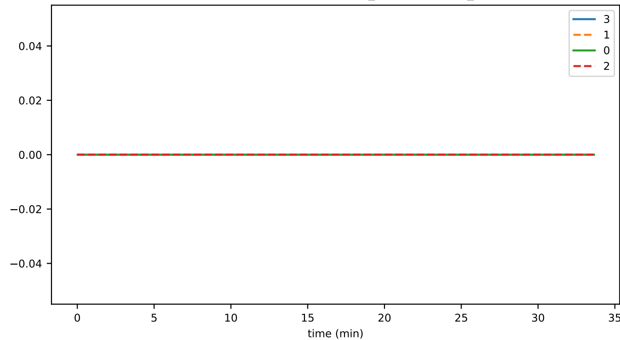
SmartContractService:Rejected_contractCallTx_total
