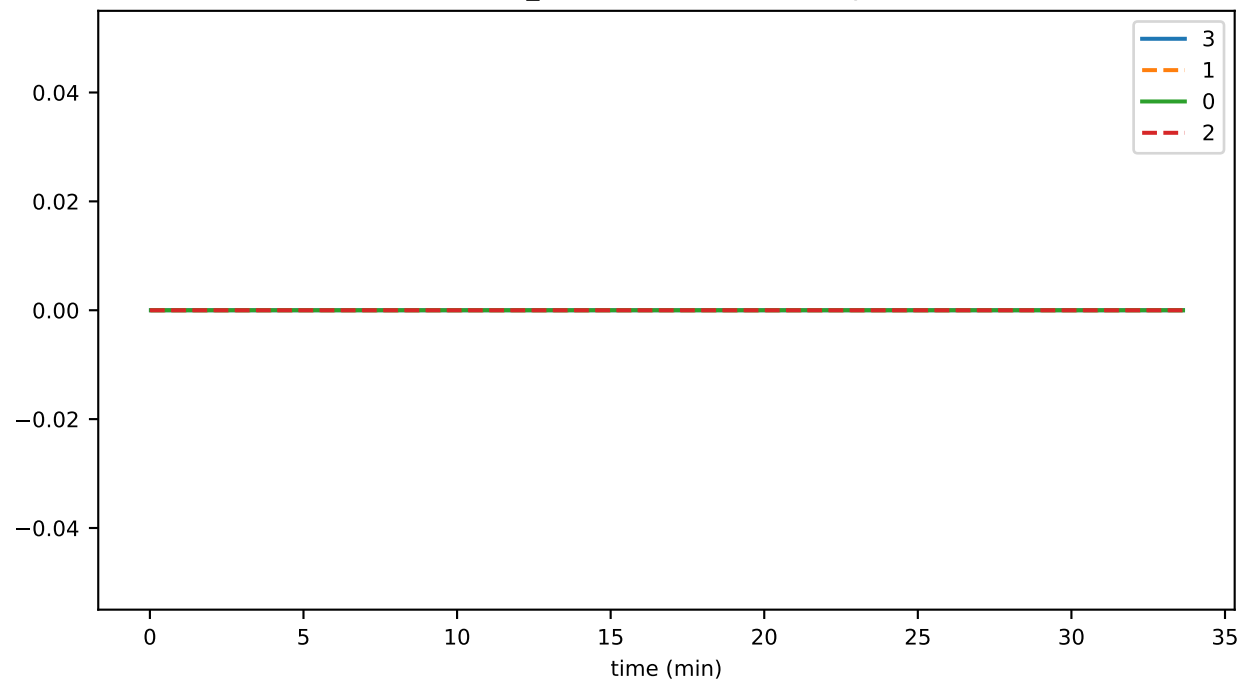
conn_closed
