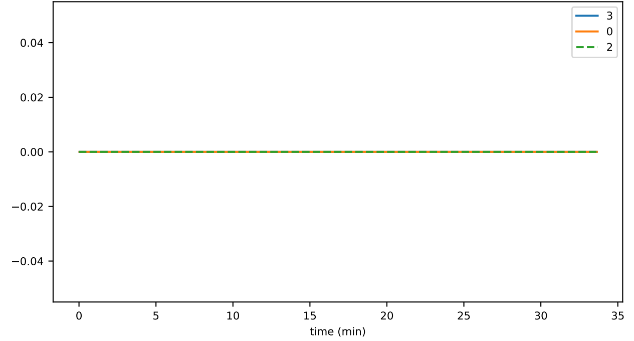
reconnectRejections_per_sec_01
