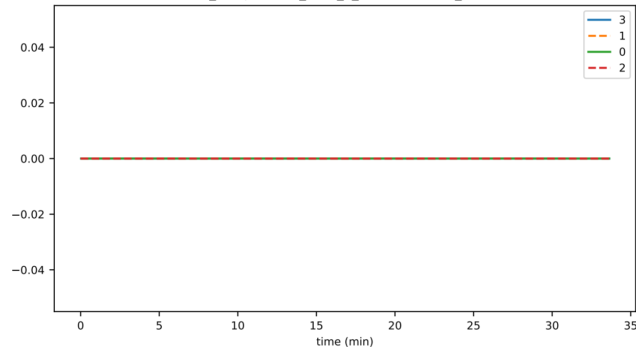
ds_compactions_level_5_leafKeysTimeMs_state
