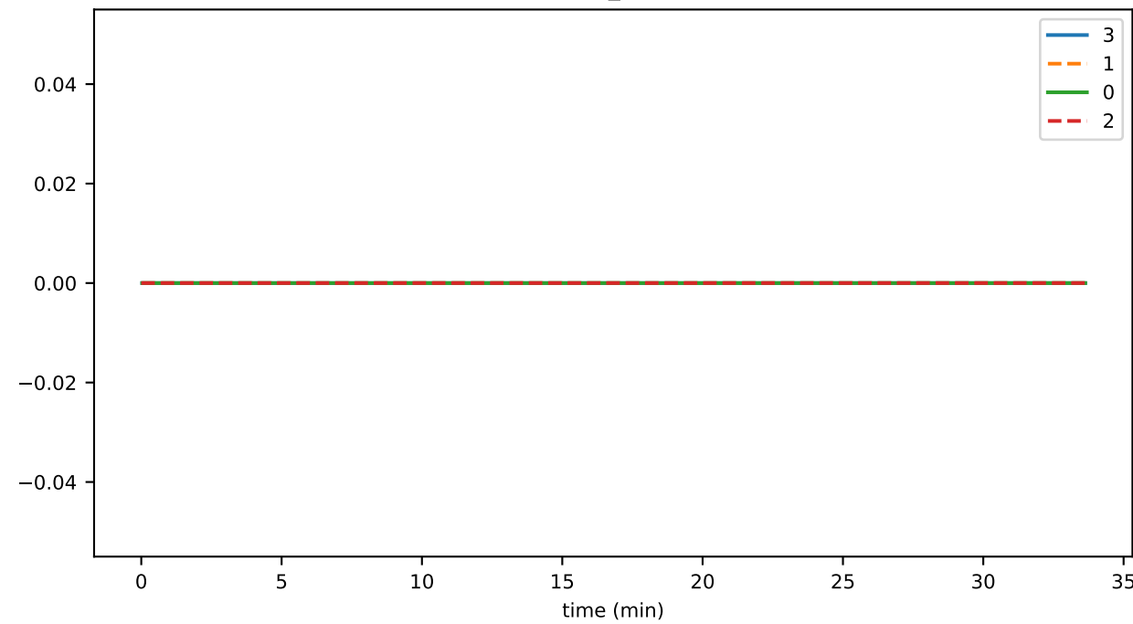
connRecv_skipBlock
