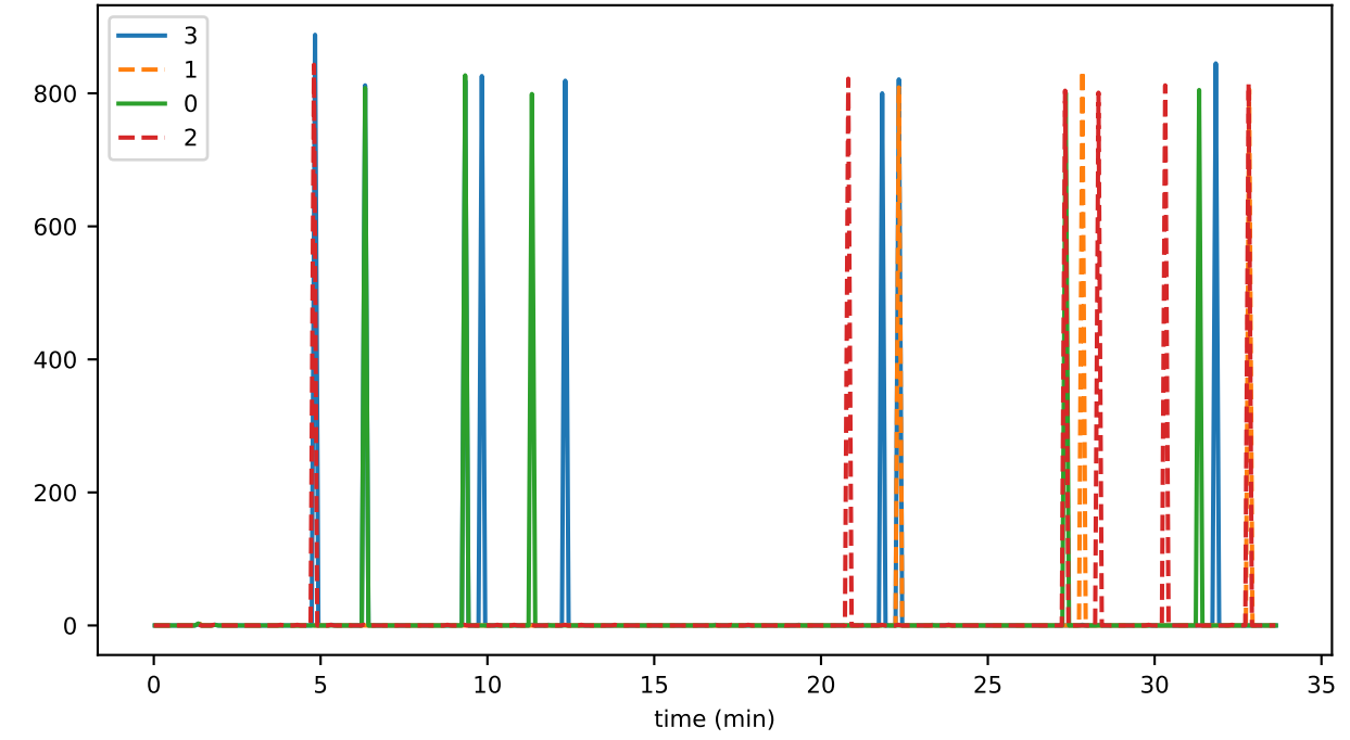
ds_compactions_level_1_leafKeysTimeMs_state
