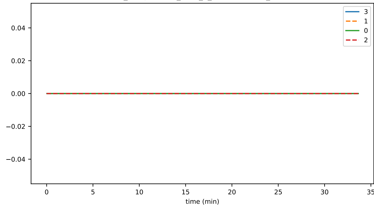
ds_compactions_level_8_hashesTimeMs_state
