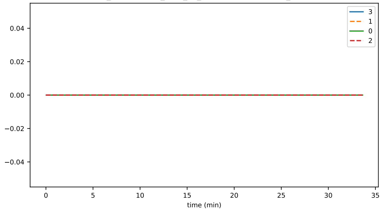
ds_compactions_level_10_leavesSavedSpaceMb_state
