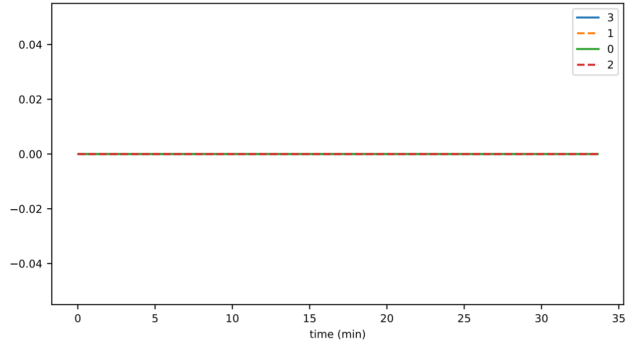
PlatformStatus
