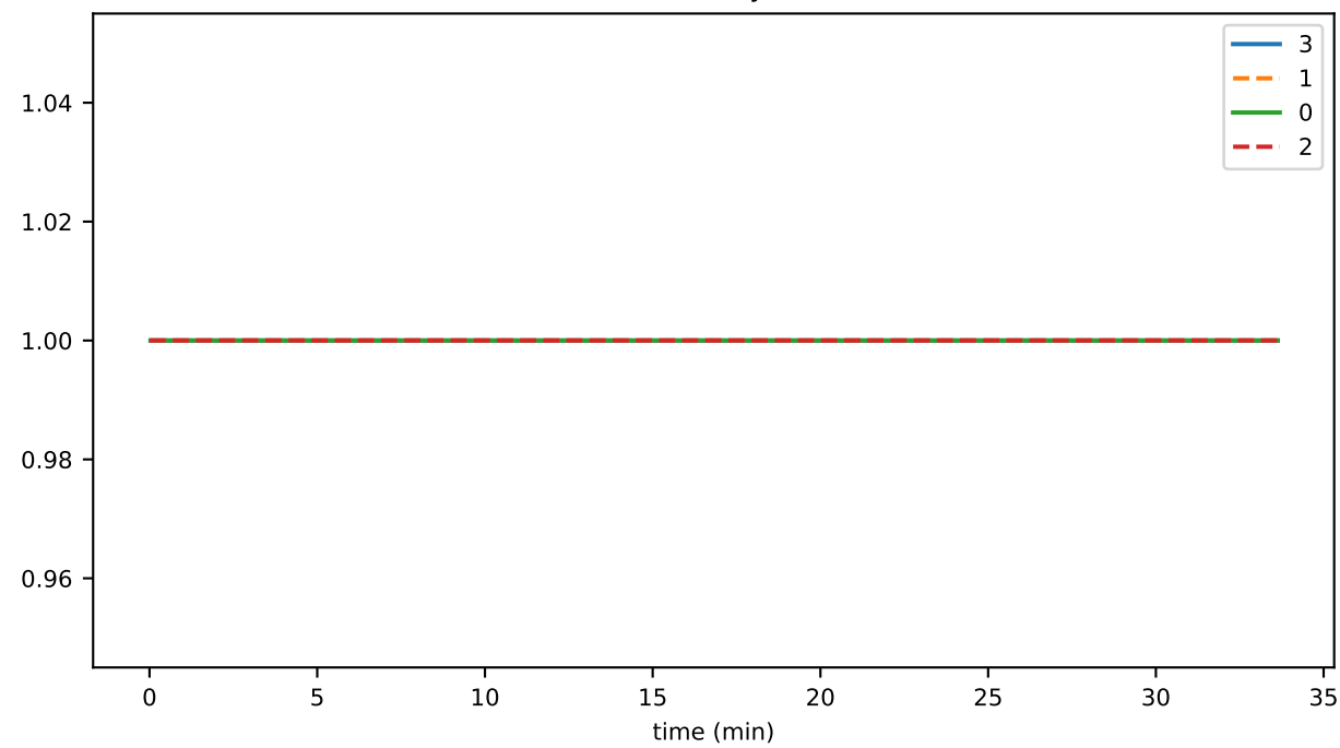
healthy
