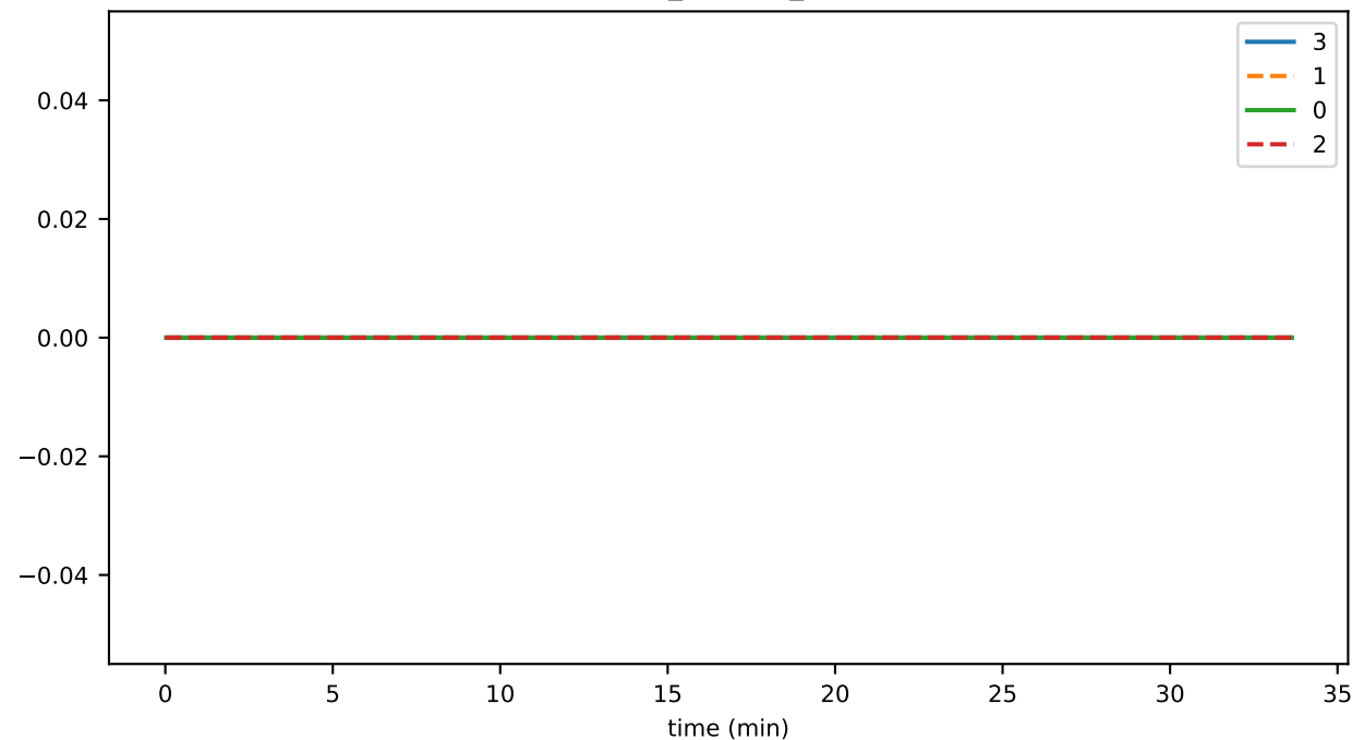
eventCreation_fraction_QUIESCENCE
