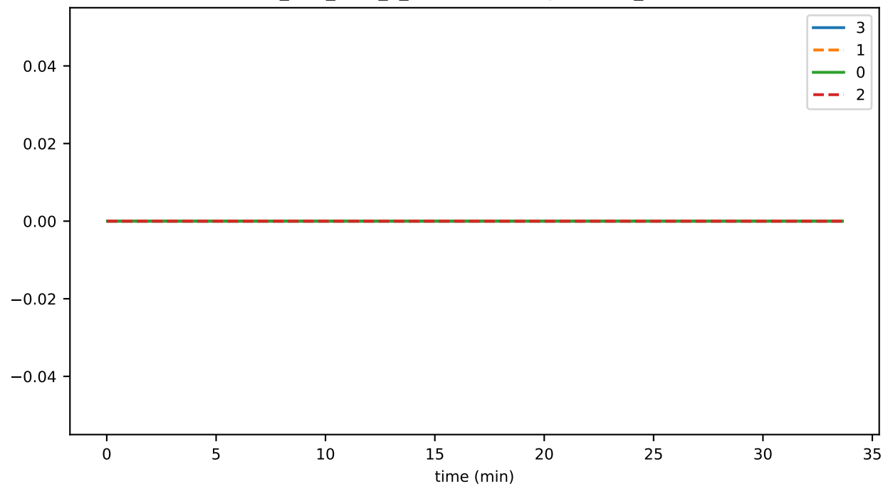
ds_flushes_hashesStoreFileSizeMb_state
