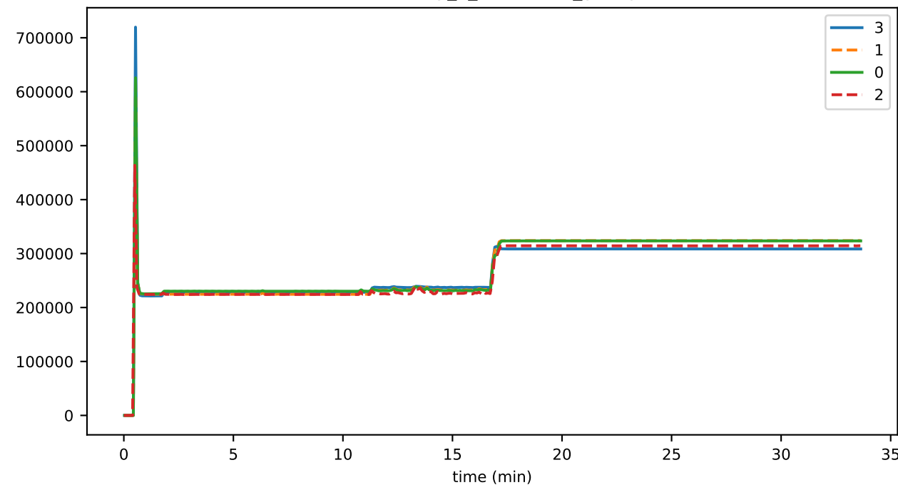
eventDelay_7_consensus_runtime
