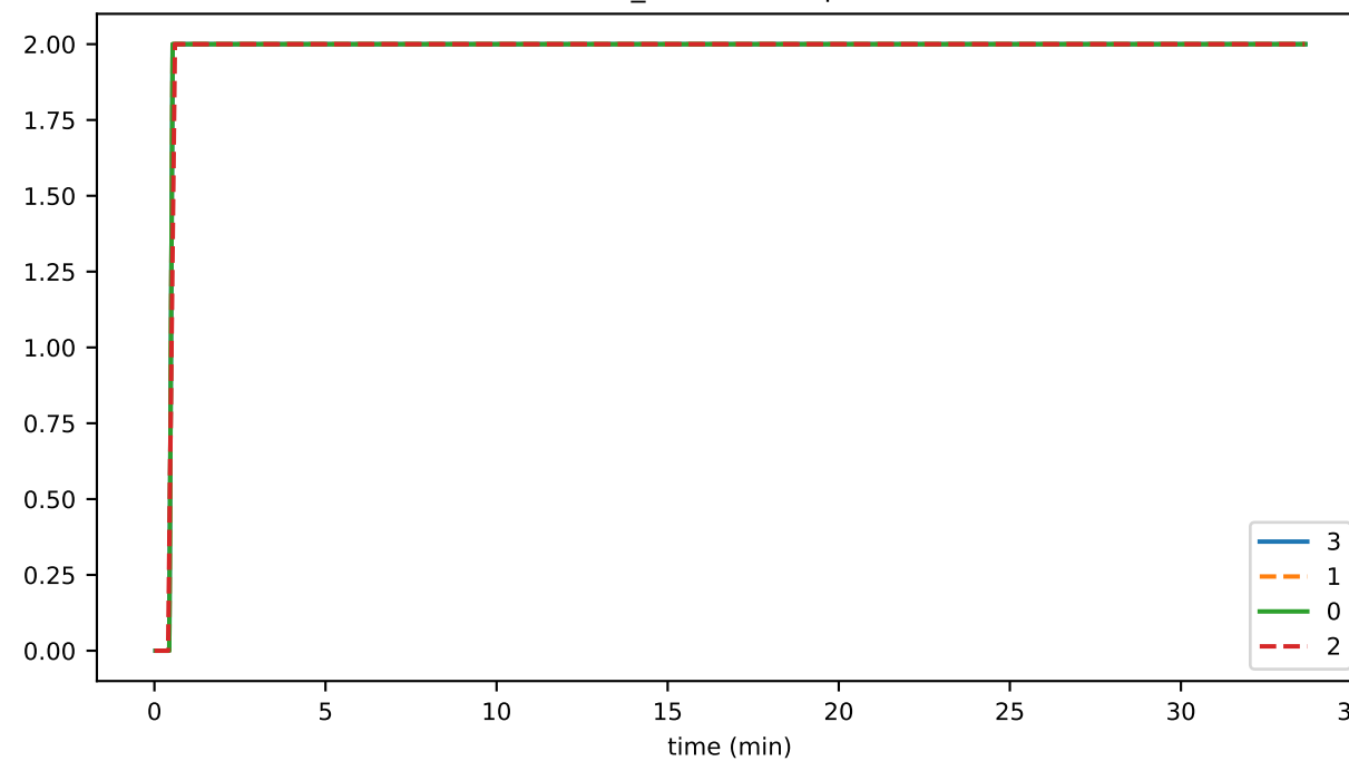
buffer_numBlocksOpened
