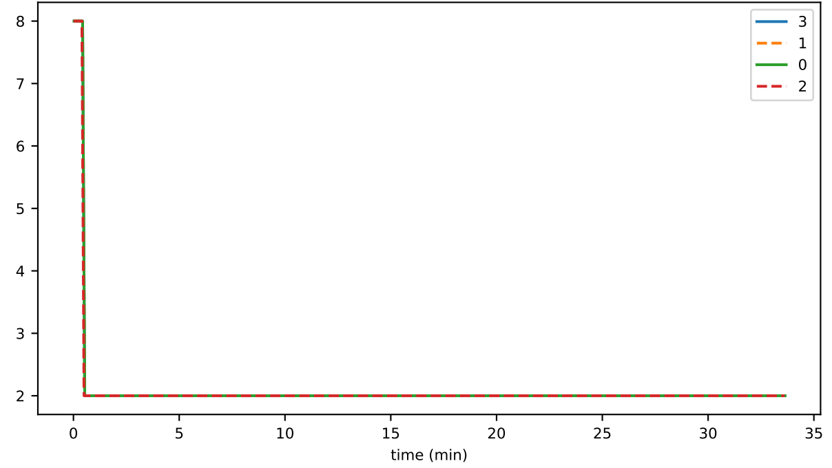
PlatformStatus
