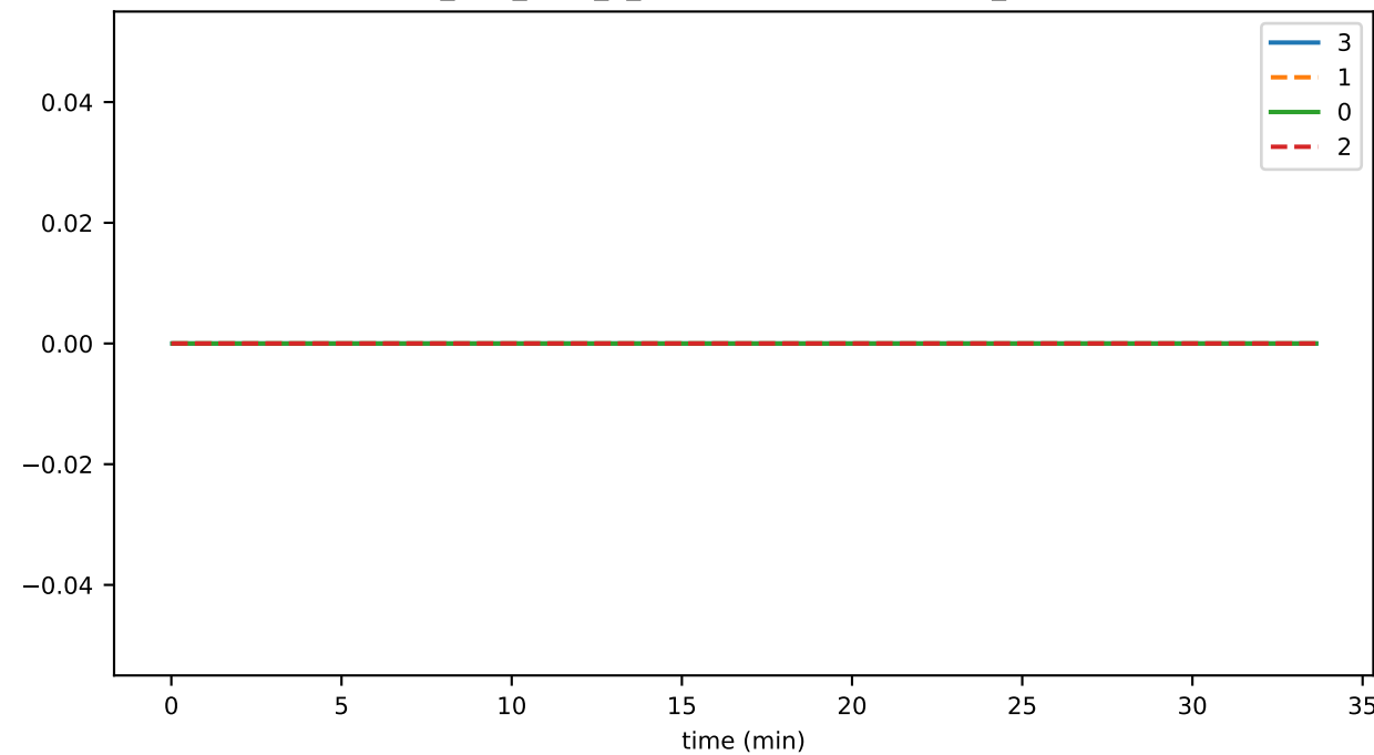
ds_files_level_6_leavesFileSizeByLevelMb_state
