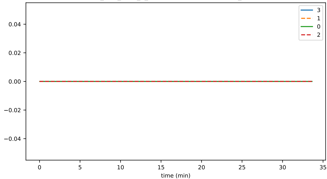
ds_files_level_6_leafKeysFileSizeByLevelMb_state
