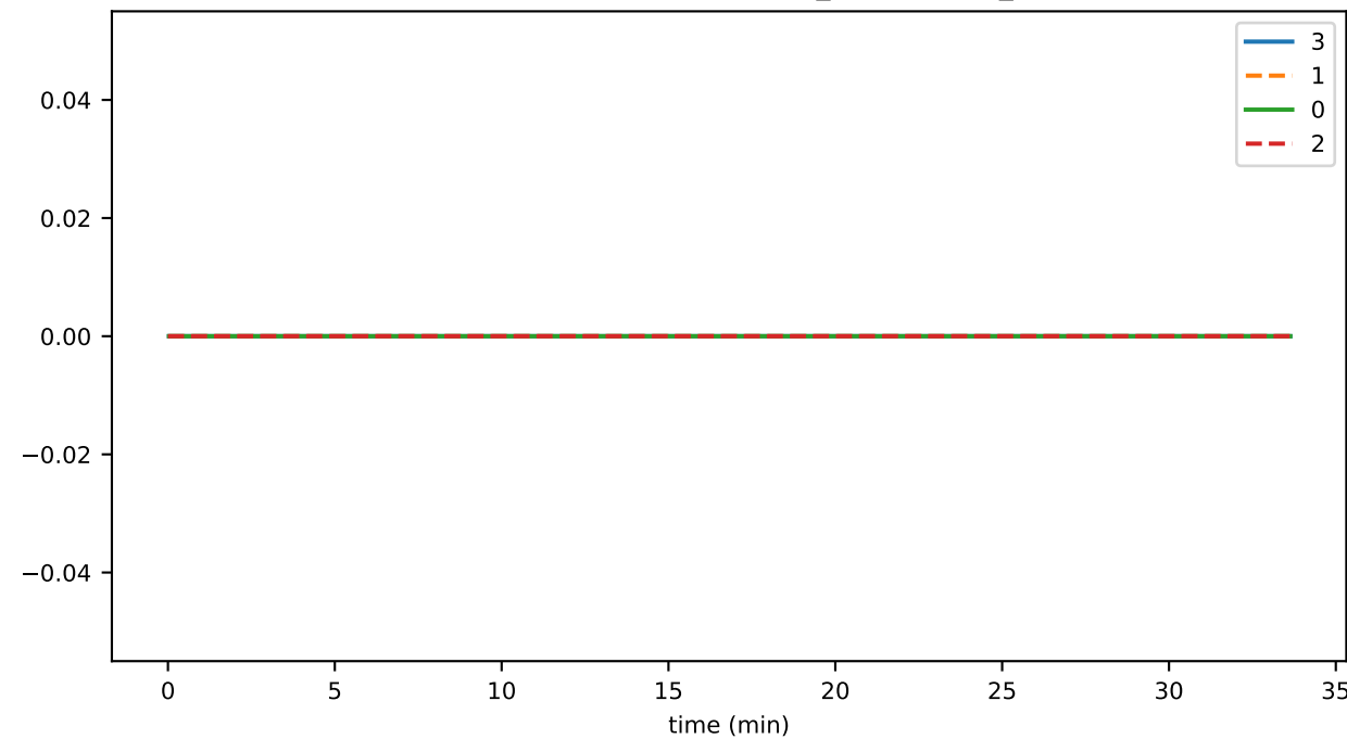
SmartContractService:Rejected_ethereumTx_total
