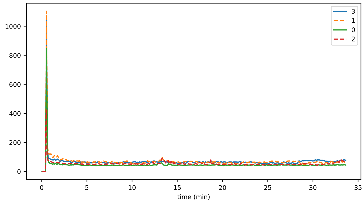
eventDelay_3_deduplication_runtime
