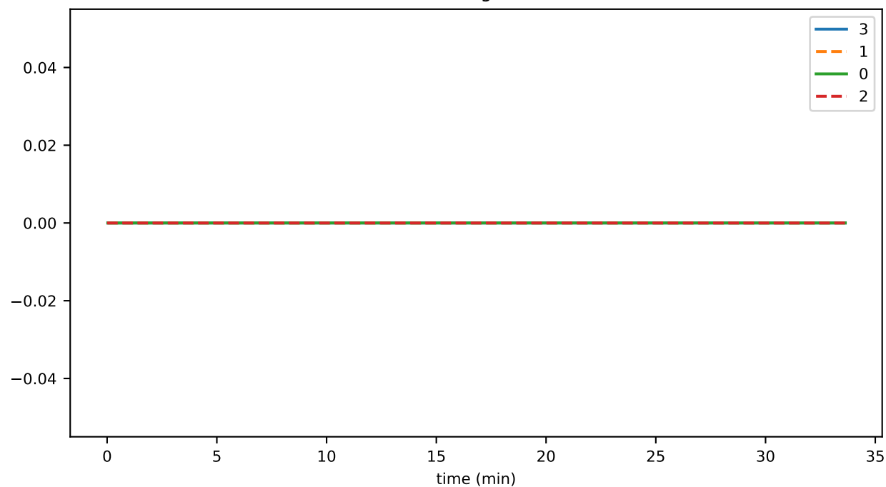
trans_per_event
