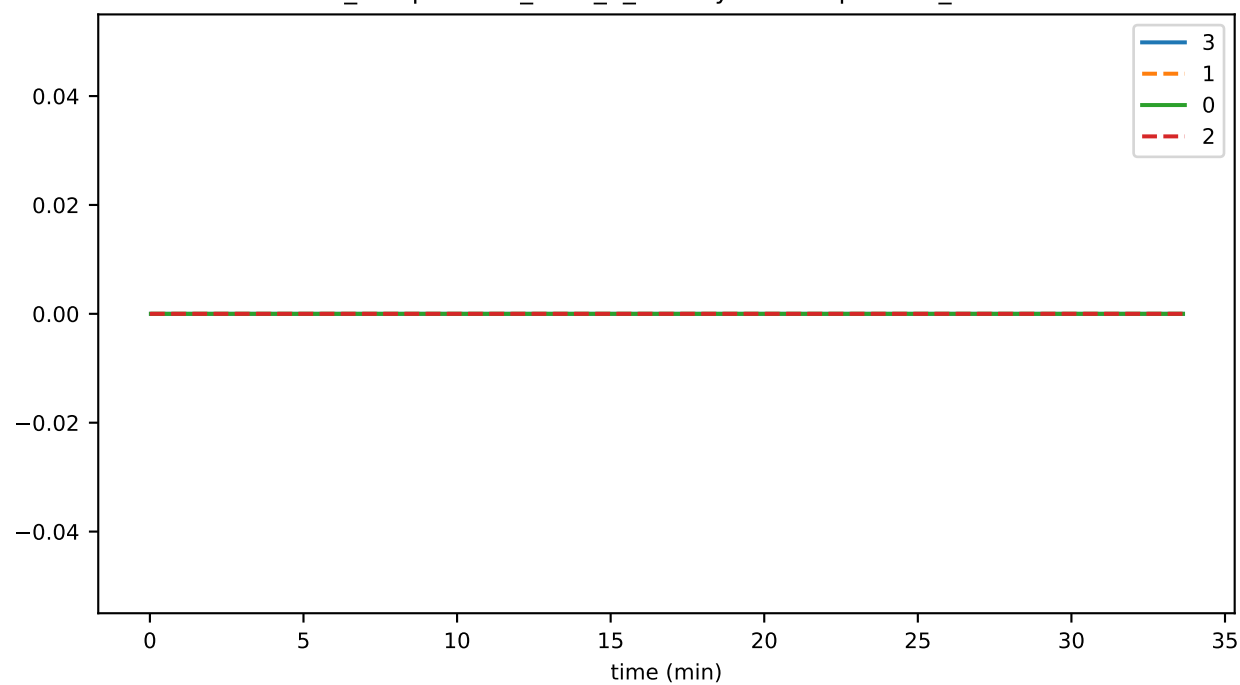
ds_compactions_level_5_leafKeysSavedSpaceMb_state
