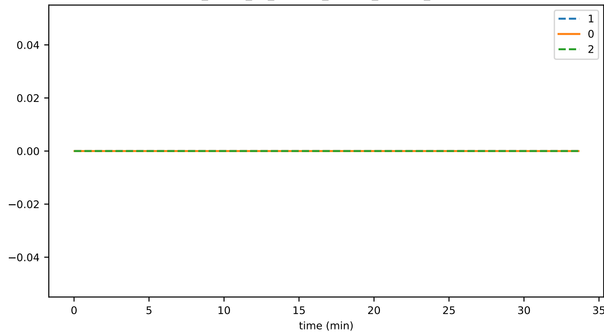
sync_phase_03_fraction_OTHER_FALLEN_BEHIND
