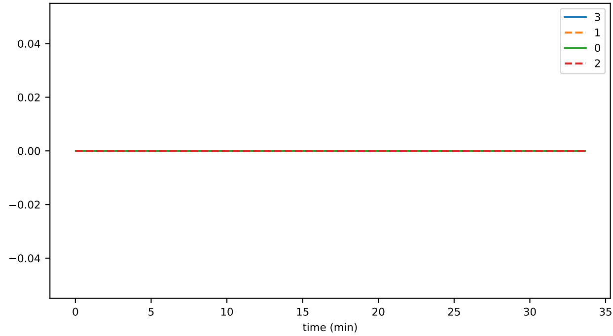
connRecv_endStream_timeout
