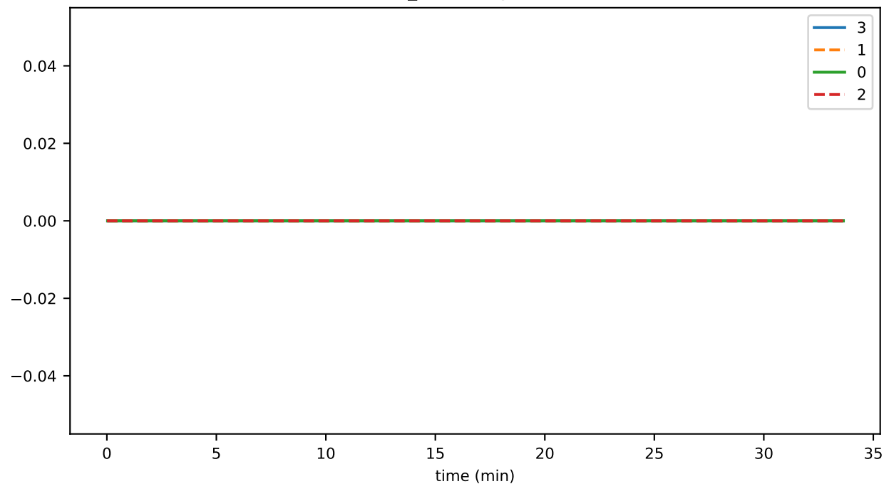
consensus_fraction_CREATING_SIGNED_STATE
