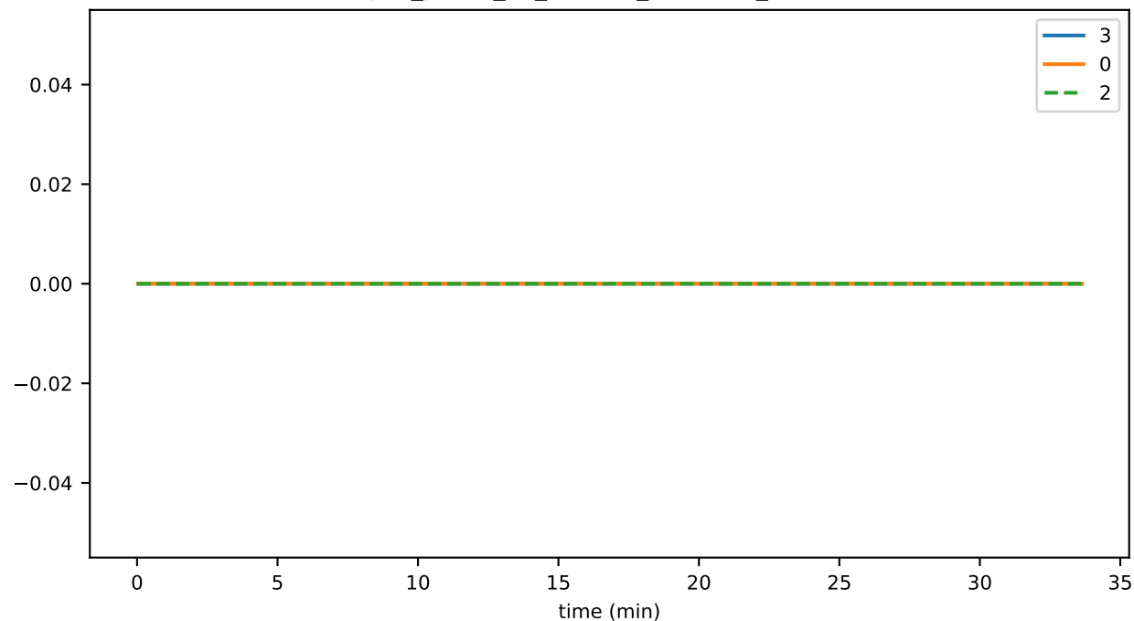
sync_phase_02_fraction_EXCHANGING_TIPS
