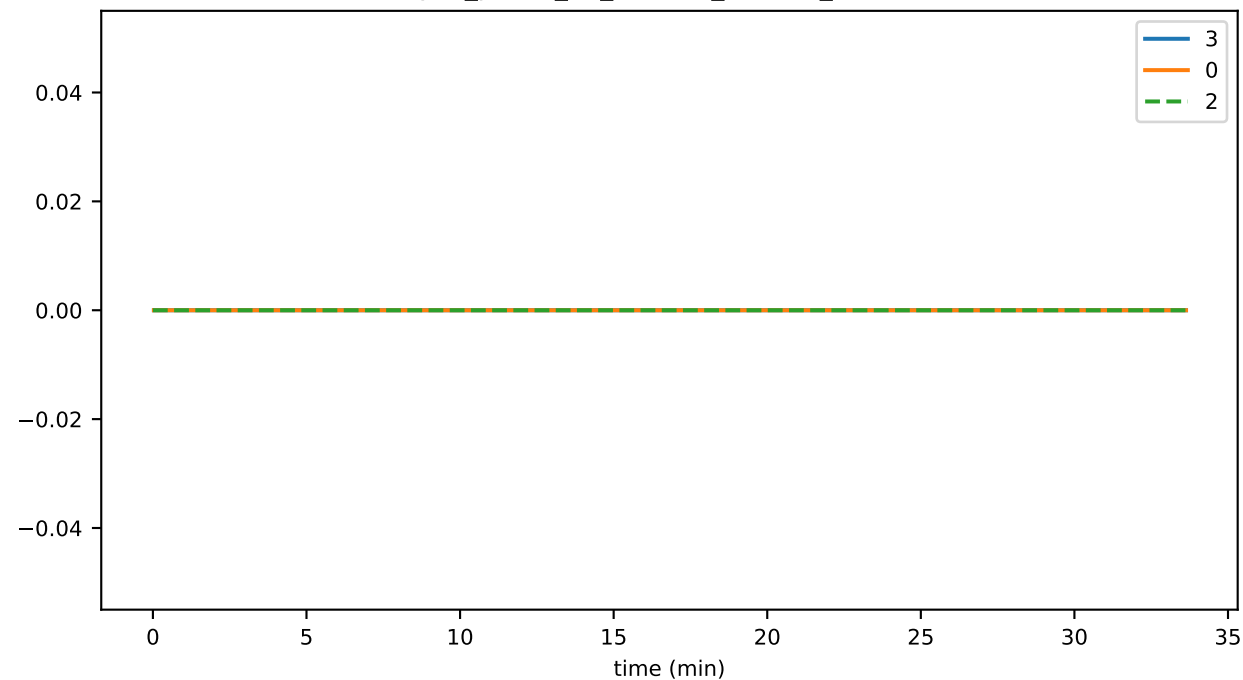
sync_phase_01_fraction_NO_PERMIT
