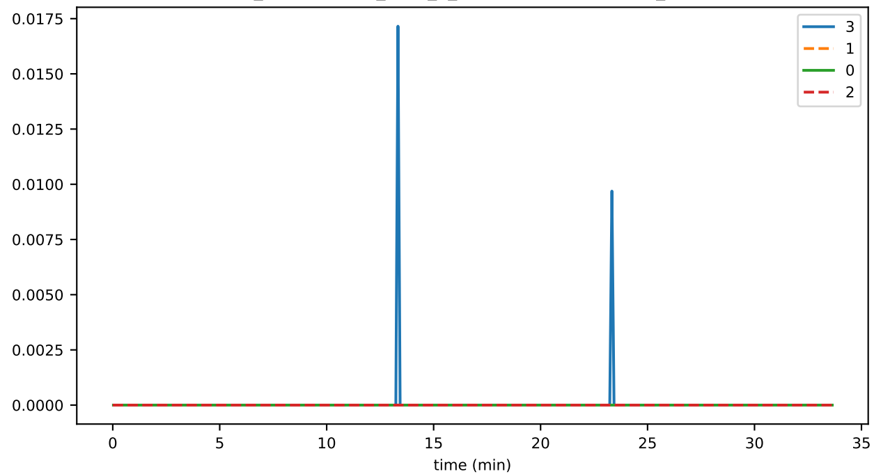
ds_compactions_level_2_hashesSavedSpaceMb_state
