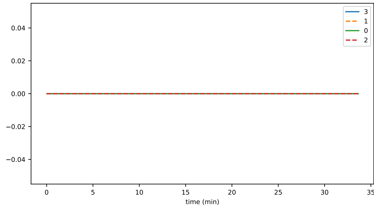
timeToDeleteState
