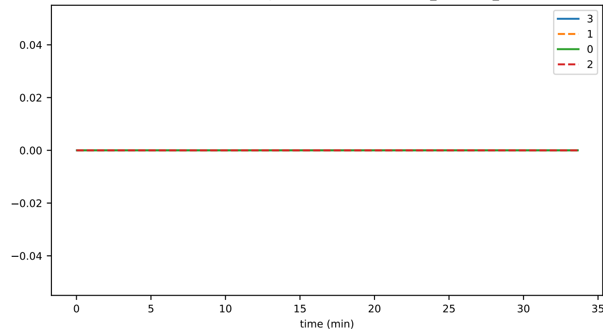
SmartContractService:SystemContractMethodCall_ALIASES_failed
