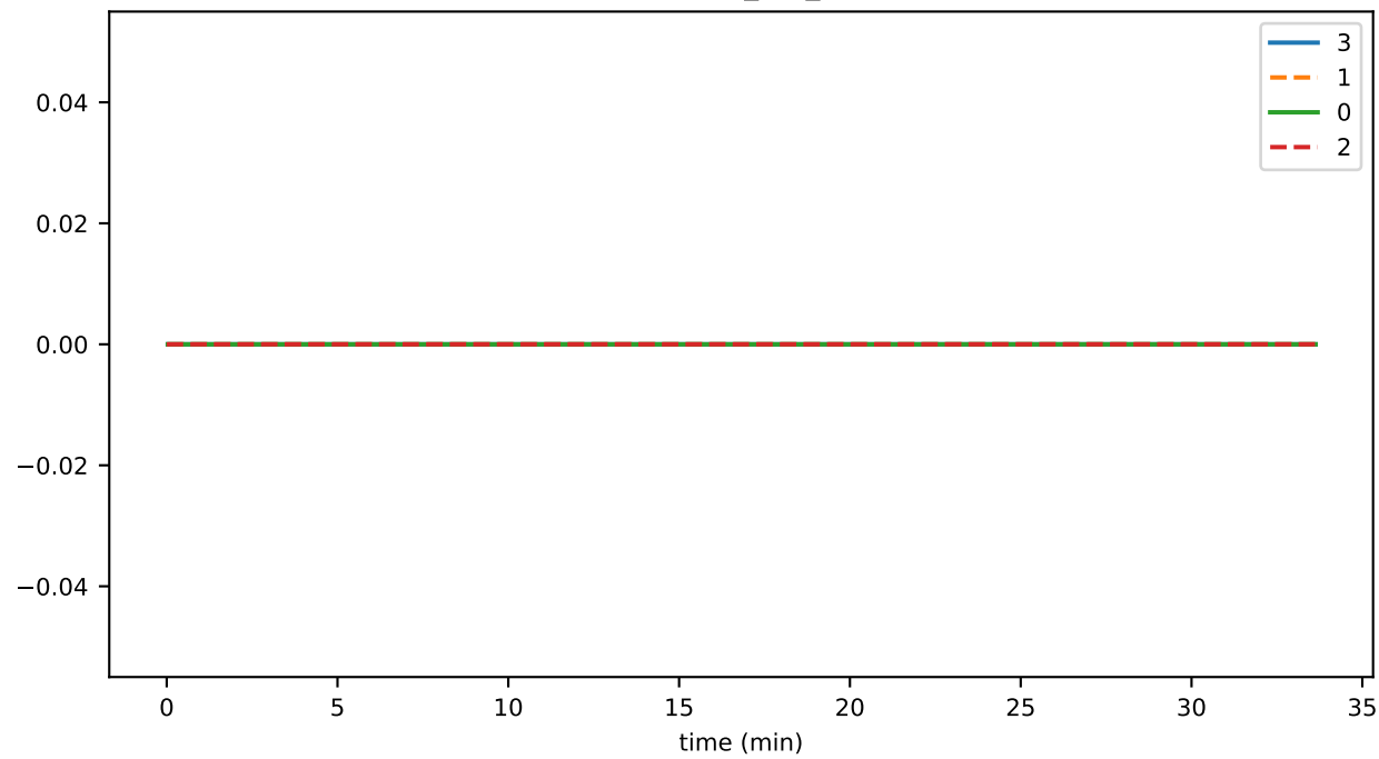
SigSpans_per_sec
