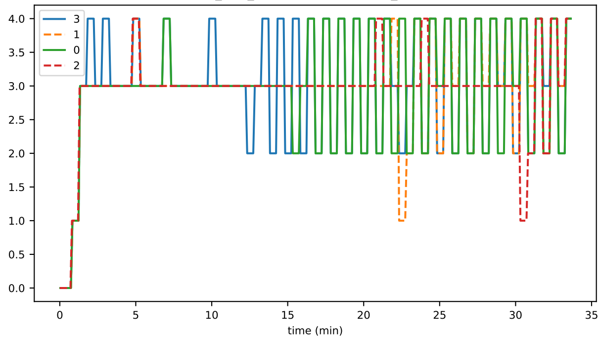
ds_files_hashesStoreFileCount_state
