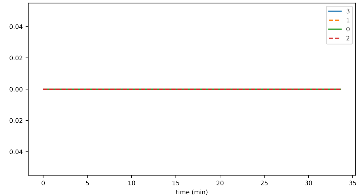
connRecv_resendBlock
