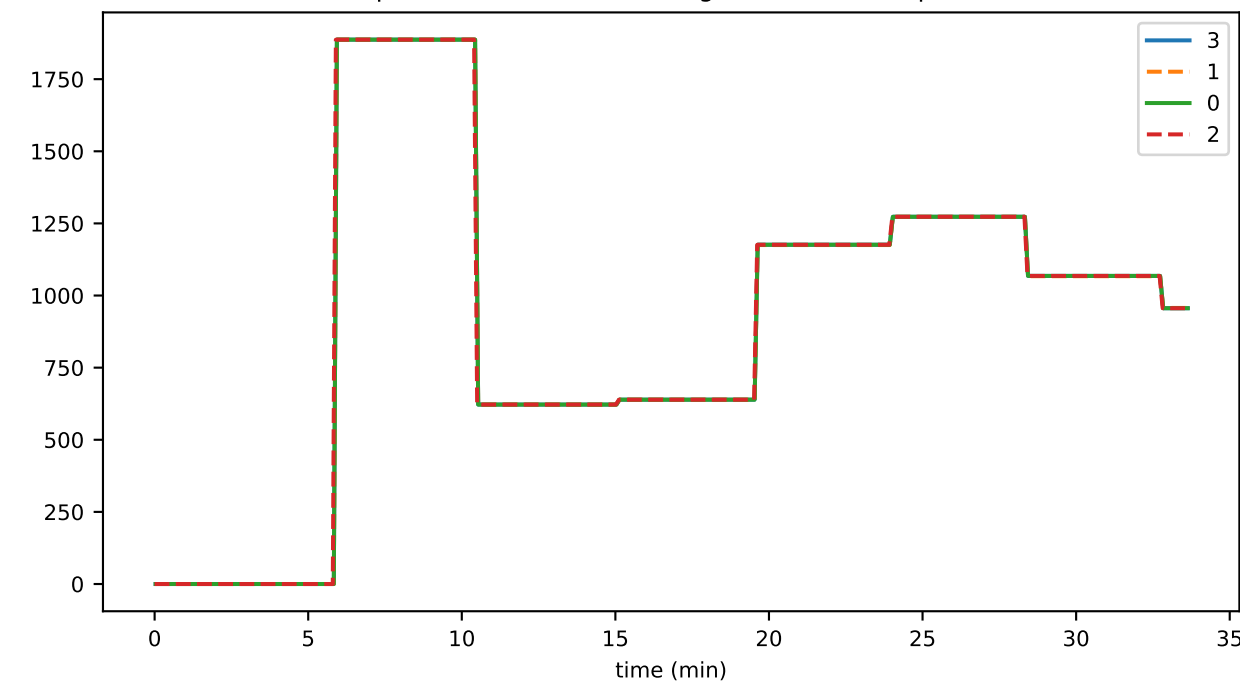
preconsensusEventAverageUnutilizedFileSpan
