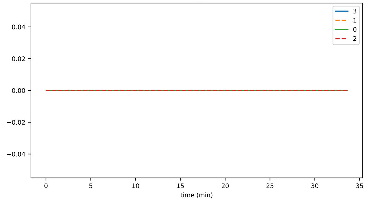
recordHashes_highestBlock
