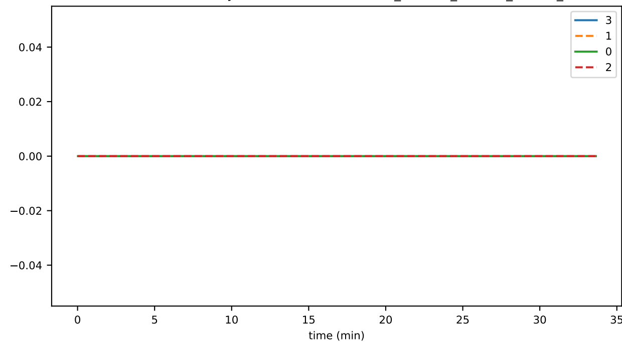
SmartContractService:SystemContractMethodCall_CREATE_DELETE_TOKEN_failed
