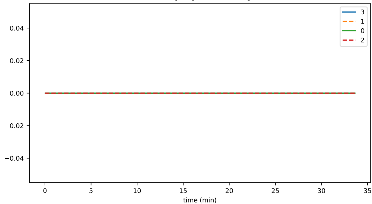
hintsSigningSuccessMsAvg
