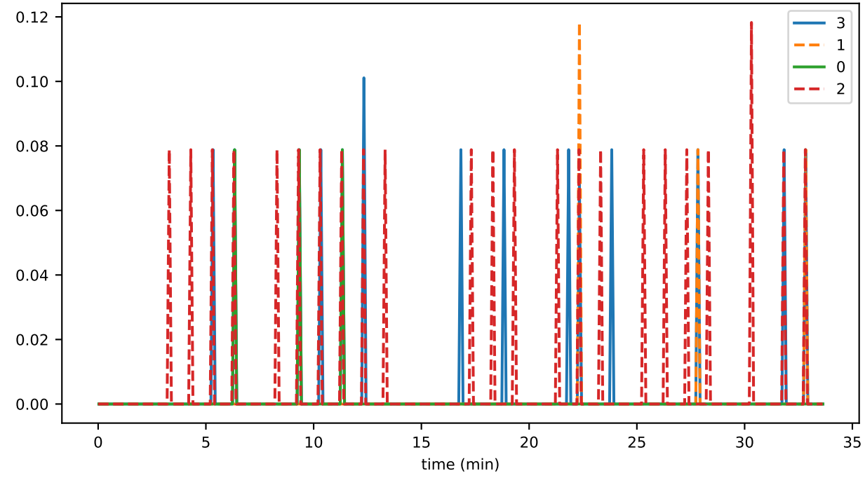
ds_compactions_level_1_leafKeysSavedSpaceMb_state
