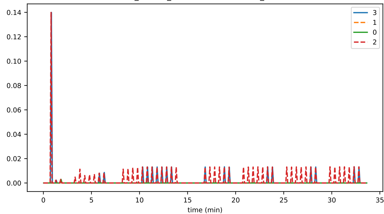
ds_flushes_leavesStoreFileSizeMb_state
