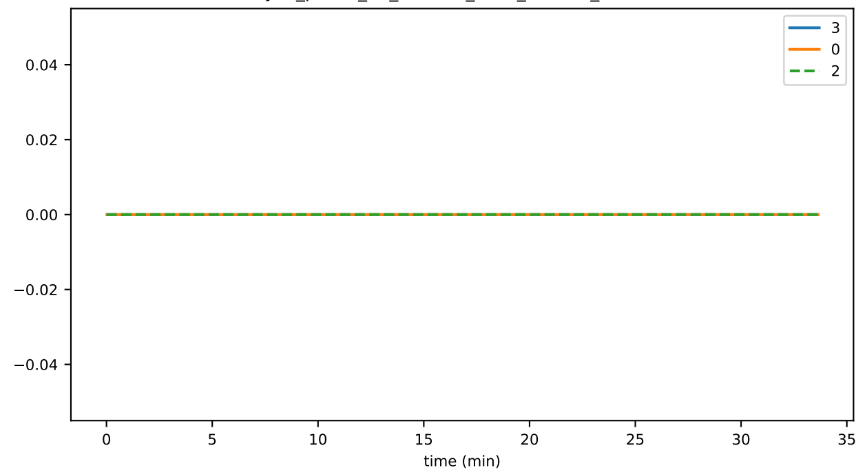
sync_phase_01_fraction_SELF_FALLEN_BEHIND
