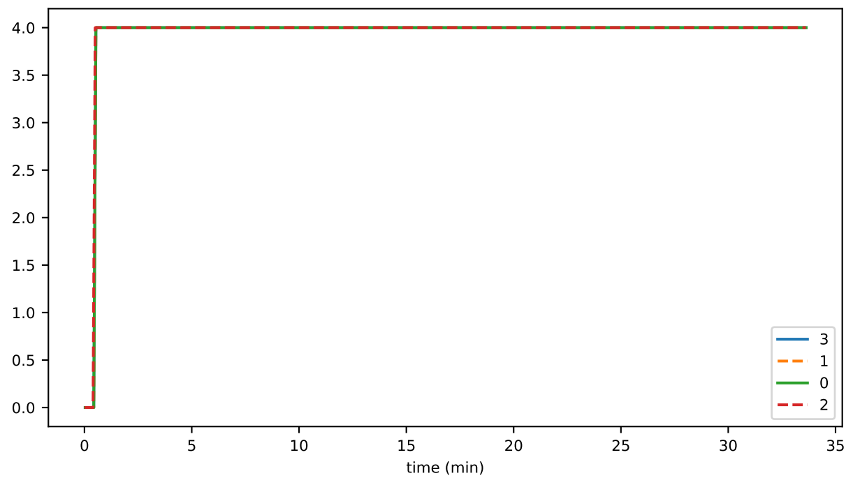
nodesPercentUsed
