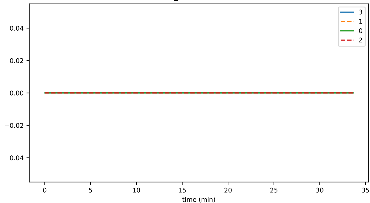
buffer_saturation
