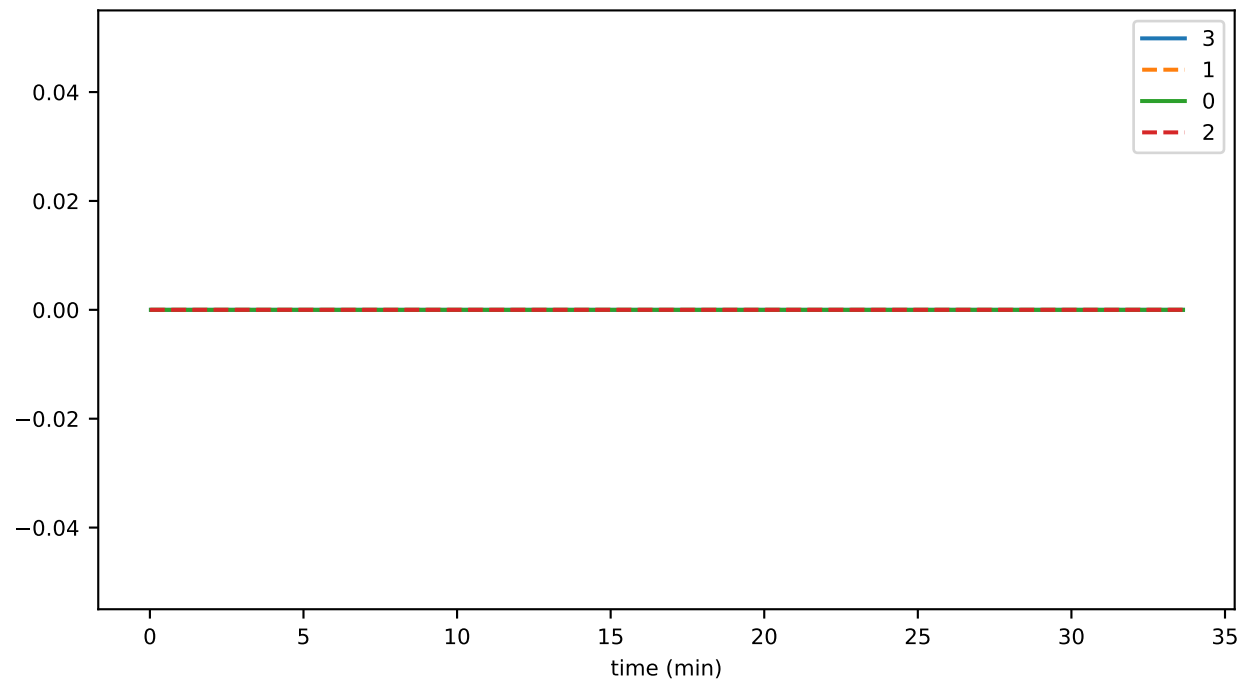
broadcastDisabledDueToLag
