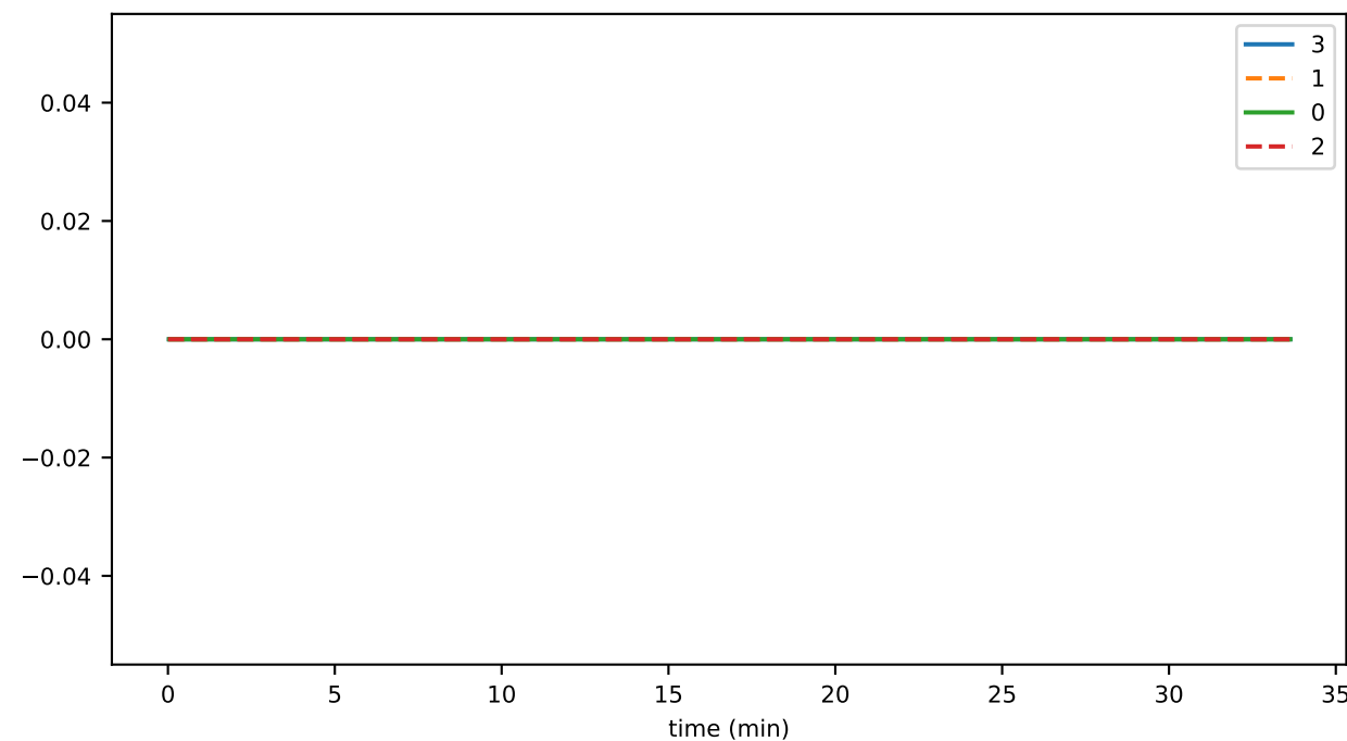
startsReconnectAsSender
