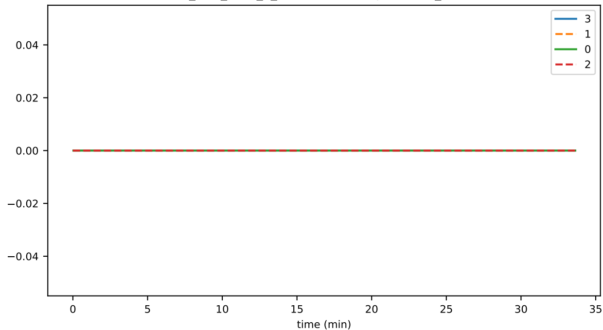
ds_files_level_3_leavesFileSizeByLevelMb_state
