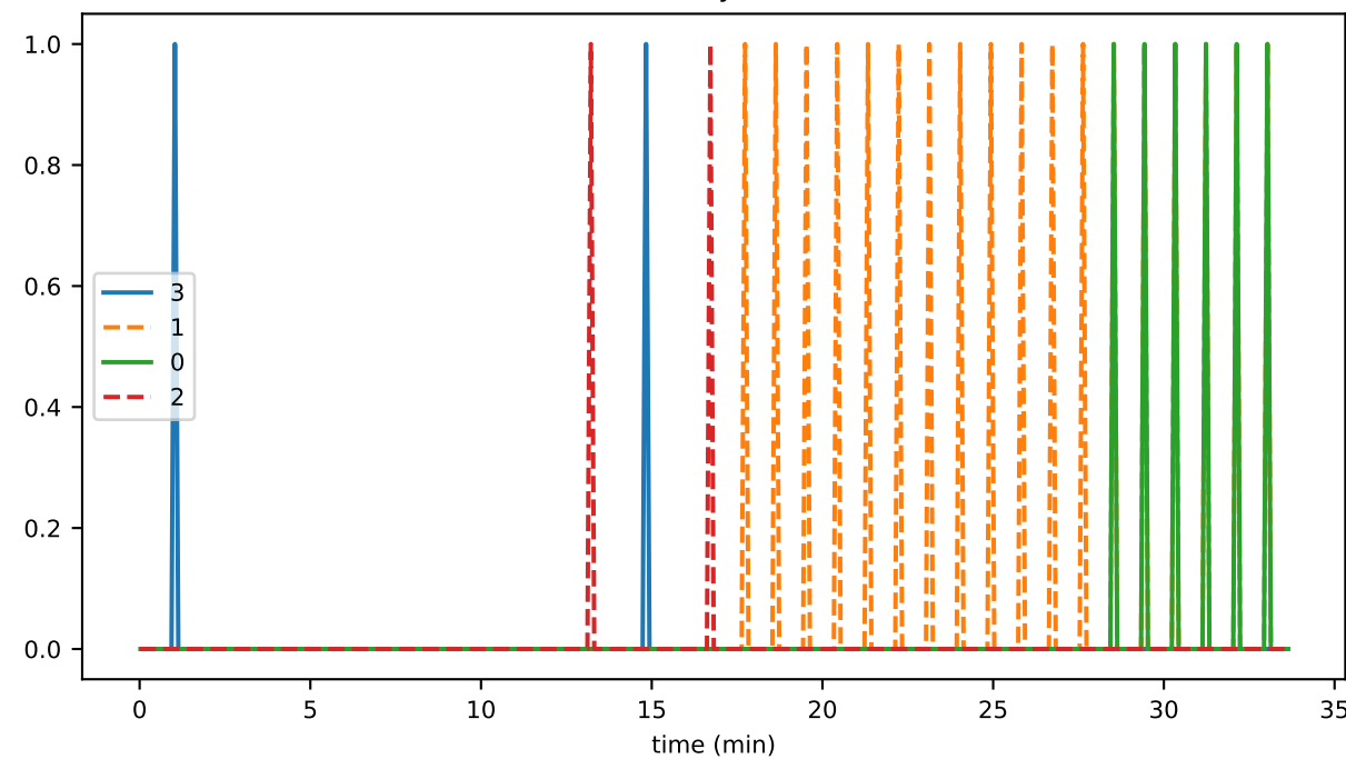
bufferedPriorityTransactions
