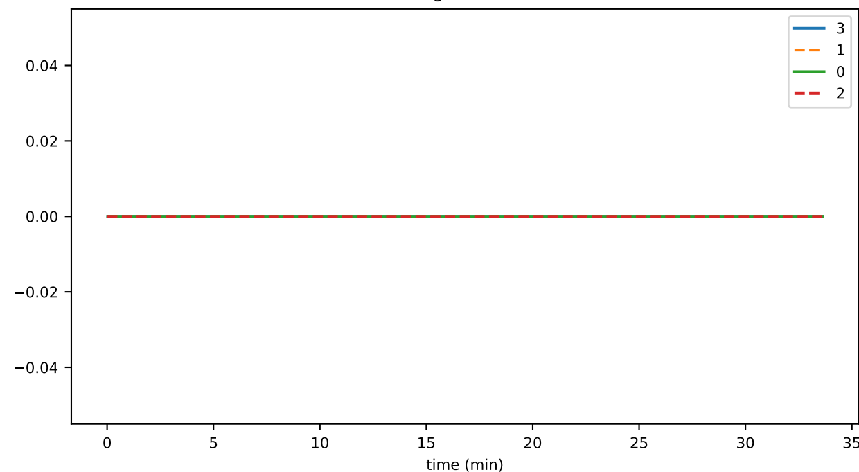
sync_per_secC
