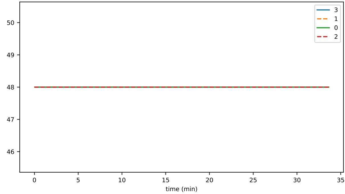
reconnectRejections_per_sec_00
