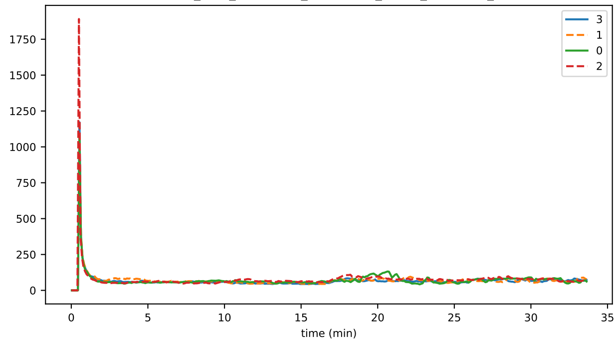
ConsensusEngine_busy_fraction
