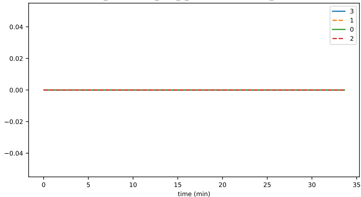
ds_compactions_level_10_hashesSavedSpaceMb_state
