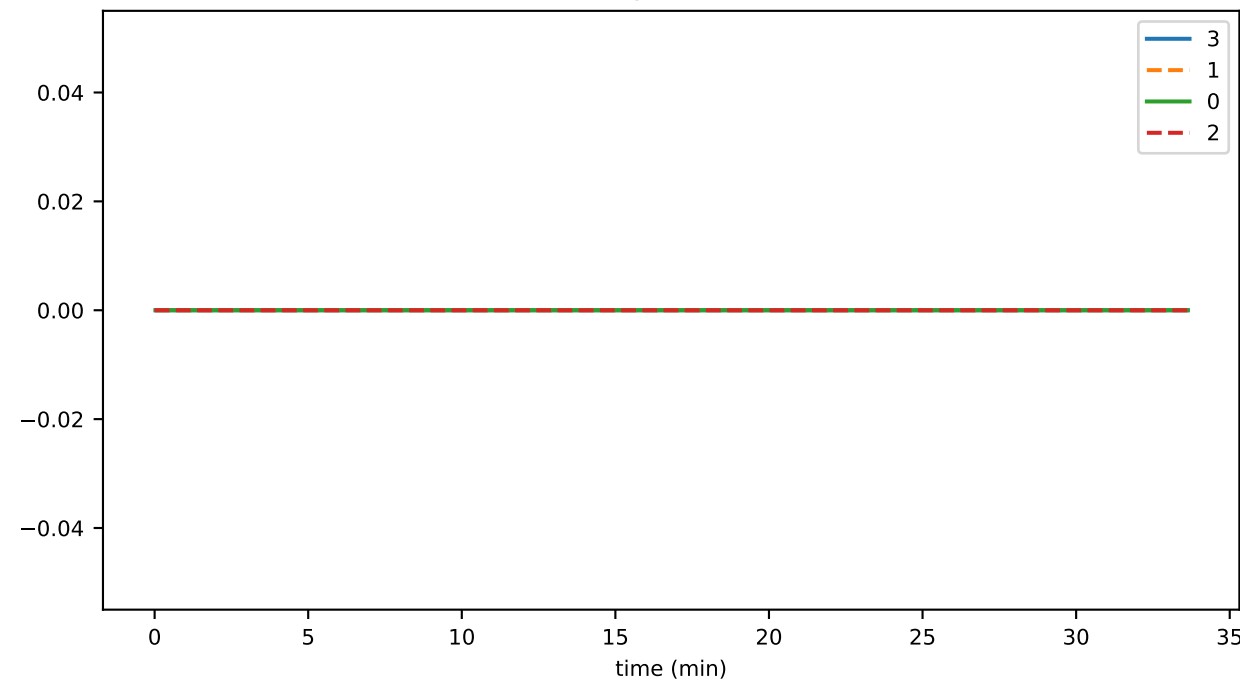
sigStateHash
