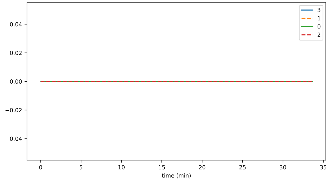
broadcastDisabledDueToOverload
