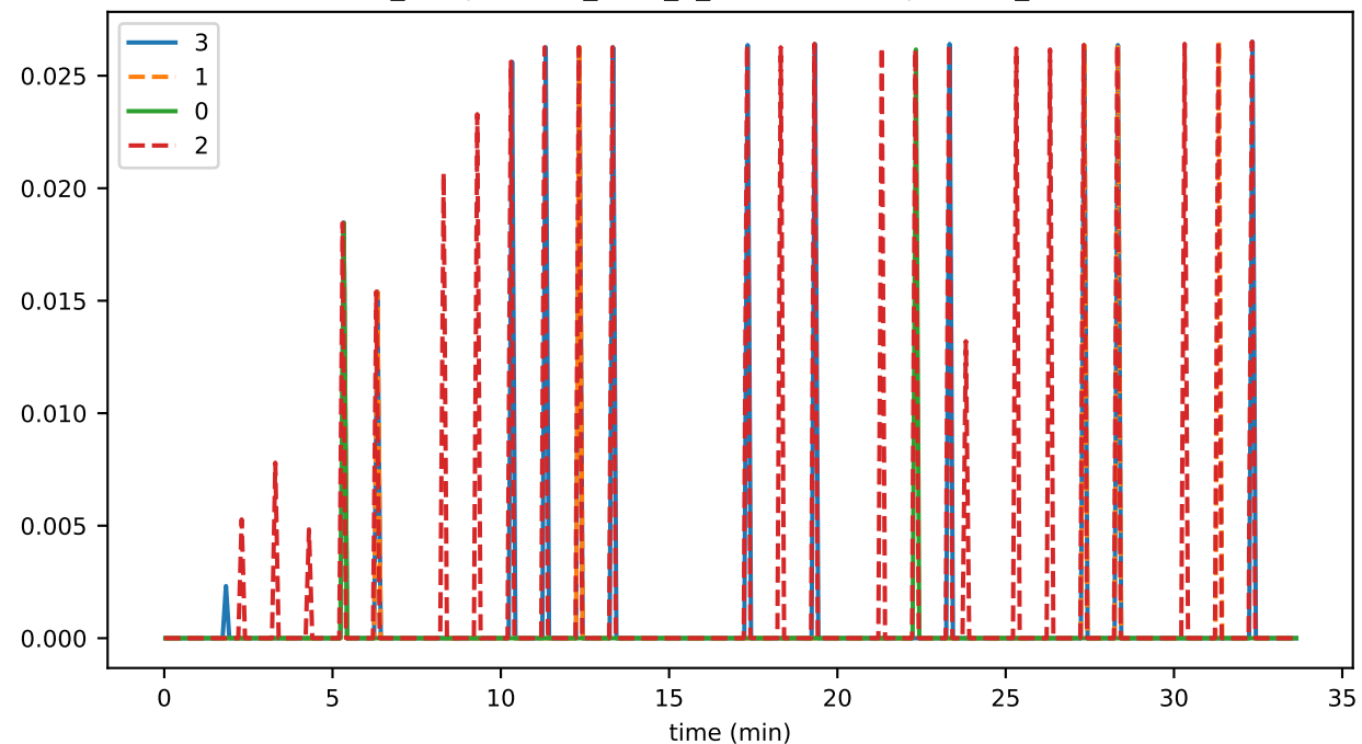
ds_compactions_level_2_hashesSavedSpaceMb_state
