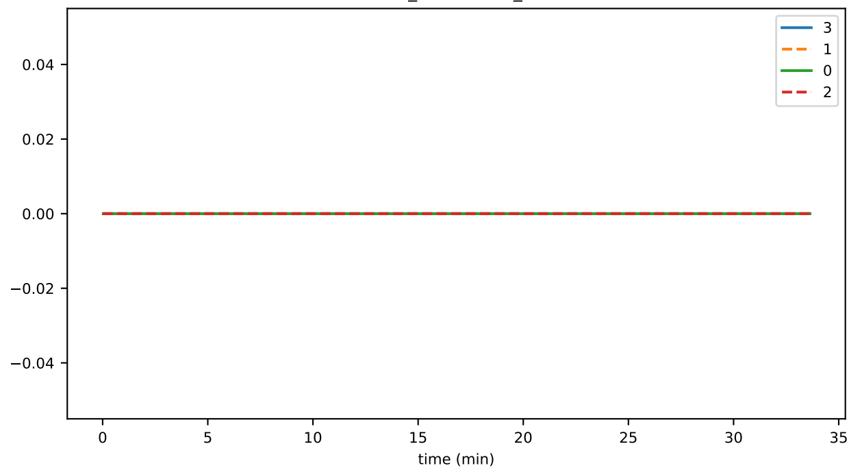
connSend_endStream_timeout
