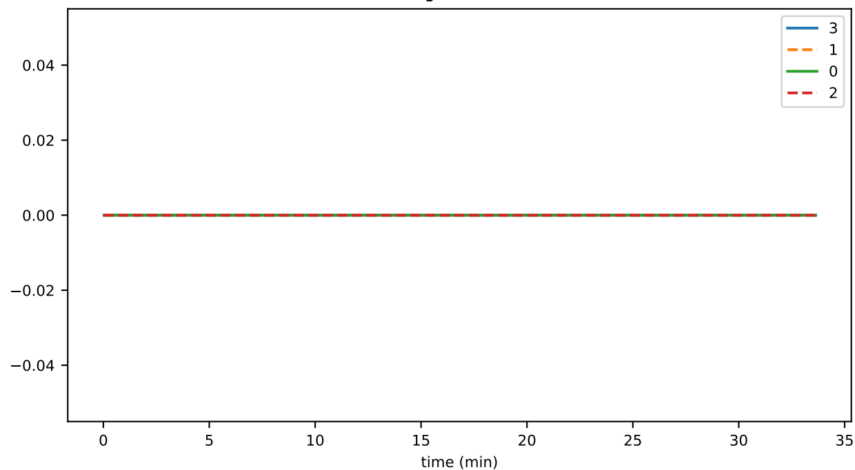
directMemPercent
