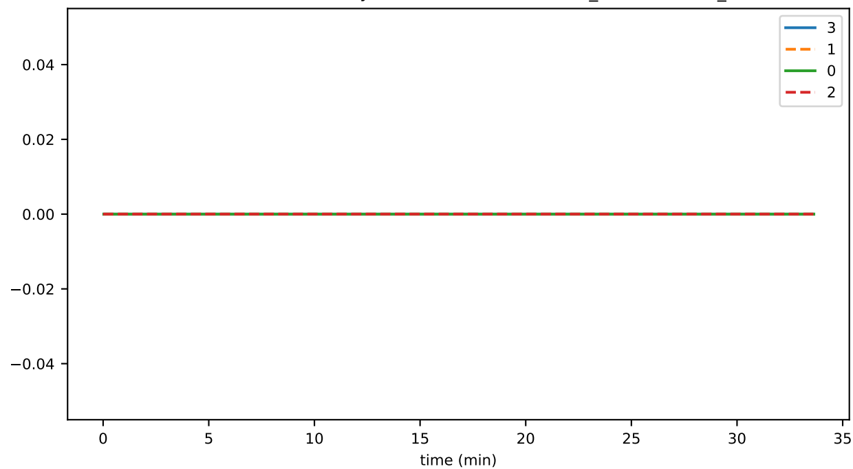
SmartContractService:SystemContractMethodCall_ASSOCIATION_total
