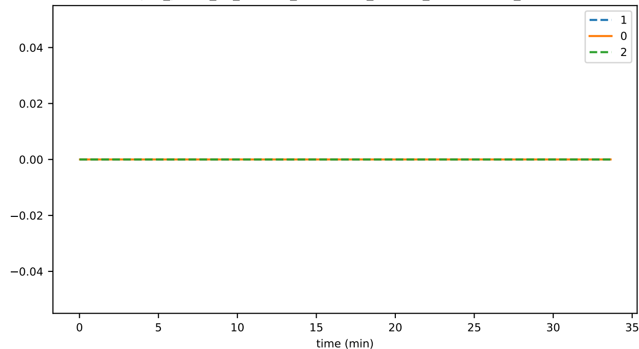
sync_phase_03_fraction_SELF_FALLEN_BEHIND
