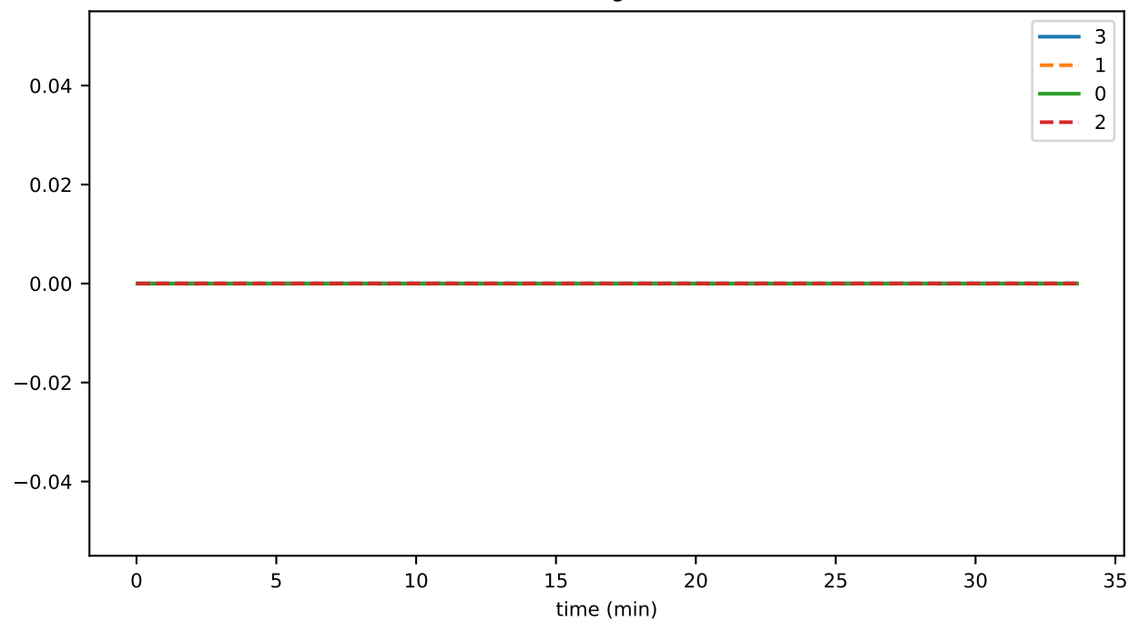
branchingEvents
