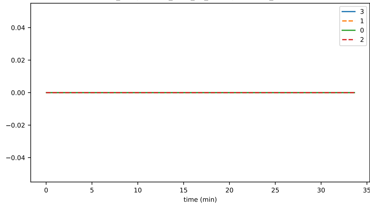
ds_compactions_level_10_leavesTimeMs_state
