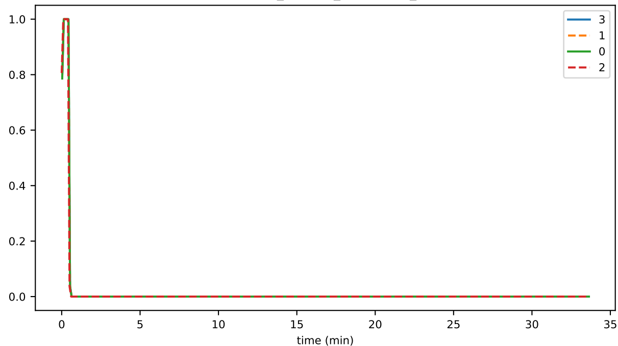
eventCreation_fraction_PLATFORM_STATUS
