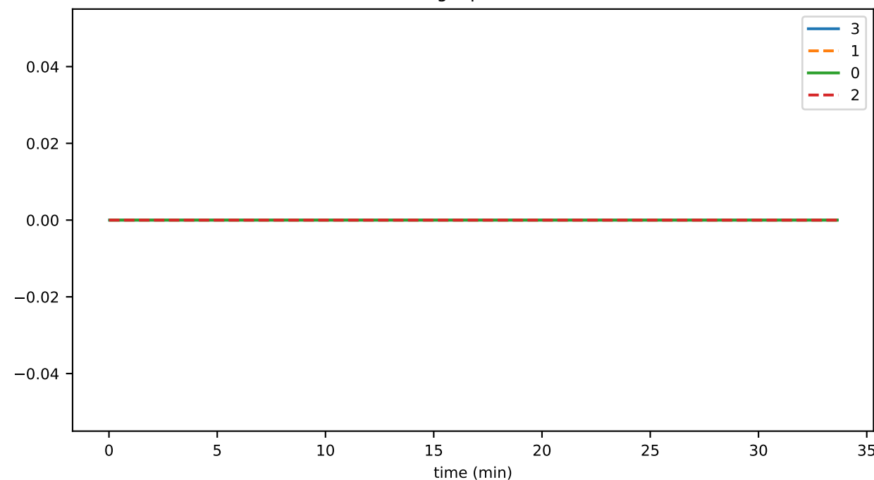
preconsensusEventAverageUnutilizedFileSpan
