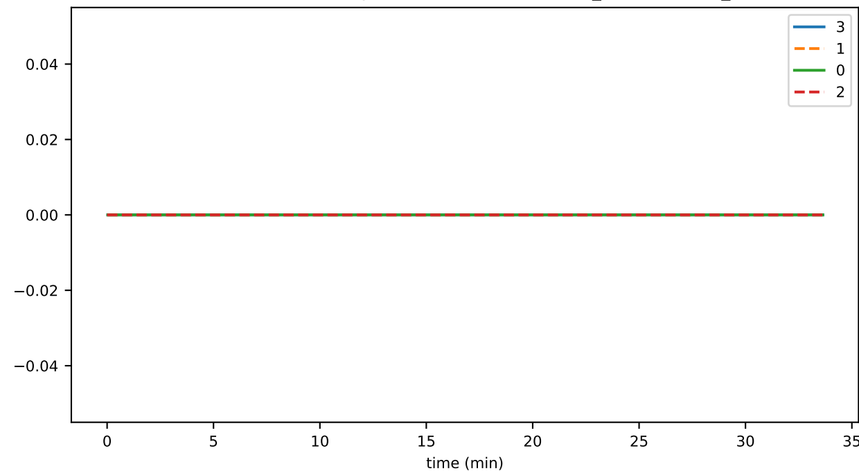
SmartContractService:SystemContractMethodCall_CREATE_DELETE_TOKEN_failed
