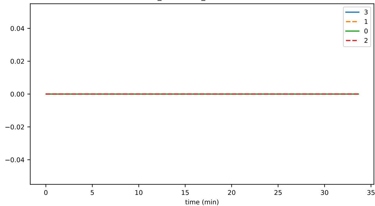
conn_connClose_newConnection
