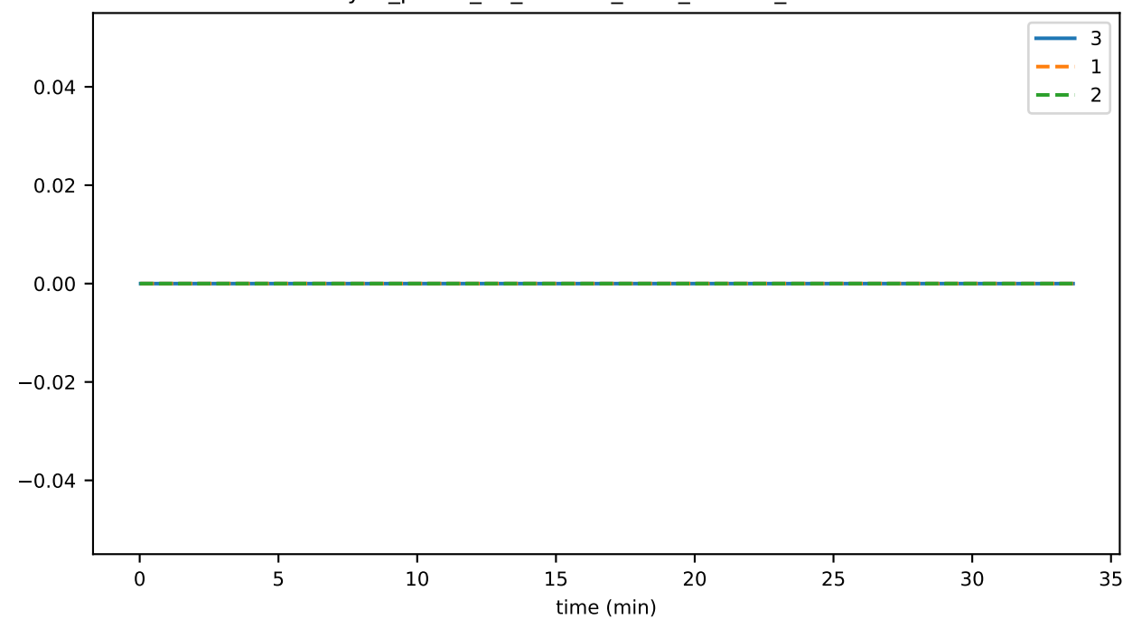
sync_phase_00_fraction_SELF_FALLEN_BEHIND
