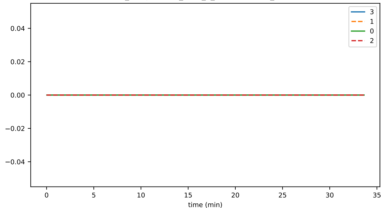
ds_compactions_level_10_hashesTimeMs_state
