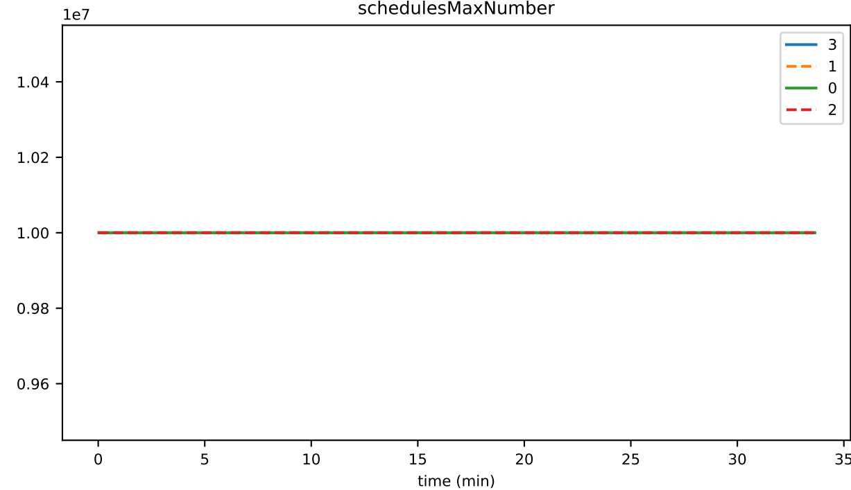
schedulesMaxNumber
