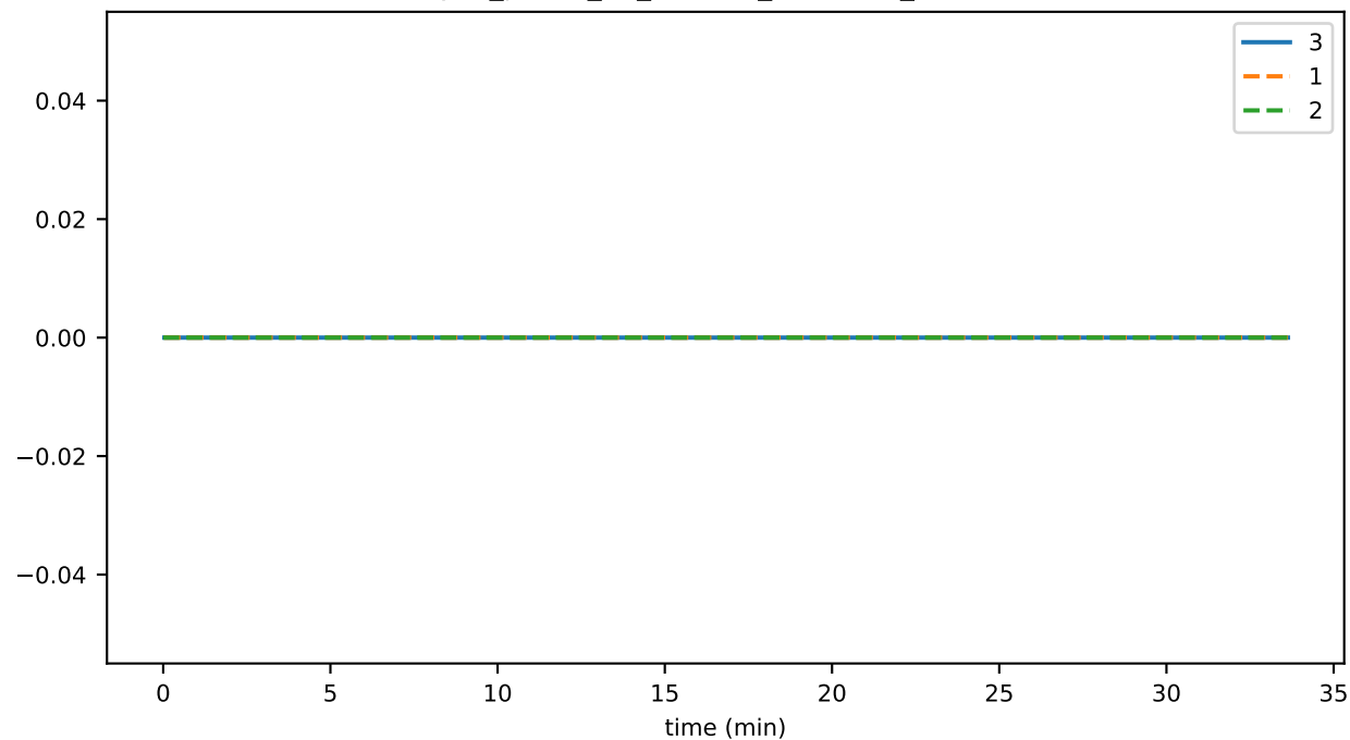
sync_phase_01_fraction_EXCHANGING_TIPS
