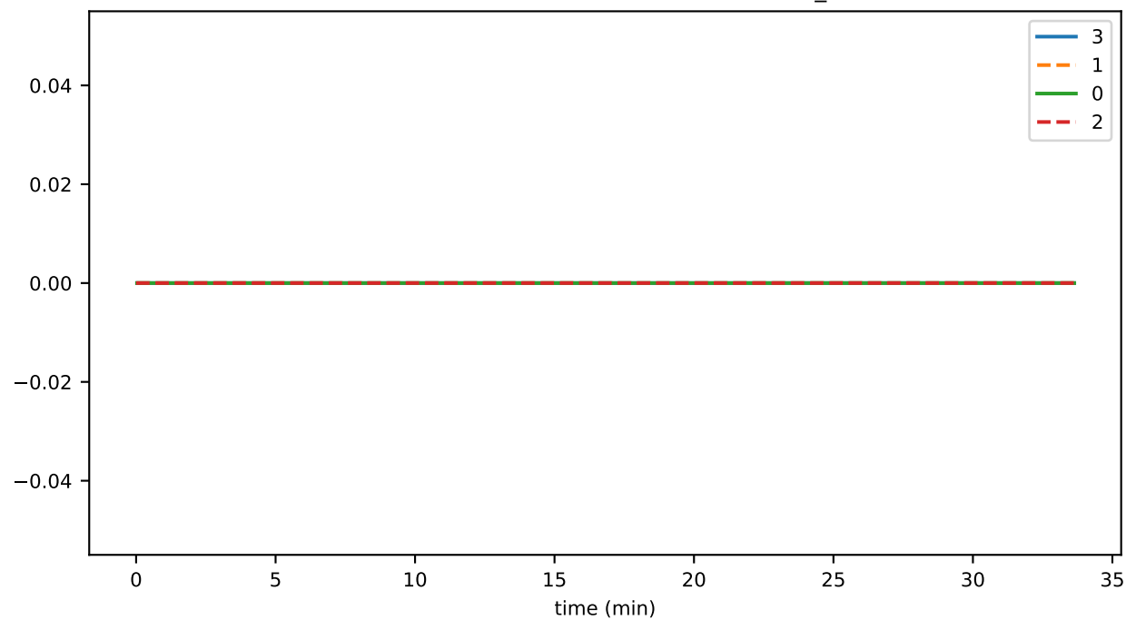
SmartContractService:TransactionDuration_count
