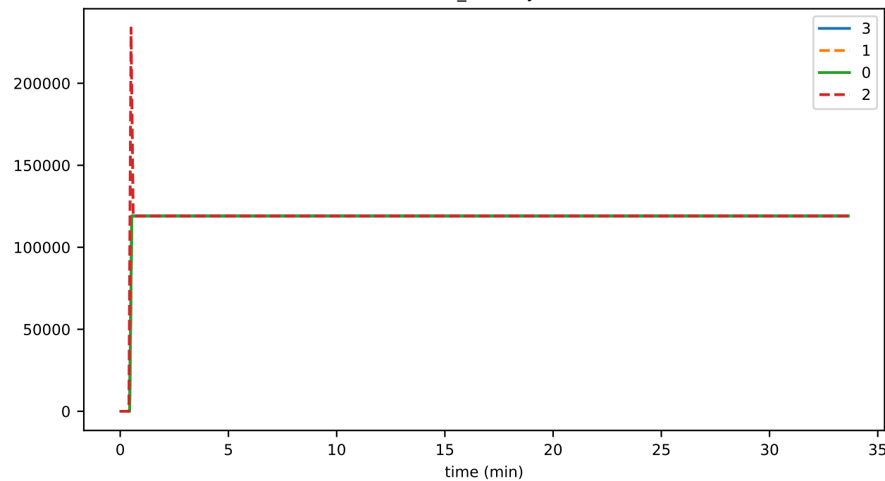
buffer_blockBytes
