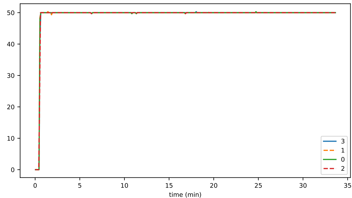
buffer_backPressureState
