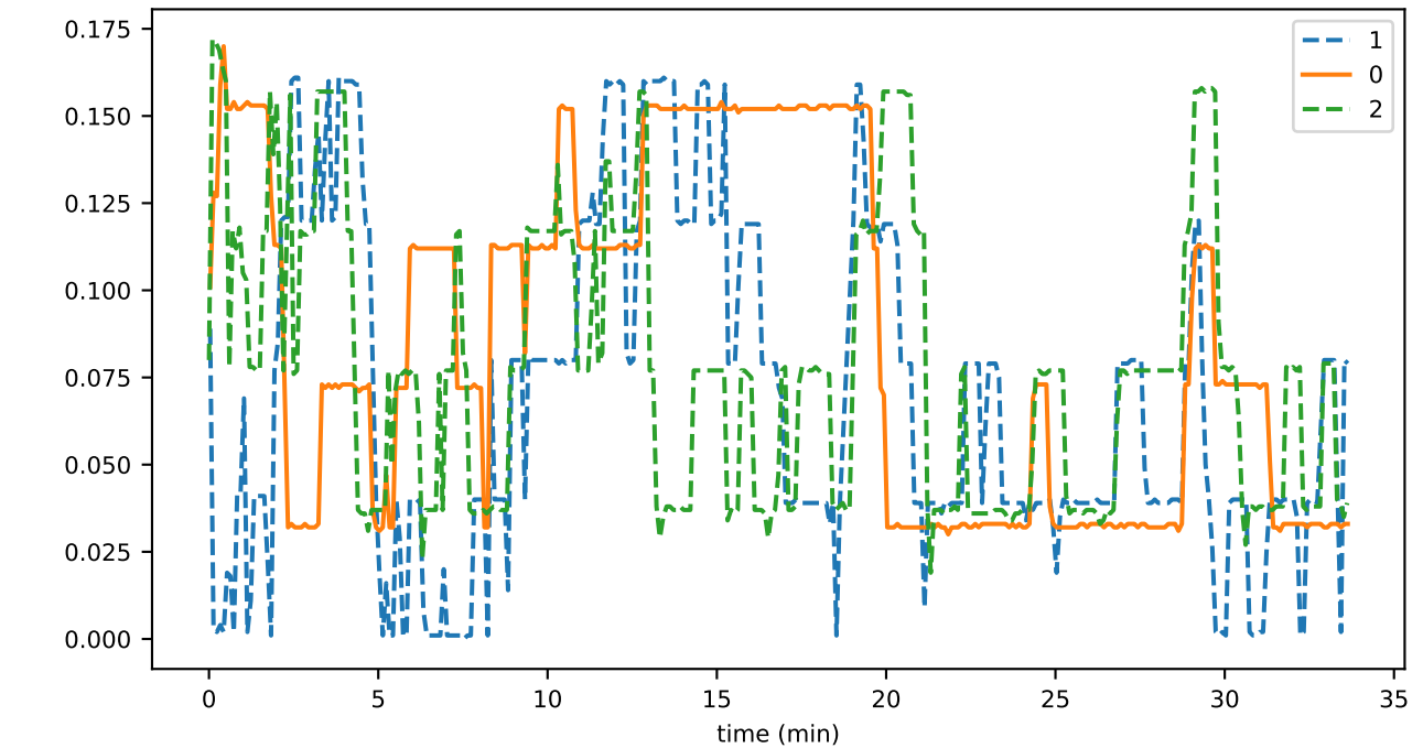
sync_phase_03_fraction_EXCHANGING_WINDOWS
