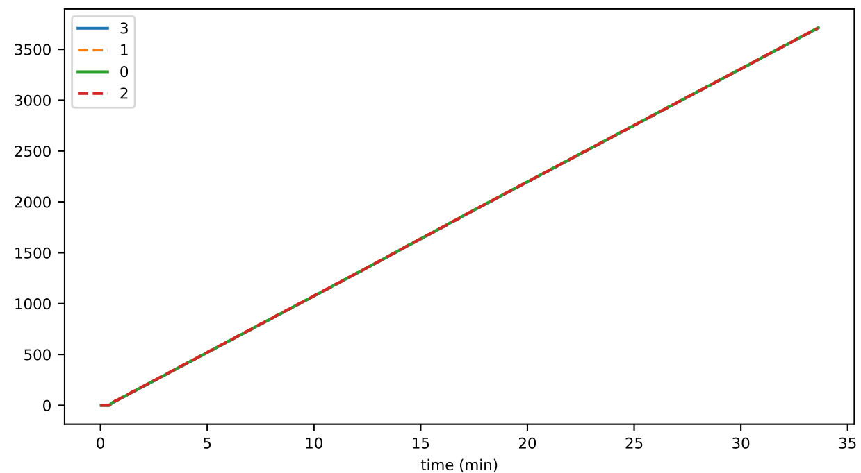
trans_per_sec
