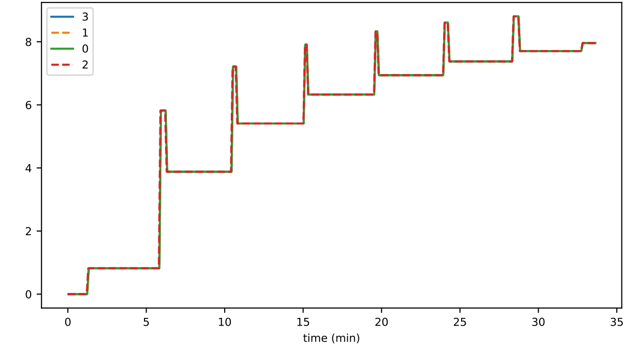
preconsensusEventFileOldestIdentifier
