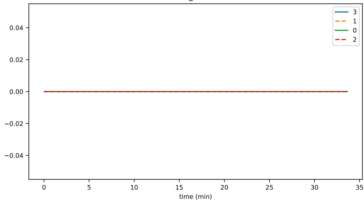
conn_pipelineOperationTimeout
