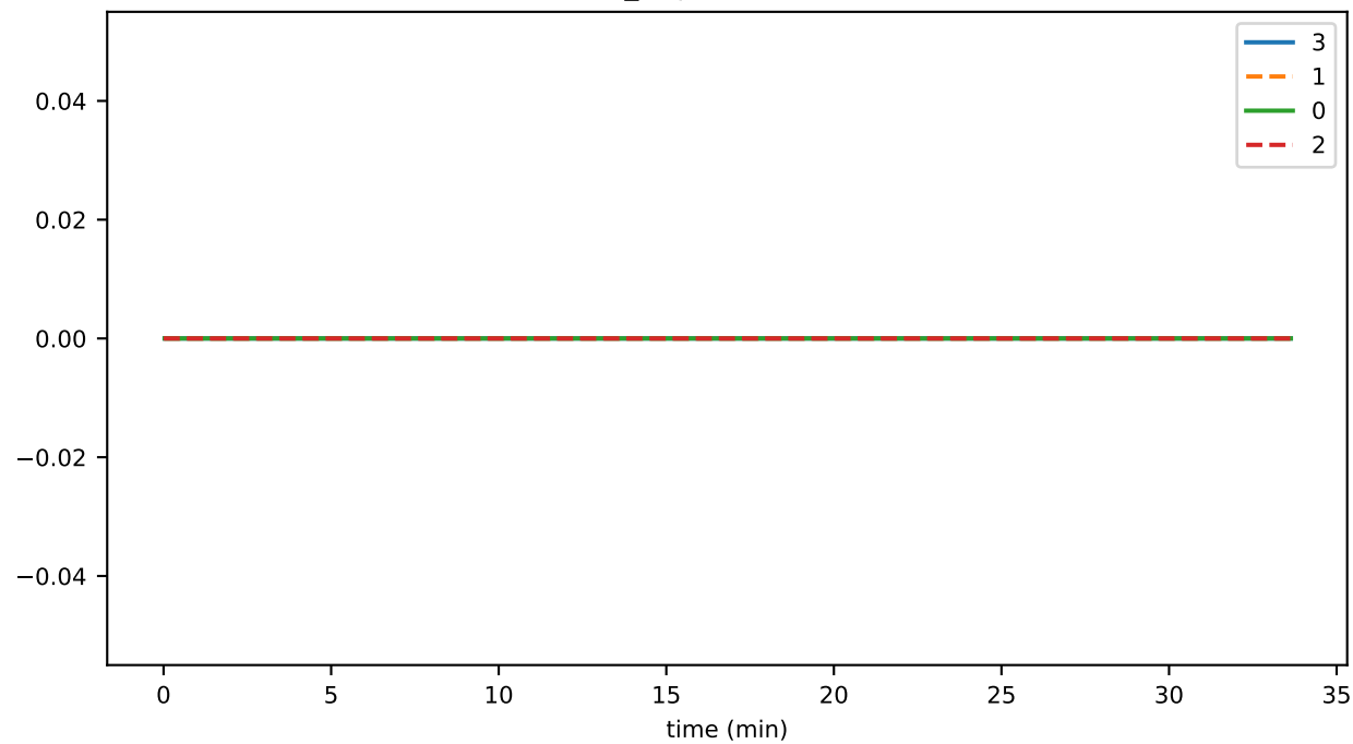
connSend_requestExceedsHardLimit
