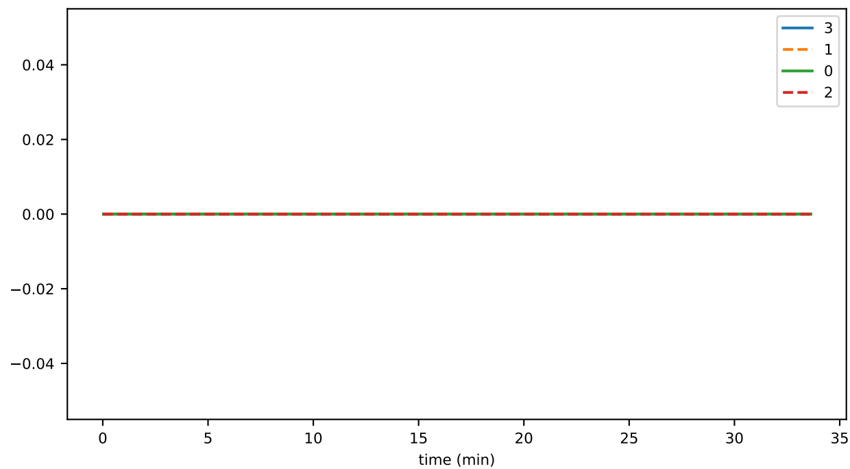
nodesPercentUsed
