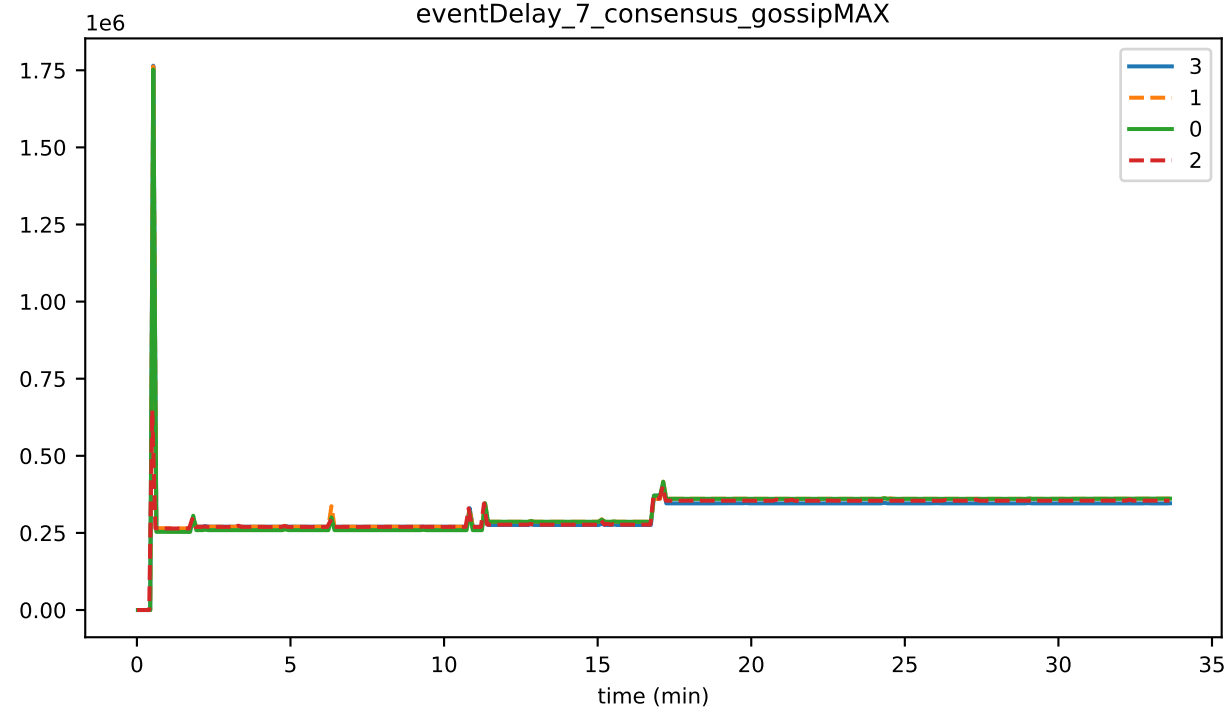
eventDelay_7_consensus_gossipMAX
