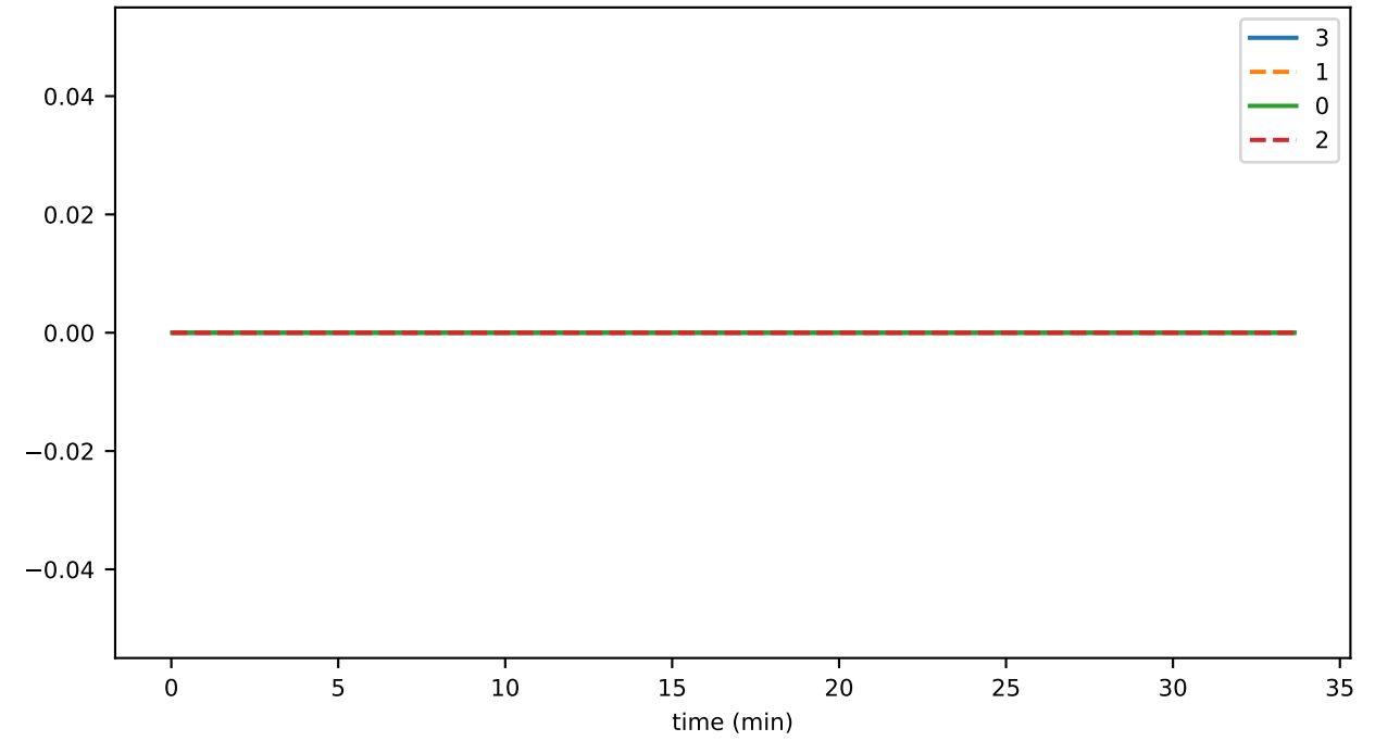
roundIncEqParents
