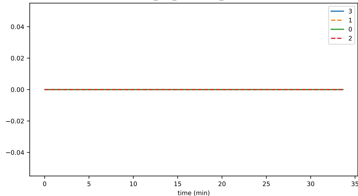
ds_flushes_hashesWritten_state
