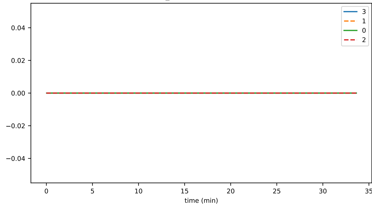
connRecv_latestBlockResendBlock
