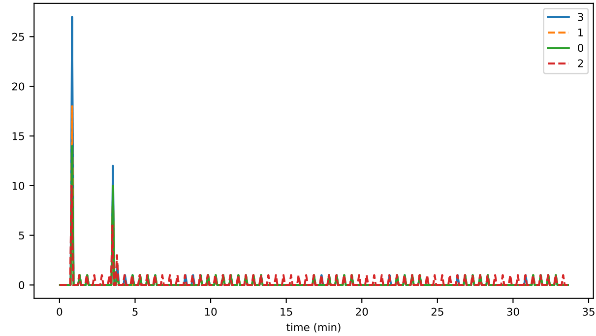
dupEvPercent
