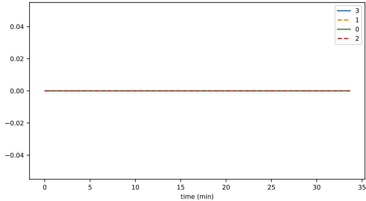
ds_compactions_level_8_leavesTimeMs_state
