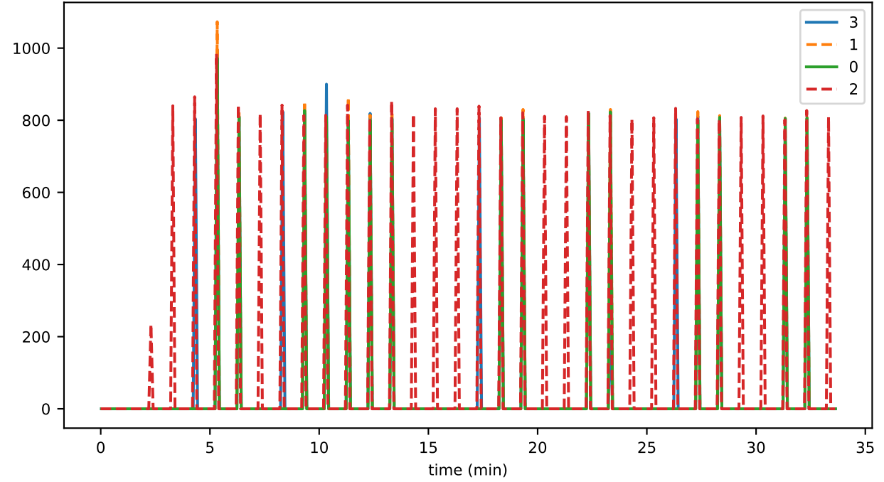
ds_compactions_level_1_leafKeysTimeMs_state
