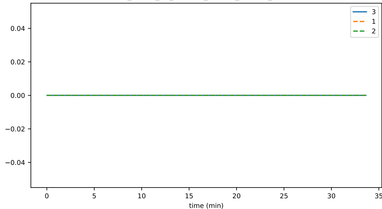
sync_phase_00_fraction_OTHER_FALLEN_BEHIND
