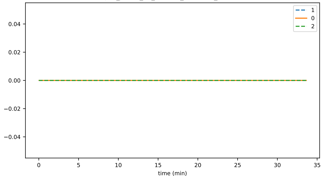
syncIndicatorDiff
