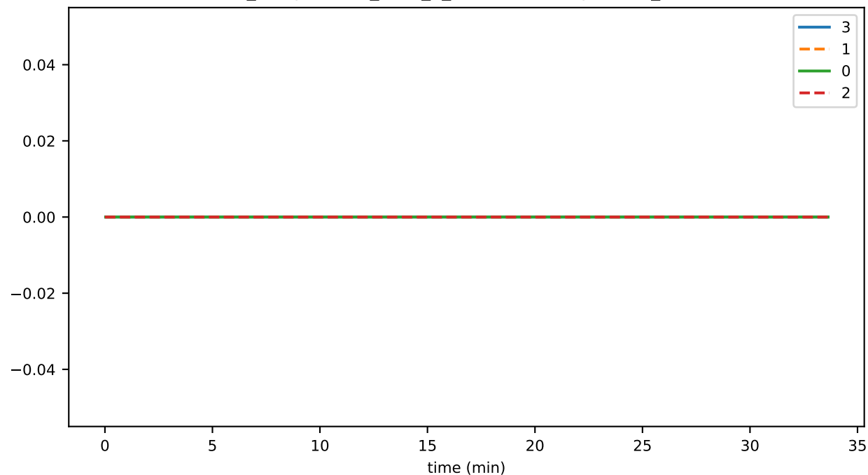
ds_compactions_level_5_leafKeysSavedSpaceMb_state
