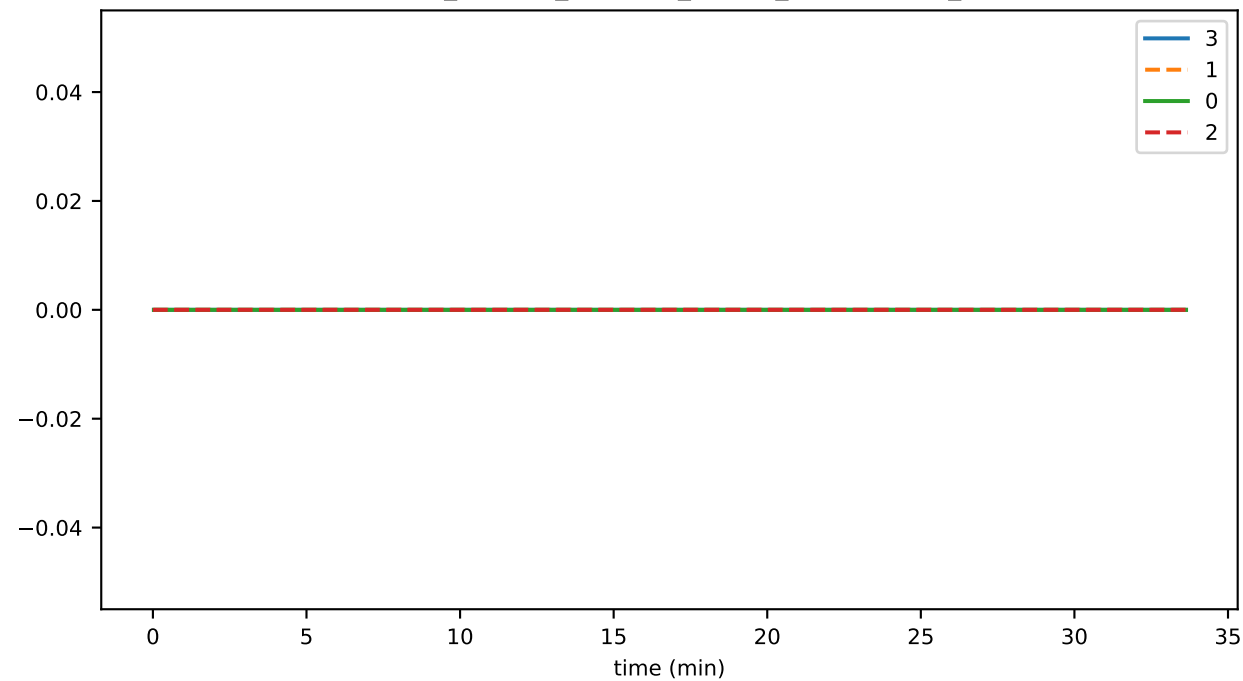
consensus_fraction_SETTING_EVENT_CONSENSUS_DATA
