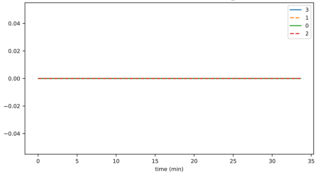
SmartContractService:TransactionGasUsed_sum
