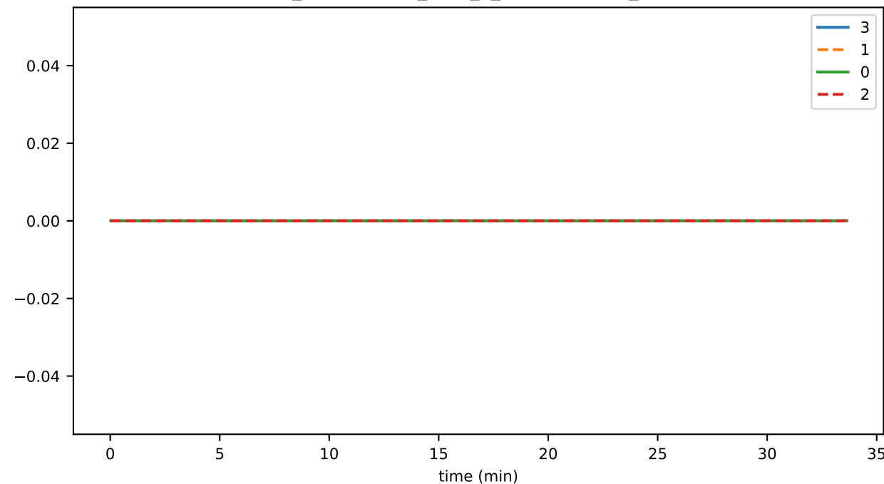
ds_compactions_level_2_leavesTimeMs_state
