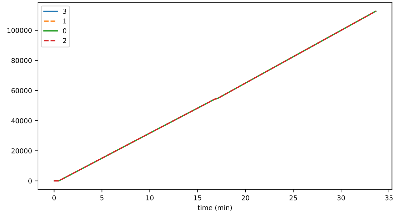
roundIncEqParents
