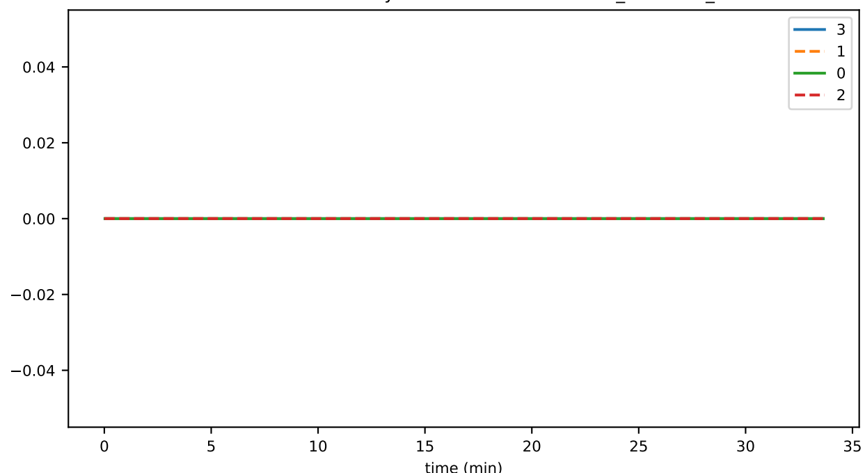
SmartContractService:SystemContractMethodCall_AIRDROP_total
