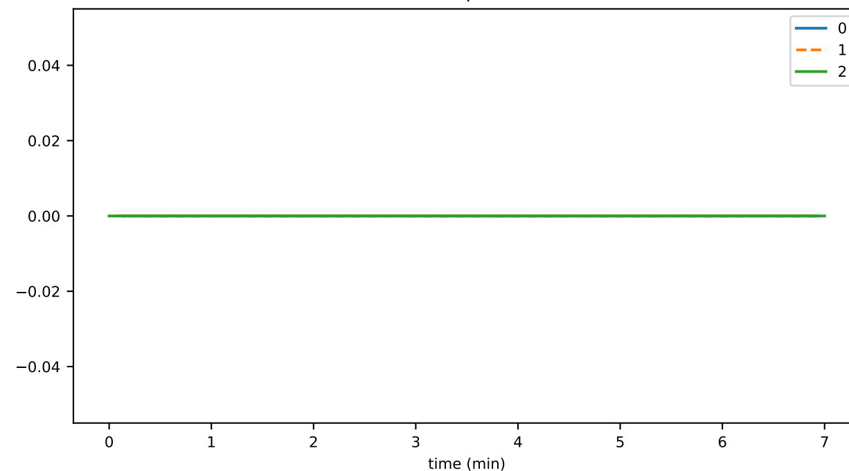
tokenAirdropDurationMax
