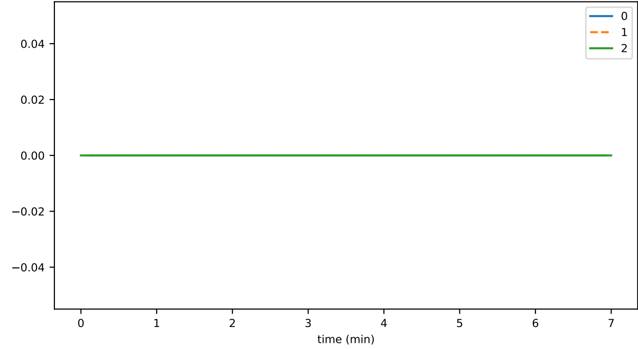
ds_files_level_0_leavesFileSizeByLevelMb_state
