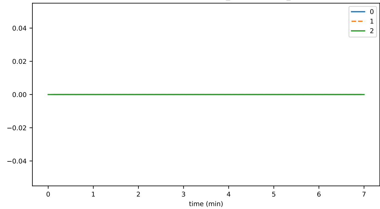
SmartContractService:Rejected_contractCallTx_total
