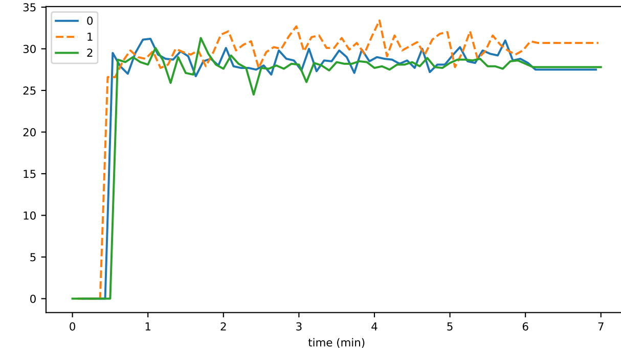
eventsFailedSignatureValidation
