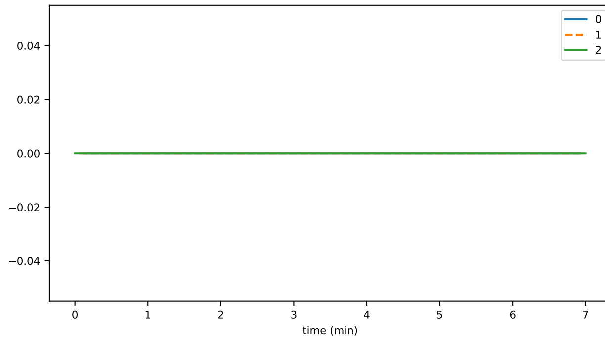
ev_per_syncRMAX
