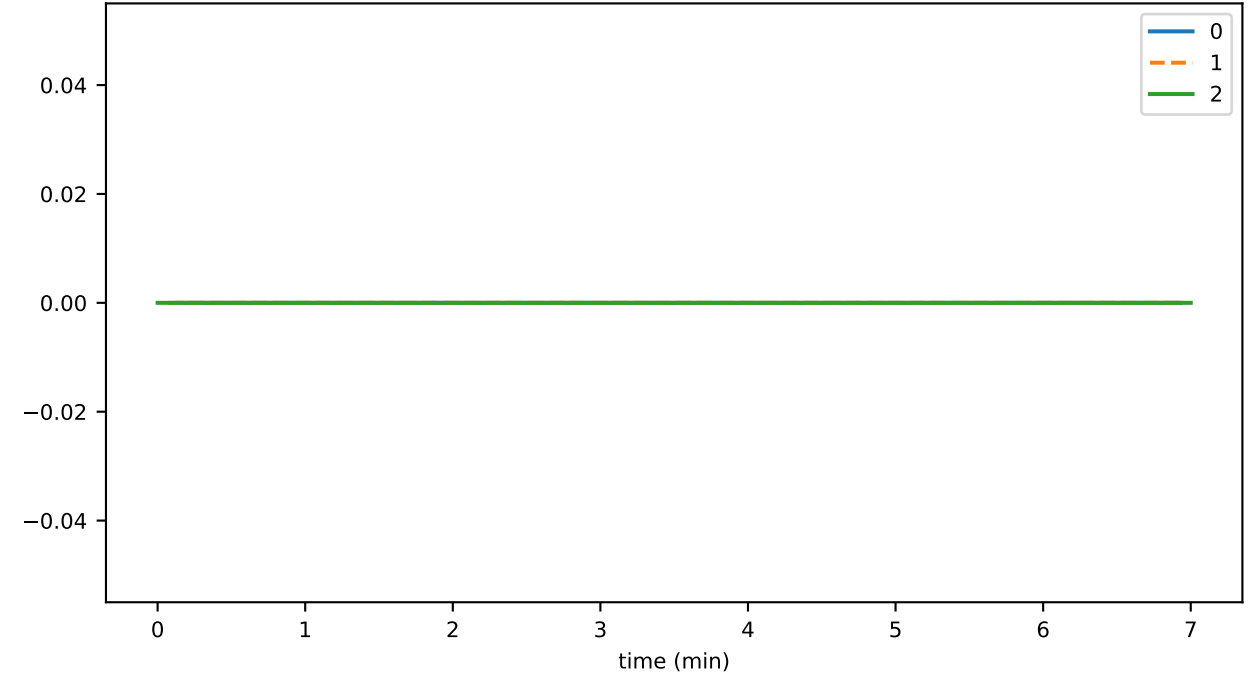
receiverReconnectDurationSeconds
