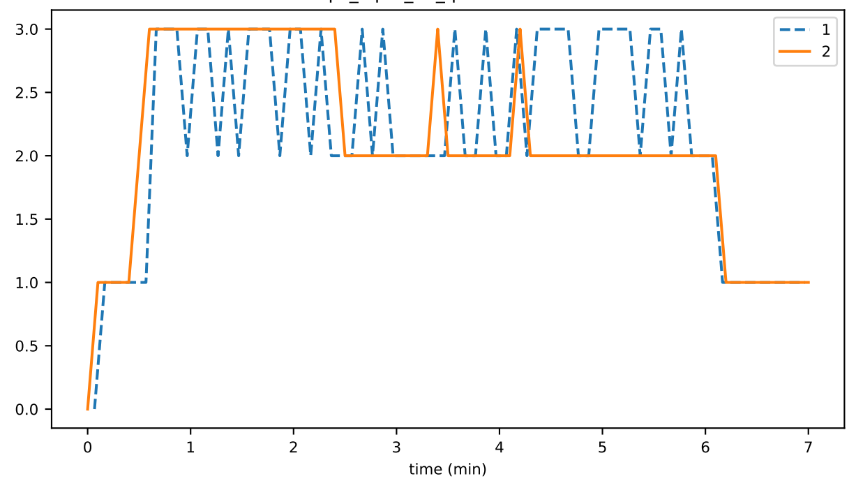
rpc_input_00_queueMaxSize
