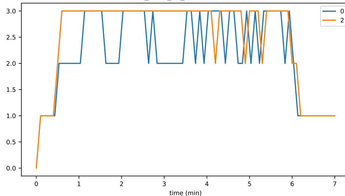
rpc_input_02_queueMaxSize
