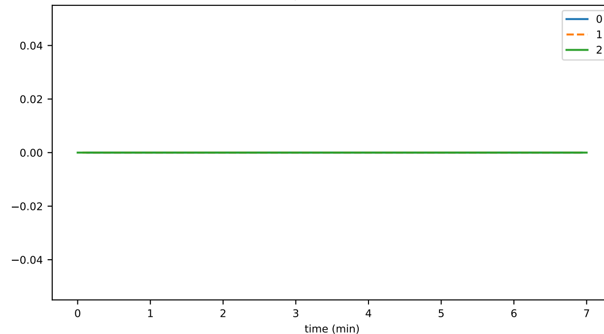
NonGovernanceOversizedTxnsRcv
