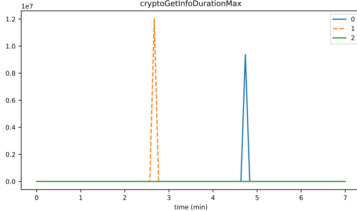
cryptoGetInfoDurationMax
