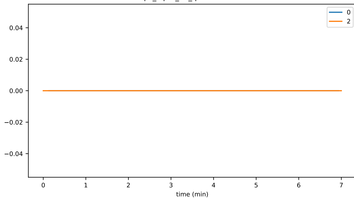
rpc_input_01_queueMinSize
