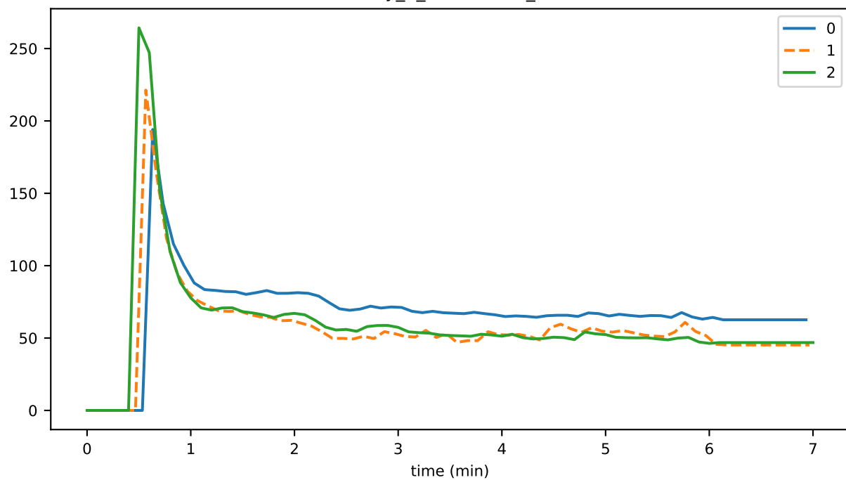
eventDelay_4_verification_runtime
