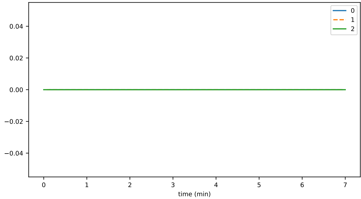
registeredNodeUpdateDurationMax
