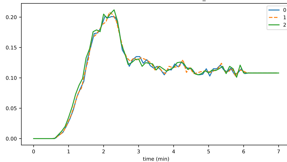
roundsSinceLastConsensusEvent_0
