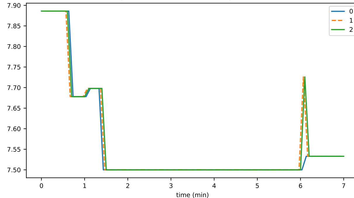
preconsensusEventFileOldestIdentifier
