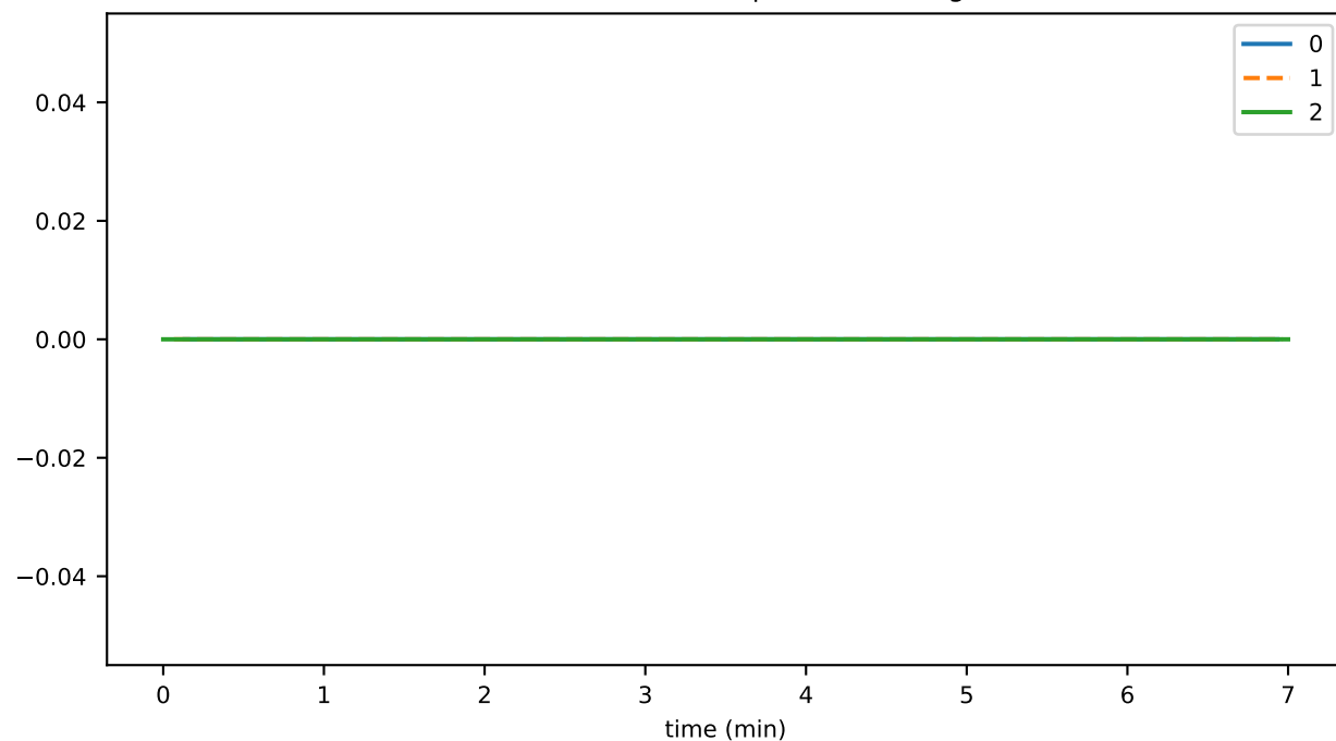
consensusDeleteTopicDurationAvg
