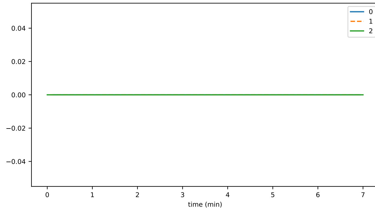
cryptoGetLiveHashThrottledTxns
