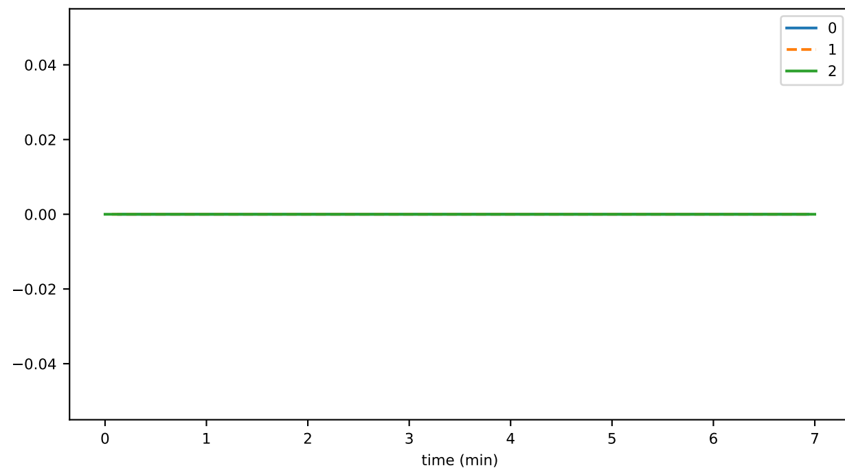
scheduleGetInfoDurationAvg
