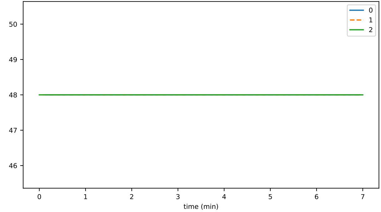
receiverReconnectDurationSeconds
