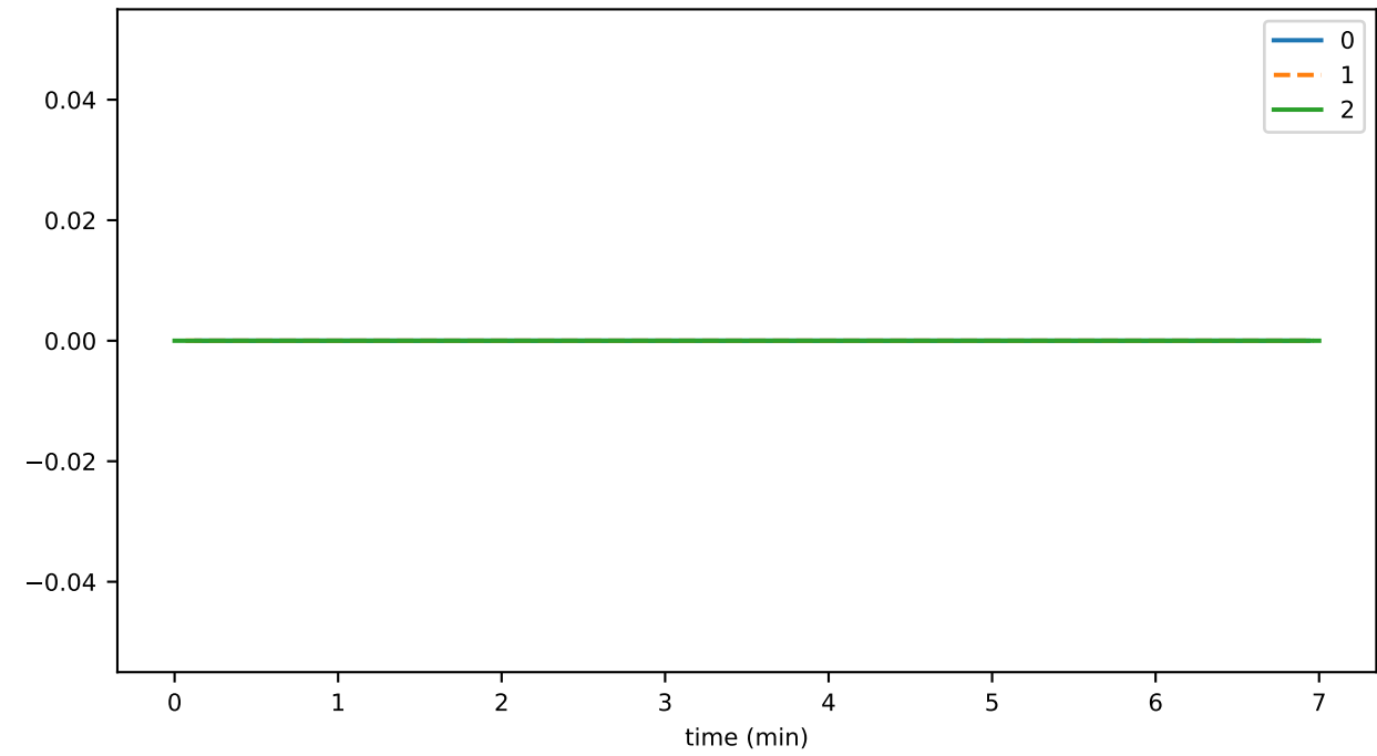
ds_compactions_level_2_hashesSavedSpaceMb_state
