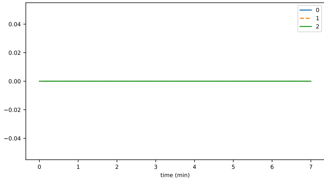
registeredNodeDeleteDurationAvg
