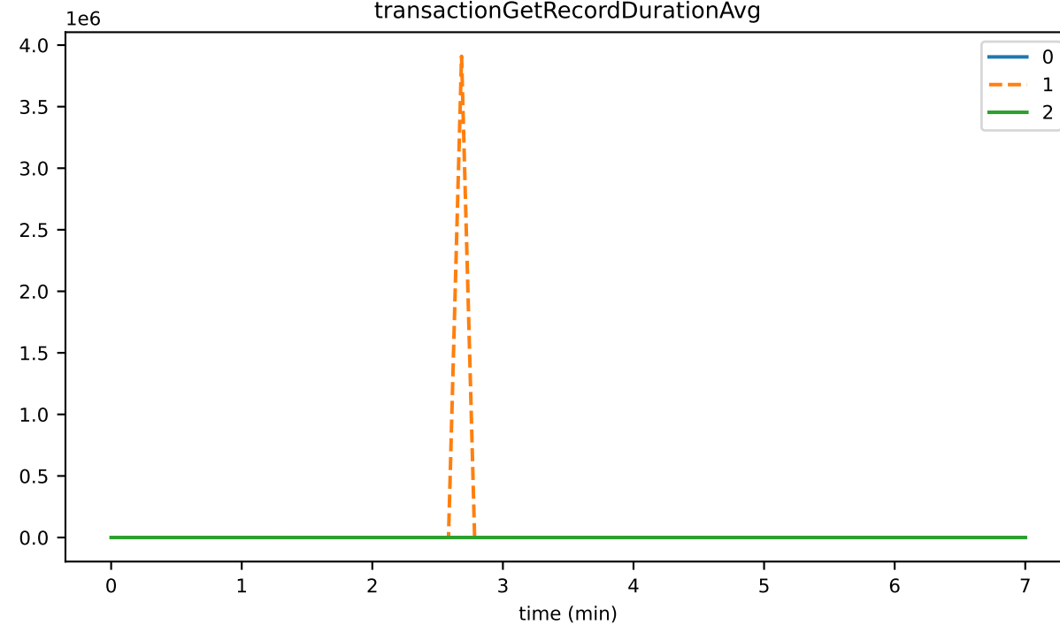
transactionGetRecordDurationAvg
