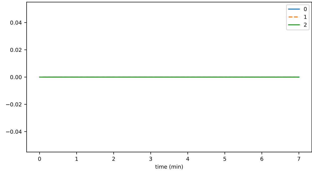
syncPermitsAvailable
