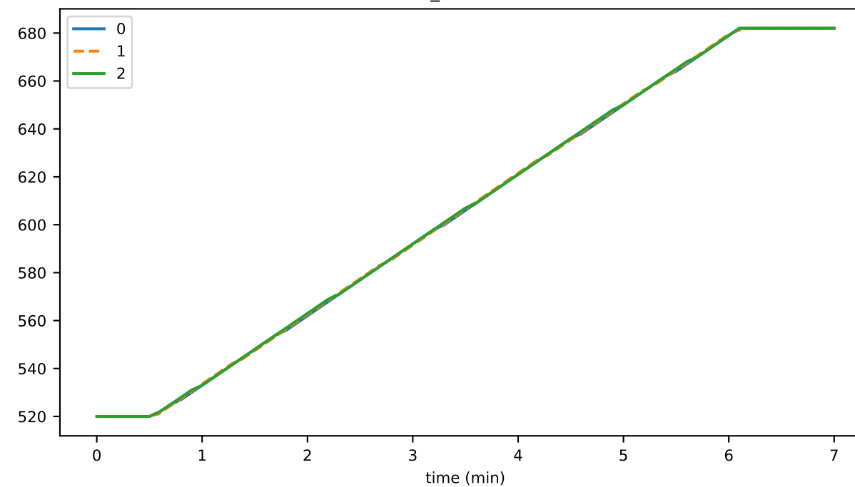
buffer_newestBlock
