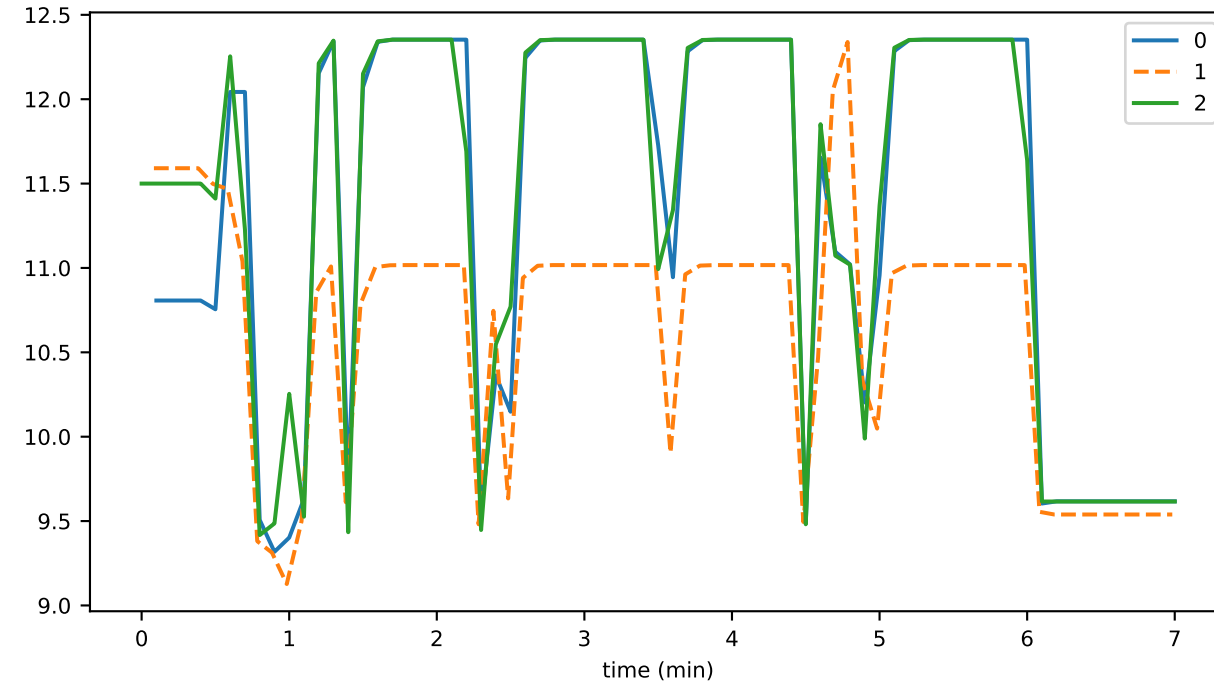
numEventsAddedUntilConsensus
