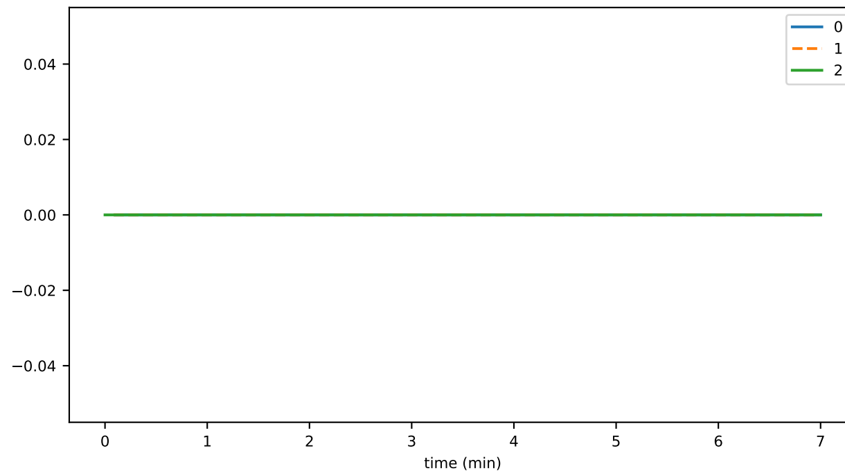
numVotingRounds
