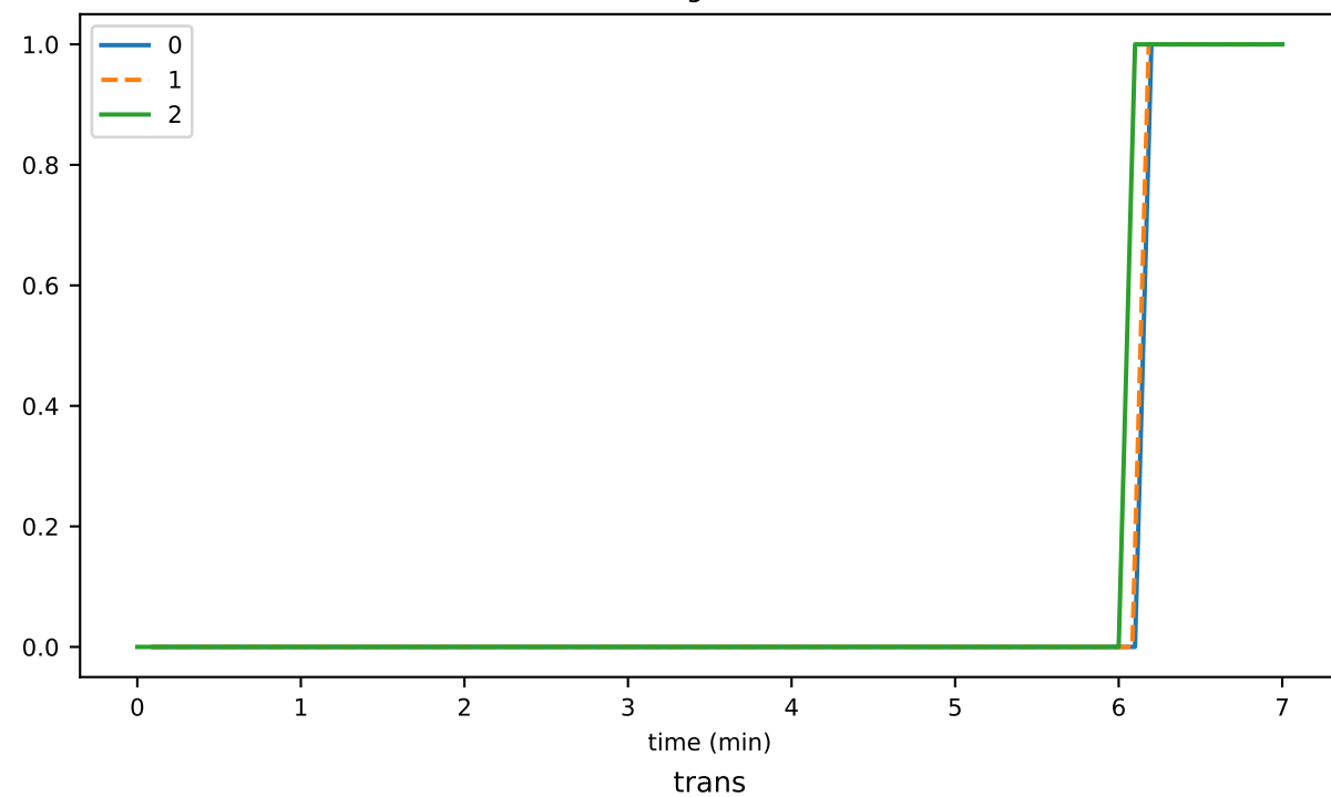
totalNeverSignedDiskStates
