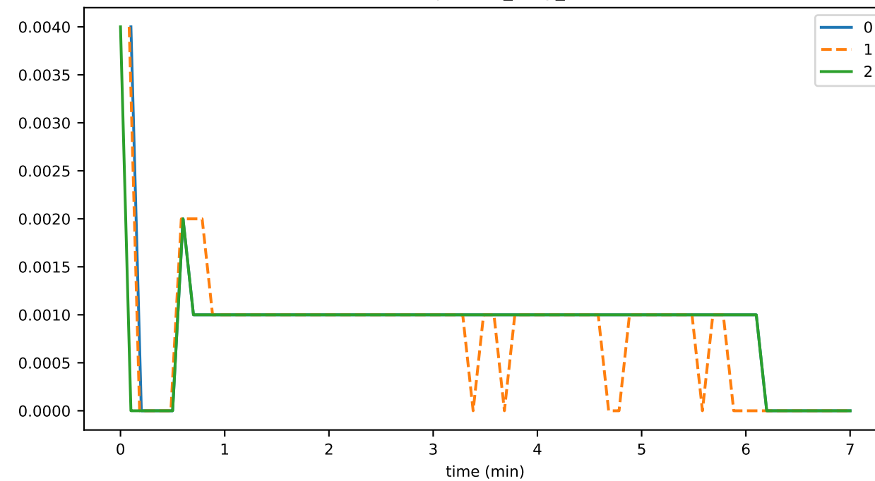
eventDelay_1_eventCreation_runtime
