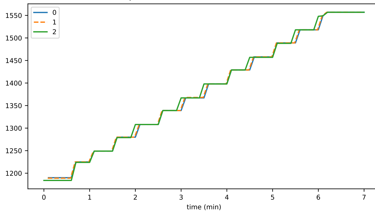
preconsensusEventFileOldestSeconds
