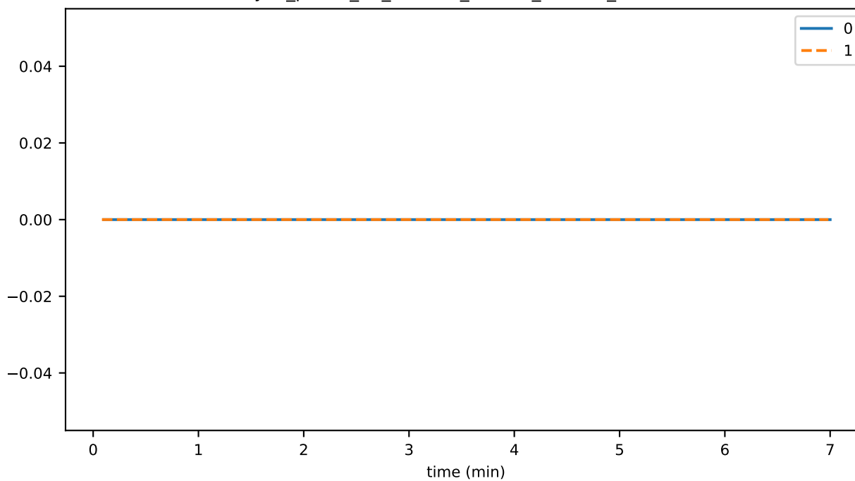
sync_phase_02_fraction_OTHER_FALLEN_BEHIND
