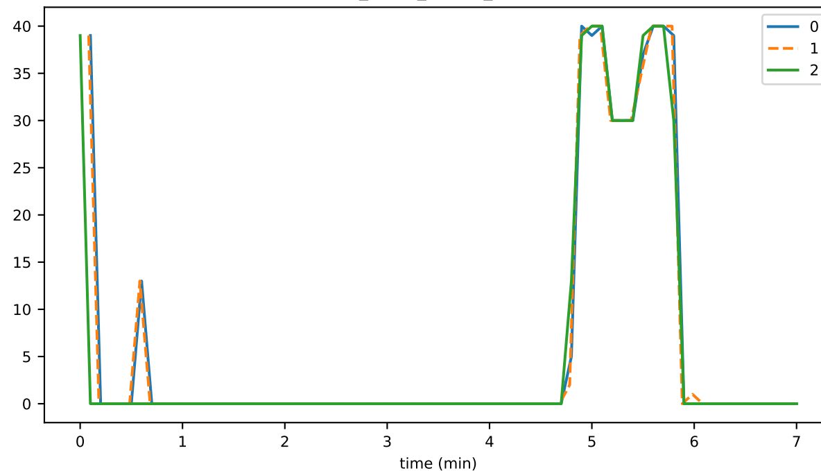
ds_reads_leaves_state
