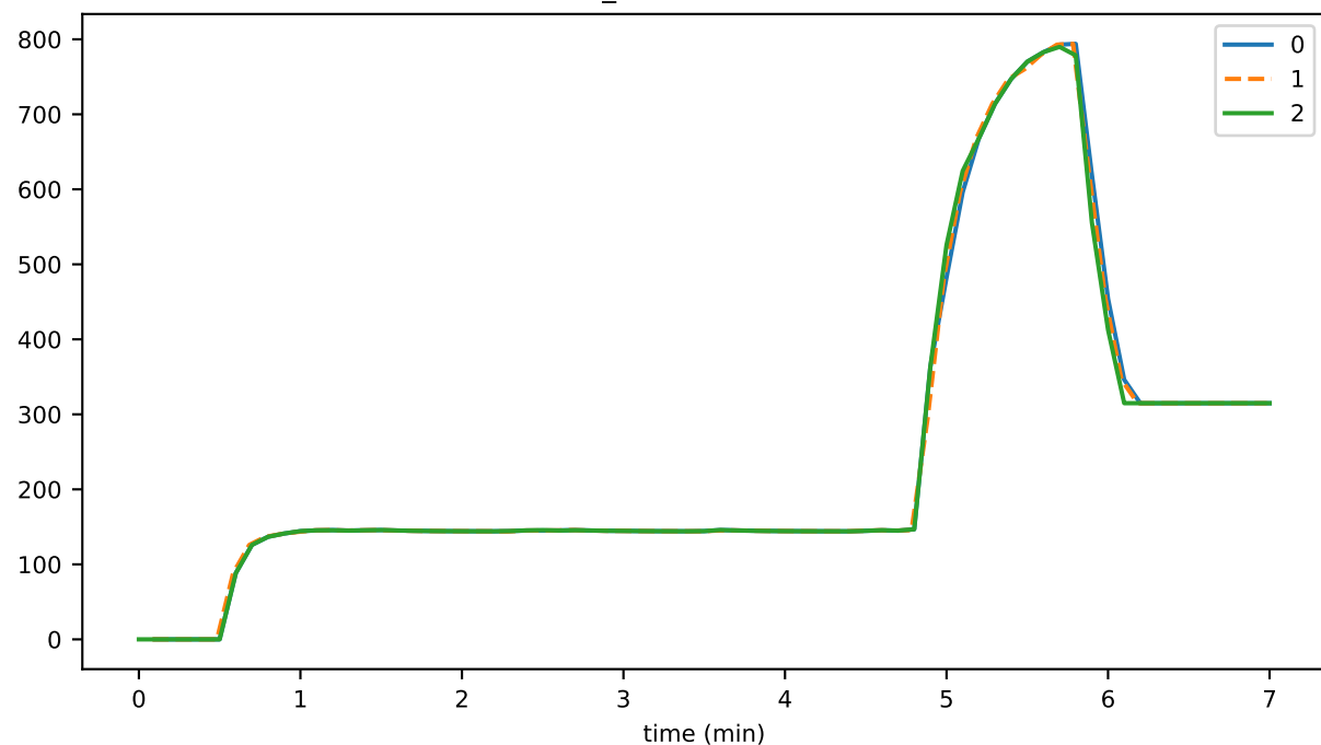
buffer_latestBlockOpened
