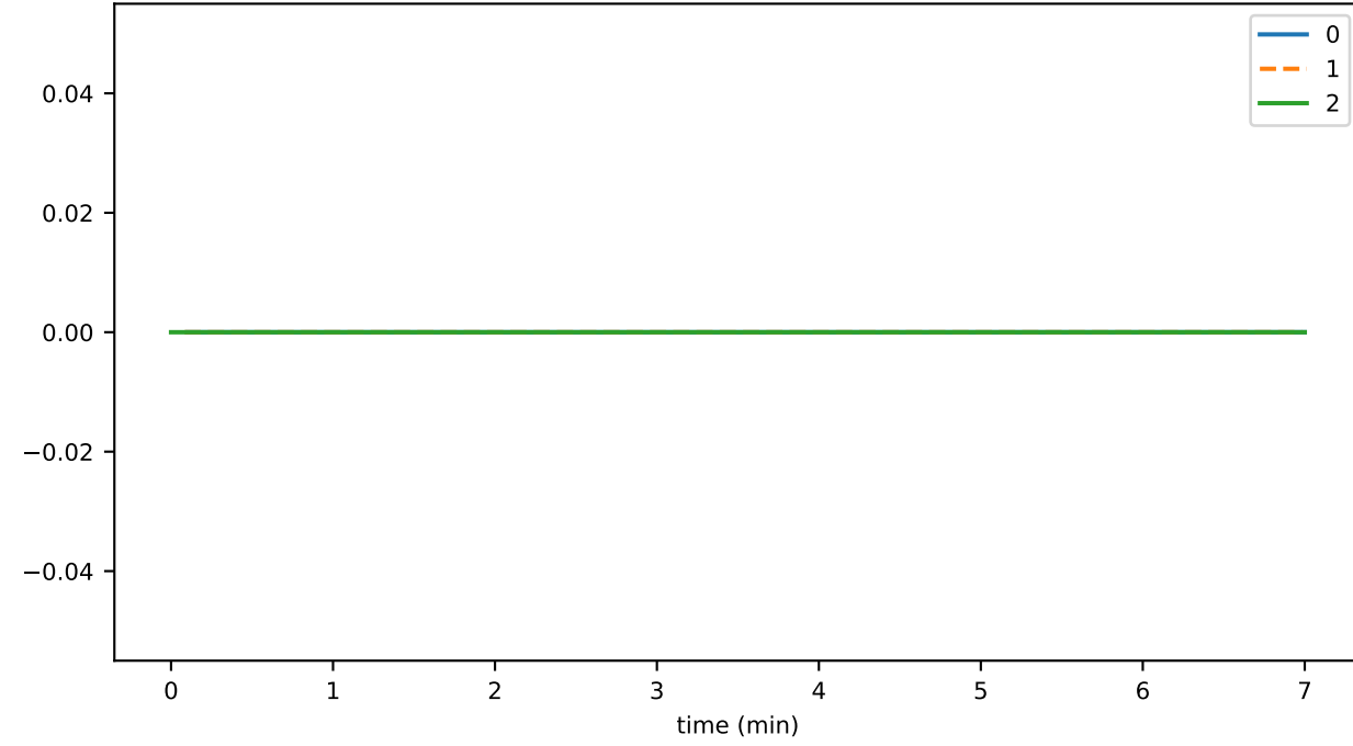
SmartContractService:SuccessfulTransactionDuration_avg
