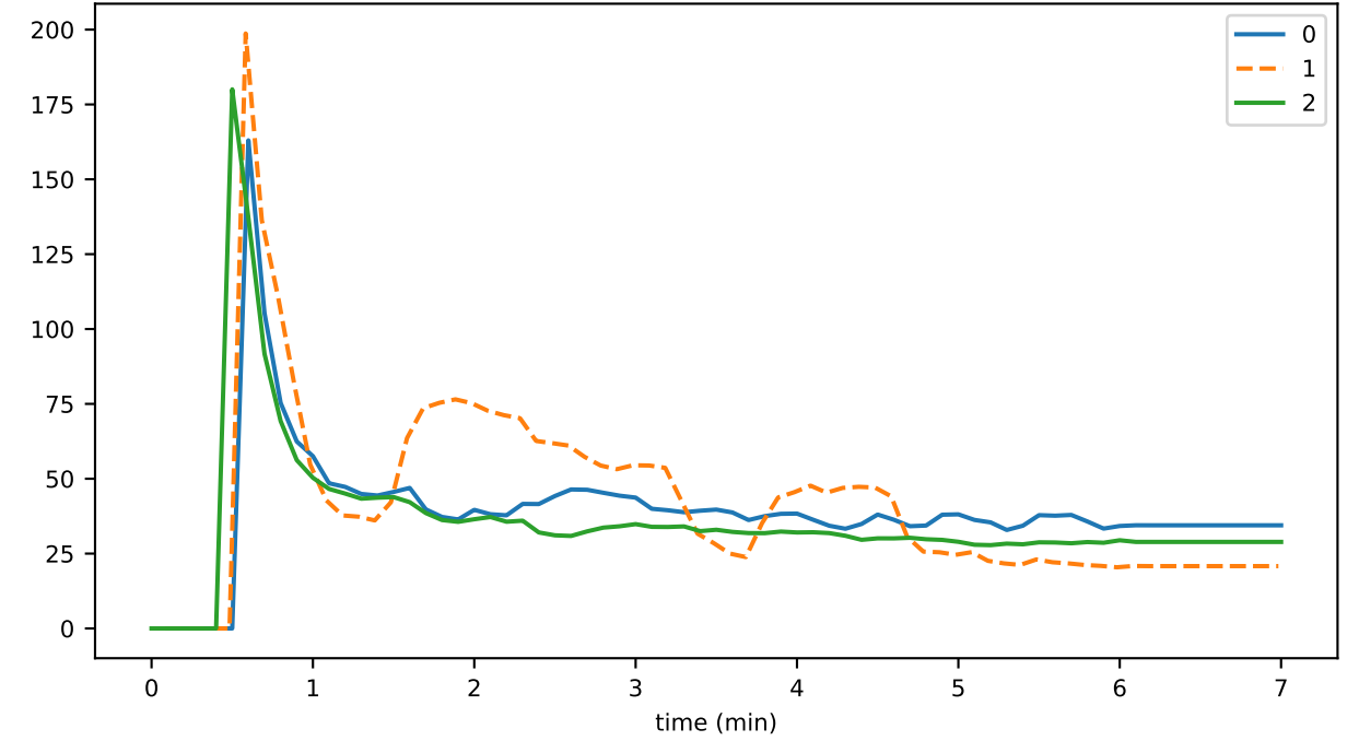
eventDelay_2_validation_runtime
