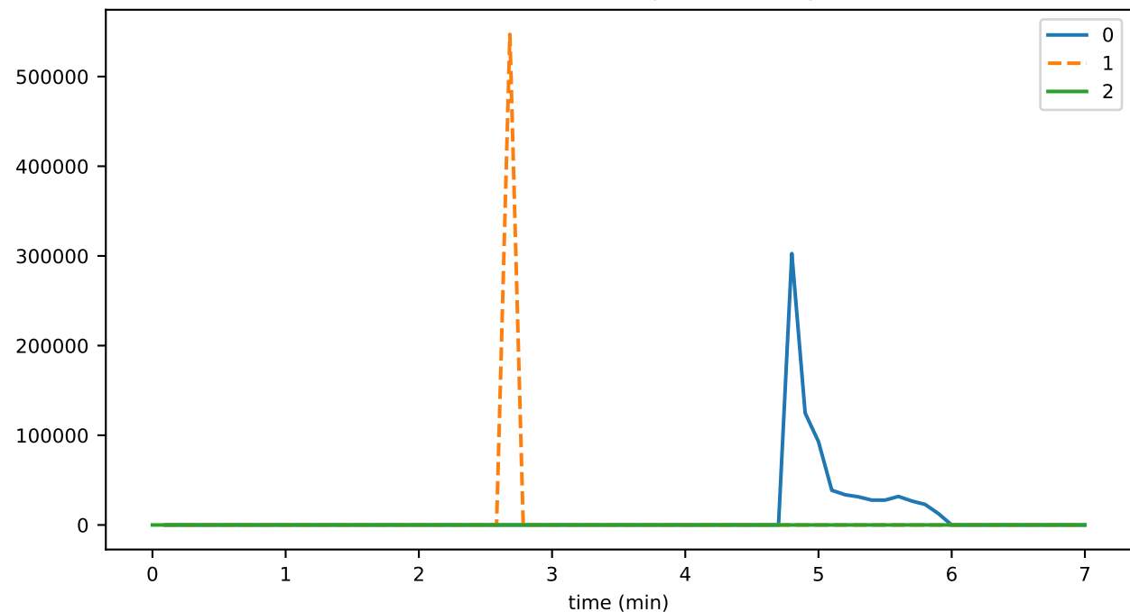
transactionGetReceiptThrottledTxns
