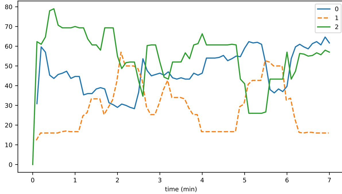
doNotSyncRemoteProcessingEvents
