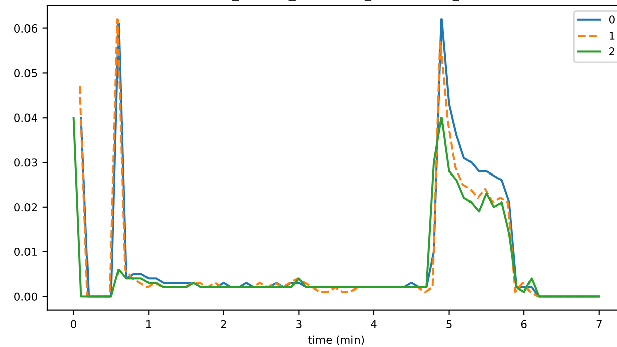
consensus_fraction_SETTING_EVENT_CONSENSUS_DATA
