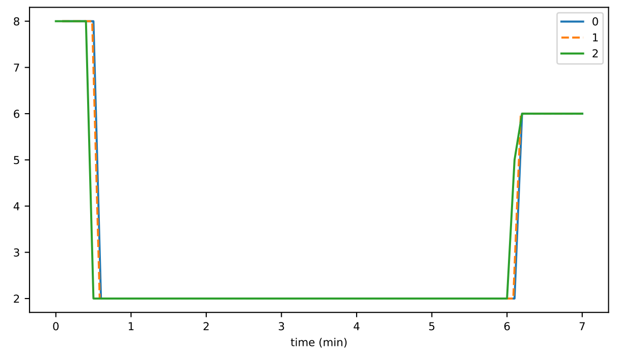
PlatformStatus
