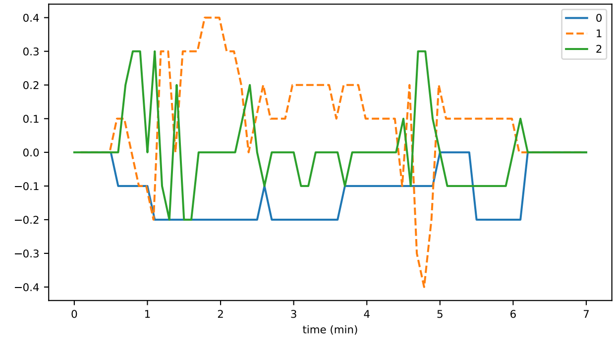
syncIndicatorDiff
