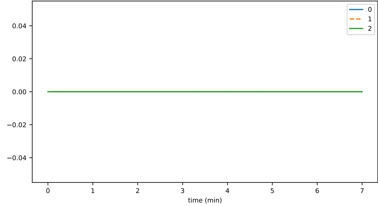
connSend_endStream_timeout
