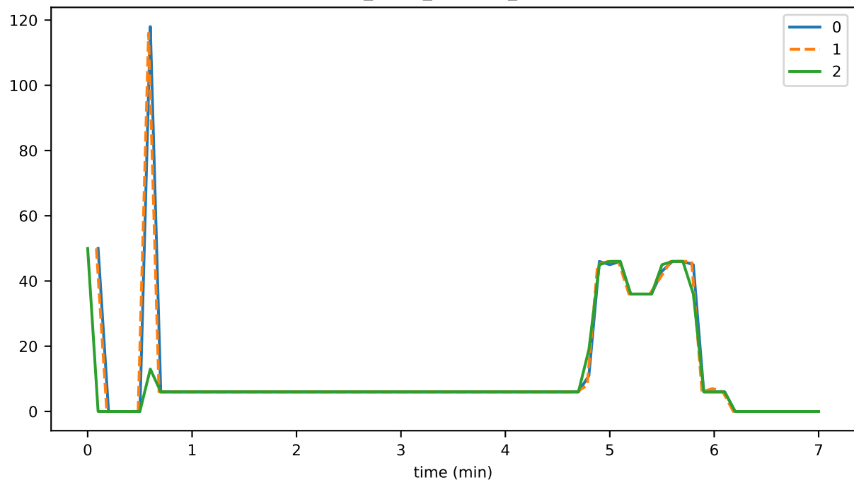
ds_reads_leafKeys_state
