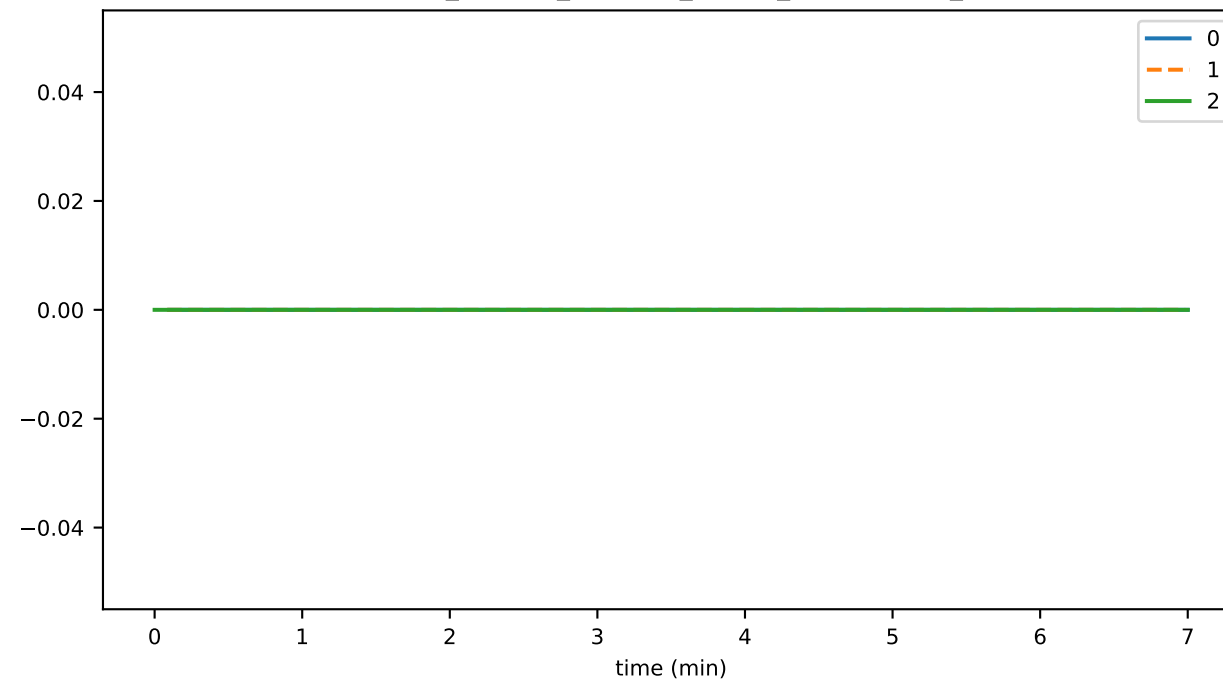
consensus_fraction_SETTING_EVENT_CONSENSUS_DATA
