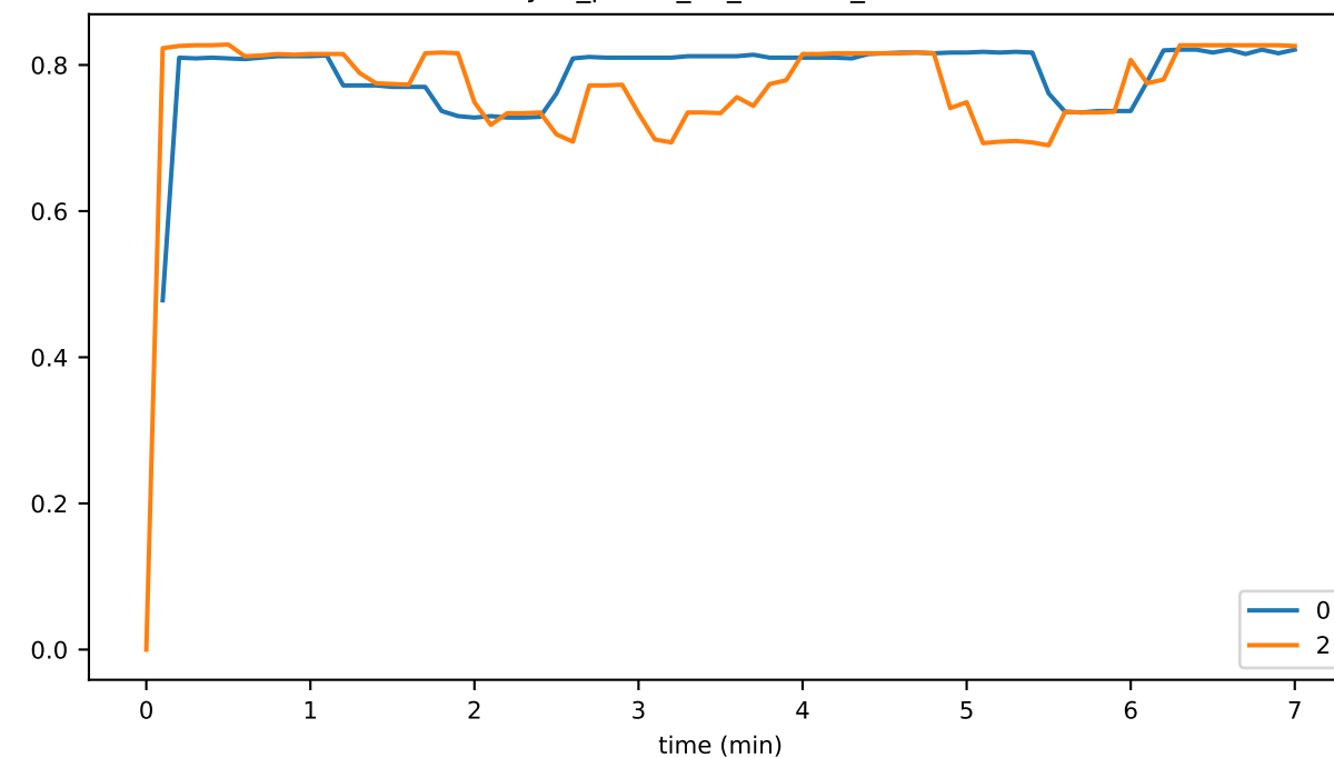
sync_phase_01_fraction_OTHER_FALLEN_BEHIND
