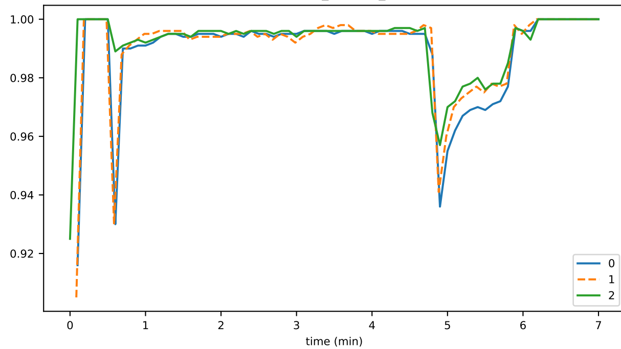
consensus_fraction_IDLE
