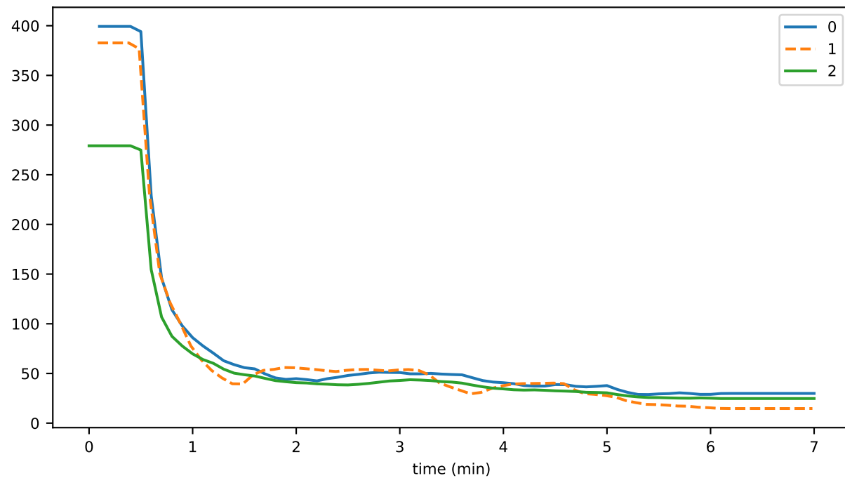
uptimeComputationTime
