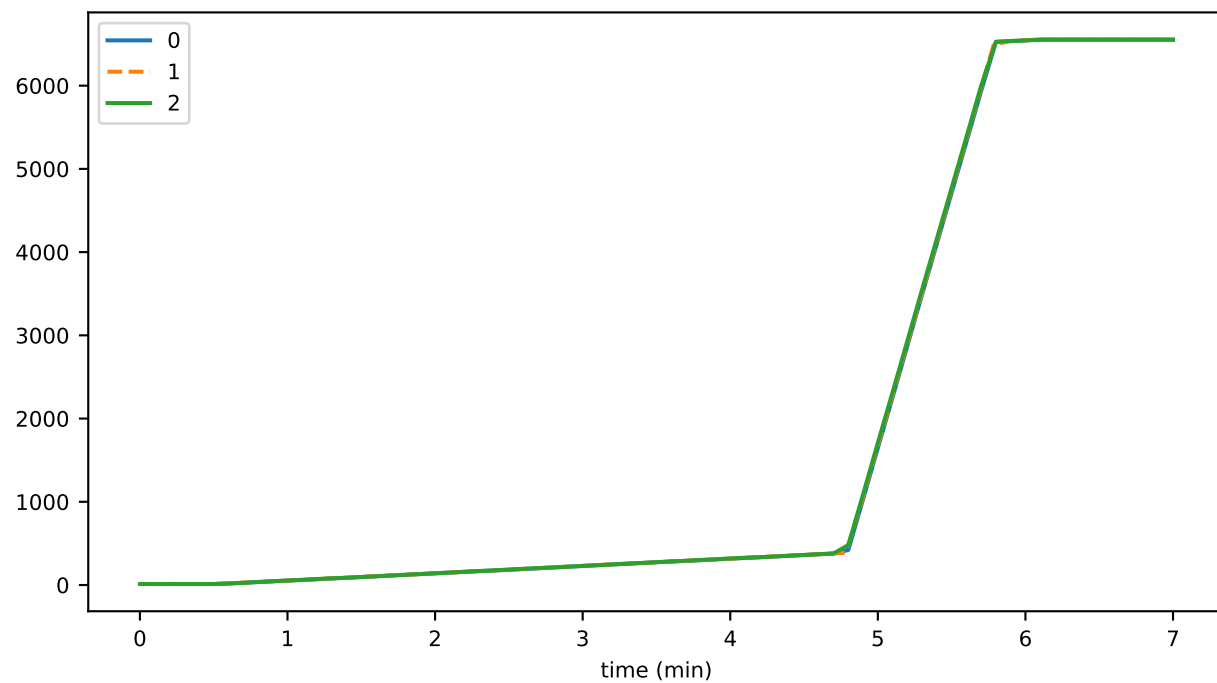
trans
