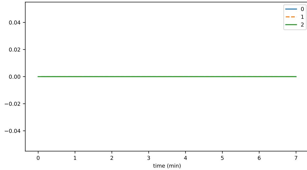
ds_compactions_level_7_leafKeysTimeMs_state
