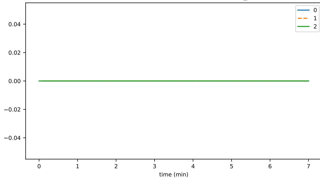
SmartContractService:LatestGasPrice
