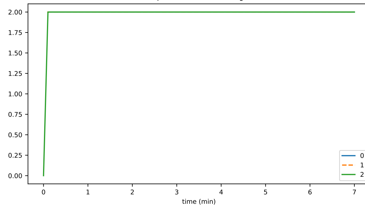
scheduleCreateDurationAvg
