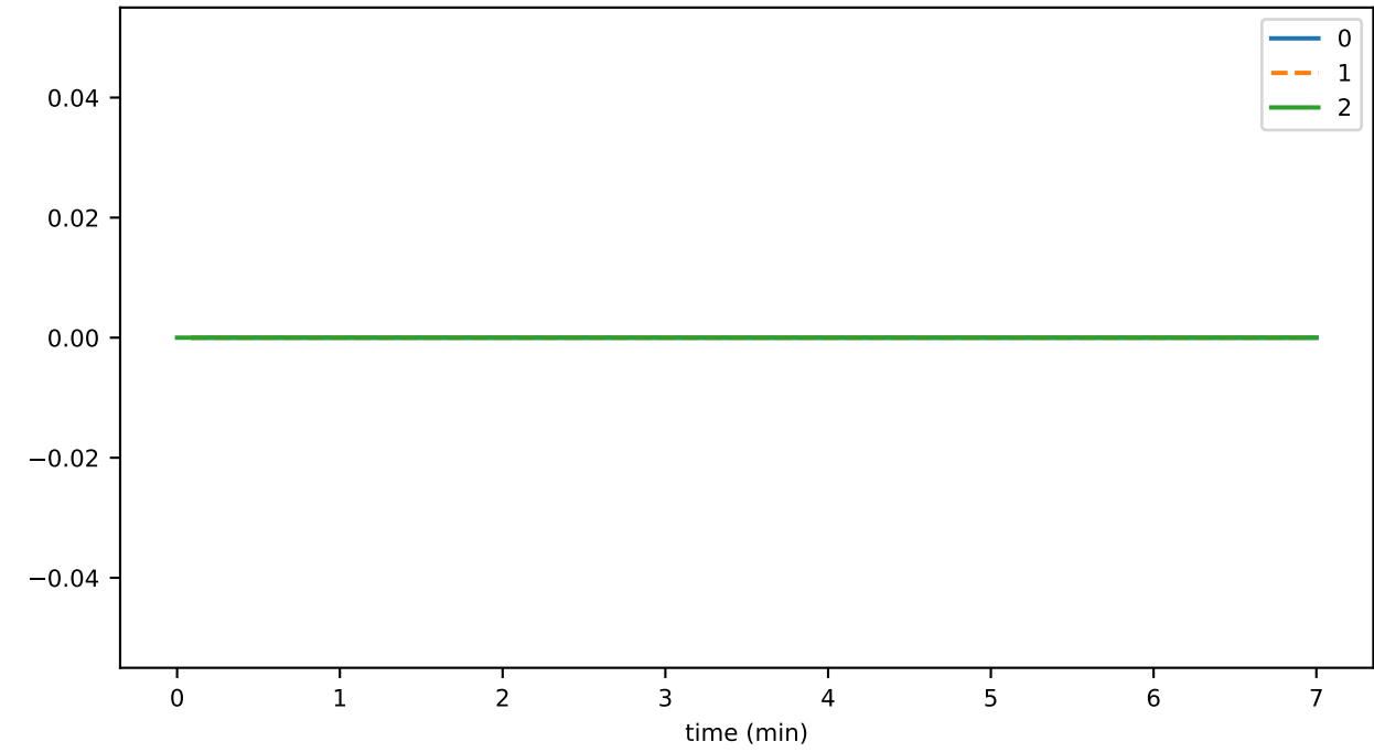
SmartContractService:SuccessfulTransactionDuration_count
