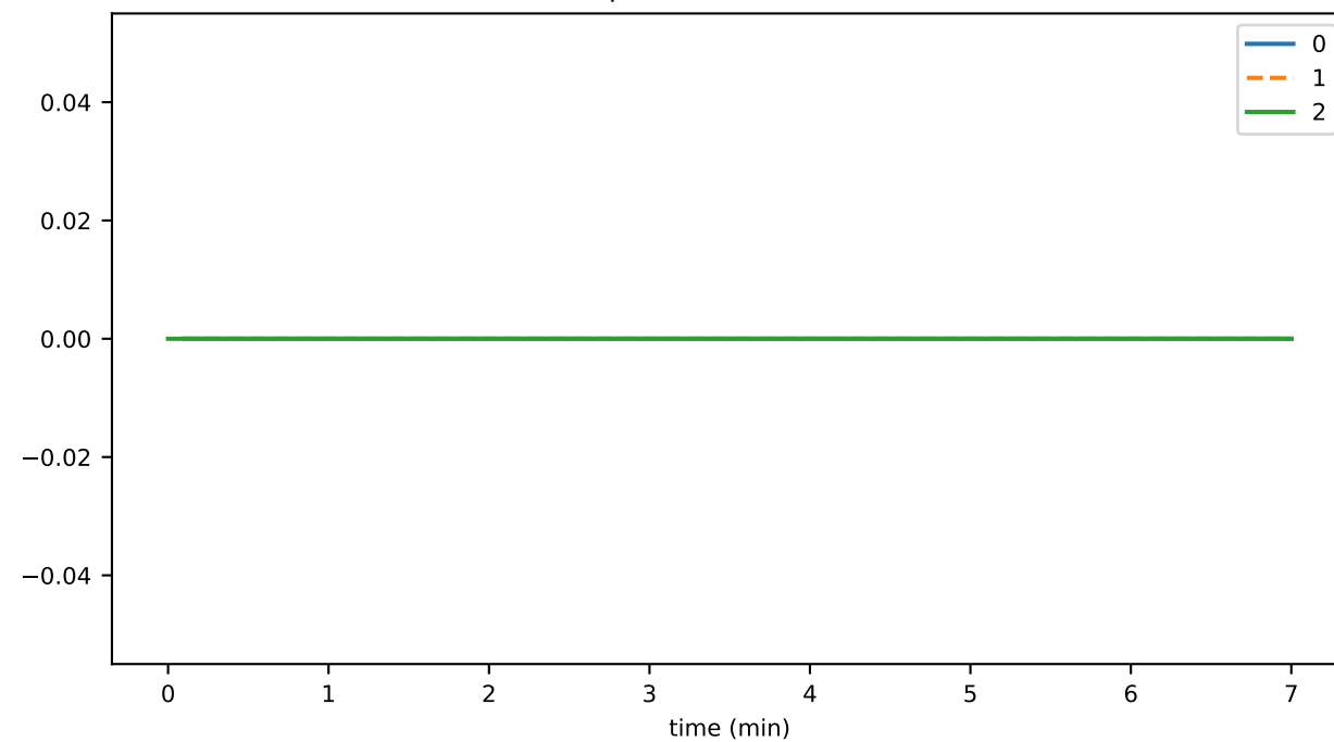
consOpsDurationPercentUsed
