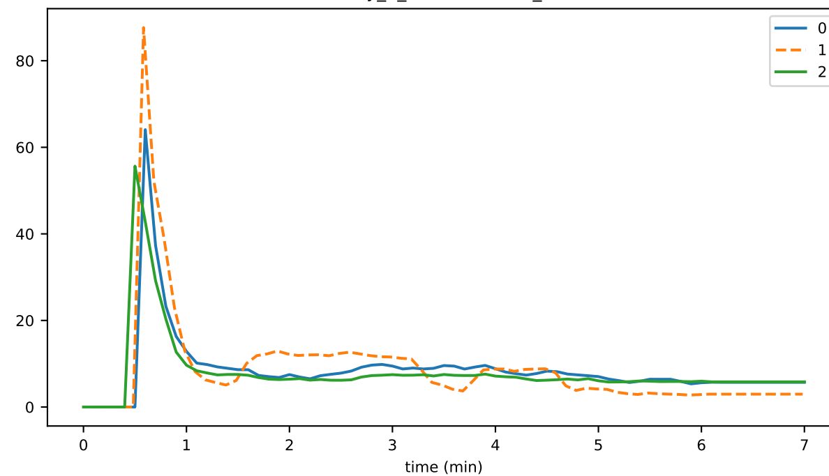
eventDelay_1_eventCreation_runtime
