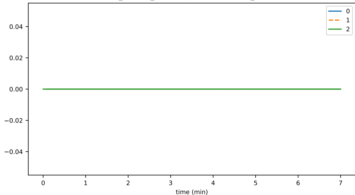
ds_reads_leafKeys_state
