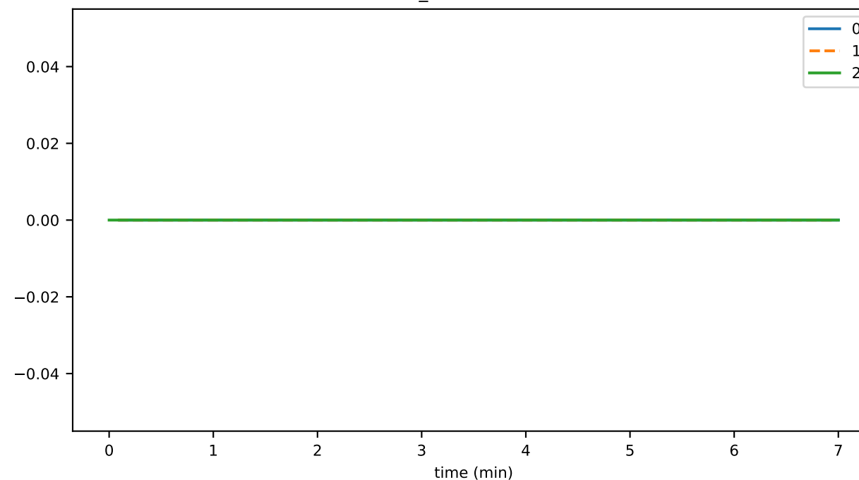
buffer_newestBlock
