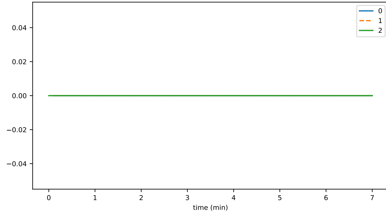
SmartContractService:SuccessfulTransactionDuration_avg
