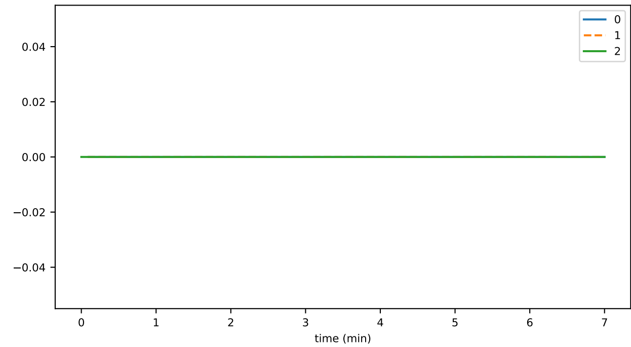
contractCallLocalDurationMax
