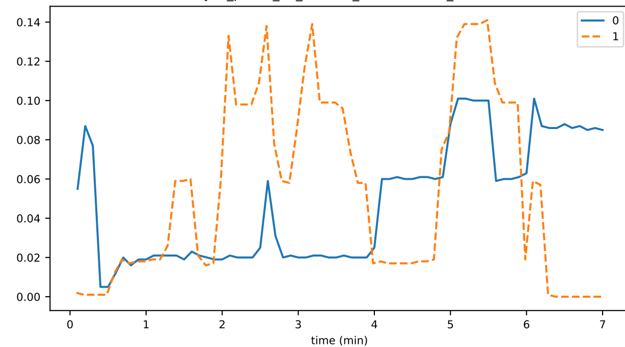
sync_phase_02_fraction_EXCHANGING_TIPS
