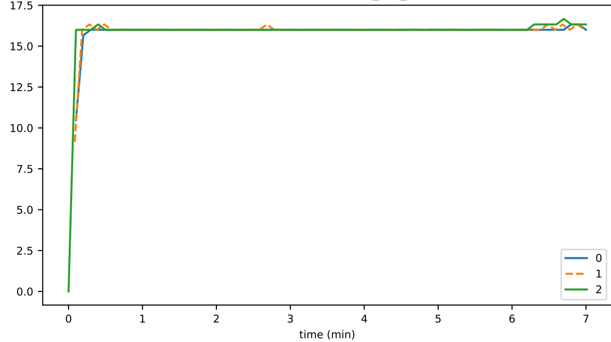
outgoingSyncRequests_per_sec
