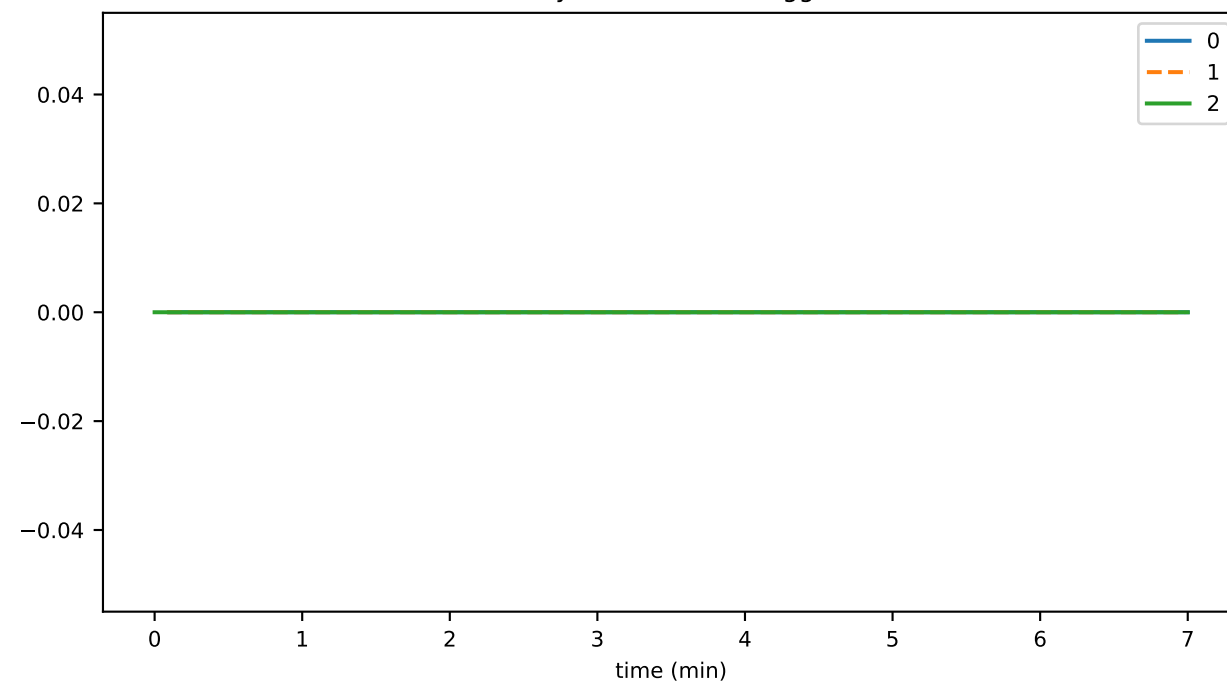
historyProofTransR3ToFailCnt
