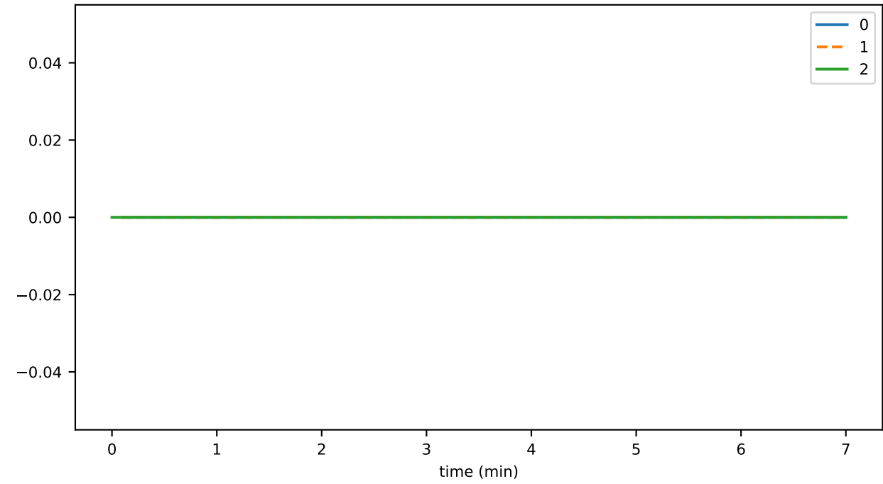
ds_compactions_level_7_leavesSavedSpaceMb_state
