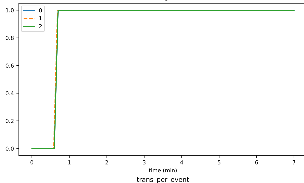
totalNeverSignedStates
