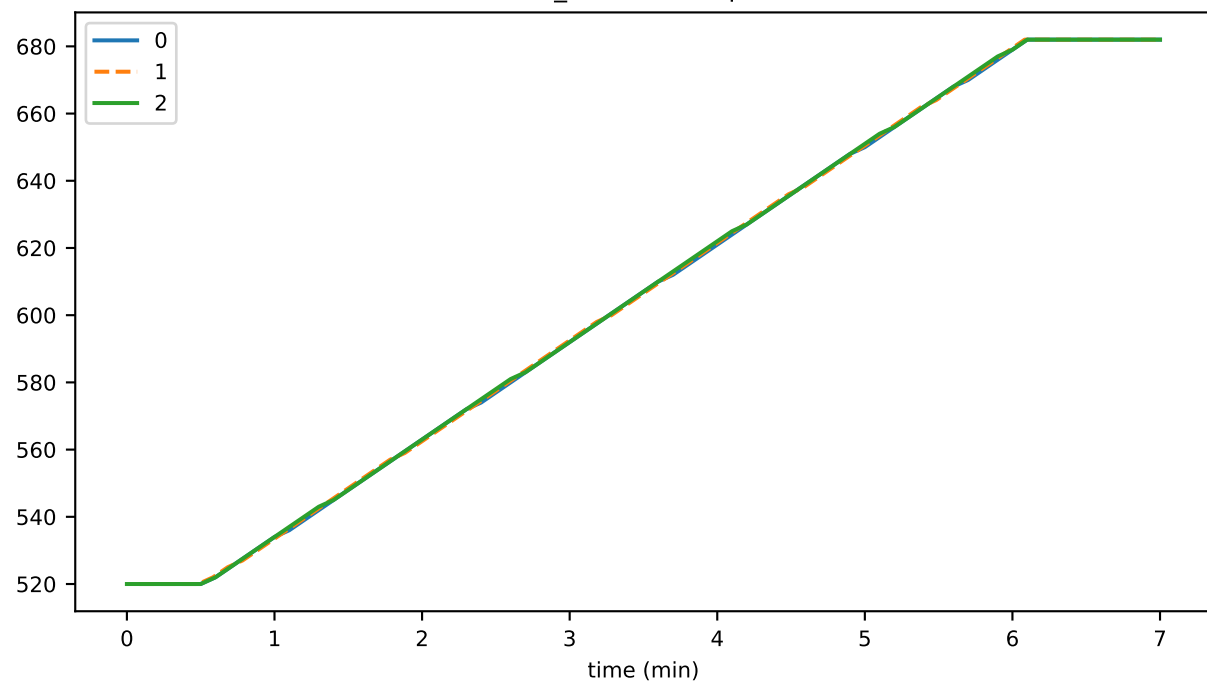
buffer_latestBlockOpened
