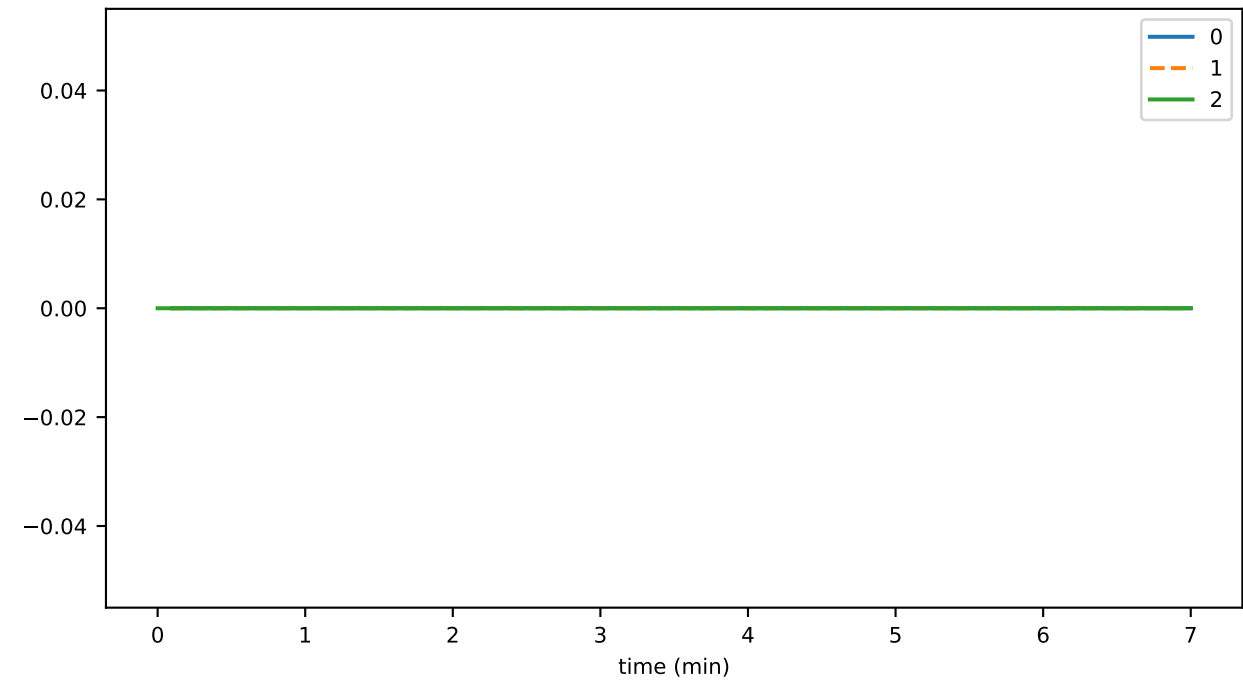
ds_compactions_level_4_leafKeysSavedSpaceMb_state
