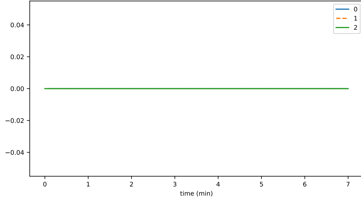
vmap_lifecycle_familySizeBackpressureMs_state
