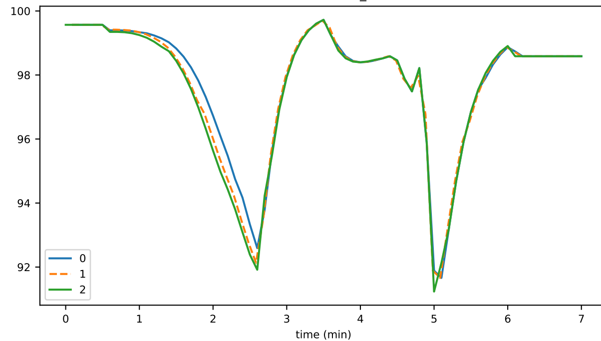
nodeActivePercent_node1
