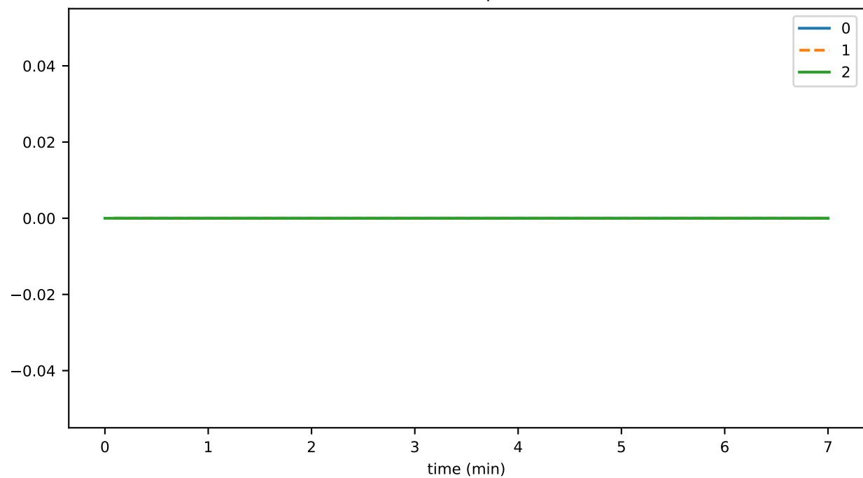
transactionGetReceiptThrottledTxns
