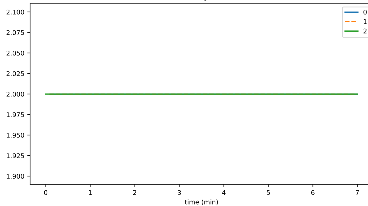
numVotingRounds
