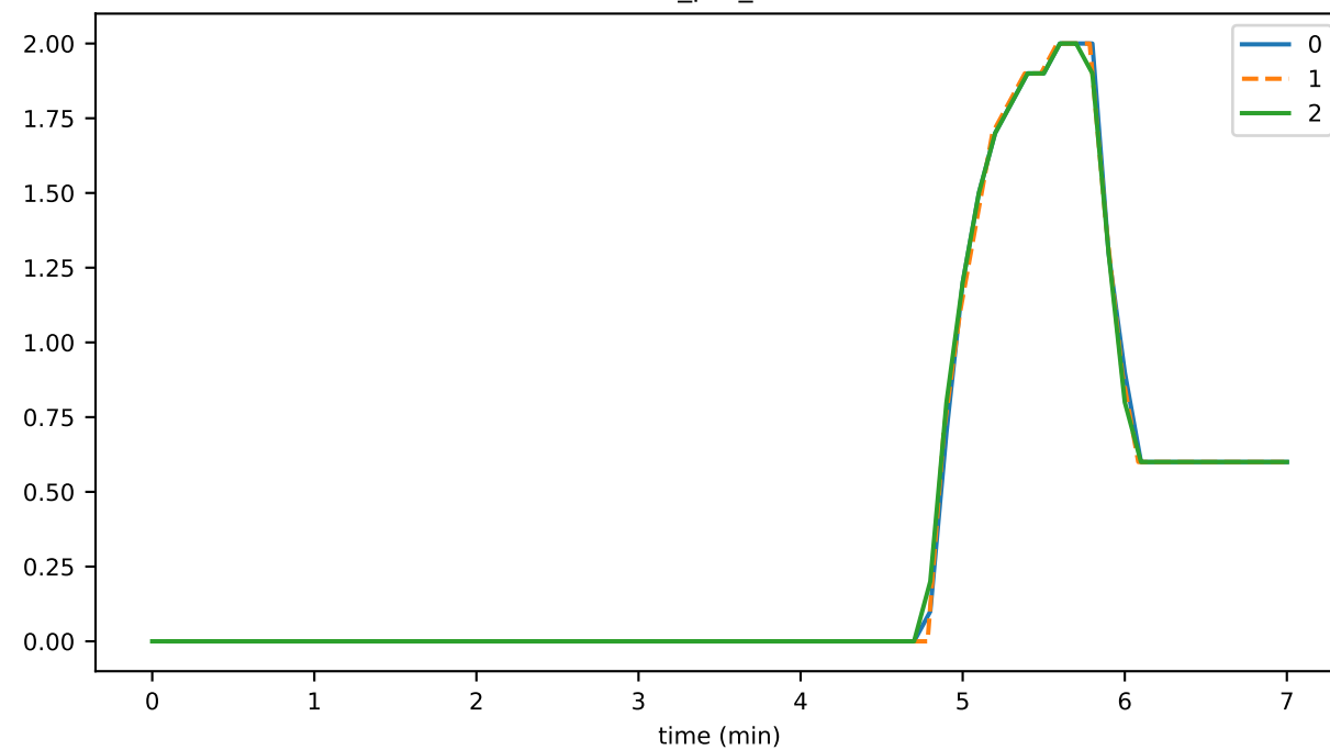
trans_per_event
