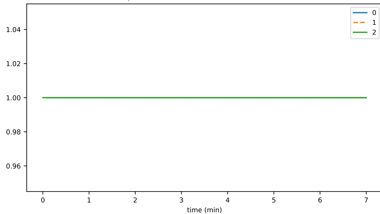
preconsensusEventFileOldestIdentifier
