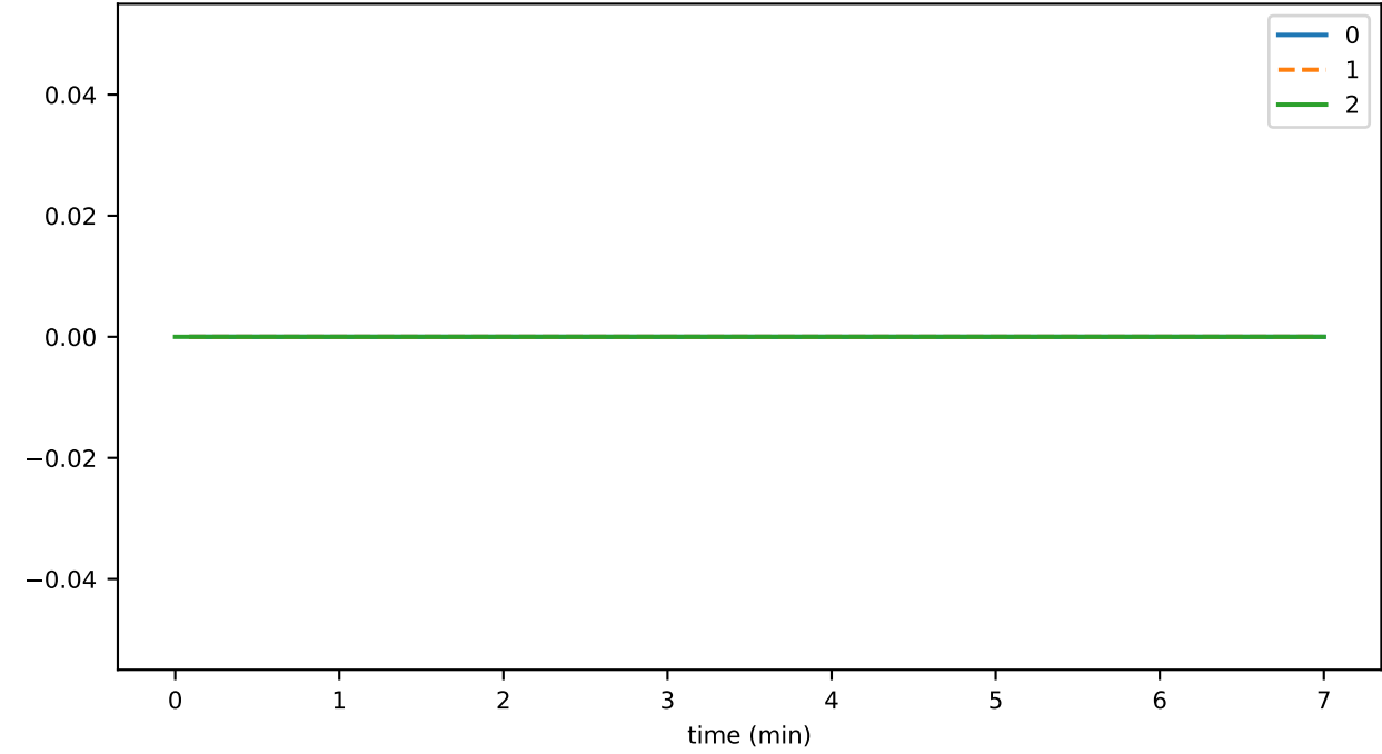
ds_compactions_level_0_hashesSavedSpaceMb_state
