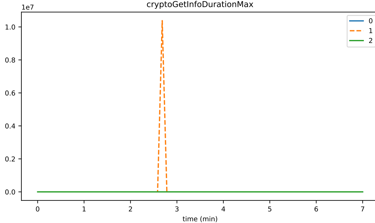
cryptoGetInfoDurationMax
