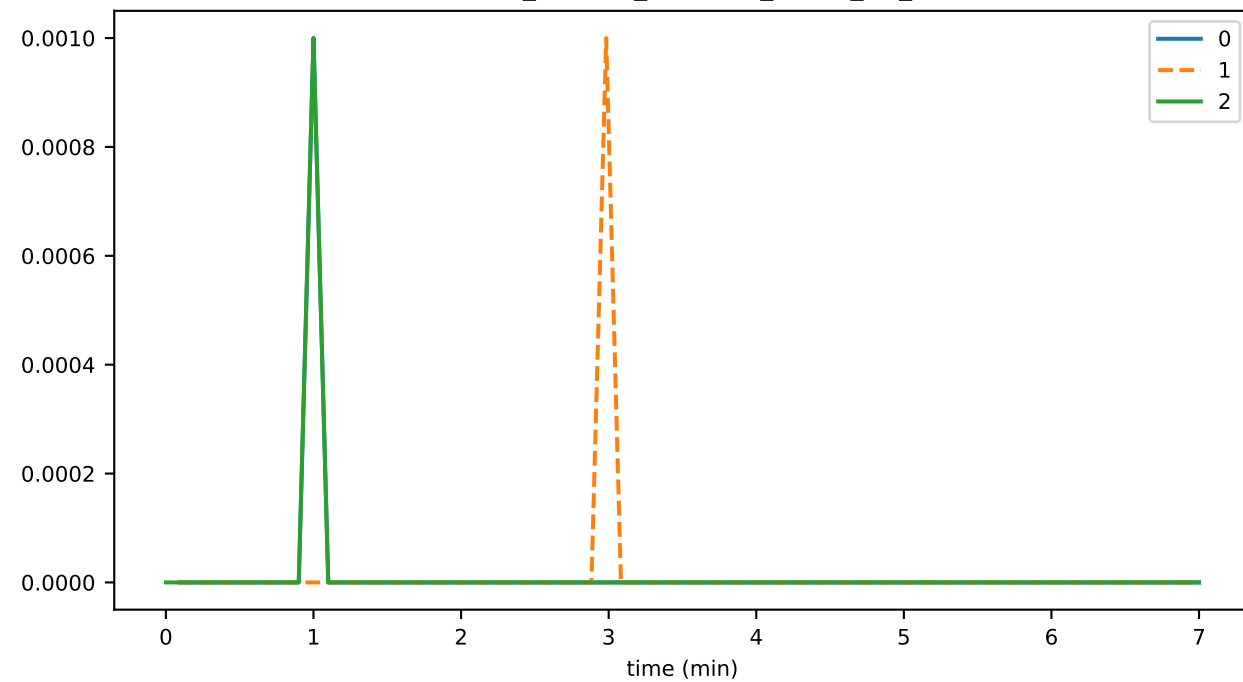
consensus_fraction_IDLE
