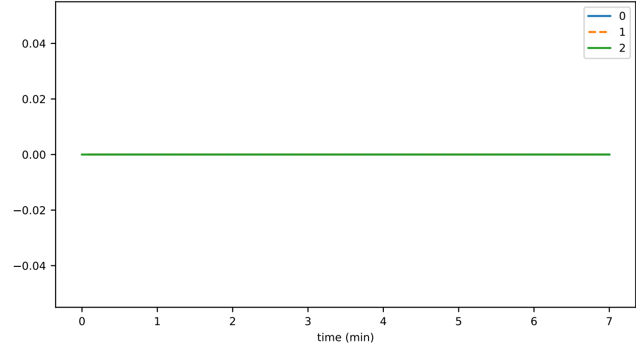
SmartContractService:SuccessfulTransactionDuration_count
