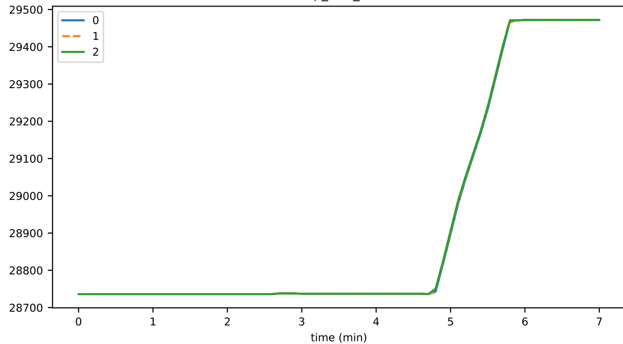
vmap_size_state
