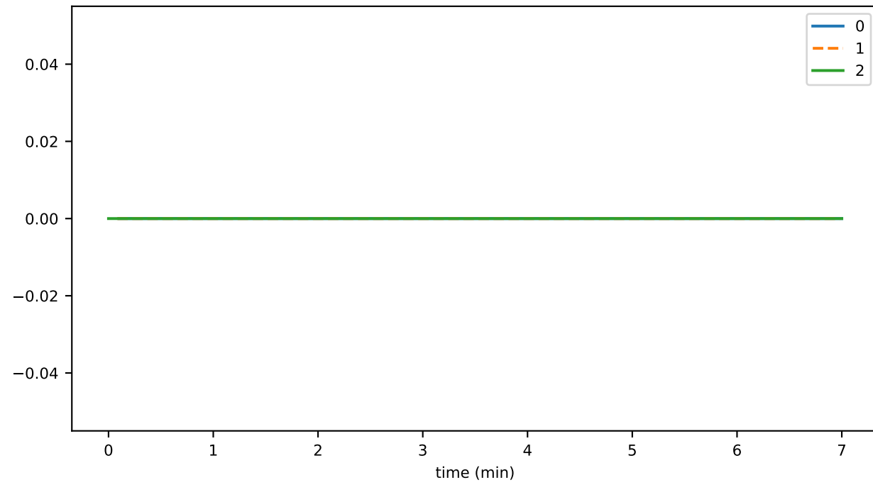
ds_compactions_level_4_hashesTimeMs_state
