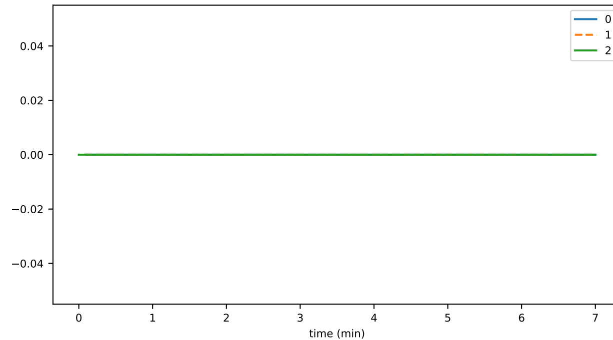
utilPrngDurationAvg
