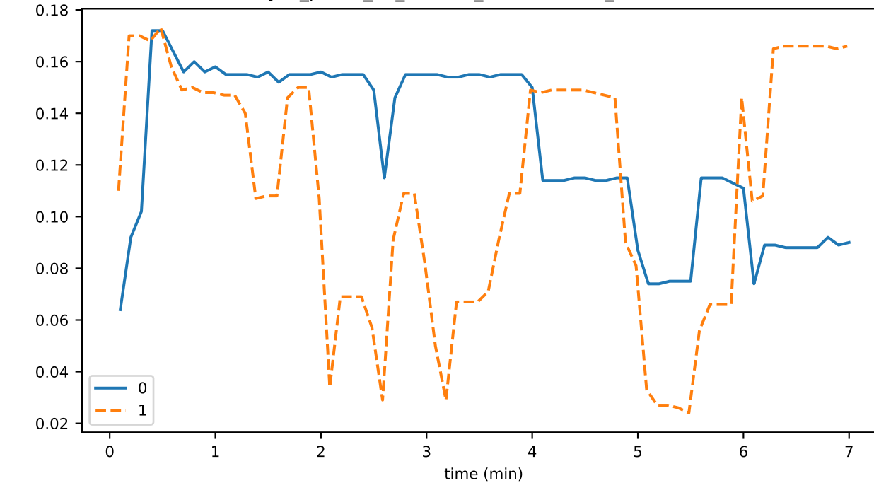
sync_phase_02_fraction_EXCHANGING_WINDOWS
