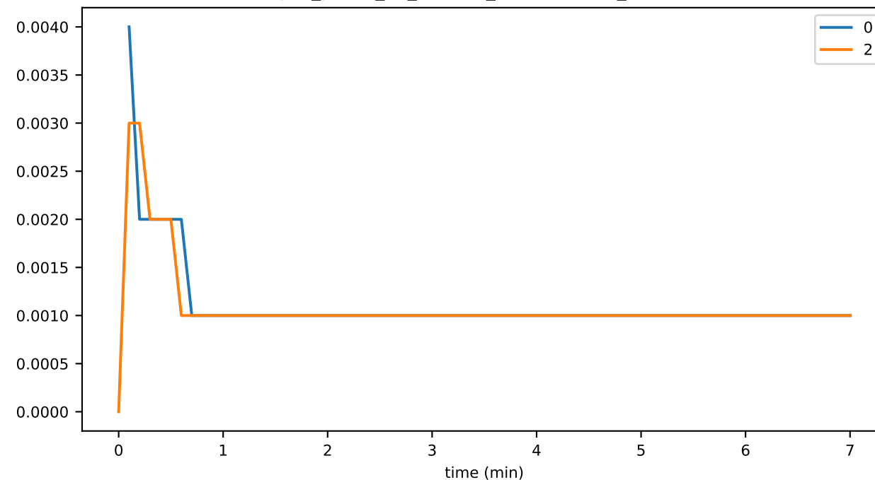
sync_phase_01_fraction_EXCHANGING_WINDOWS
