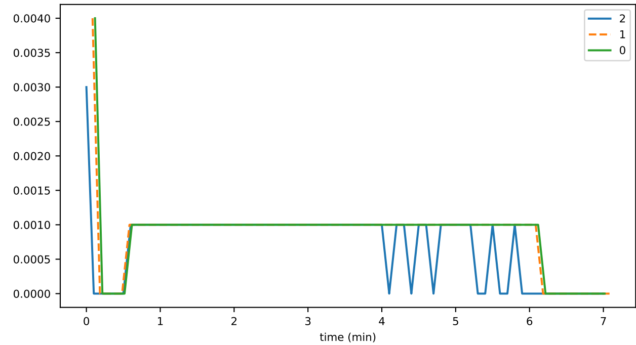
eventDelay_1_eventCreation_runtime
