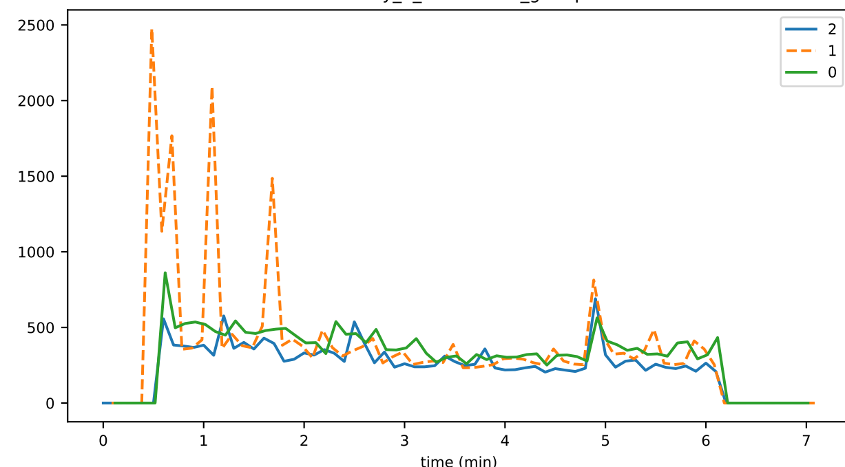
eventDelay_4_verification_gossipMAX
