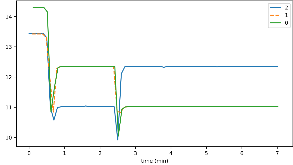
numEventsAddedUntilConsensus
