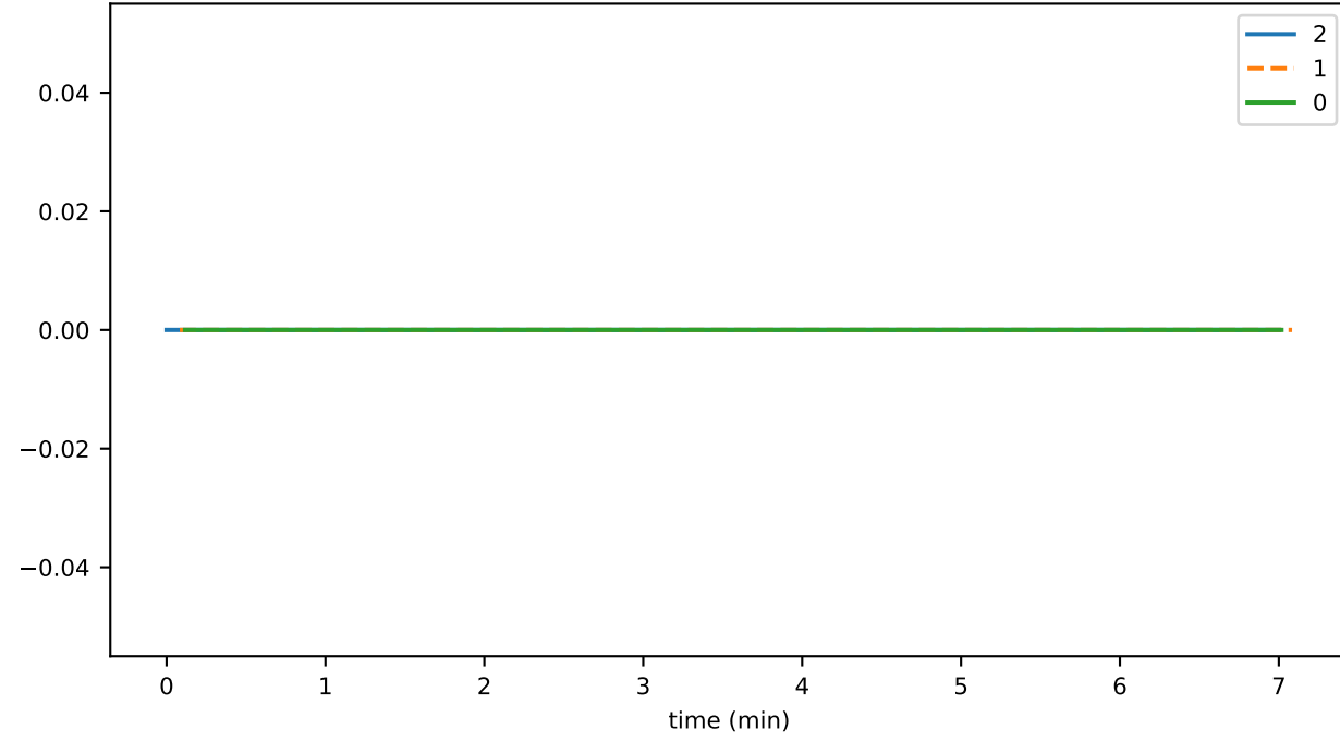
receiverReconnectDurationSeconds
