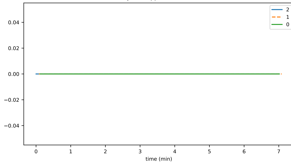
rejectedAppTransactions
