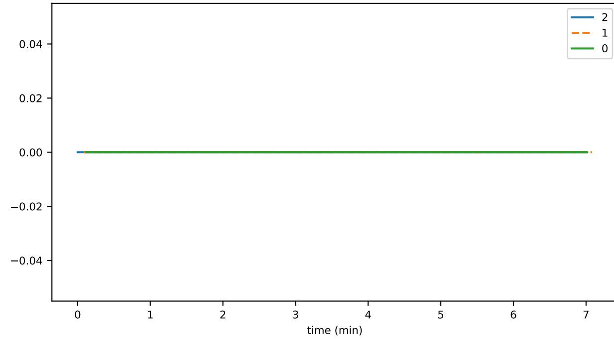
uptimeComputationTime
