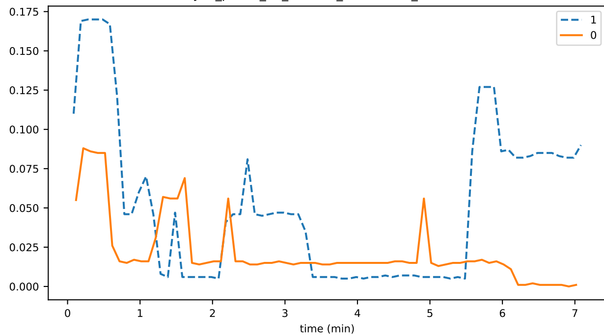
sync_phase_02_fraction_RECEIVING_EVENTS
