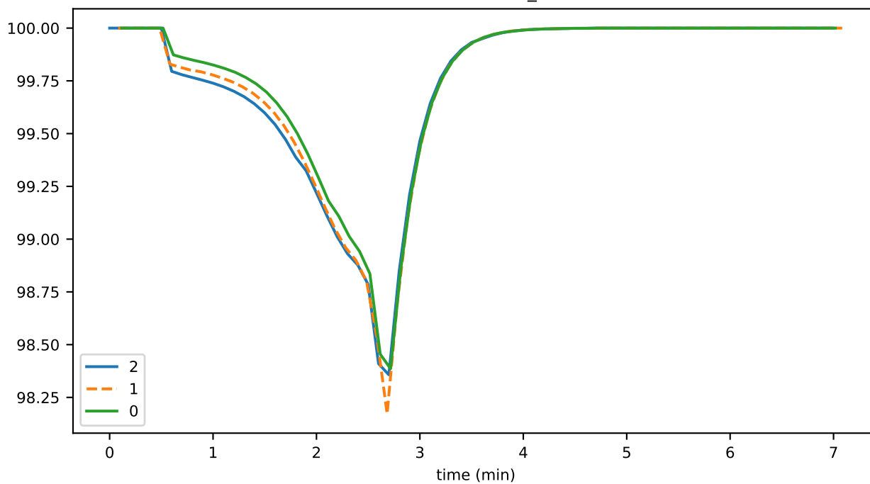
nodeActivePercent_node1
