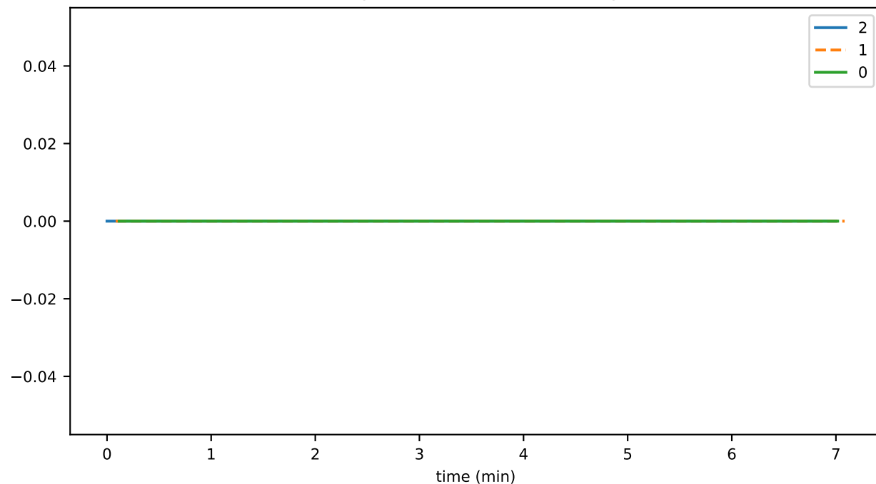
ledgerIdPublicationThrottledTxns
