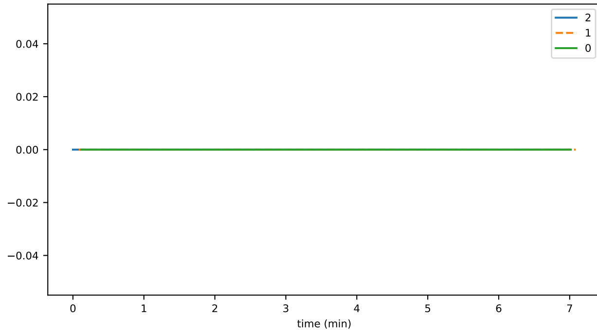
consensusSubmitMessageDurationAvg
