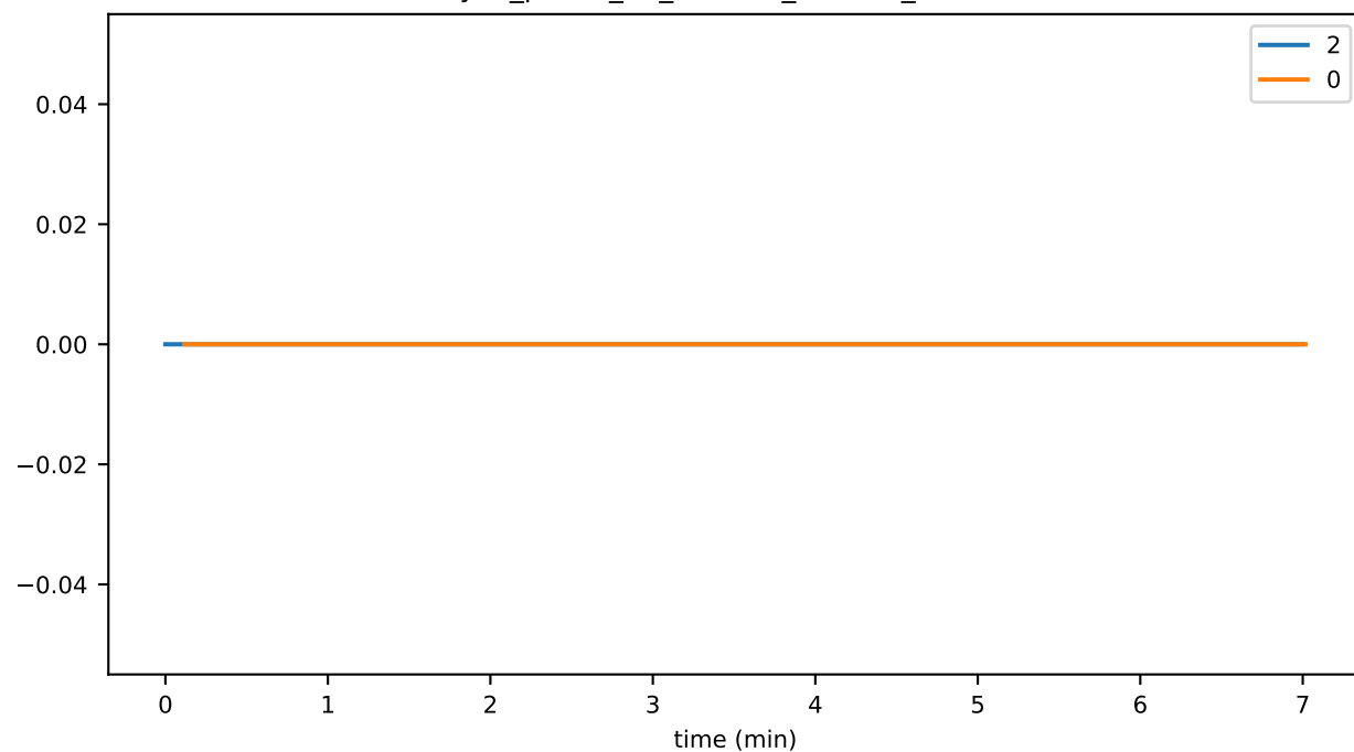
sync_phase_01_fraction_NO_PERMIT
