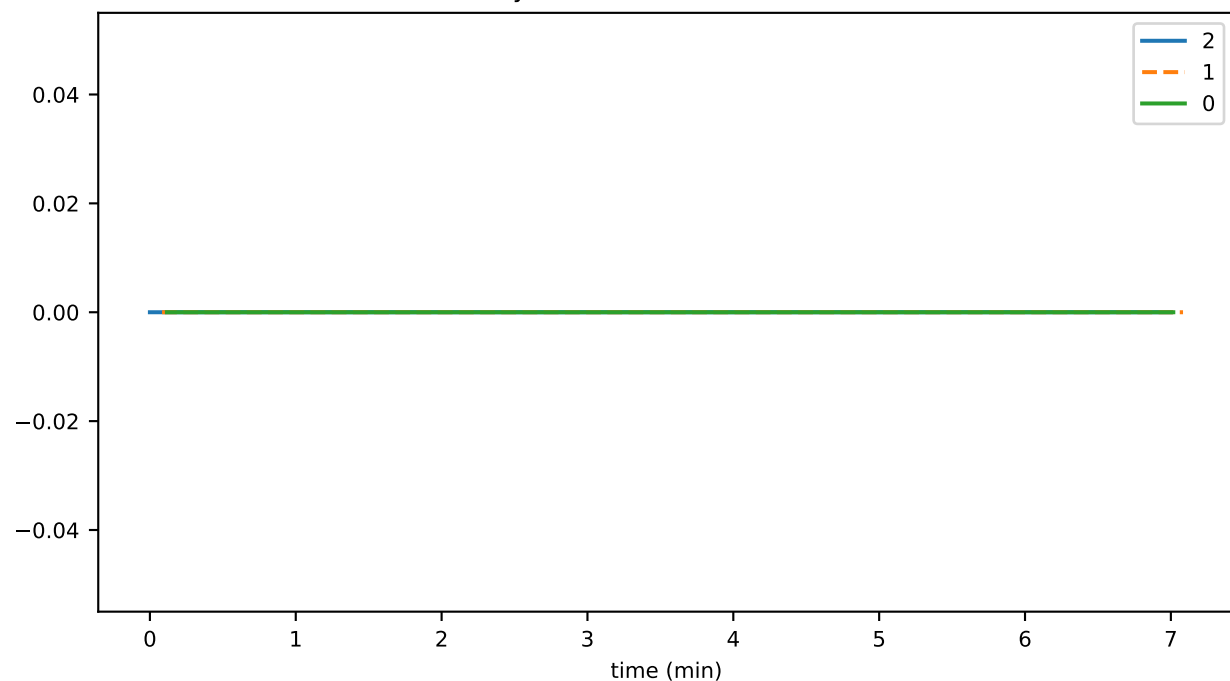
historyProofVoteDurationMax
