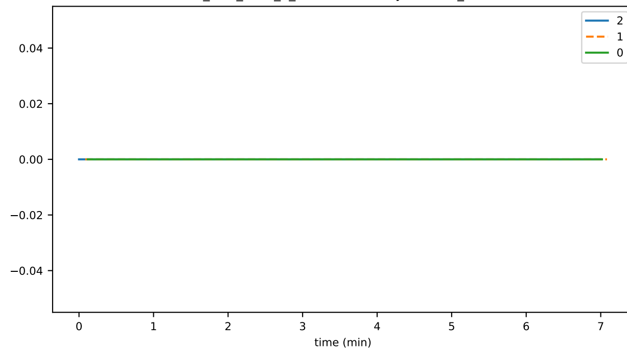
ds_files_level_9_leavesFileSizeByLevelMb_state
