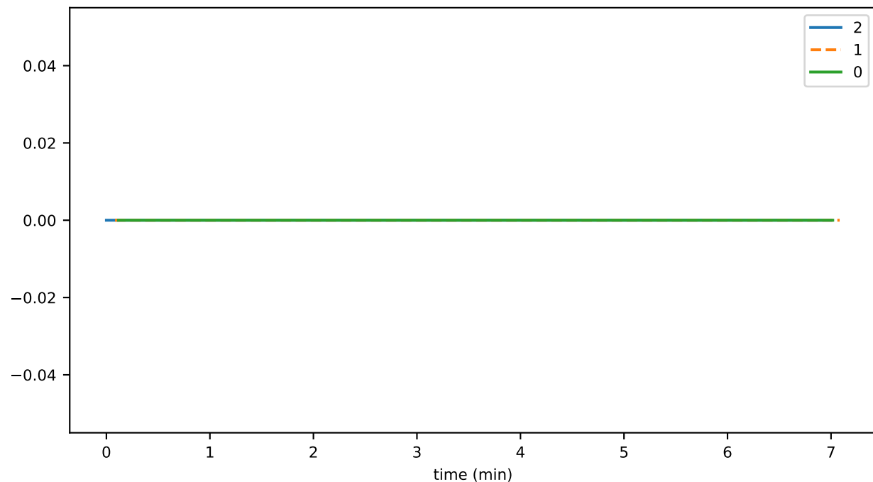
scheduleDeleteDurationAvg
