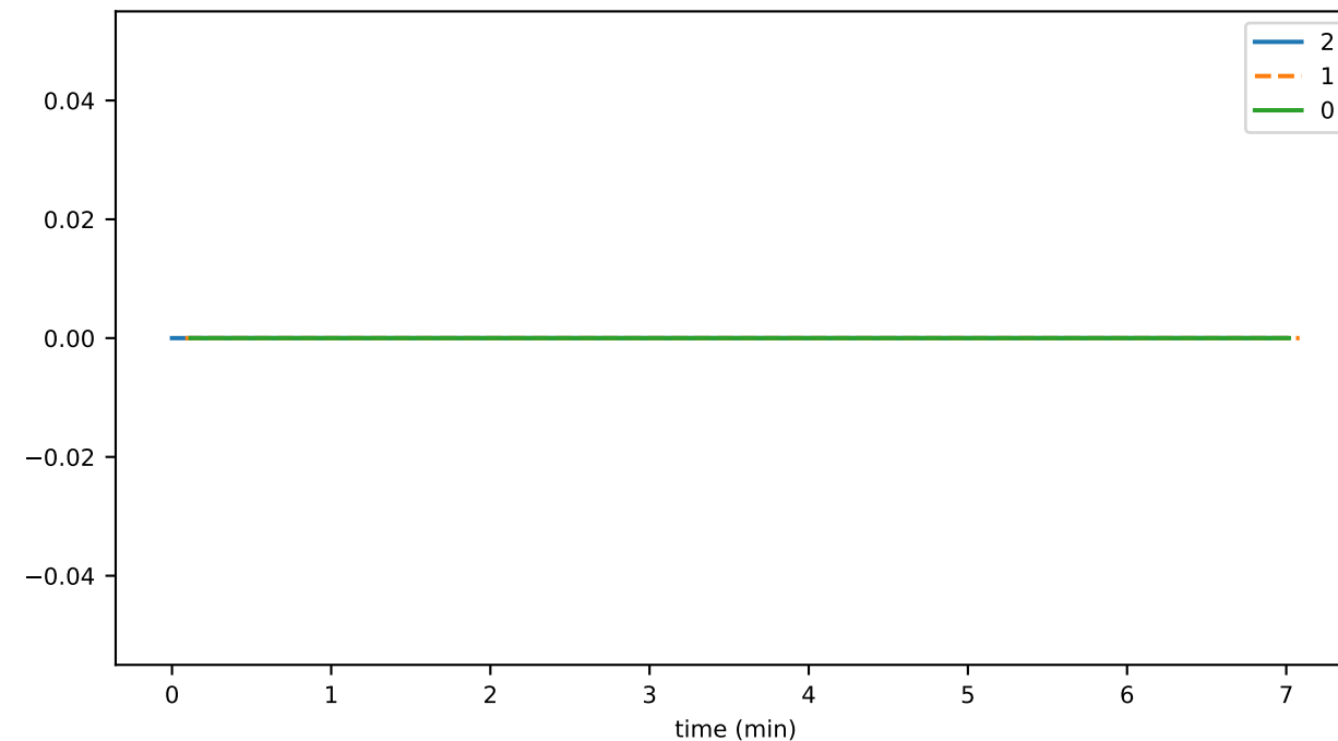
hintsPartialSignatureDurationAvg
