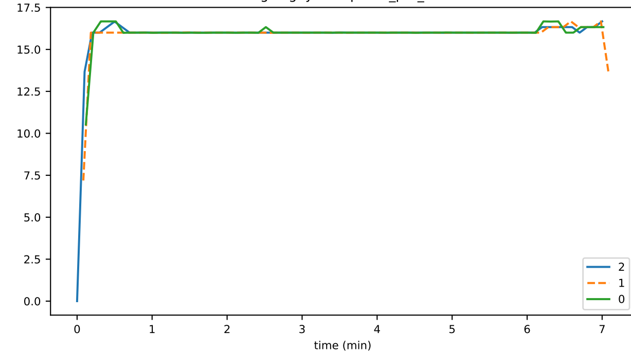
outgoingSyncRequests_per_sec
