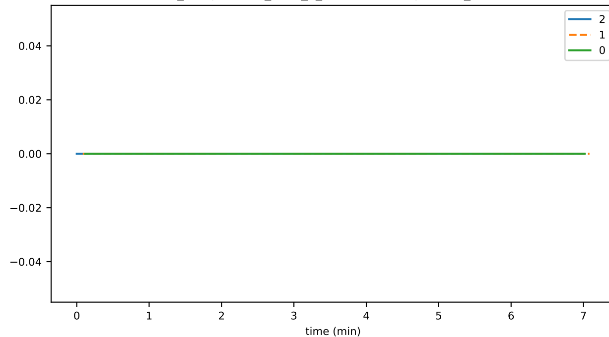
ds_compactions_level_6_leafKeysSavedSpaceMb_state
