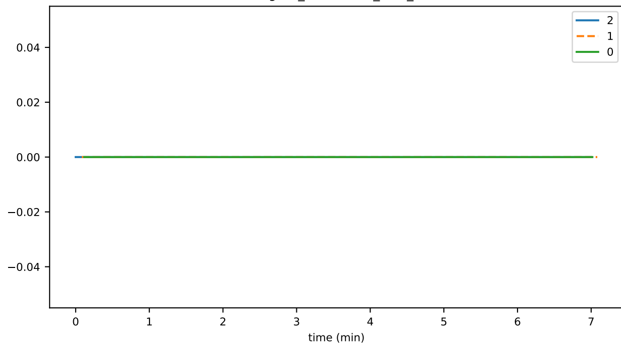
StateSigner_unhandled_task_count
