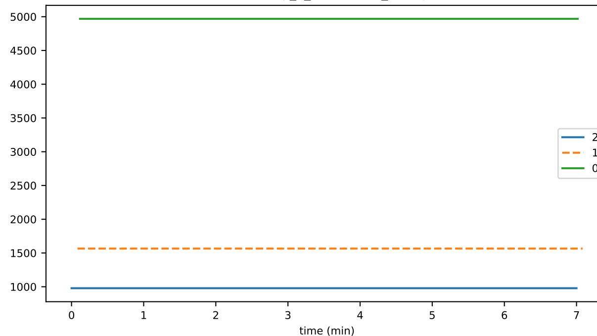
eventDelay_5_orphanBuffer_gossip
