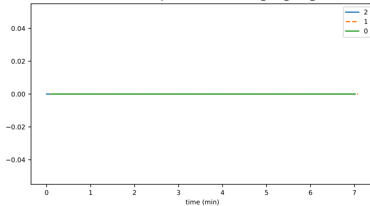
SmartContractService:SystemContractMethodCall_MINT_BURN_failed
