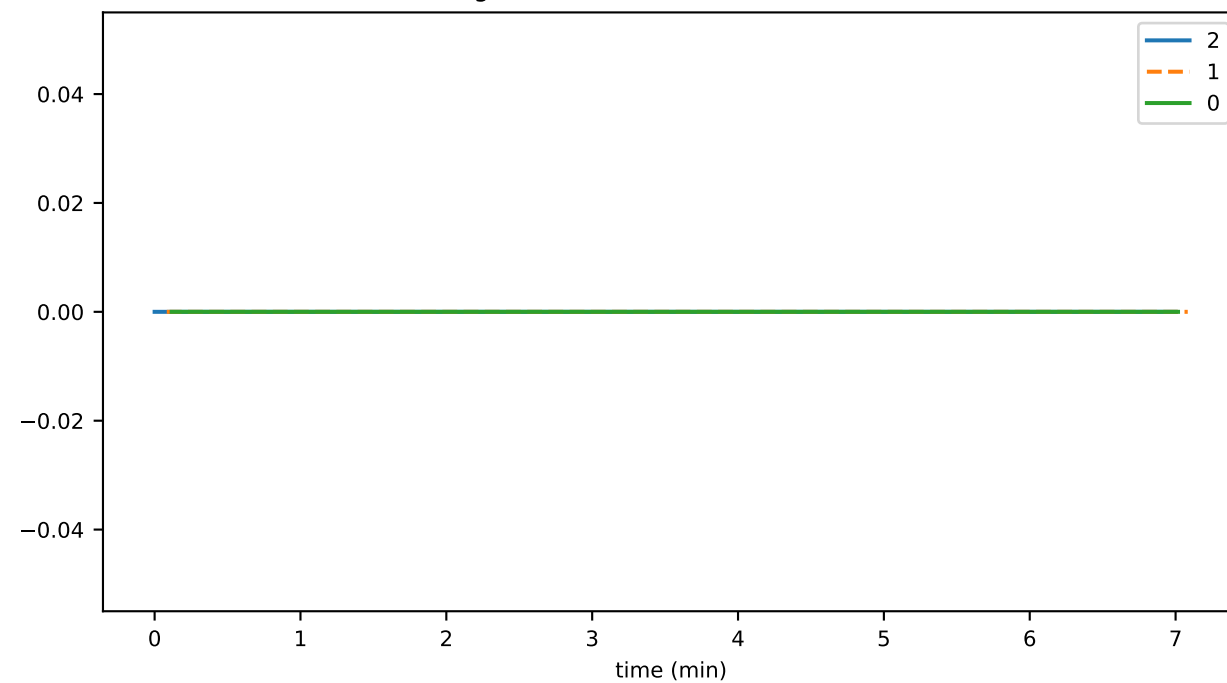
registeredNodeCreateDurationMax
