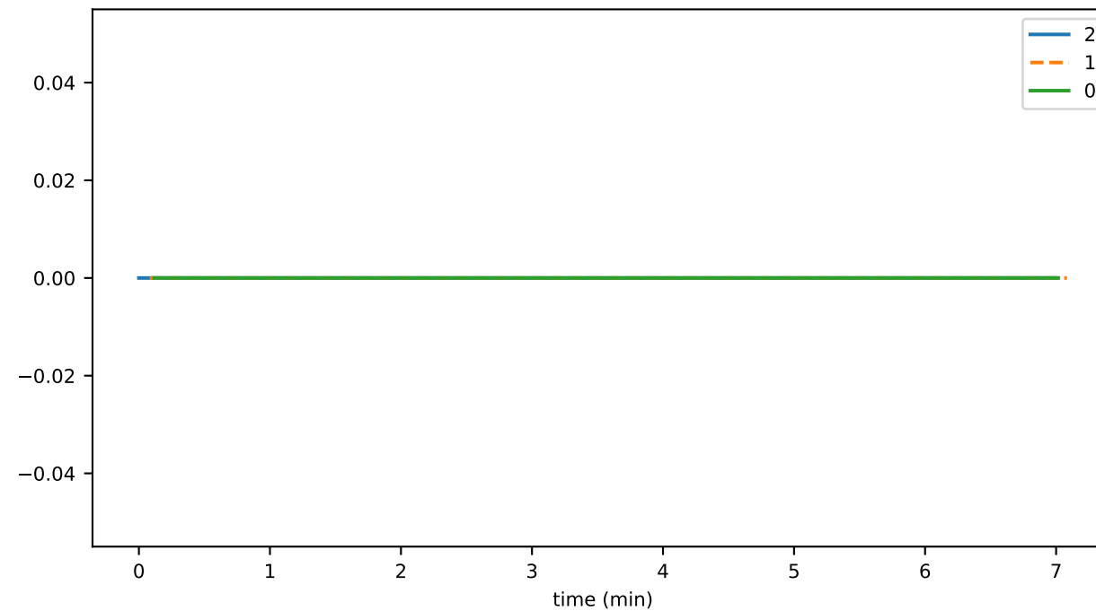
consensusCreateTopicDurationAvg
