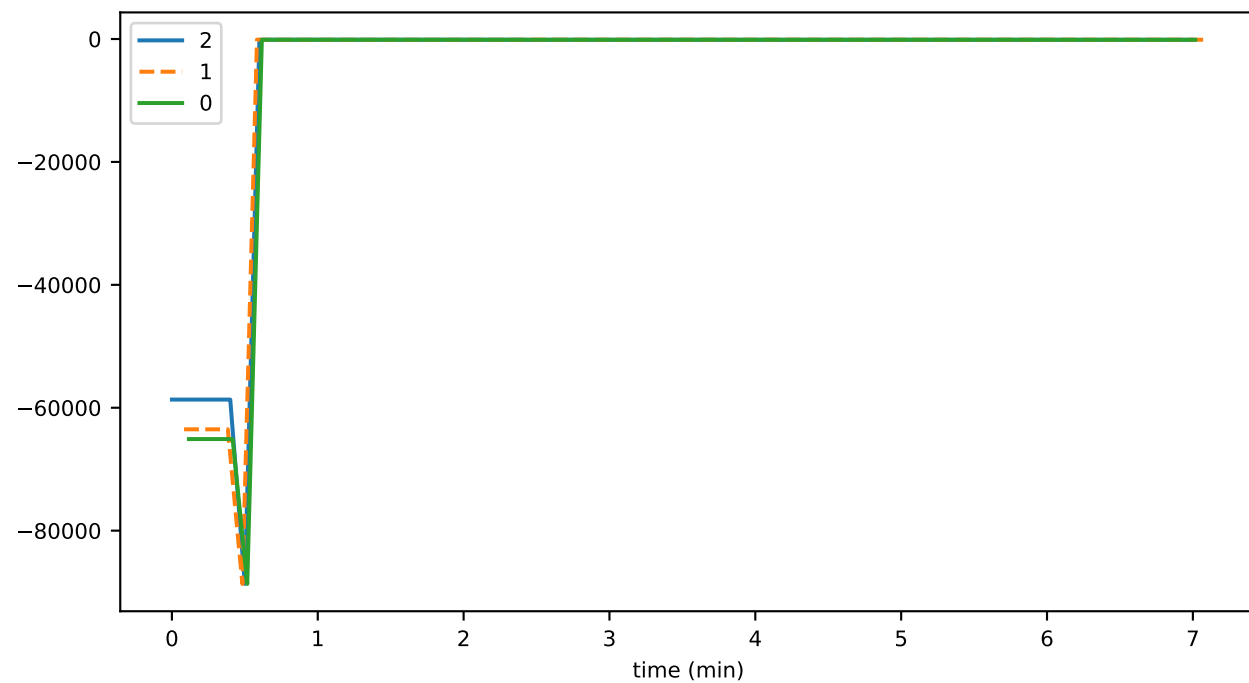
consensusTimeDeviation
