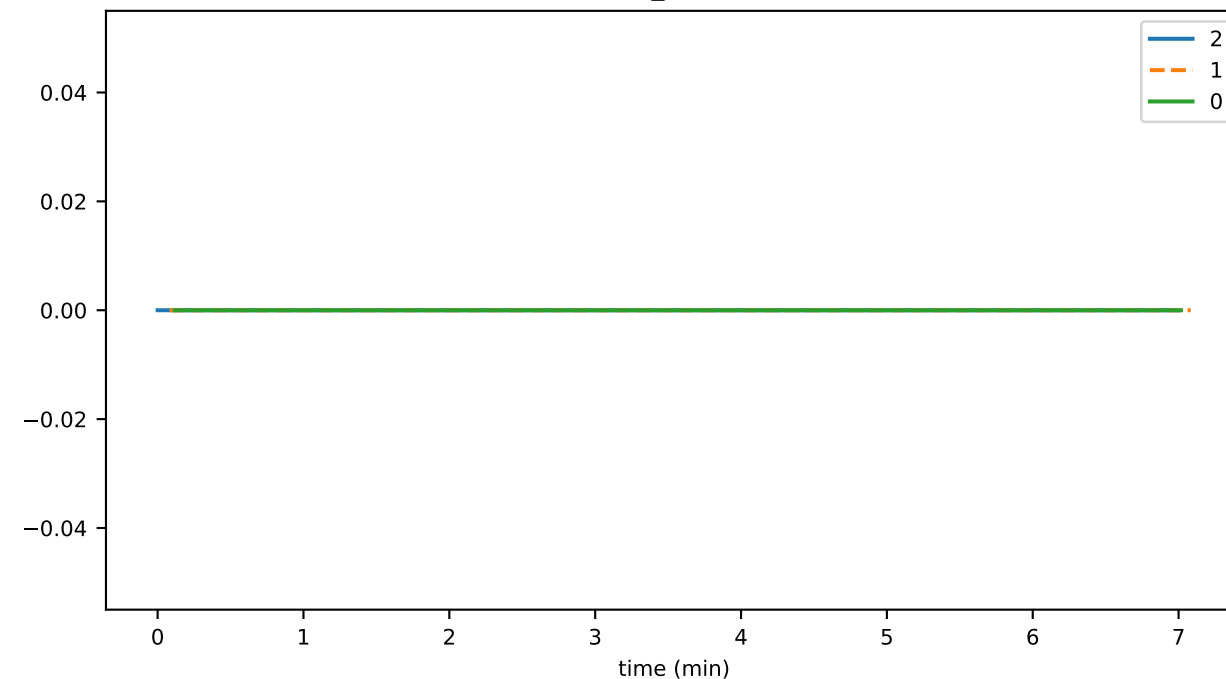
conn_pipelineOperationTimeout
