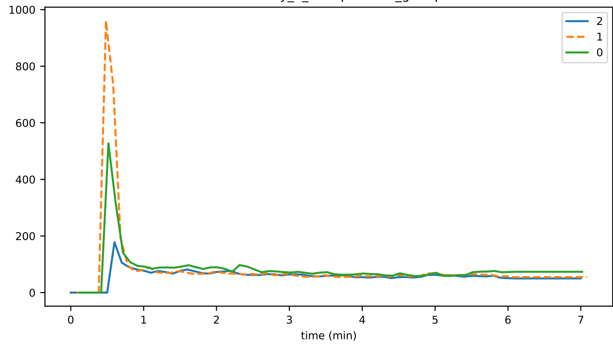
eventDelay_3_deduplication_gossip
