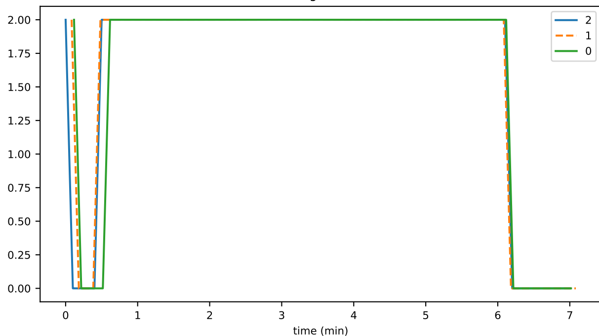
opAgeDiff
