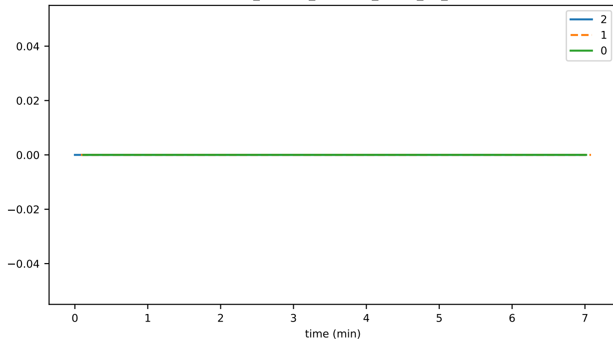
consensus_fraction_IDLE
