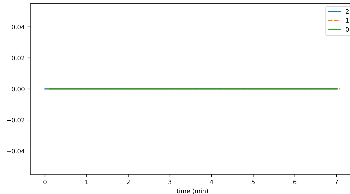
nodeDeleteDurationAvg
