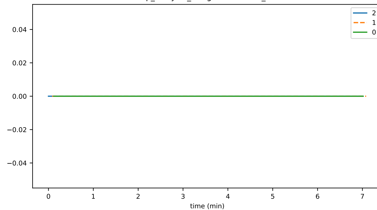
vmap_lifecycle_mergeDurationMs_state
