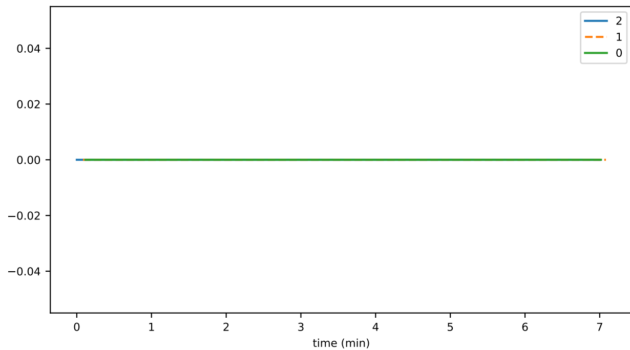
tokenUnfreezeAccountDurationMax
