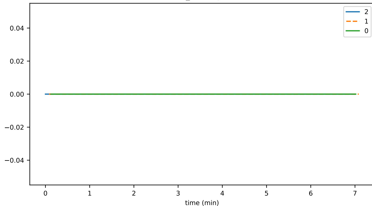
conn_opened
