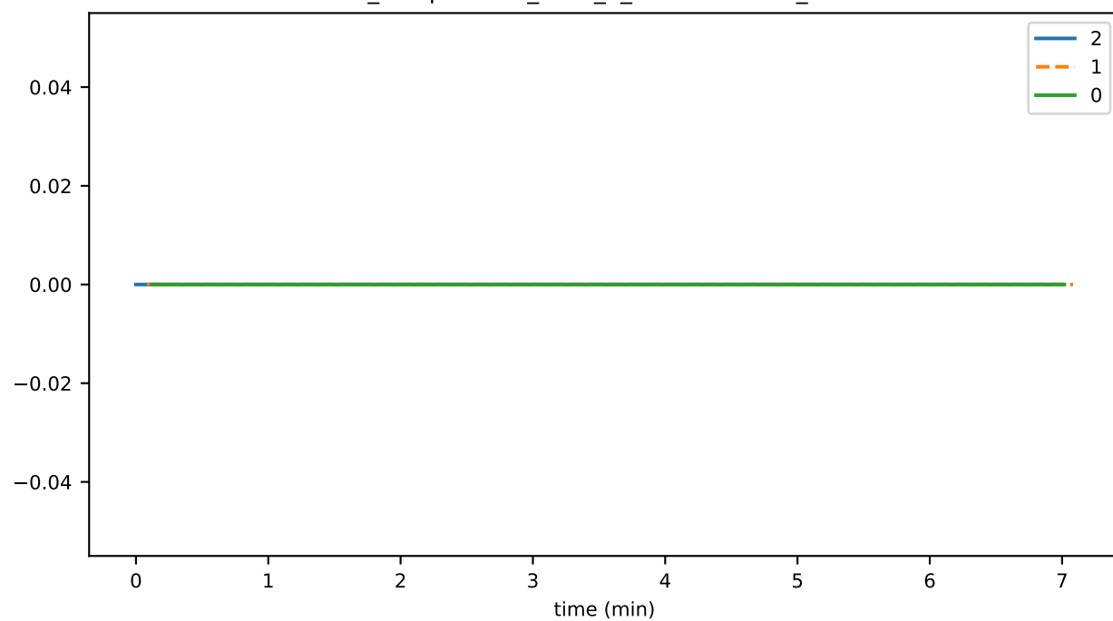
ds_compactions_level_8_leavesTimeMs_state
