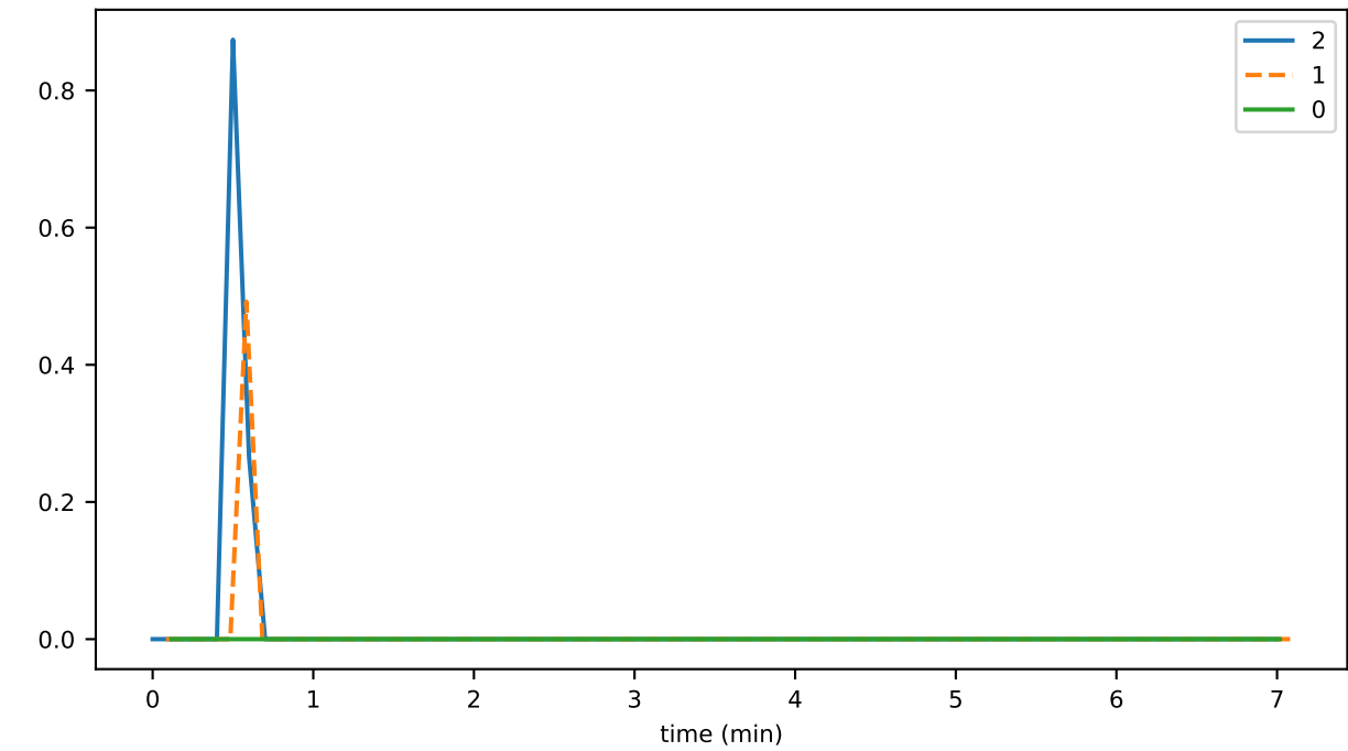
eventCreation_fraction_PIPELINE_INSERTION
