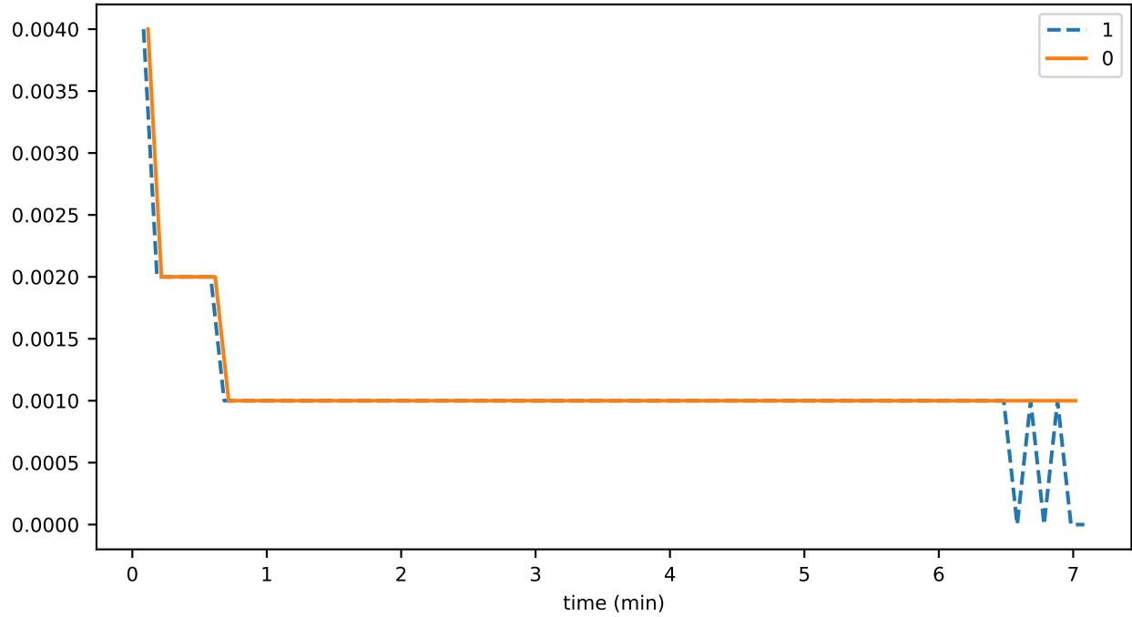
sync_phase_02_fraction_EXCHANGING_WINDOWS
