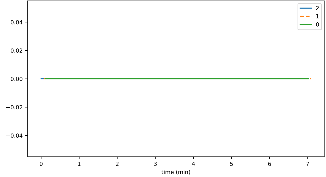
Dig_per_sec
