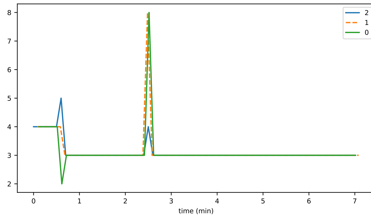
eventsPerRound
