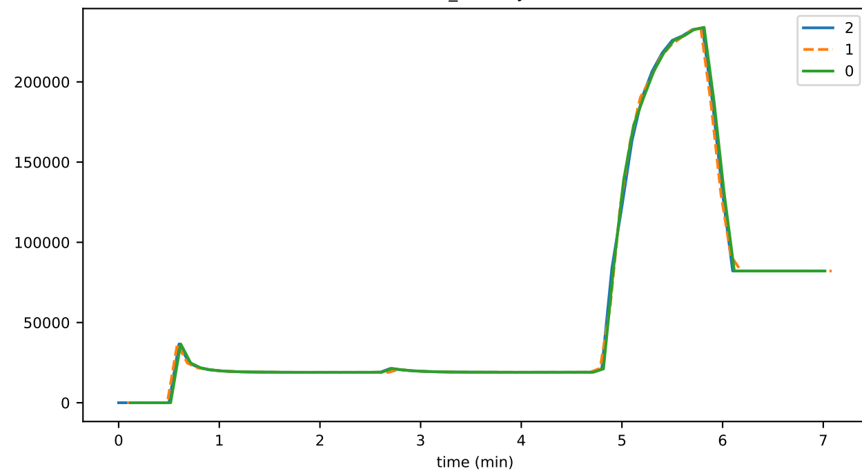
buffer_blockBytes
