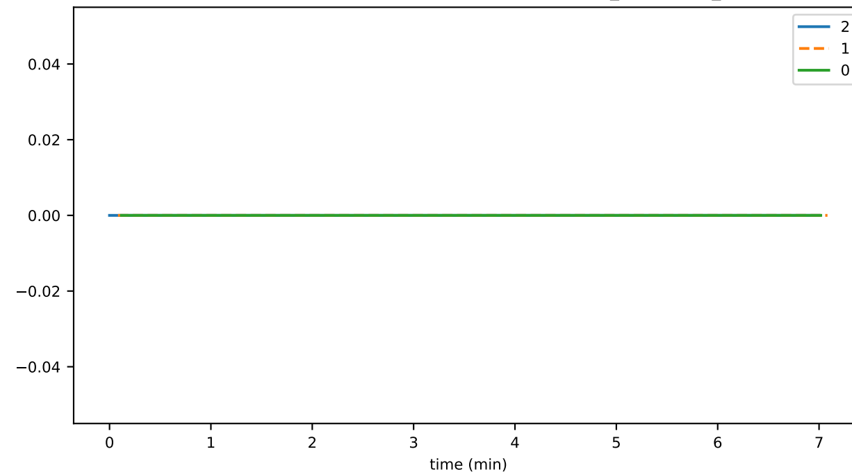
SmartContractService:SystemContractMethodCall_APPROVAL_failed
