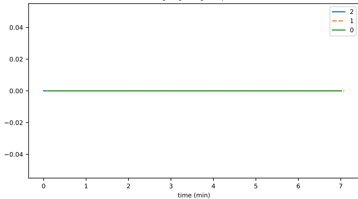
hintsSigningNoSigCompletions
