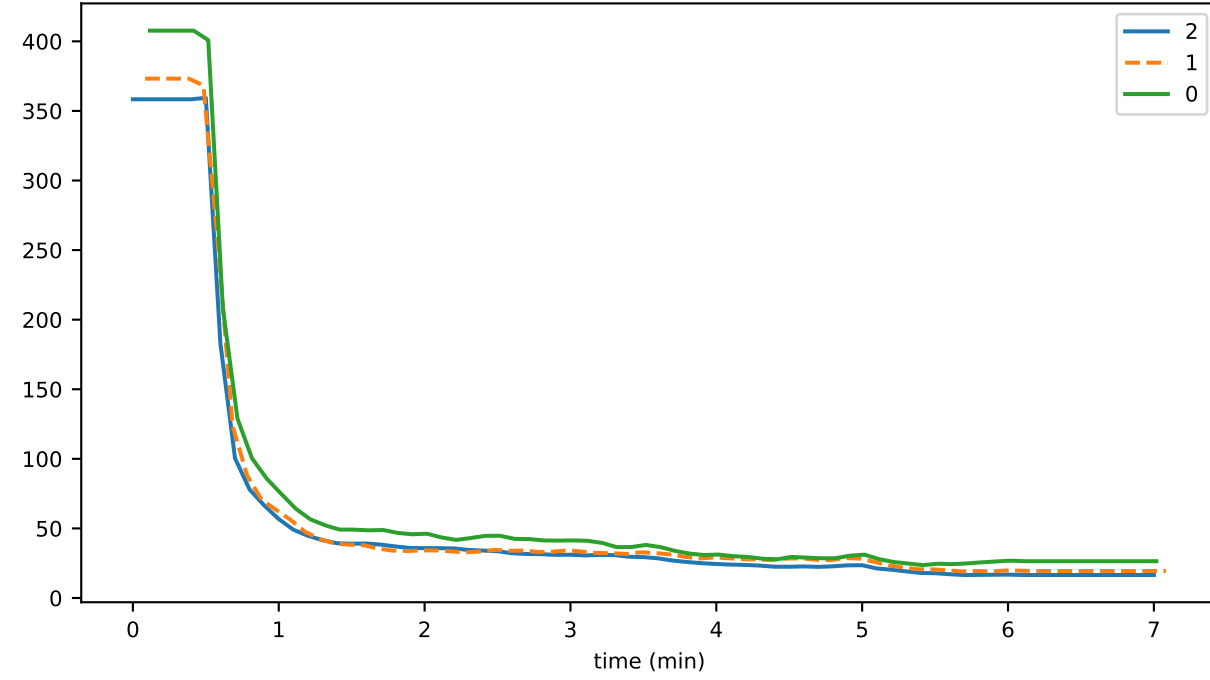
uptimeComputationTime
