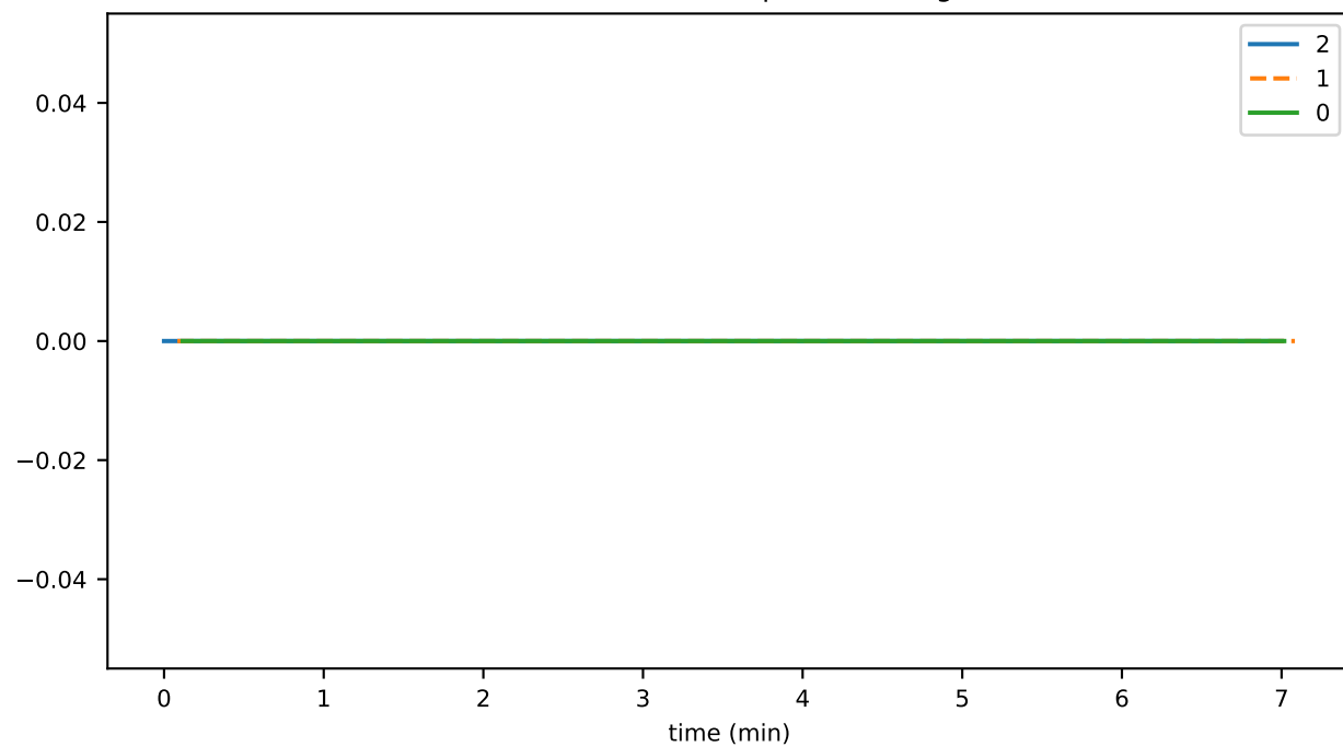
tokenCancelAirdropDurationAvg
