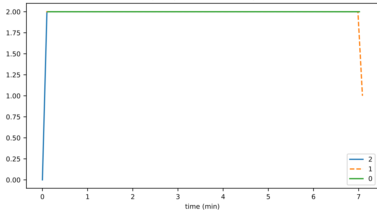
rpcWriteThreadRunning
