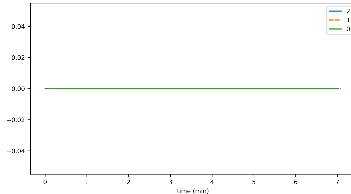
vmap_lifecycle_mergeDurationMs_state
