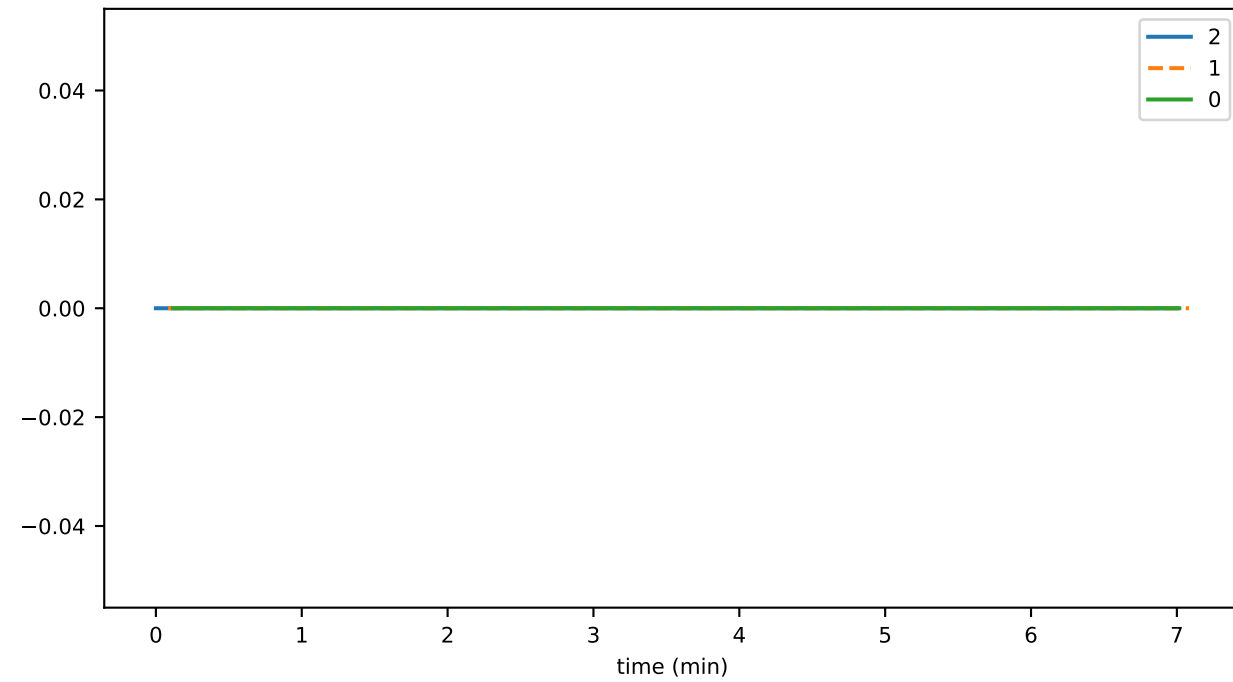
graphDepthUntilConsensusMAX
