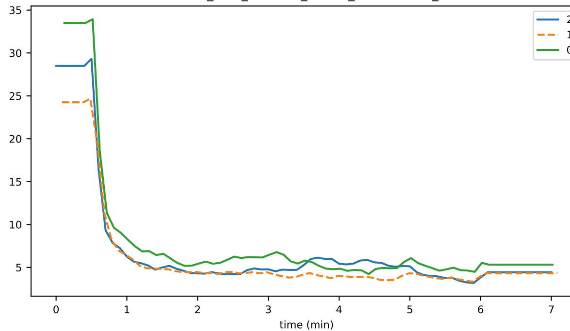
consensus_time_SETTING_EVENT_CONSENSUS_DATA
