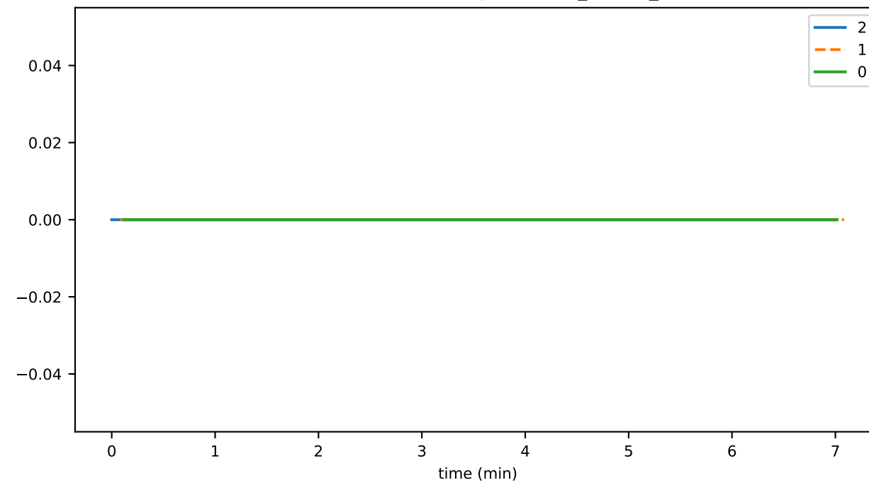
SmartContractService:Rejected_contractCallTx_total
