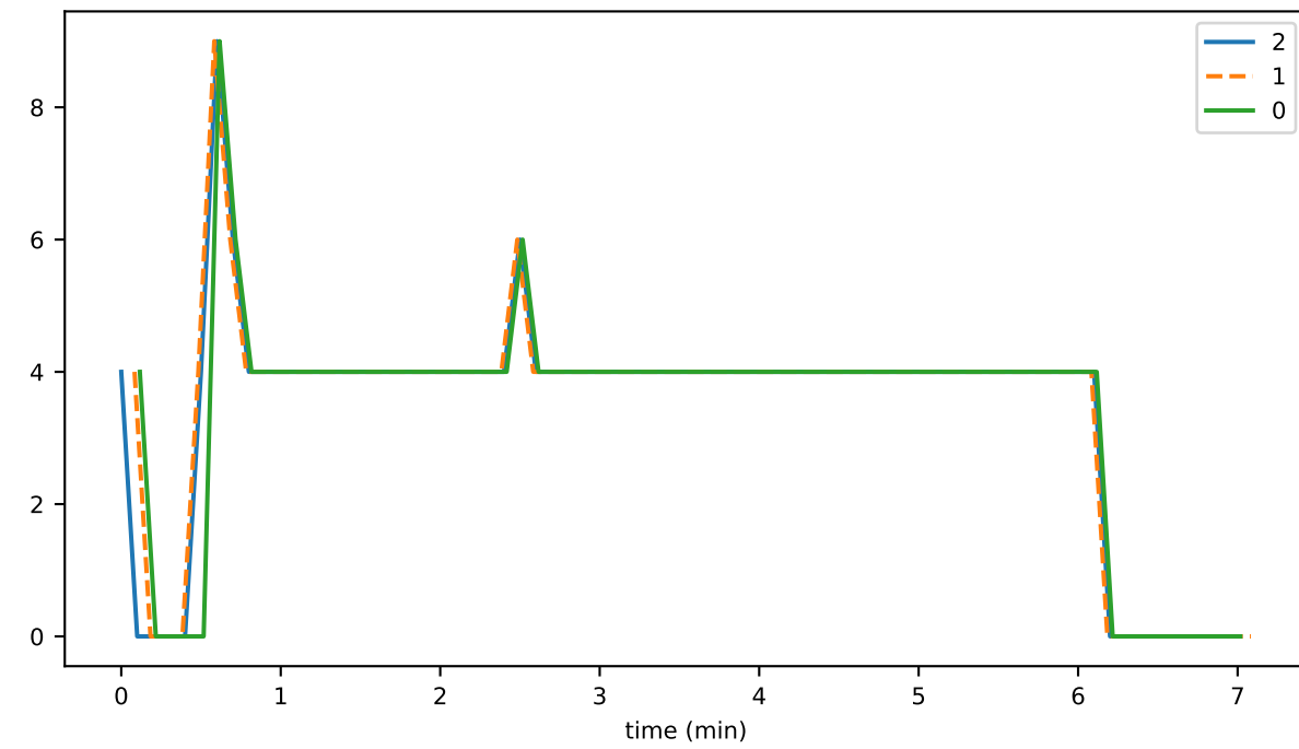
graphDepthUntilConsensusMAX
