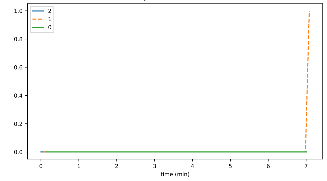
syncPermitsAvailable
