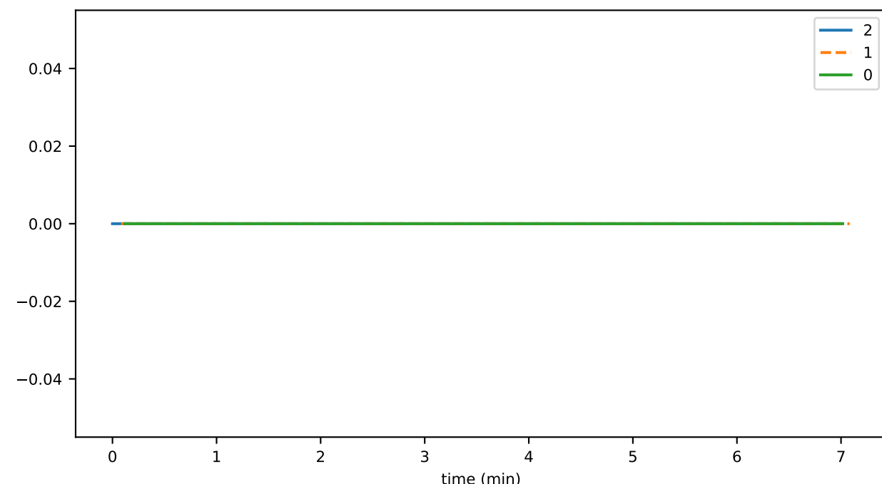
fileCreateDurationMax
