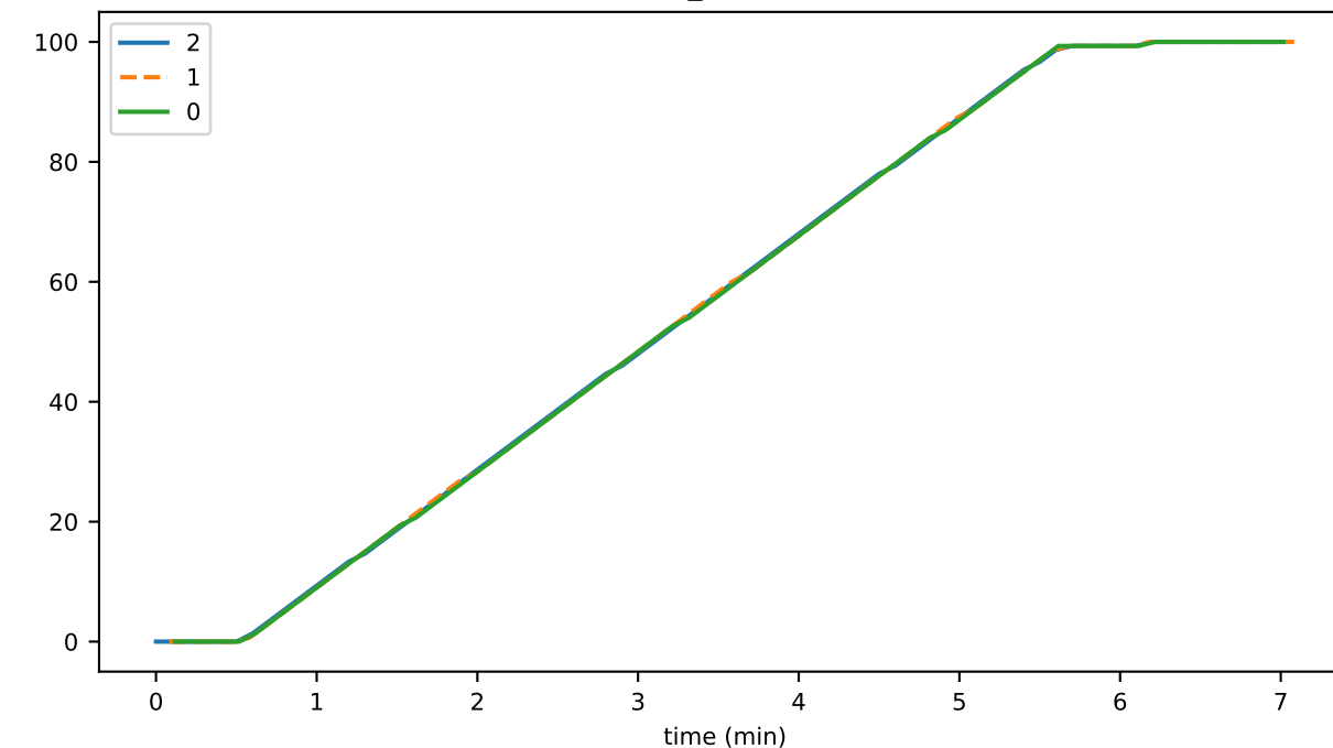
bufferedTransactions
