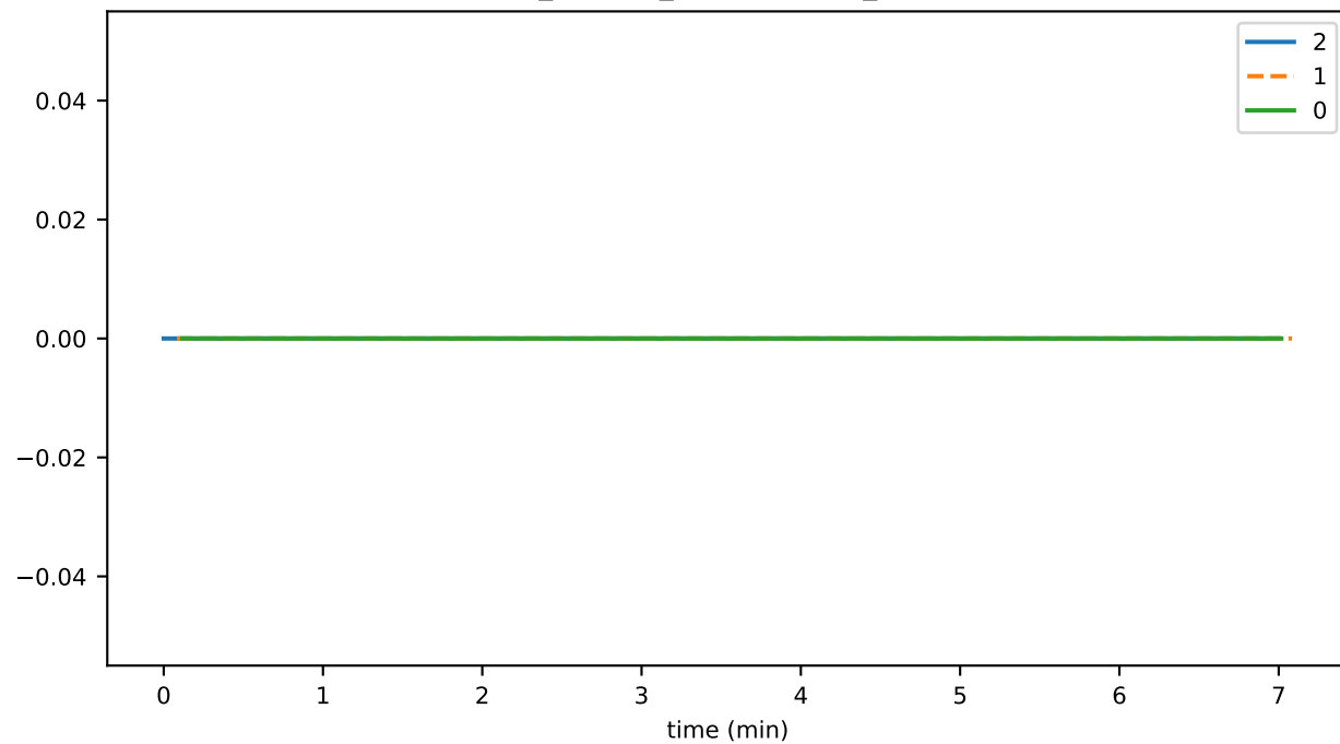
ds_offheap_hashesListMb_state
