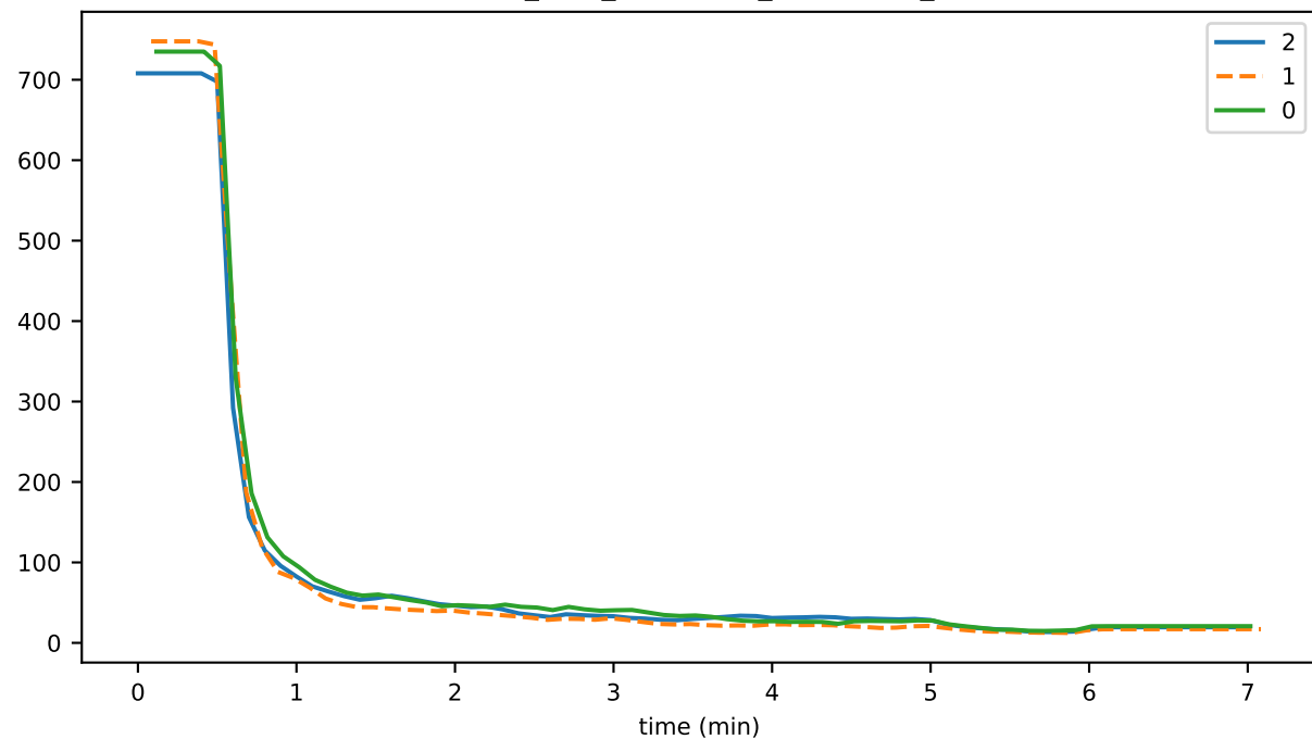
consensus_time_WAITING_FOR_PREHANDLE
