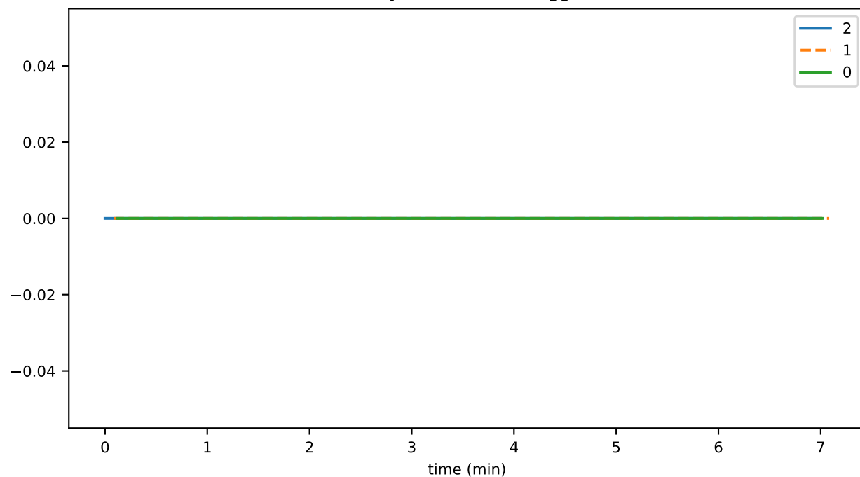
historyProofTransR3ToAggMs
