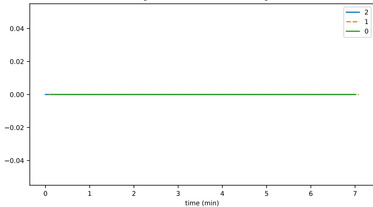
registeredNodeCreateDurationAvg
