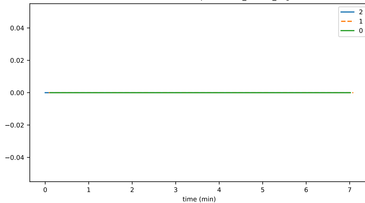
SmartContractService:OpsDuration_PerTxn_avg
