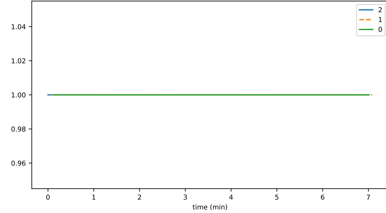
1e6 filesMaxNumber
