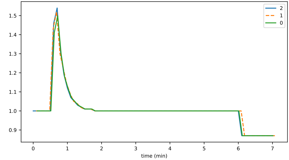
utilPrngDurationAvg
