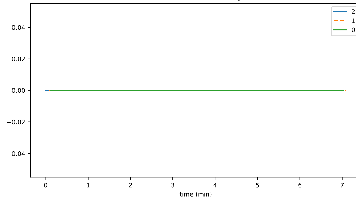
tokenDeleteDurationAvg
