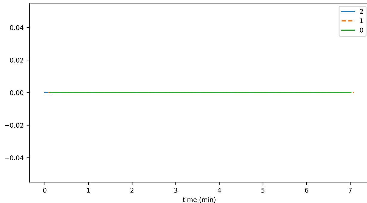
hintsKeyPublicationThrottledTxns
