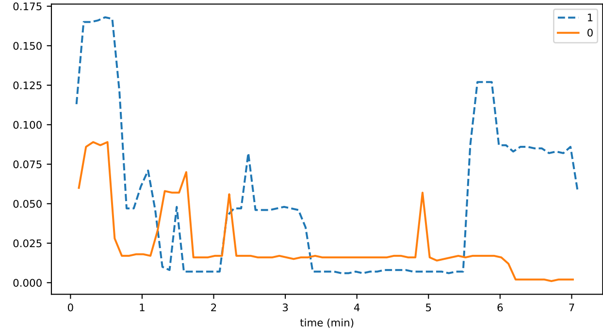
sync_phase_02_fraction_EXCHANGING_WINDOWS
