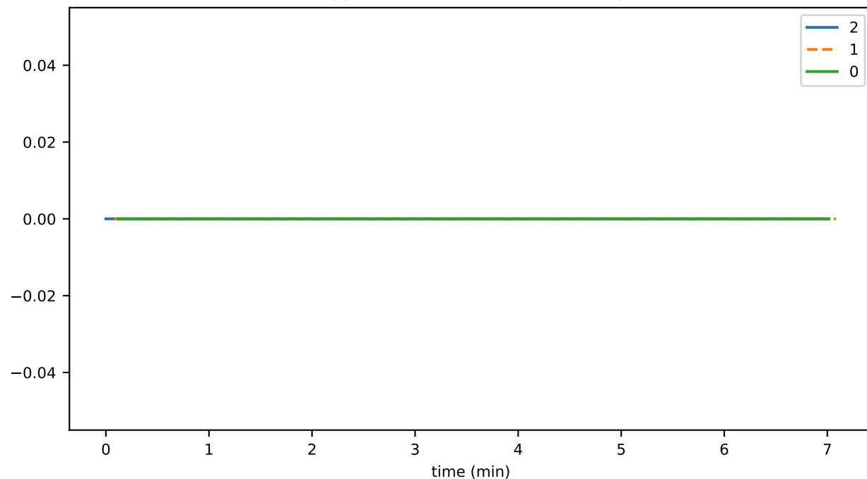
cryptoDeleteLiveHashThrottledTxns
