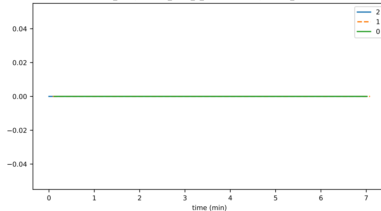
ds_compactions_level_9_hashesSavedSpaceMb_state
