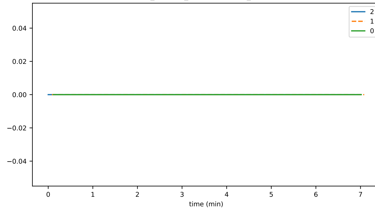
ds_offheap_leavesIndexMb_state
