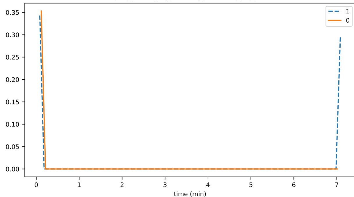
sync_phase_02_fraction_RECEIVING_EVENTS
