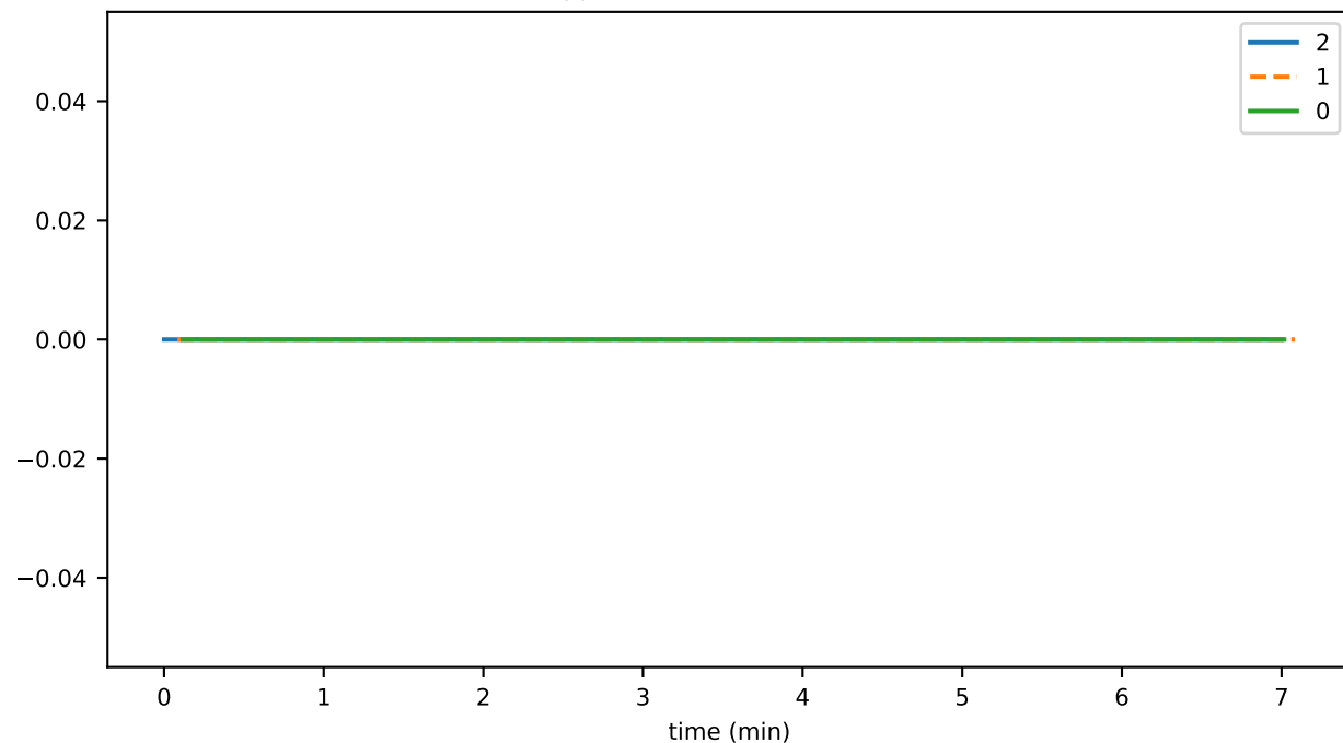
cryptoGetLiveHashDurationMax
