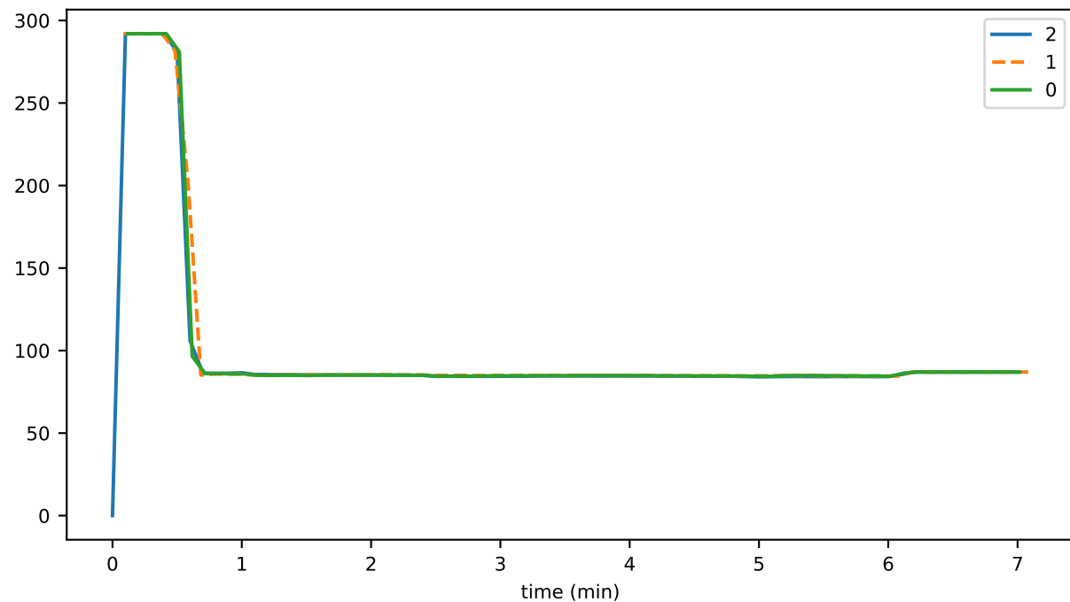
lambdaSStoreDurationMax
