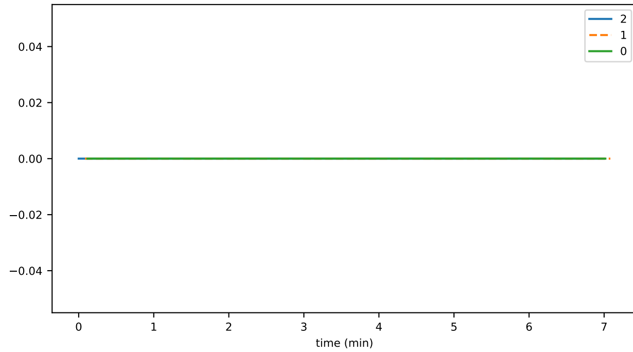
eventsWithTooManyTransactionBytes
