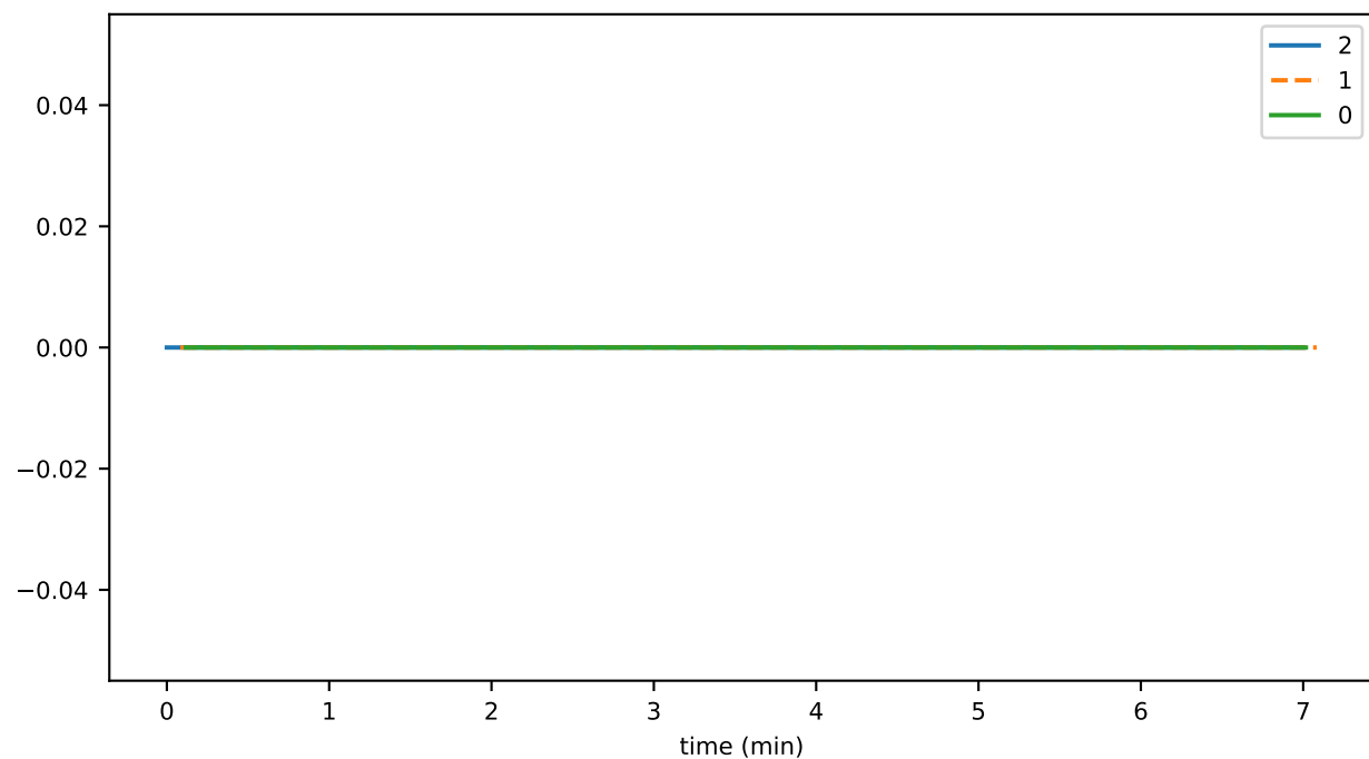
nodeActivePercent_node0
