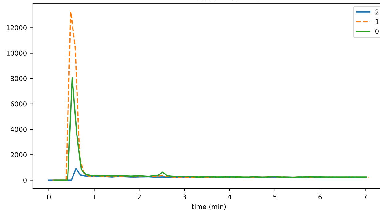
eventDelay_6_pces_runtime
