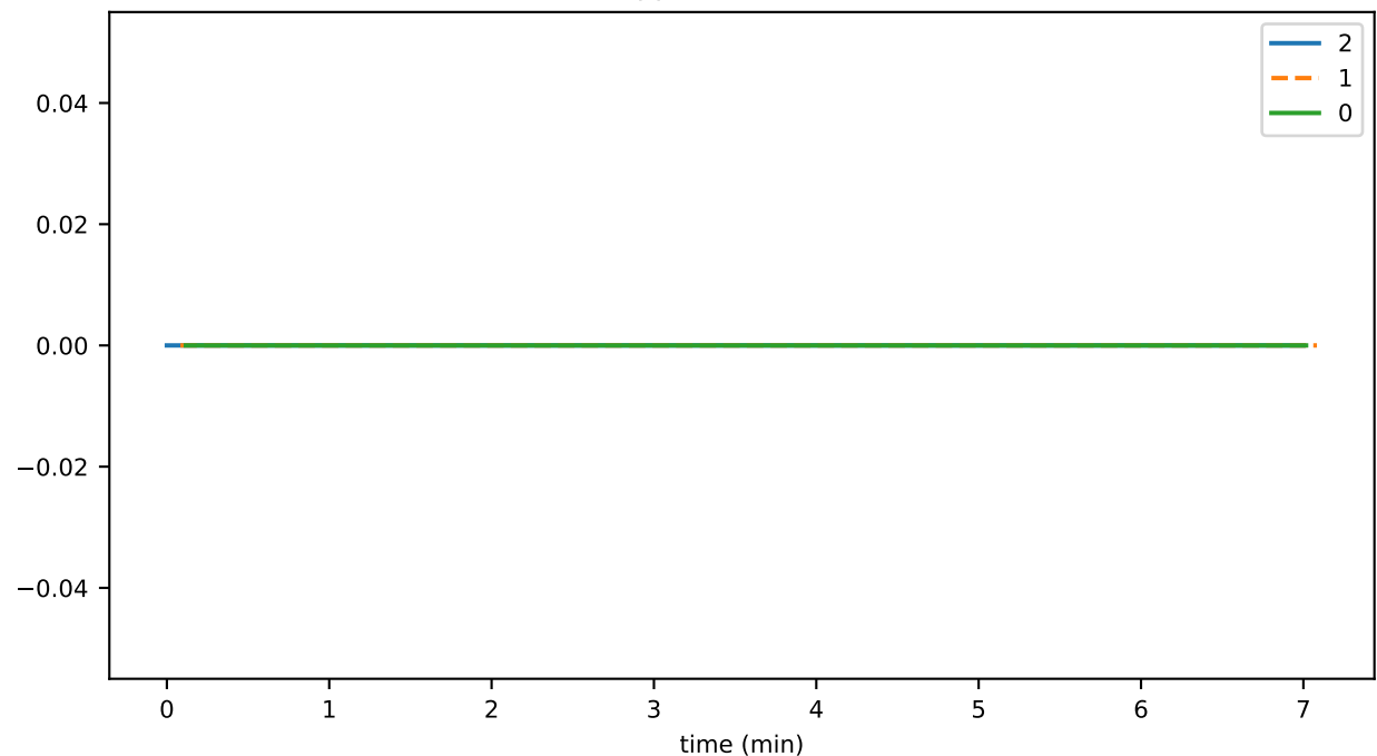
fileCreateDurationAvg
