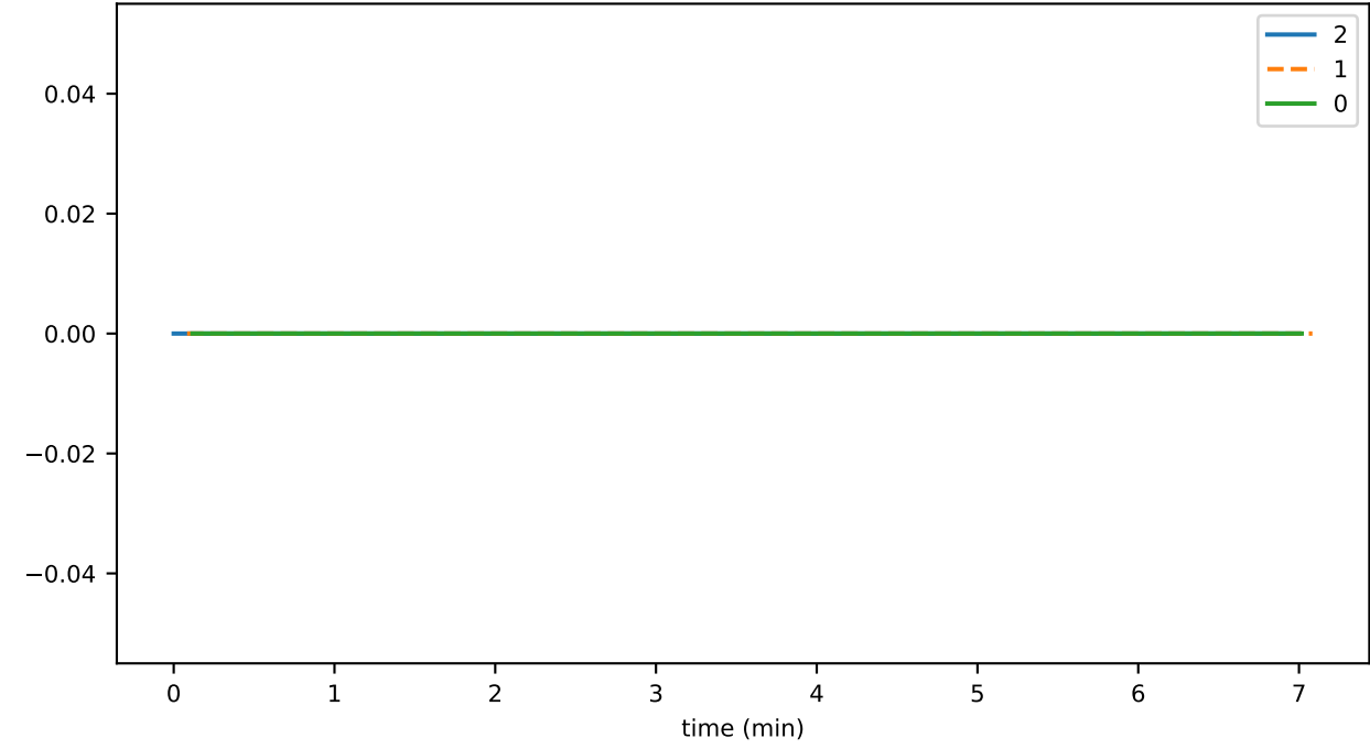
tokenGrantKycToAccountDurationAvg
