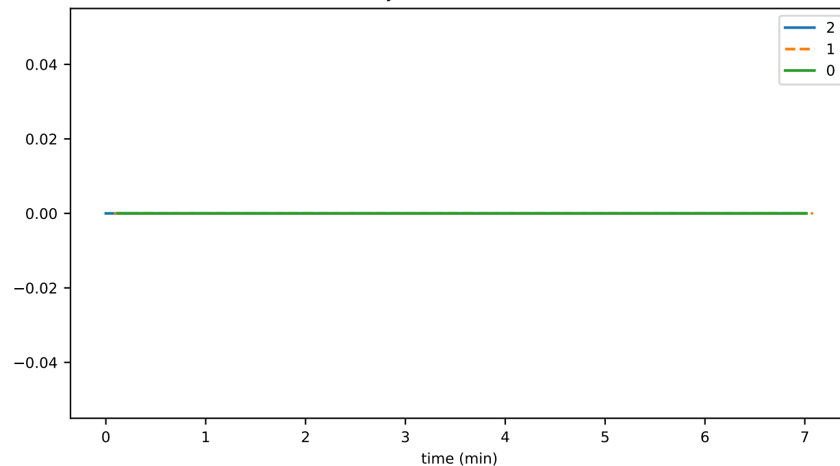
historyProofTransR1ToR2Cnt
