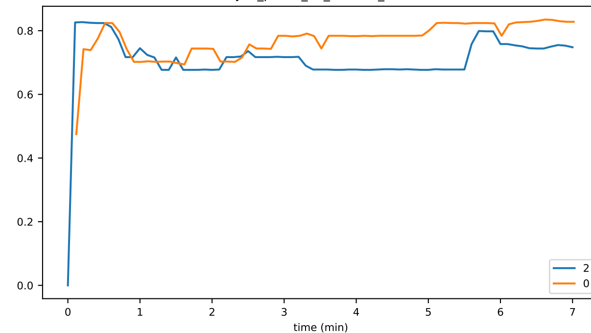
sync_phase_01_fraction_OTHER_FALLEN_BEHIND
