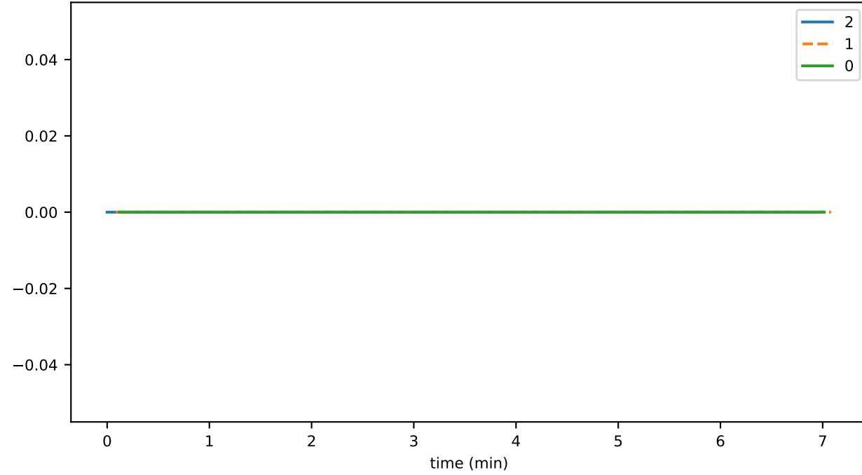
NonGovernanceOversizedTxnsRcv
