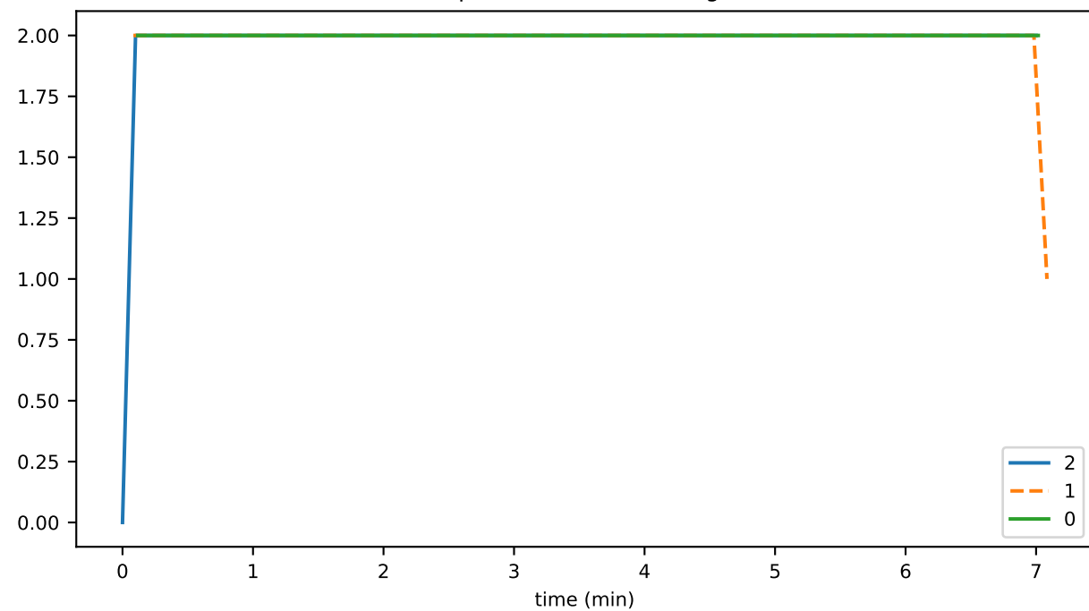
rpcWriteThreadRunning
