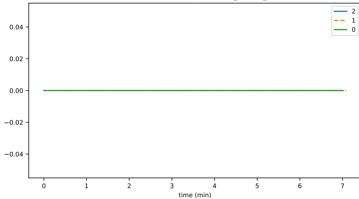
SmartContractService:OpsDuration_TxnsThrottled
