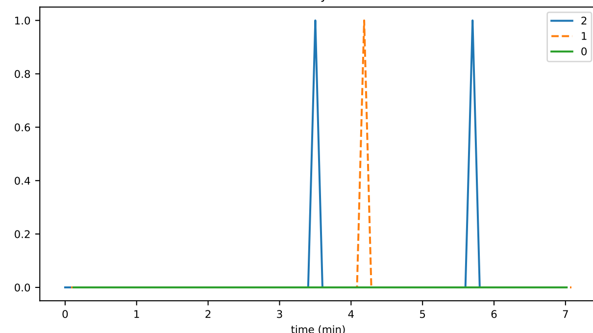
bufferedPriorityTransactions
