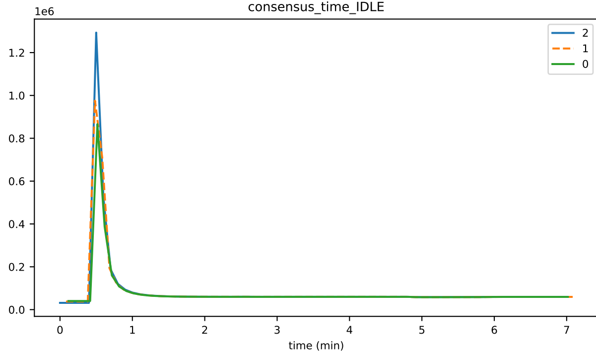
consensus_time_IDLE
