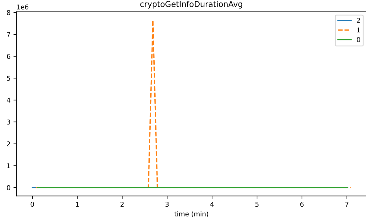
cryptoGetInfoDurationAvg
