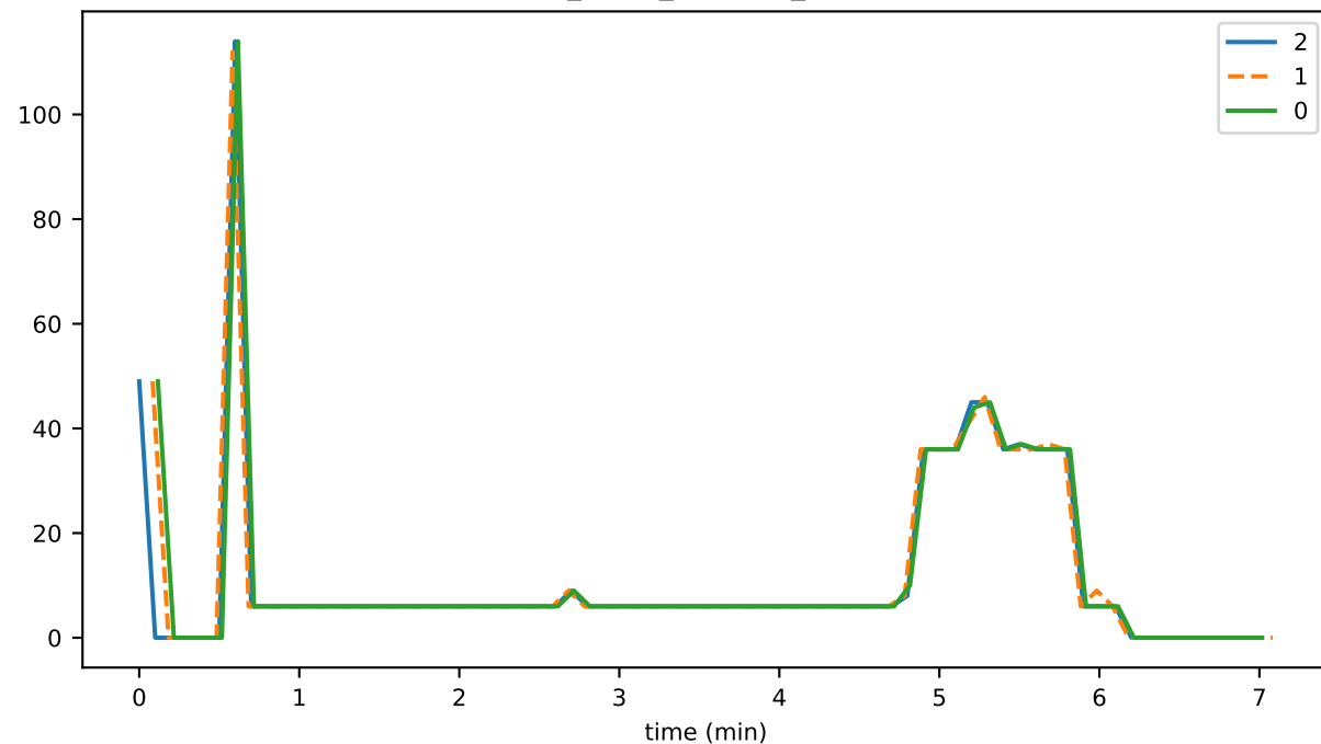
ds_reads_leafKeys_state
