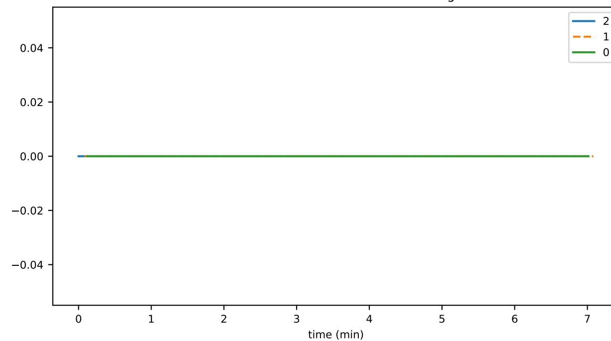
tokenGetAccountNftInfosDurationAvg
