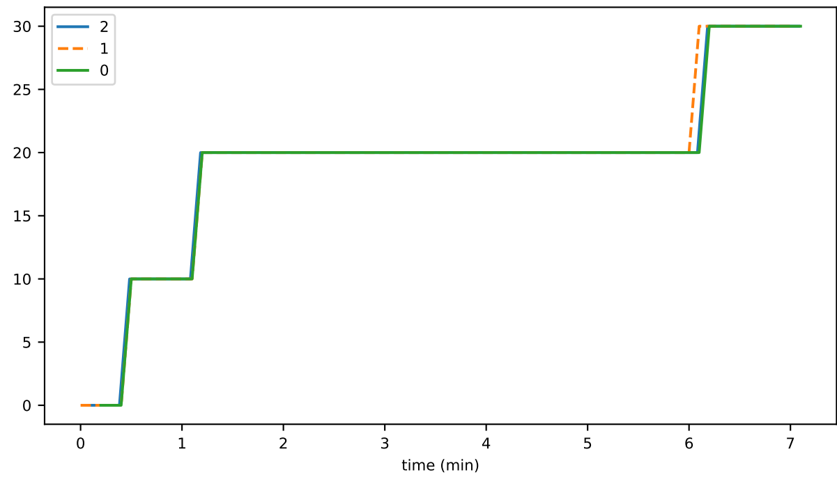
directMemInMB
