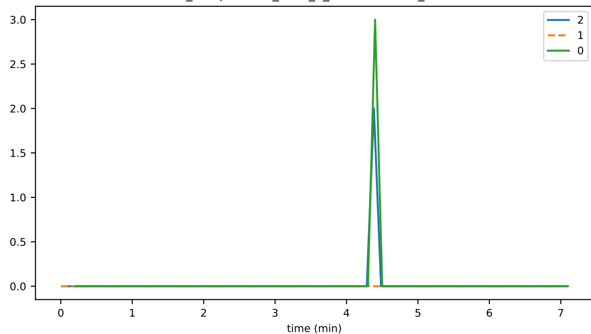
ds_compactions_level_3_hashesTimeMs_state
