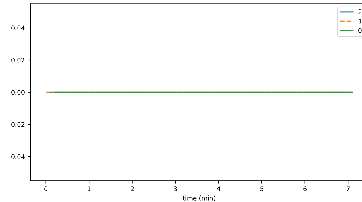
numIndirectProofs
