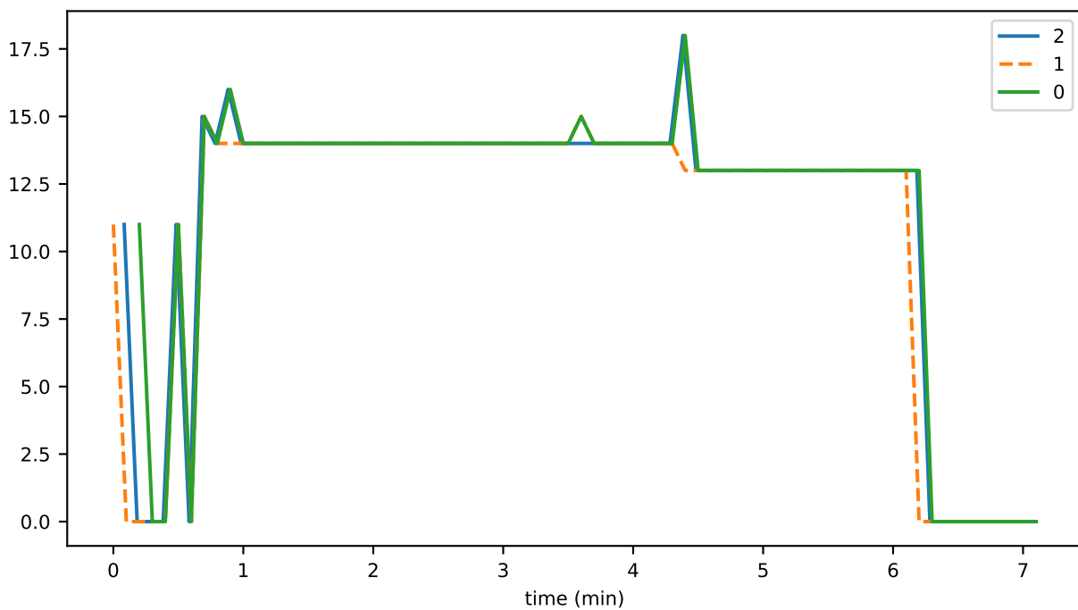
numEventsAddedUntilConsensusMAX
