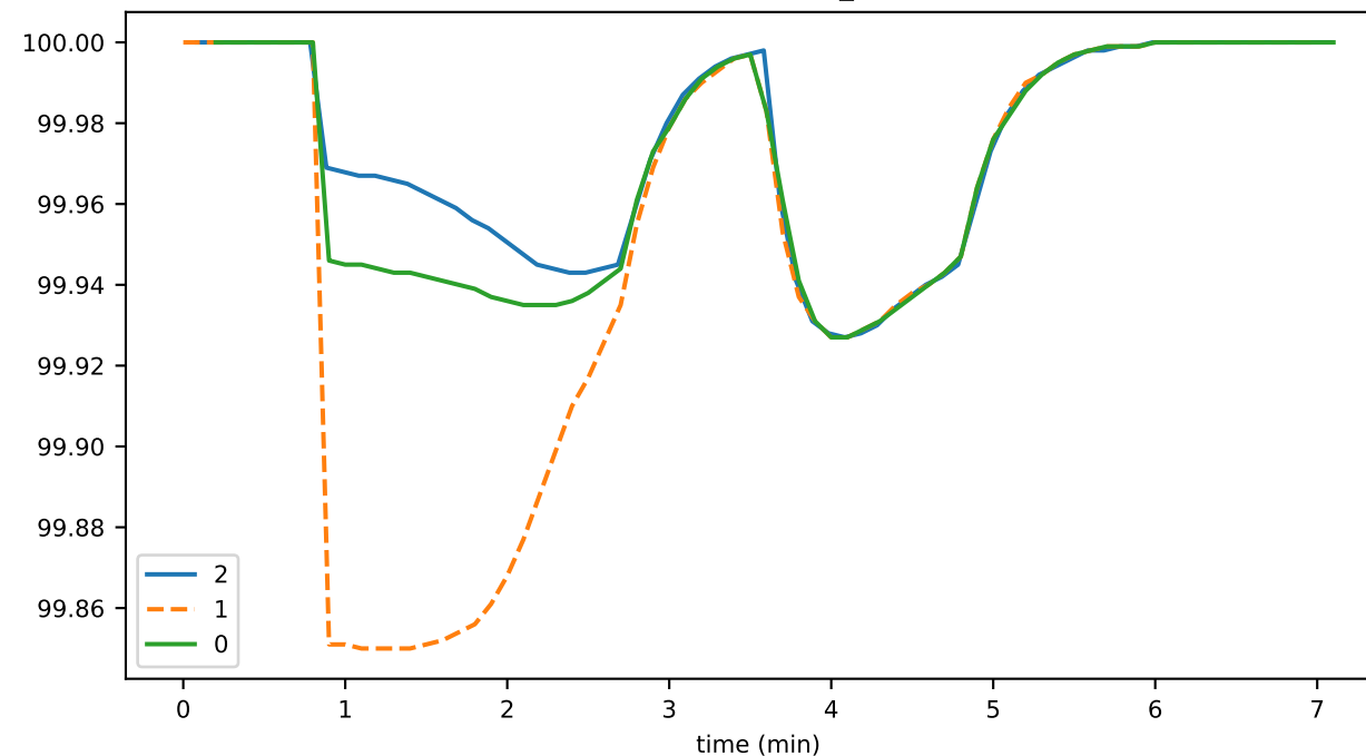
nodeActivePercentSnapshot_node0
