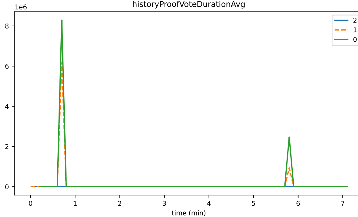
historyProofVoteDurationAvg
