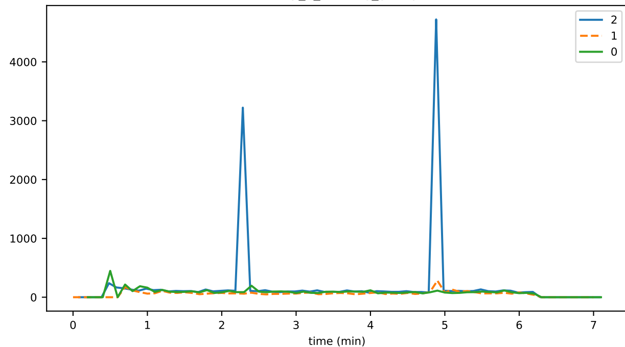
eventDelay_1_hashing_storageMAX
