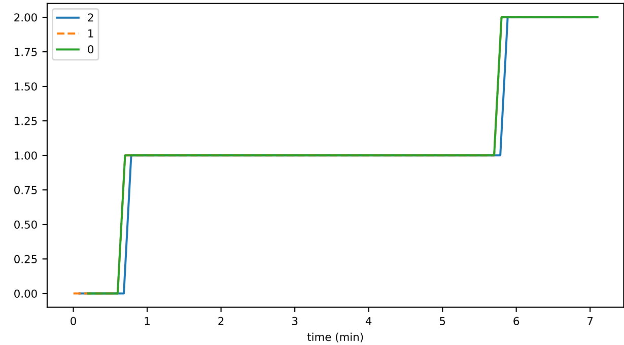
historyProofTransR3ToAggCnt
