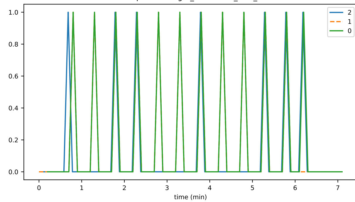
StateSnapshotManager_unhandled_task_count
