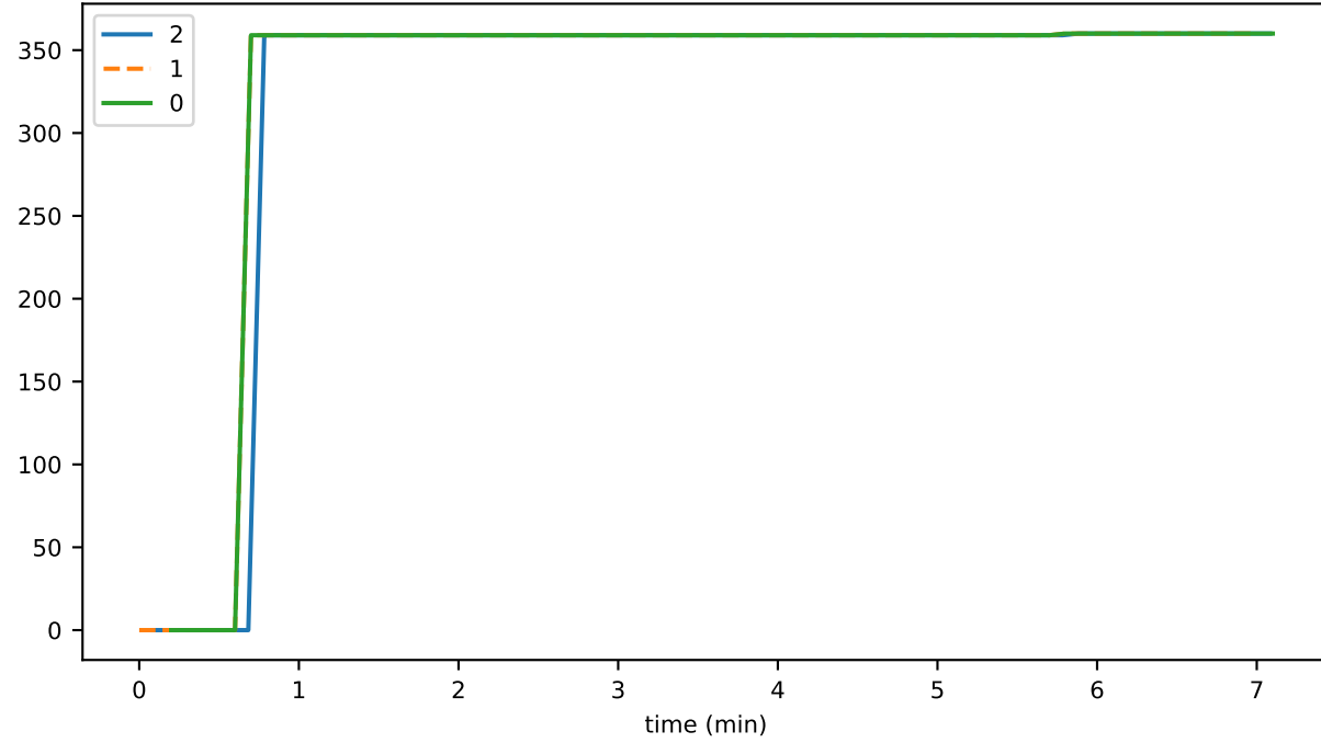
historyProofTransR2ToR3Ms
