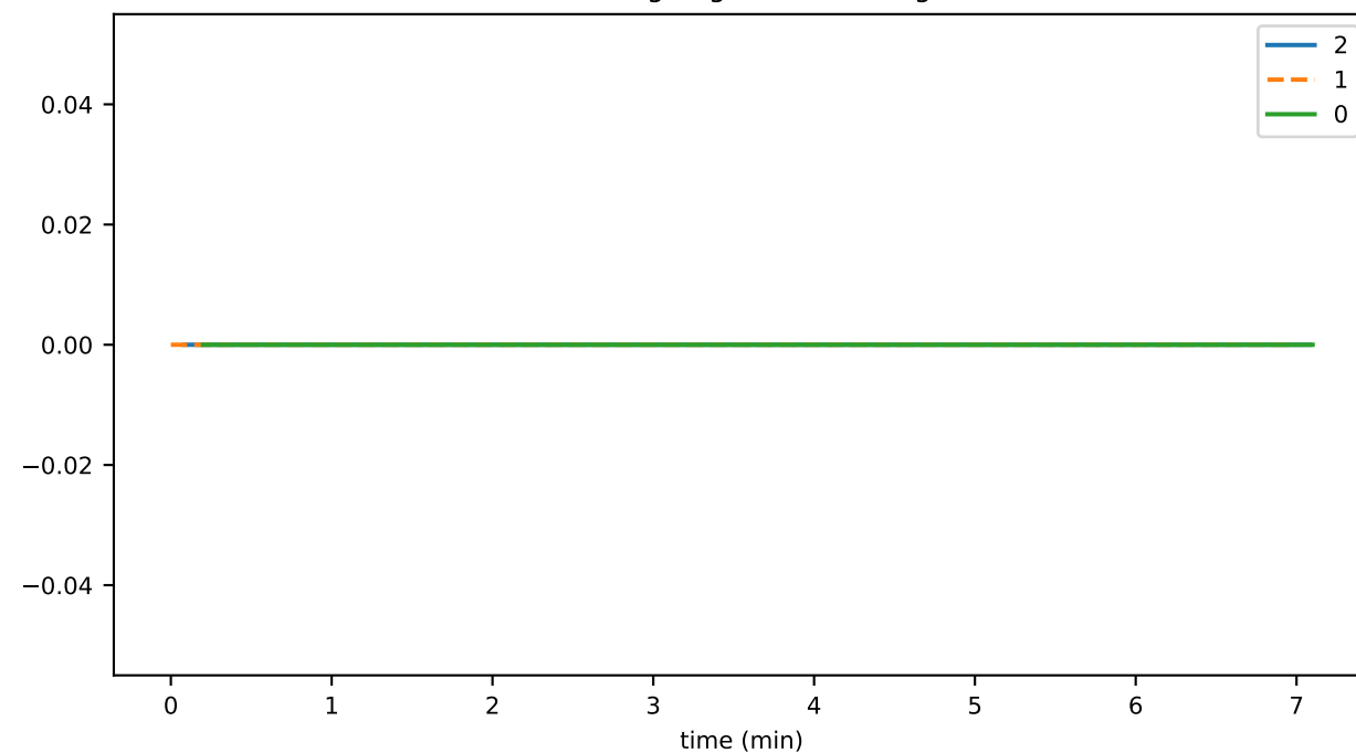
historyAssemblySignatureDurationMax
