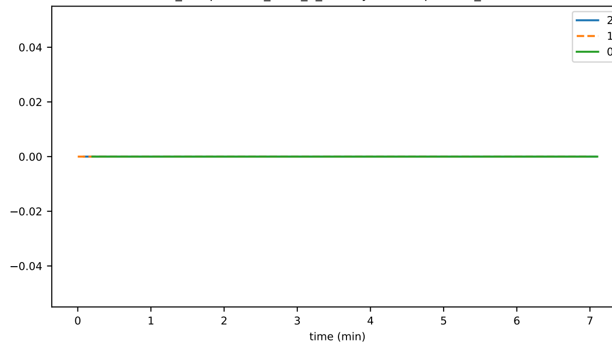
ds_compactions_level_3_leafKeysSavedSpaceMb_state
