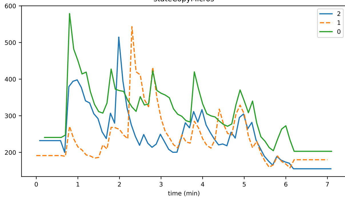
stateCopyMicros
