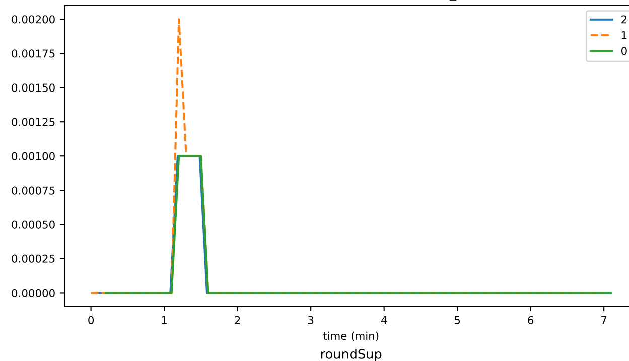
roundsSinceLastConsensusEvent_1
