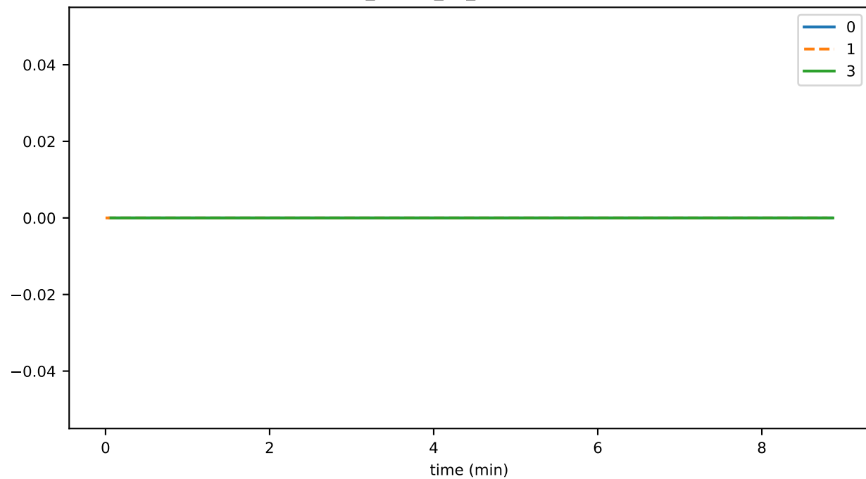
rpc_output_02_queueMinSize
