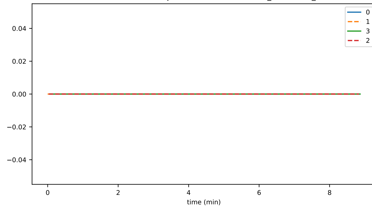
SmartContractService:SystemContractMethodCall_TRANSFER_total
