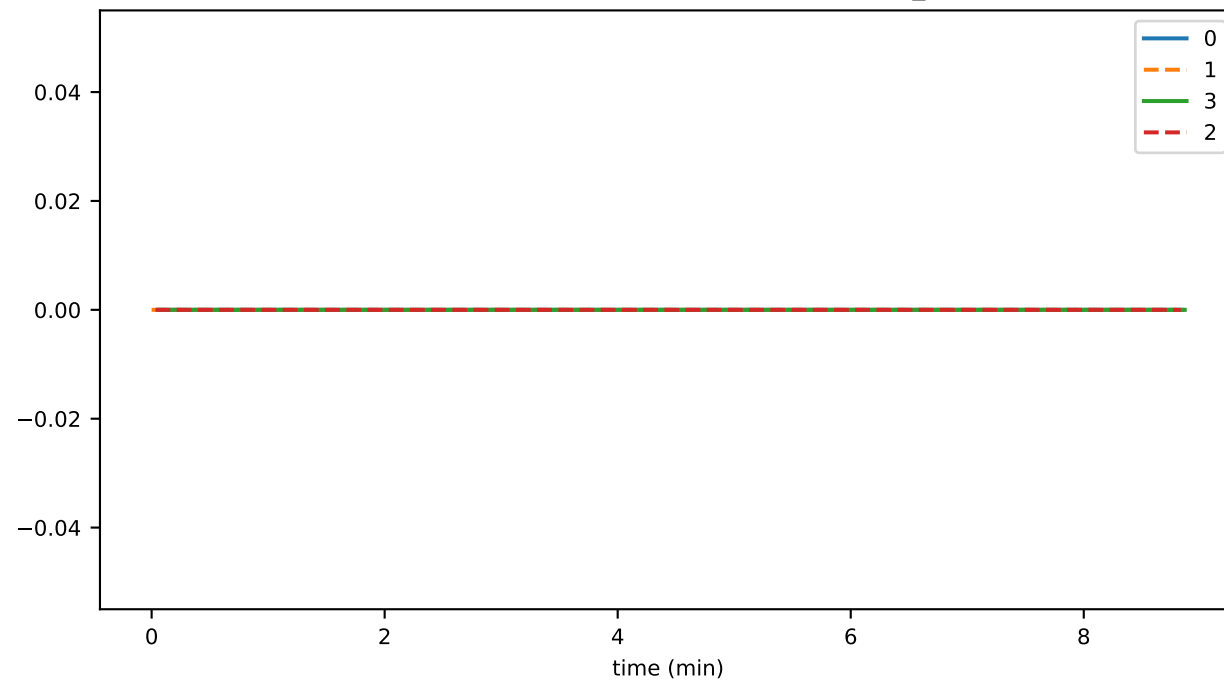
SmartContractService:TransactionGasUsed_avg
