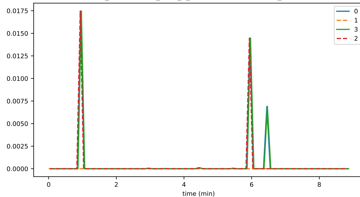
ds_compactions_level_1_leavesSavedSpaceMb_state
