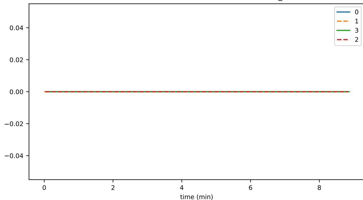
SmartContractService:OpsDuration_PerTxn_avg
