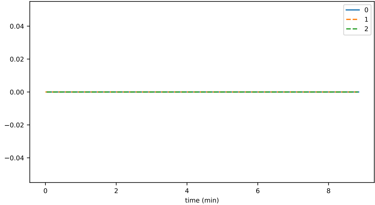
sync_phase_03_fraction_SELF_FALLEN_BEHIND
