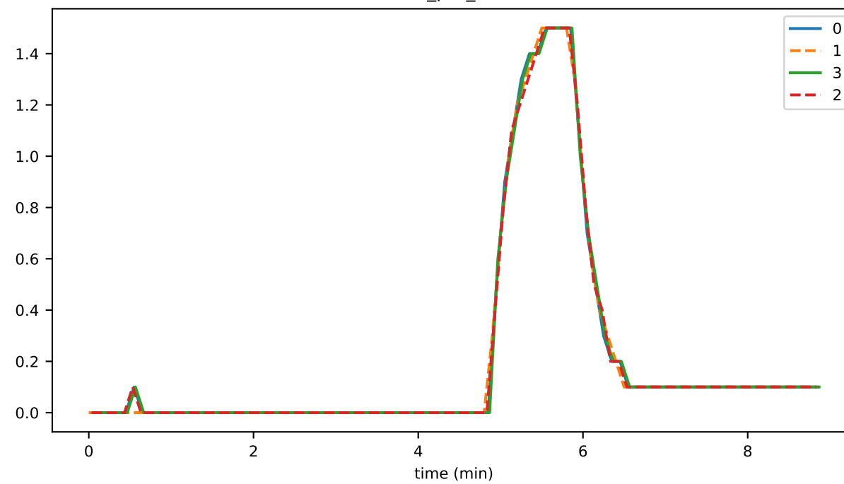
trans_per_event
