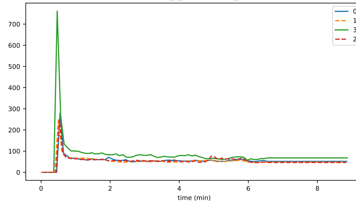
eventDelay_3_deduplication_gossip
