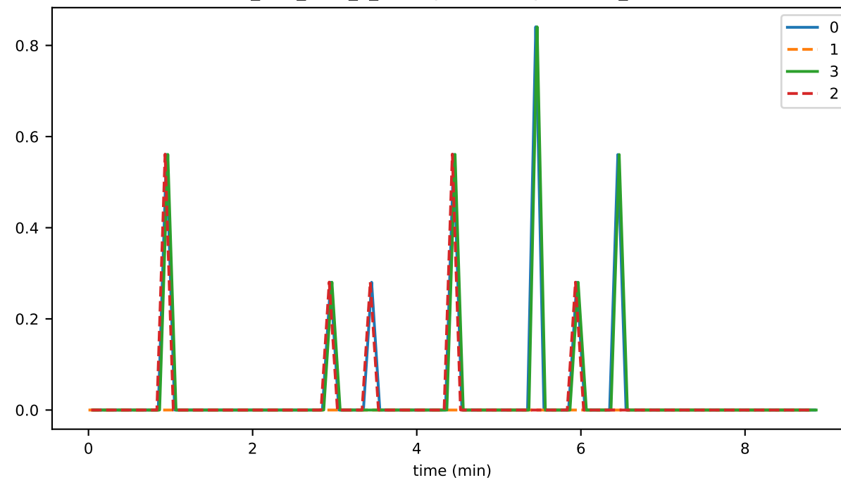
ds_files_level_3_hashesFileSizeByLevelMb_state
