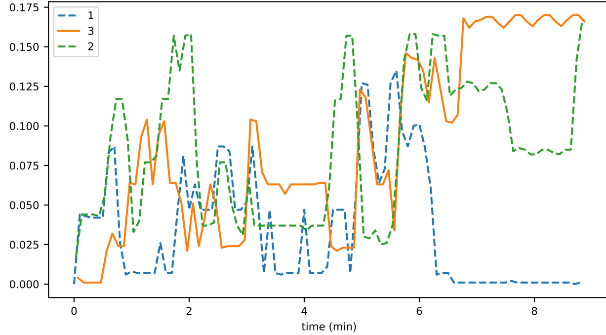
sync_phase_00_fraction_EXCHANGING_WINDOWS
