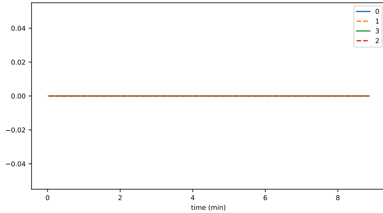
sigStateHash
