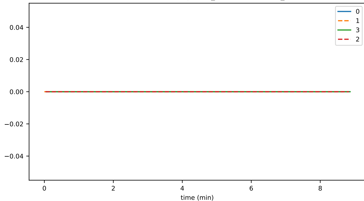
SmartContractService:Rejected_ethereumTx_total
