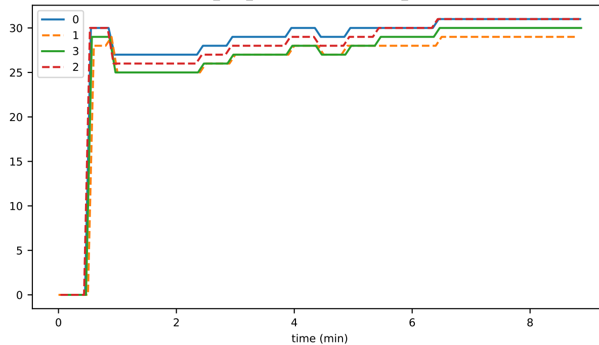
ds_files_leafKeysStoreFileCount_state
