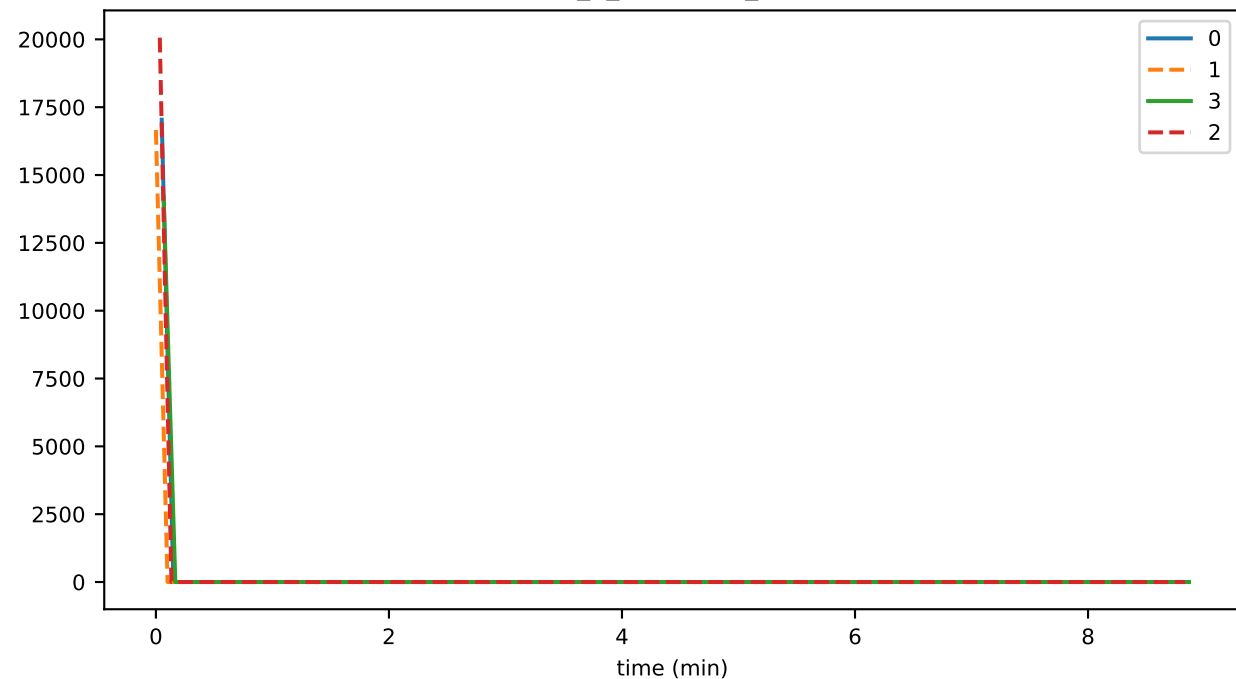
eventDelay_2_validation_storageMAX
