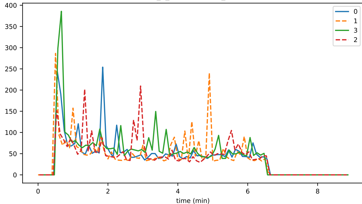
eventDelay_3_deduplication_runtimeMAX
