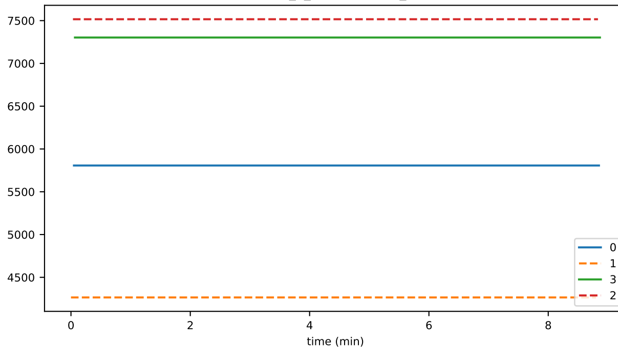
eventDelay_3_deduplication_storage
