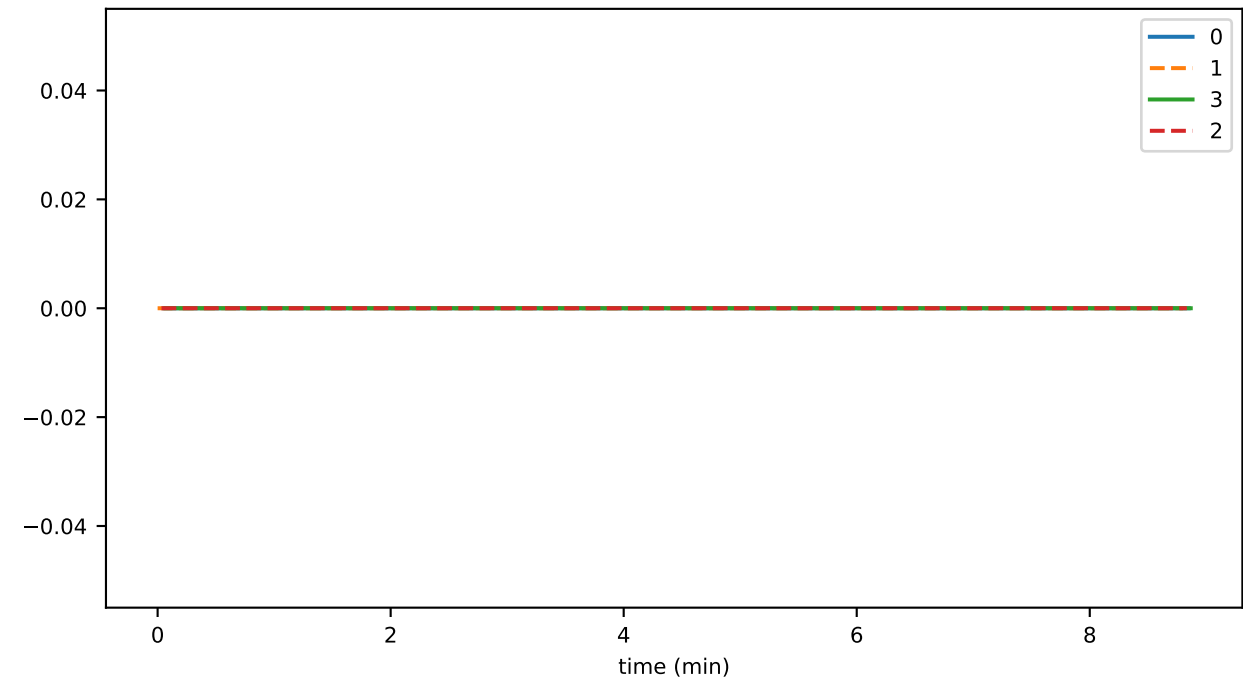
ds_files_level_8_leafKeysFileSizeByLevelMb_state
