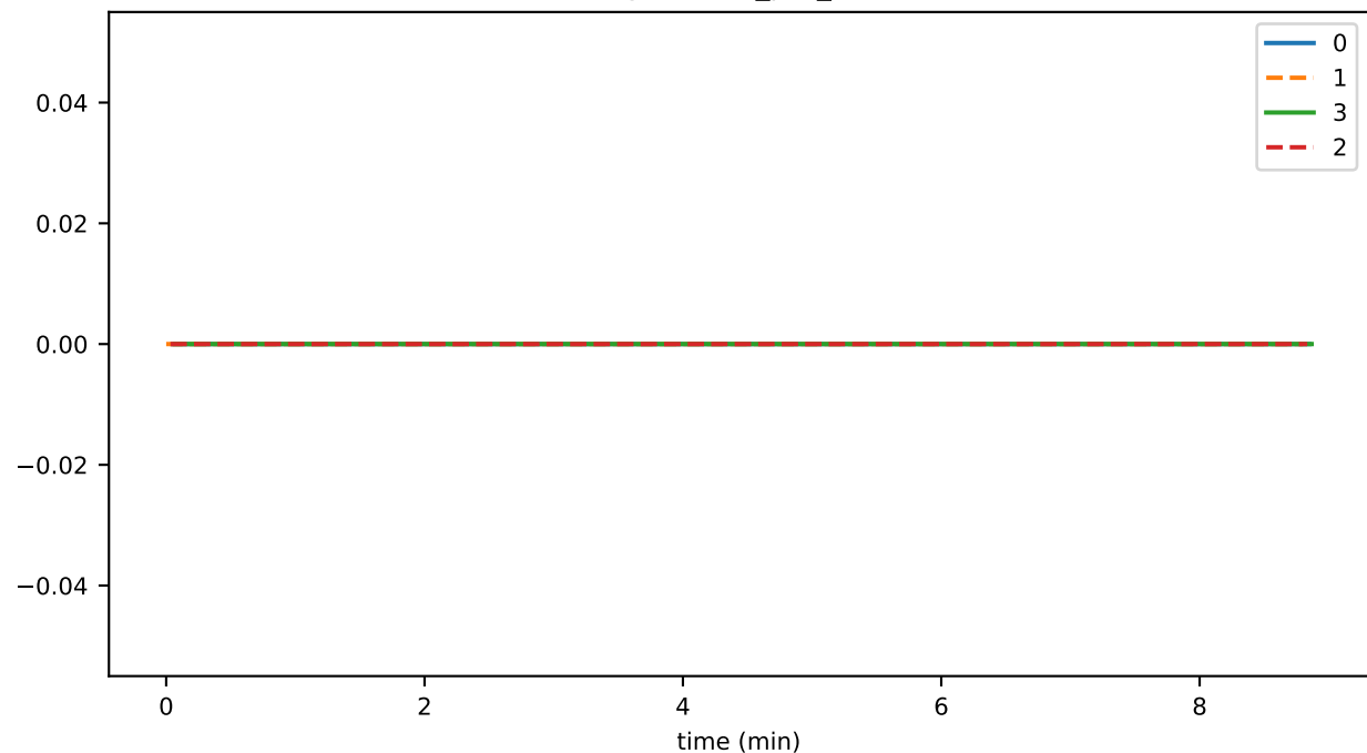
SigIntakeEnqueueTime
