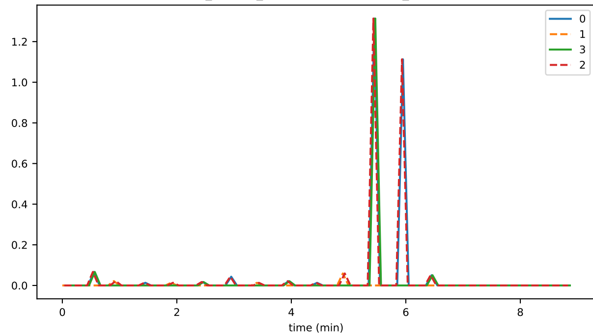
ds_flushes_leavesStoreFileSizeMb_state
