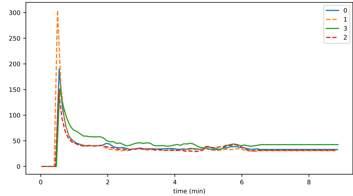
eventDelay_4_verification_runtime
