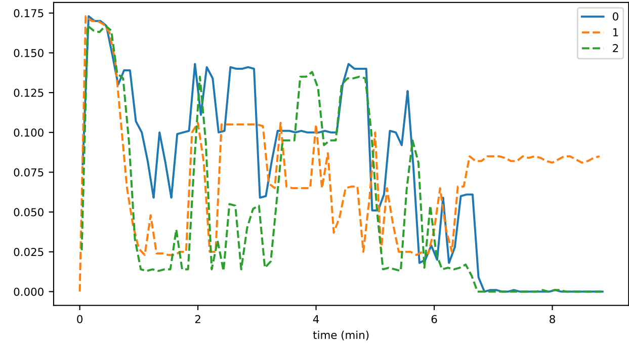
sync_phase_03_fraction_SENDING_EVENTS
