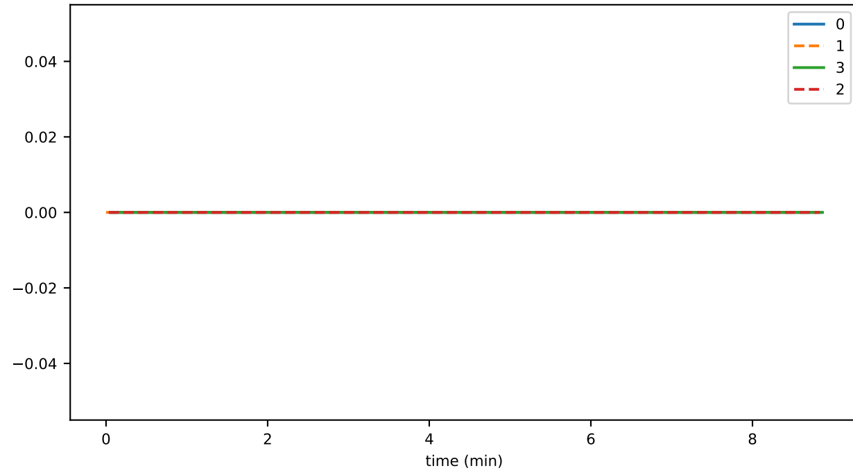
ds_compactions_level_10_hashesTimeMs_state
