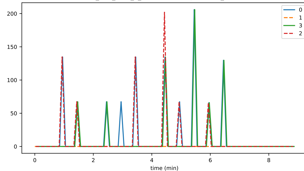
ds_files_level_10_leafKeysFileSizeByLevelMb_state
