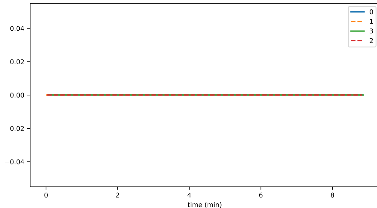
cryptoDeleteDurationMax
