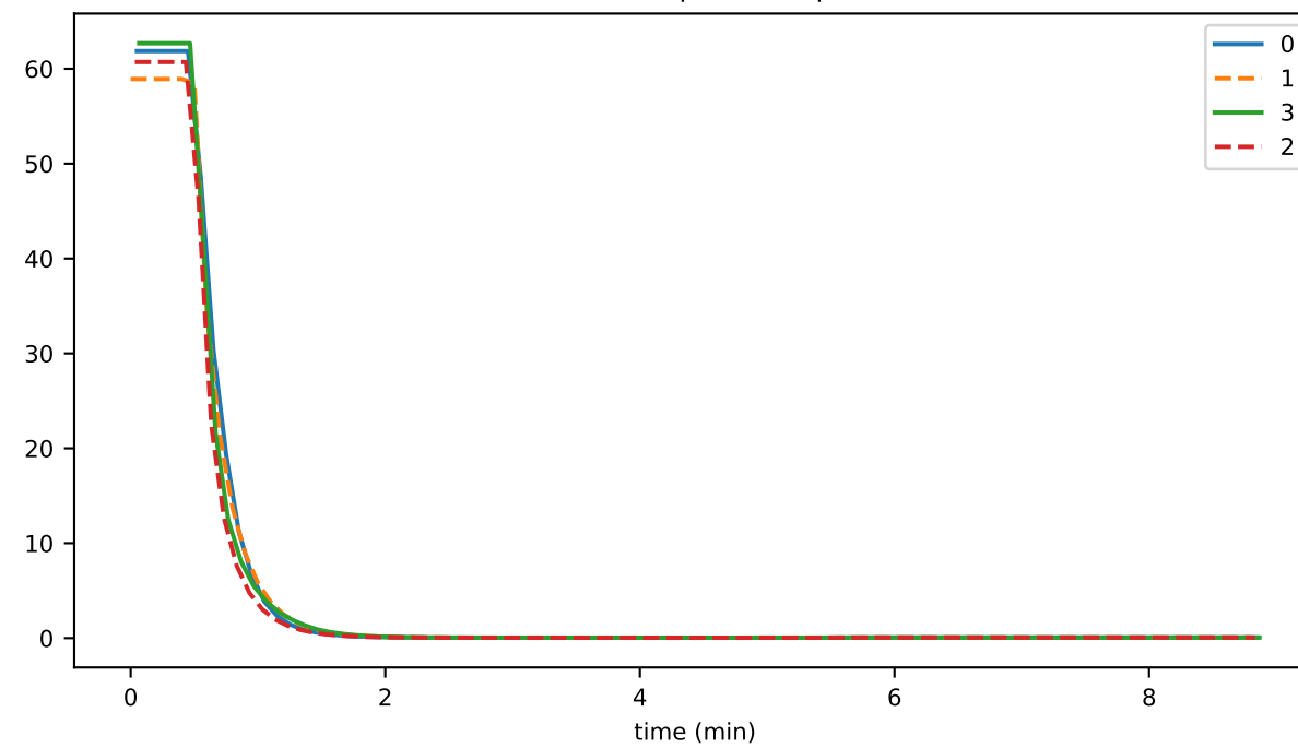
secGossipRoundtrip
