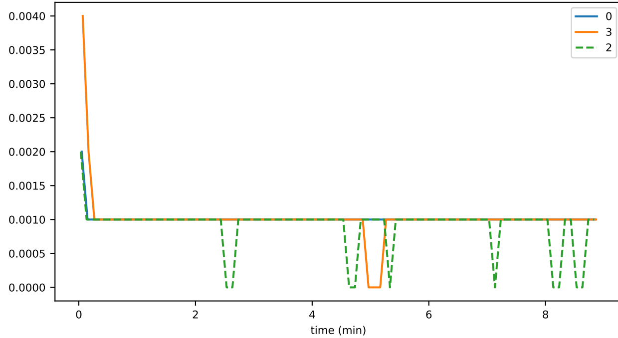
sync_phase_01_fraction_EXCHANGING_WINDOWS
