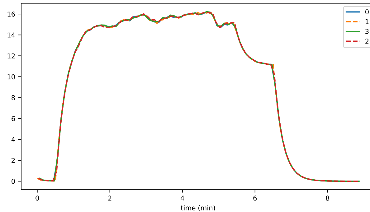
rounds_per_sec
