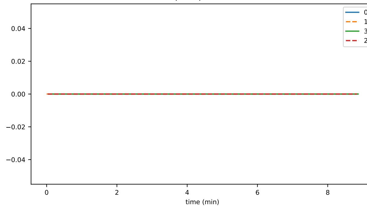
sync_per_secR
