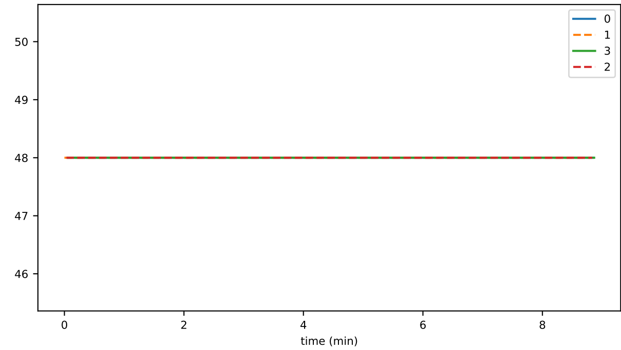
receiverReconnectDurationSeconds
