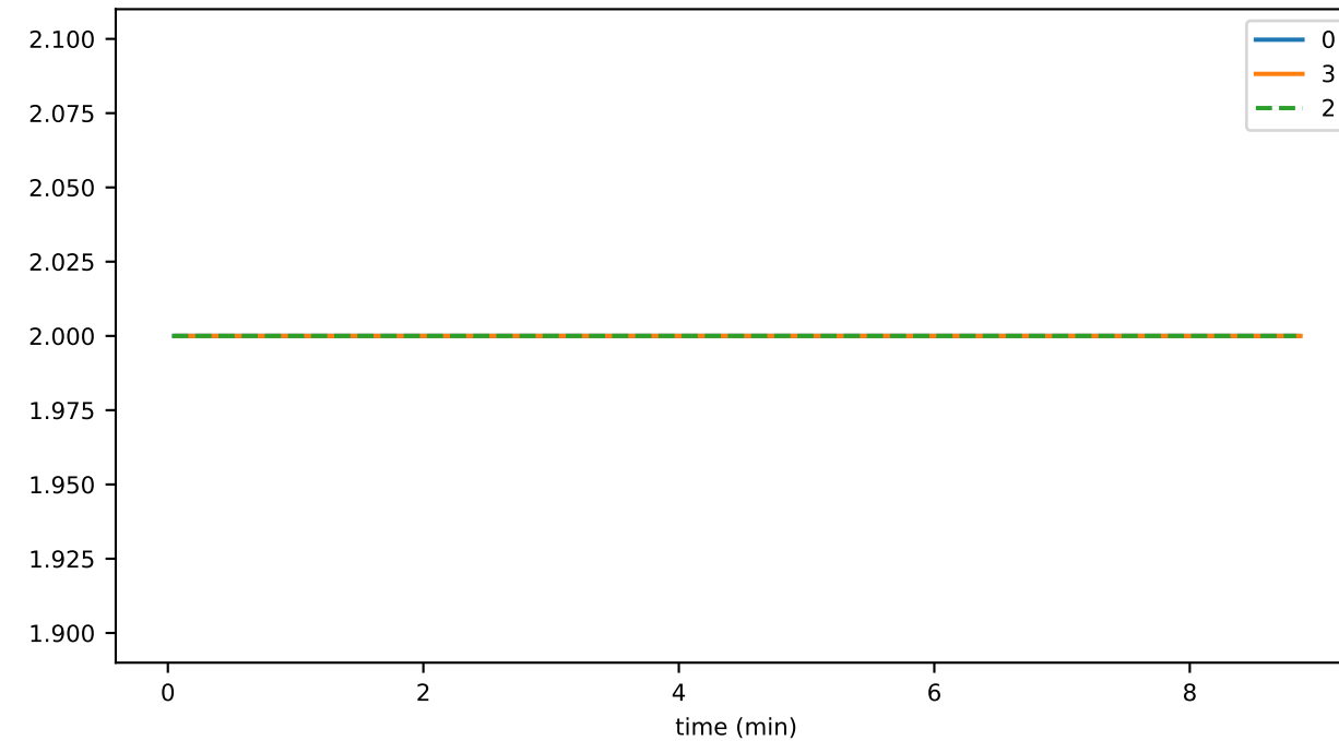
rpc_output_01_queueMaxSize
