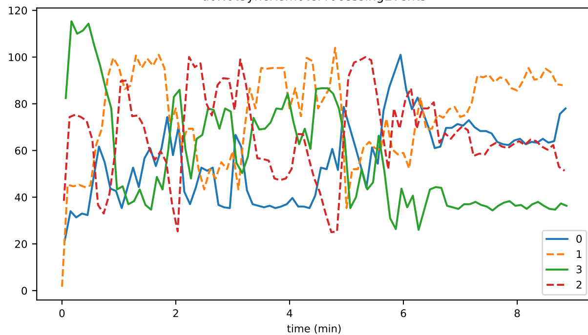
doNotSyncRemoteProcessingEvents
