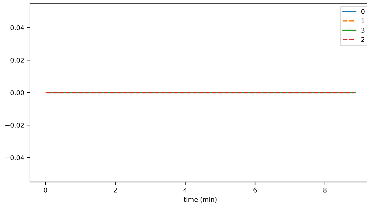
stateCopyMicros
