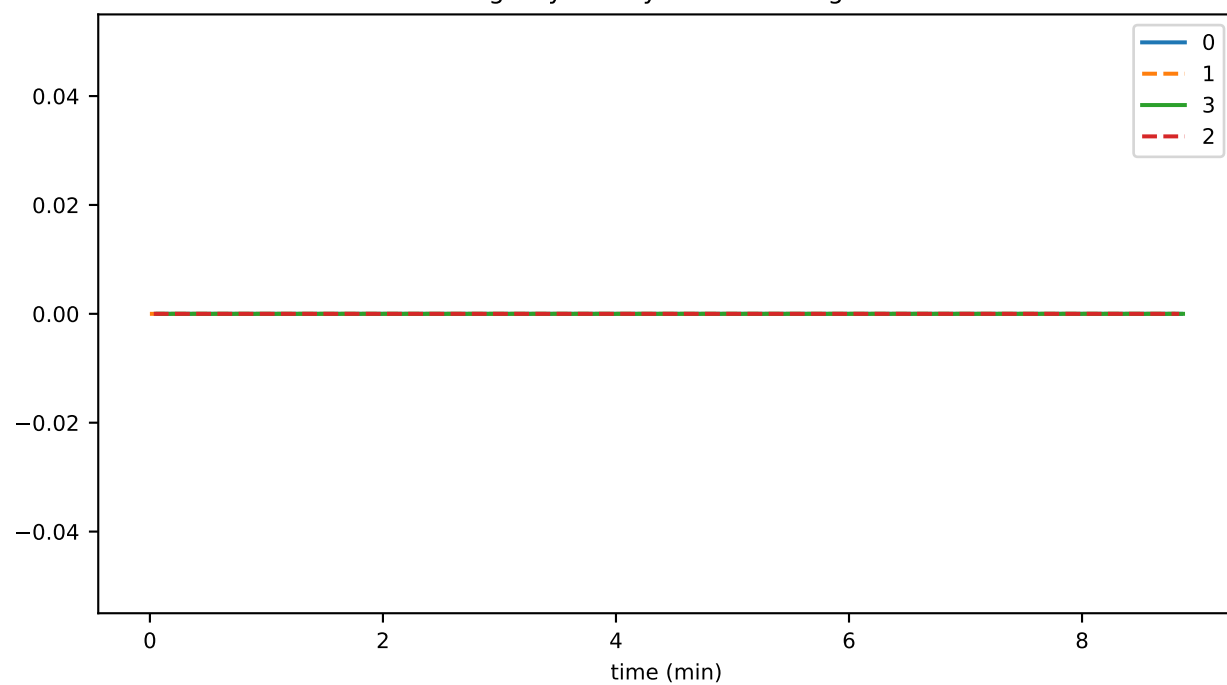
getBySolidityIDDurationAvg
