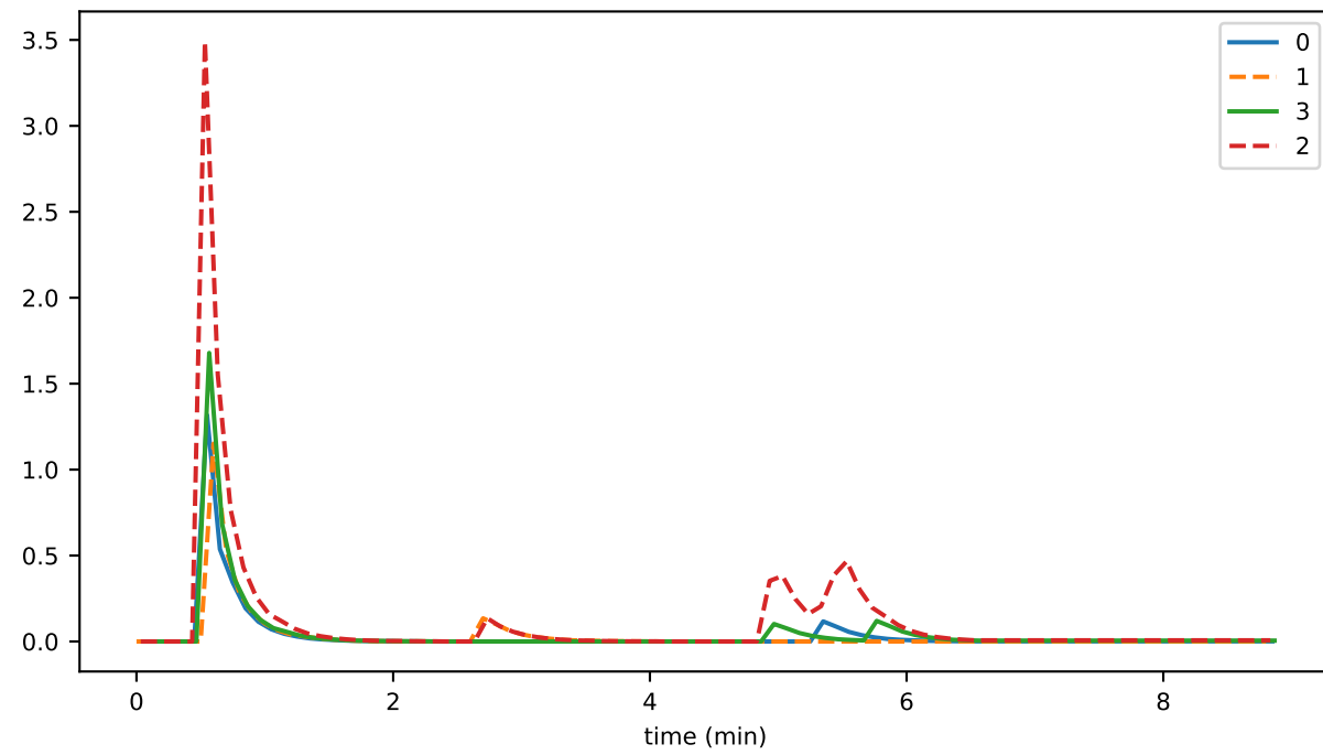
sigStateHash
