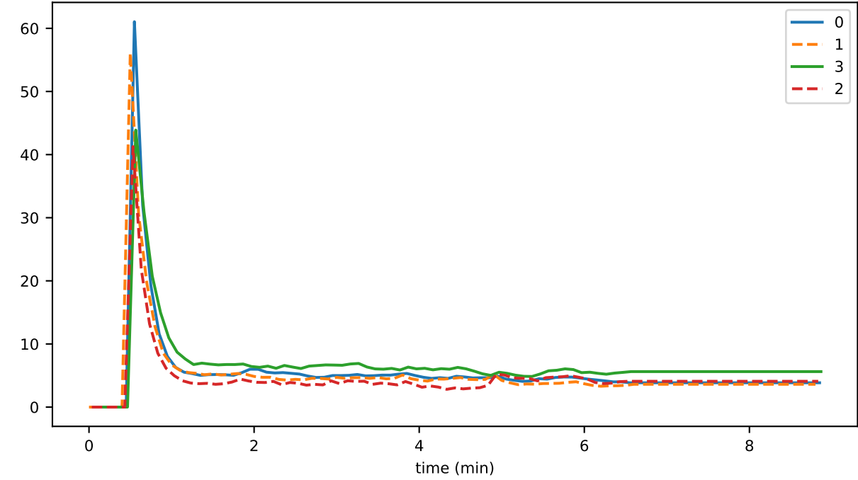
eventDelay_1_eventCreation_runtime
