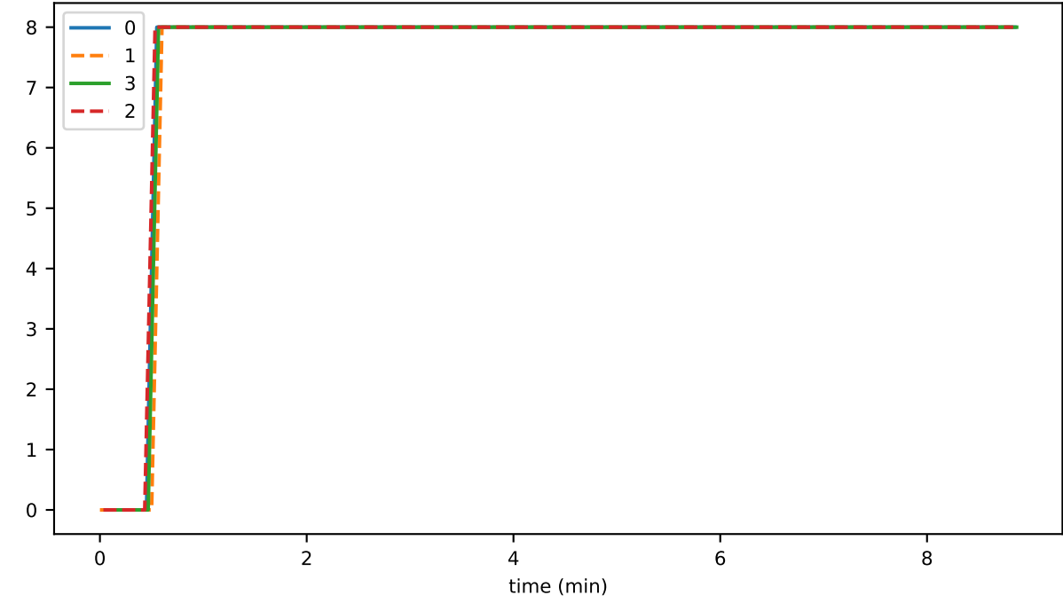
ds_offheap_leavesIndexMb_state
