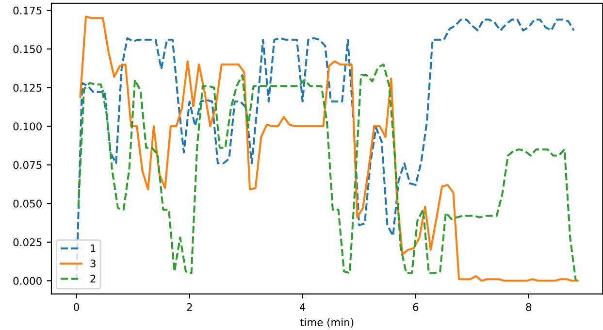
sync_phase_00_fraction_GOSSIP_HALTED
