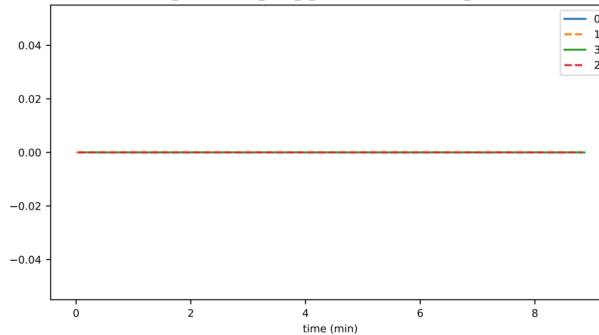
ds_compactions_level_4_leafKeysSavedSpaceMb_state
