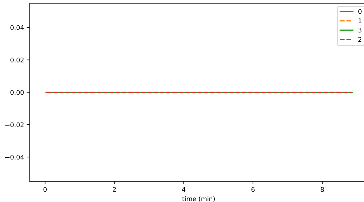
SigQuDepth
