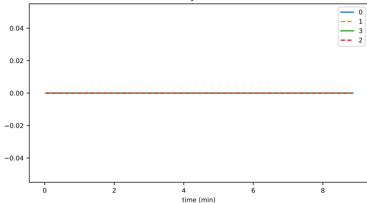
1e7 schedulesMaxNumber
