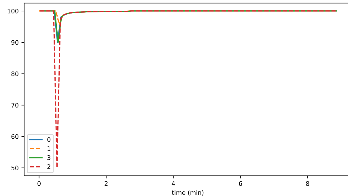
nodeCreateDurationMax
