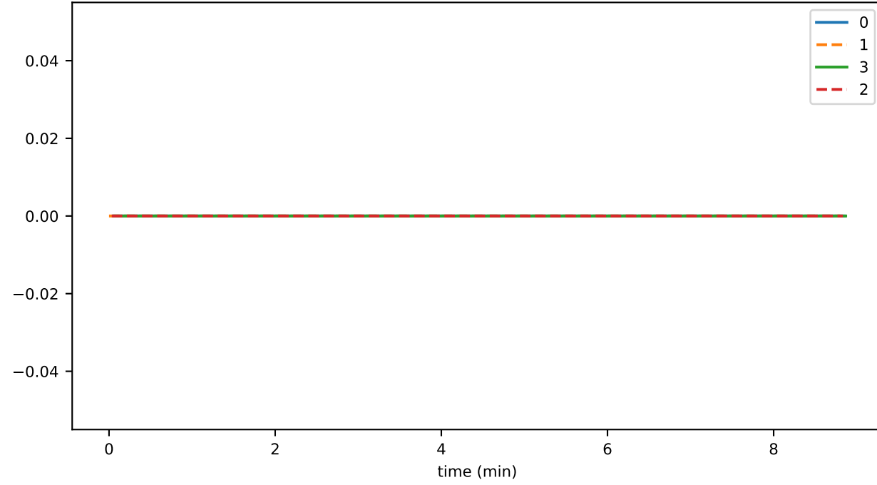
ds_compactions_level_5_leafKeysTimeMs_state
