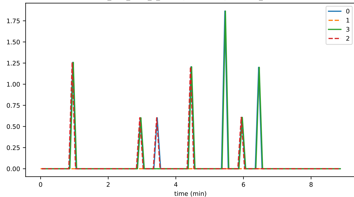
ds_files_level_10_hashesFileSizeByLevelMb_state
