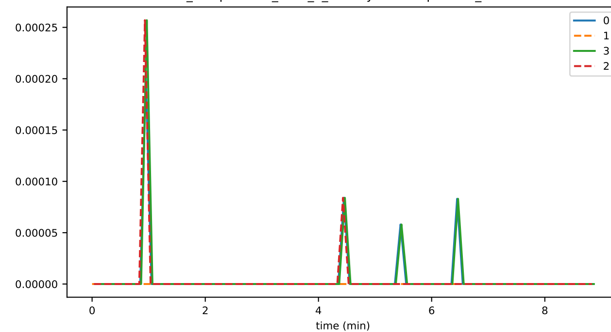
ds_compactions_level_2_leafKeysSavedSpaceMb_state
