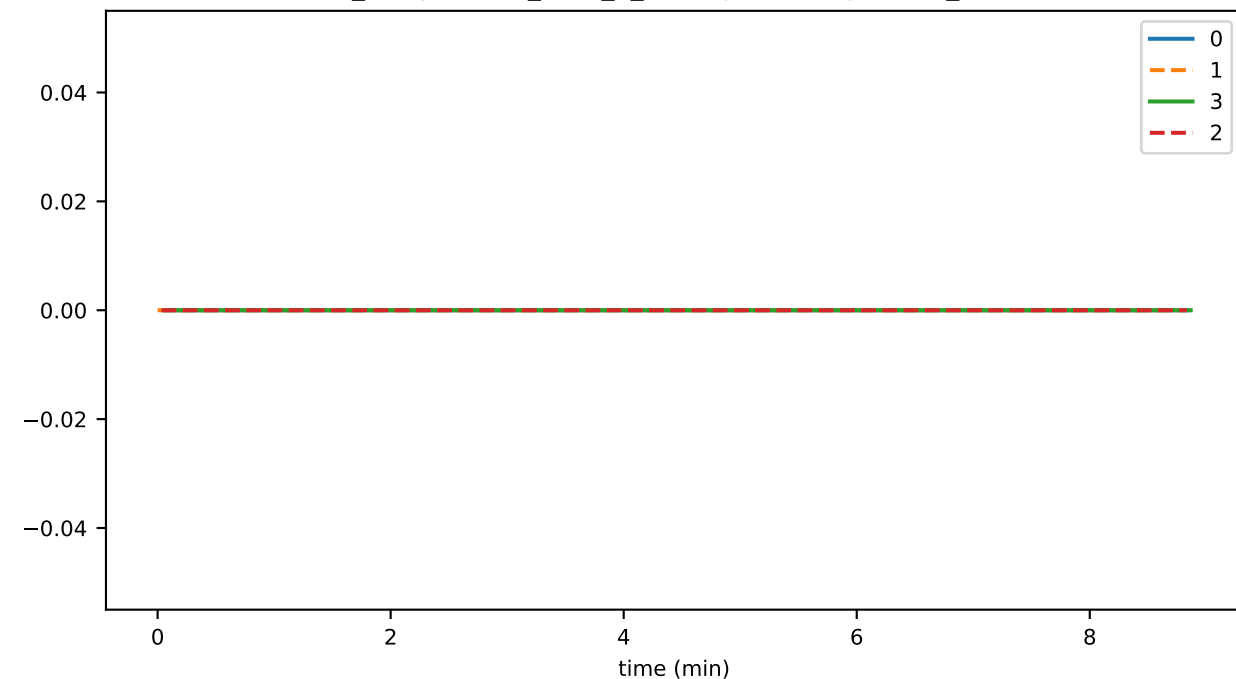
ds_compactions_level_7_leavesSavedSpaceMb_state
