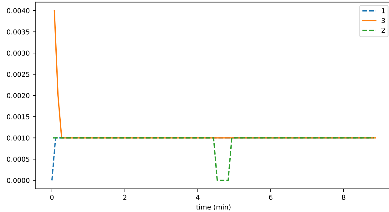
sync_phase_00_fraction_EXCHANGING_WINDOWS
