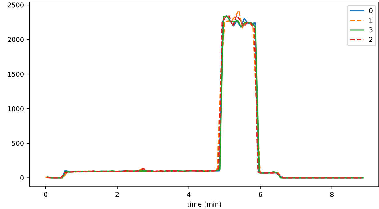
witnessesSeen
