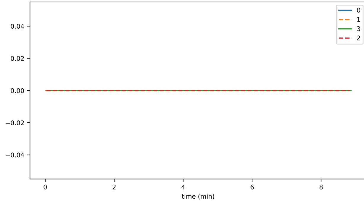
numEventsAddedUntilConsensusMAX
