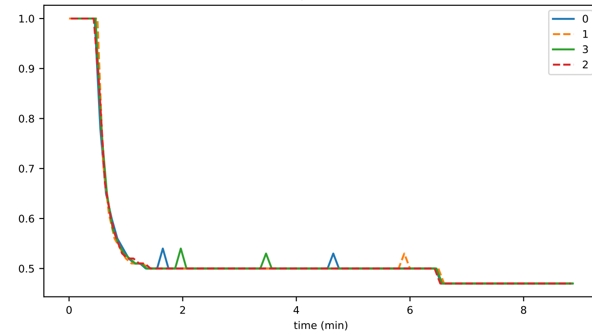
utilPrngDurationAvg
