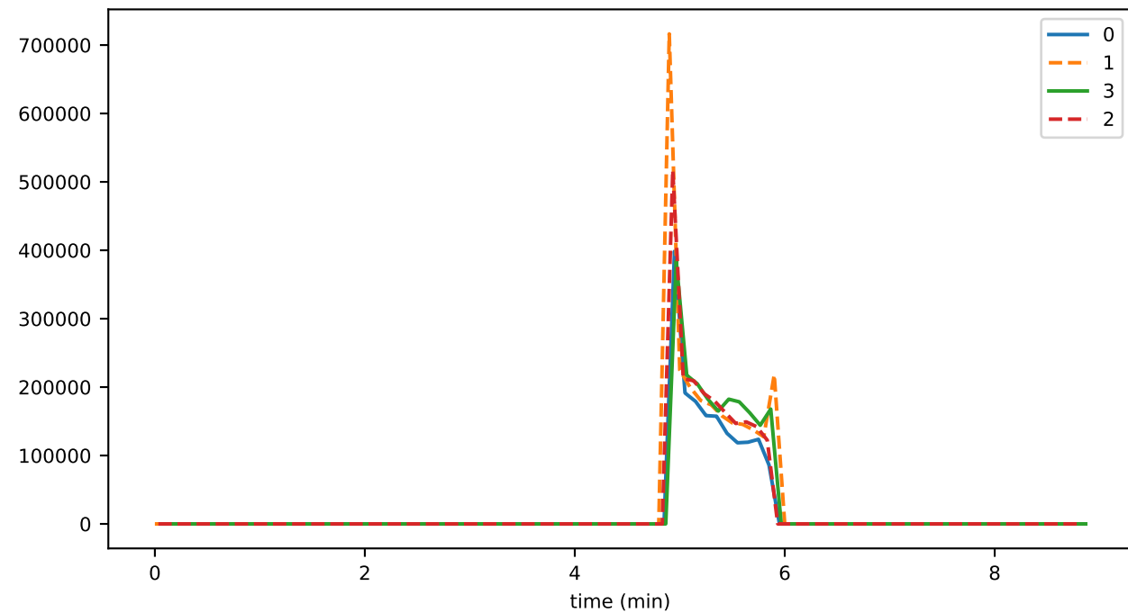
cryptoTransferDurationAvg
