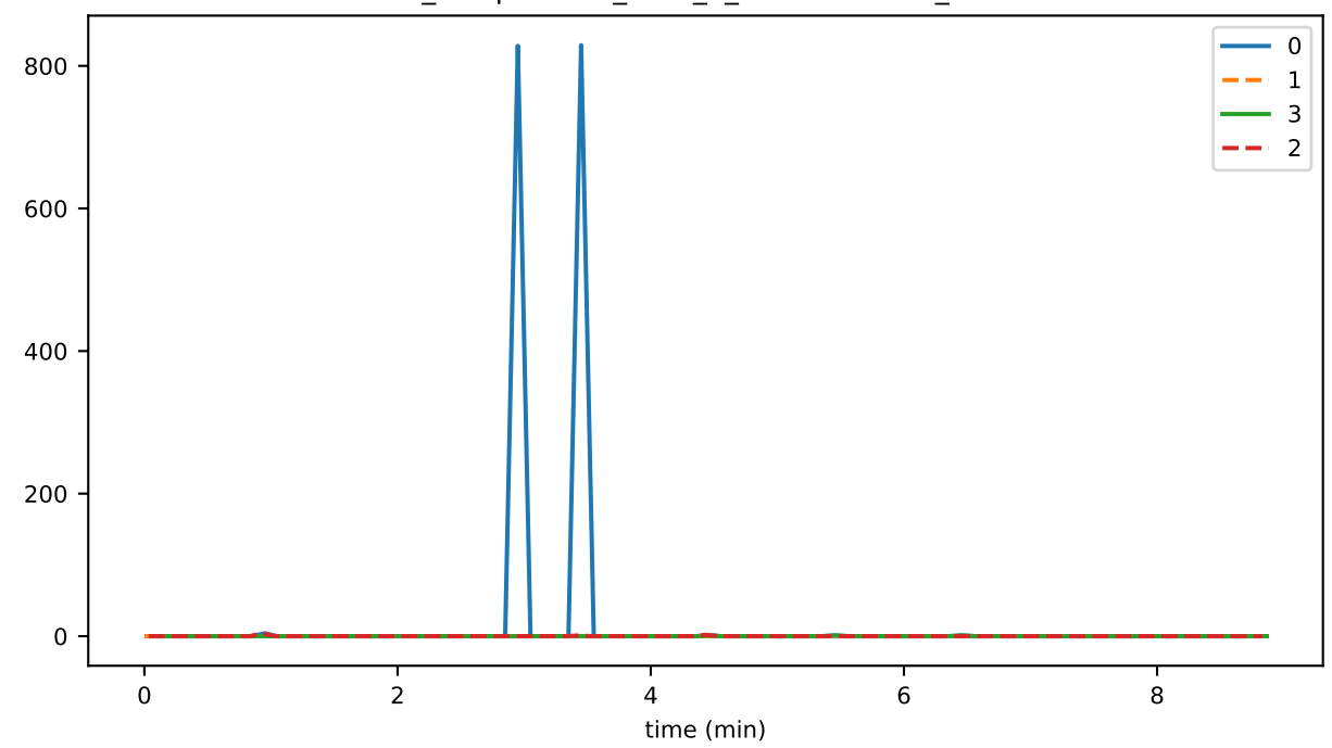
ds_compactions_level_2_leavesTimeMs_state
