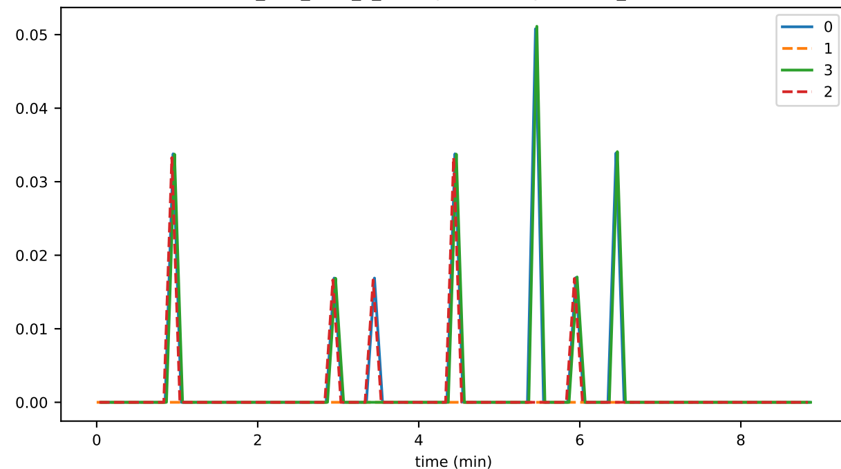
ds_files_level_4_hashesFileSizeByLevelMb_state
