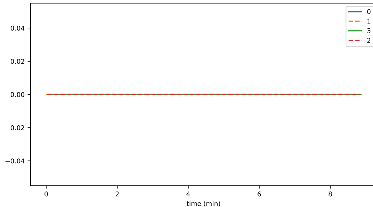
connSend_multitemRequestExceedsSoftLimit
