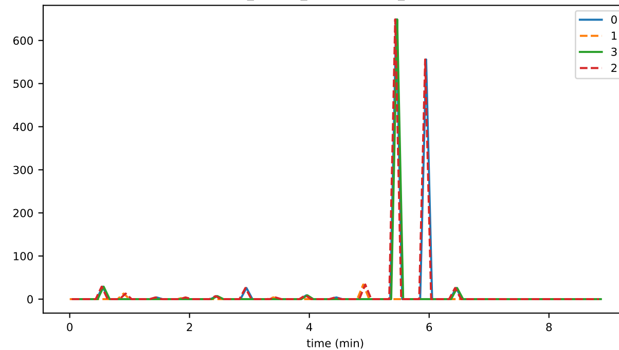
ds_flushes_leavesWritten_state
