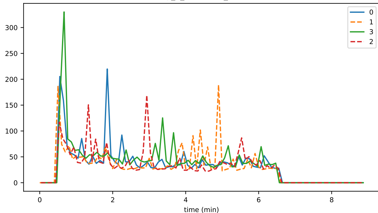
eventDelay_2_validation_storageMAX
