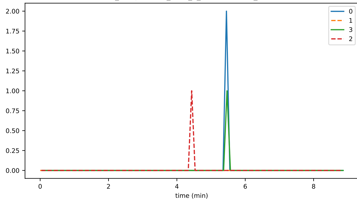
ds_compactions_level_4_hashesTimeMs_state
