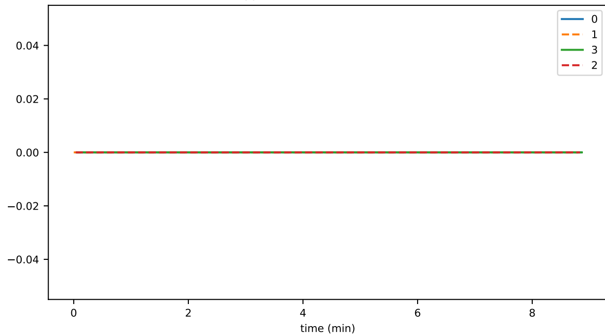
cryptoTransferDurationAvg
