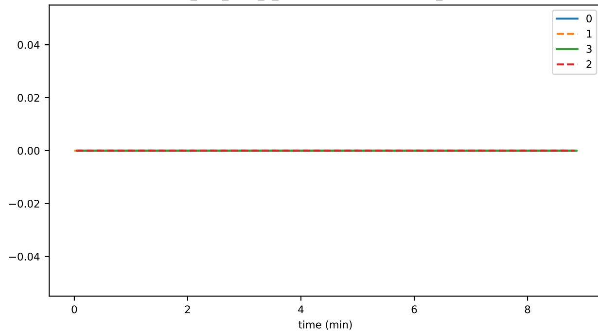
ds_files_level_8_hashesFileSizeByLevelMb_state
