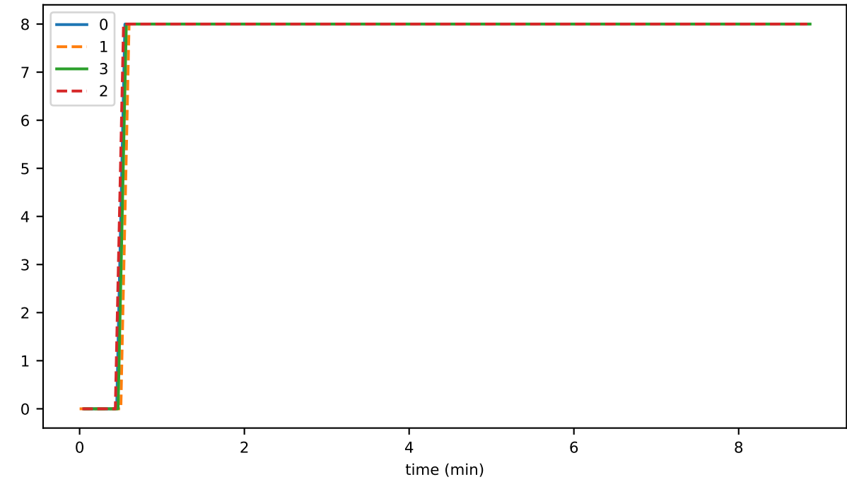
ds_offheap_leavesIndexMb_state
