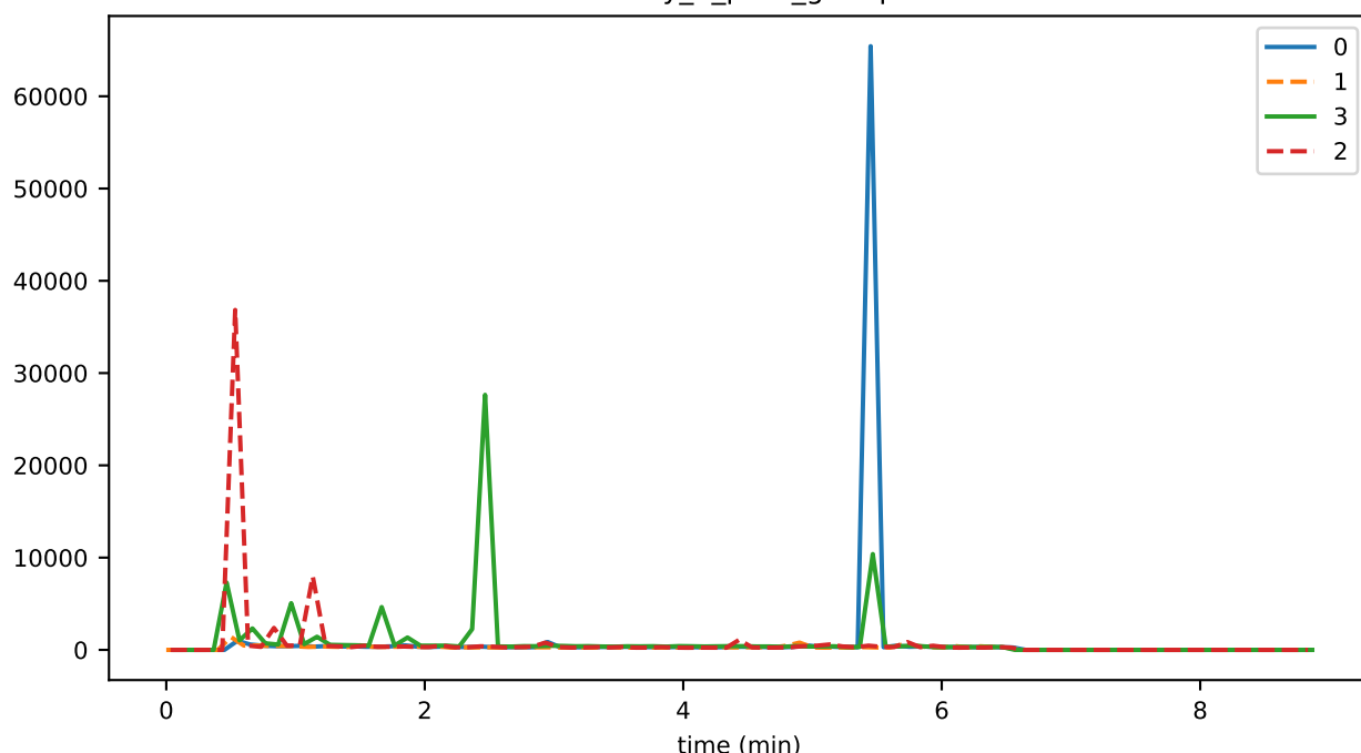
eventDelay_6_pces_gossipMAX
