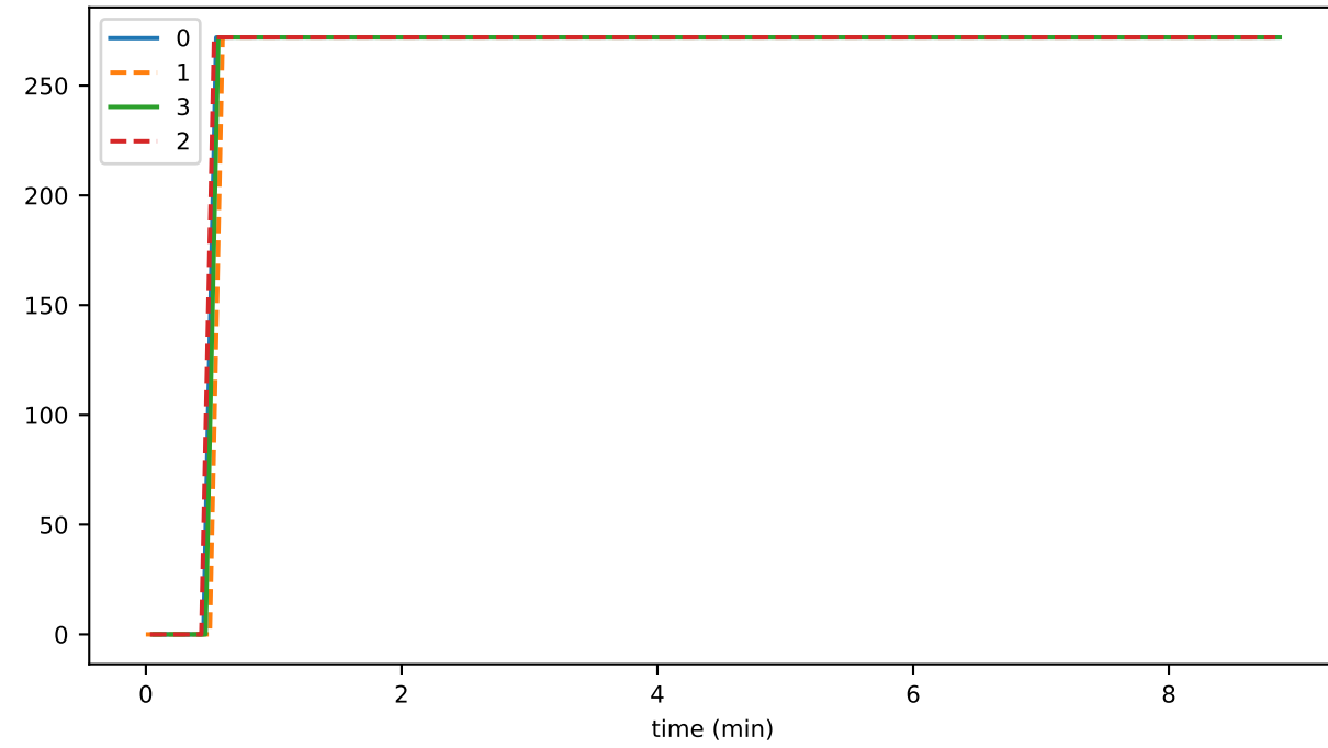
ds_offheap_hashesListMb_state
