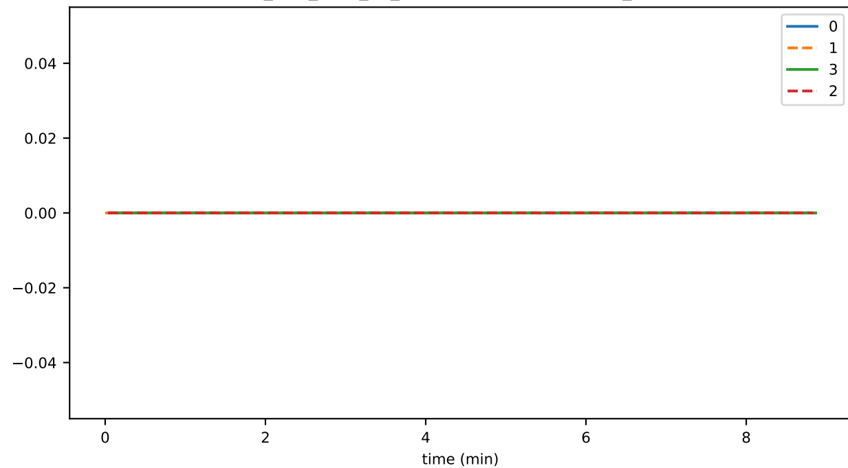
ds_files_level_10_hashesFileSizeByLevelMb_state
