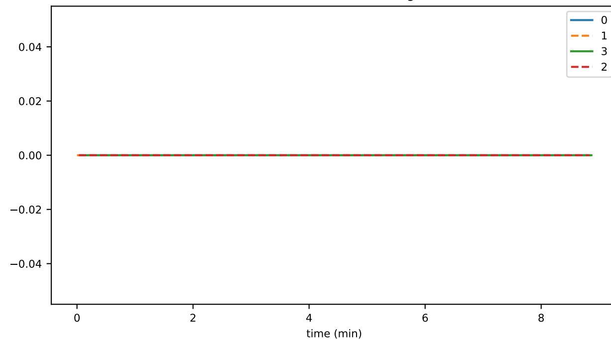
eventsWithInvalidFieldLength
