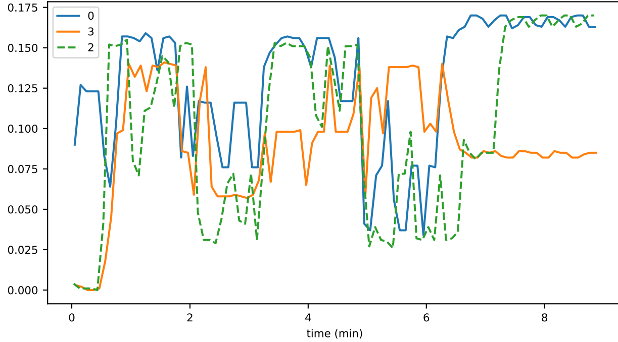
sync_phase_01_fraction_EXCHANGING_WINDOWS
