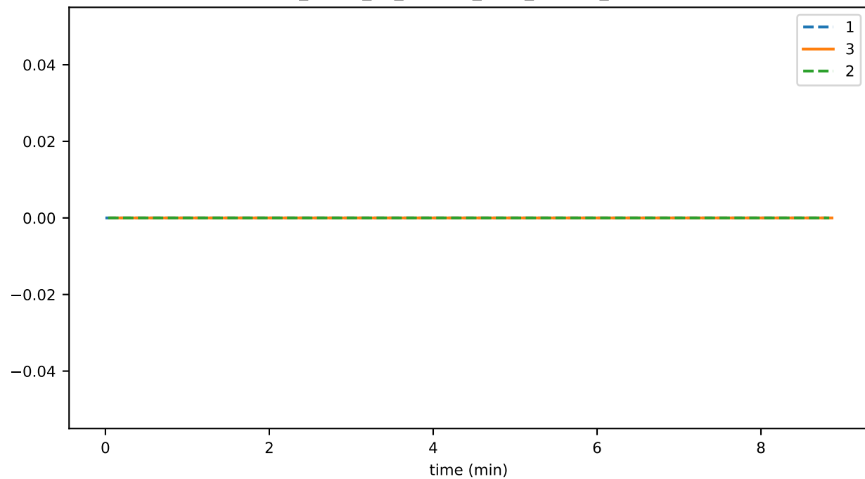
sync_phase_00_fraction_SELF_FALLEN_BEHIND
