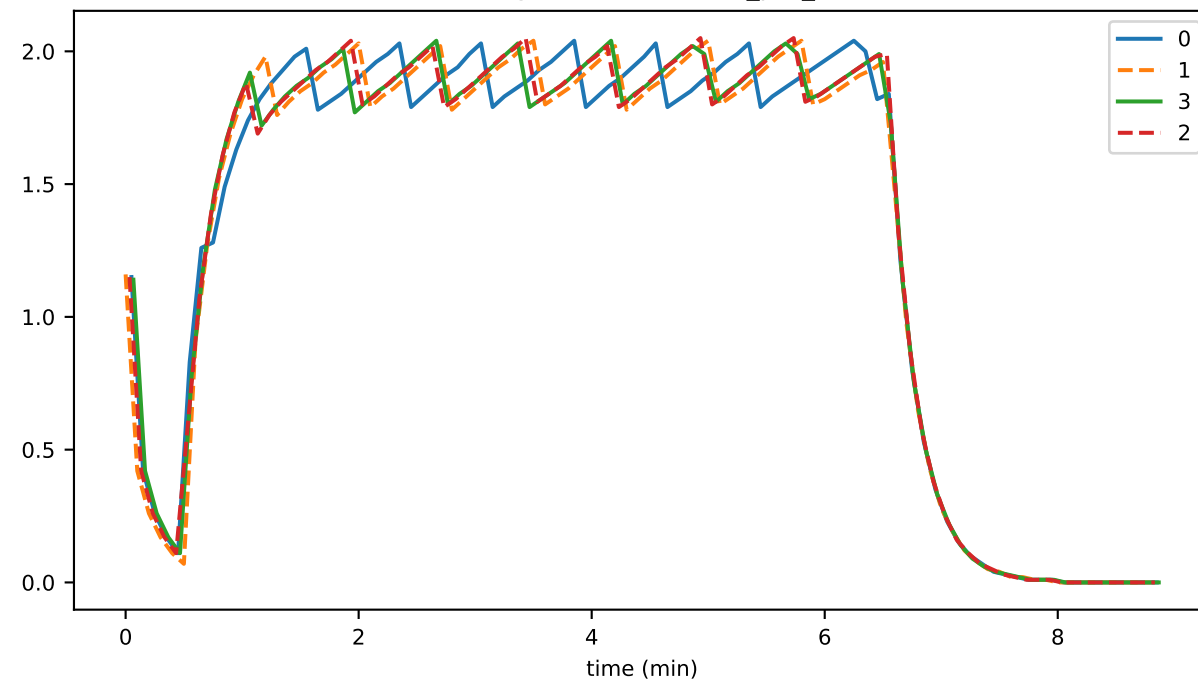
stateSignatureTransactionDurationMax
