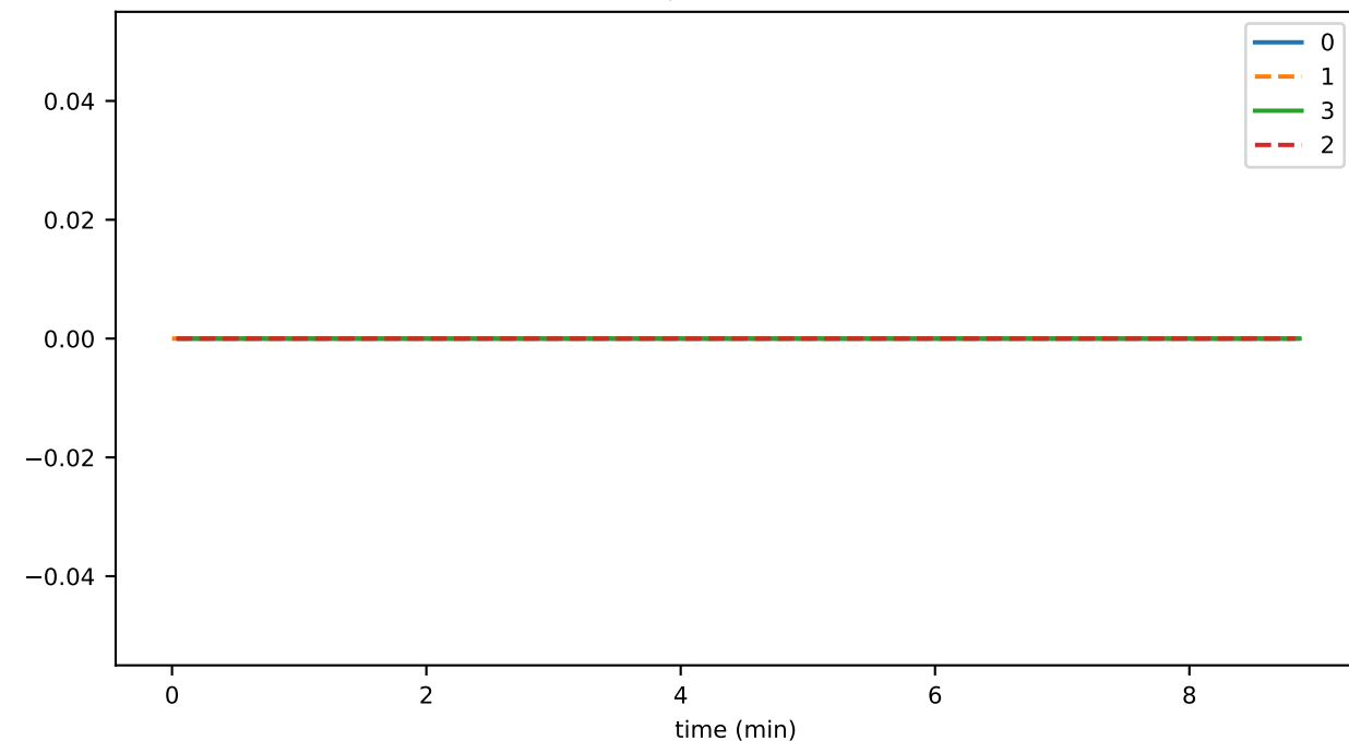
createdEventParents
