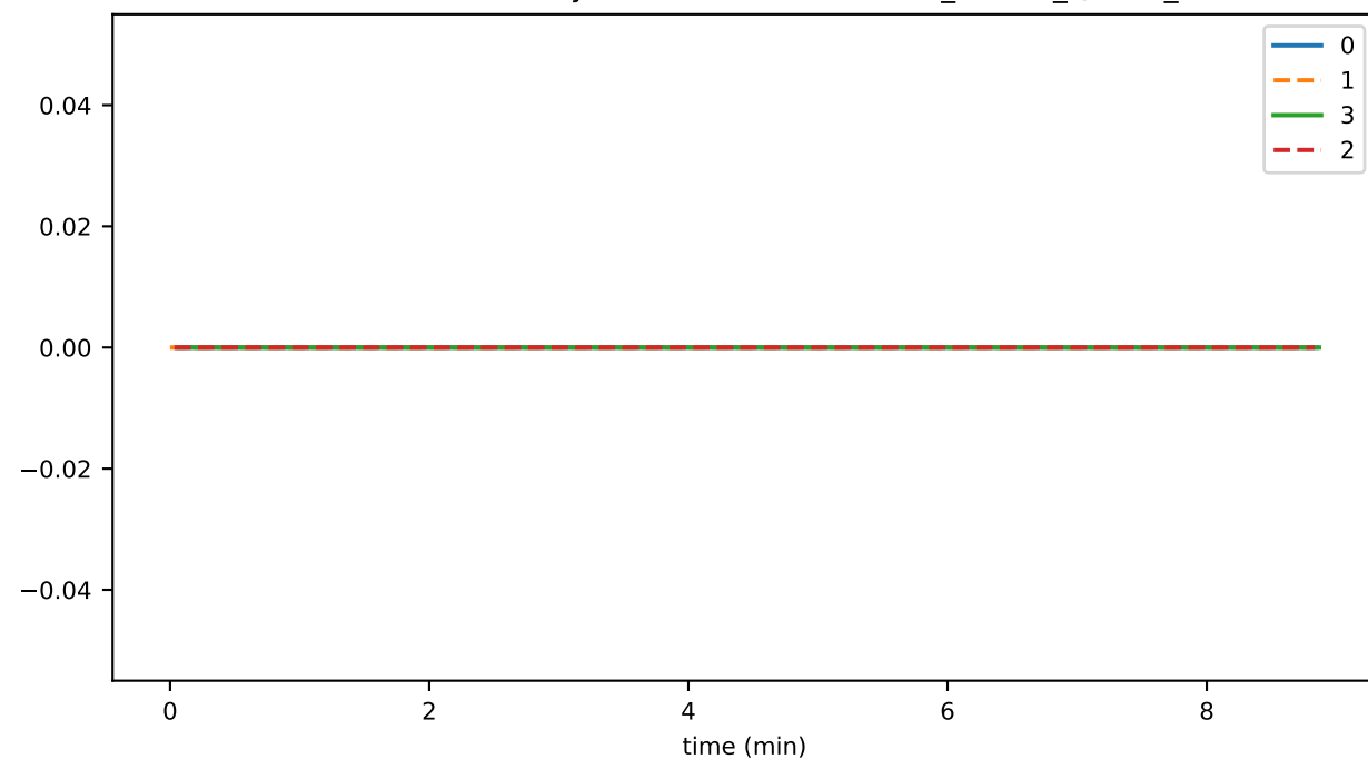
SmartContractService:SystemContractMethodCall_TRANSFER_failed
