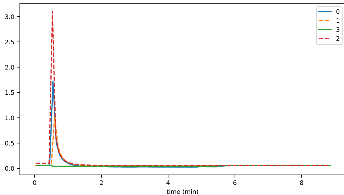
senderReconnectDurationSeconds
