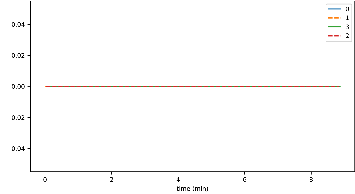
ds_compactions_level_5_leavesSavedSpaceMb_state
