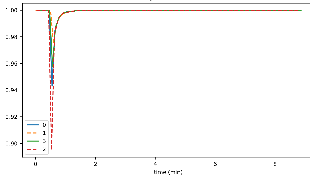
healthyNetworkFraction
