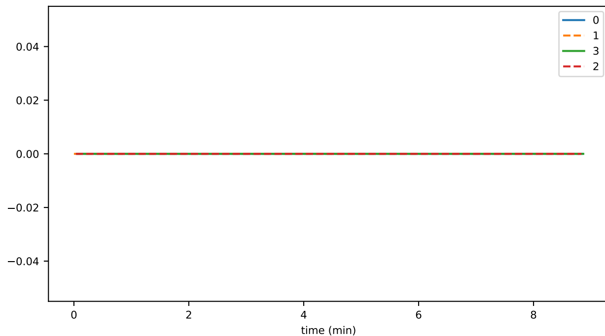
1e6 filesMaxNumber
