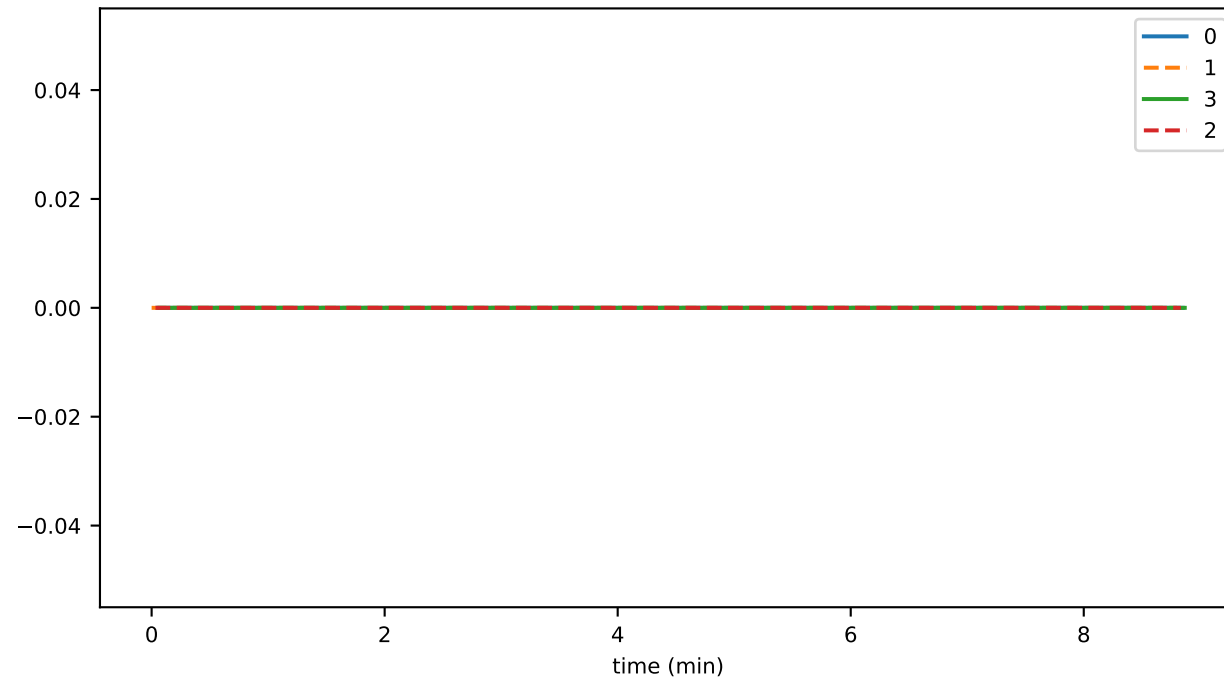
cryptoGetAccountBalanceDurationAvg
