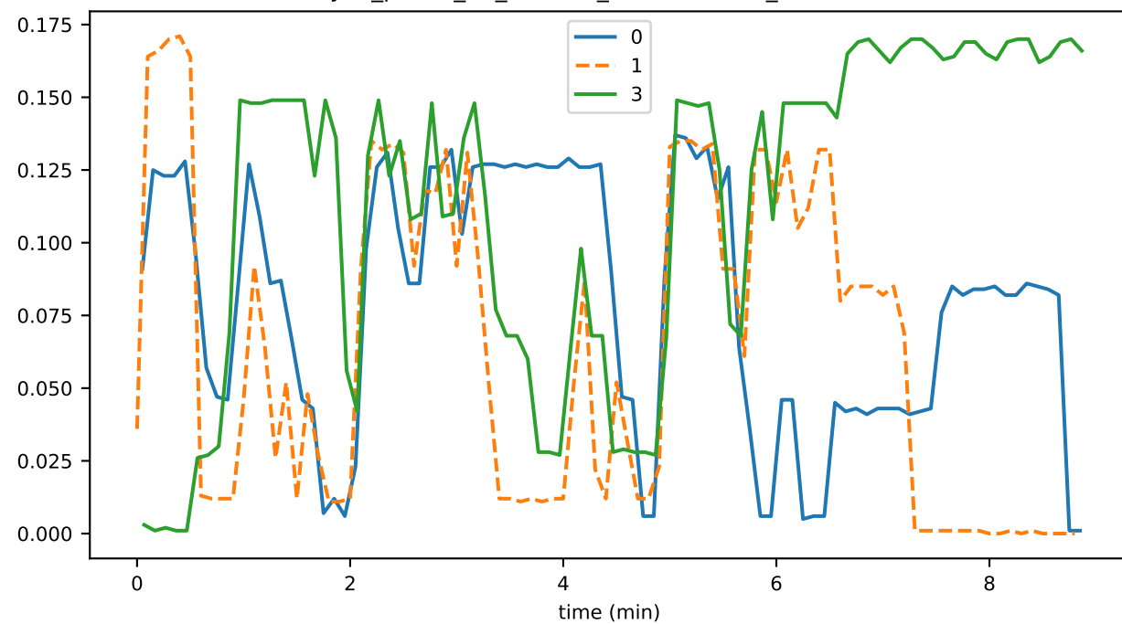
sync_phase_02_fraction_EXCHANGING_WINDOWS
