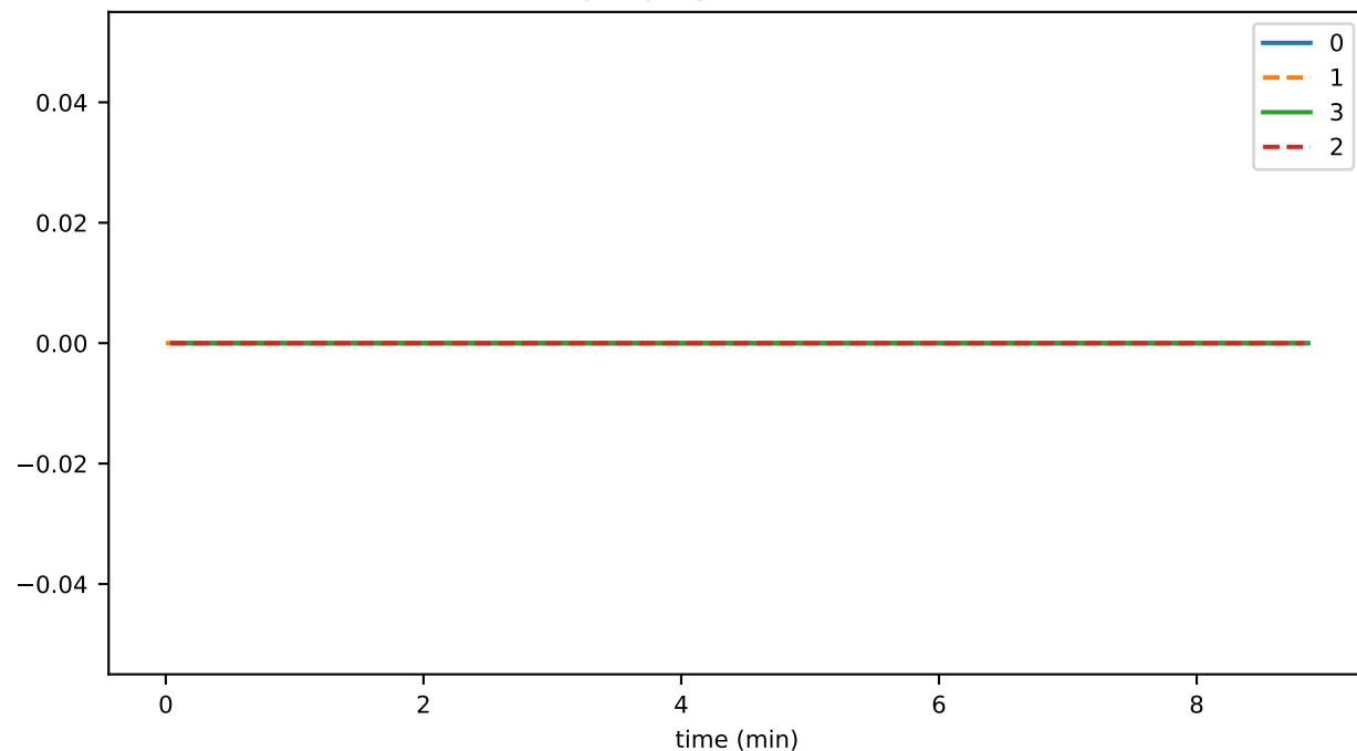
getBySolidityIDDurationAvg
