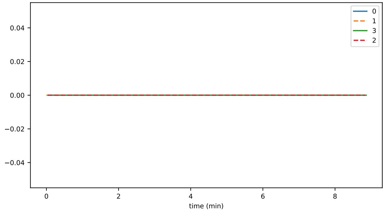
ds_compactions_level_7_leafKeysTimeMs_state
