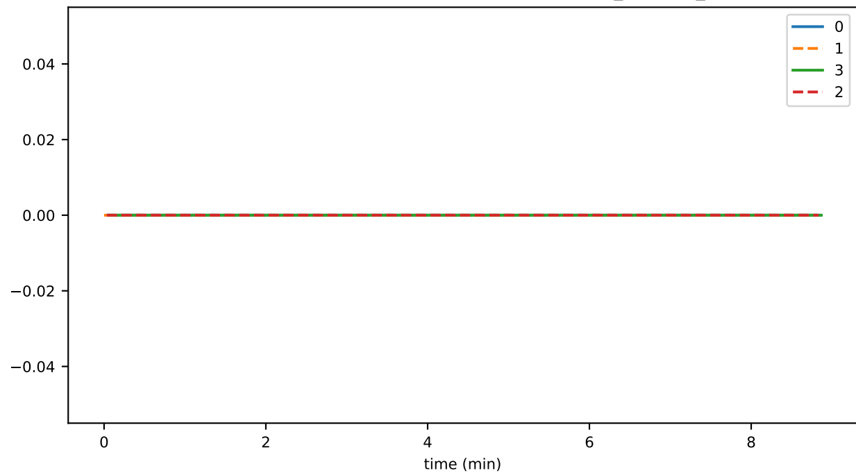
SmartContractService:SystemContractMethodCall_ALIASES_failed
