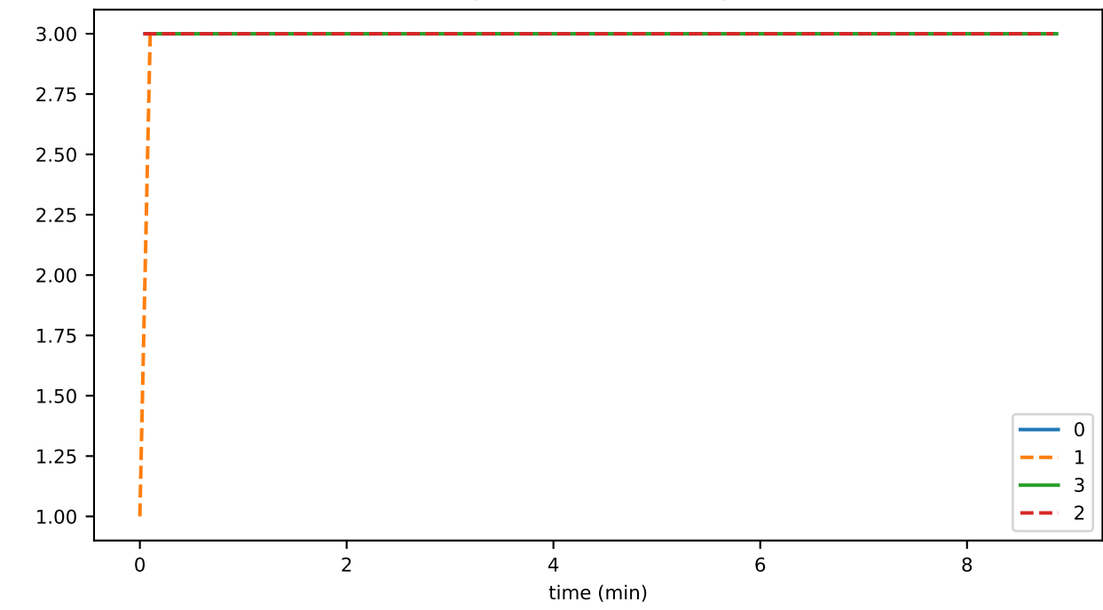
scheduleCreateDurationMax
