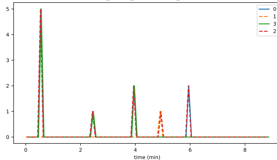
ds_flushes_leavesWritten_state
