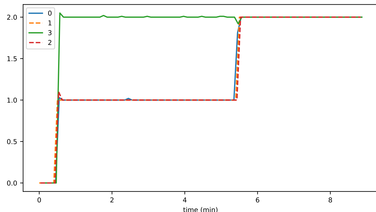
createdEventParents
