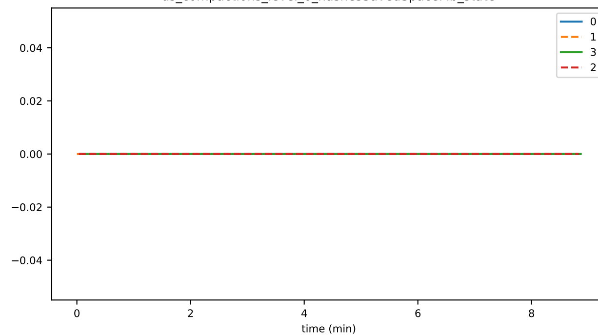
ds_compactions_level_0_hashesSavedSpaceMb_state
