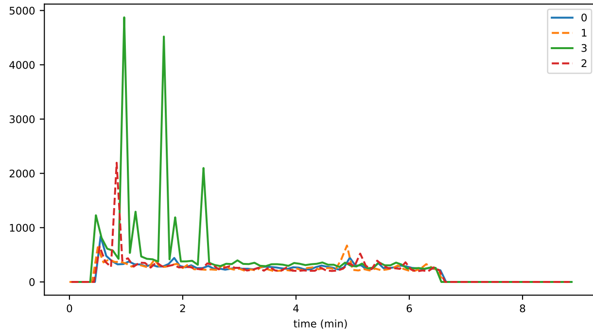
eventDelay_4_verification_gossipMAX
