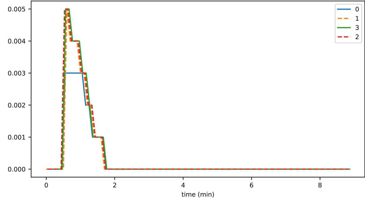
roundsSinceLastConsensusEvent_3
