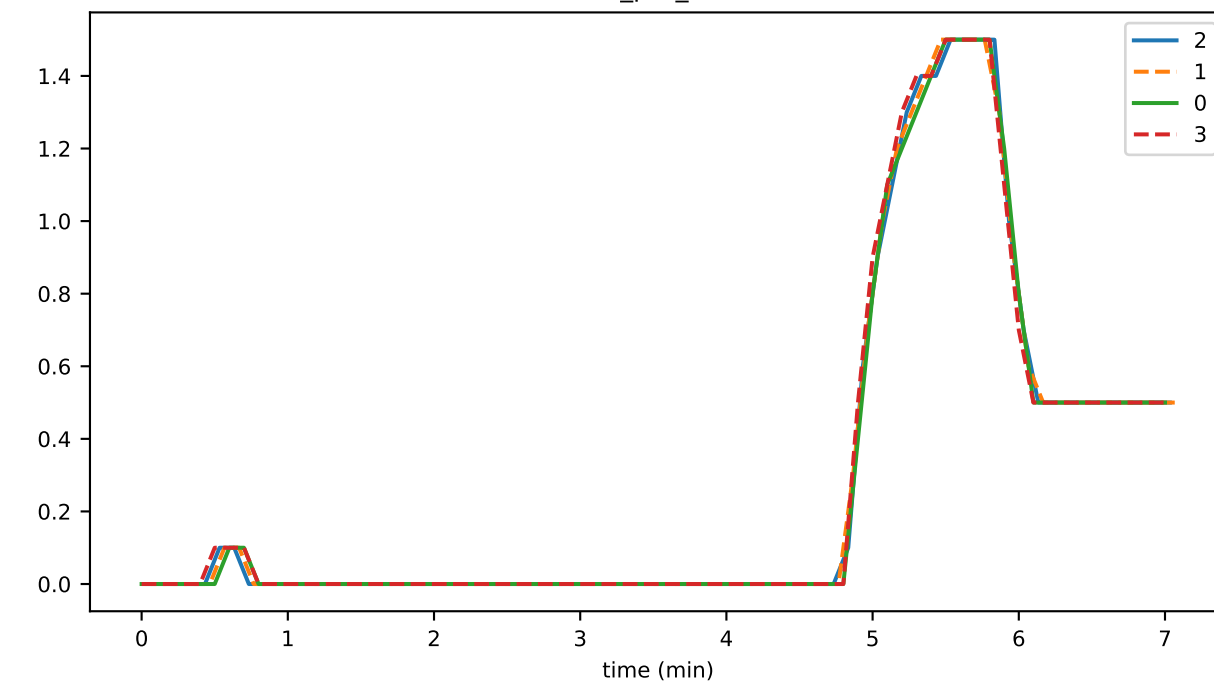
trans_per_event
