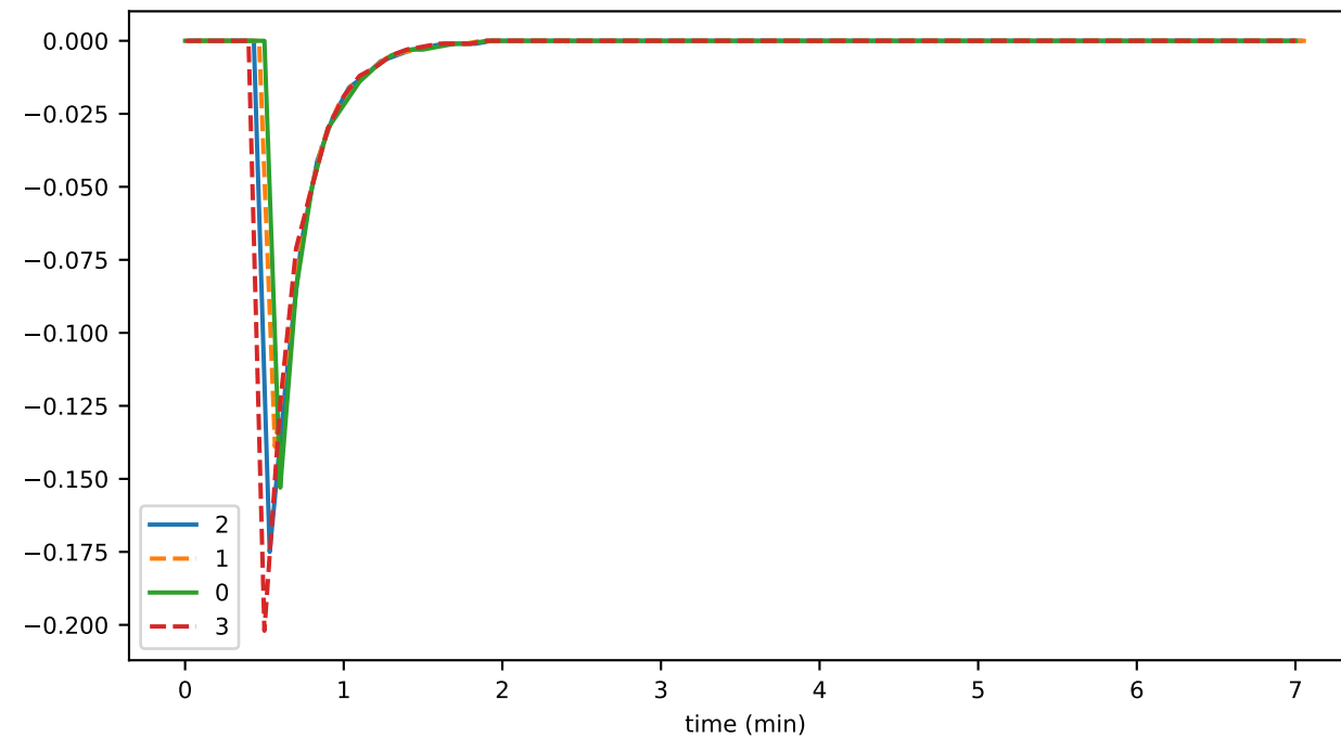
stateSignatureAge
