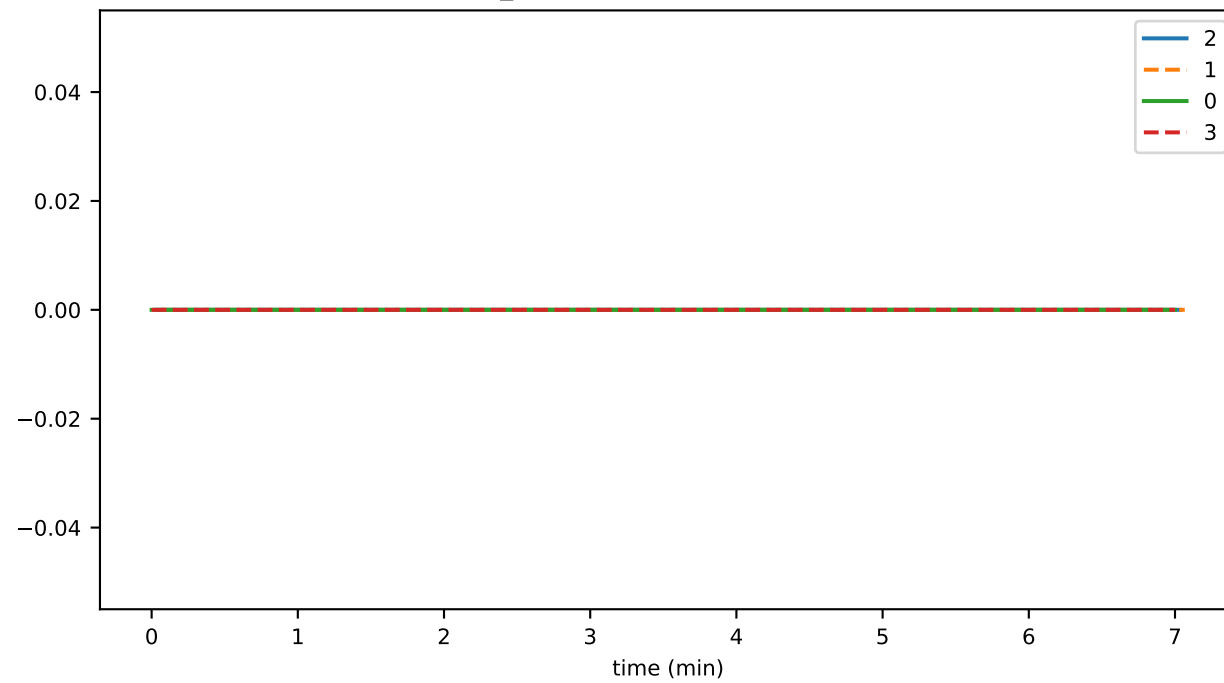
connSend_multitemRequestExceedsSoftLimit
