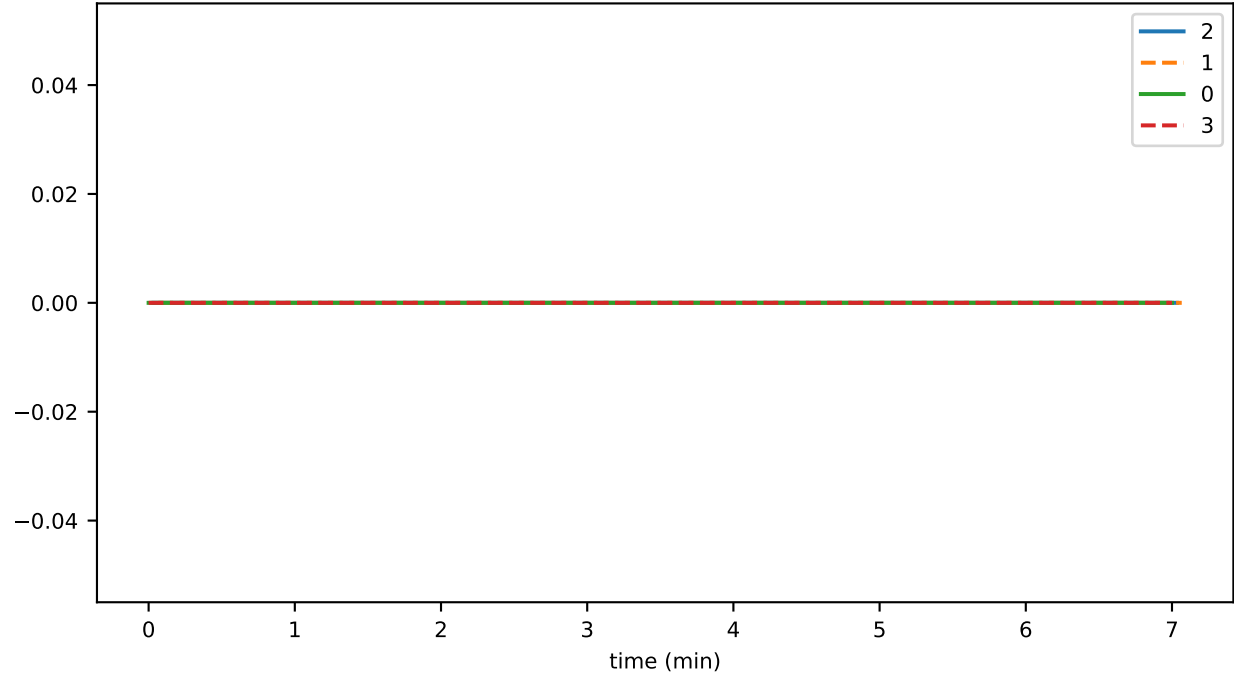
roundsSinceLastConsensusEvent_3
