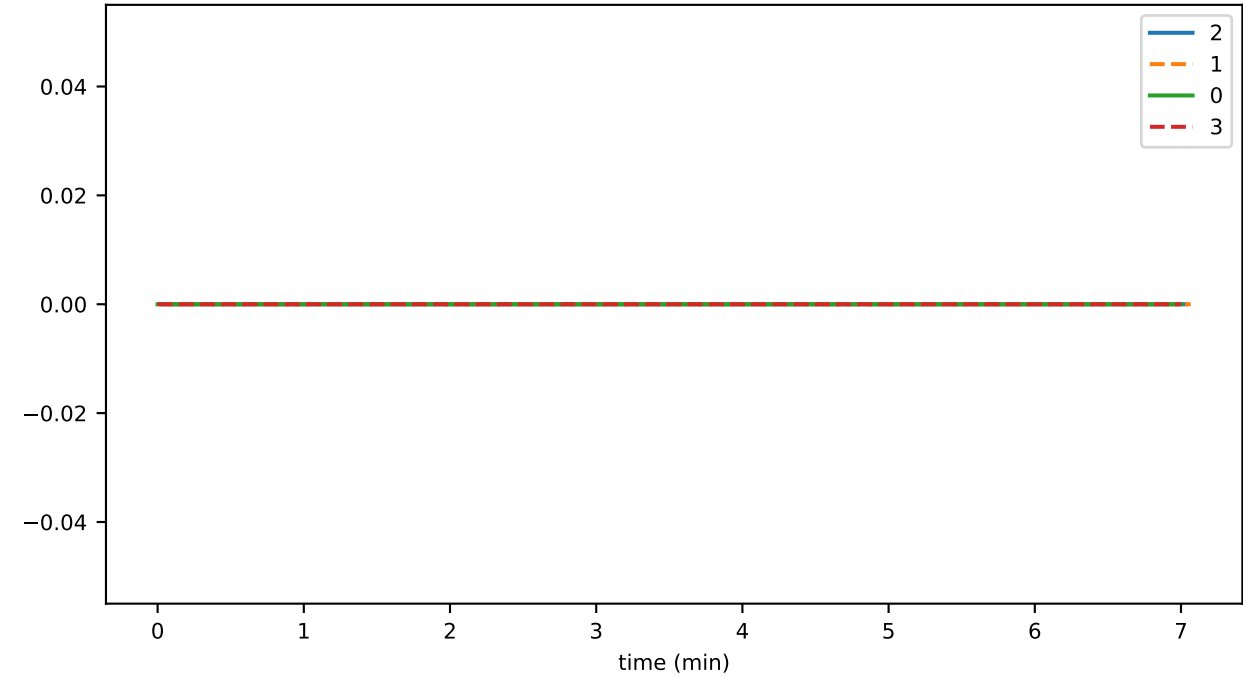
ds_compactions_level_2_leafKeysSavedSpaceMb_state
