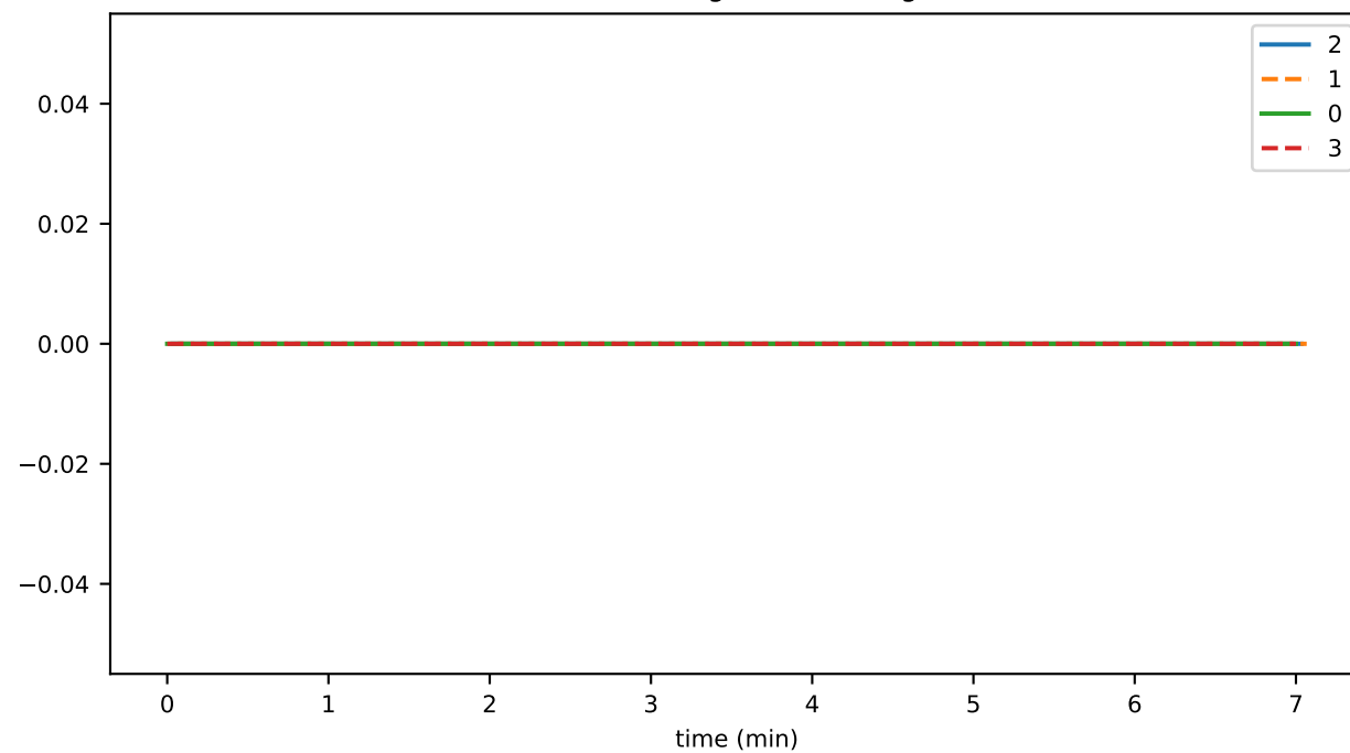
scheduleSignDurationAvg
