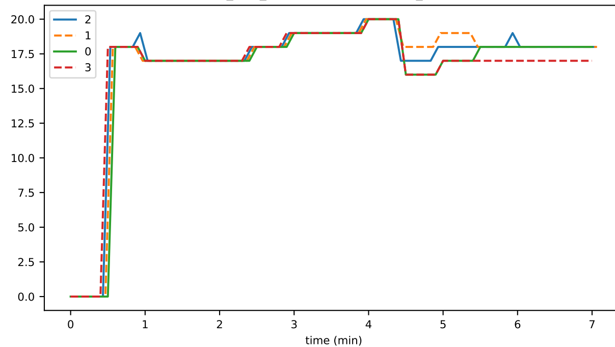
ds_files_leafKeysStoreFileCount_state
