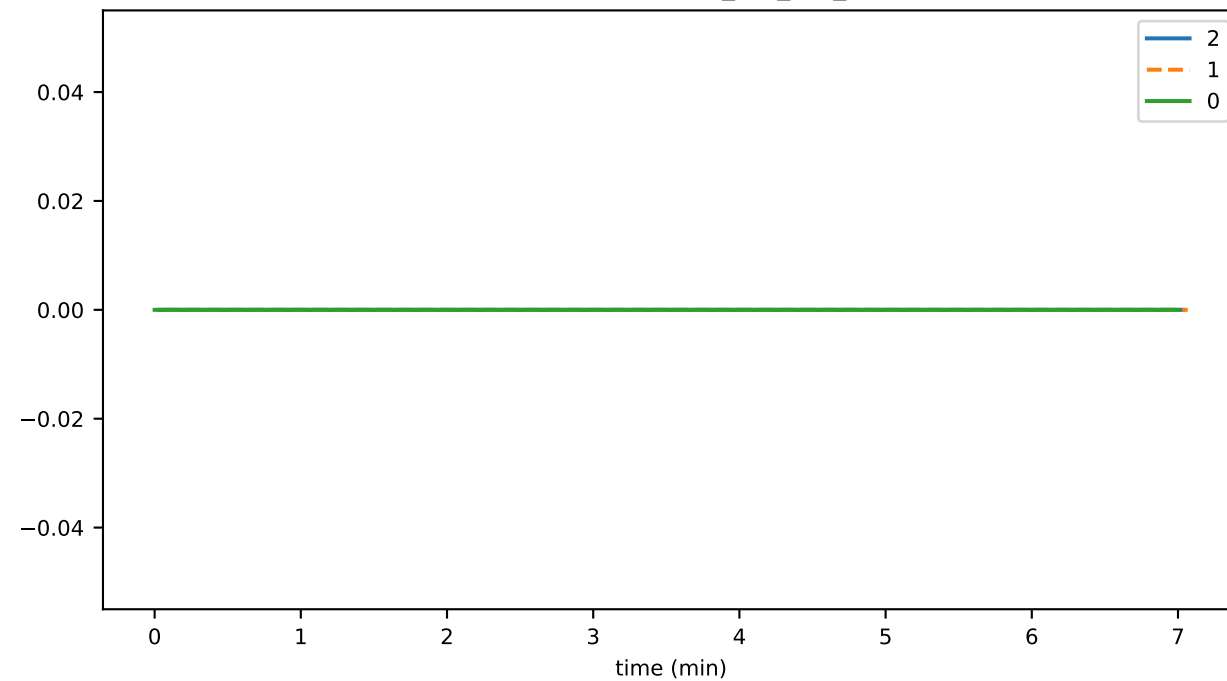
reconnectRejections_per_sec_03
