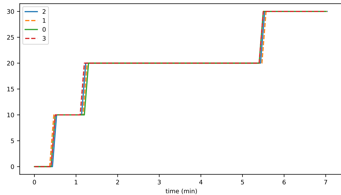
disconnects_per_sec_00
