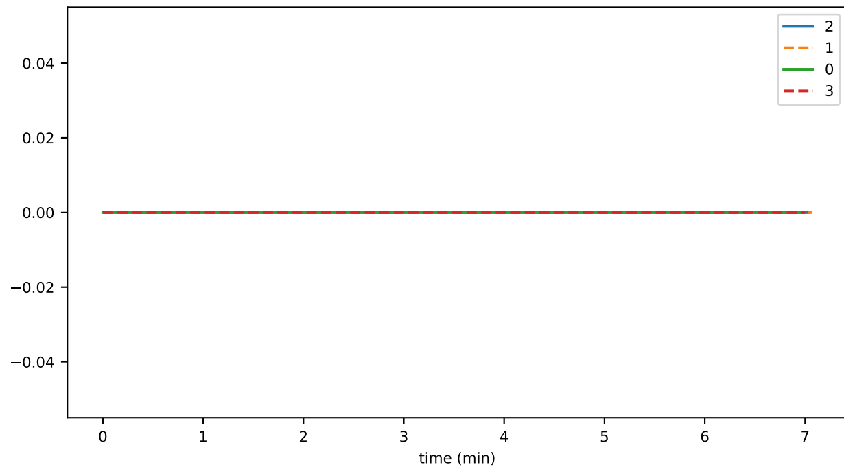
systemDeleteThrottledTxns
