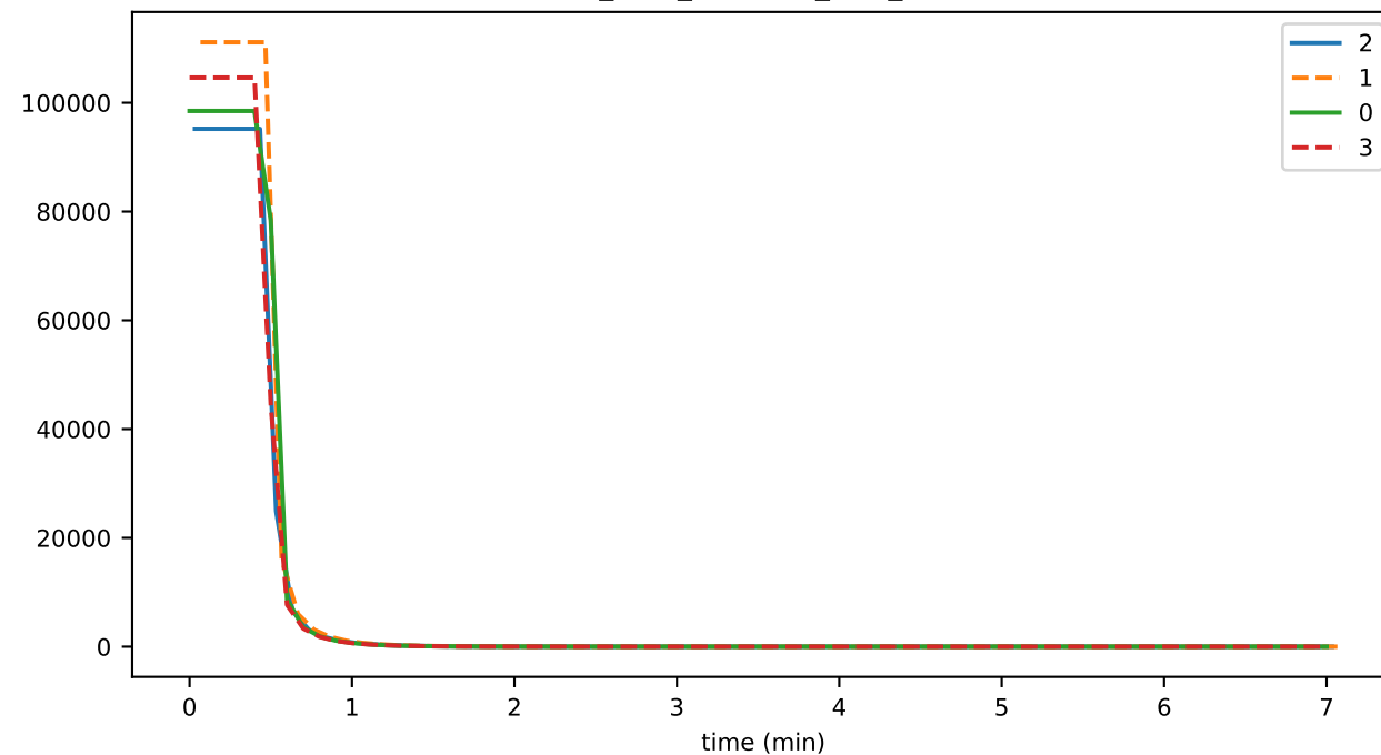
consensusCreateTopicDurationMax
