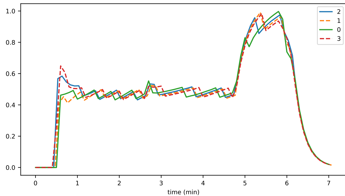
sync_per_secC
