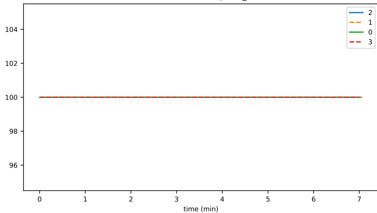
nodeActivePercentSnapshot_node0
