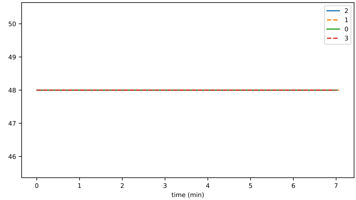
receiverReconnectDurationSeconds
