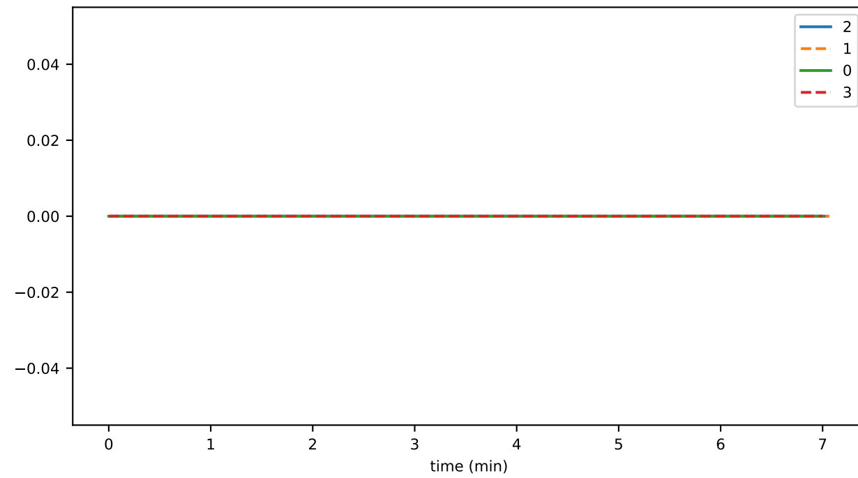
SigIntakeEnqueueTime
