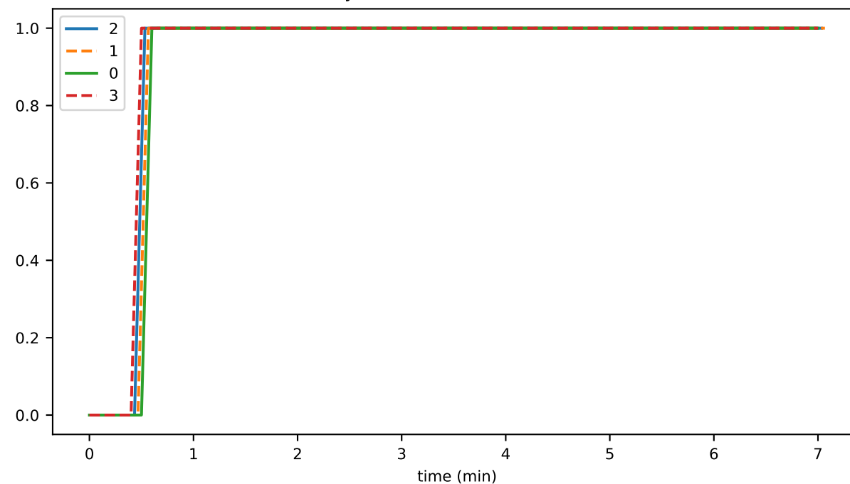
historyProofTransWMetaToWAsmCnt
