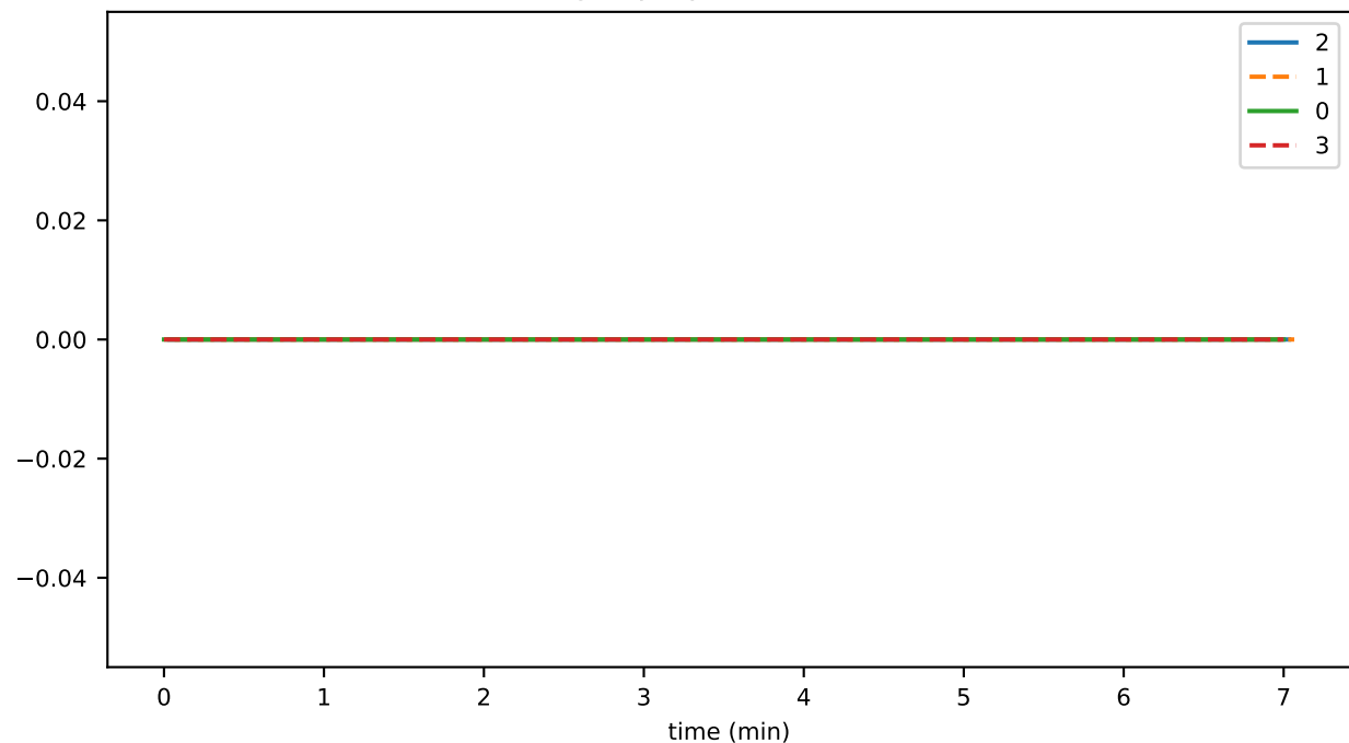
getBySolvencyIDDurationAvg
