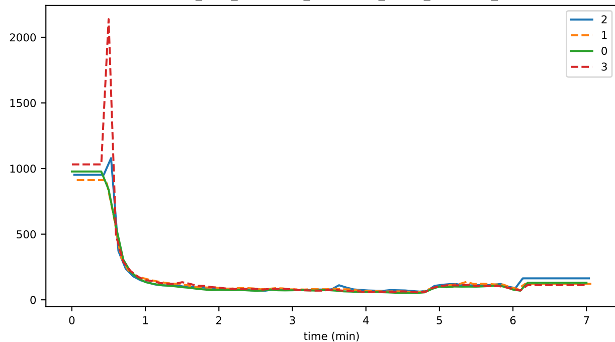
consensusCreateTopicDurationAvg
