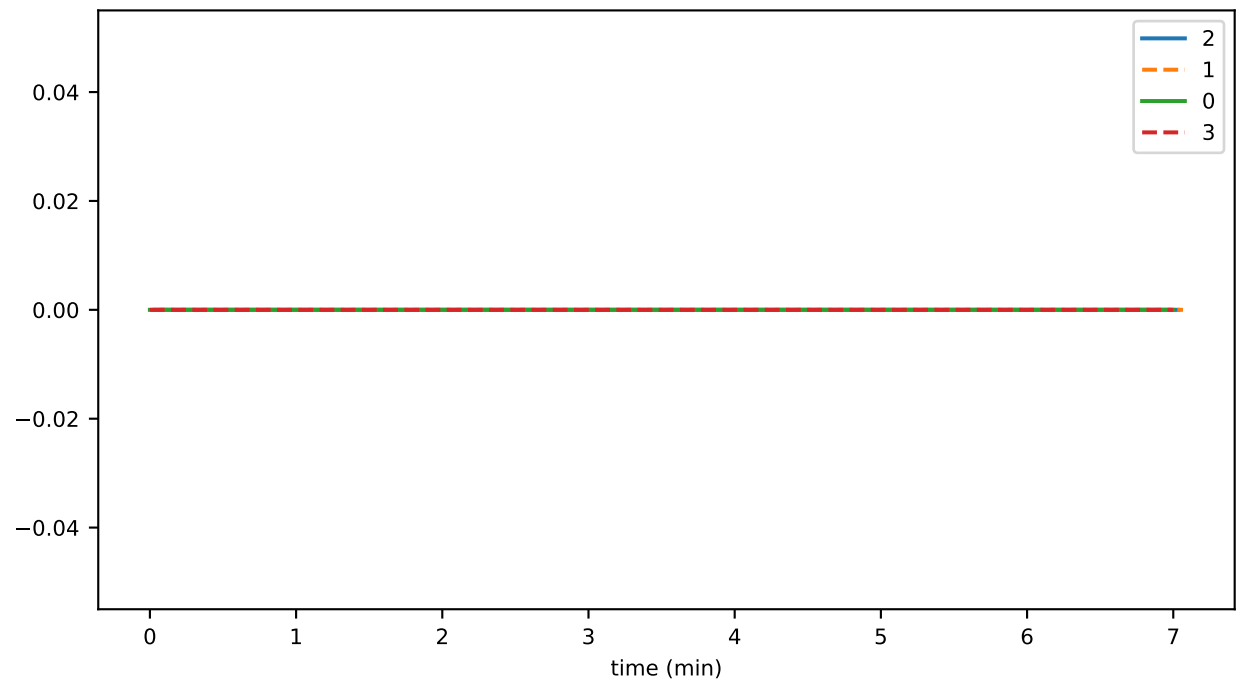
stateSignatureTransactionDurationAvg
