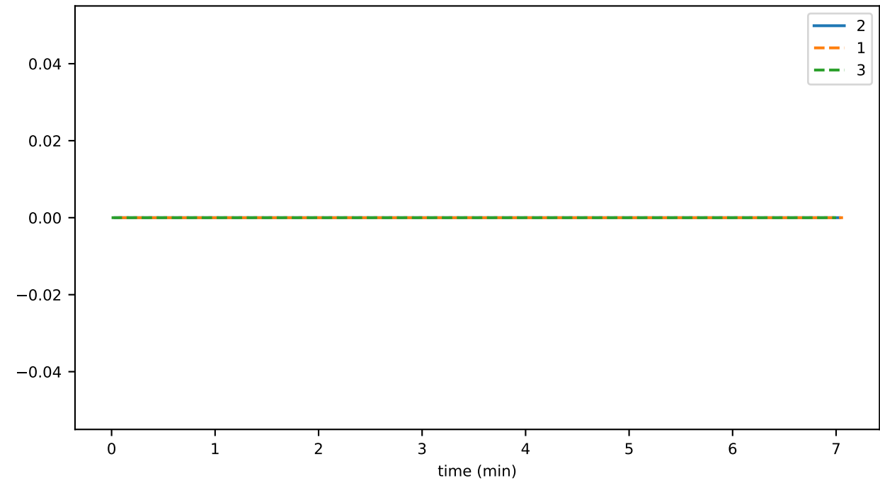
sync_phase_00_fraction_SENDING_EVENTS
