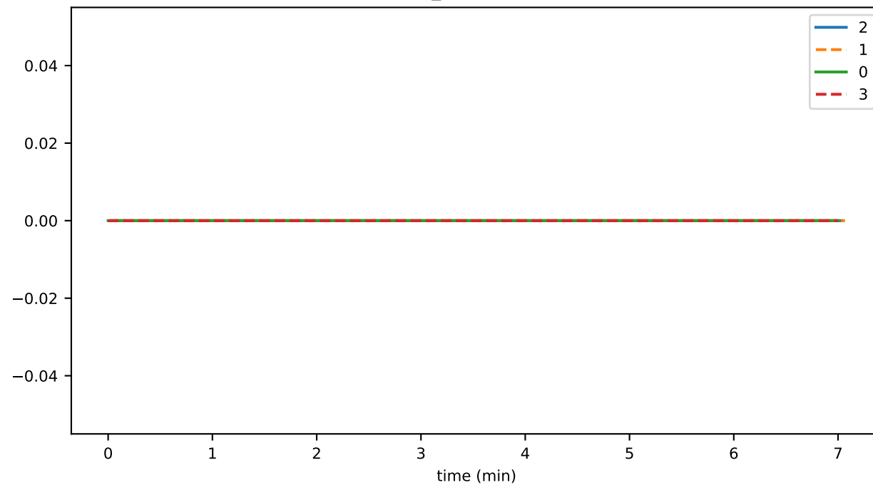
connRecv_acknowledgement
