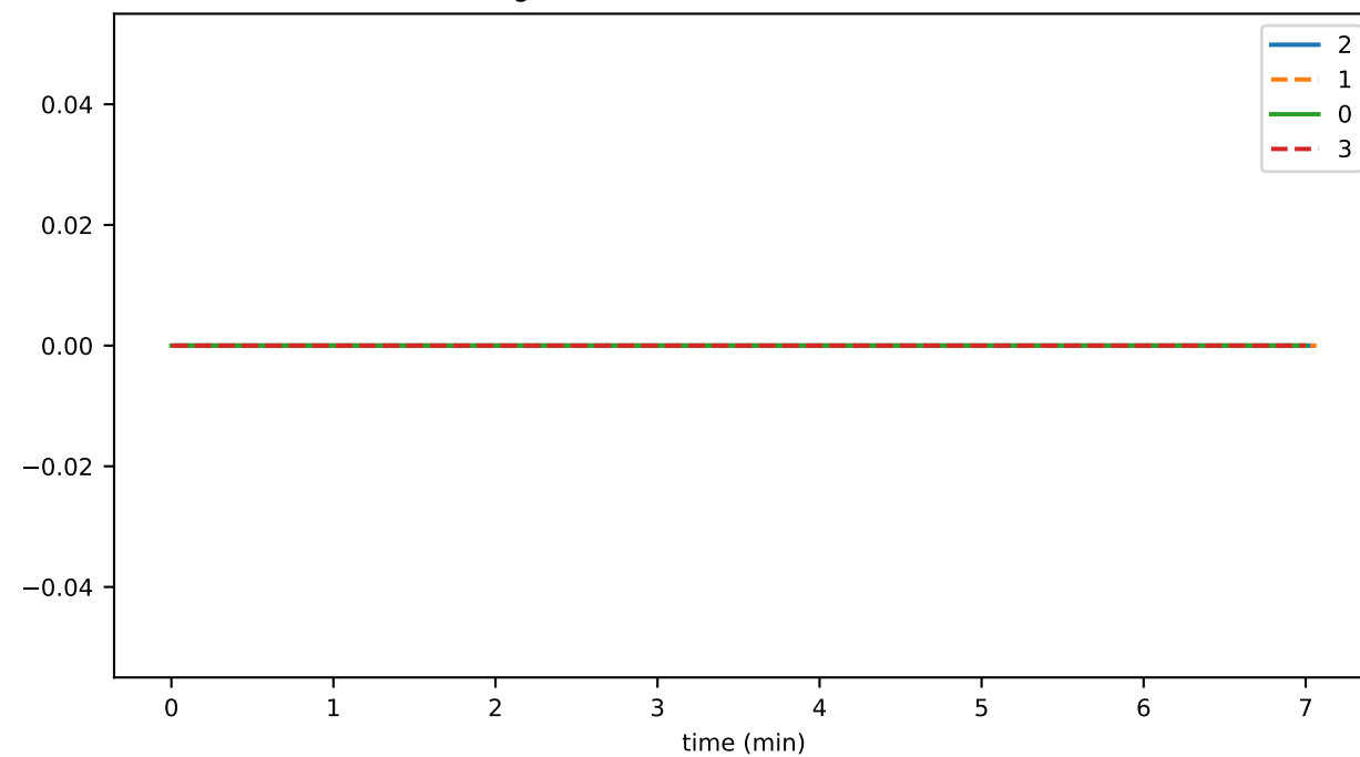
migrationRootHashVoteThrottledTxns
