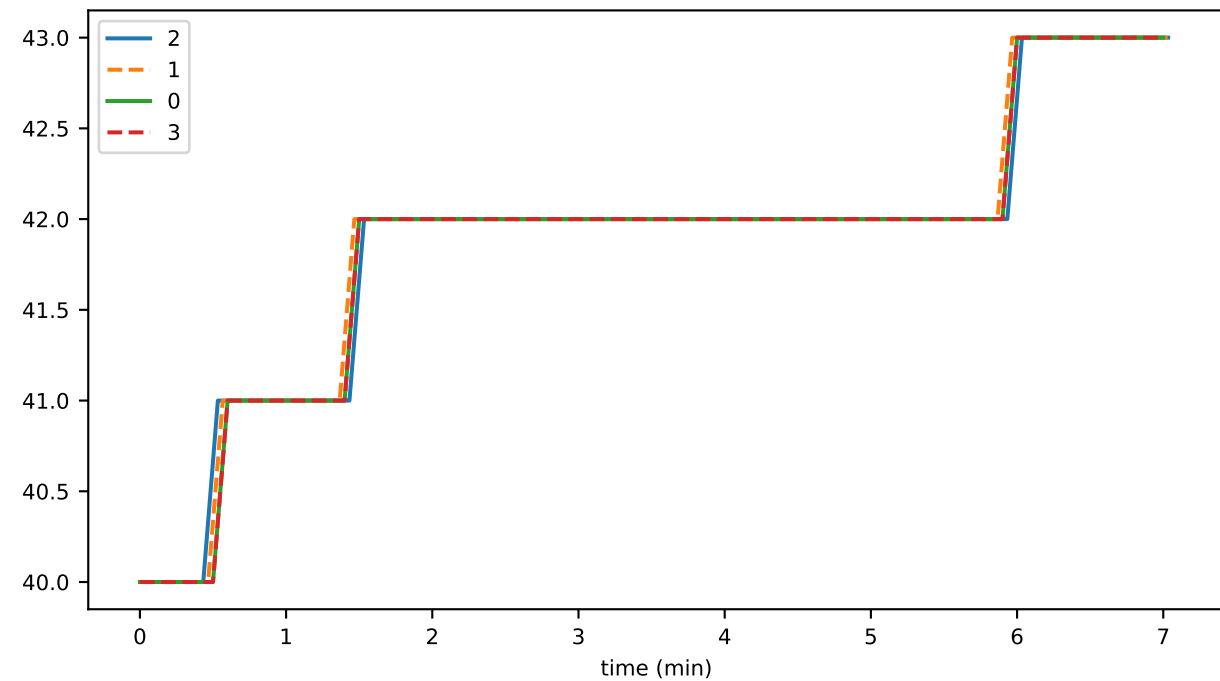
preconsensusEventFileCount
