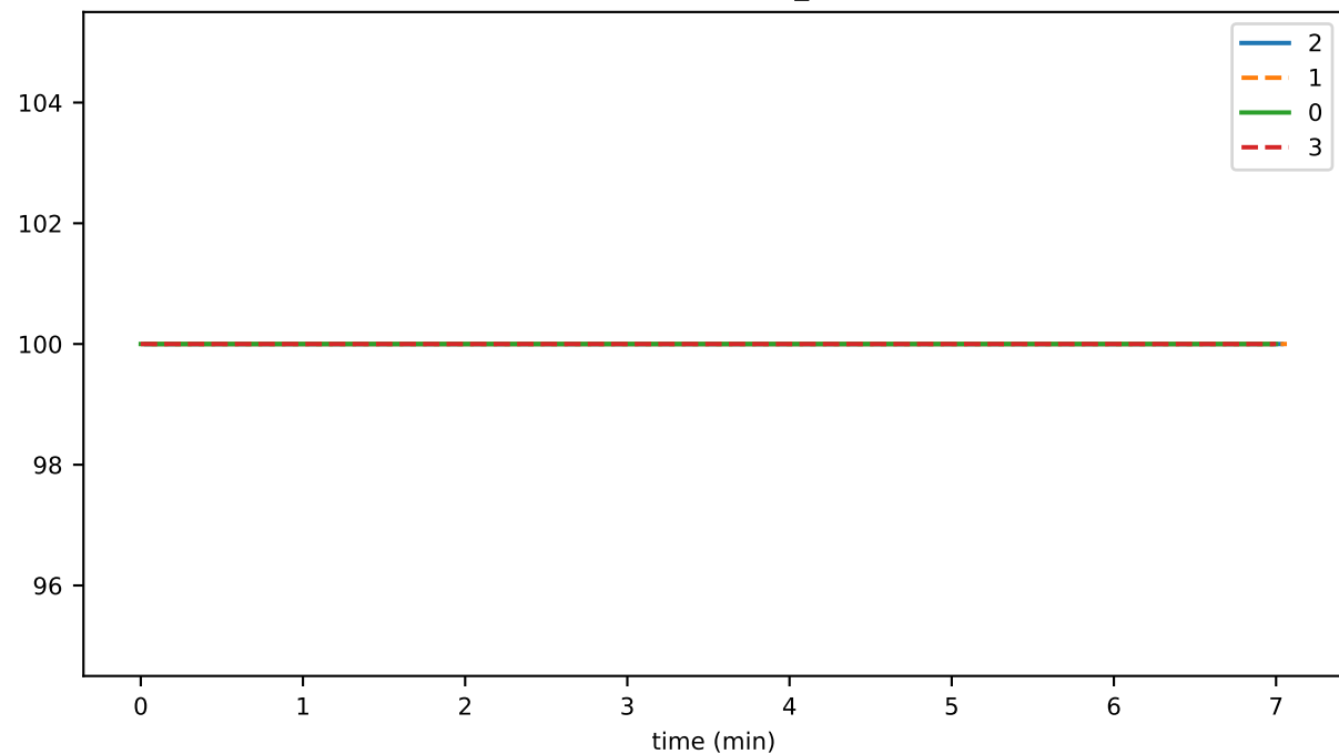
nodeActivePercentSnapshot_node0
