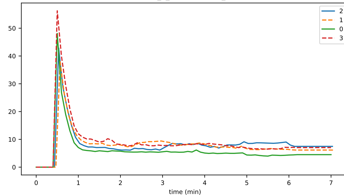
eventDelay_1_eventCreation_runtime
