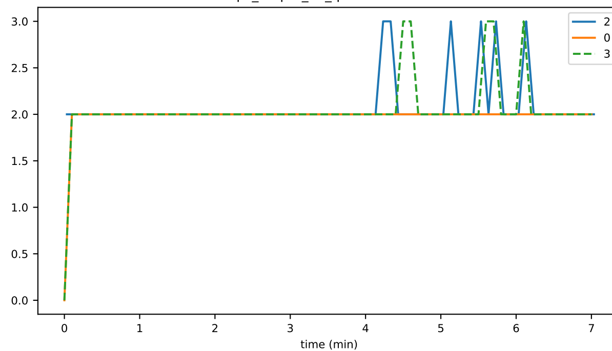
rpc_output_01_queueMaxSize
