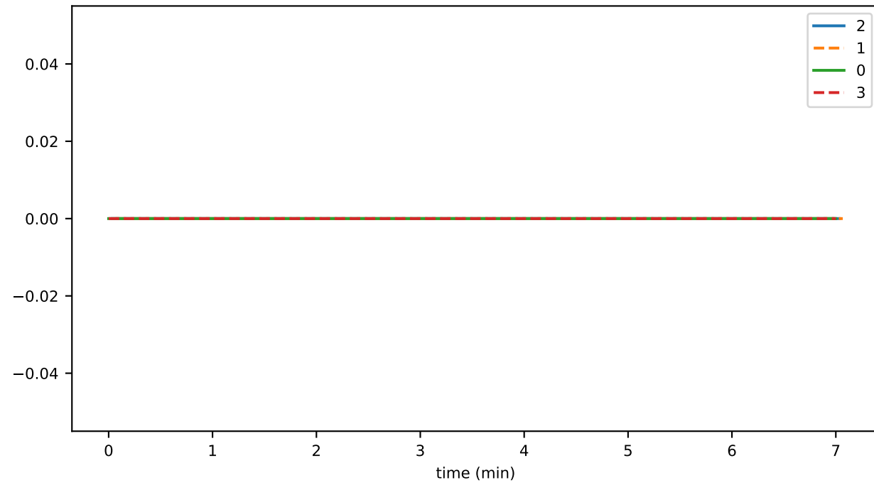
ds_compactions_level_6_hashesTimeMs_state
