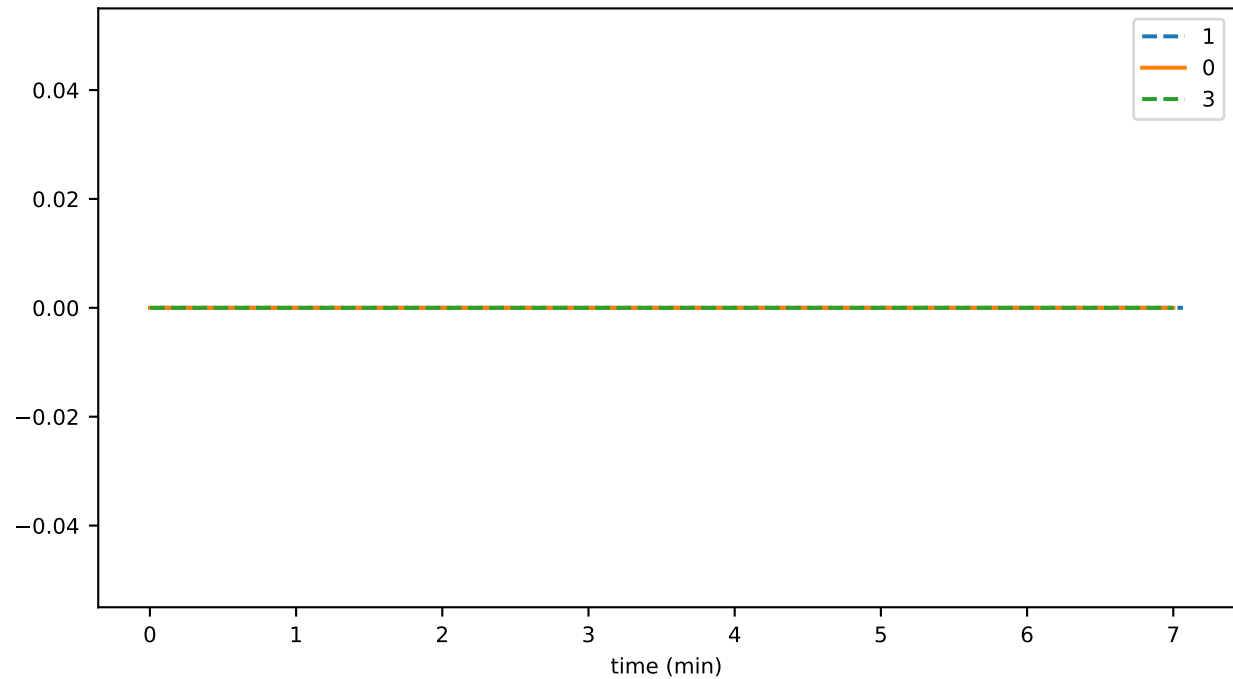
sync_phase_02_fraction_OTHER_FALLEN_BEHIND
