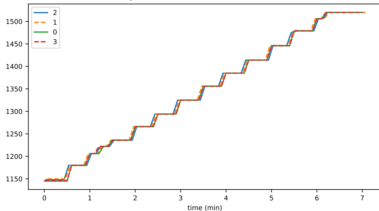
preconsensusEventFileTotalSizeGB
