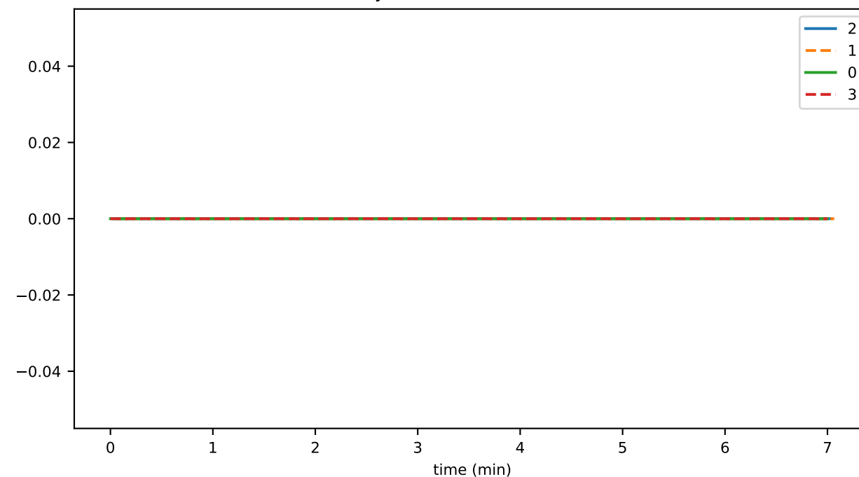
historyProofTransWMetaToWAsmCnt
