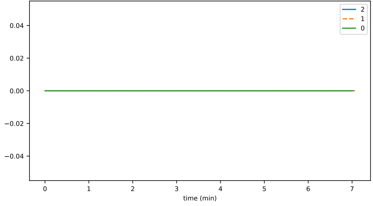
sync_phase_03_fraction_SELF_FALLEN_BEHIND
