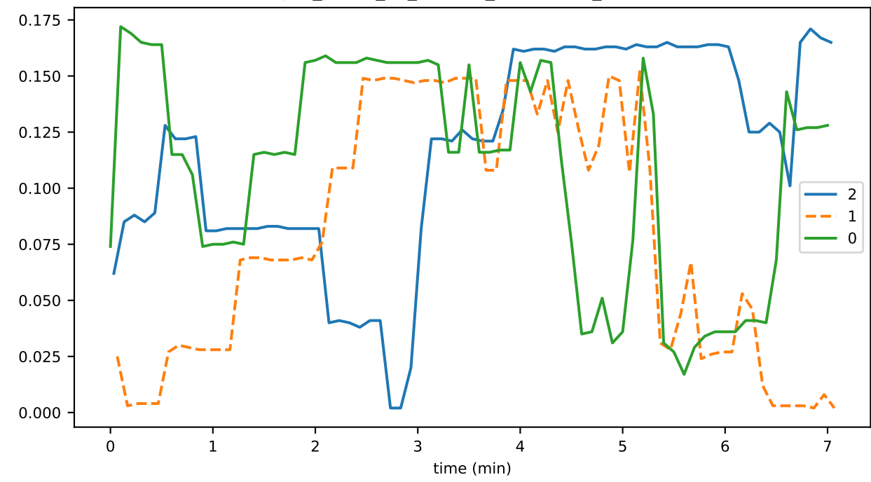
sync_phase_03_fraction_SENDING_EVENTS
