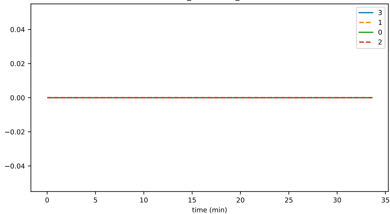
connRecv_endStream_timeout
