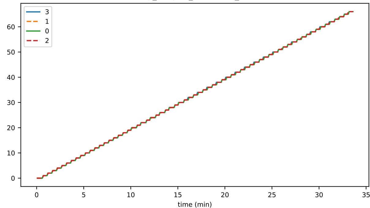
vmap_lifecycle_hashDurationMs_state
