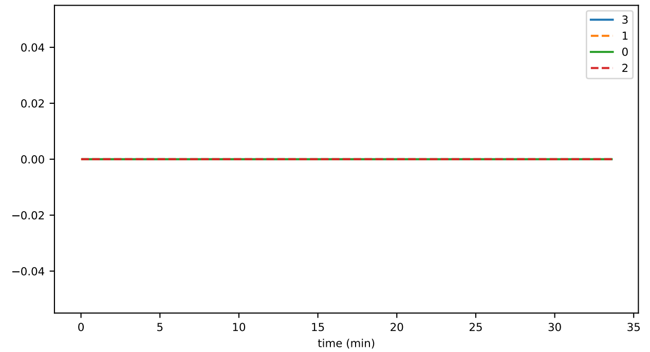
branchingNodeCount
