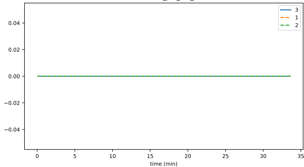
disconnects_per_sec_00
