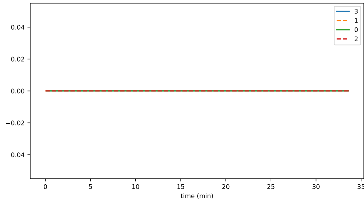
connSend_multitemRequestExceedsSoftLimit
