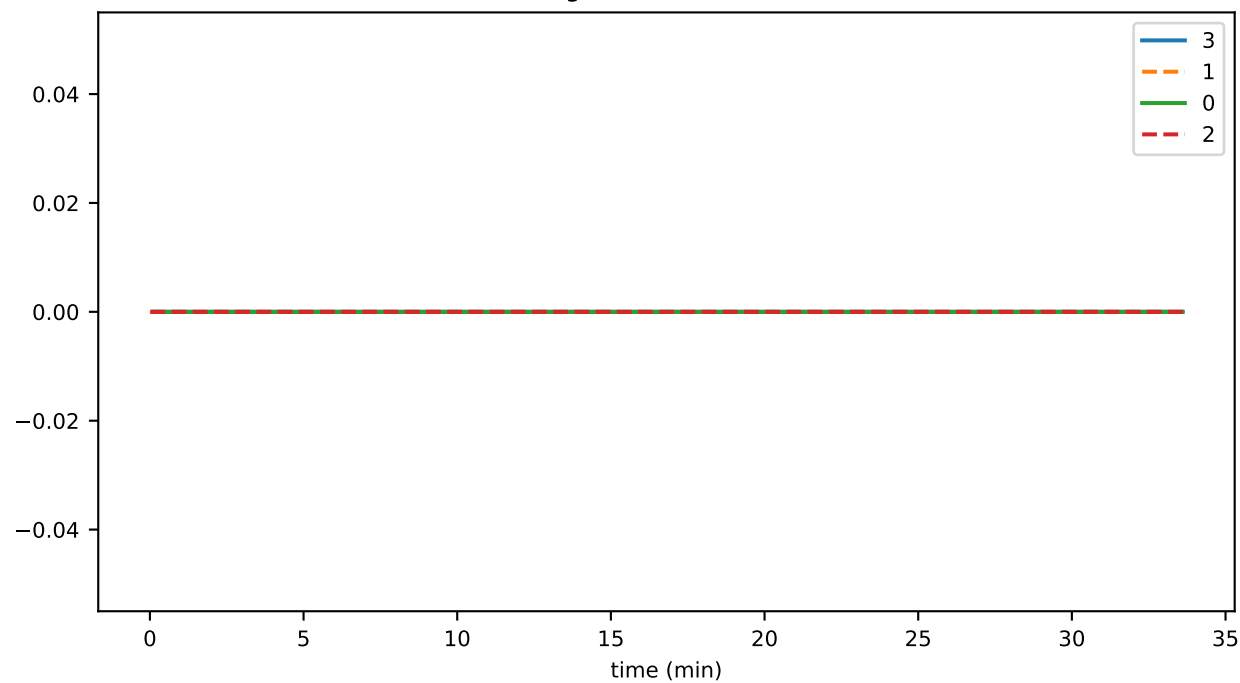
SigIntakePulseTime
