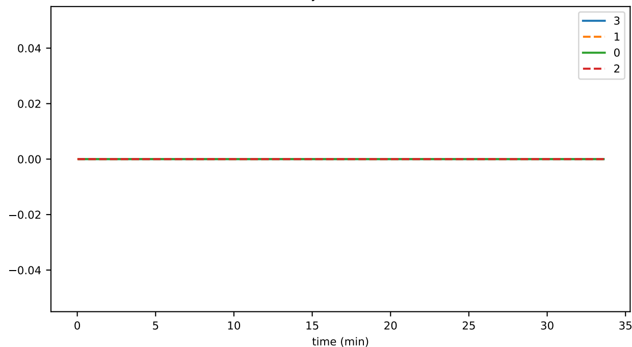
doNotSyncIntakeCounter
