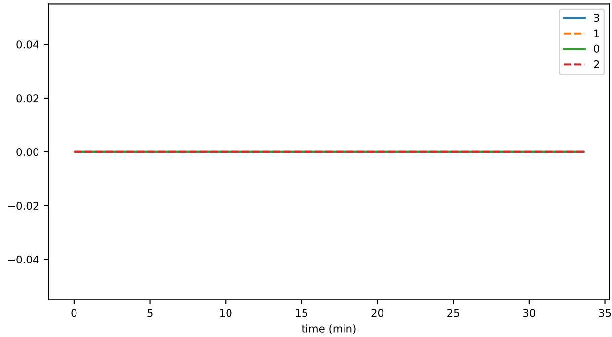
ds_compactions_level_2_hashesSavedSpaceMb_state
