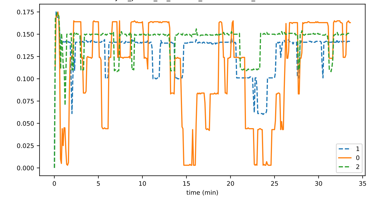
sync_phase_03_fraction_EXCHANGING_WINDOWS
