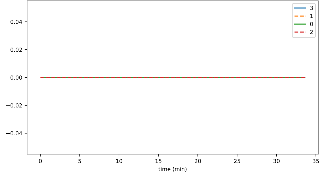
connRecv_skipBlock
