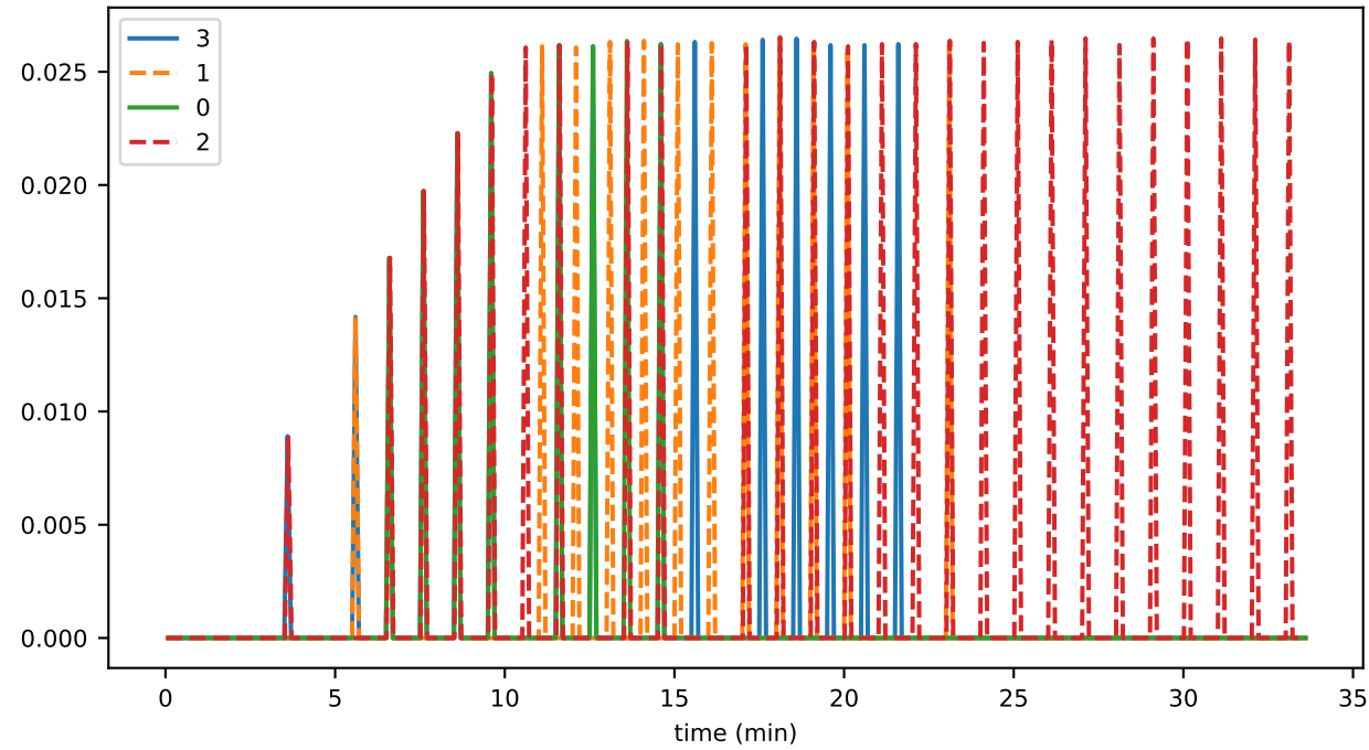
ds_compactions_level_2_hashesSavedSpaceMb_state
