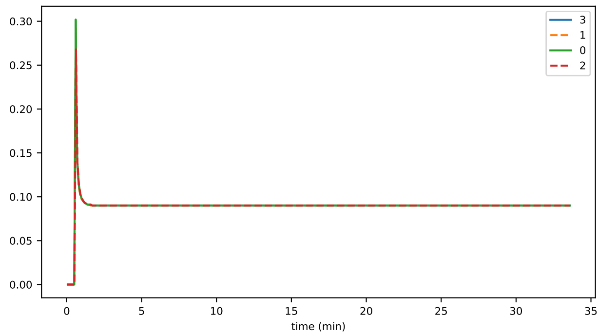
selfishness
