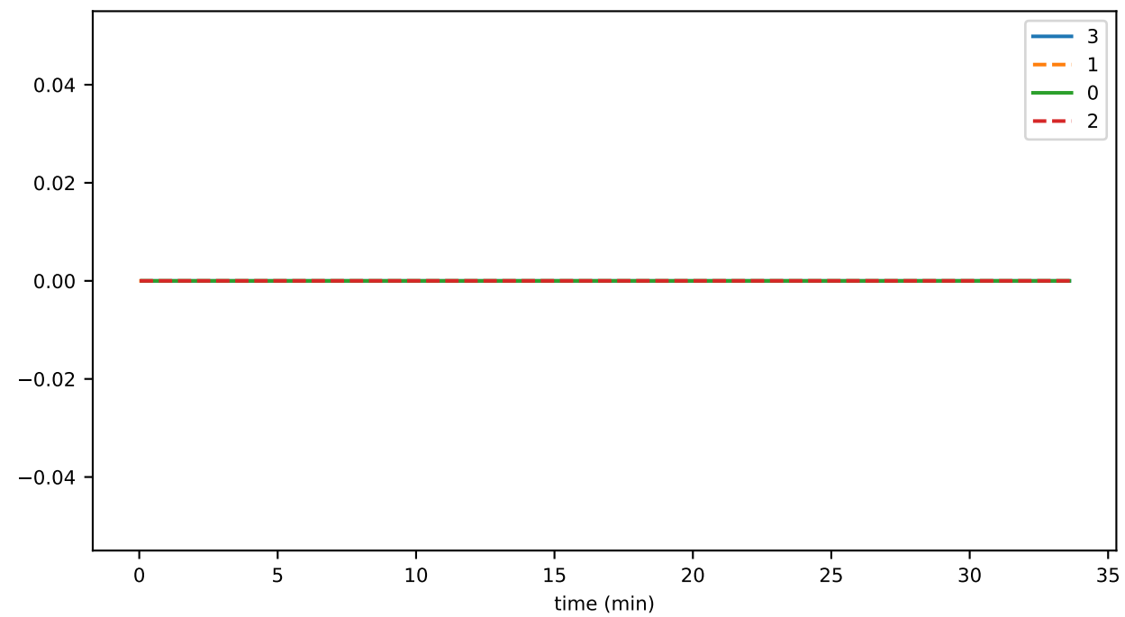
senderReconnectDurationSeconds
