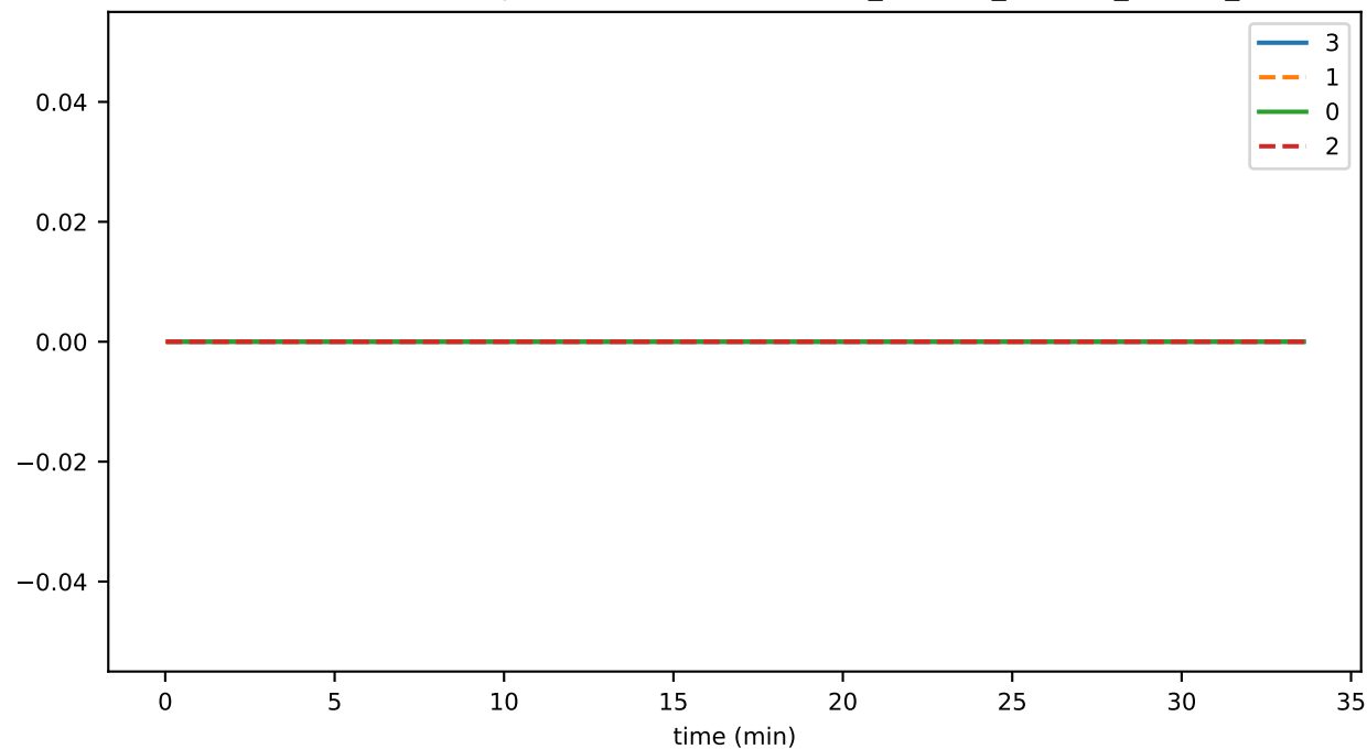
SmartContractService:SystemContractMethodCall_DIRECT_total
