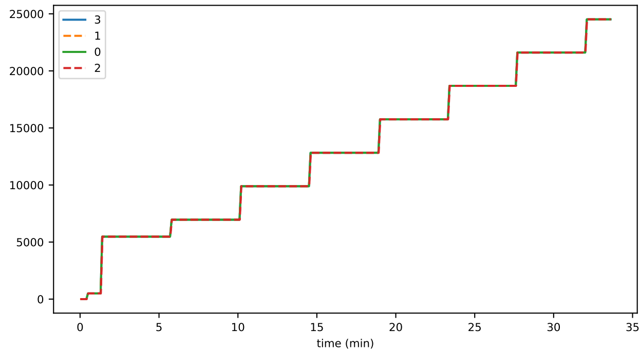
preconsensusEventFileYoungestIdentifier
