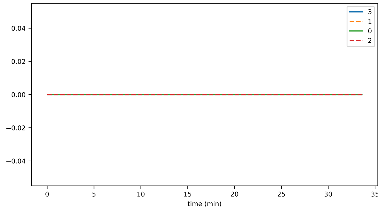
SigIntakeQueueDepth
