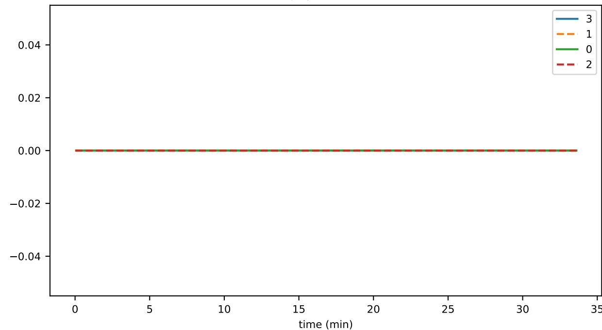
PlatformStatus
