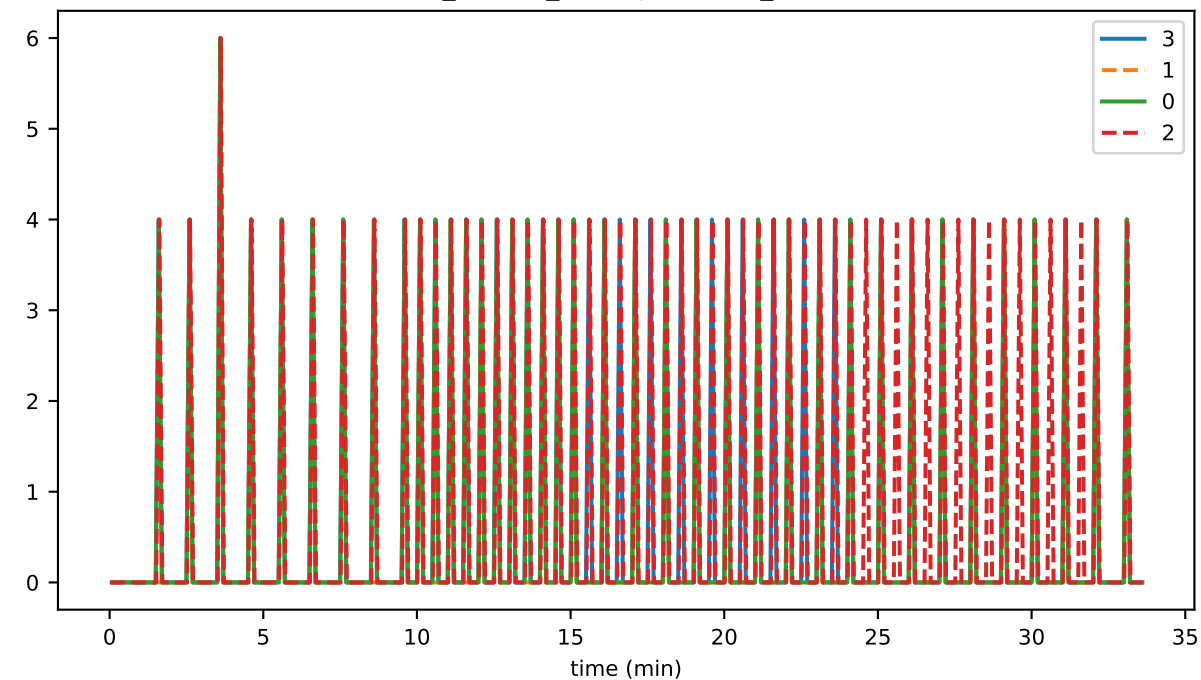
ds_flushes_leavesStoreFileSizeMb_state
