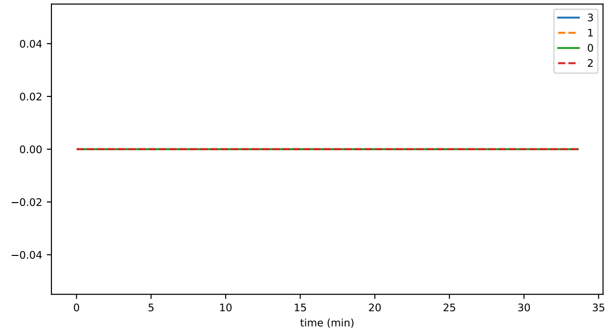
ds_compactions_level_4_hashesTimeMs_state
