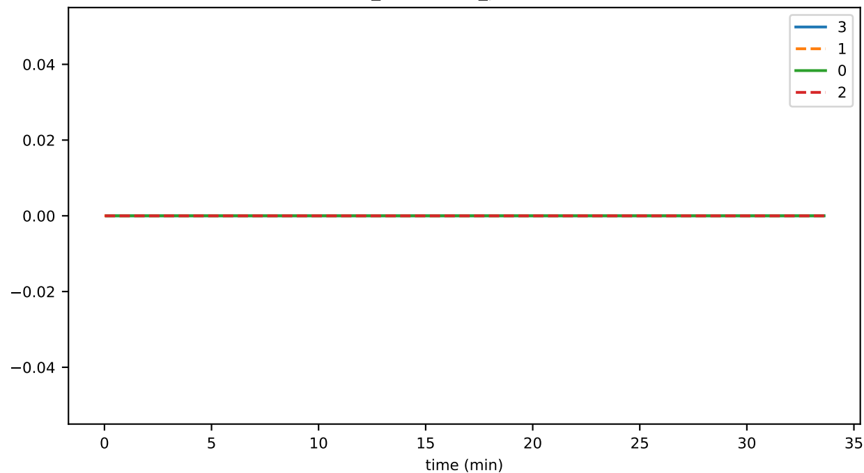
connRecv_endStream_timeout
