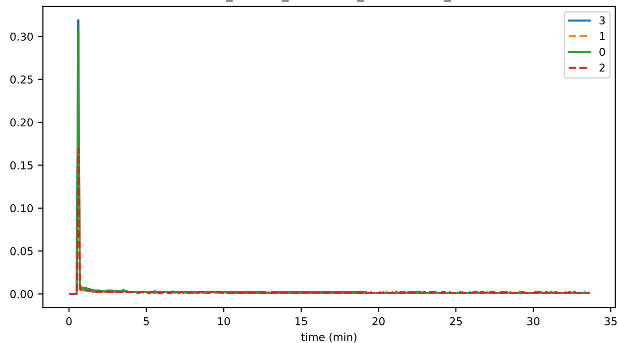
consensus_fraction_SETTING_EVENT_CONSENSUS_DATA
