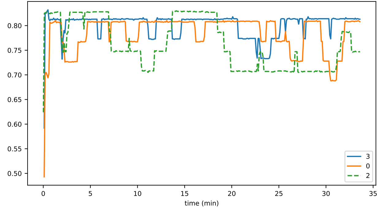
sync_phase_01_fraction_OTHER_FALLEN_BEHIND
