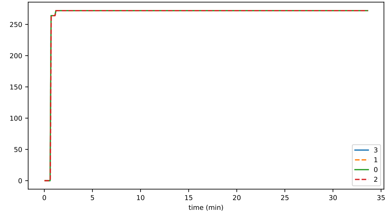
ds_offheap_hashesListMb_state
