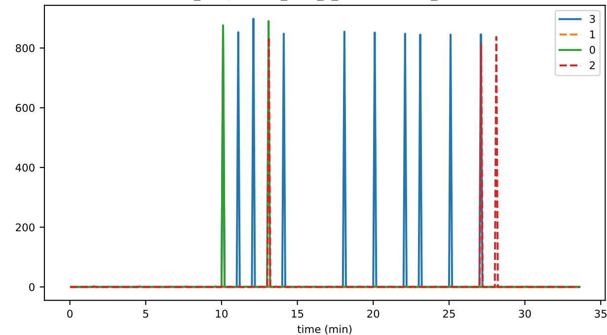
ds_compactions_level_1_leafKeysTimeMs_state
