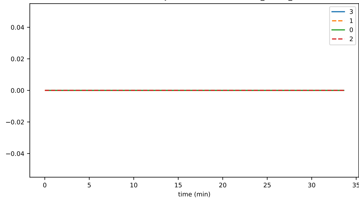
SmartContractService:SystemContractMethodCall_ERC20_failed
