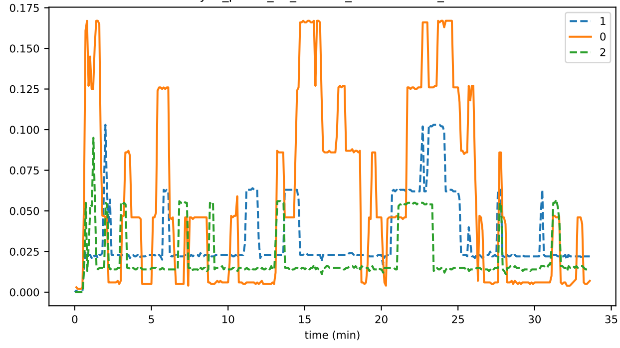
sync_phase_03_fraction_EXCHANGING_TIPS
