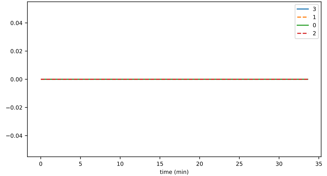
sync_per_secC
