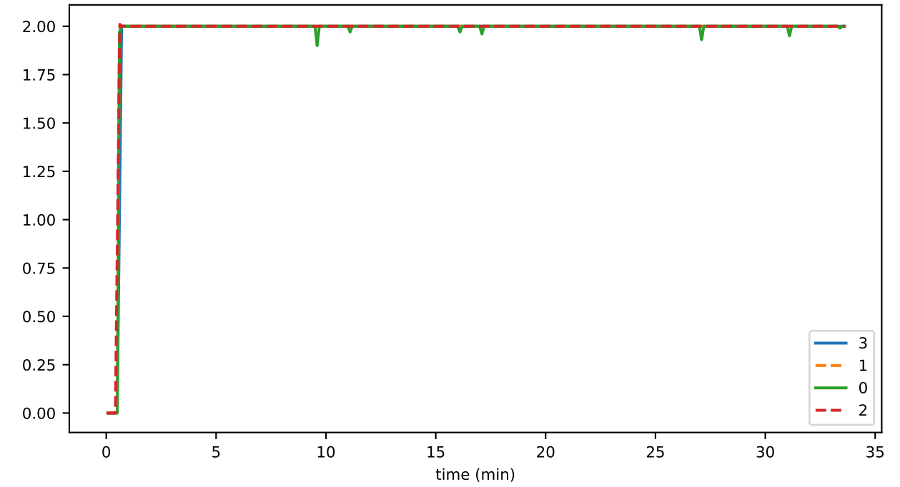
Dig_per_sec
