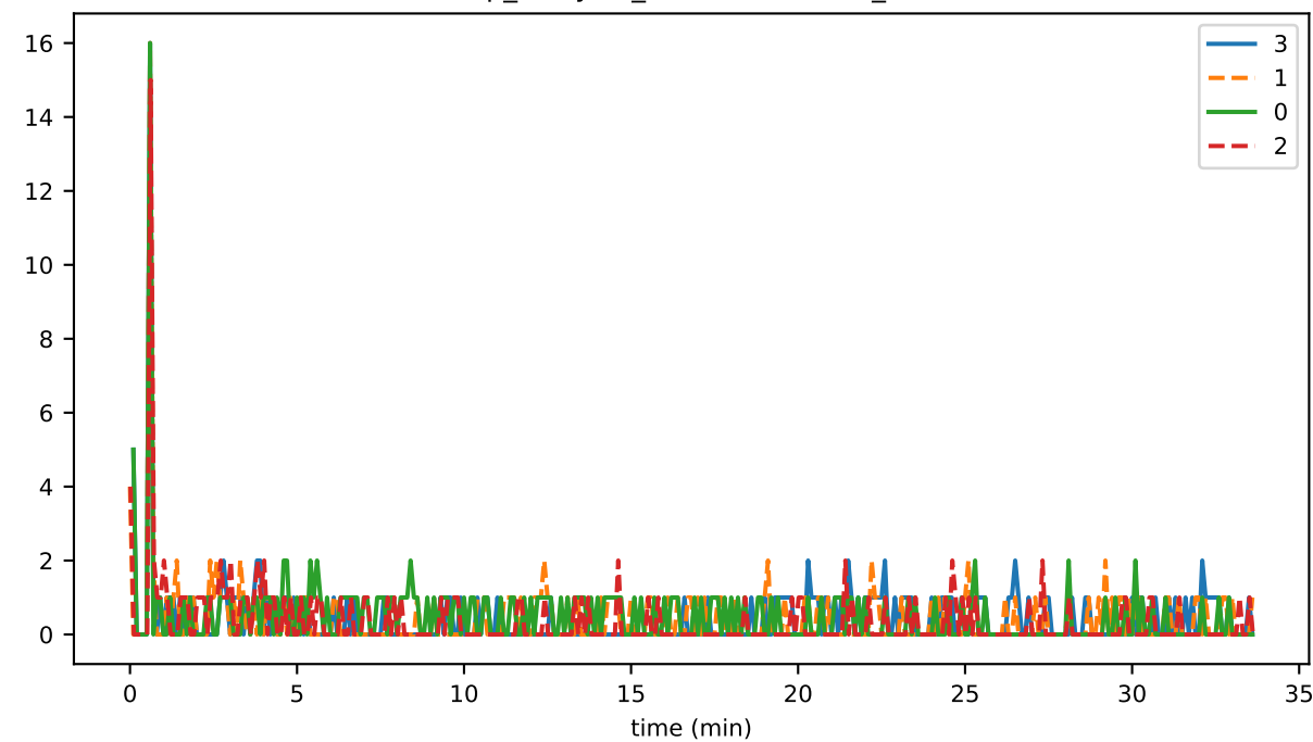
vmap_lifecycle_hashDurationMs_state
