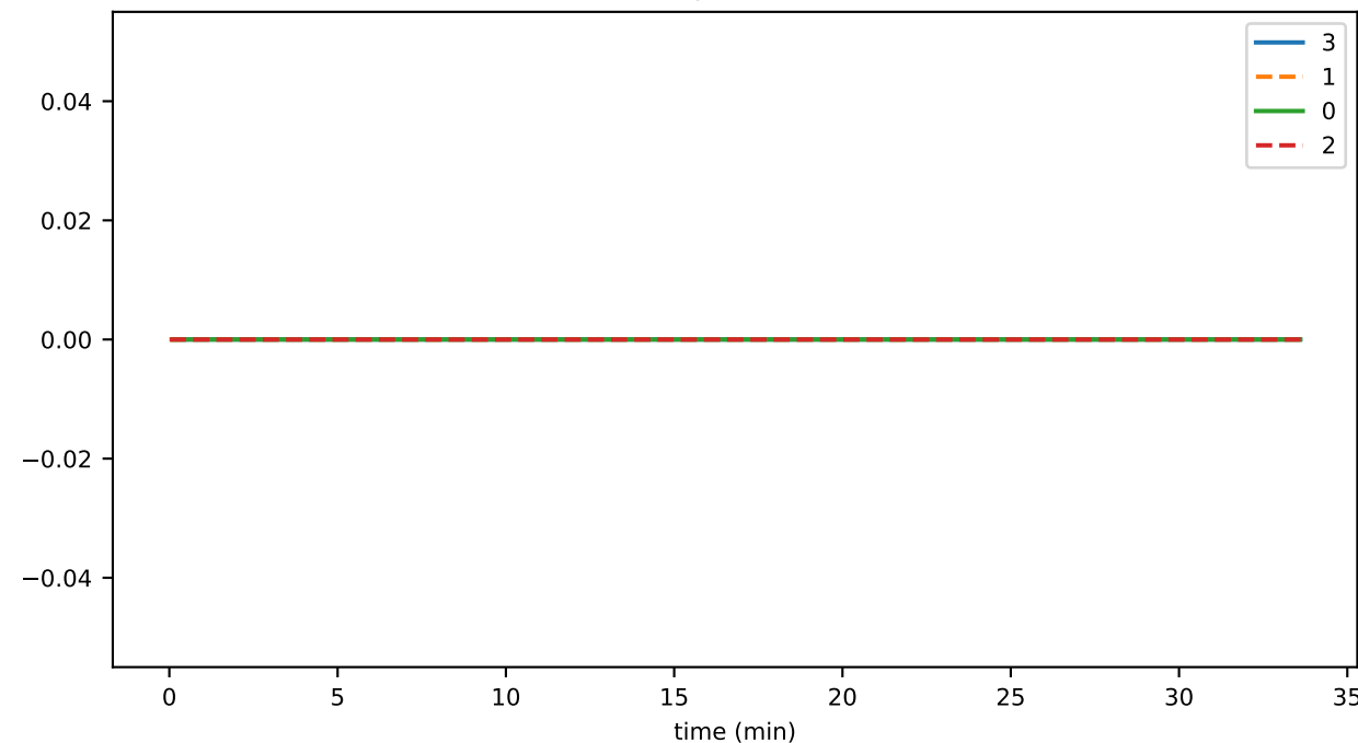
sigStateHash
