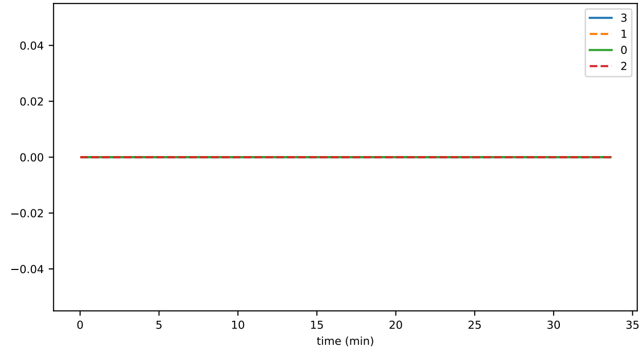
submittedPlatformTransactions
