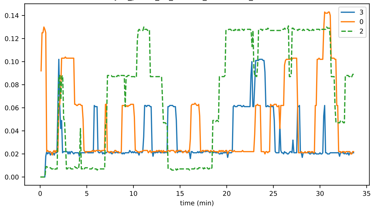
sync_phase_01_fraction_RECEIVING_EVENTS
