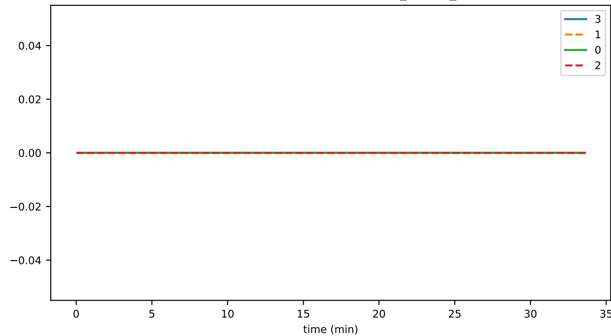
SmartContractService:Rejected_contractCallTx_total
