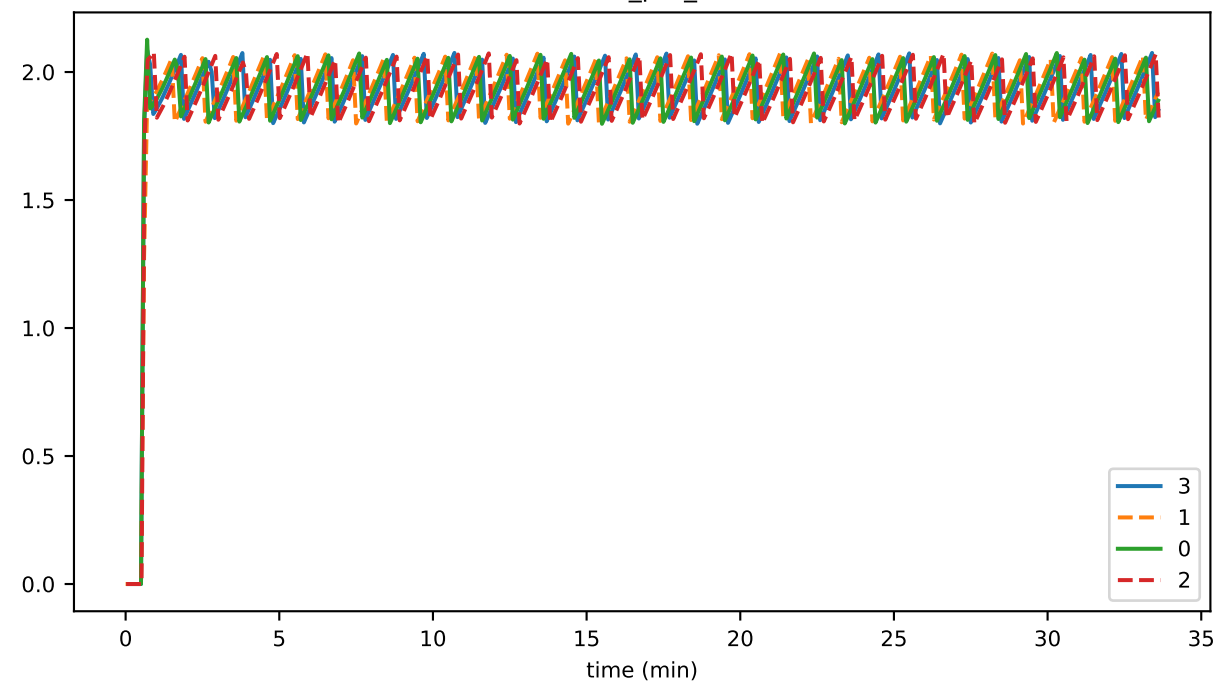
transH_per_sec
