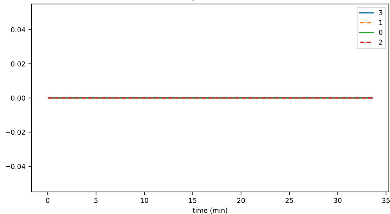
averageTimeToFullySignState
