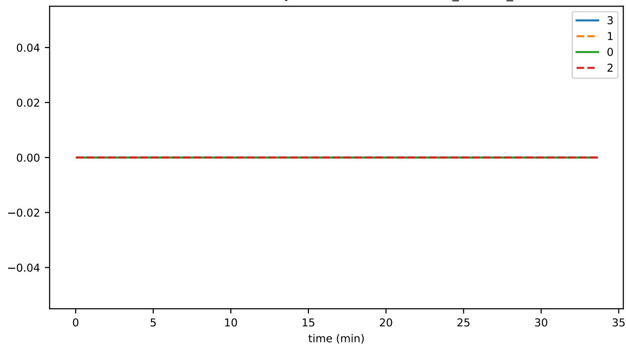
SmartContractService:SystemContractMethodCall_DIRECT_total
