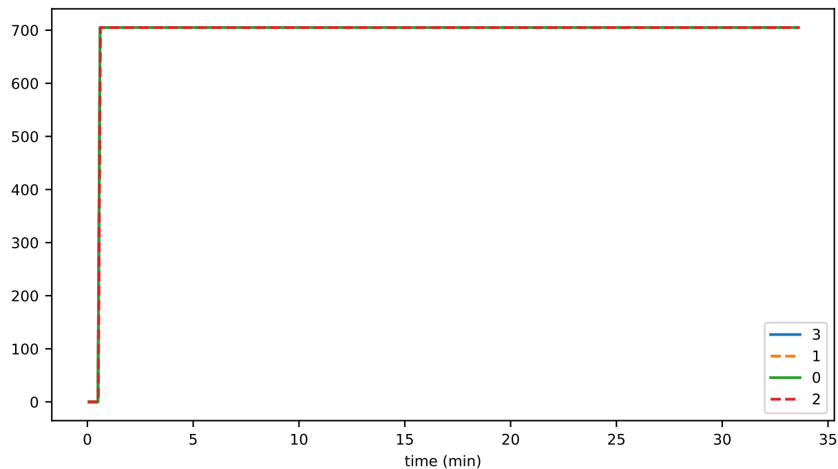
airdropsUsed
