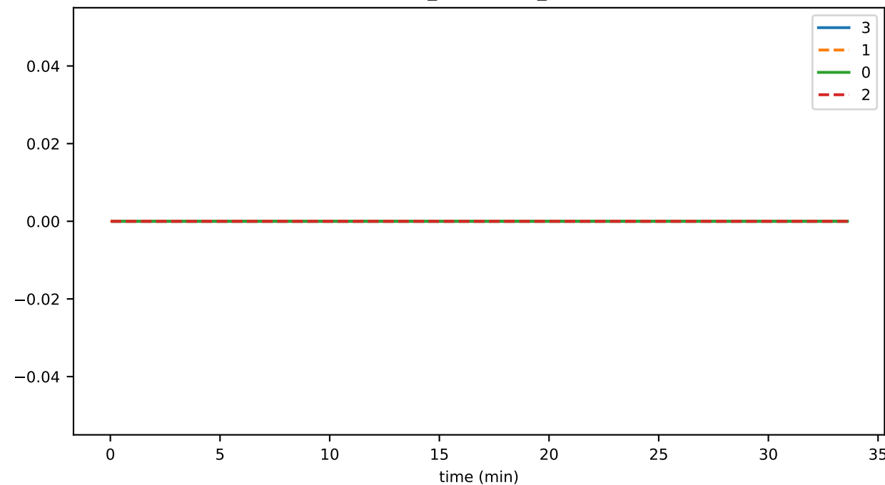
connRecv_endStream_unknown
