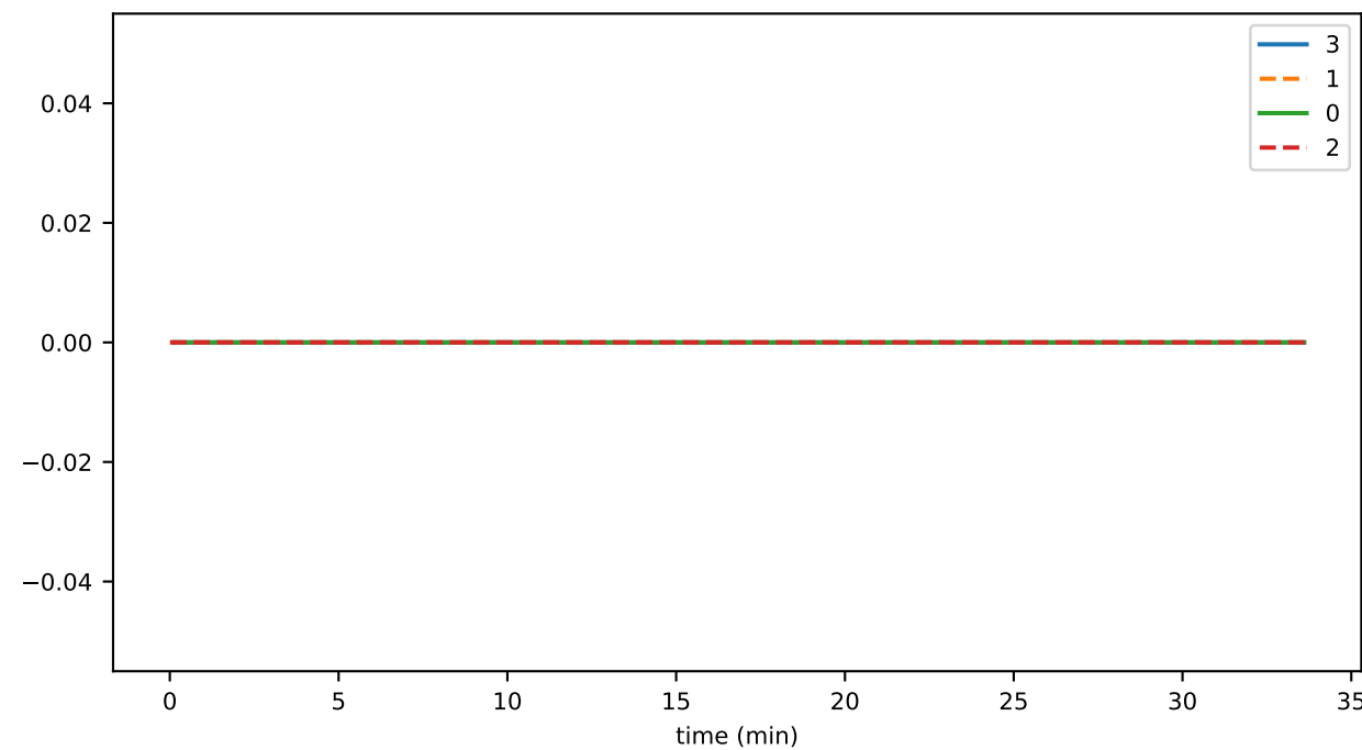
endsReconnectAsReceiver
