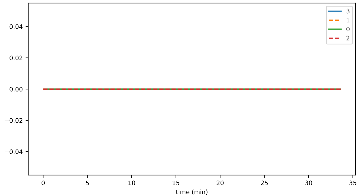
SigIntakePulseTime
