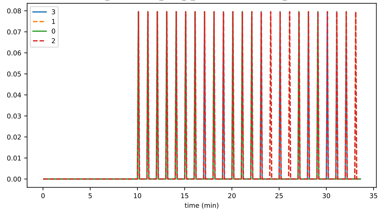
ds_compactions_level_1_leafKeysSavedSpaceMb_state
