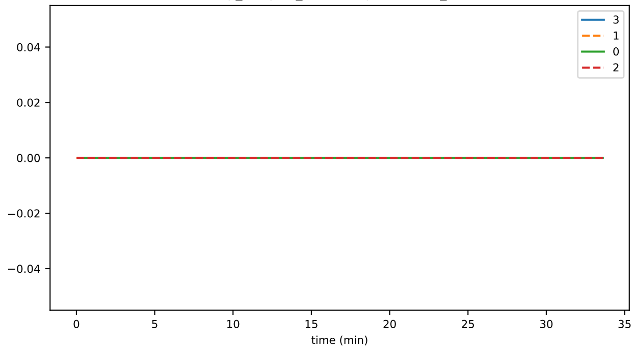
vmap_lifecycle_flushDurationMs_state
