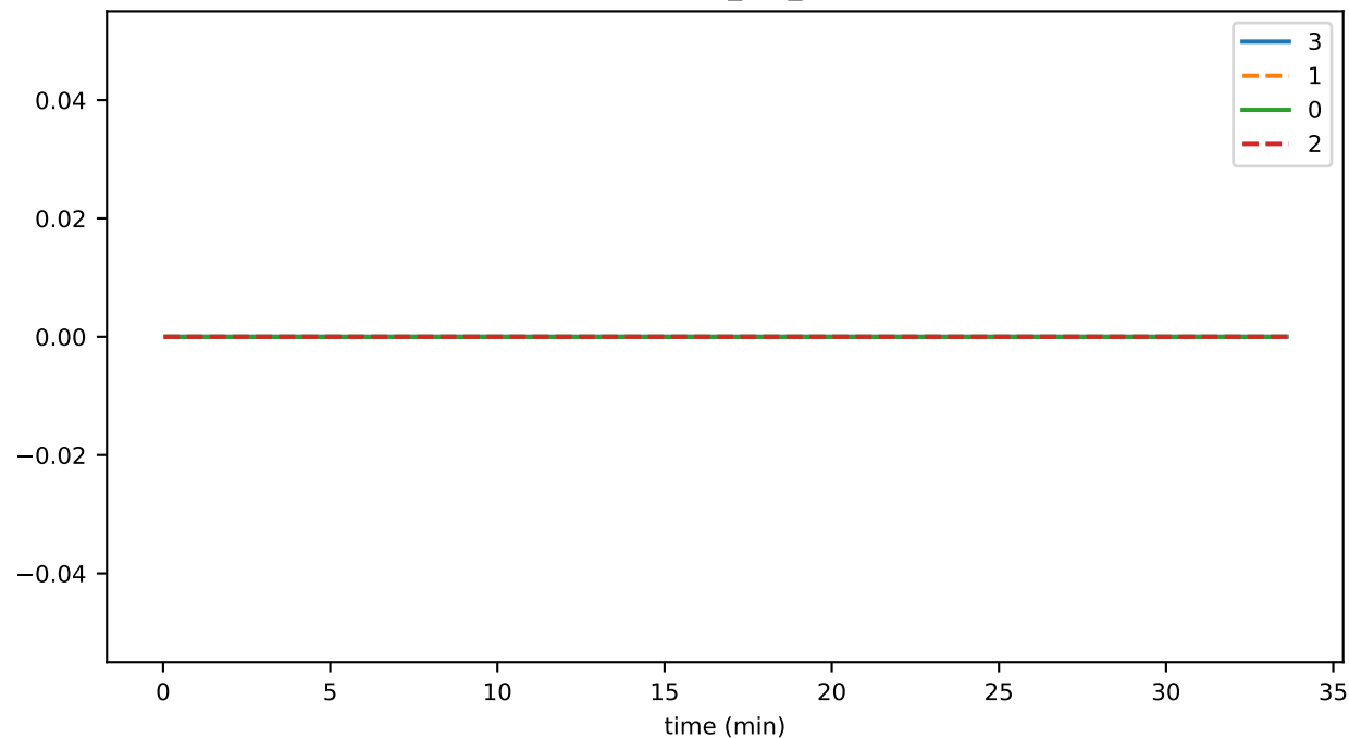
SigSpans_per_sec
