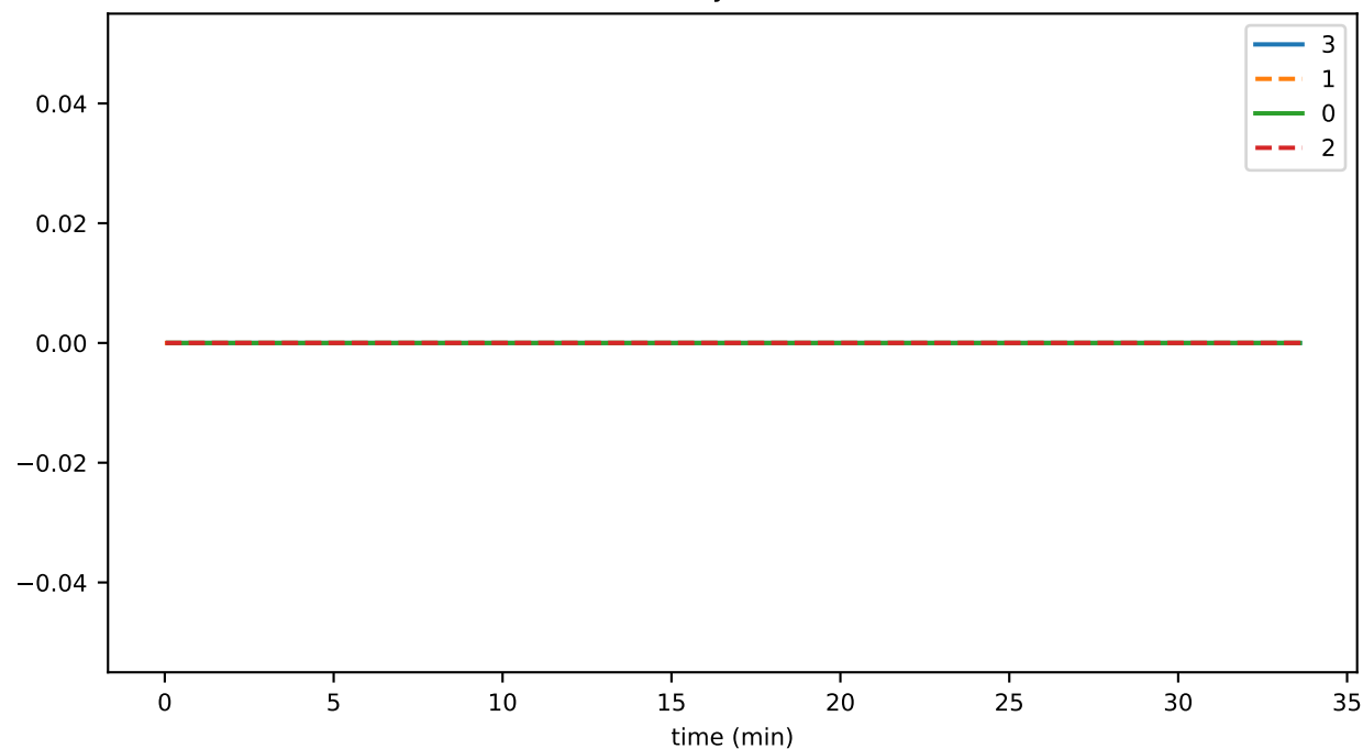
doNotSyncHalted
