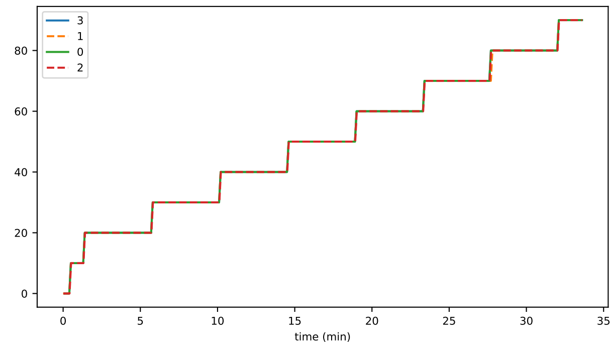
disconnects_per_sec_00
