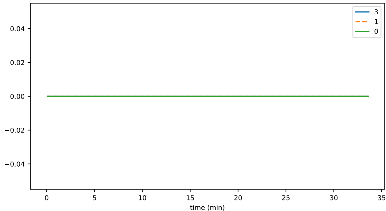
sync_phase_02_fraction_NO_PERMIT
