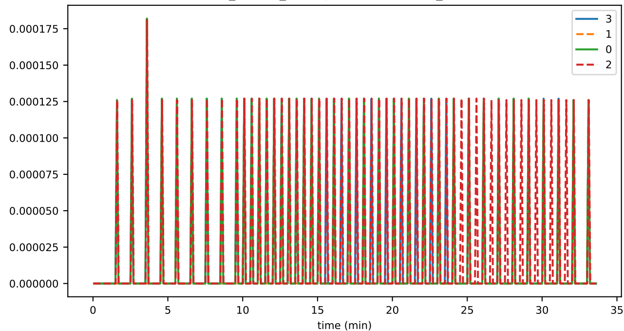
ds_flushes_leavesDeleted_state
