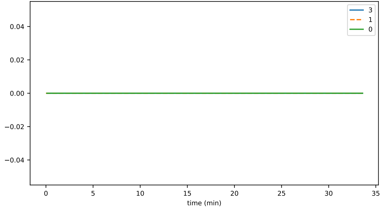
sync_phase_03_fraction_EXCHANGING_TIPS
