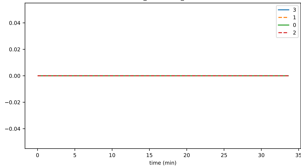
connRecv_endStream_unknown
