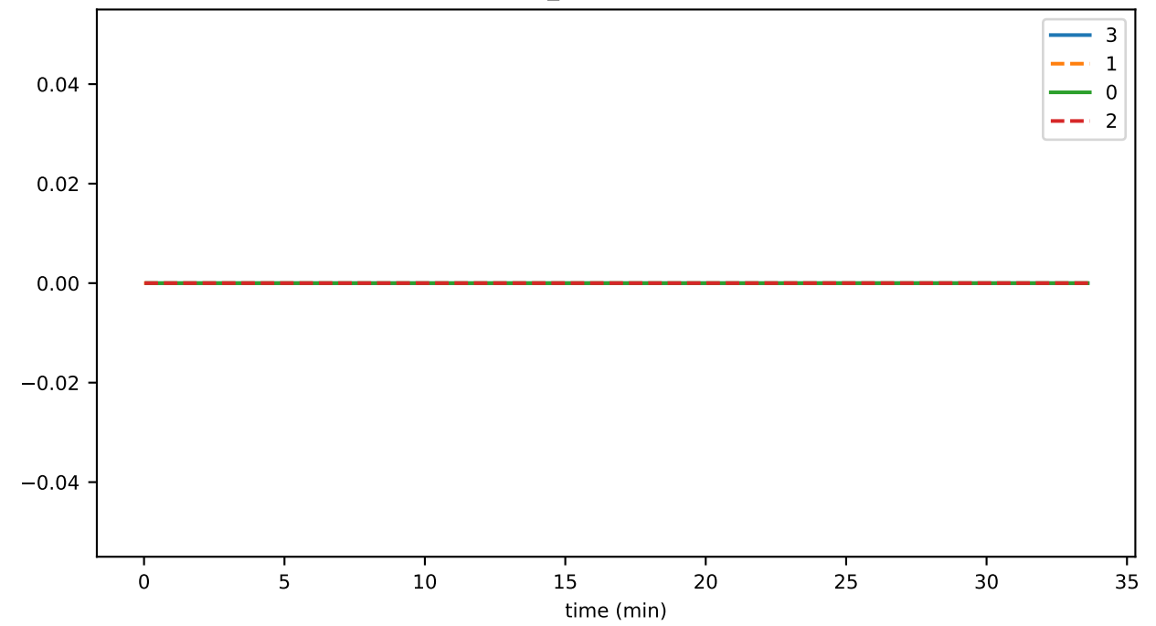
connSend_requestSendLatency
