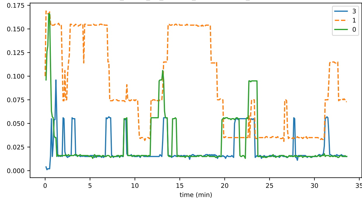
sync_phase_02_fraction_EXCHANGING_WINDOWS
