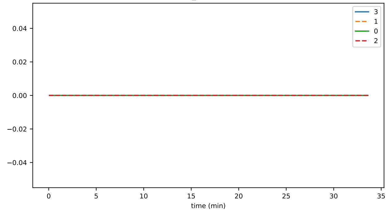
conn_onComplete
