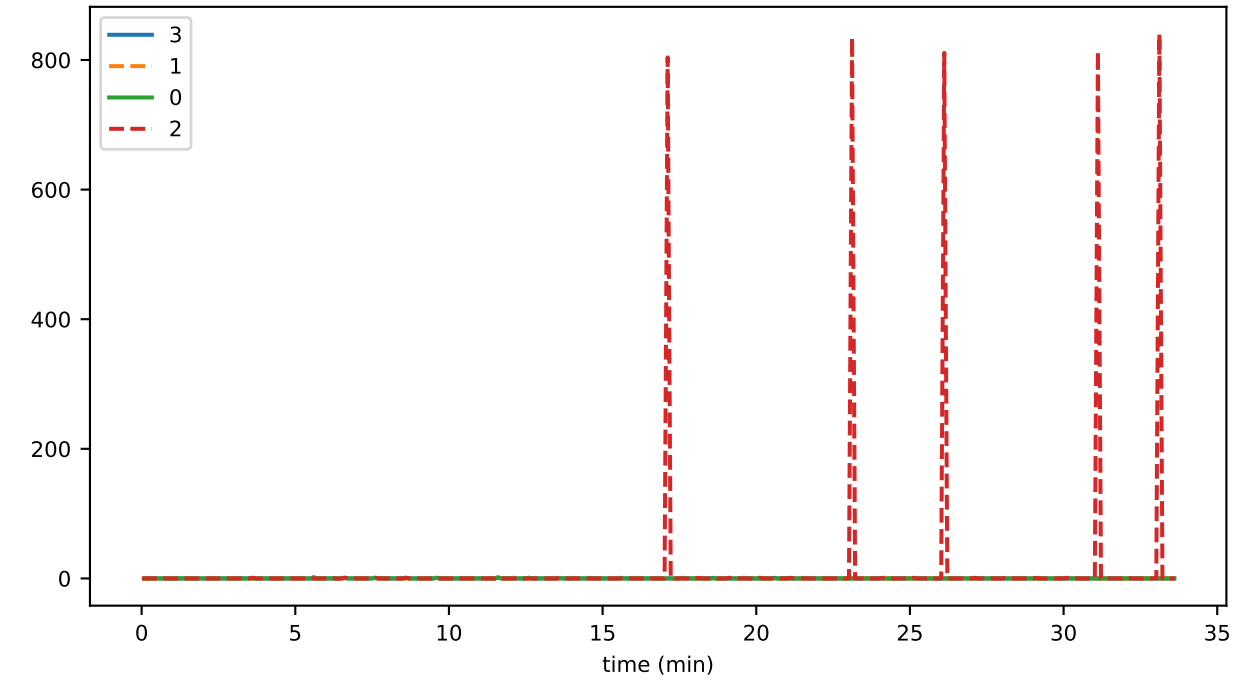
ds_compactions_level_2_hashesTimeMs_state
