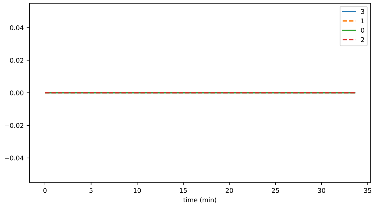
SmartContractService:OpsDuration_TxnsThrottled
