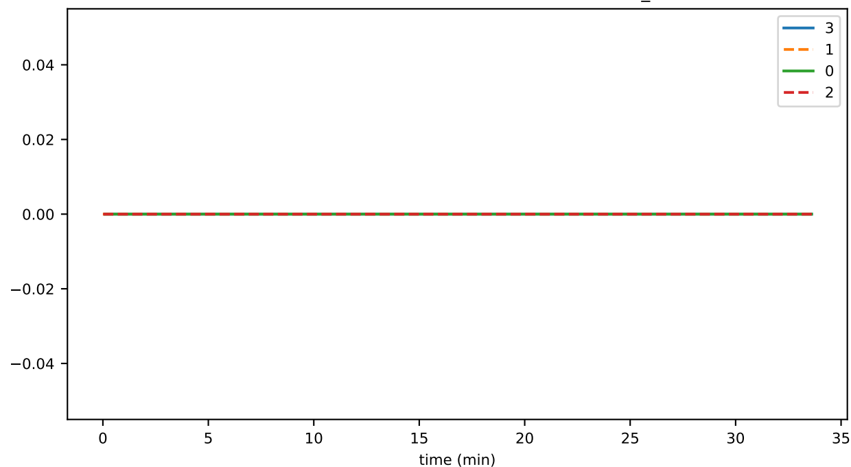
SmartContractService:LatestGasPrice
