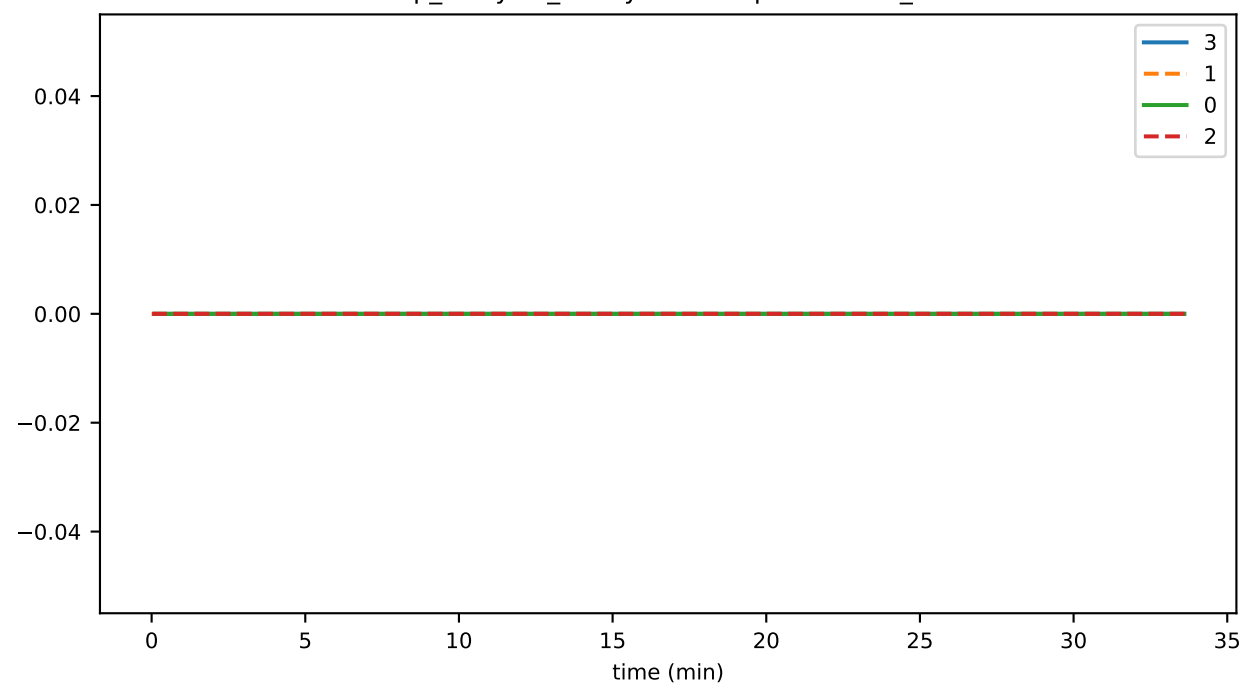
vmap_lifecycle_familySizeBackpressureMs_state
