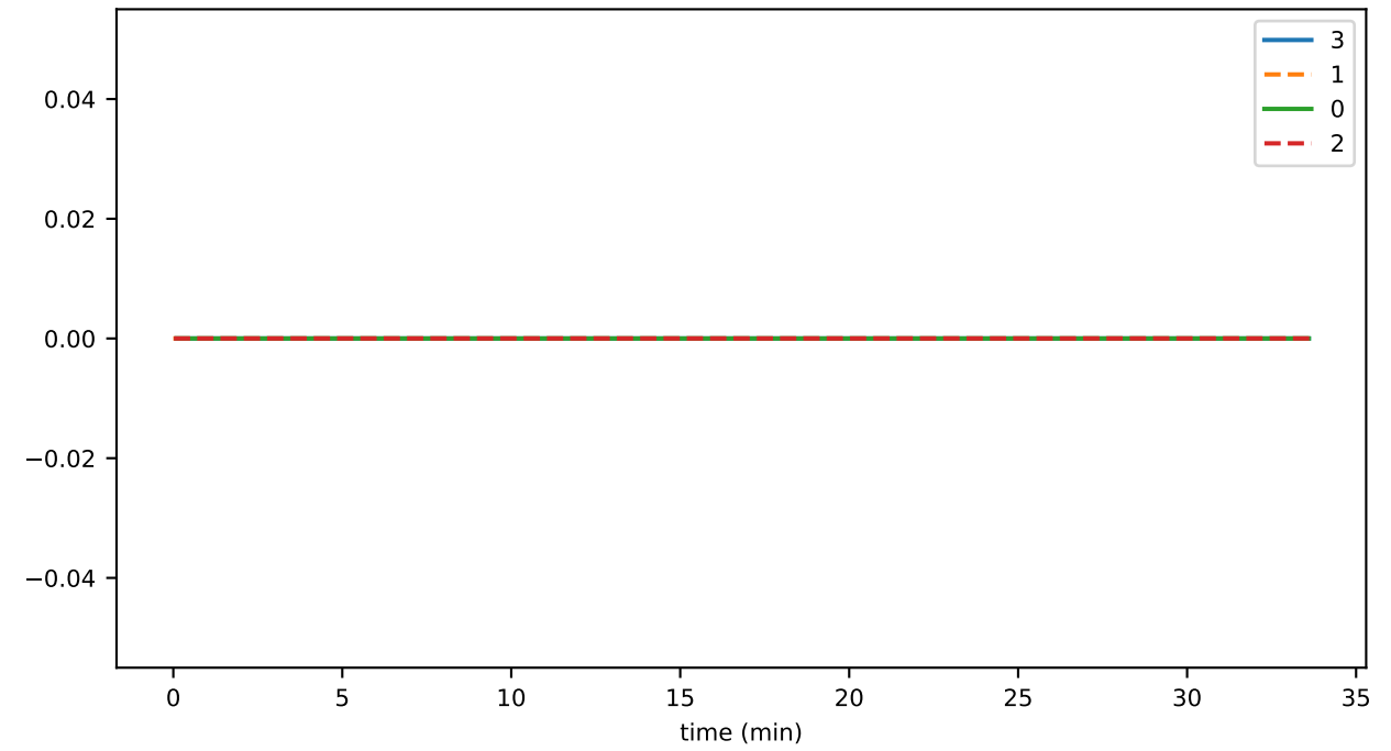
ds_compactions_level_8_leavesTimeMs_state
