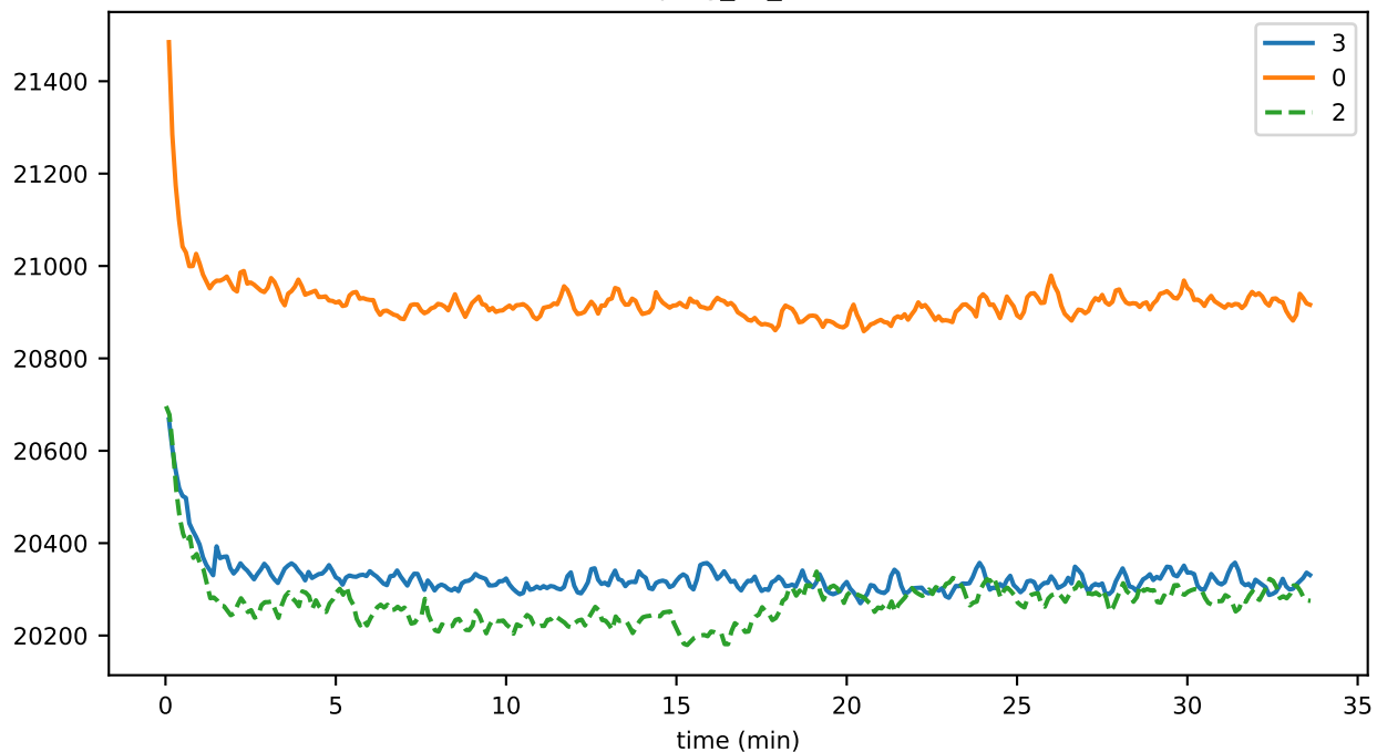
ping_us_02
