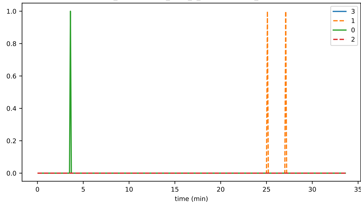
ds_compactions_level_2_leavesTimeMs_state
