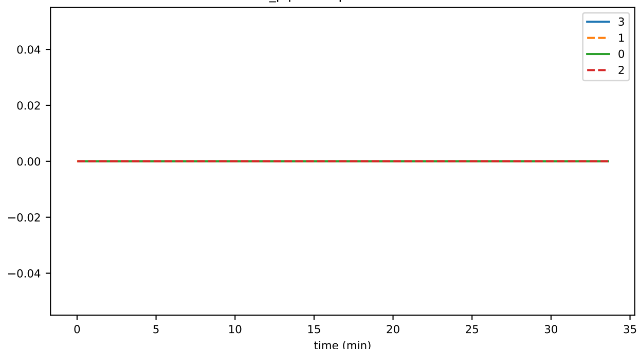
conn_pipelineOperationTimeout
