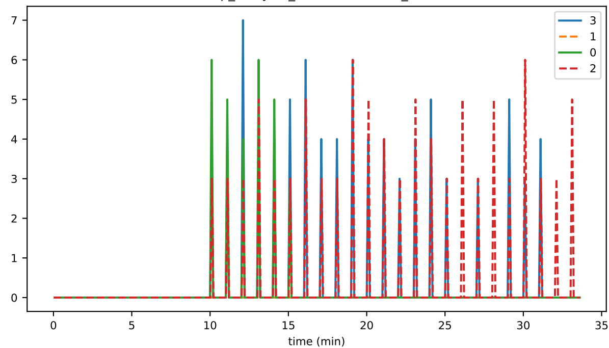
vmap_lifecycle_flushDurationMs_state
