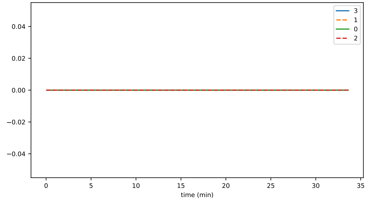
connRecv_skipBlock
