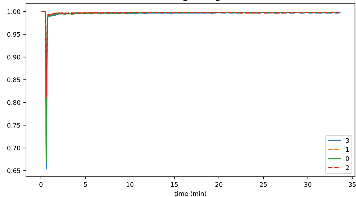
consensus_fraction_UPDATING_PLATFORM_STATE
