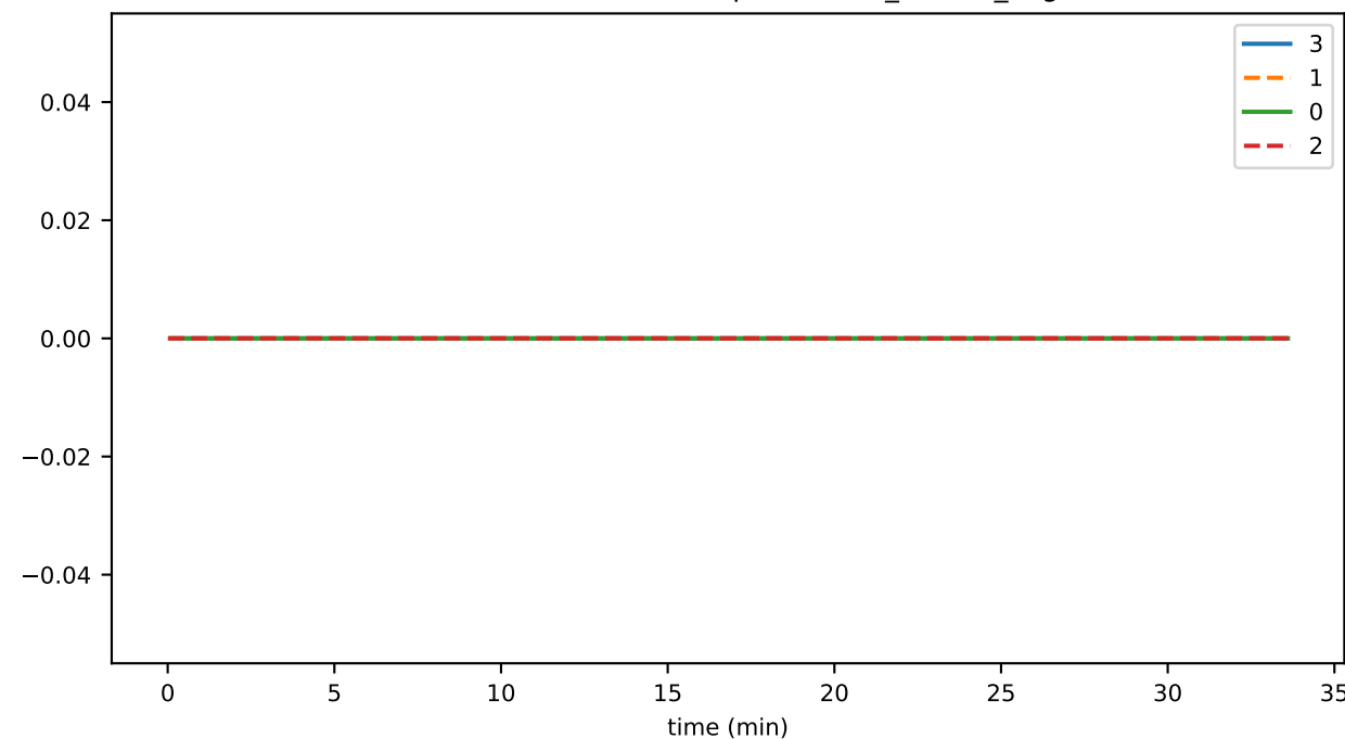
SmartContractService:OpsDuration_PerTxn_avg
