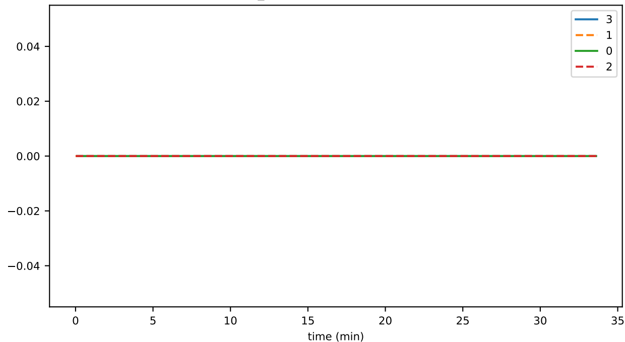
conn_endOfStreamLimitExceeded
