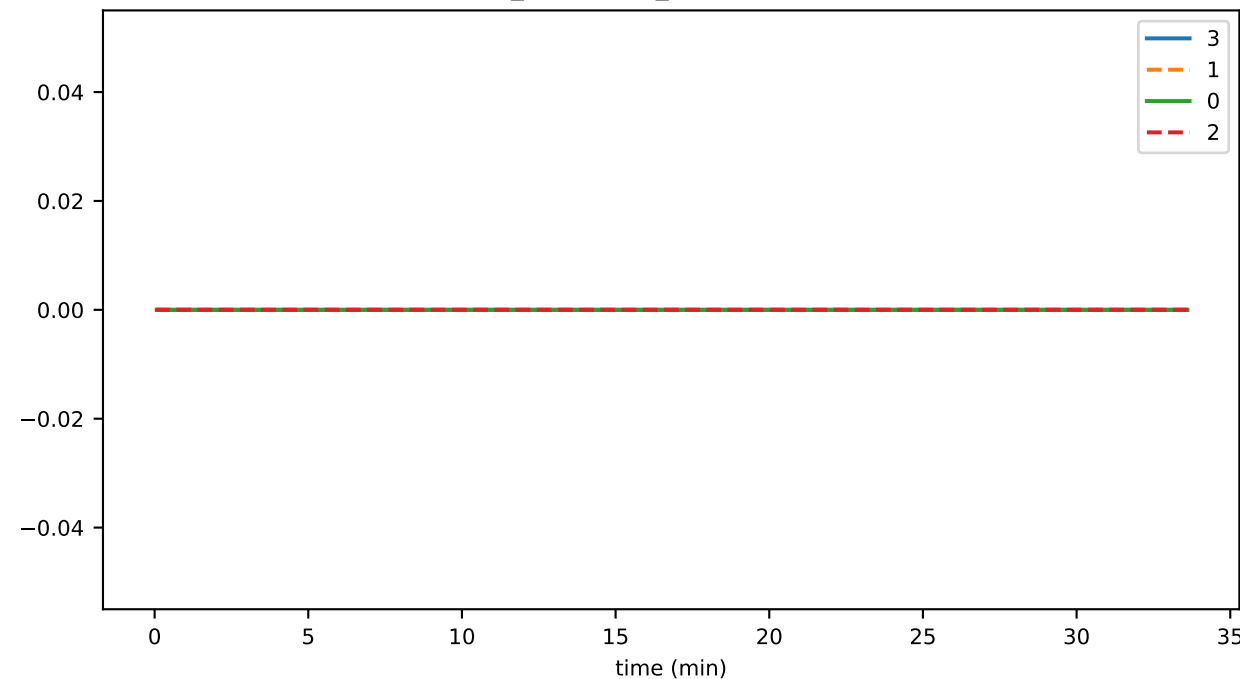
conn_connClose_blockNodeBehind
