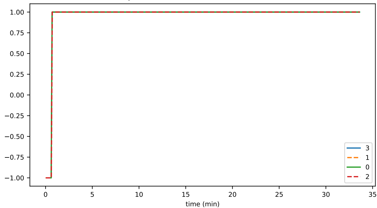
preconsensusEventFileOldestIdentifier
