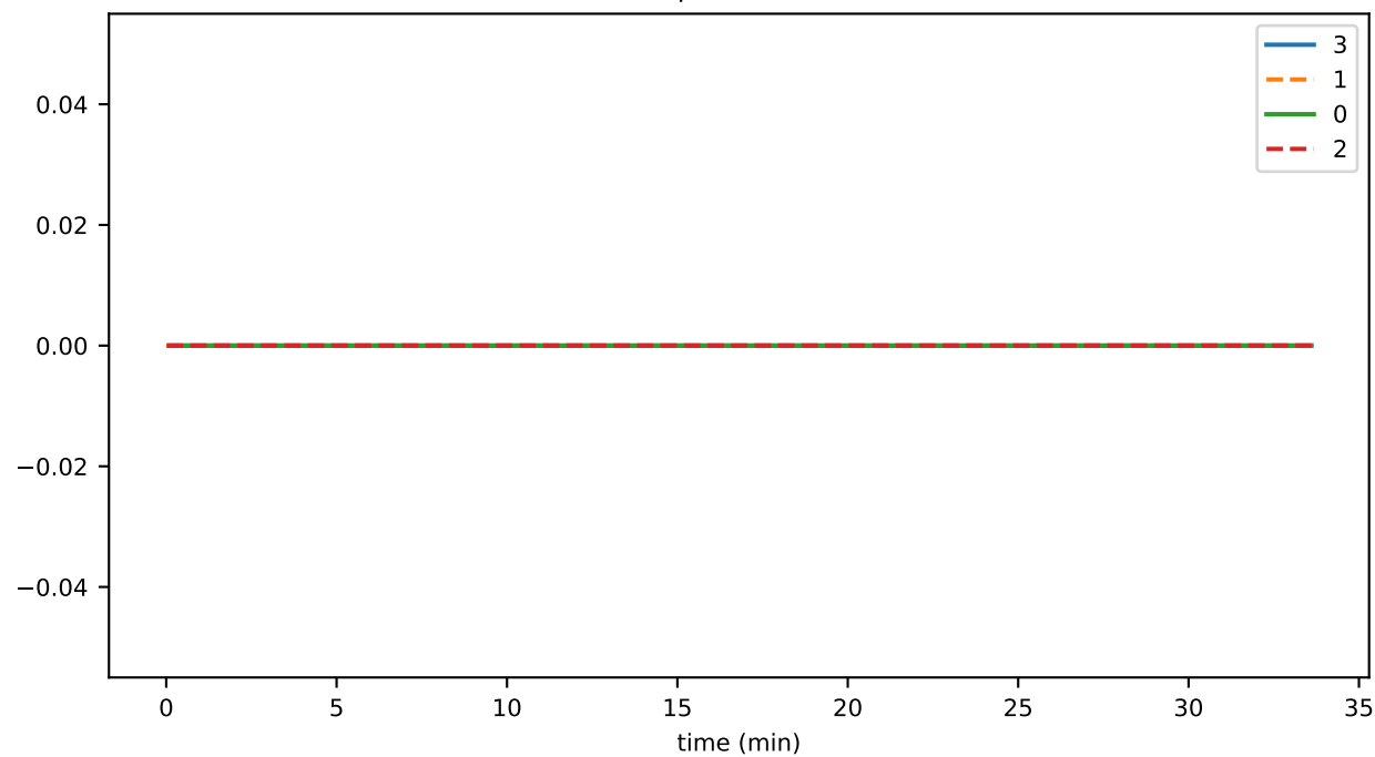
dupEvPercent
