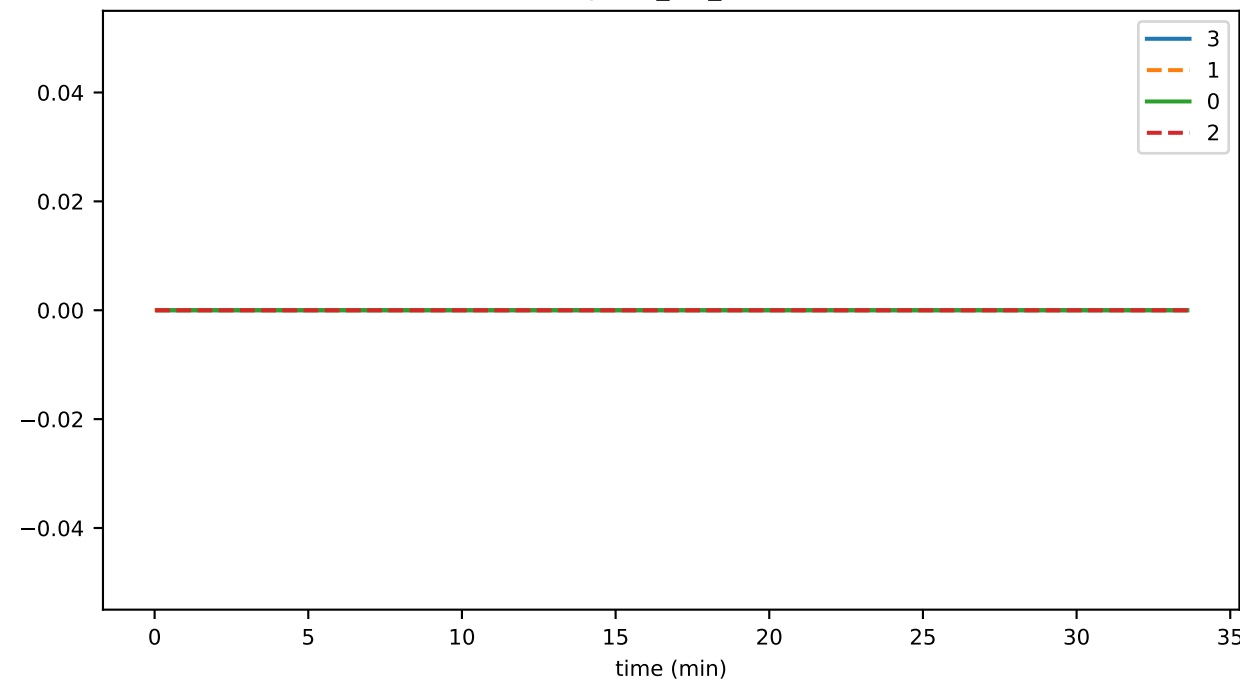
roundIncEqParents
