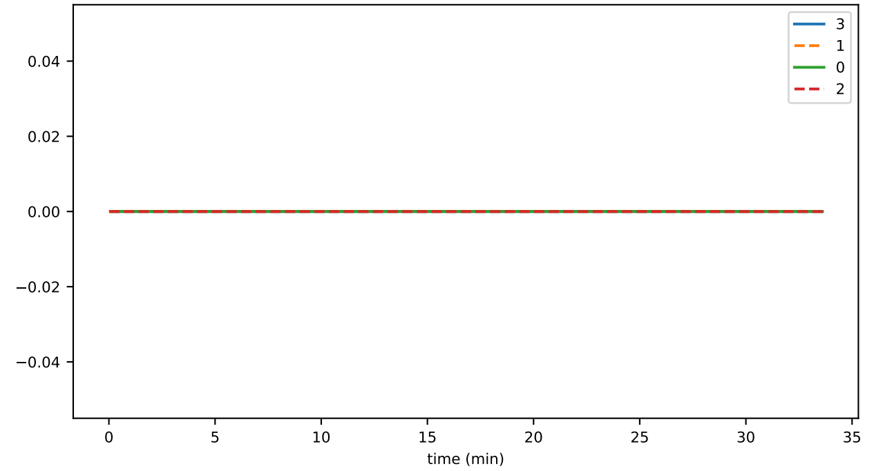
conn_connClose_connectionError
