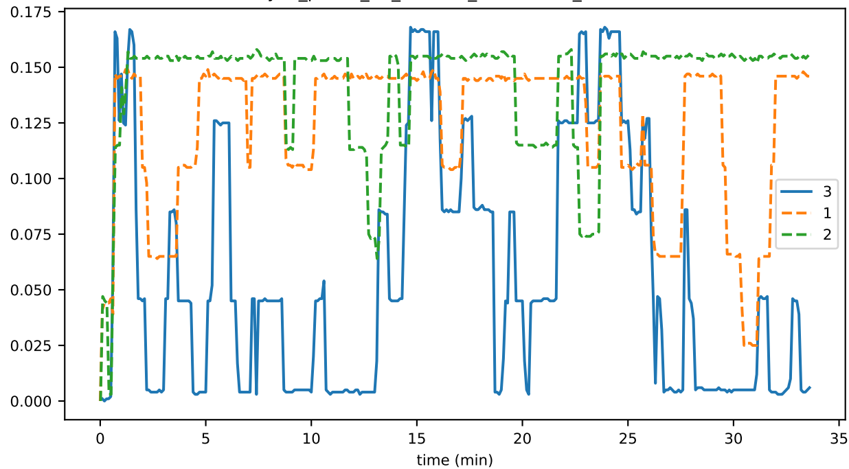
sync_phase_00_fraction_RECEIVING_EVENTS
