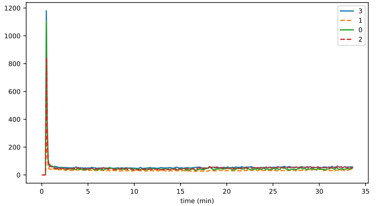
eventDelay_1_hashing_gossip
