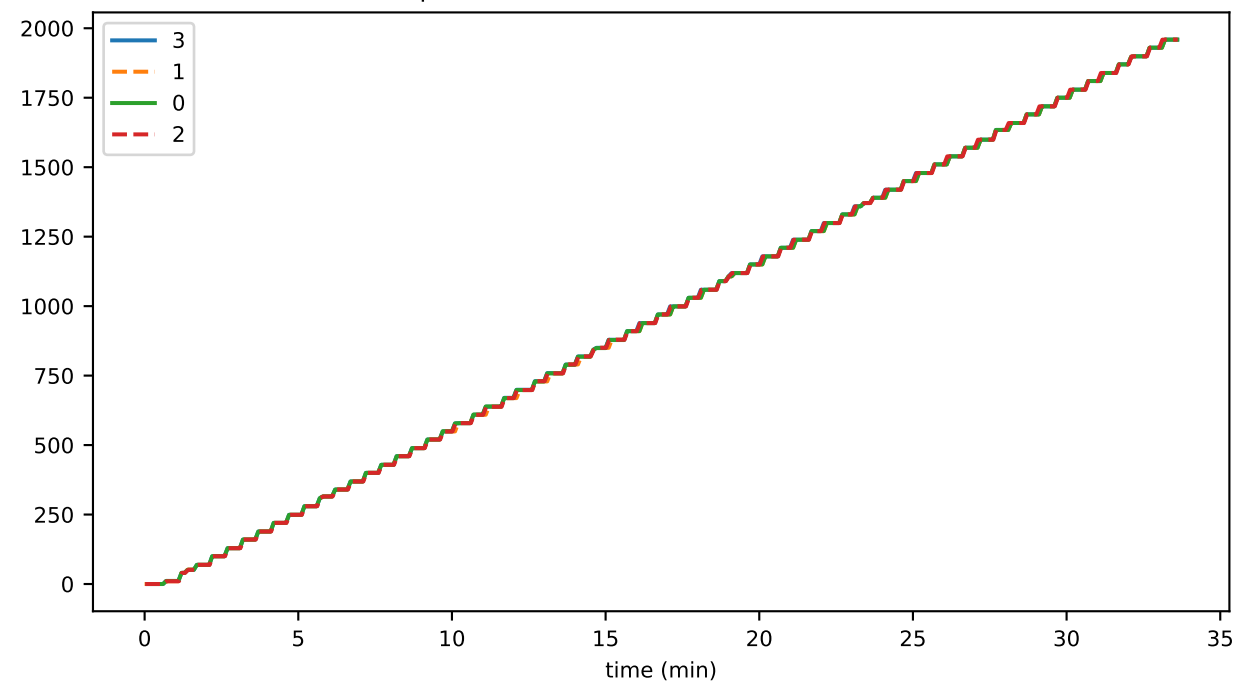
preconsensusEventFileOldestSeconds
