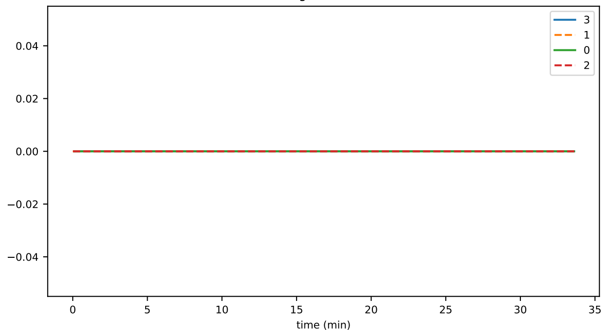
directMemPercent
