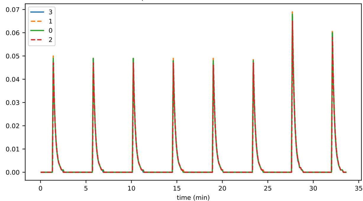
preconsensusEventFileYoungestIdentifier
