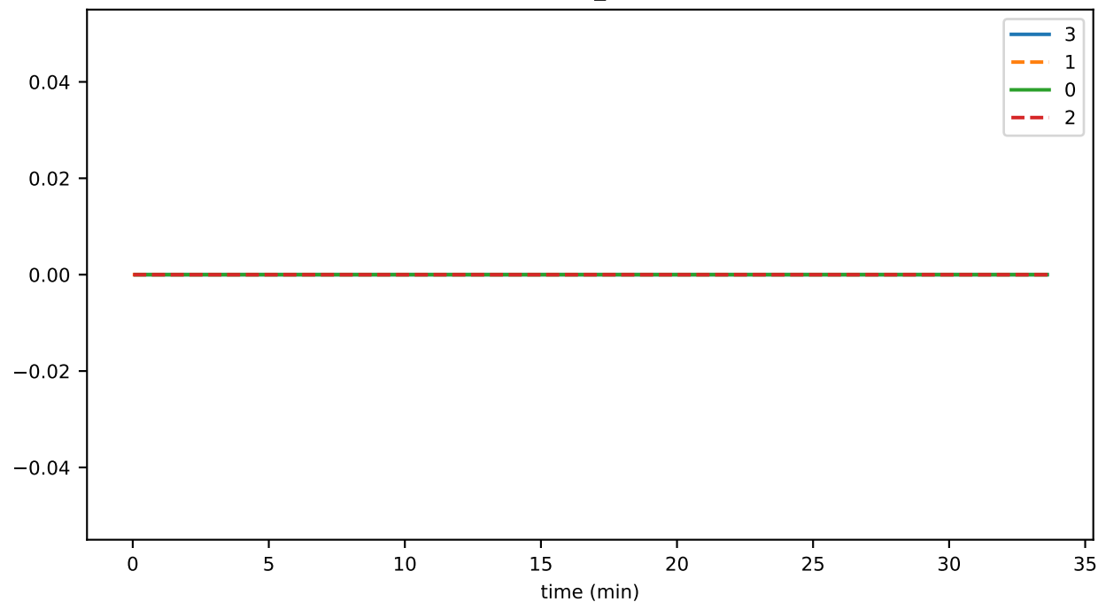
rejectedAppTransactions
