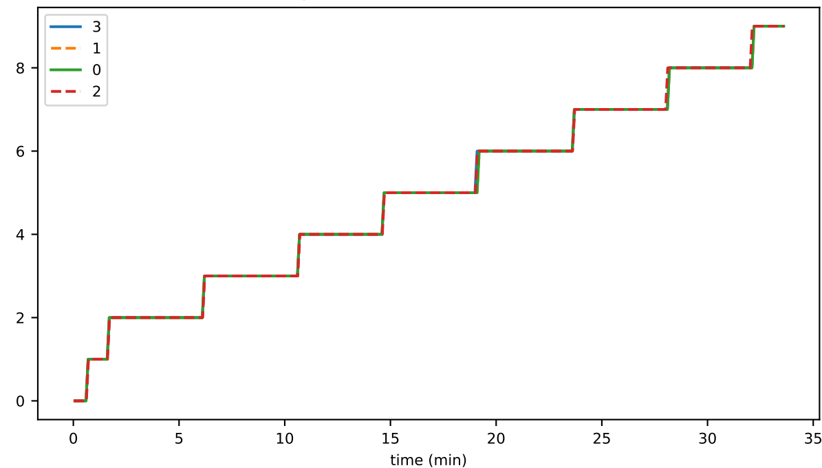
preconsensusEventFileOldestSeconds
