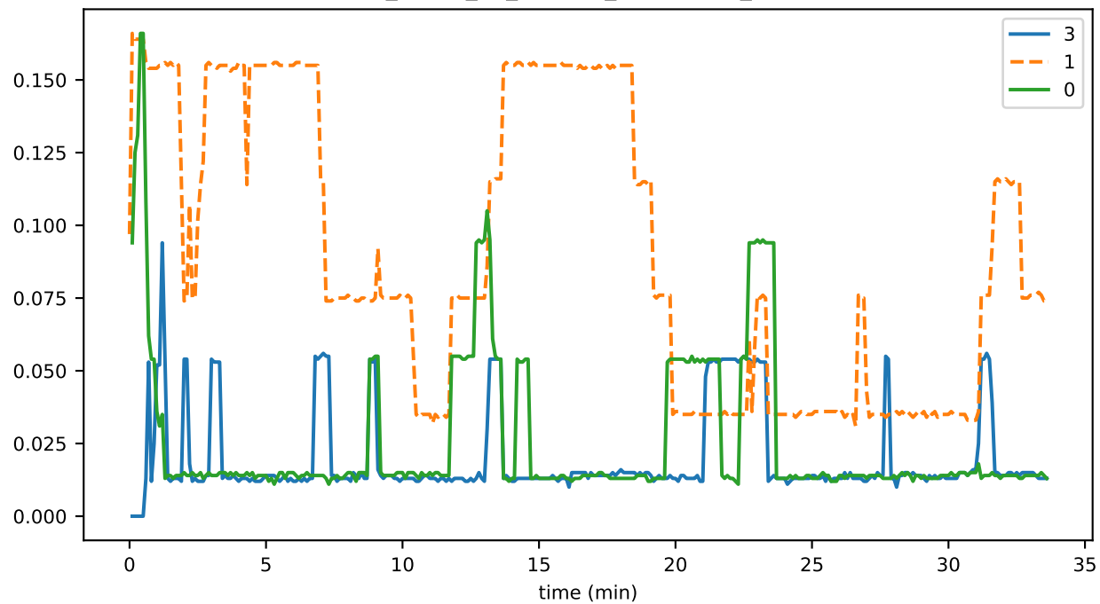
sync_phase_02_fraction_RECEIVING_EVENTS
