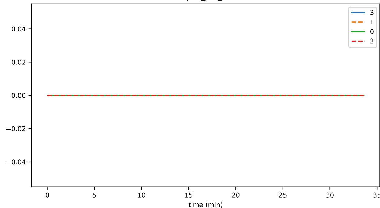
endsReconnectAsReceiver
