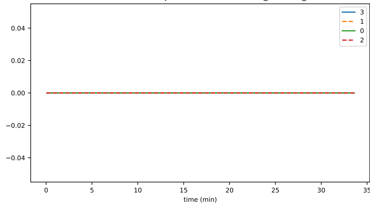
SmartContractService:SystemContractMethodCall_ALIASES_failed
