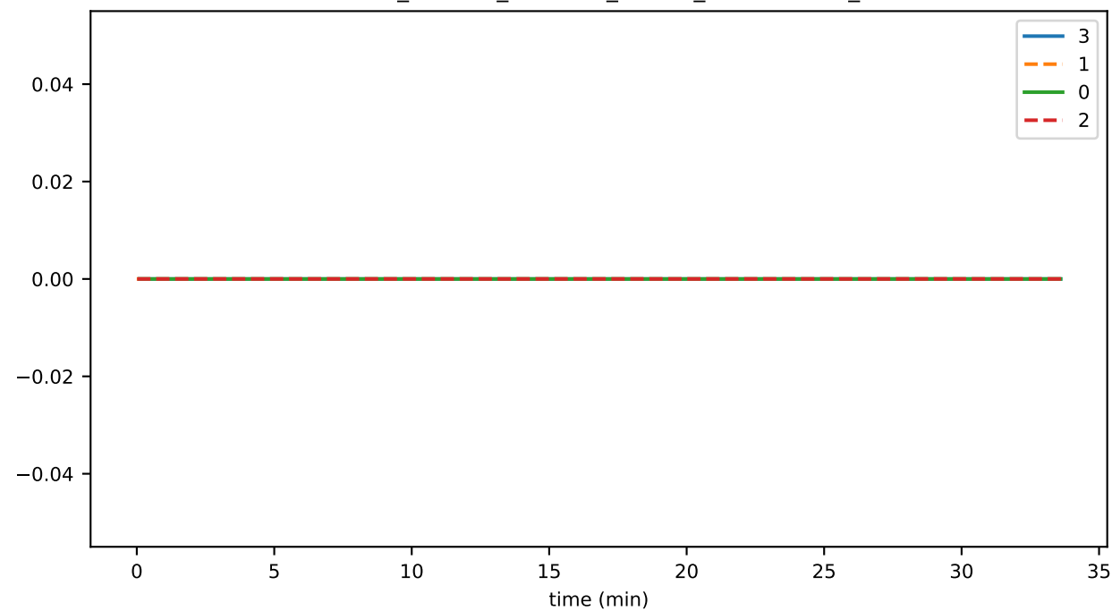
consensus_fraction_SETTING_EVENT_CONSENSUS_DATA
