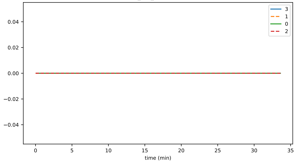
ev_per_syncRMAX
