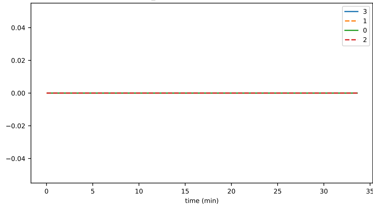
conn_headerProducedToAckLatency
