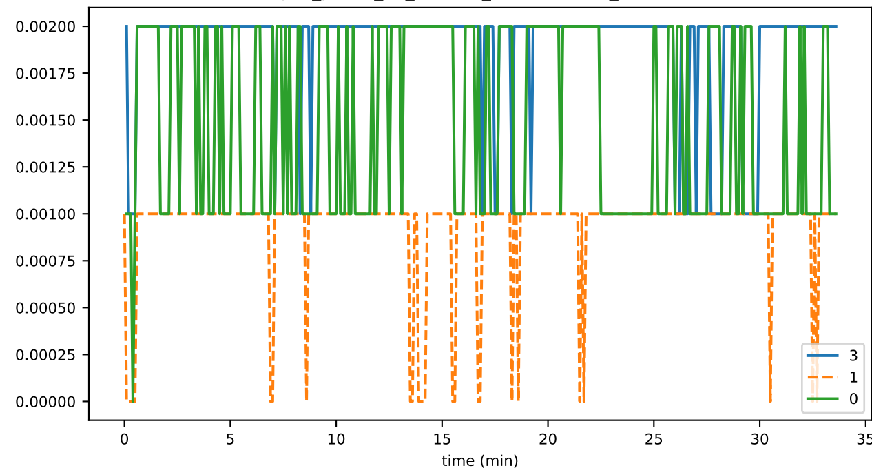
sync_phase_02_fraction_EXCHANGING_WINDOWS
