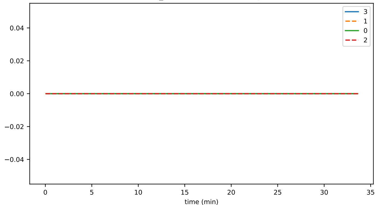
conn_closed
