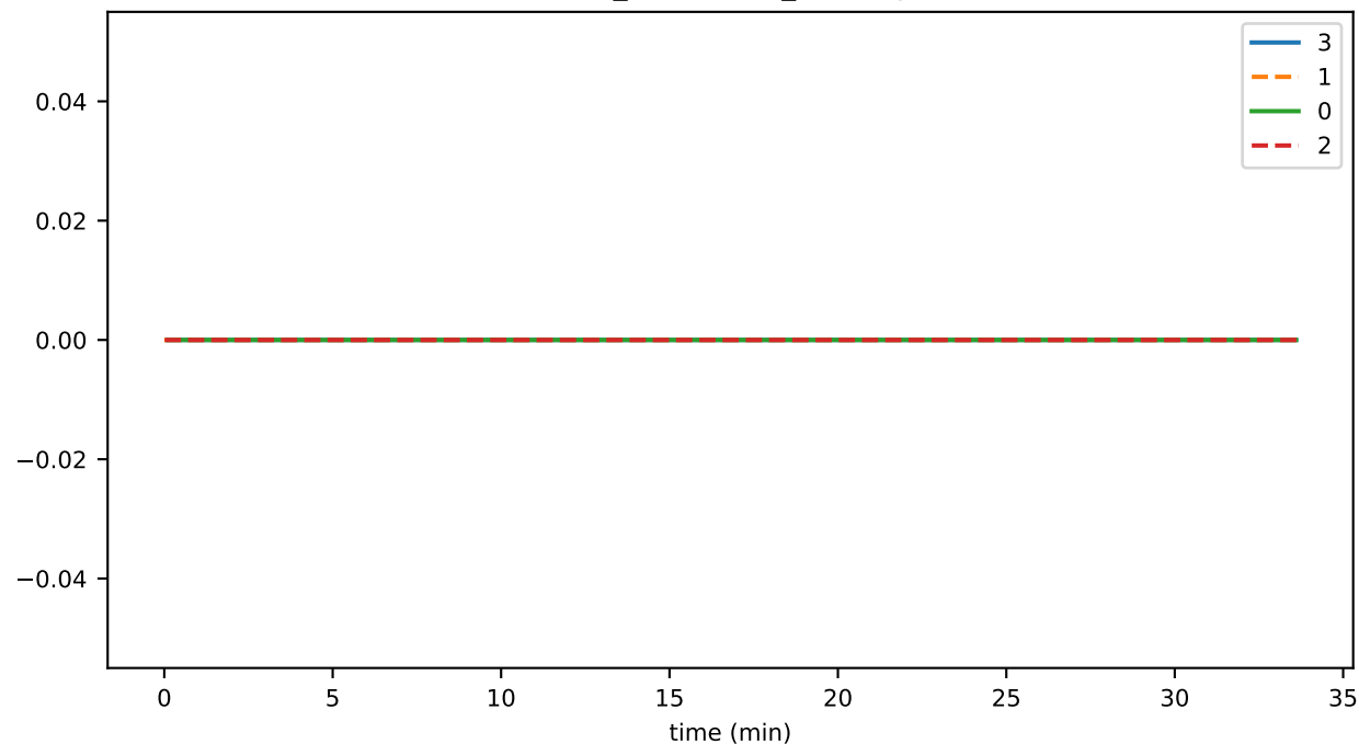
connSend_latestBlockEndOfBlock
