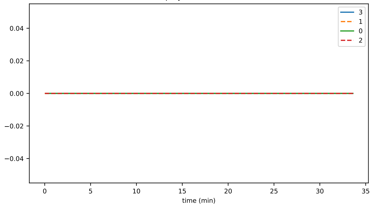
hapiFreeQueryLimitsPercentUsed
