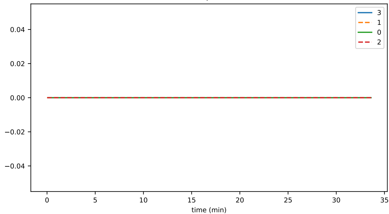
airdropsUsed
