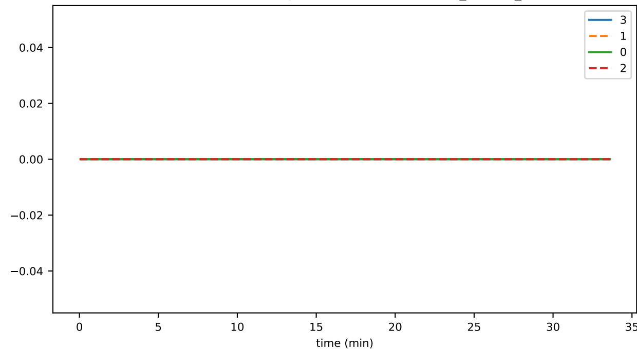
SmartContractService:SystemContractMethodCall_ERC20_failed
