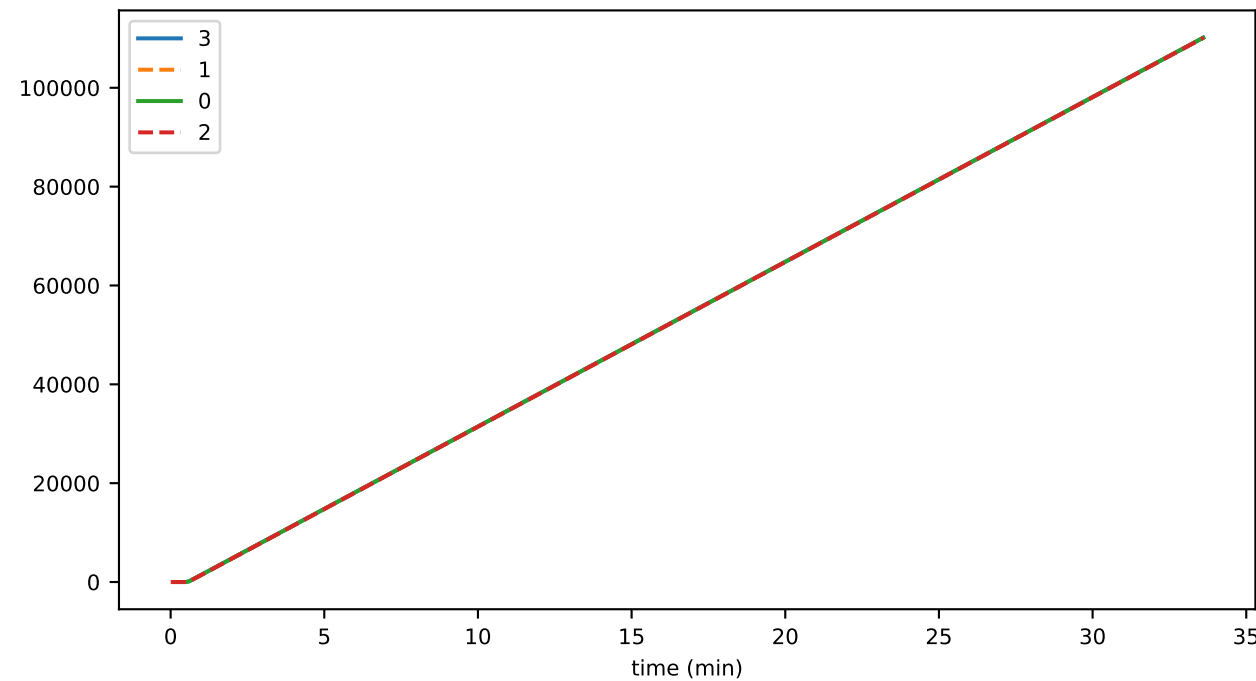
roundIncEqParents
