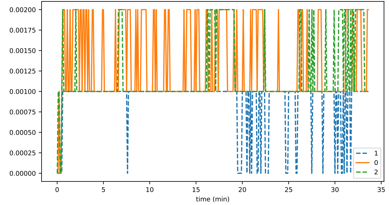
sync_phase_03_fraction_EXCHANGING_WINDOWS
