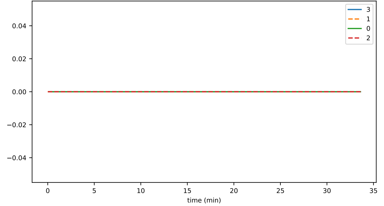
Dig_per_sec
