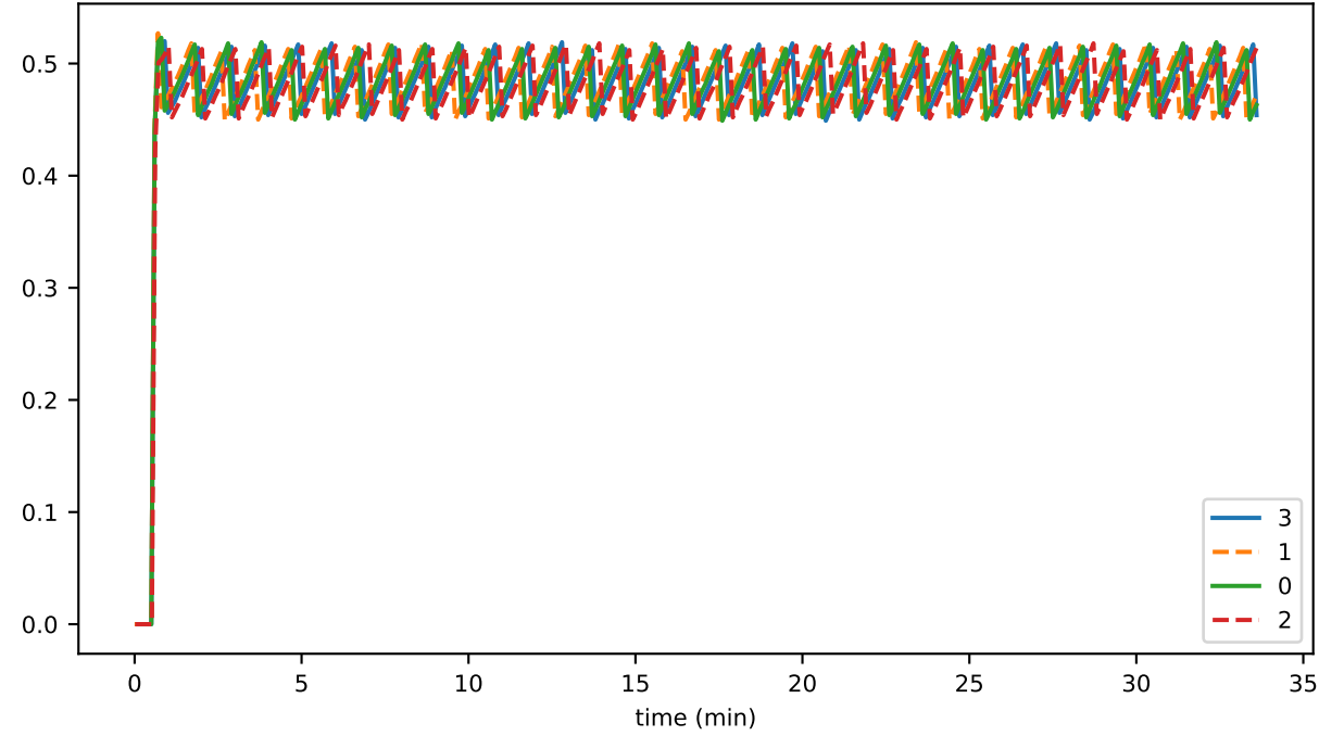
submittedPlatformTransactions
