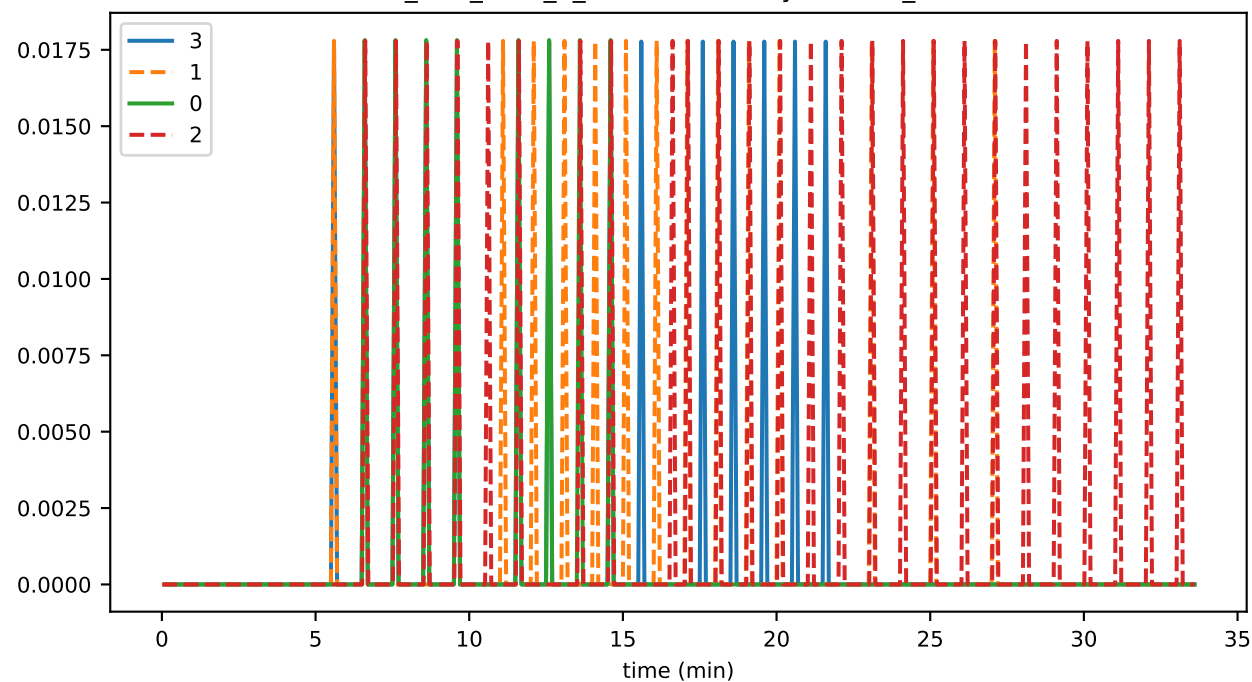
ds_files_level_2_leafKeysFileSizeByLevelMb_state
