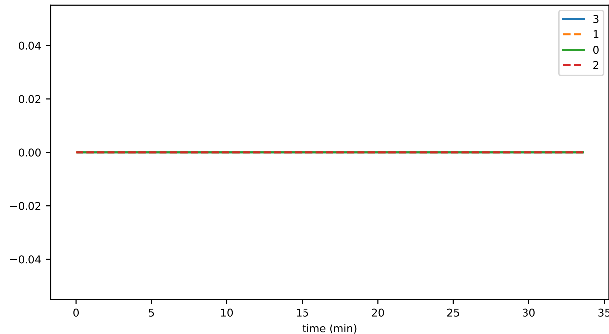
SmartContractService:SystemContractMethodCall_TRANSFER_failed
