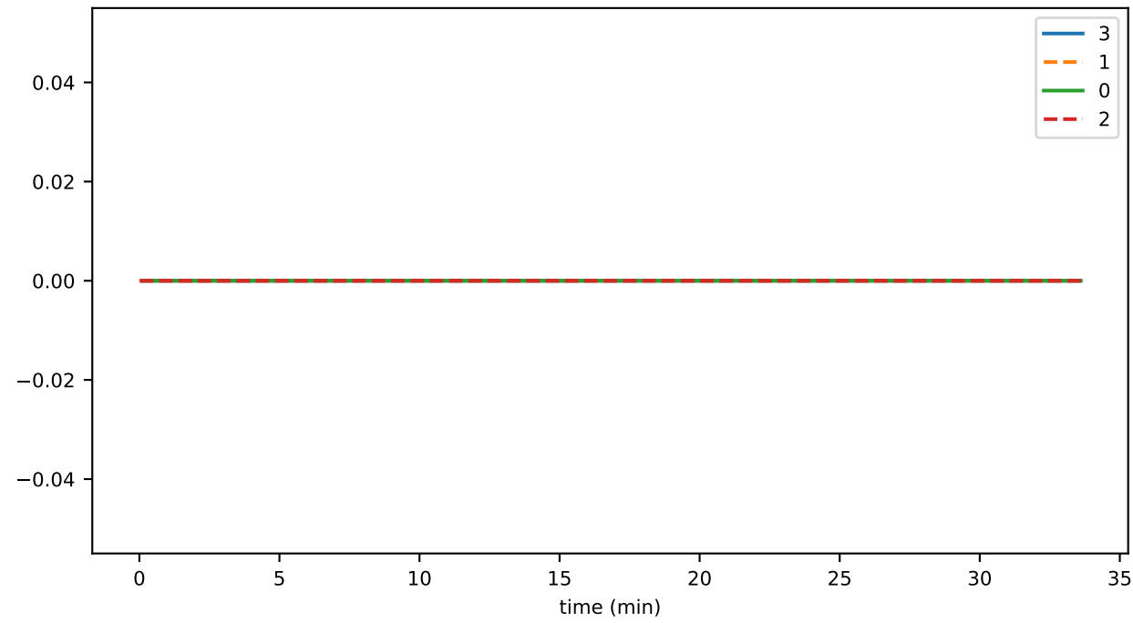
branchingEvents
