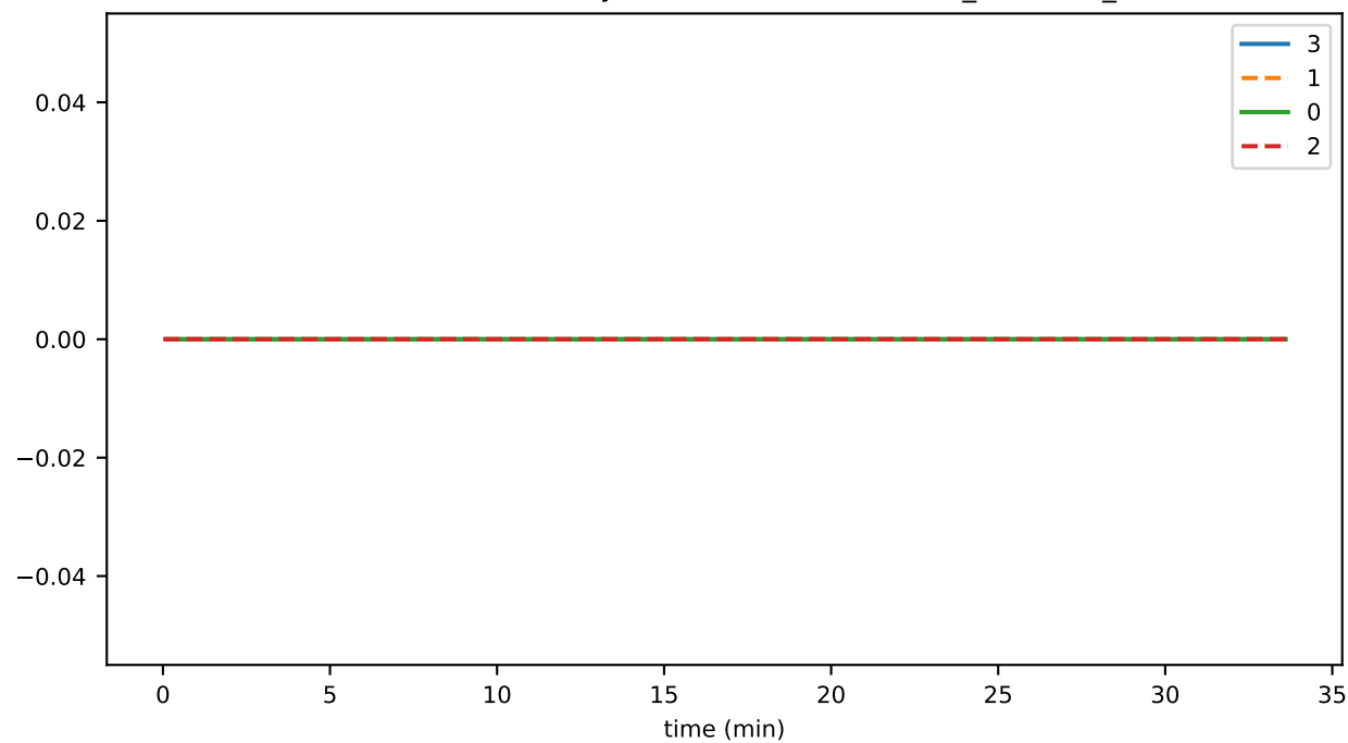
SmartContractService:SystemContractMethodCall_AIRDROP_total
