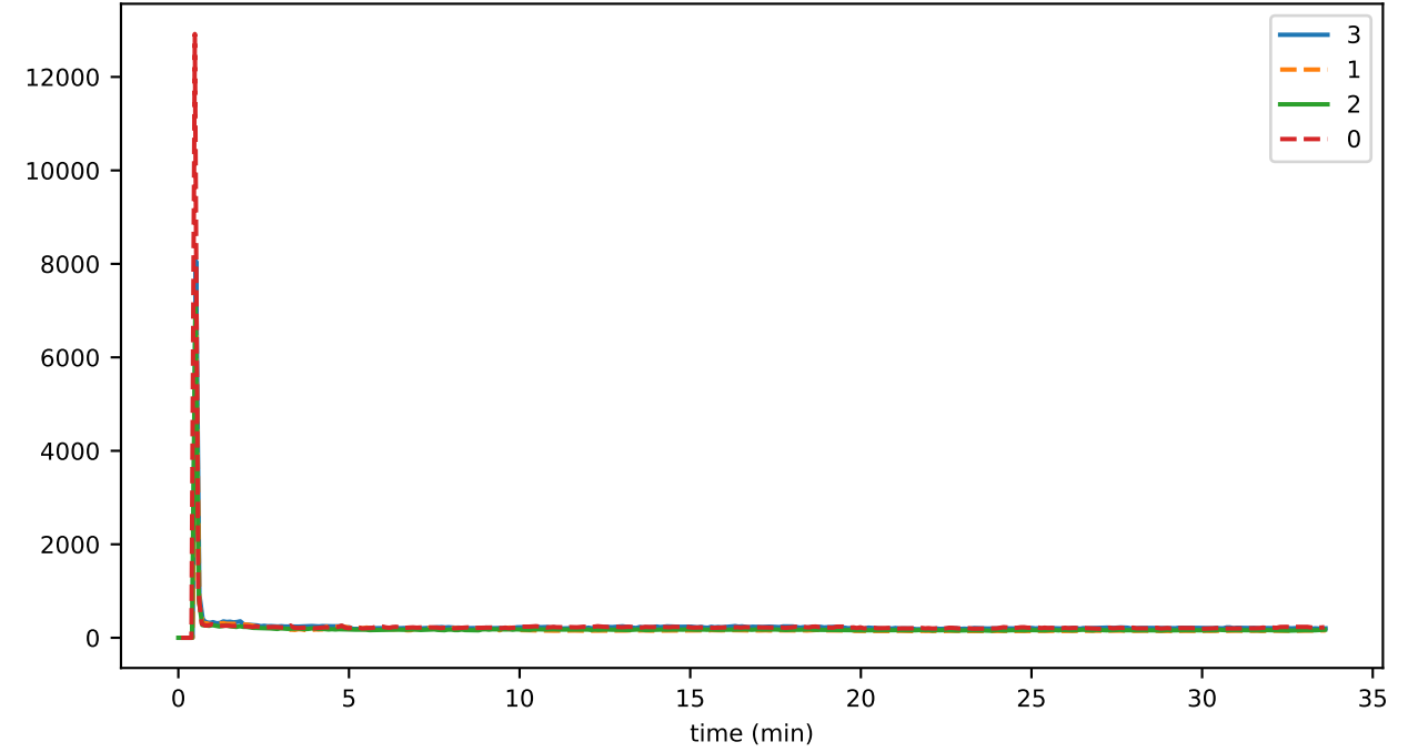
eventDelay_4_verification_gossip
