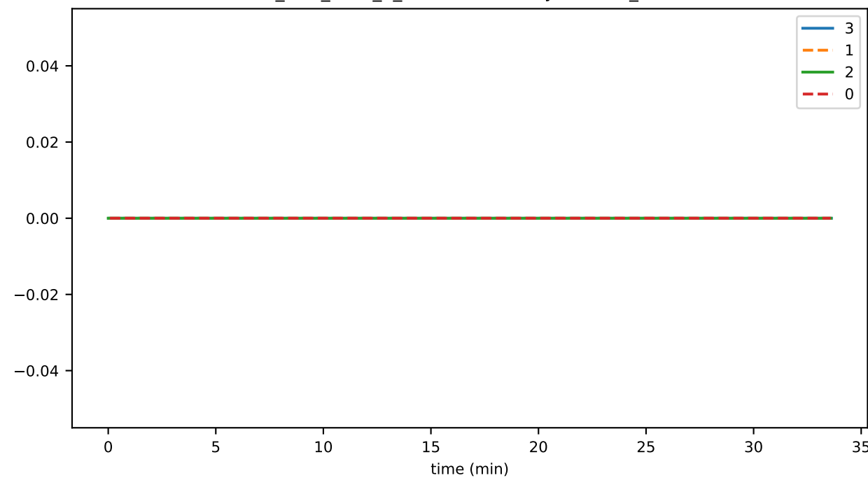
ds_files_level_8_hashesFileSizeByLevelMb_state
