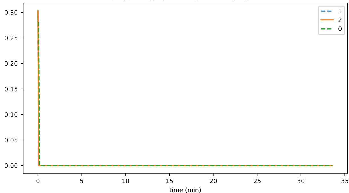
sync_phase_03_fraction_RECEIVING_EVENTS
