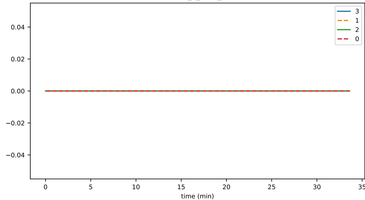
eventDelay_6_pces_storage
