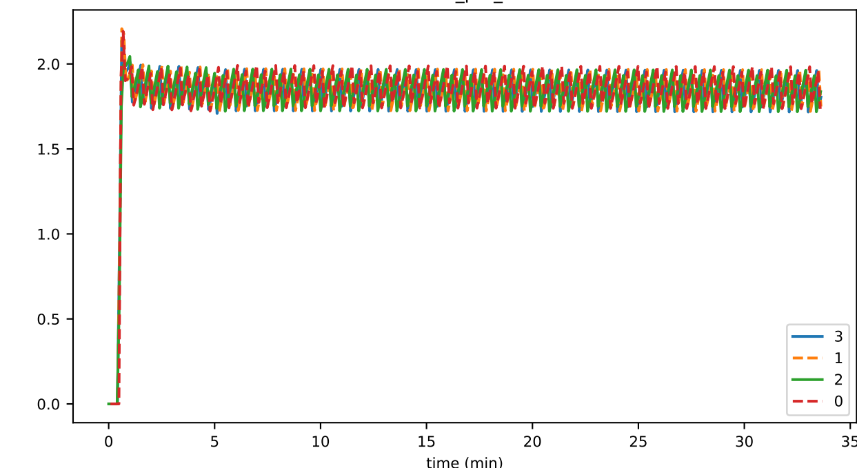
transH_per_sec
