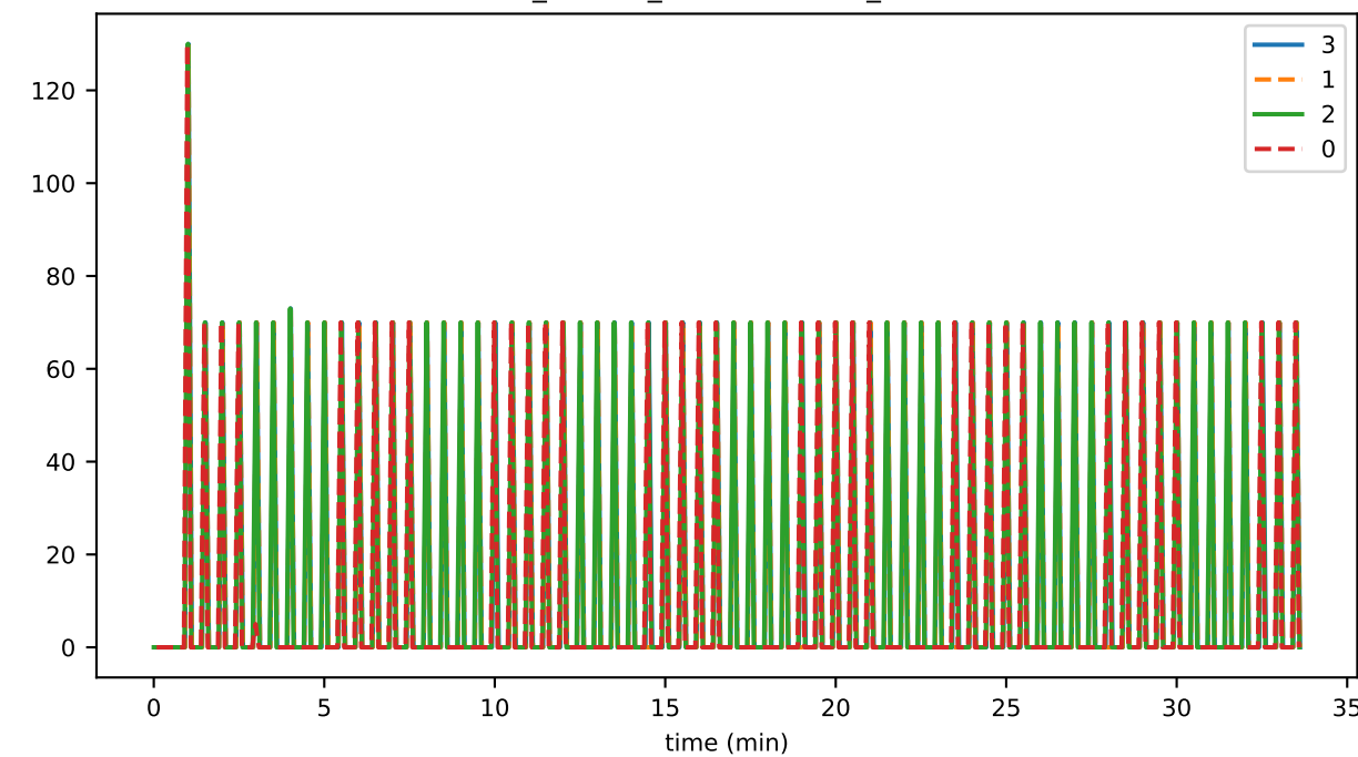
ds_flushes_hashesWritten_state
