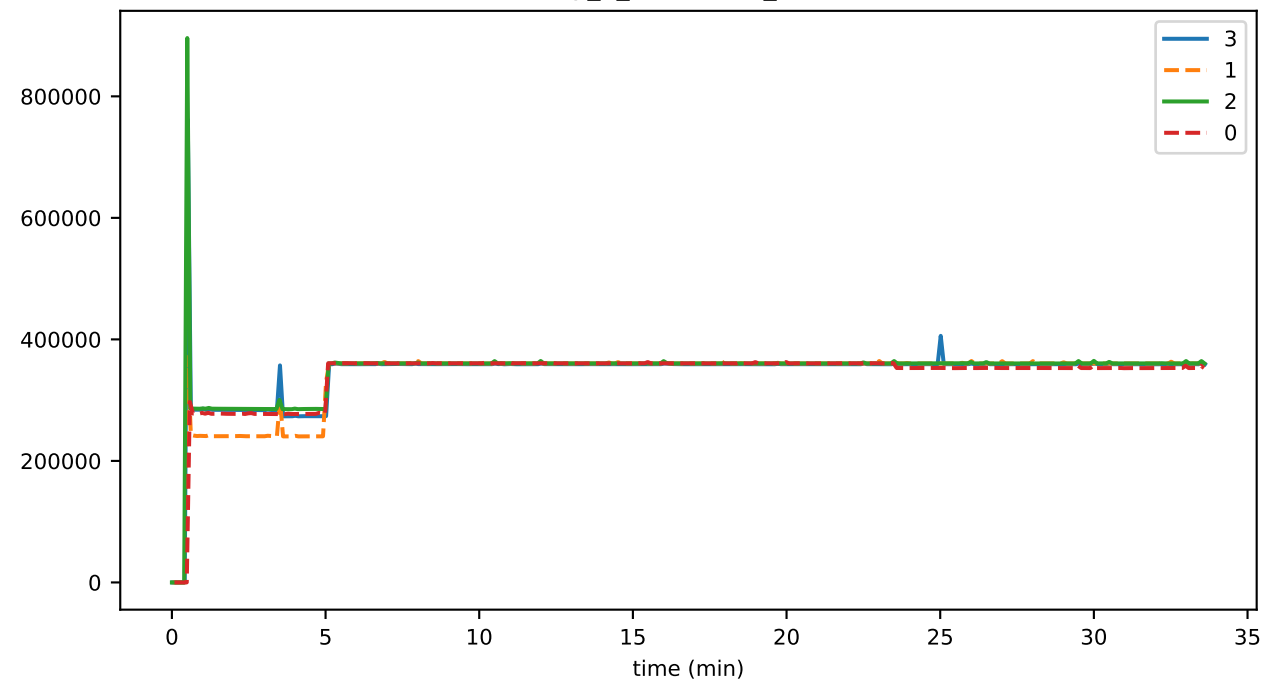
eventDelay_7_consensus_storageMAX
