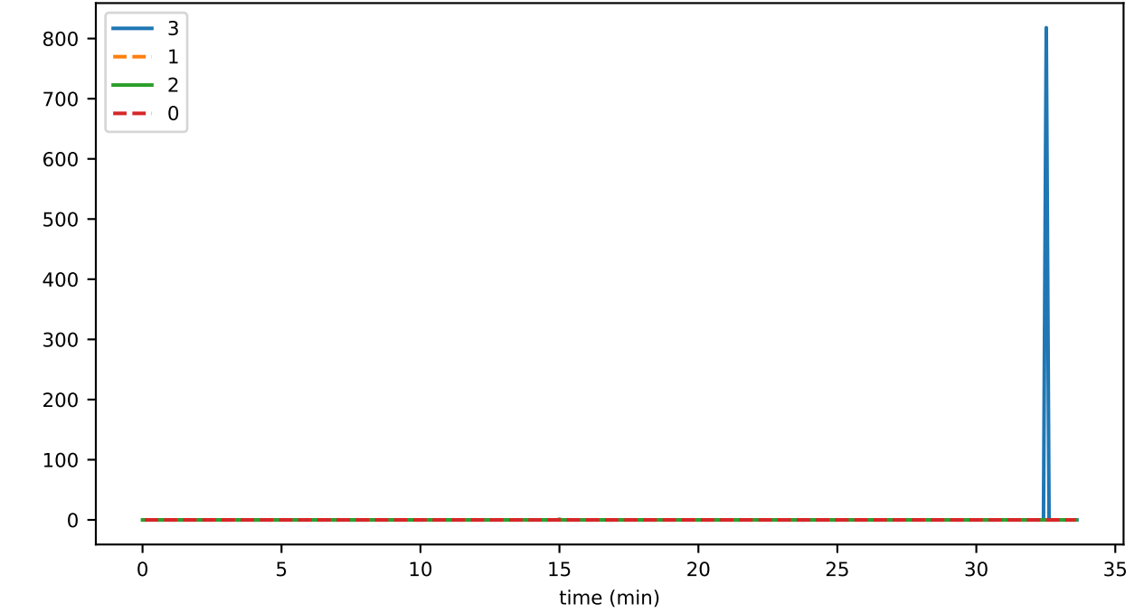
ds_compactions_level_2_leavesTimeMs_state
