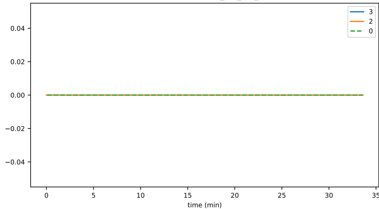
reconnectRejections_per_sec_01
