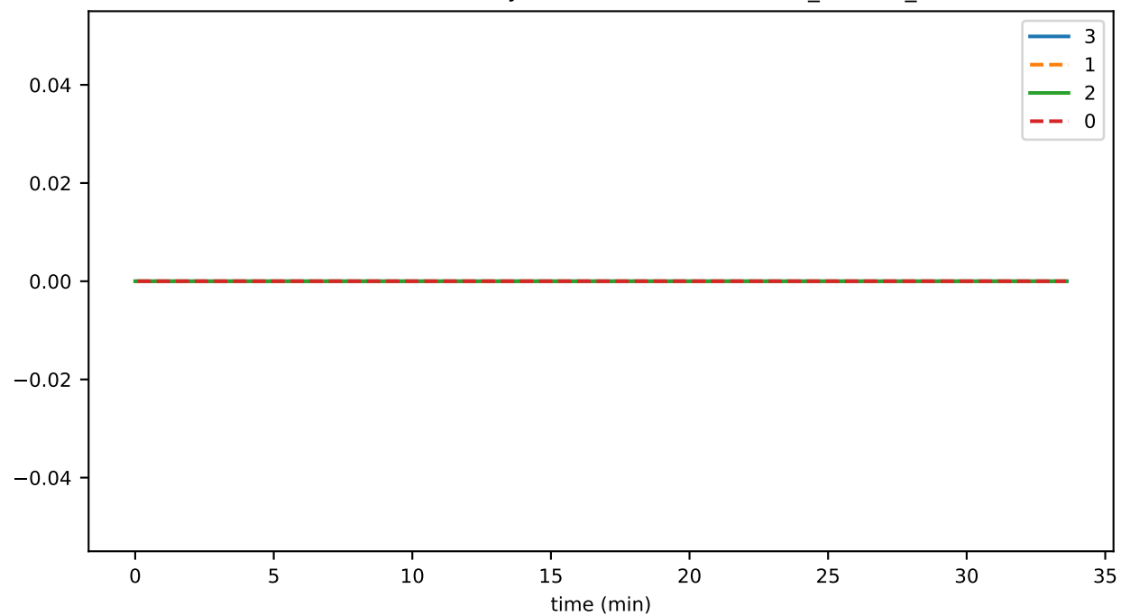
SmartContractService:SystemContractMethodCall_DIRECT_total
