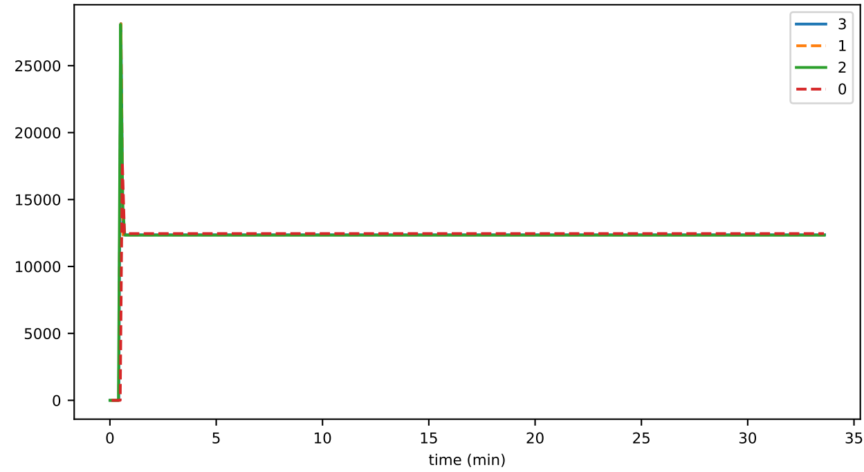
buffer_latestBlockAcked
