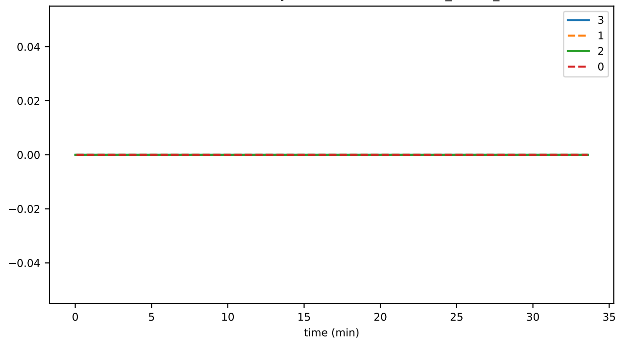
SmartContractService:SystemContractMethodCall_ERC20_failed
