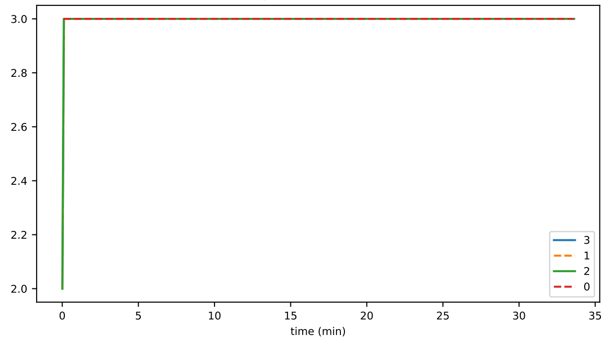
syncs_in_progress
