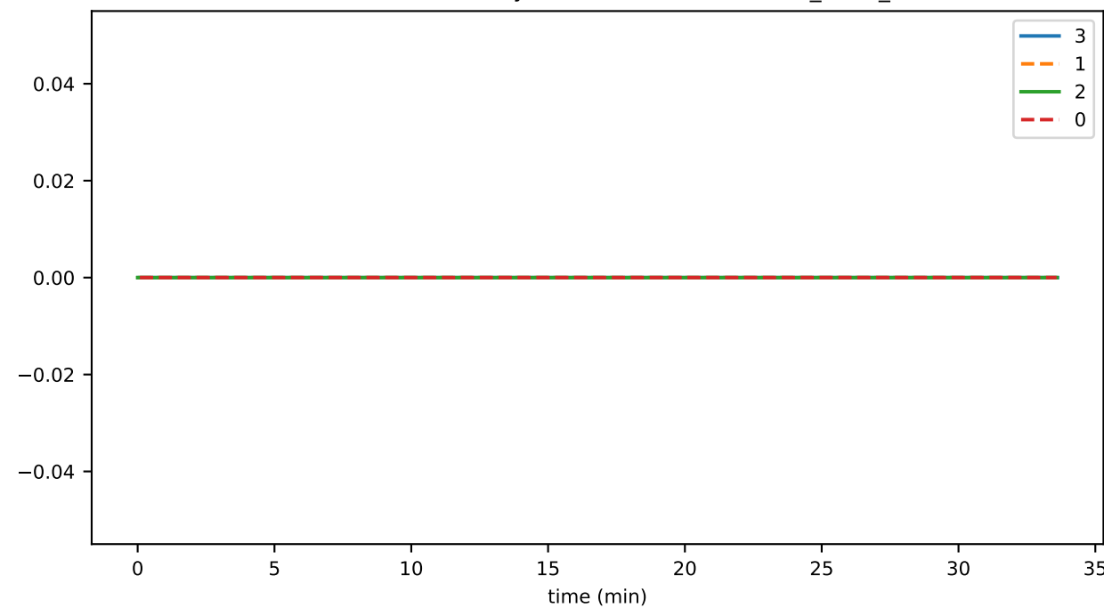
SmartContractService:SystemContractMethodCall_WIPE_failed
