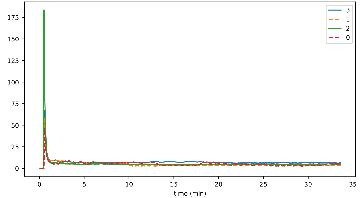
eventDelay_1_hashing_gossip
