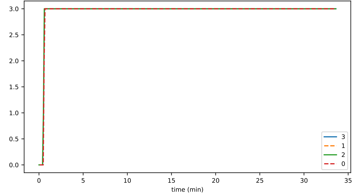
buffer_latestBlockOpened
