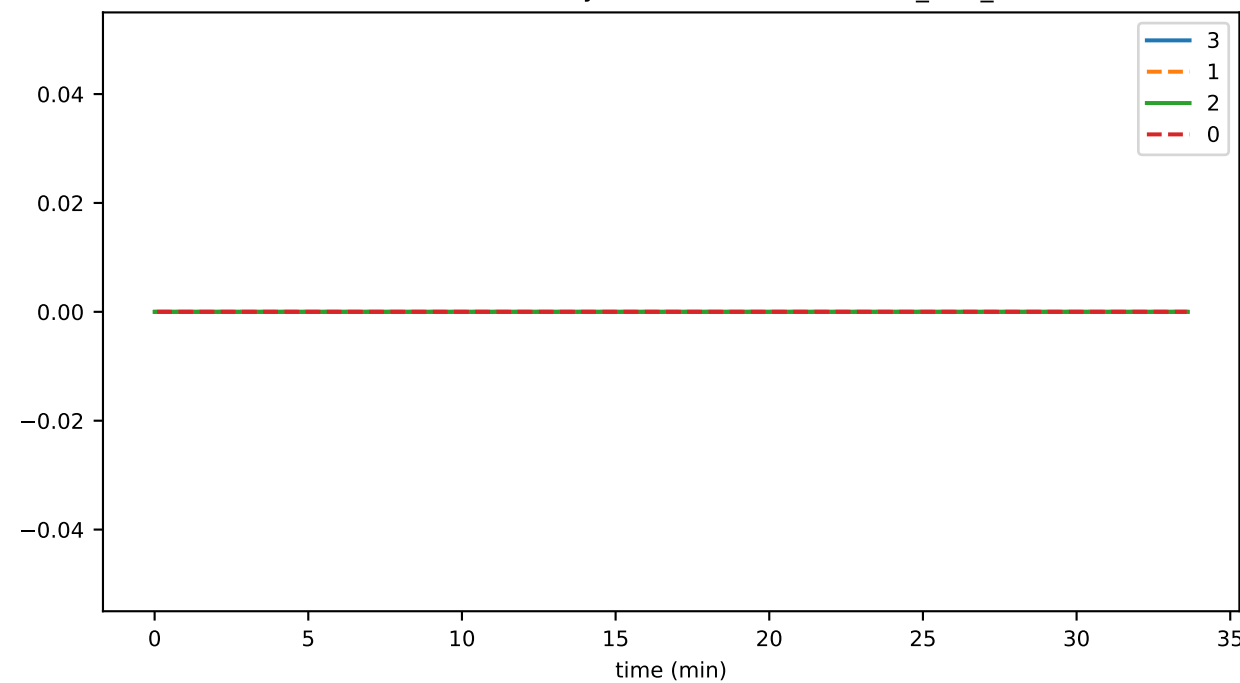
SmartContractService:SystemContractMethodCall_HSS_failed
