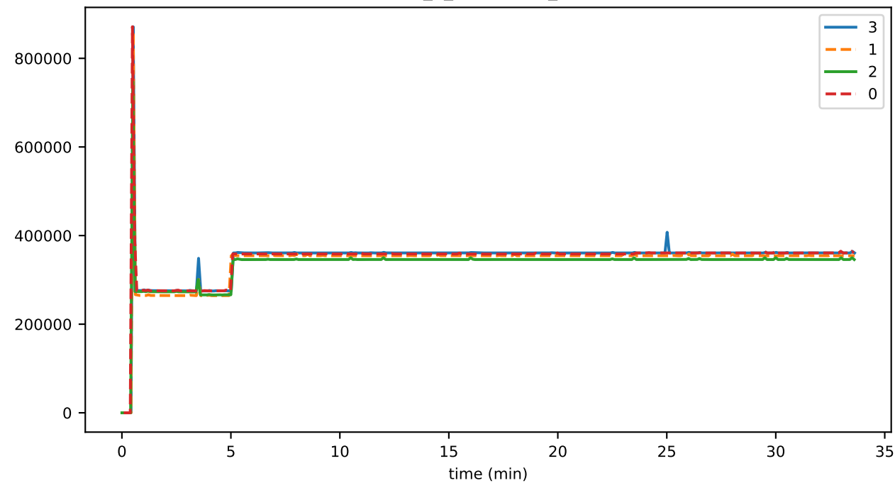
eventDelay_7_consensus_gossipMAX
