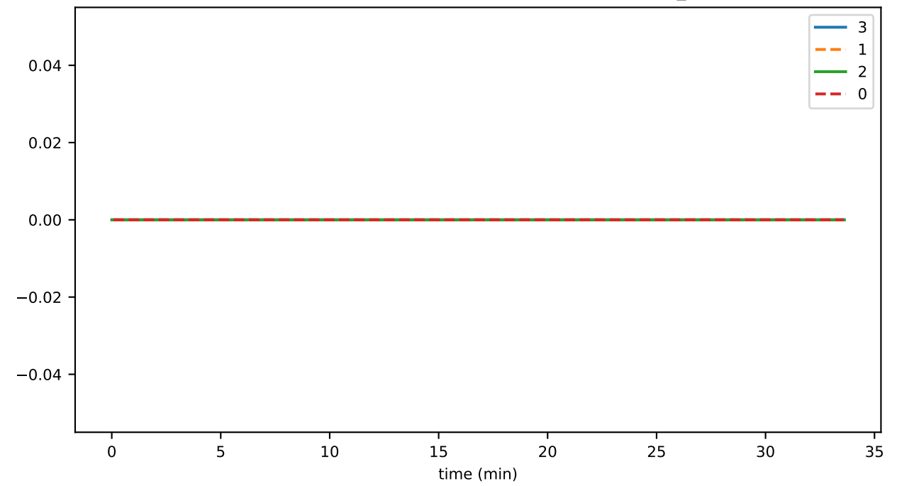
SmartContractService:FailedTransactionDuration_avg
