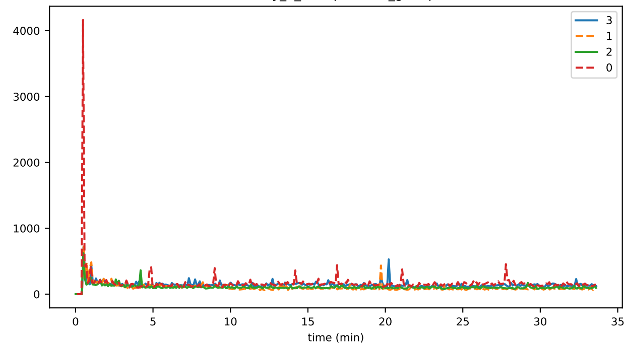
eventDelay_3_deduplication_gossipMAX
