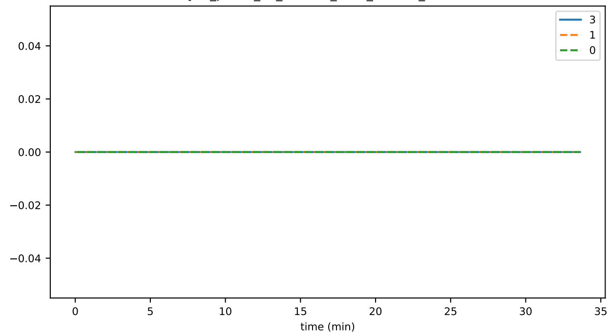
sync_phase_02_fraction_SELF_FALLEN_BEHIND
