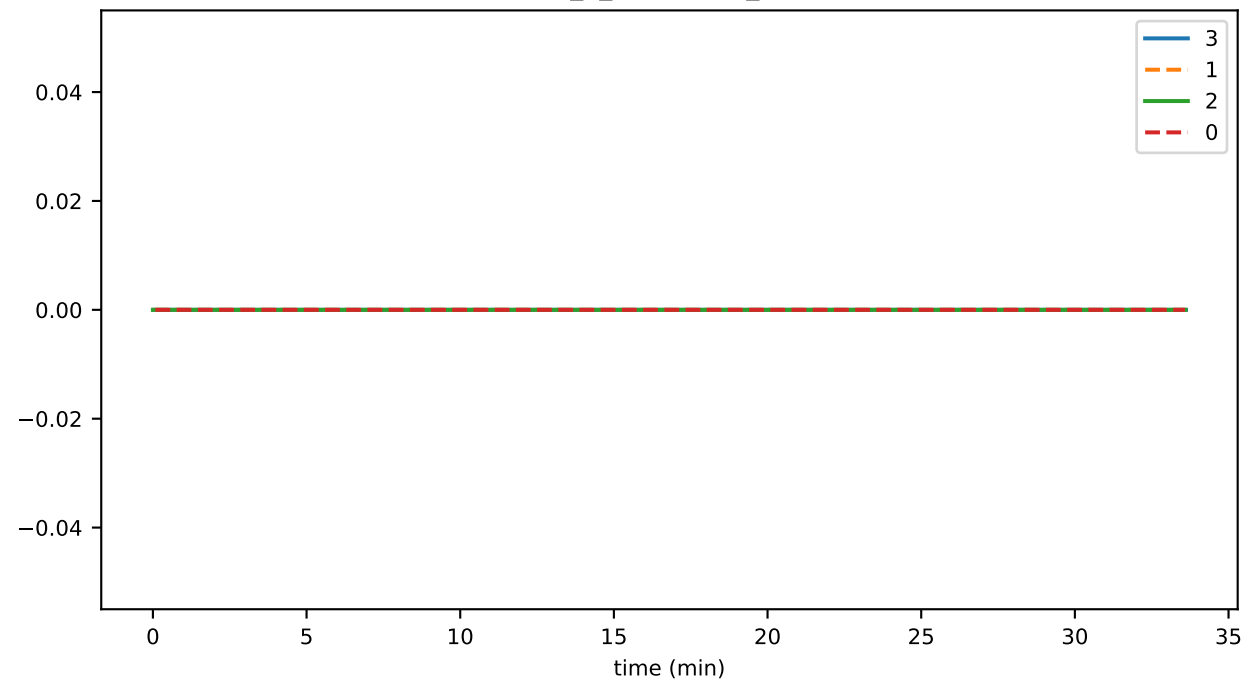
eventDelay_7_consensus_storageMAX
