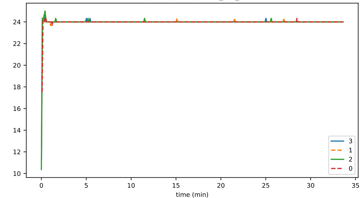
accountsPercentUsed
