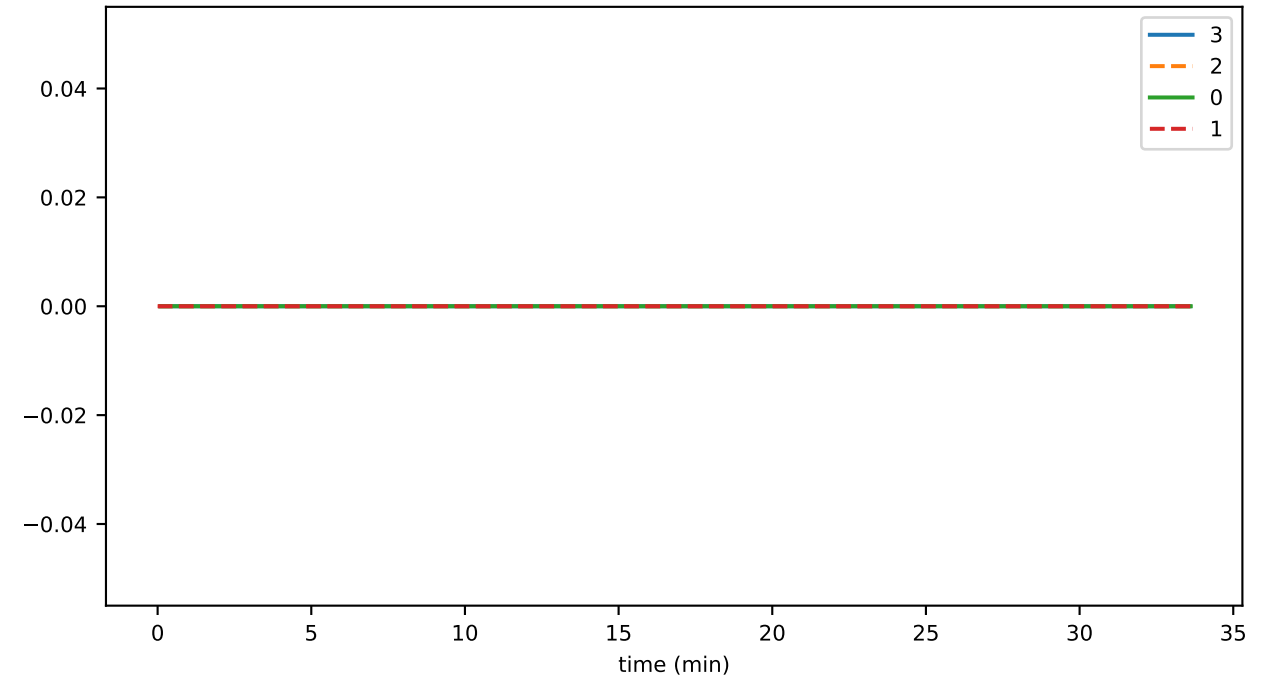
eventCreation_fraction_QUIESCENCE
