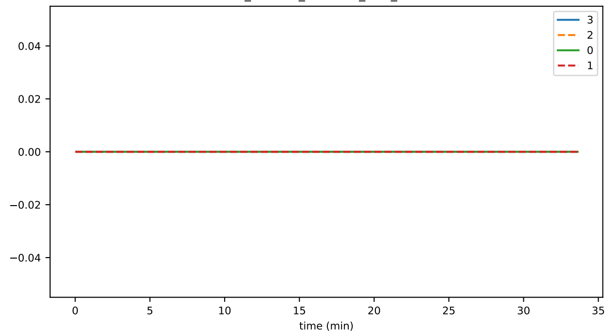
consensus_time_GETTING_STATE_TO_SIGN
