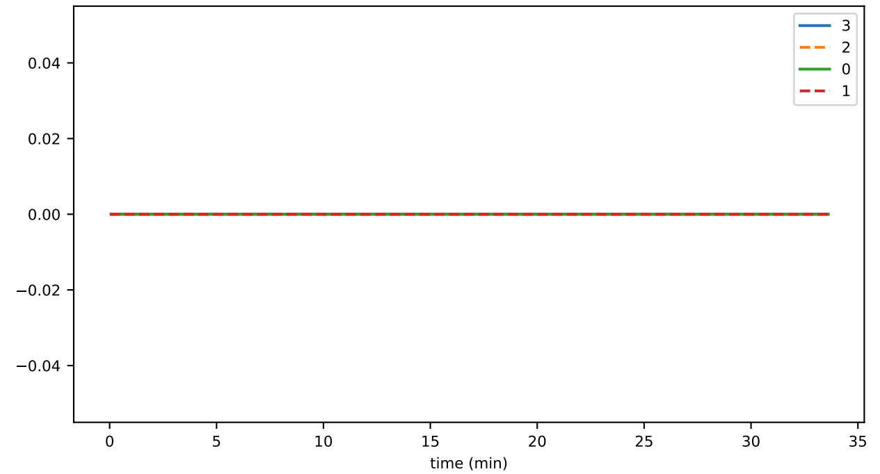
connRecv_endStream_invalidRequest
