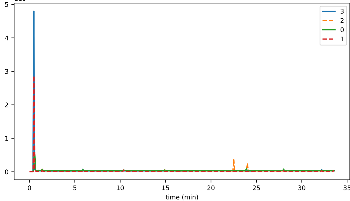
pcesAvgTotalWriteDuration
