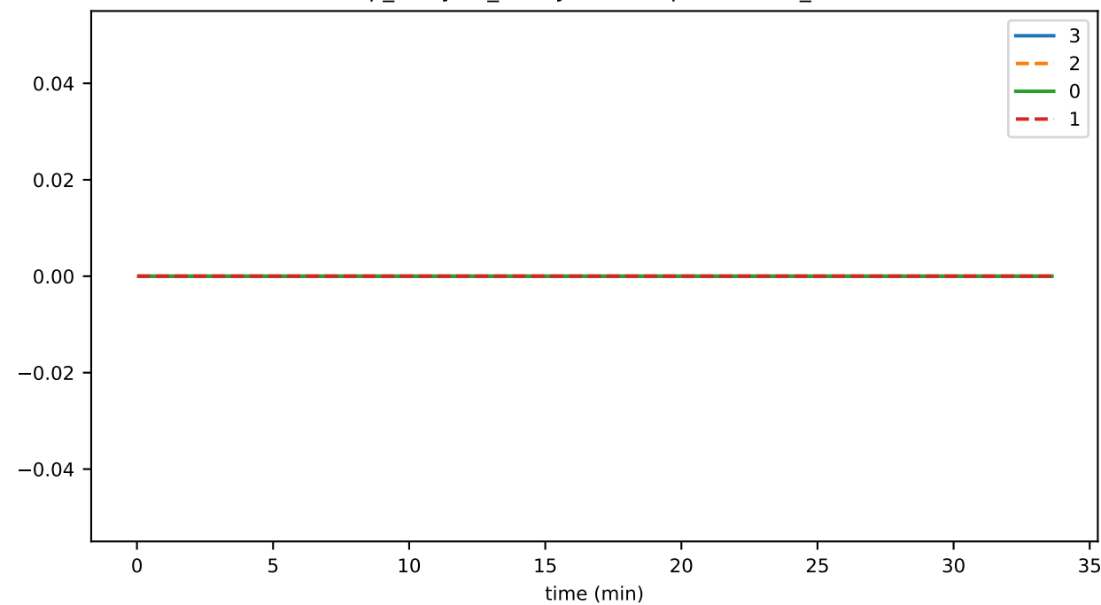
vmap_lifecycle_familySizeBackpressureMs_state
