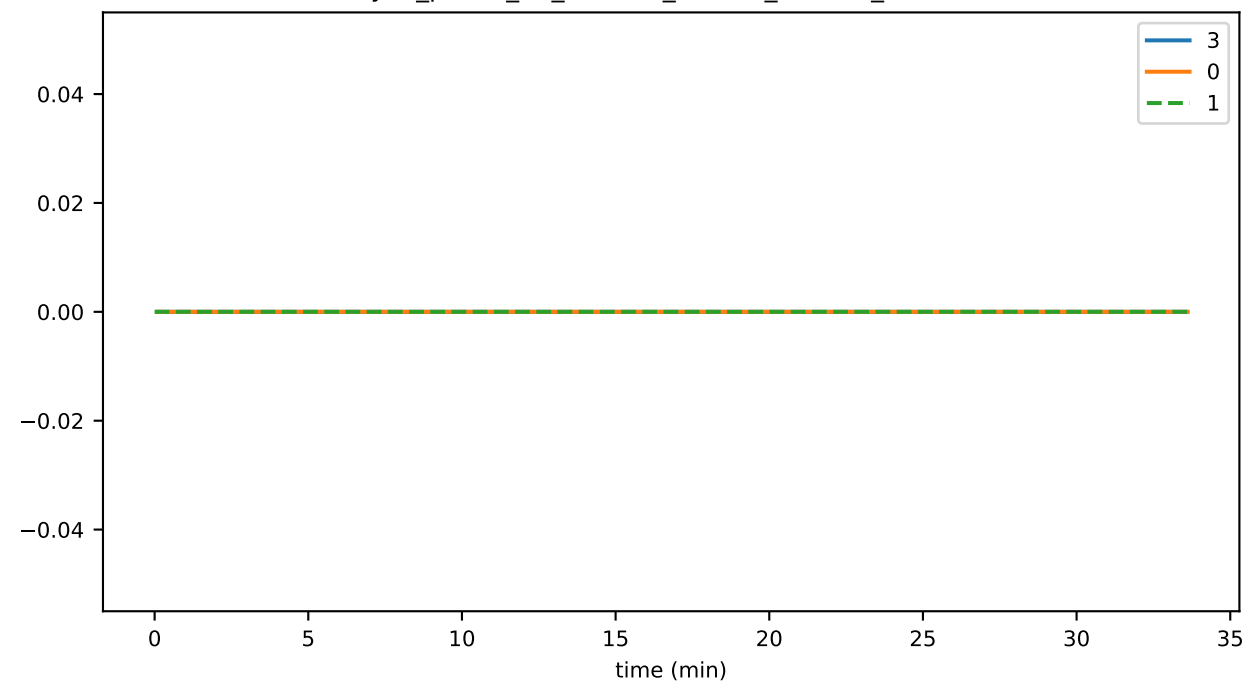
sync_phase_02_fraction_OTHER_FALLEN_BEHIND
