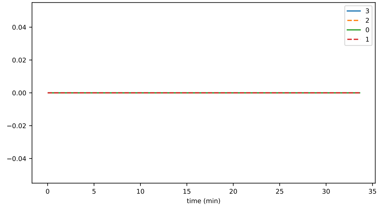
senderReconnectDurationSeconds
