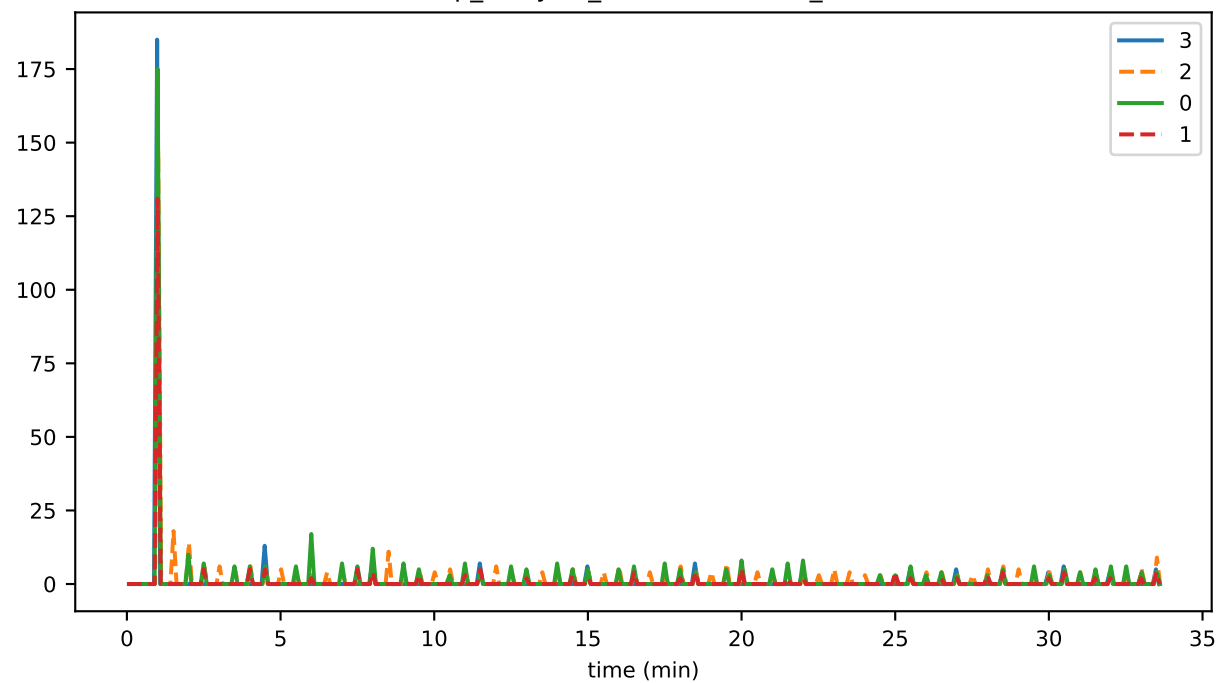
vmap_lifecycle_flushDurationMs_state
