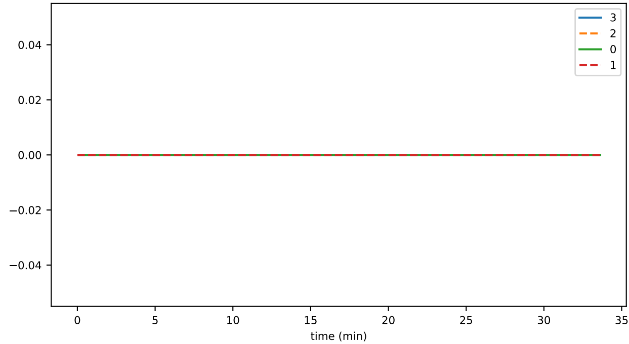
eventCreation_fraction_PLATFORM_STATUS
