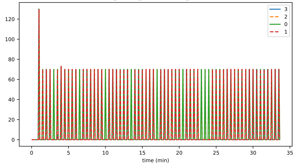
ds_flushes_hashesWritten_state
