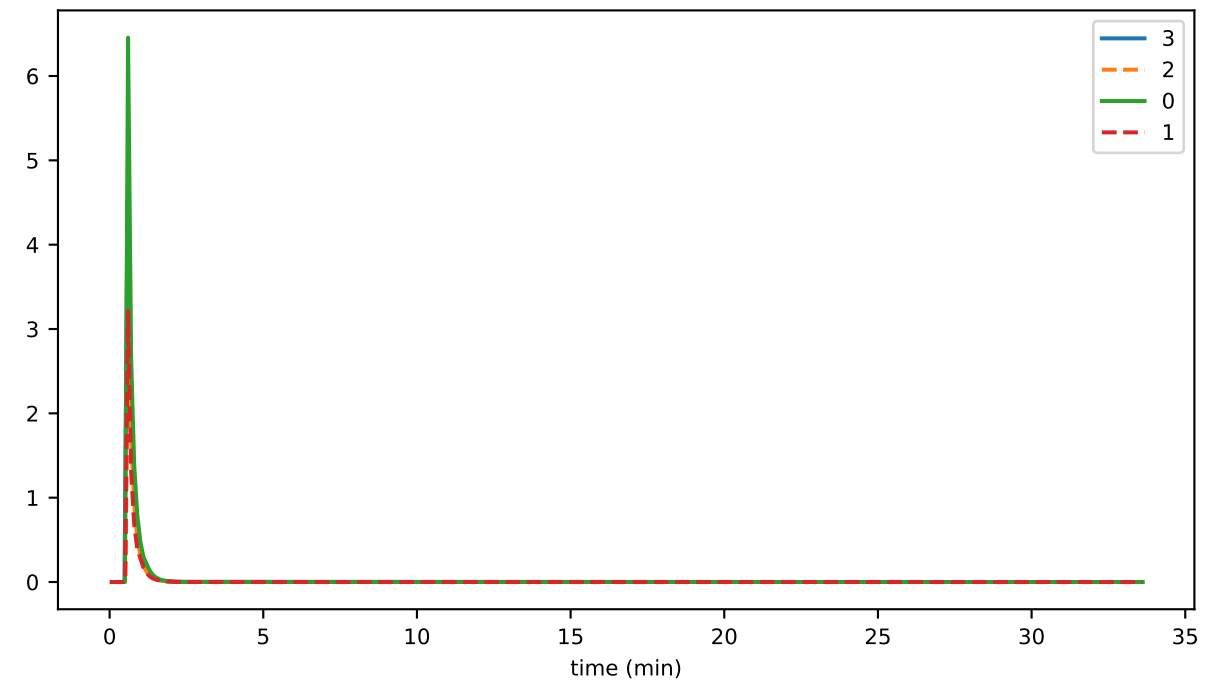
sigStateHash
