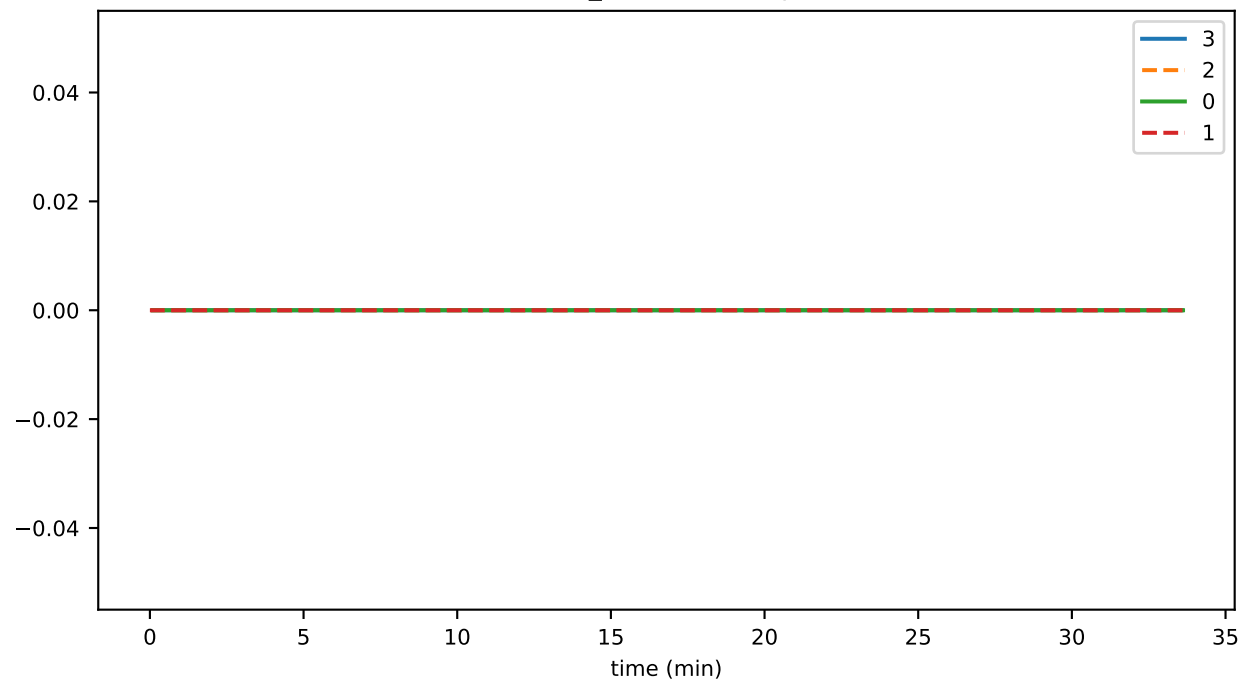
connRecv_resendBlock
