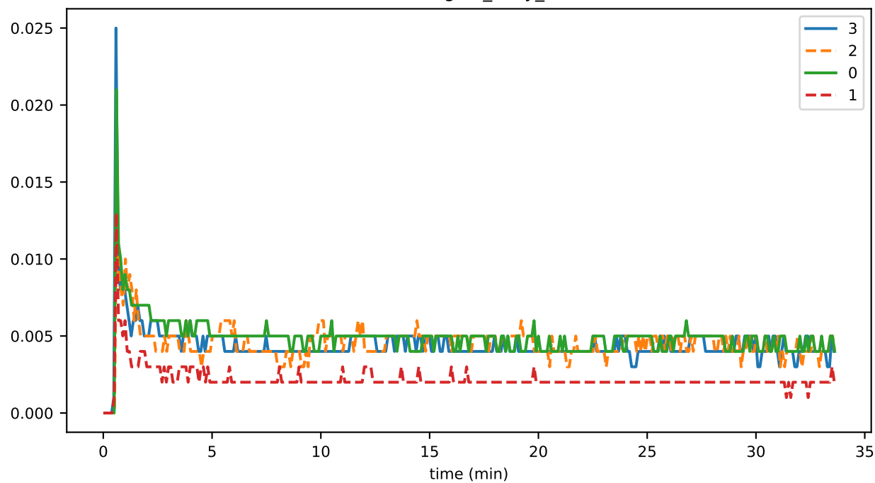
ConsensusEngine_busy_fraction
