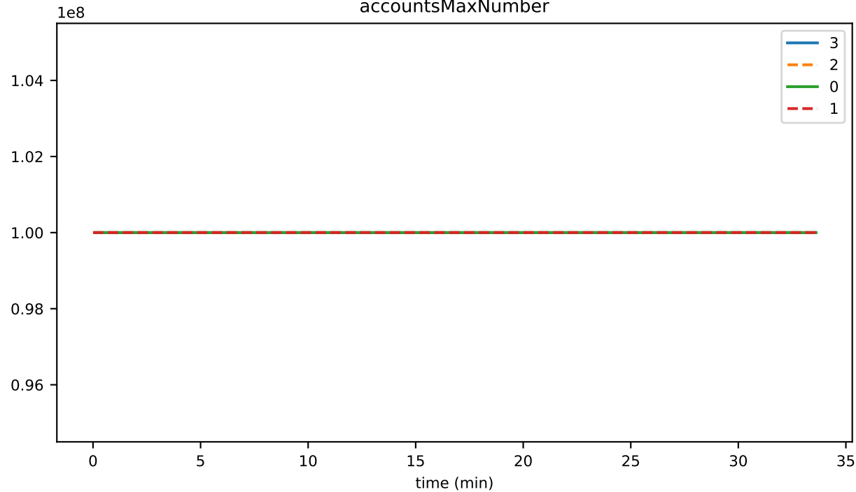
accountsMaxNumber
