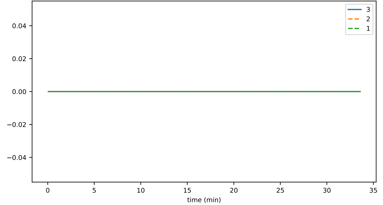
sync_phase_00_fraction_OTHER_FALLEN_BEHIND
