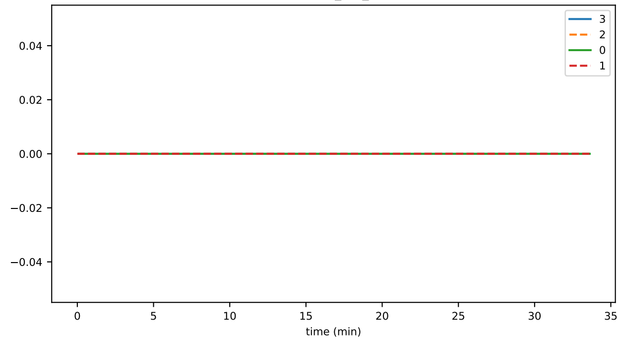
SigSpans_per_sec
