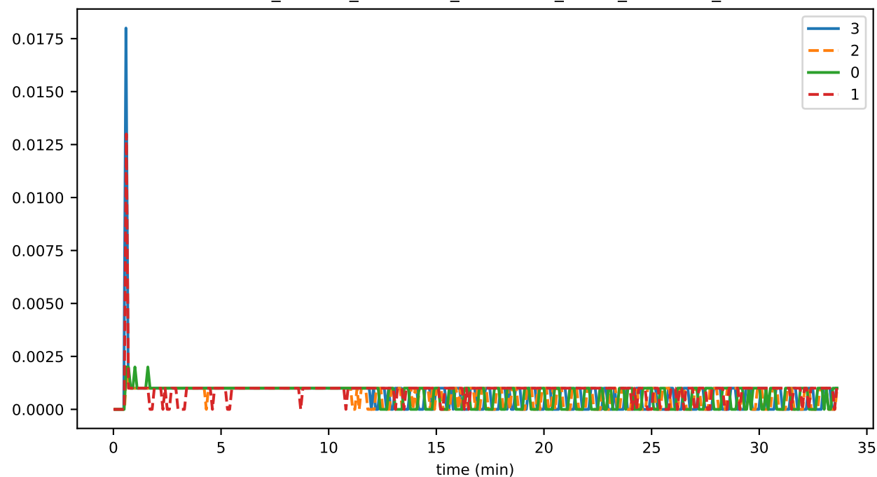
consensus_time_CREATING_SIGNED_STATE
