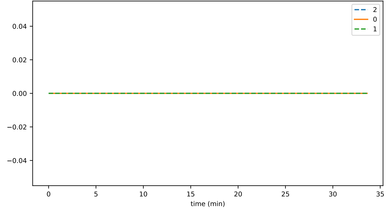
sync_phase_03_fraction_OTHER_FALLEN_BEHIND
