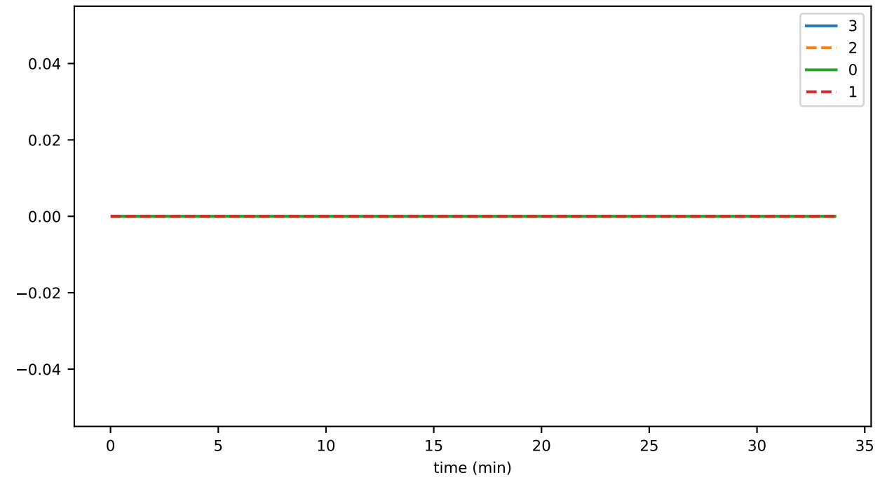
sigStateHash
