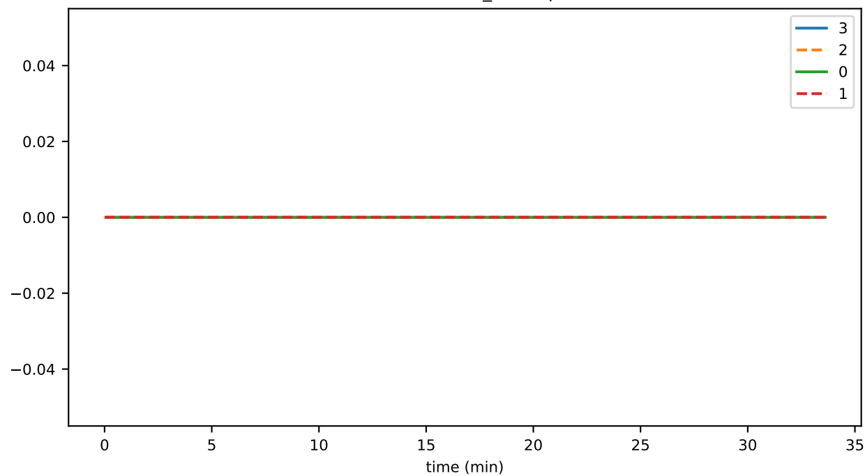
recordHashes_hasGaps
