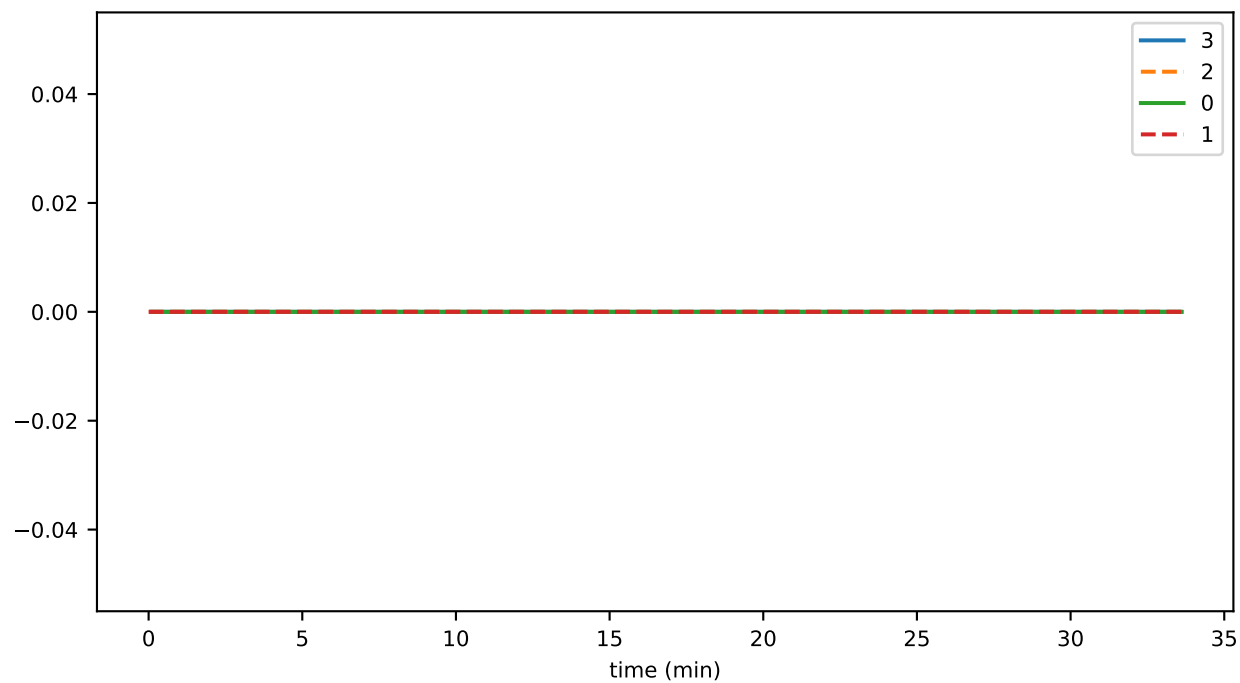
accountsPercentUsed
