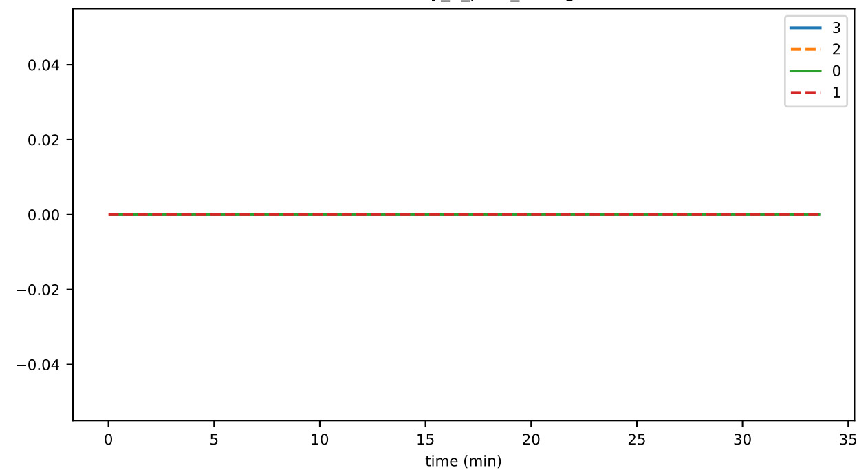
eventDelay_6_pces_storage
