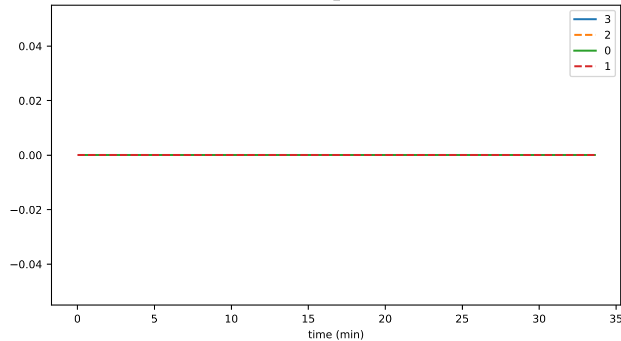
connRecv_skipBlock
