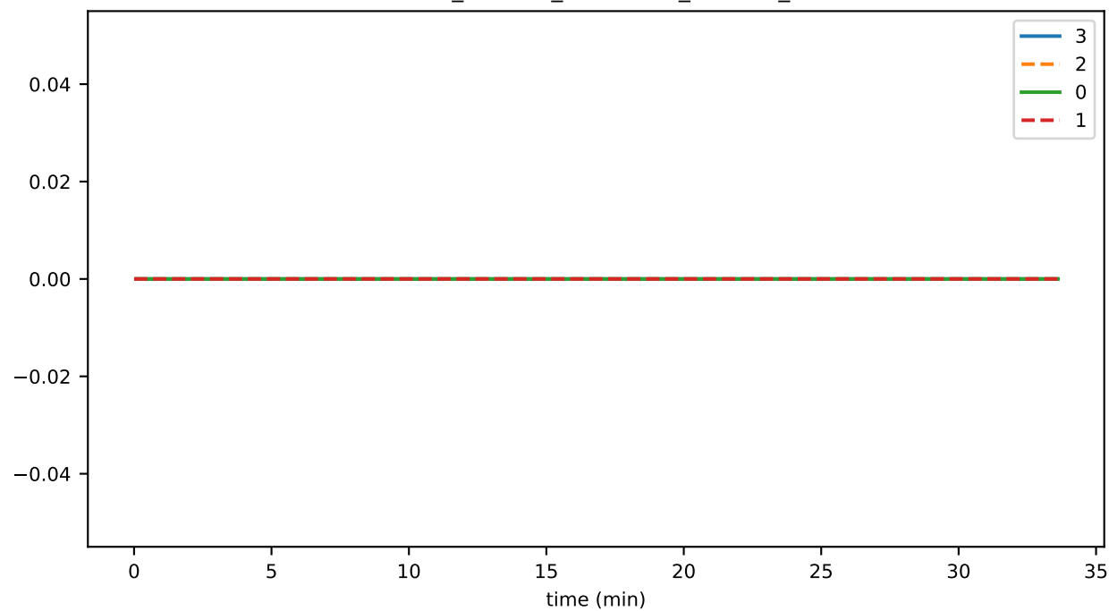
consensus_fraction_CREATING_SIGNED_STATE
