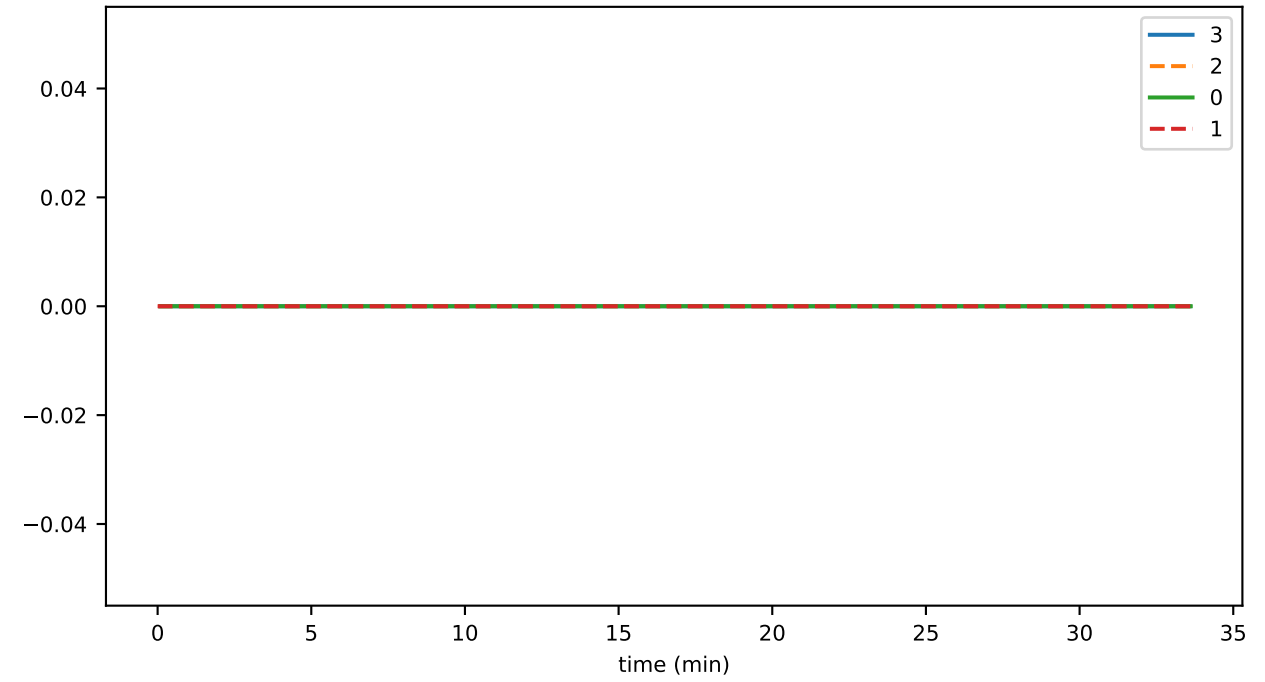
ds_compactions_level_6_leavesTimeMs_state
