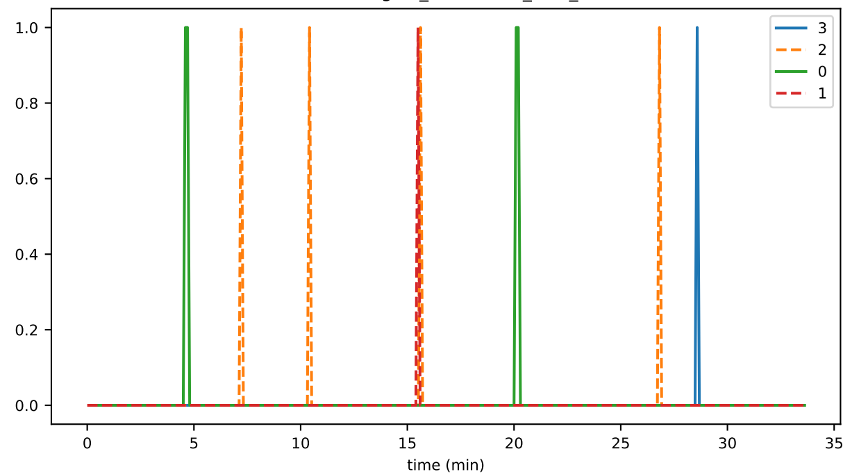
ConsensusEngine_unhandled_task_count
