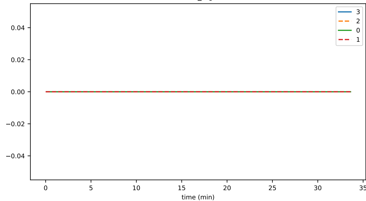
recordHashes_highestBlock
