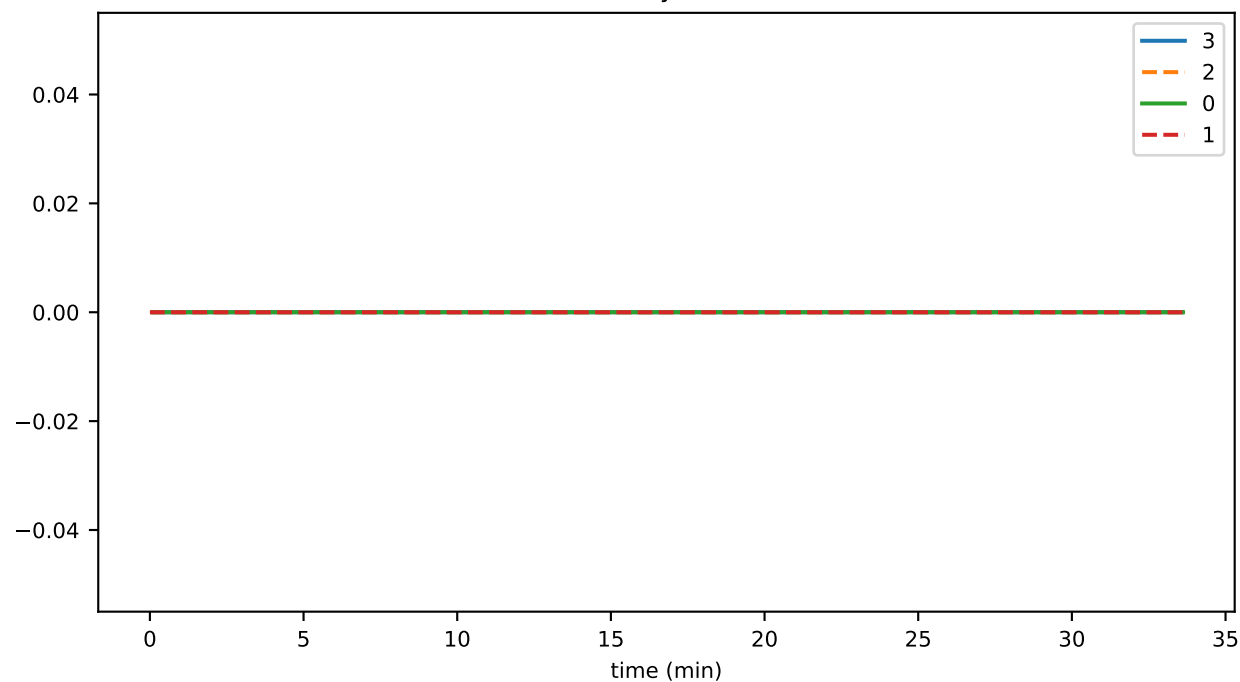
uptimeComputationTime
