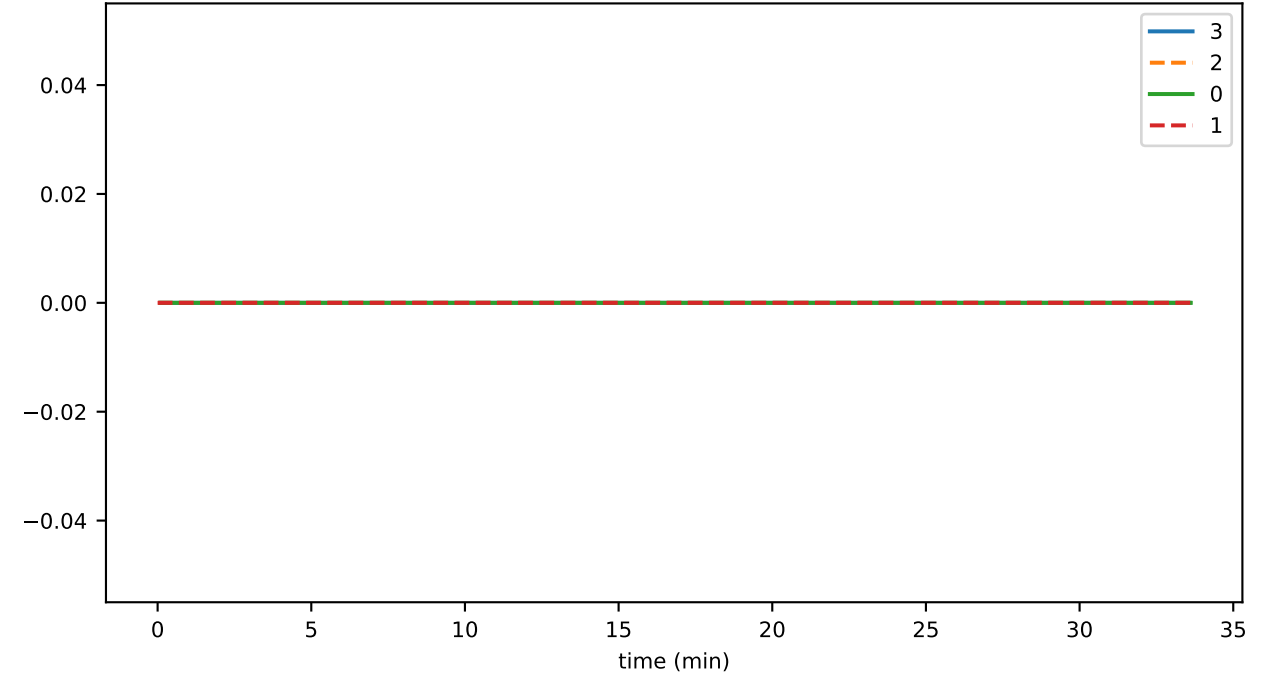
conn_connClose_transientEndStreamReceived
