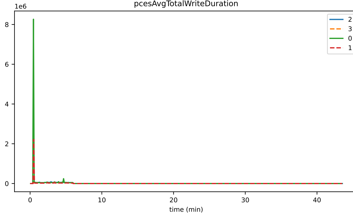
pcesAvgTotalWriteDuration
