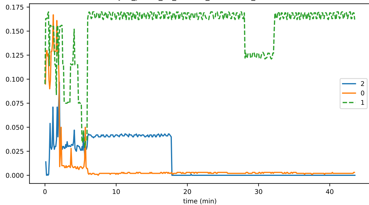
sync_phase_03_fraction_RECEIVING_EVENTS
