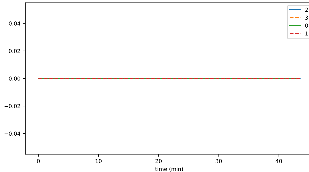
EventDeduplicator_busy_fraction
