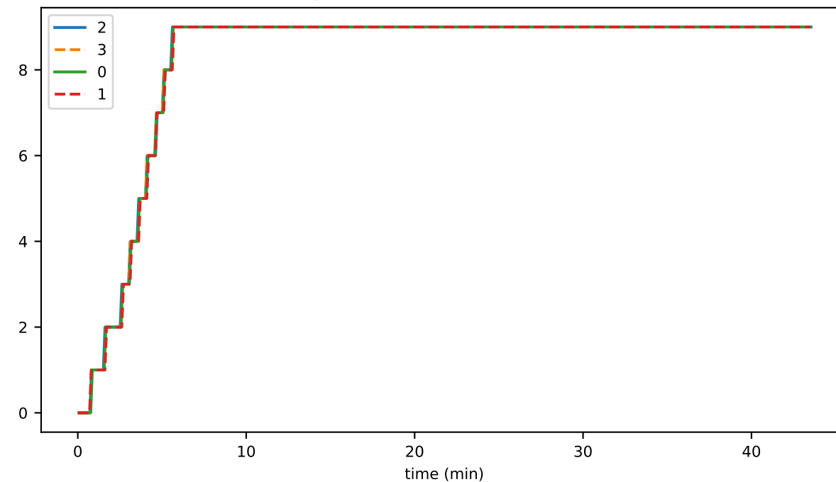
preconsensusEventFileOldestSeconds
