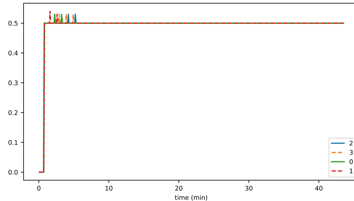
vmap_lifecycle_familySizeBackpressureMs_state
