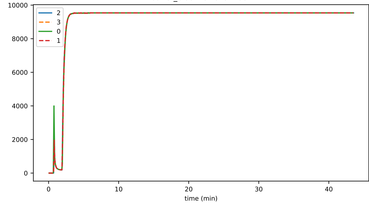
buffer_latestBlockOpened
