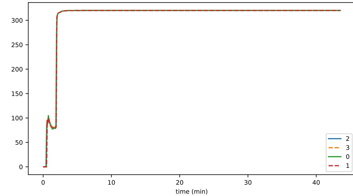
buffer_latestBlockAcked
