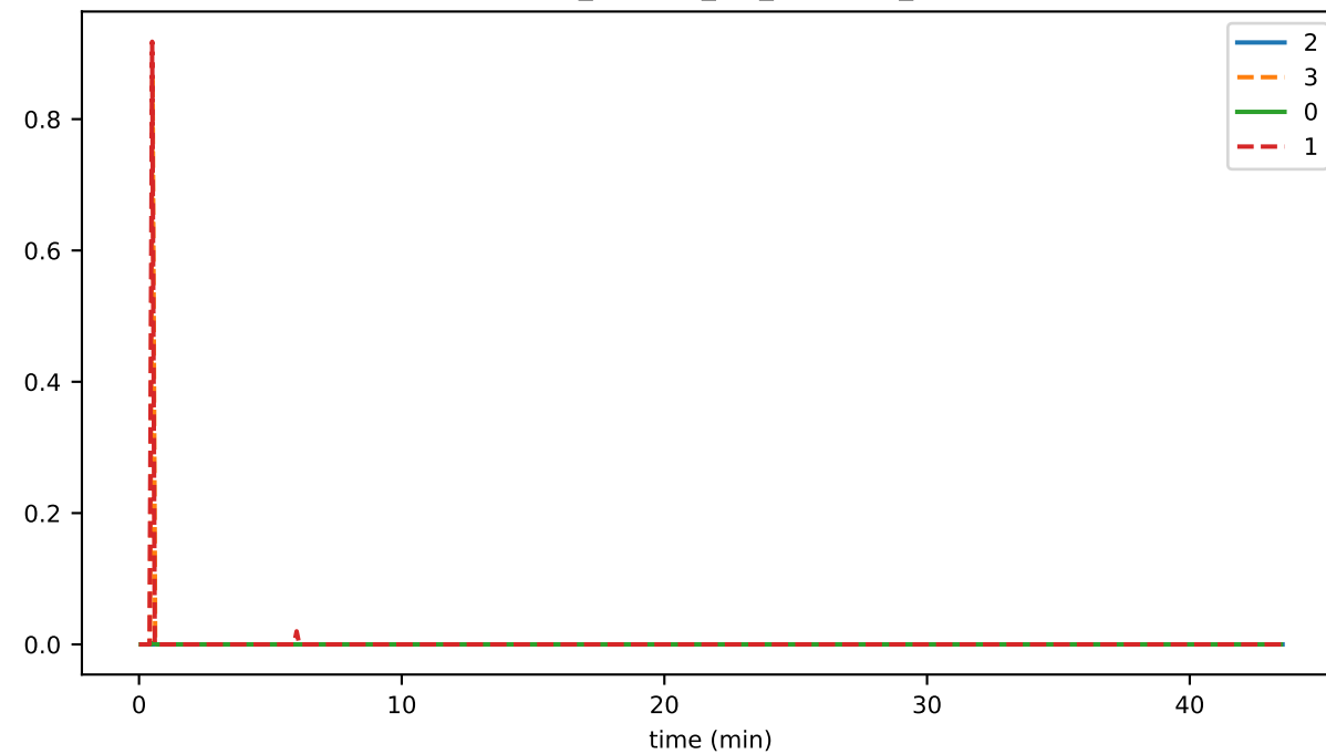
eventCreation_fraction_NO_ELIGIBLE_PARENTS
