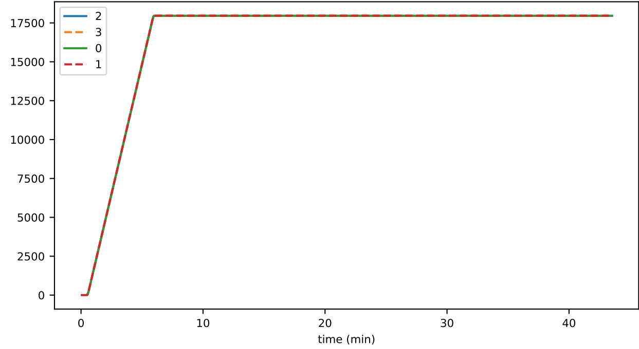
roundIncEqParents
