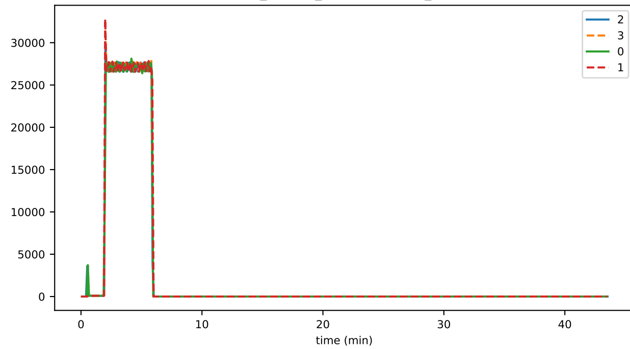
vmap_queries_updatedEntities_state
