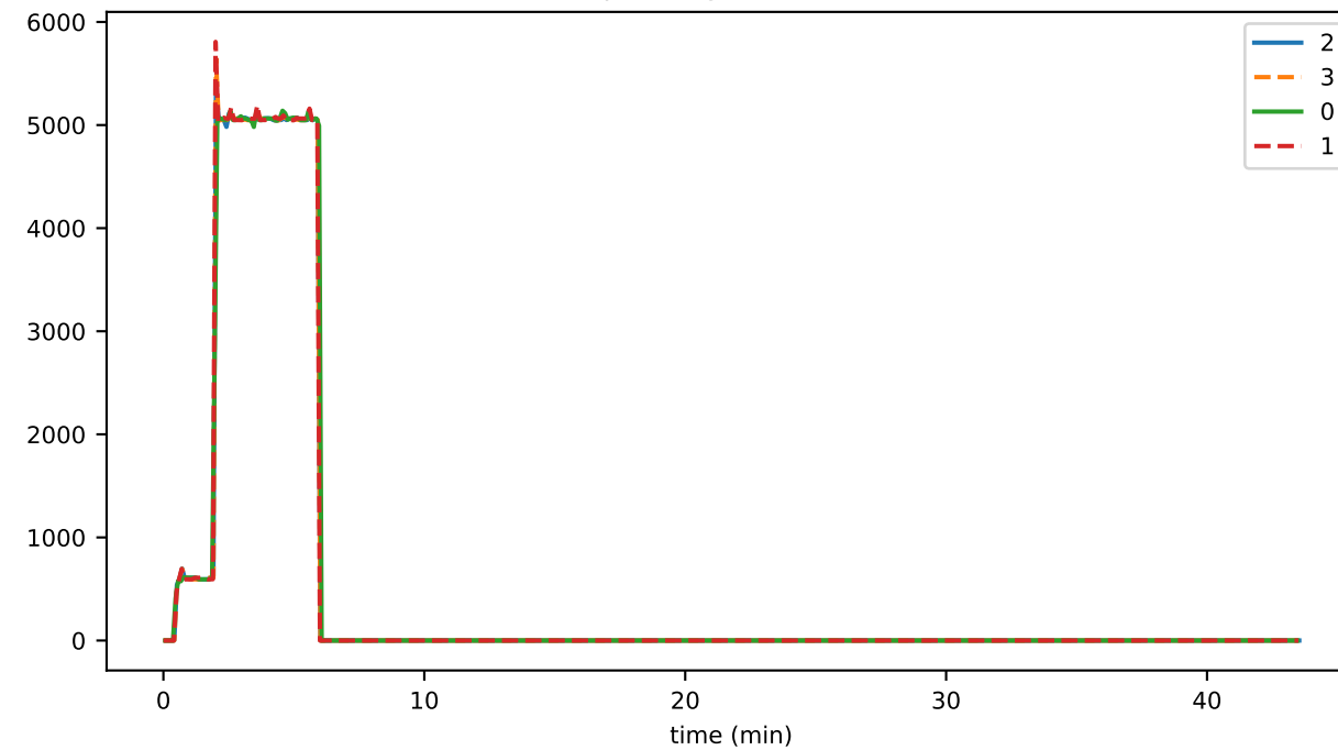
pcesAvgTotalWriteDuration
