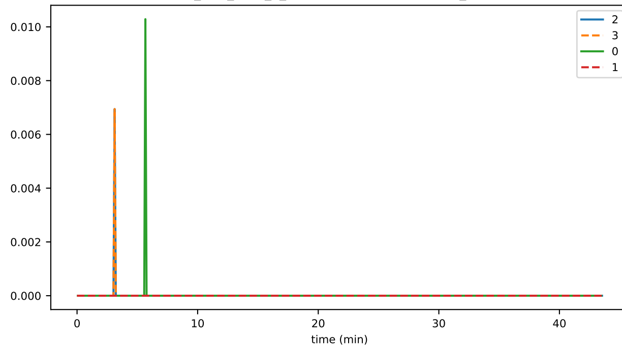
ds_files_level_1_leafKeysFileSizeByLevelMb_state
