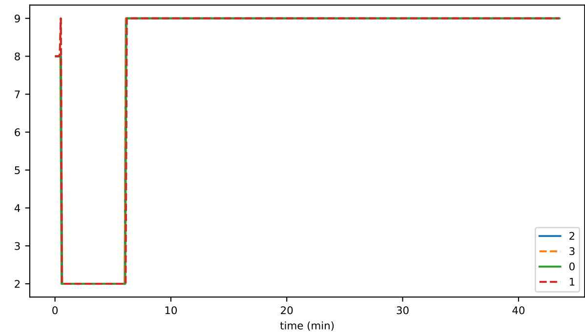
PlatformStatus
