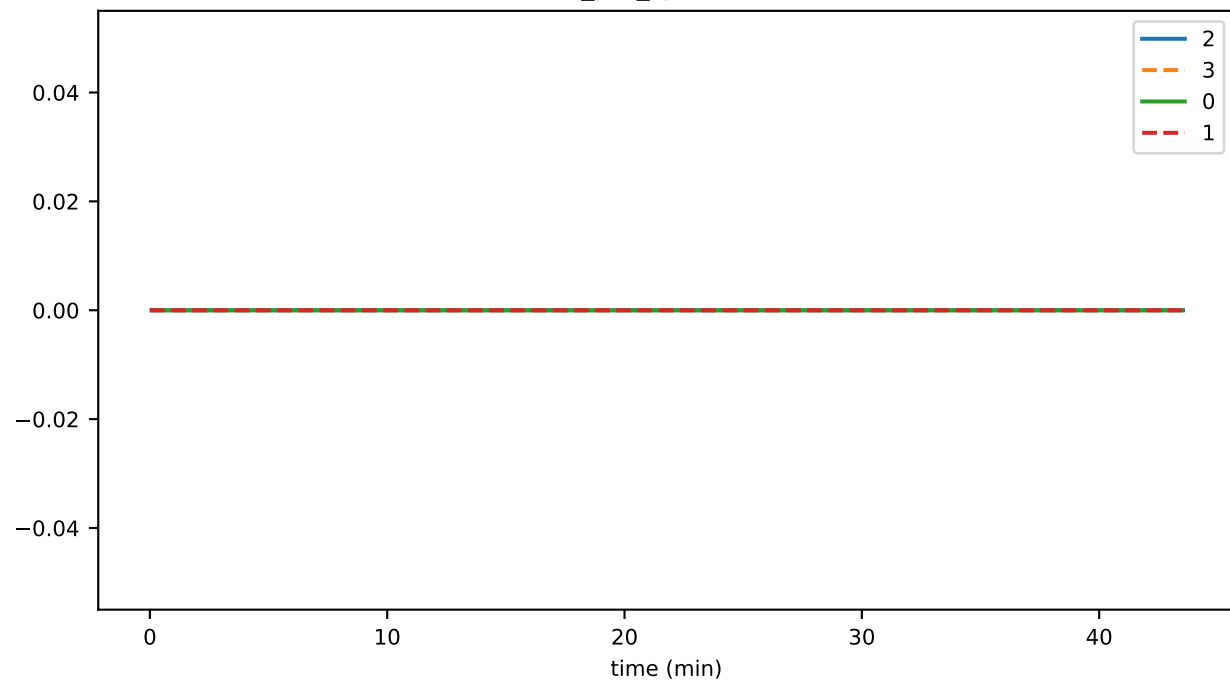
eventCreation_fraction_IDLE
