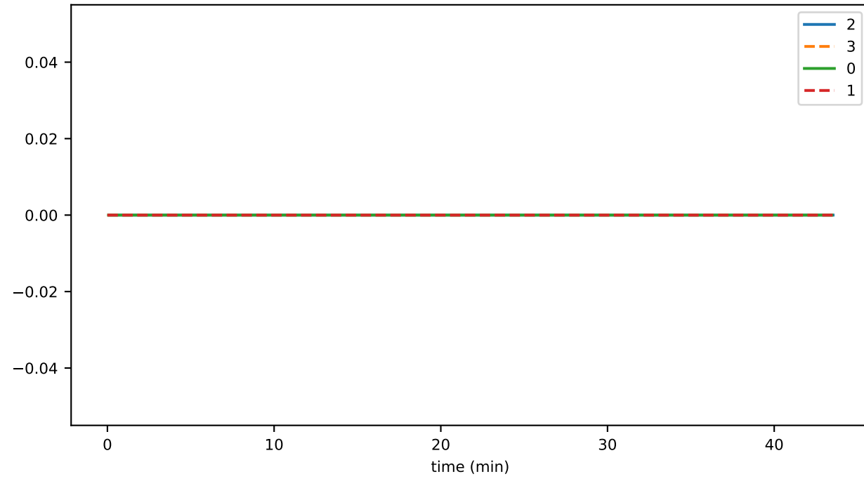
ds_compactions_level_3_leafKeysSavedSpaceMb_state
