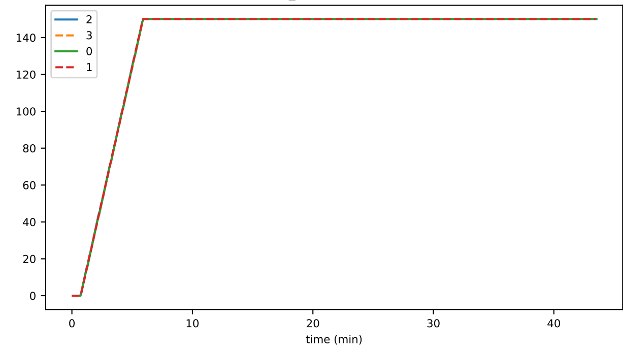
buffer_latestBlockOpened
