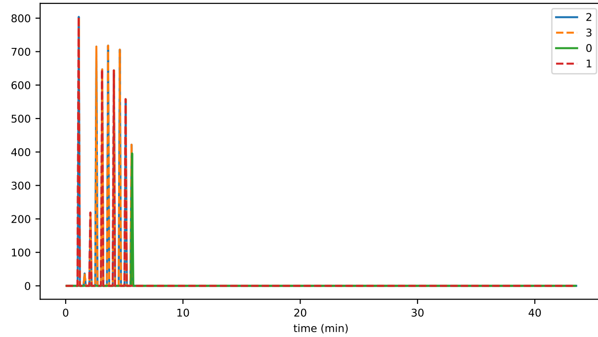
ds_offheap_hashesIndexMb_state
