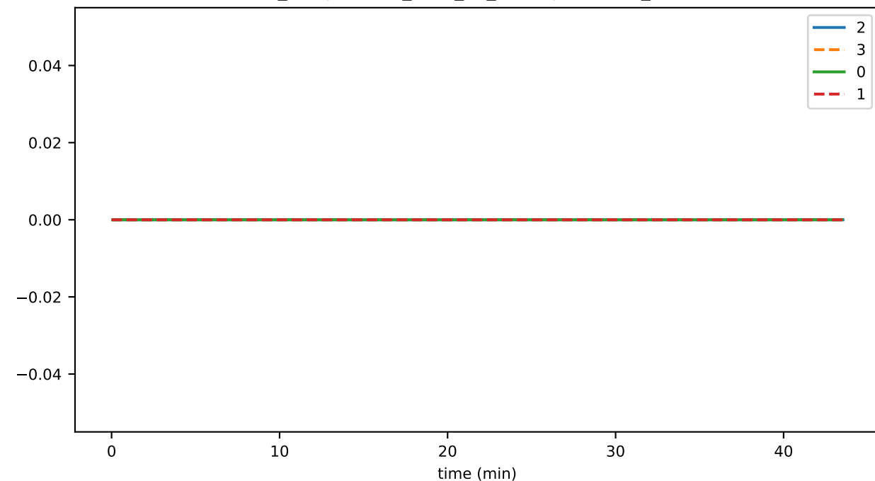
ds_compactions_level_10_leavesTimeMs_state
