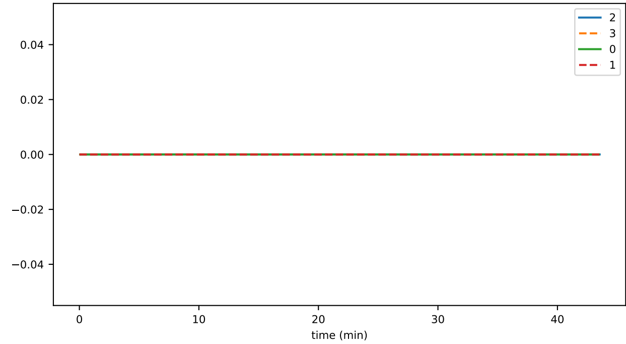
roundIncEqParents
