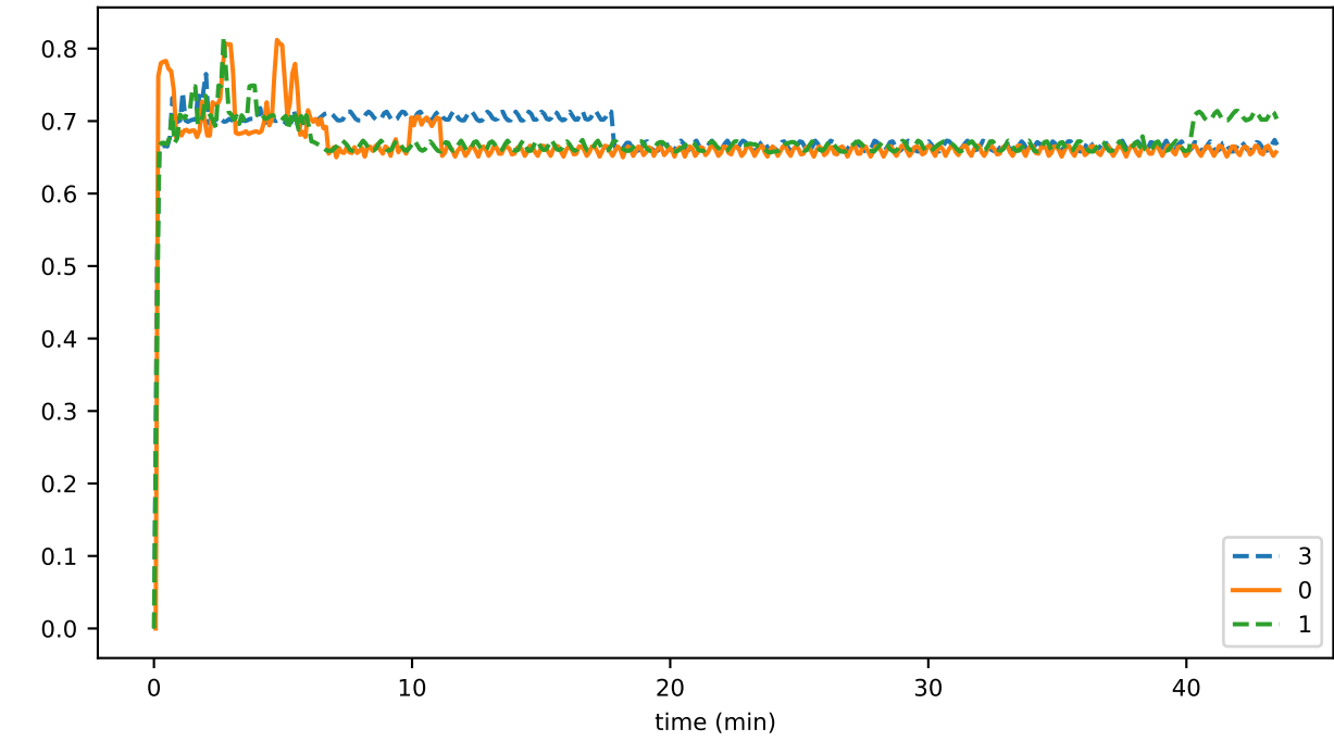
sync_phase_02_fraction_OTHER_FALLEN_BEHIND
