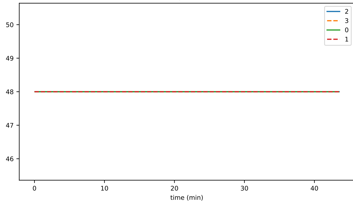
reconnectRejections_per_sec_00
