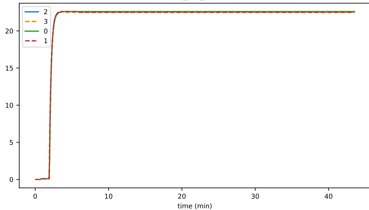
trans_per_event
