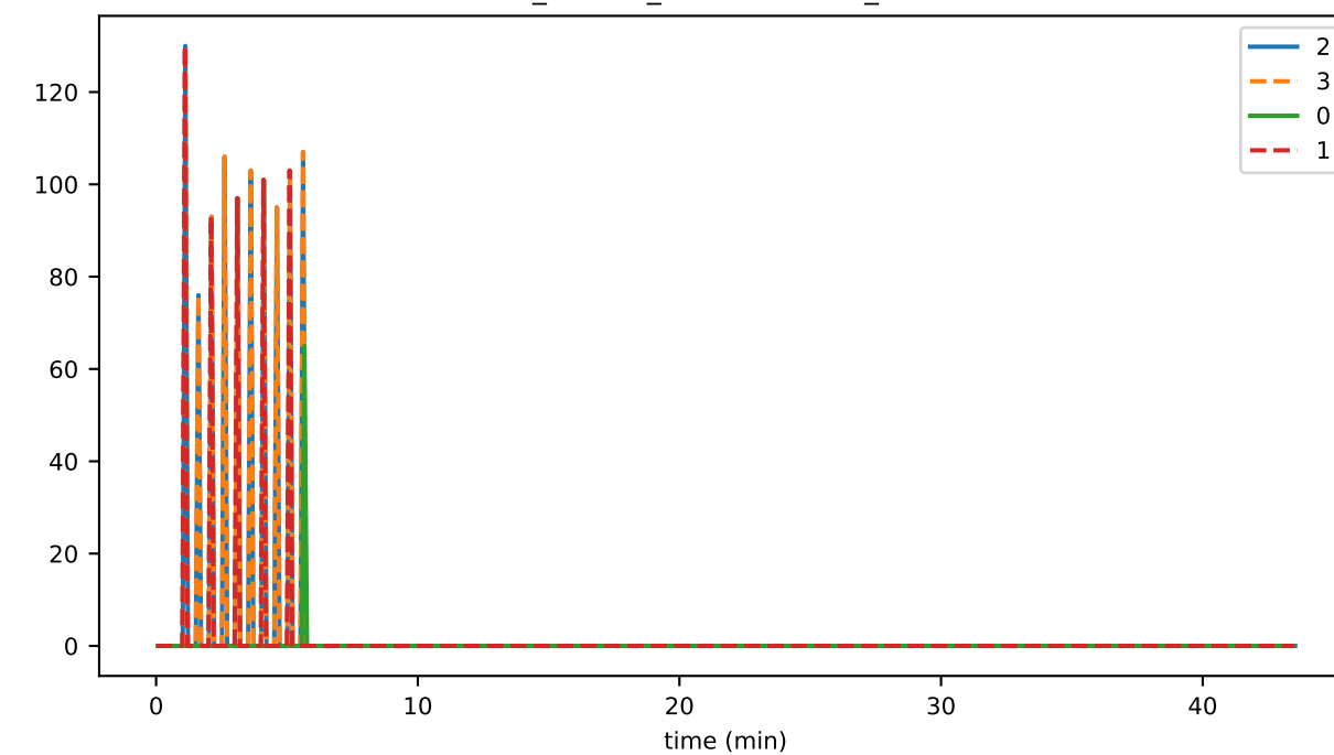
ds_flushes_hashesWritten_state
