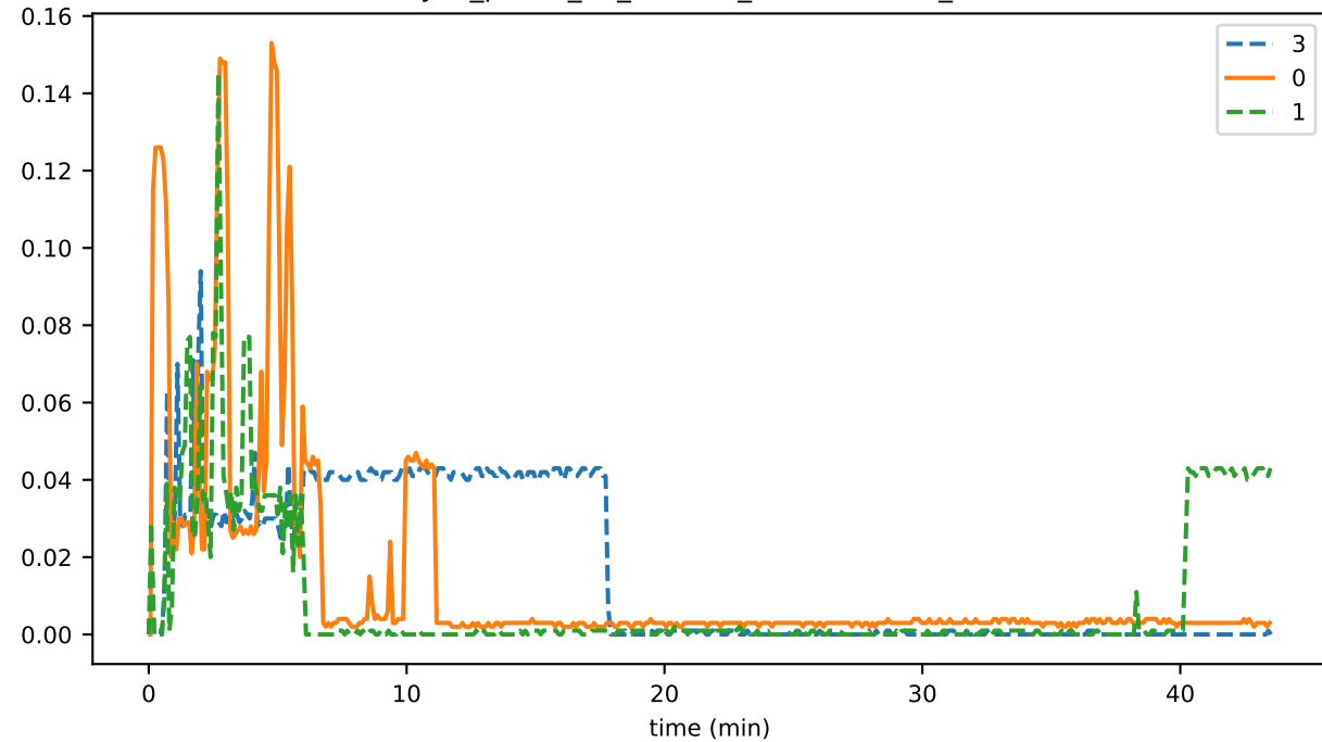
sync_phase_02_fraction_EXCHANGING_TIPS
