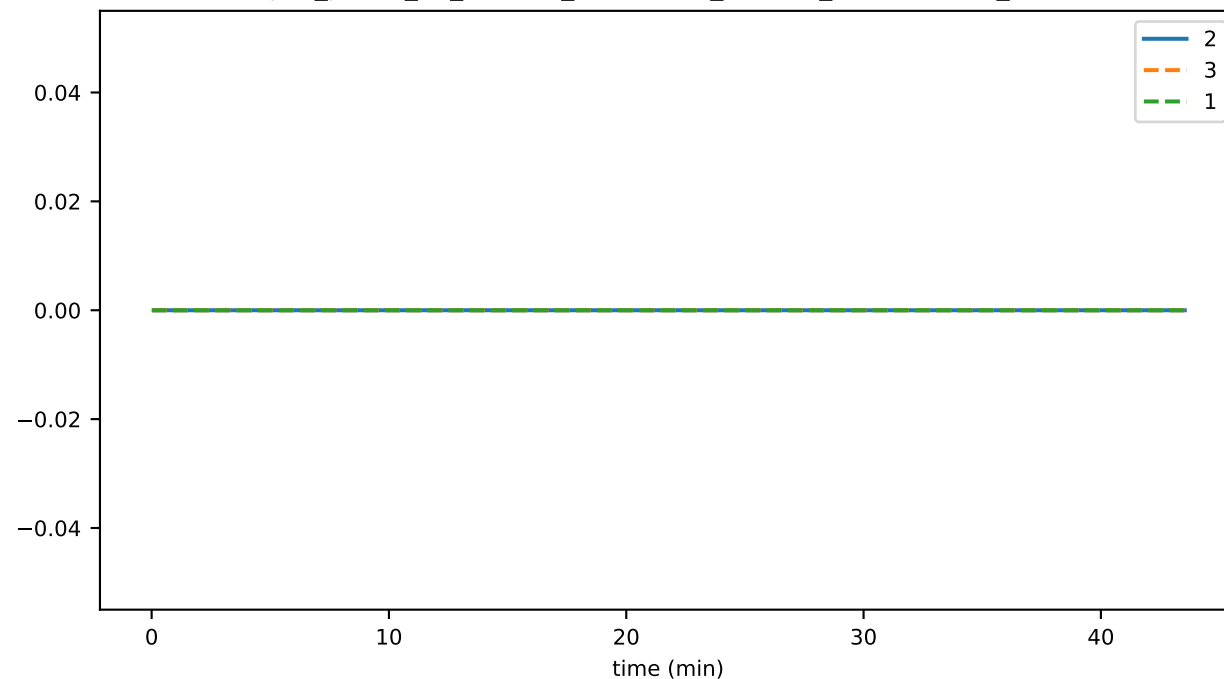
sync_phase_00_fraction_SELF_FALLEN_BEHIND
