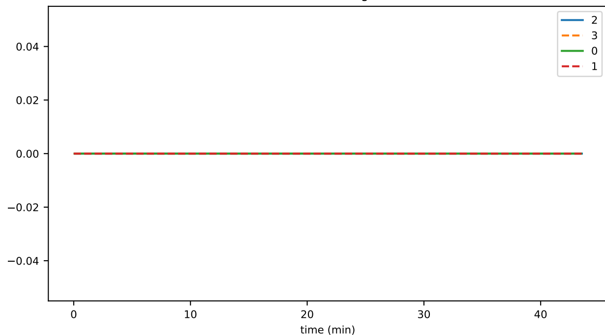
branchingEvents
