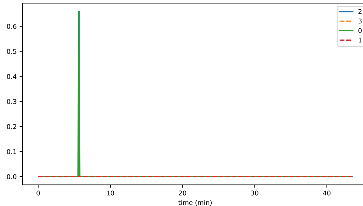
ds_files_level_2_leavesFileSizeByLevelMb_state
