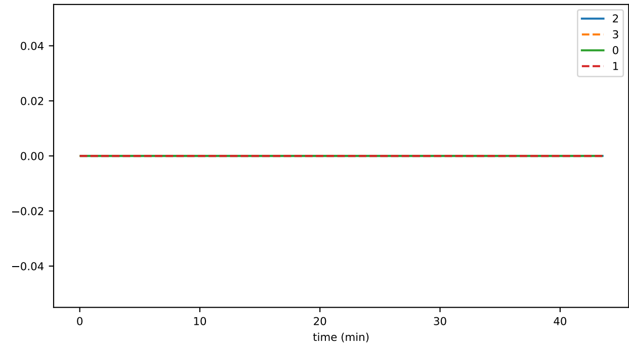
doNotSyncIntakeCounter
