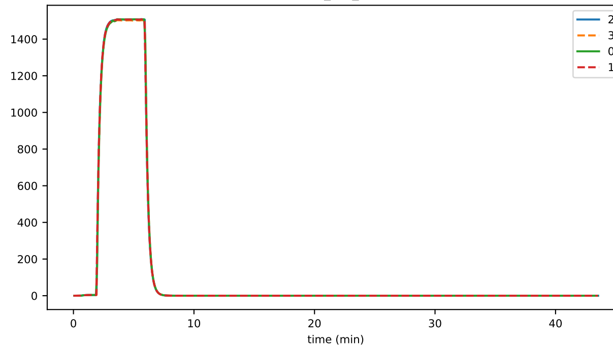
trans_per_sec
