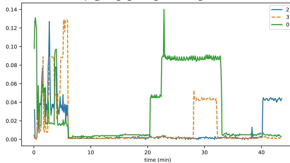
sync_phase_01_fraction_EXCHANGING_WINDOWS
