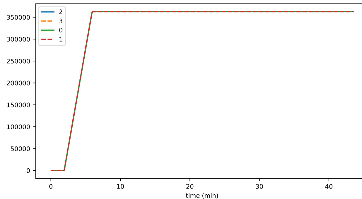
trans_per_sec
