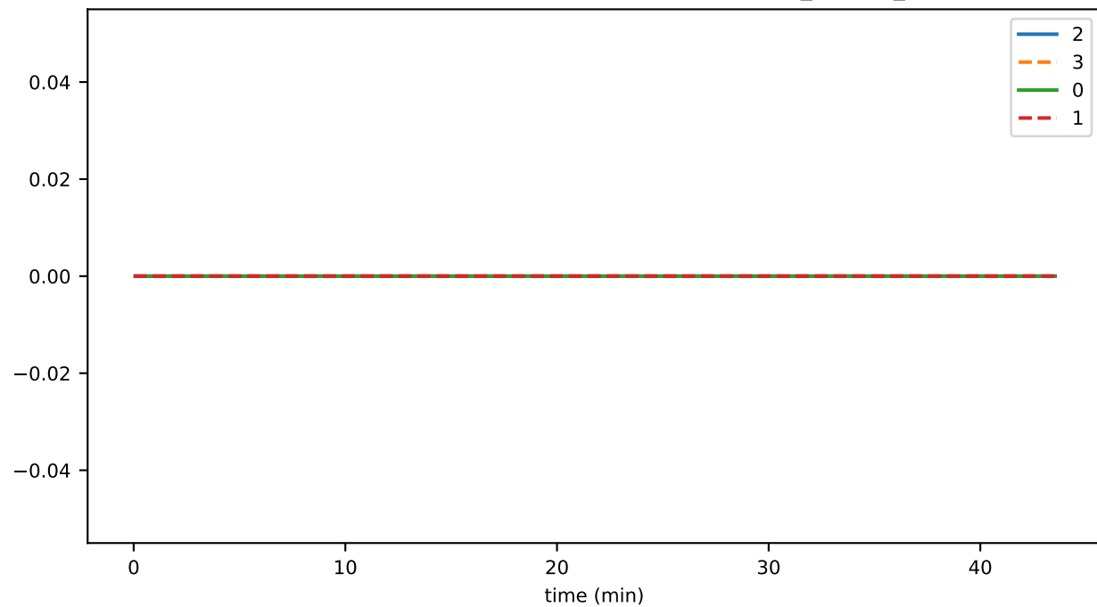
SmartContractService:SystemContractMethodCall_REJECT_total
