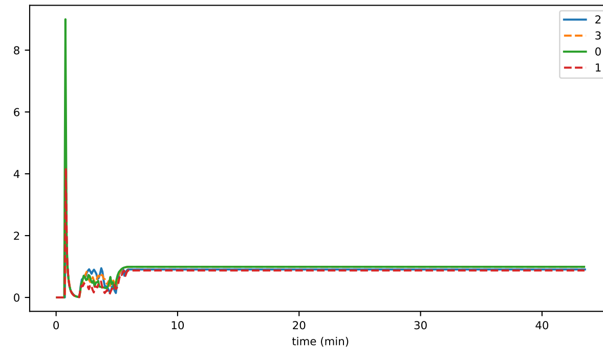
sigStateHash
