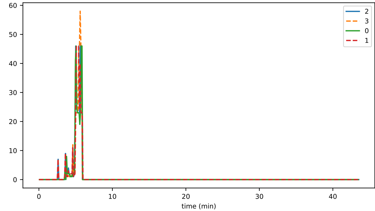
vmap_size_state
