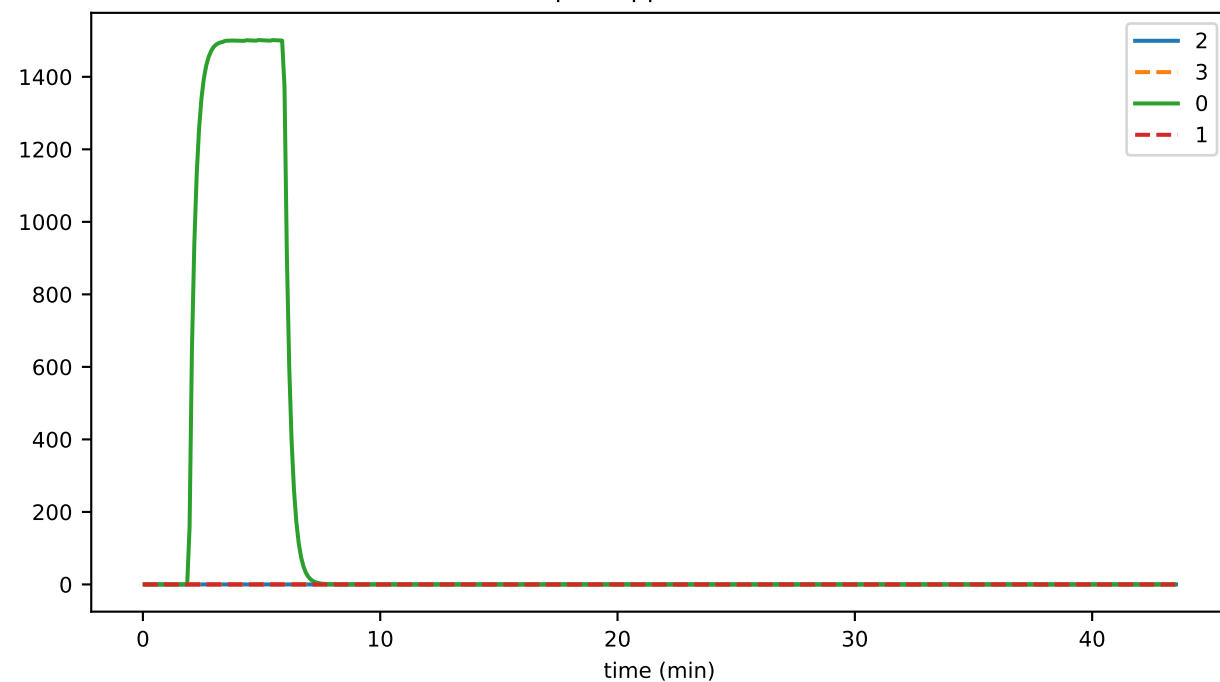
accountsMaxNumber
