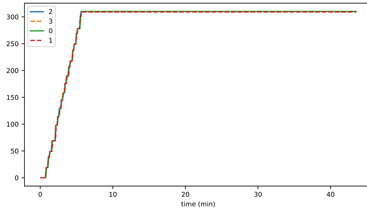
preconsensusEventFileOldestSeconds
