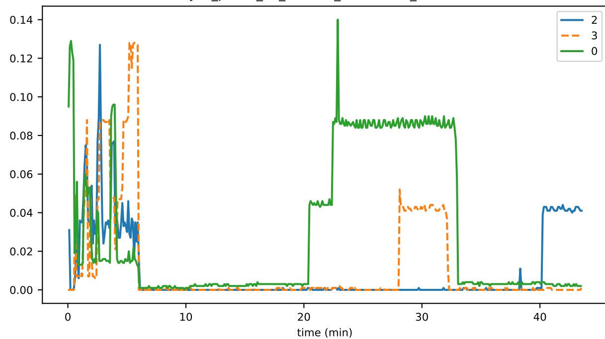
sync_phase_01_fraction_RECEIVING_EVENTS
