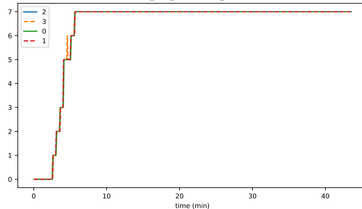
ds_flushes_hashesWritten_state
