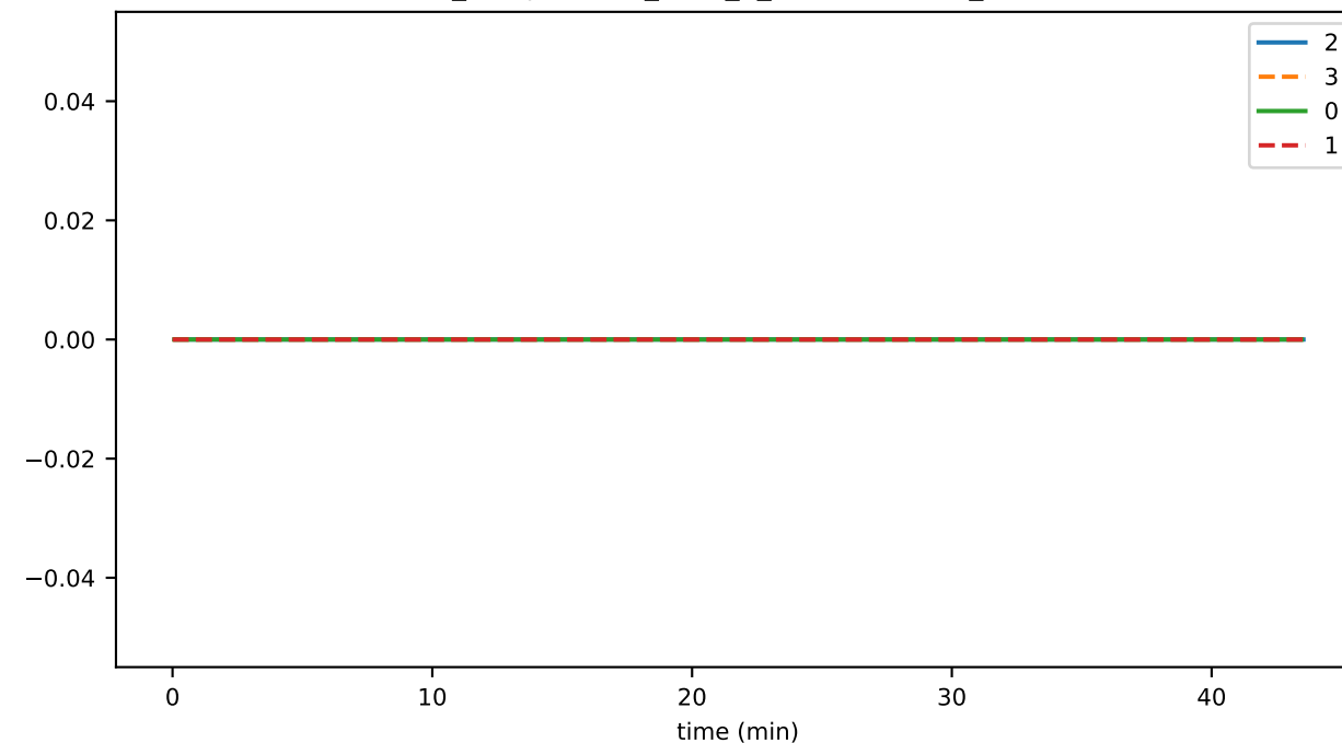
ds_compactions_level_6_hashesTimeMs_state
