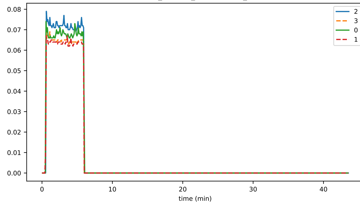
eventCreation_fraction_NO_ELIGIBLE_PARENTS
