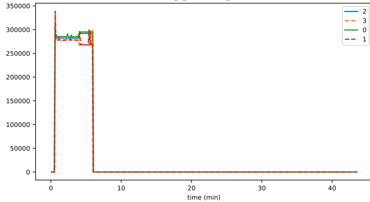
eventDelay_7_consensus_storageMAX
