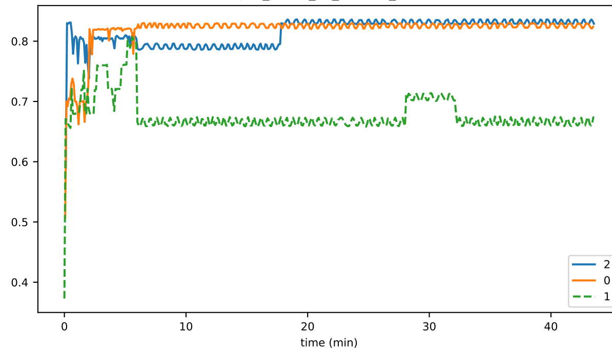
sync_phase_03_fraction_OTHER_FALLEN_BEHIND
