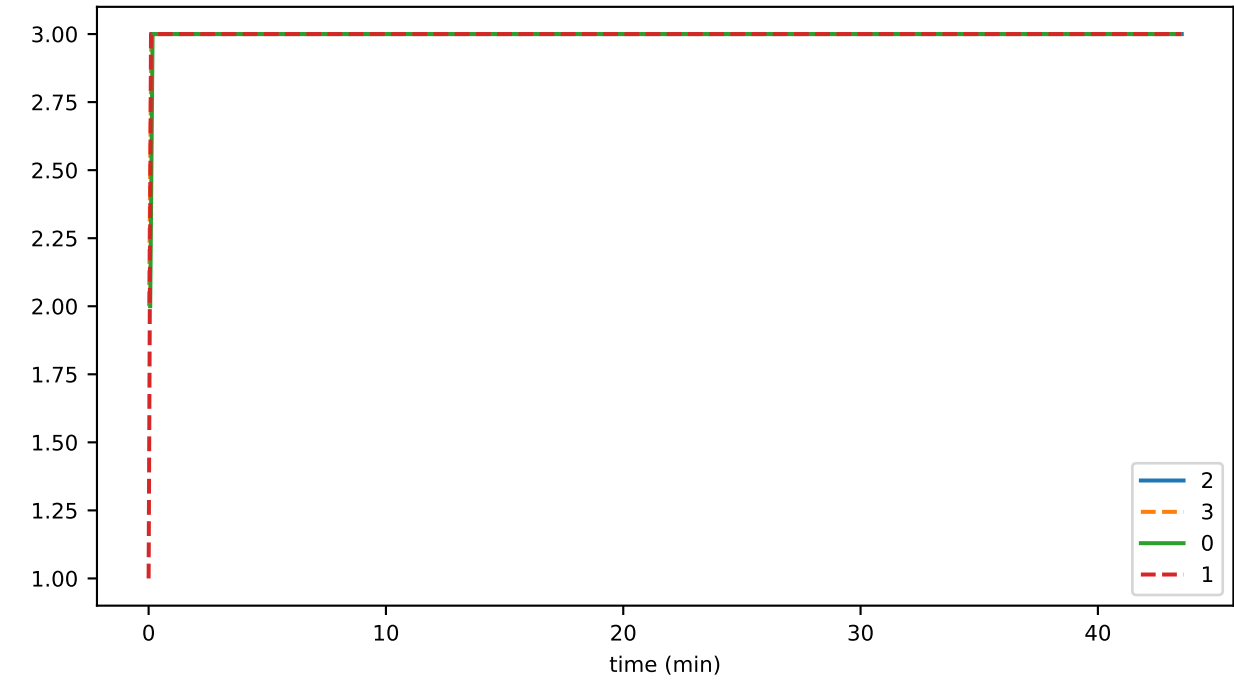
schedulesMaxNumber
