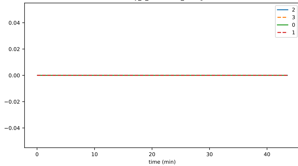
eventDelay_7_consensus_storageMAX
