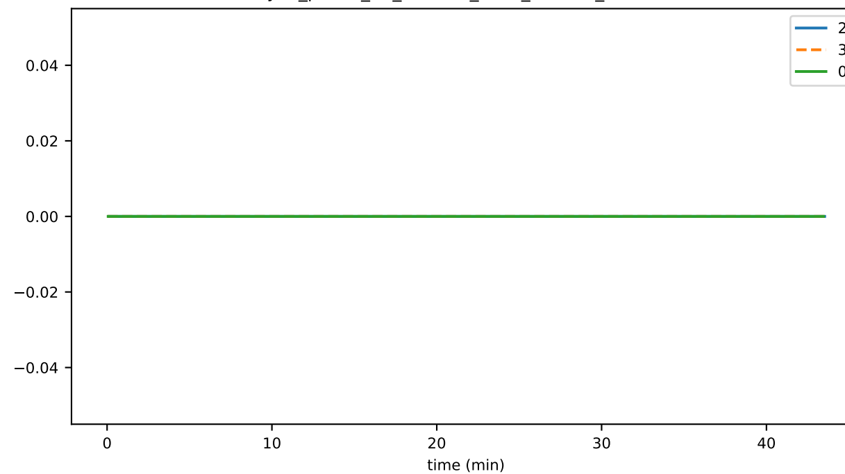
sync_phase_01_fraction_SELF_FALLEN_BEHIND
