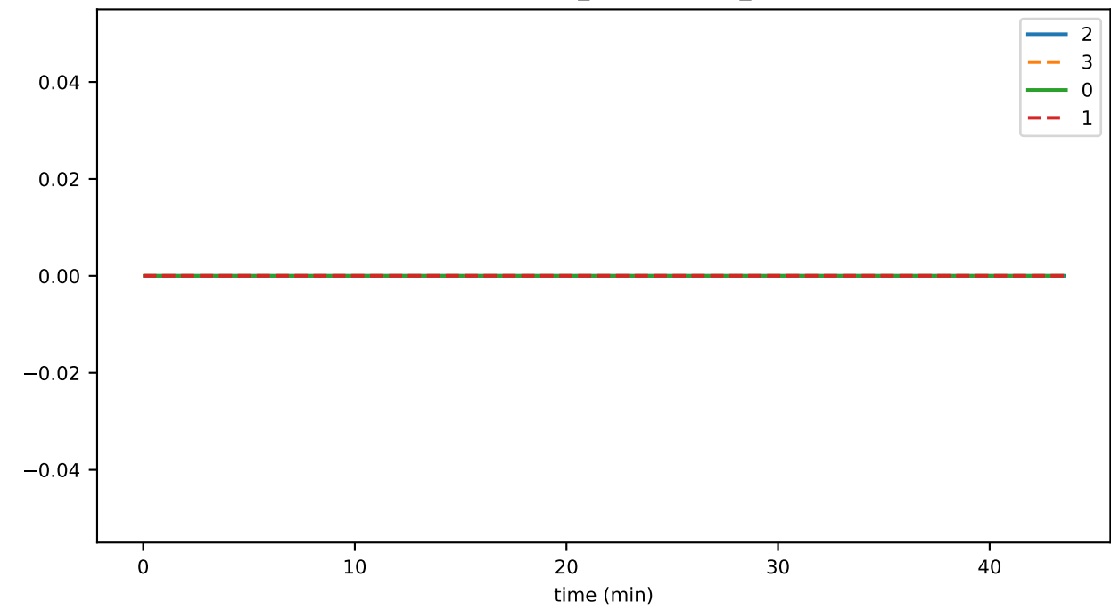
futureEventBuffer_eventCreator_maxBR
