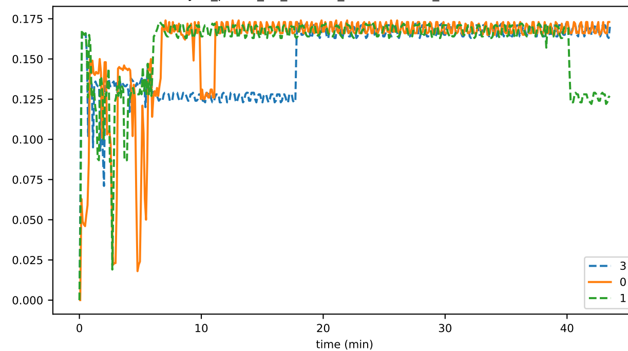
sync_phase_02_fraction_EXCHANGING_WINDOWS
