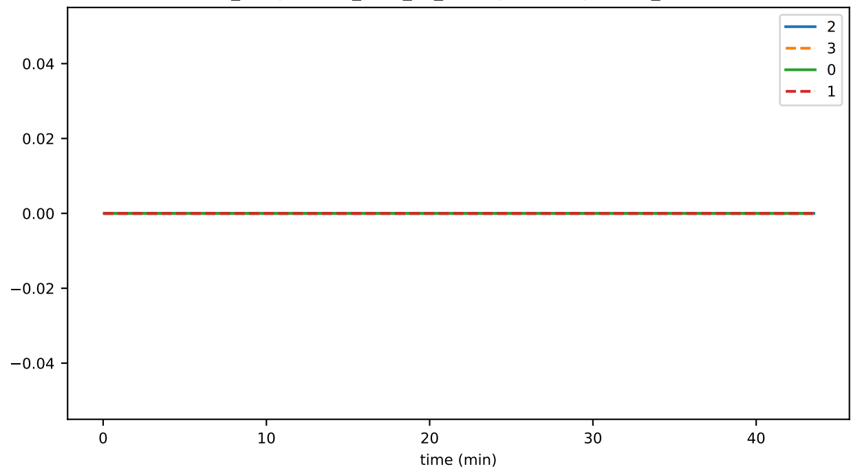
ds_compactions_level_10_leavesSavedSpaceMb_state
