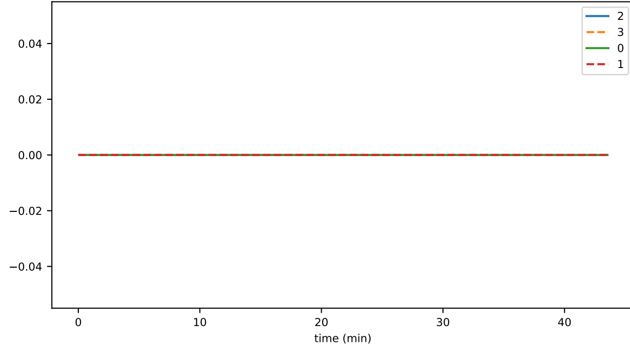
SigIntakePulseTime
