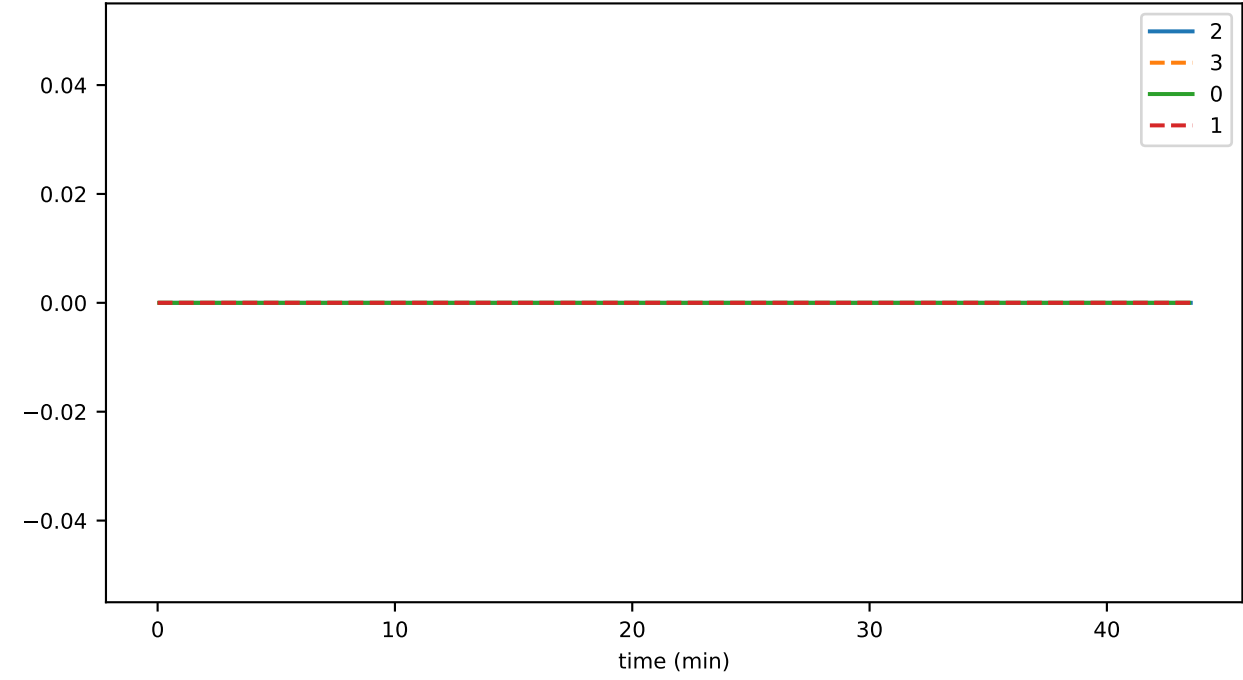
ds_files_level_5_leafKeysFileSizeByLevelMb_state
