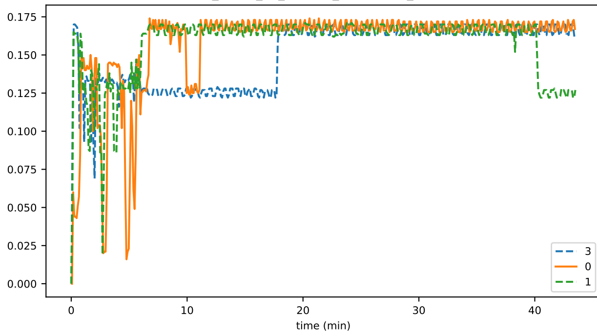
sync_phase_02_fraction_RECEIVING_EVENTS
