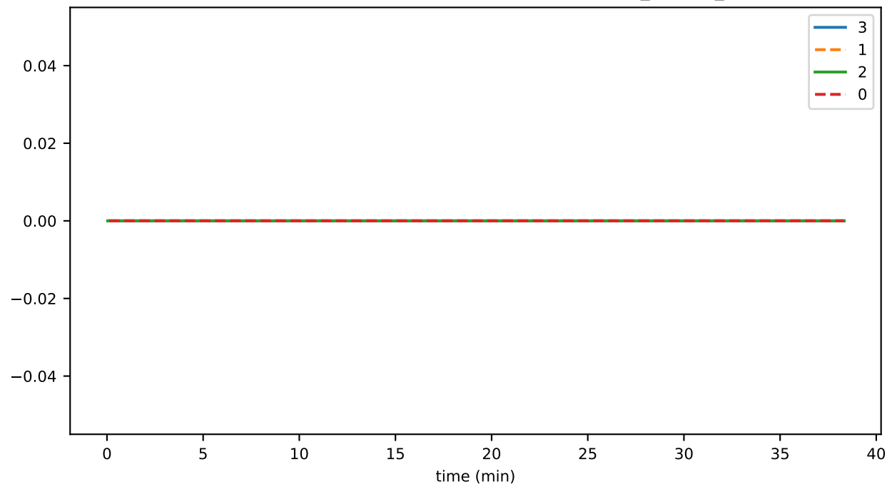
SmartContractService:SystemContractMethodCall_REJECT_total
