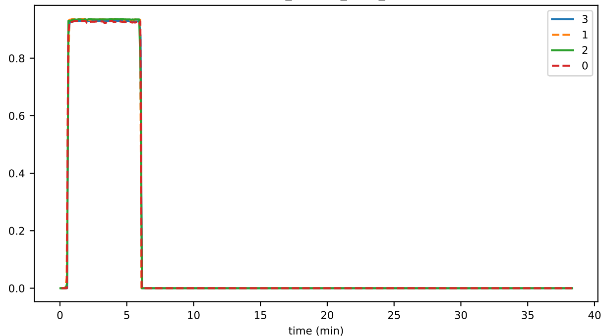
EventManager_unhandled_task_count
