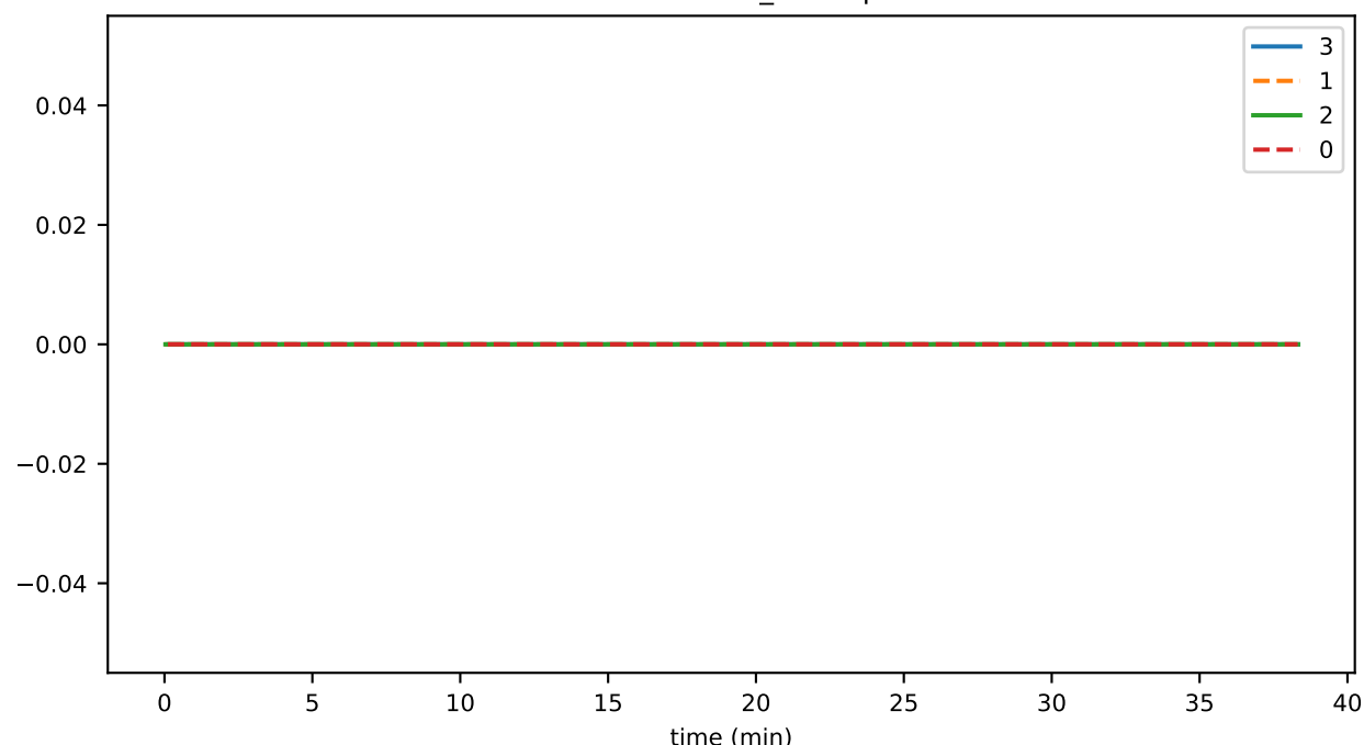
recordHashes_hasGaps
