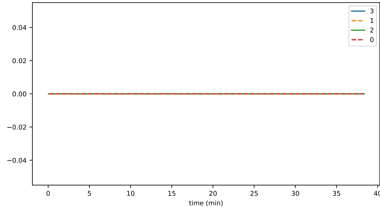
SmartContractService:SystemContractMethodCall_TRANSFER_failed
