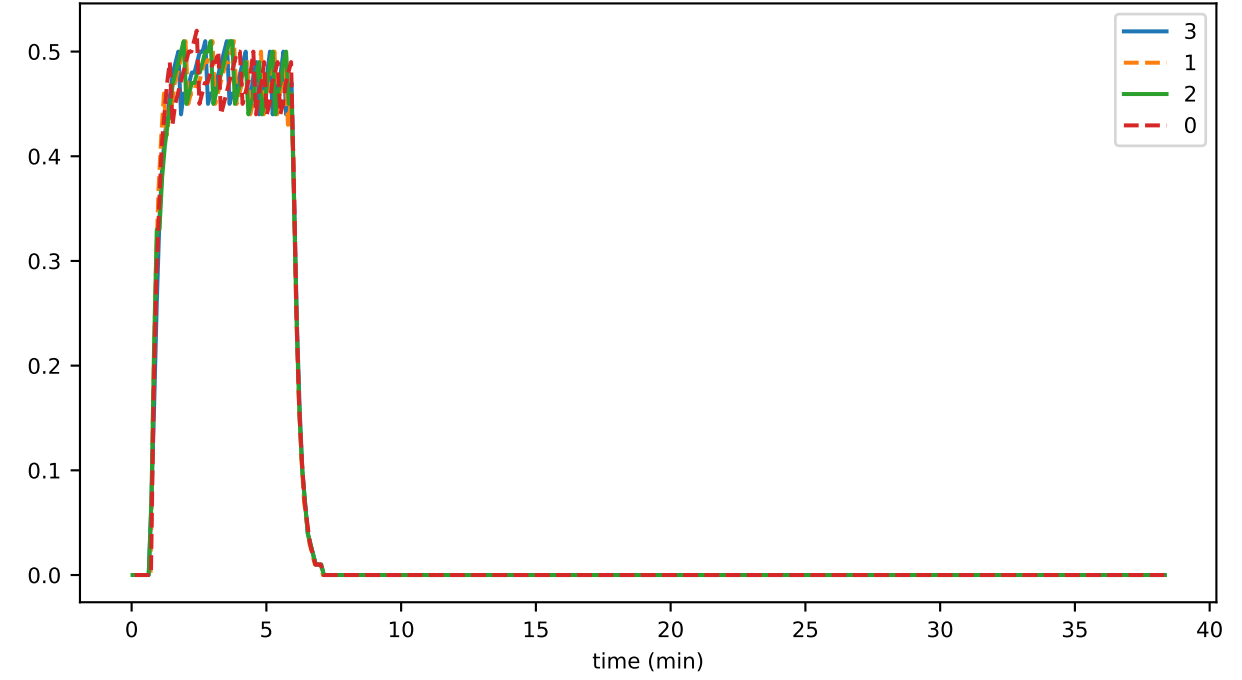
sstatesSigned_per_sec
