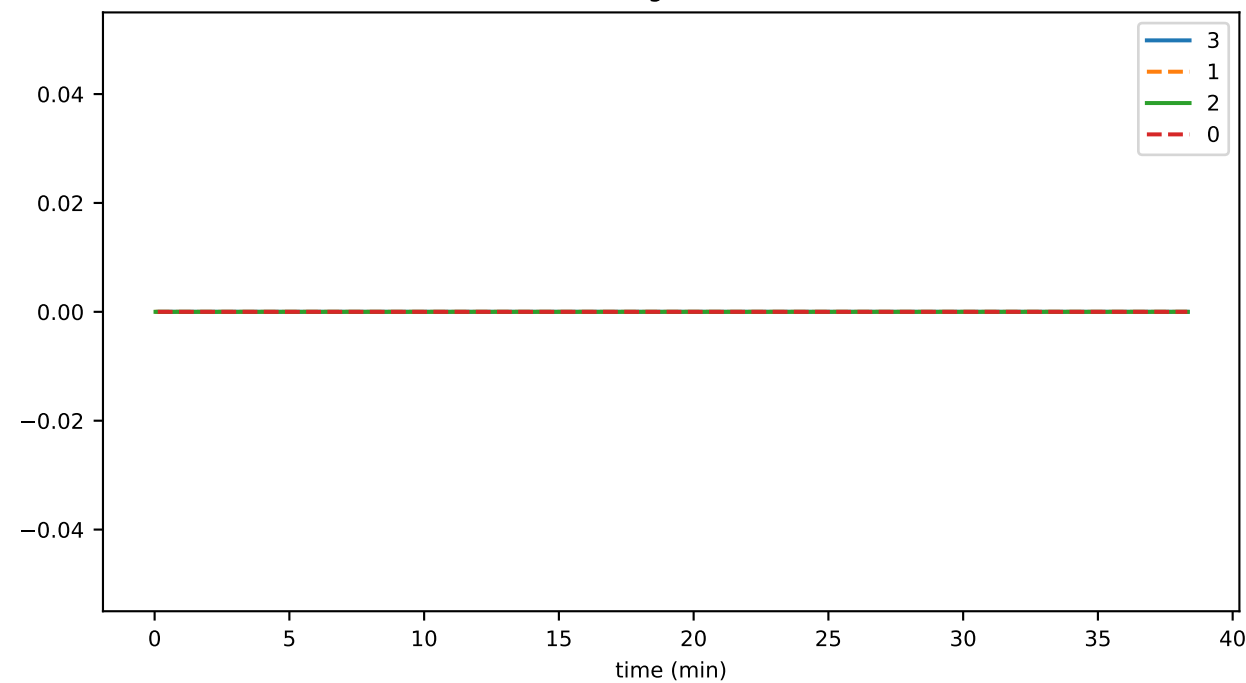
branchingNodeCount
