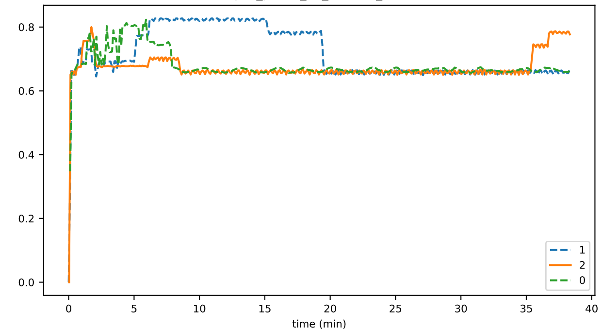
sync_phase_03_fraction_OTHER_FALLEN_BEHIND
