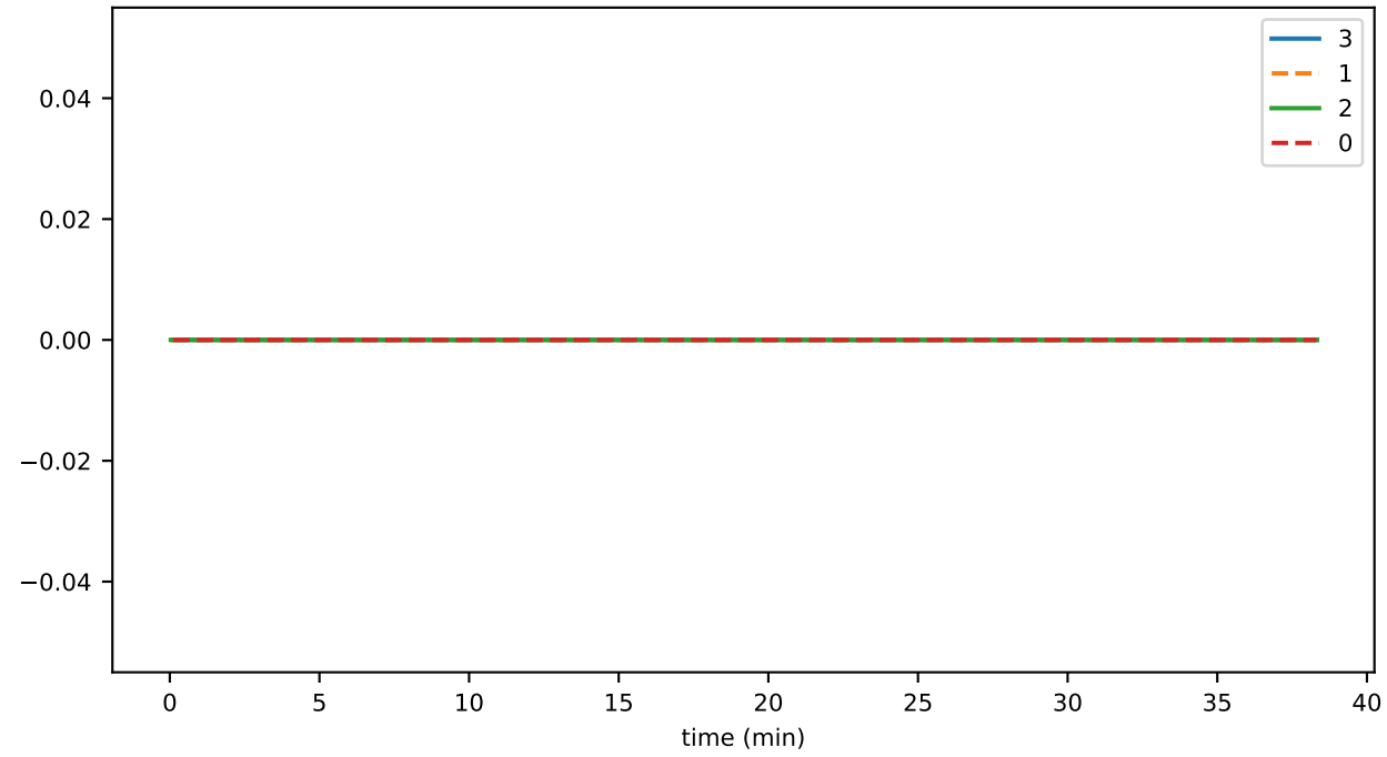
SmartContractService:TransactionGasUsed_sum
