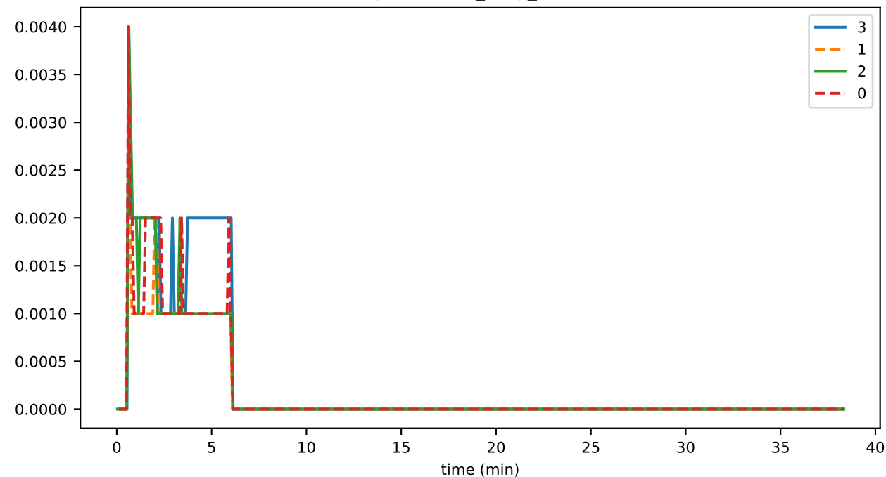
orphanBufferSize
