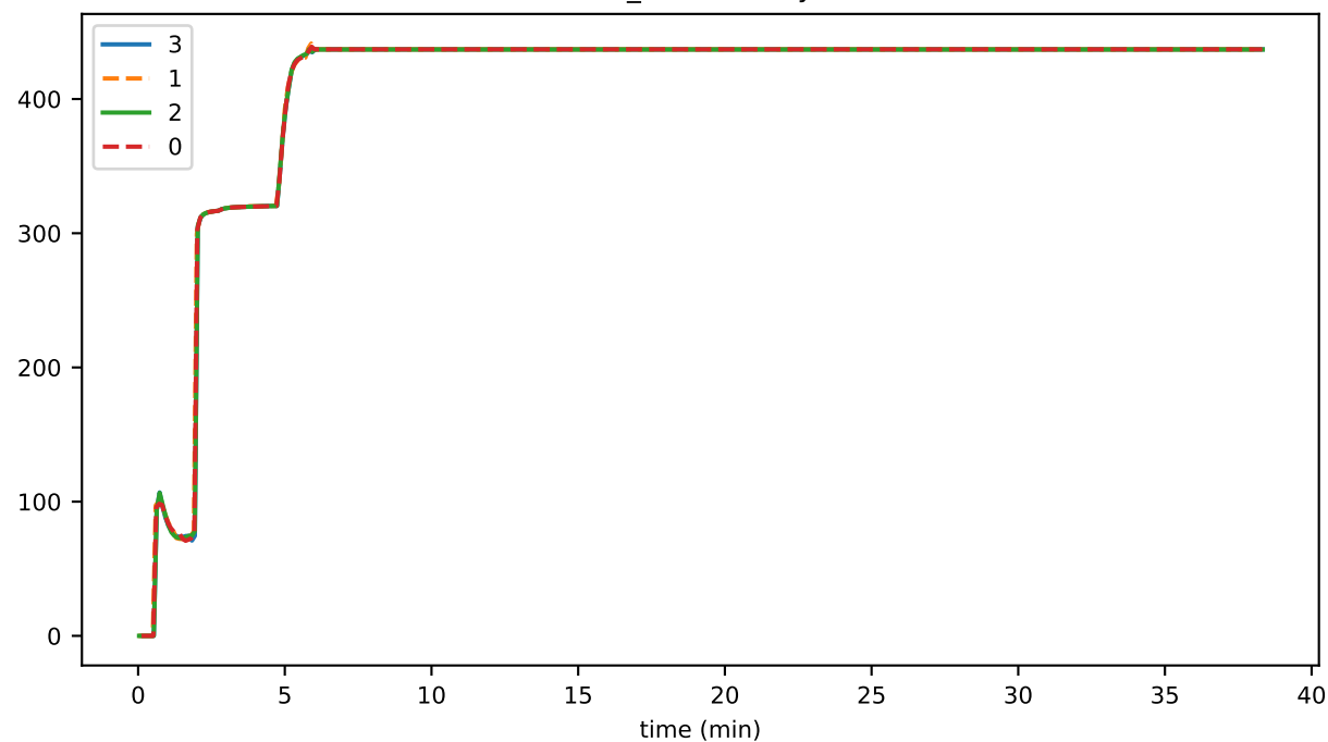
buffer_latestBlockAcked
