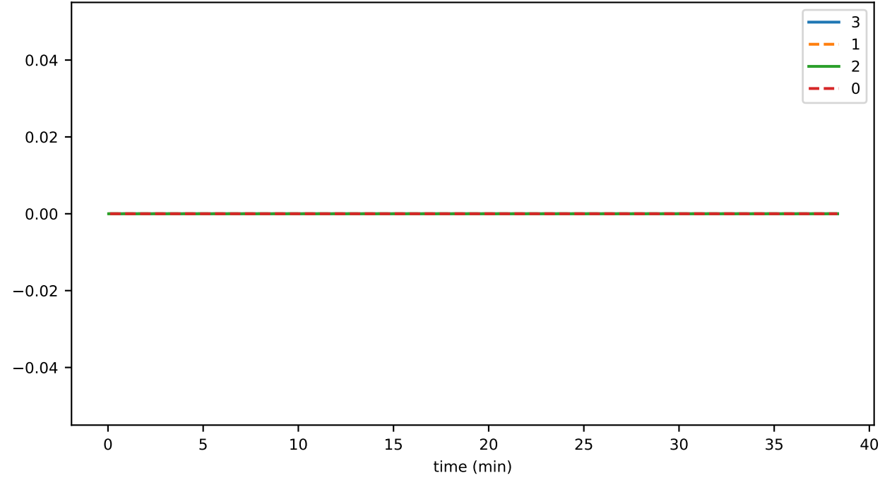
airdropsUsed
