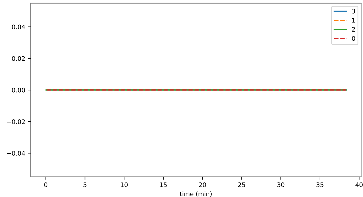
connRecv_endStream_unknown
