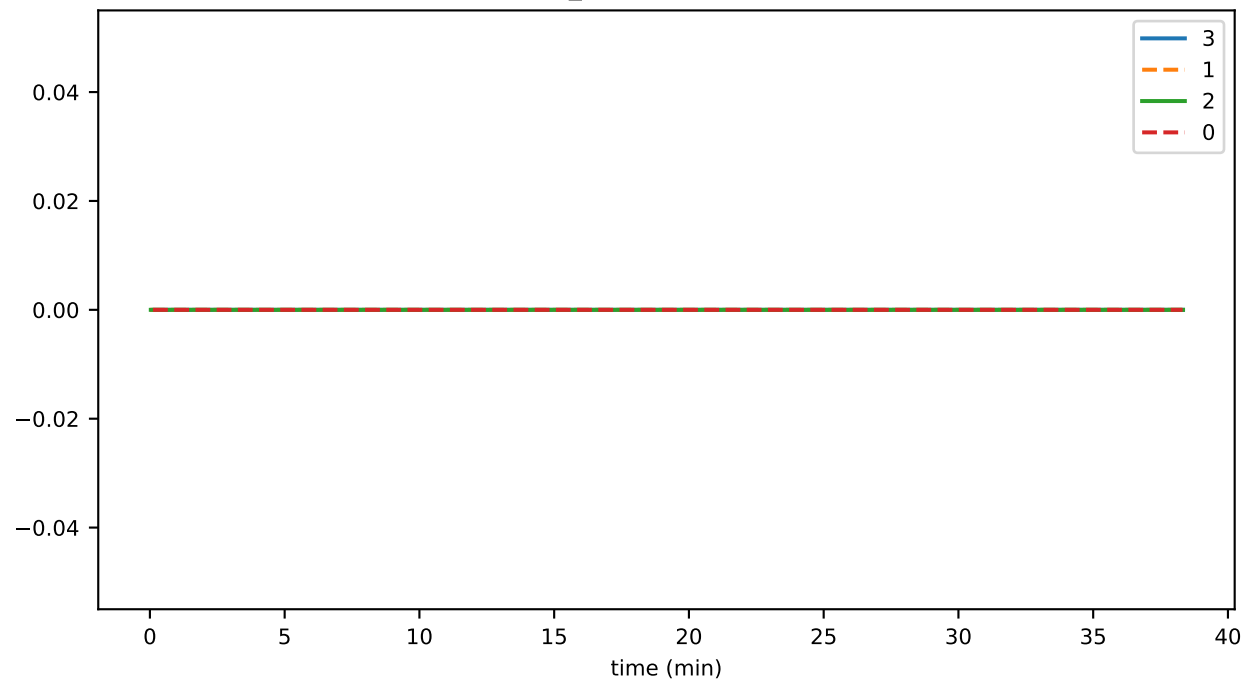
conn_highLatencyEvents
