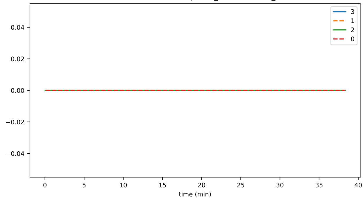
SmartContractService:Rejected_contractCallTx_total
