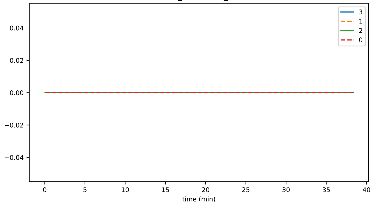
connSend_endStream_timeout
