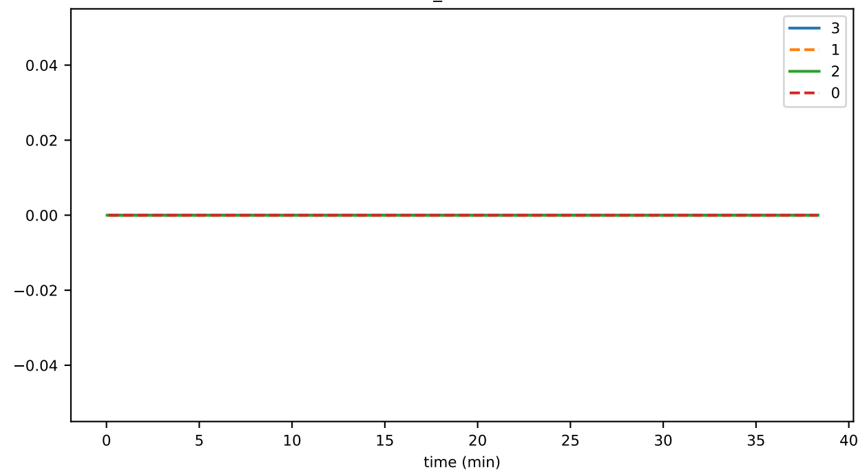
bufferedPriorityTransactions
