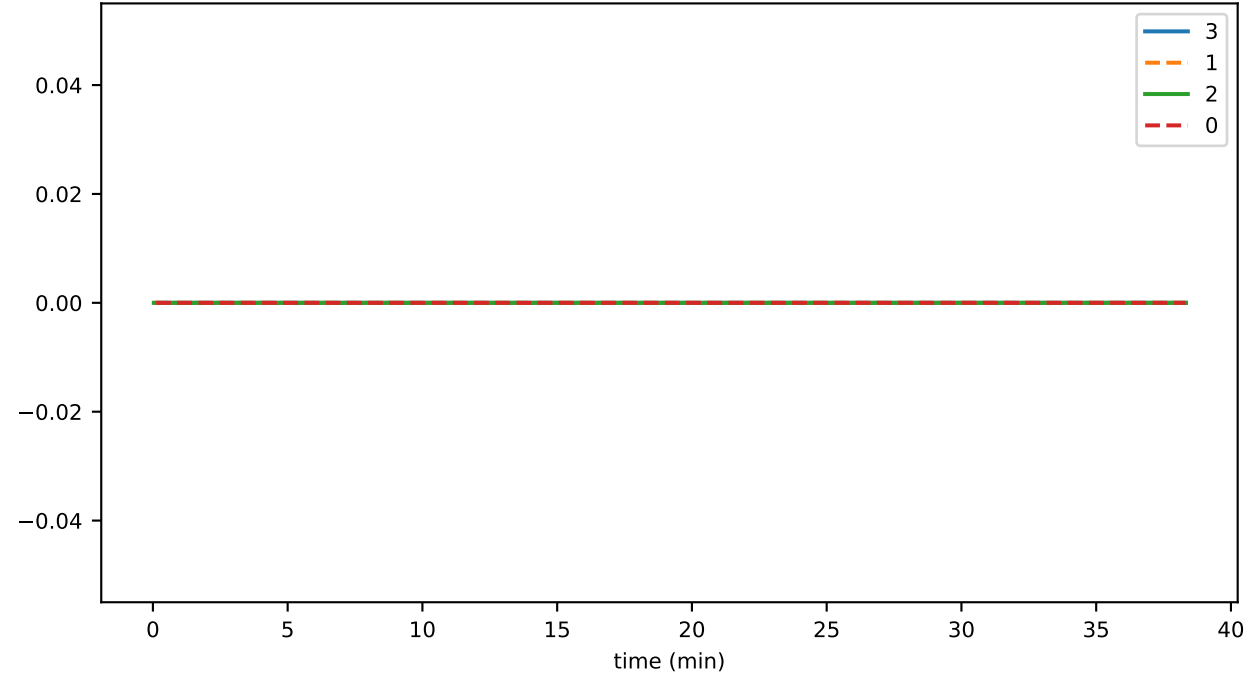
connRecv_endStream_error
