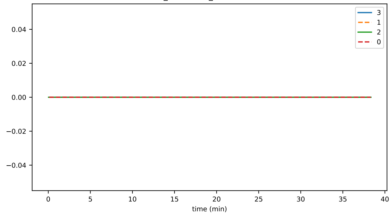
conn_connClose_newConnection
