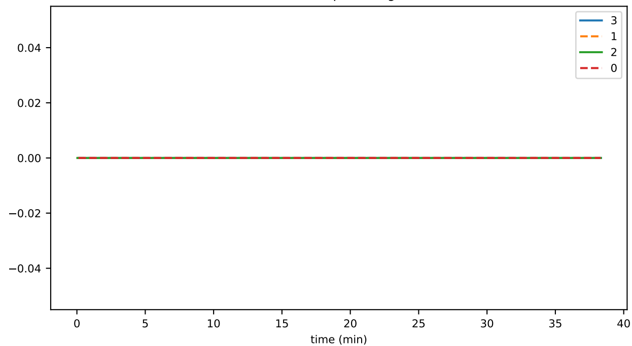
eventsWithDisparateSignature
