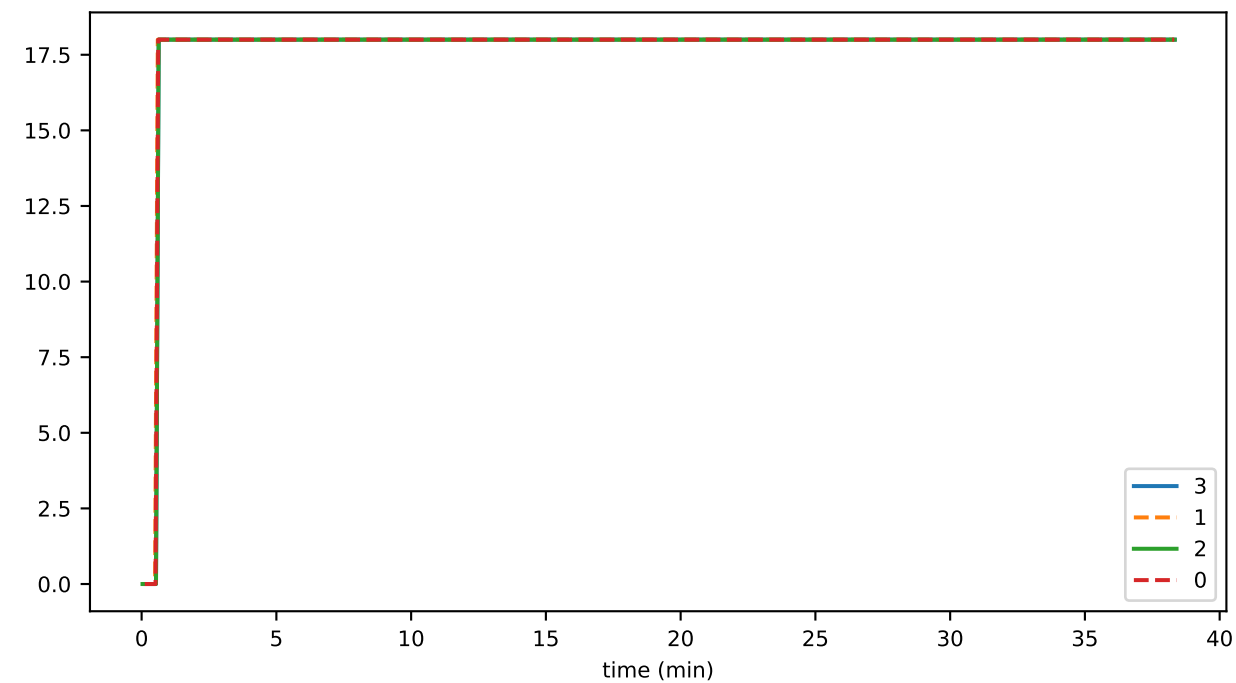
filesUsed
