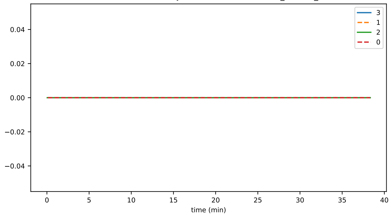
SmartContractService:SystemContractMethodCall_DIRECT_total
