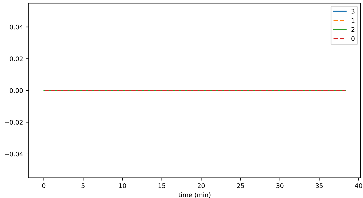
ds_files_hashesStoreFileCount_state
