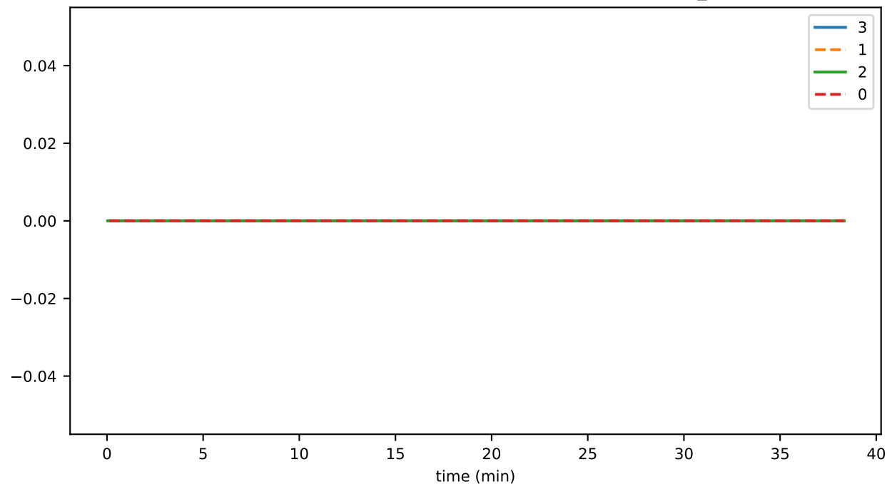
SmartContractService:SuccessfulTransactionDuration_avg
