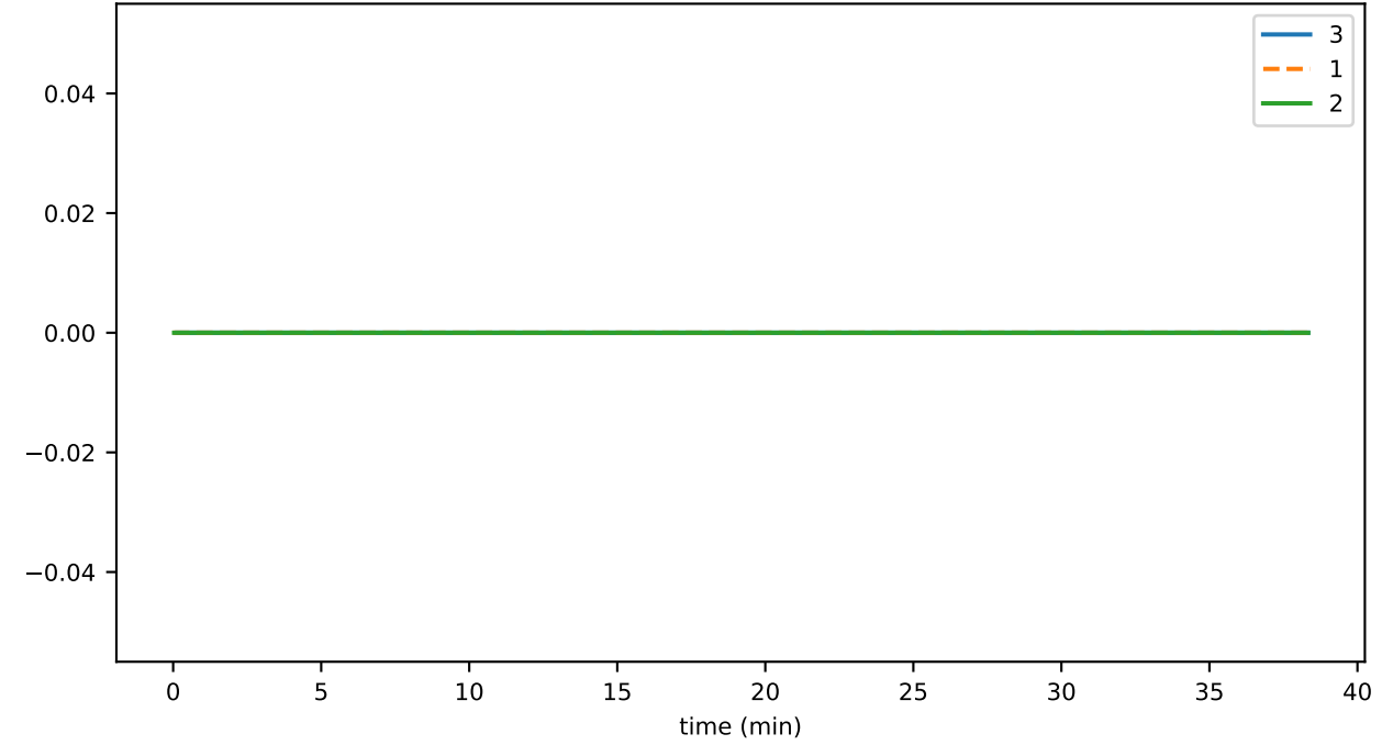
disconnects_per_sec_00
