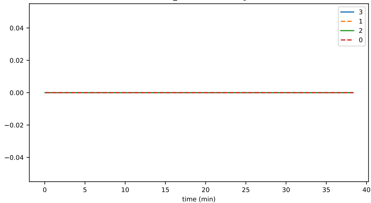
buffer_numBlocksMissing
