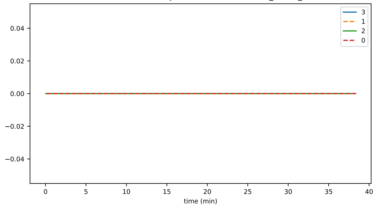
SmartContractService:SystemContractMethodCall_ERC20_failed
