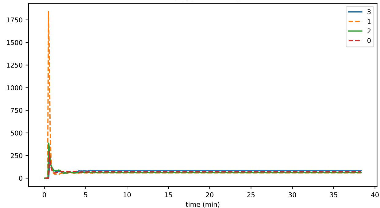
eventDelay_4_verification_storage
