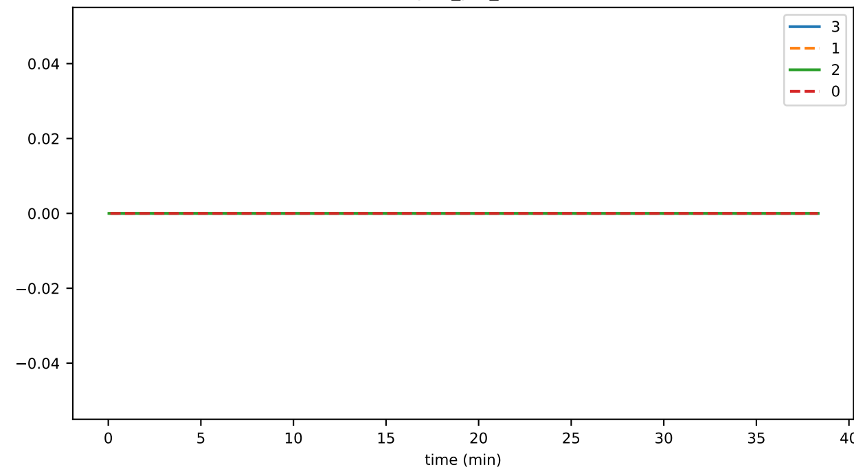
SmartContractService:FailedTransactionDuration_avg
