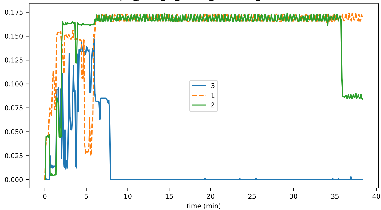
sync_phase_00_fraction_RECEIVING_EVENTS
