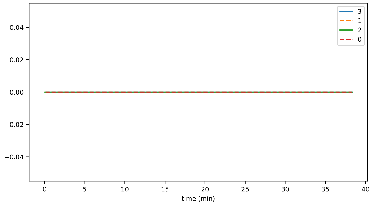
connRecv_resendBlock
