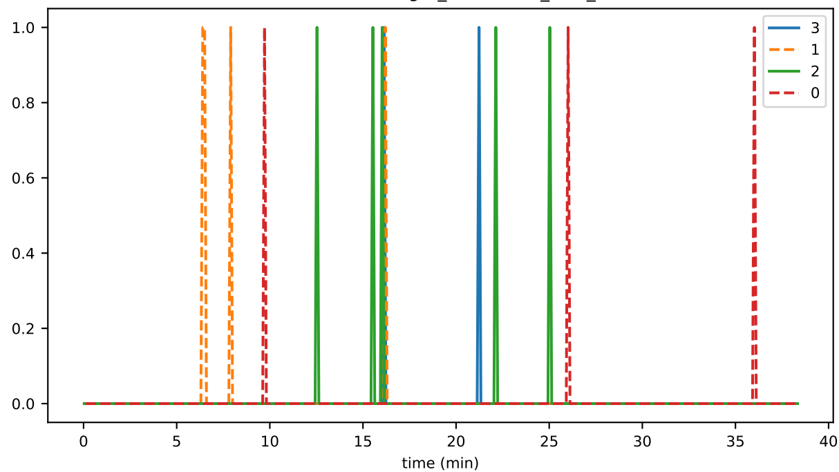
EventManager_unhandled_task_count
