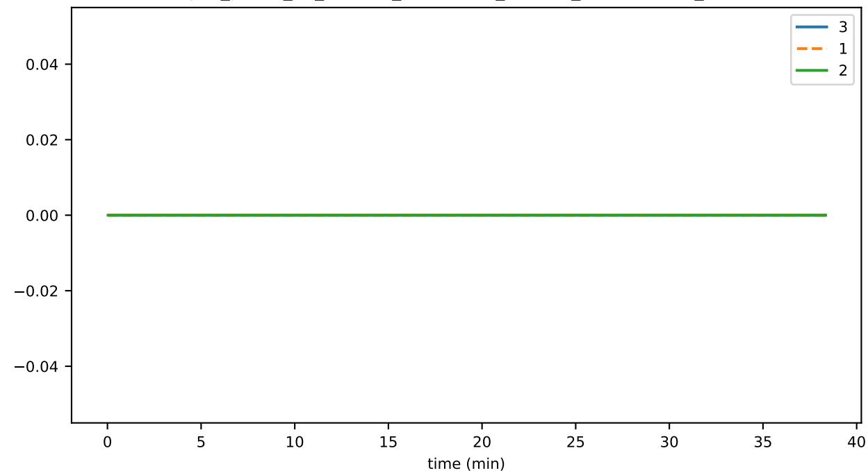
sync_phase_00_fraction_SELF_FALLEN_BEHIND
