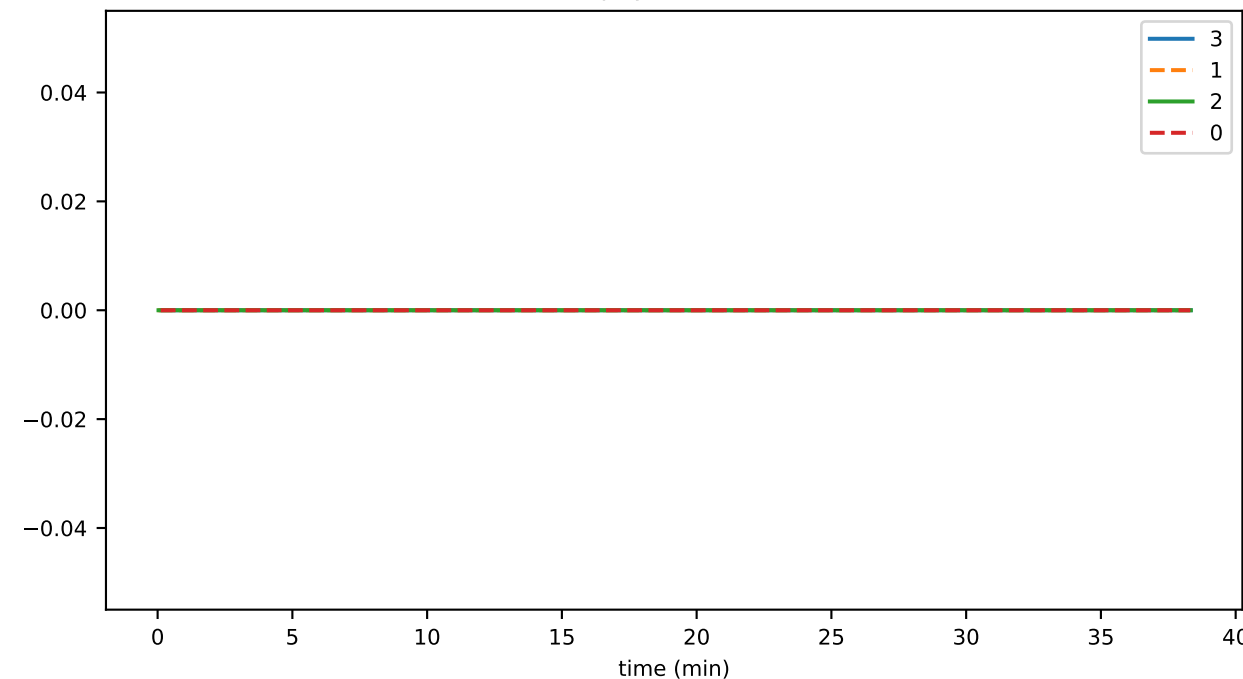
PlatformStatus
