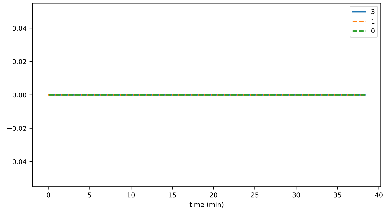
sync_phase_02_fraction_OTHER_FALLEN_BEHIND
