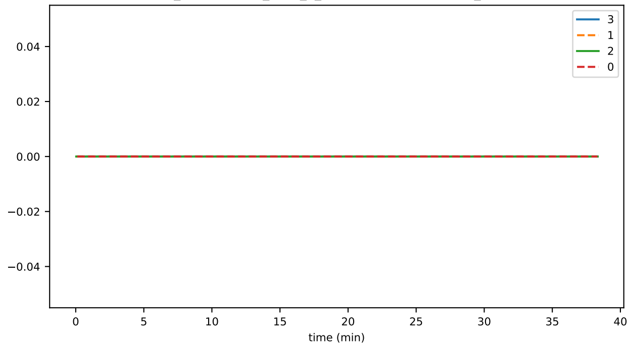
ds_compactions_level_5_leafKeysSavedSpaceMb_state
