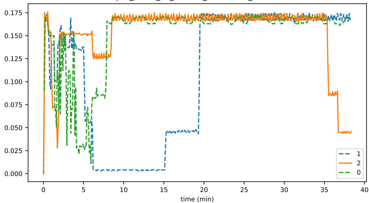
sync_phase_03_fraction_RECEIVING_EVENTS
