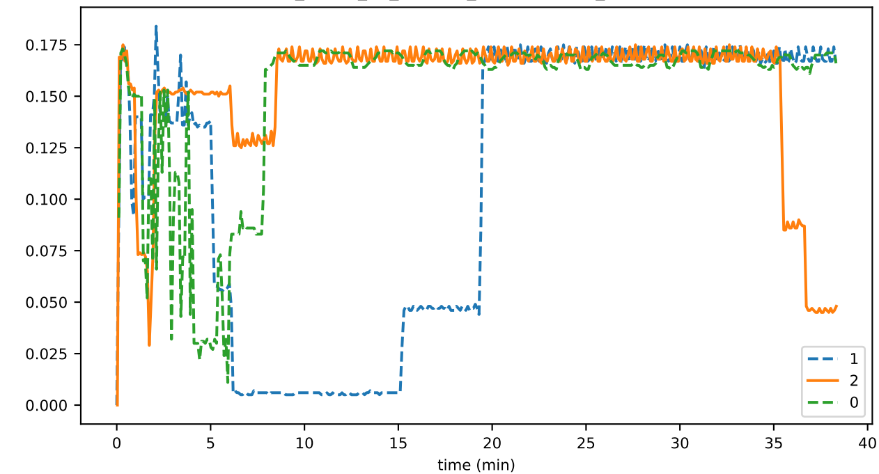
sync_phase_03_fraction_EXCHANGING_WINDOWS
