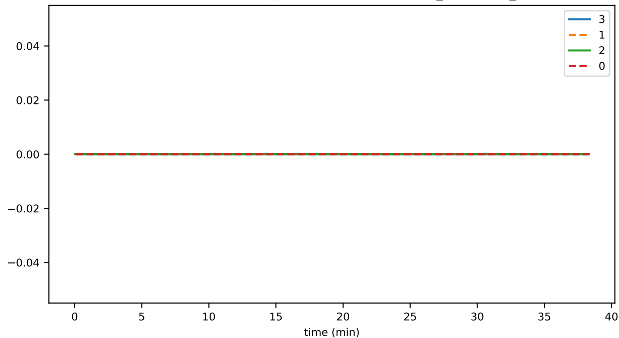
SmartContractService:SystemContractMethodCall_ASSOCIATION_total
