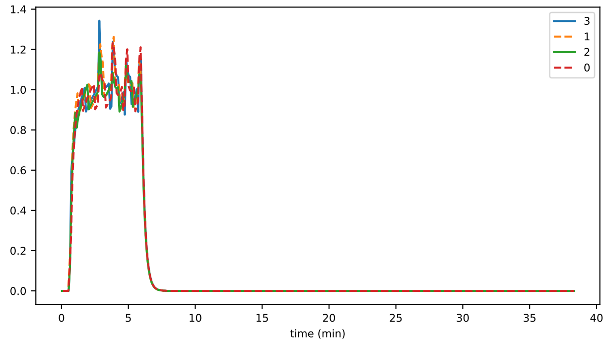
submittedPlatformTransactions
