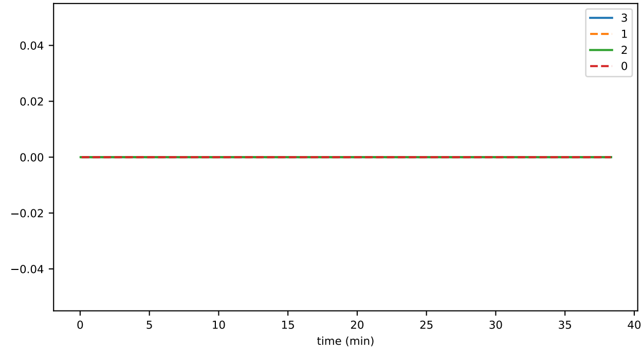
broadcastDisabledDueToLag
