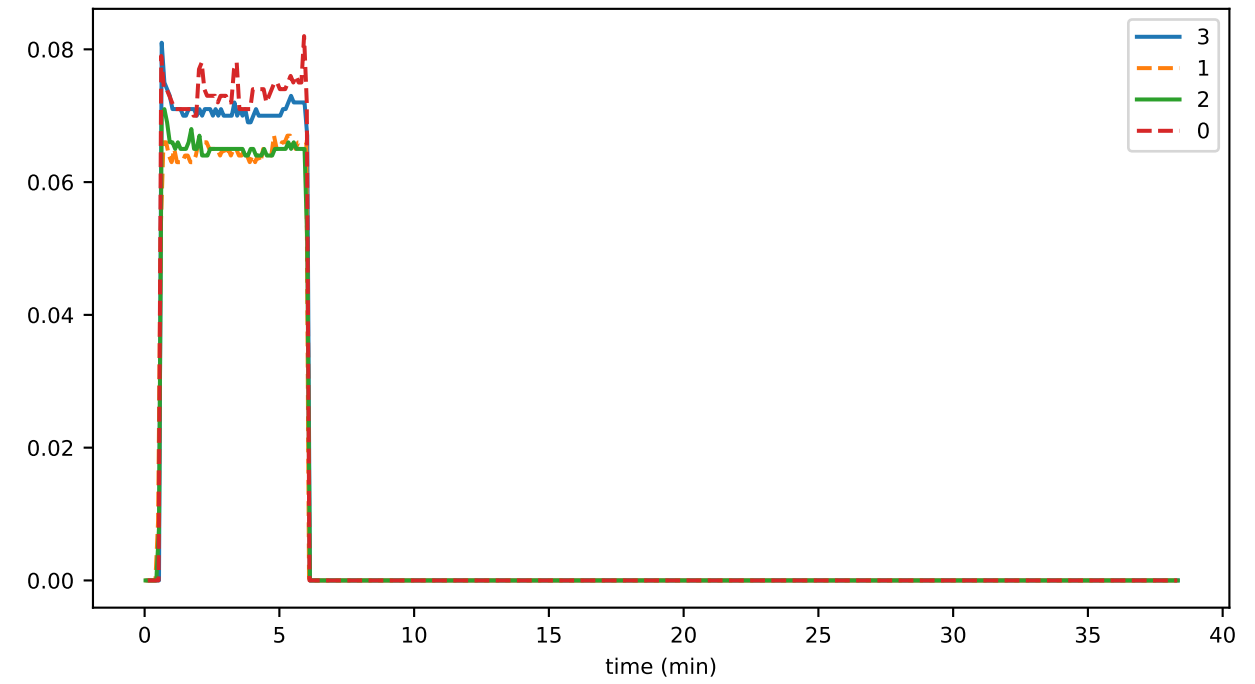
eventCreation_fraction_NO_ELIGIBLE_PARENTS
