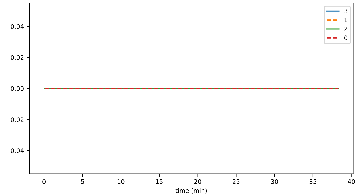
SmartContractService:Rejected_contractCallTx_total
