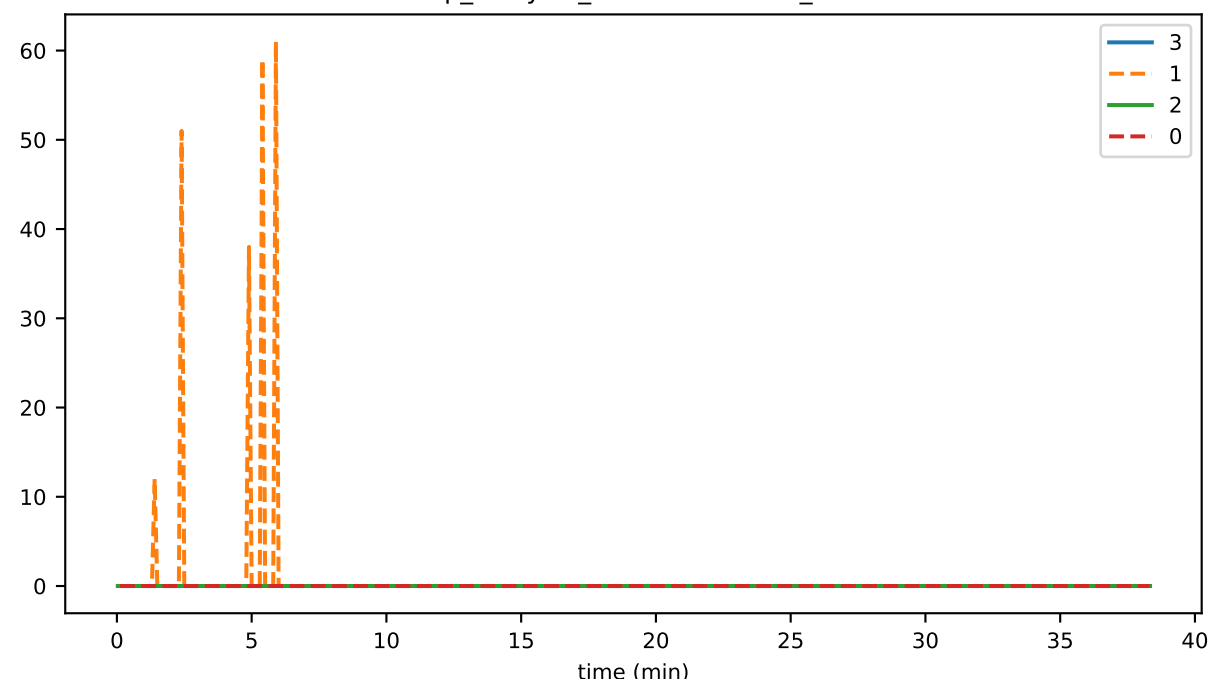
vmap_lifecycle_flushDurationMs_state
