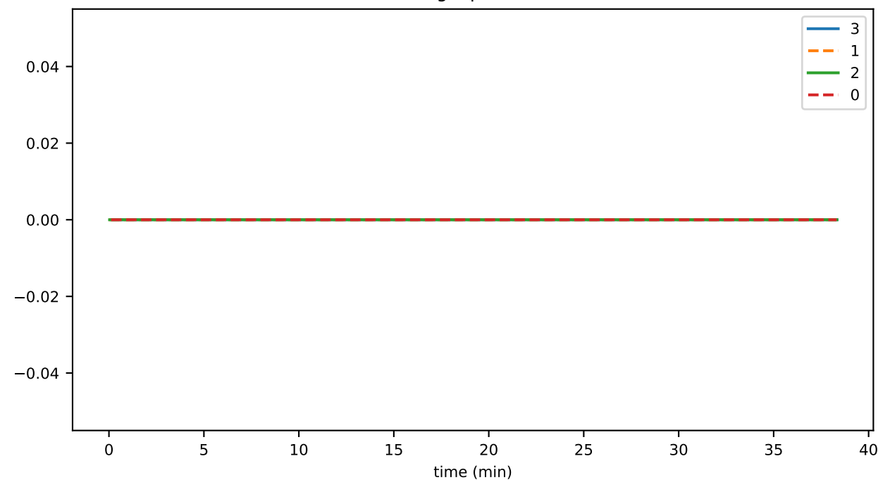
preconsensusEventAverageUnutilizedFileSpan
