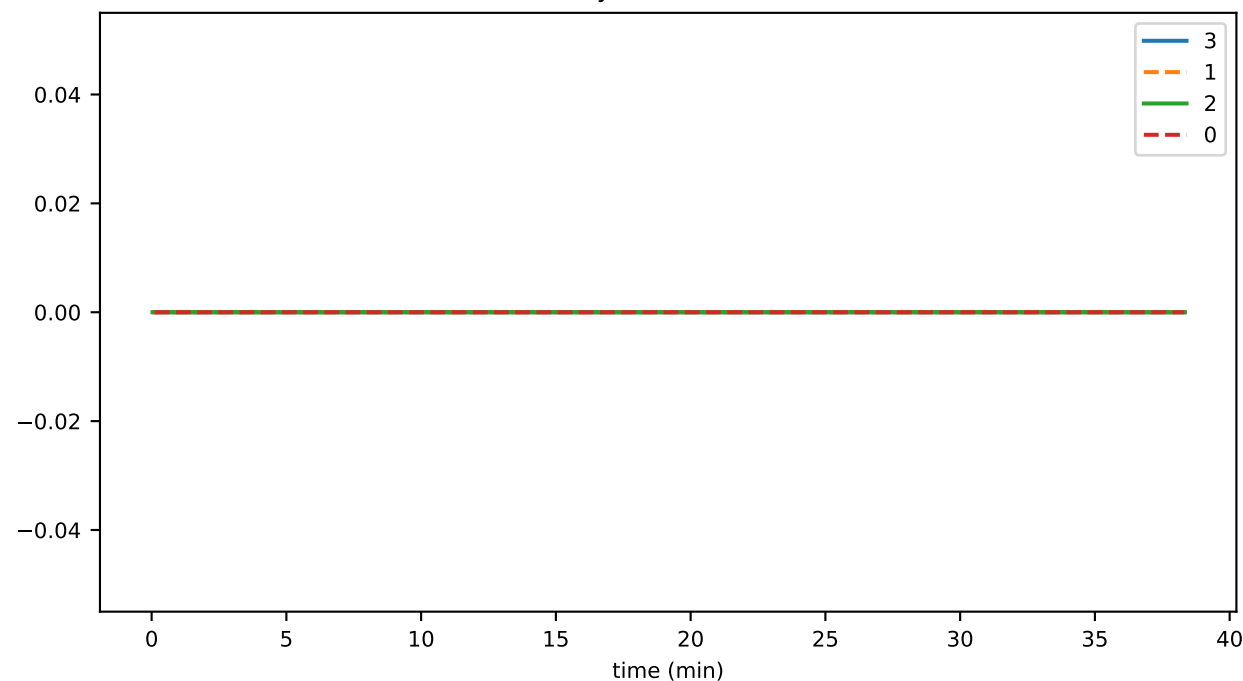
doNotSyncRemoteProcessingEvents
