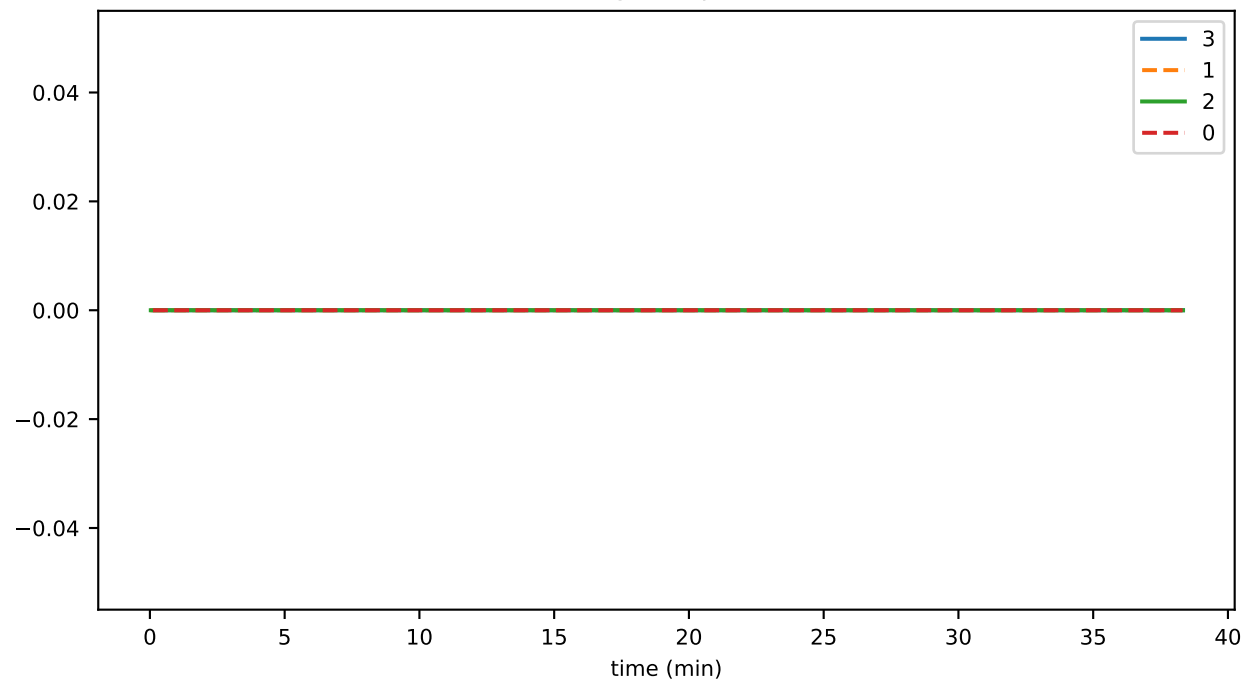
SigSpans_per_sec
