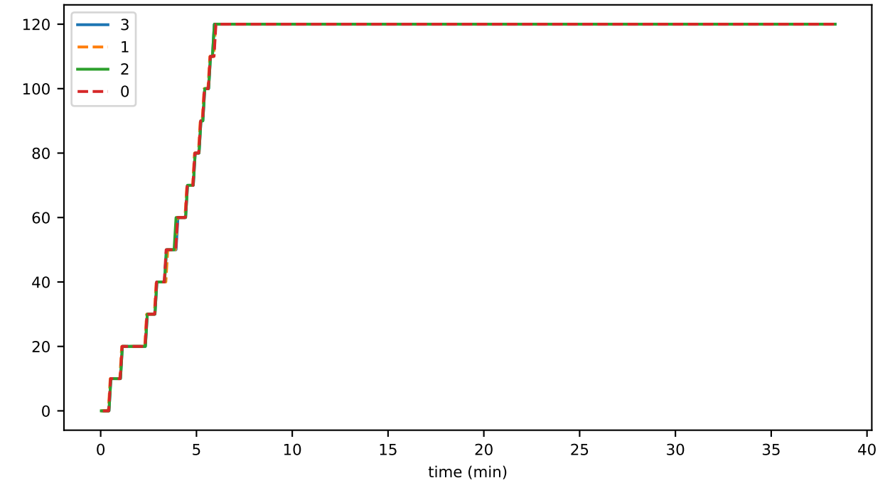
disconnects_per_sec_00
