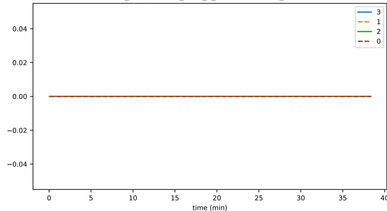
ds_compactions_level_4_leavesTimeMs_state
