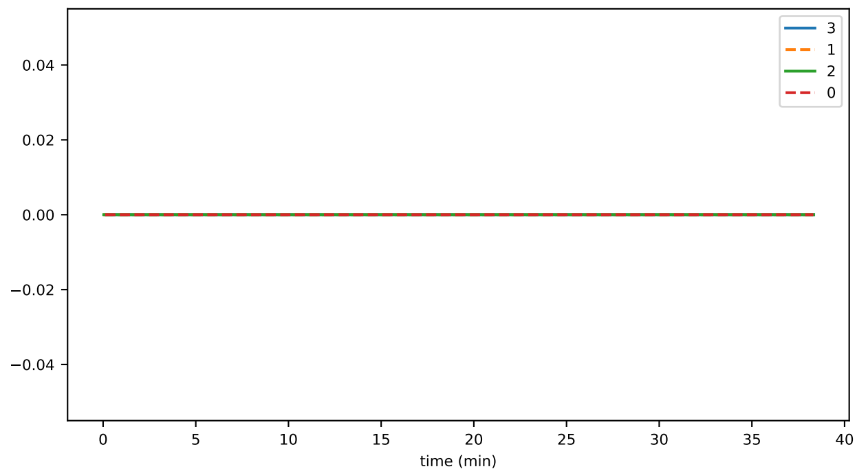
eventsWithInvalidParents
