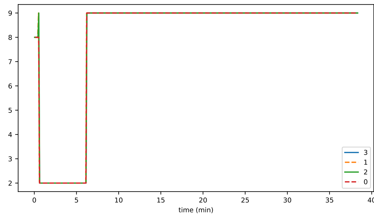
PlatformStatus
