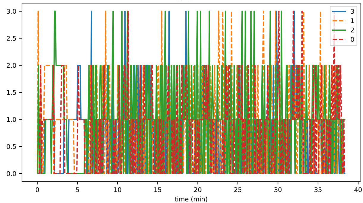
syncs_in_progress
