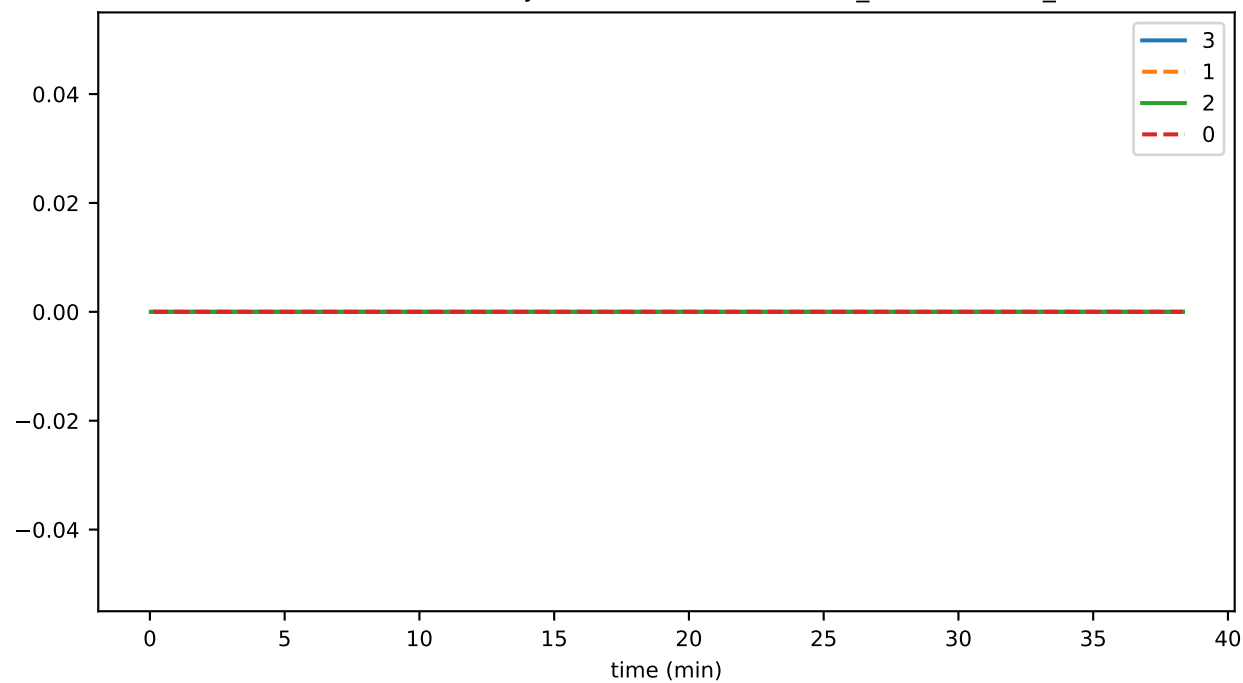
SmartContractService:SystemContractMethodCall_ASSOCIATION_total
