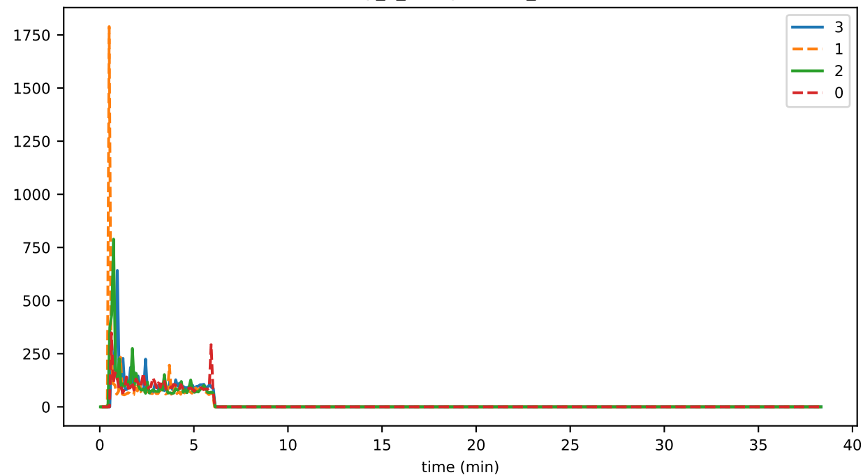
eventDelay_3_deduplication_storageMAX
