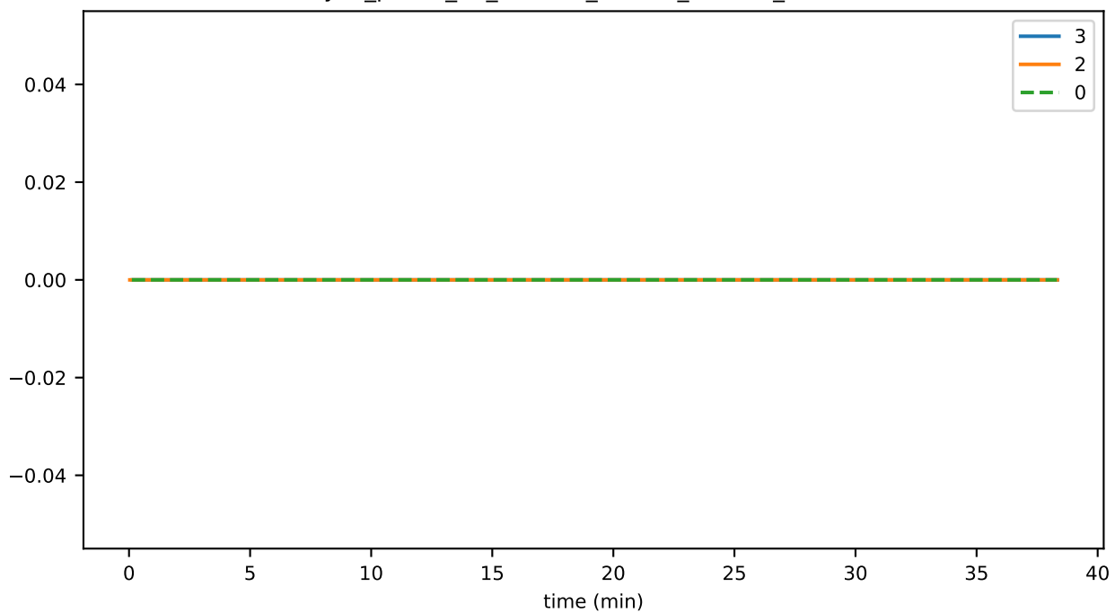
sync_phase_01_fraction_OTHER_FALLEN_BEHIND
