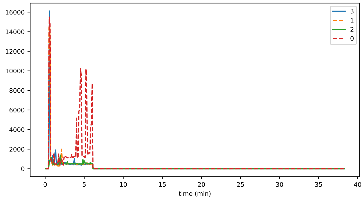
eventDelay_4_verification_runtimeMAX
