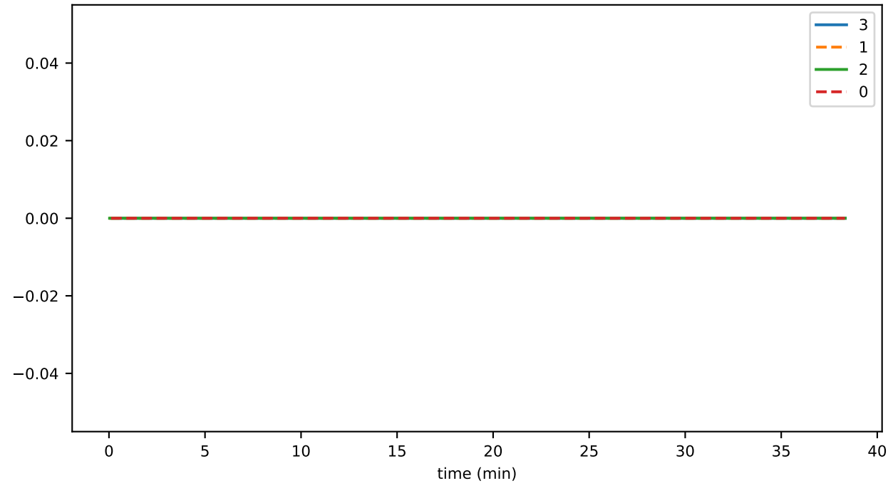
hapiFreeQueryLimitsPercentUsed
