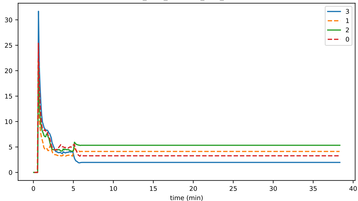
ConsensusEngine_unhandled_task_count
