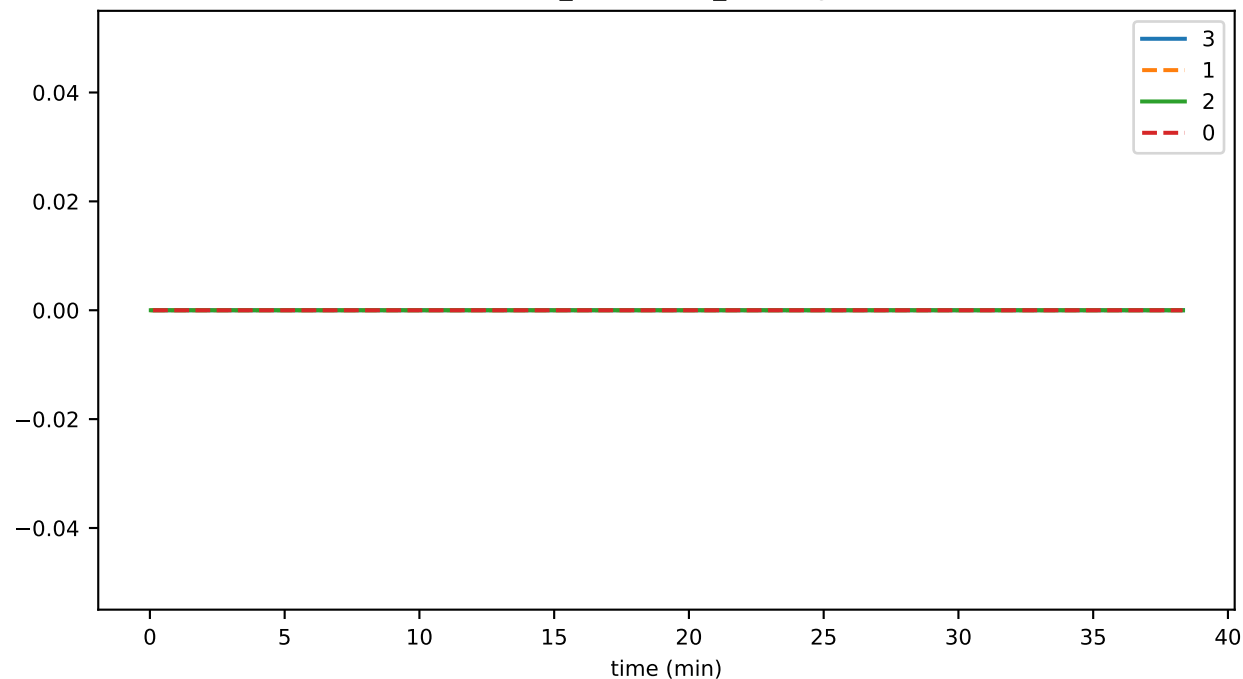
connSend_latestBlockEndOfBlock
