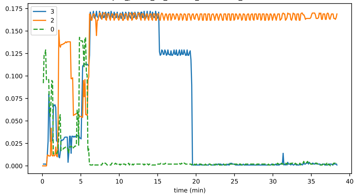
sync_phase_01_fraction_RECEIVING_EVENTS
