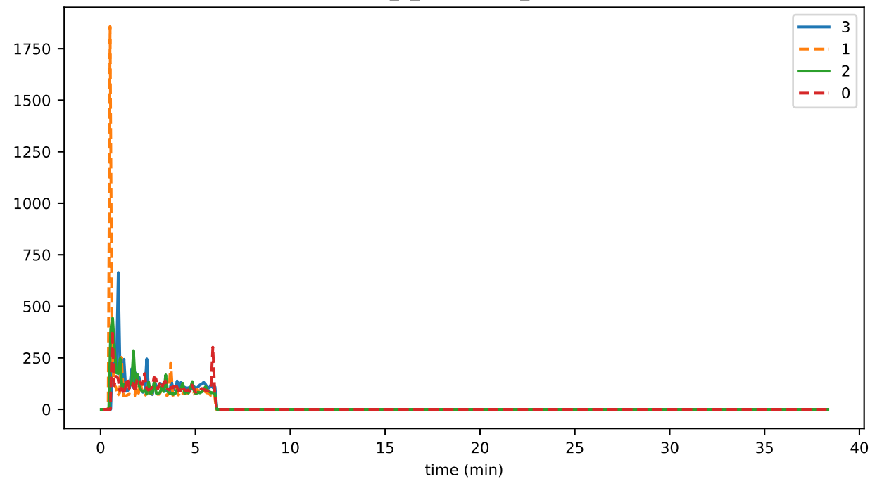
eventDelay_4_verification_runtimeMAX
