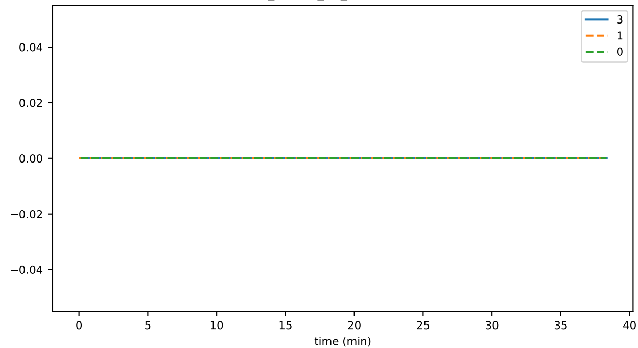
rpc_output_02_queueMinSize
