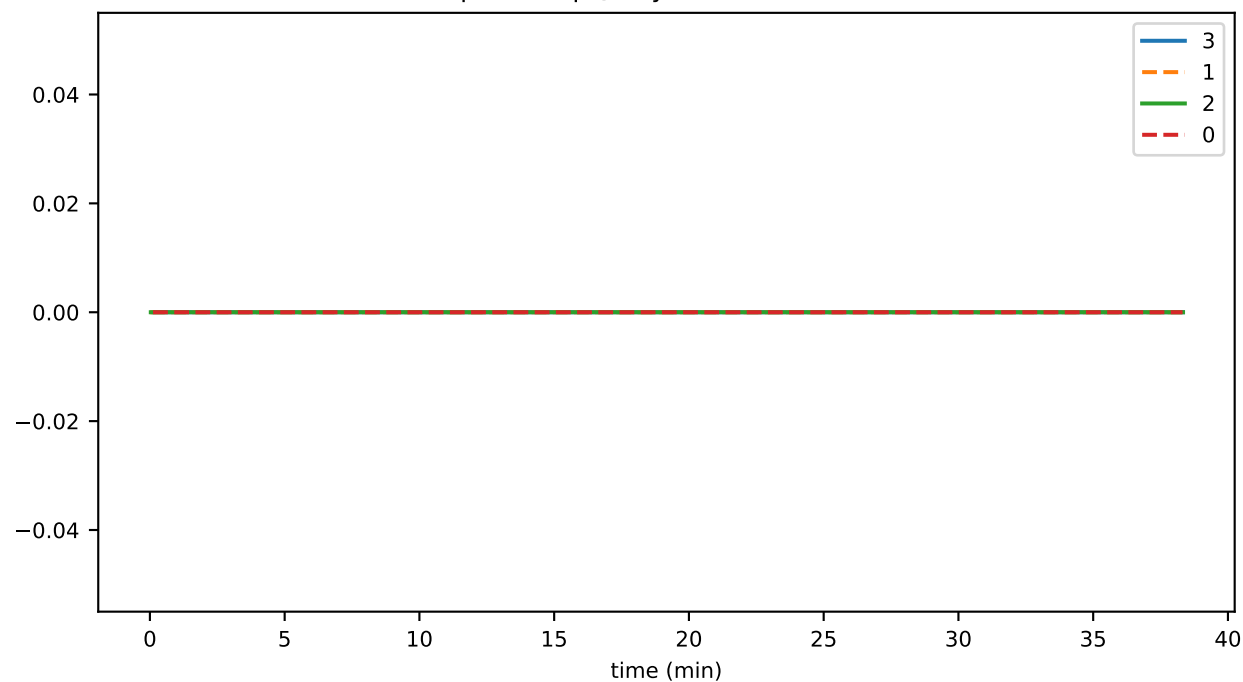
hasFallenBehind
