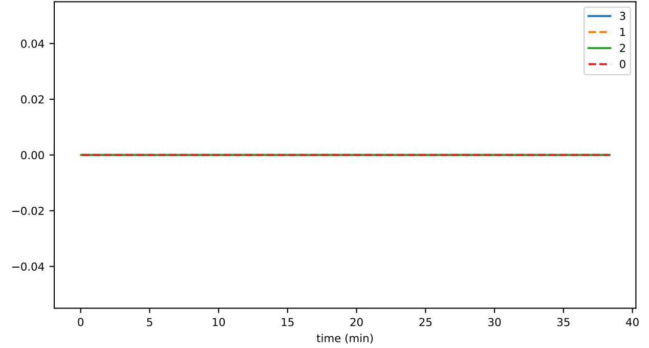
connRecv_endStream_invalidRequest
