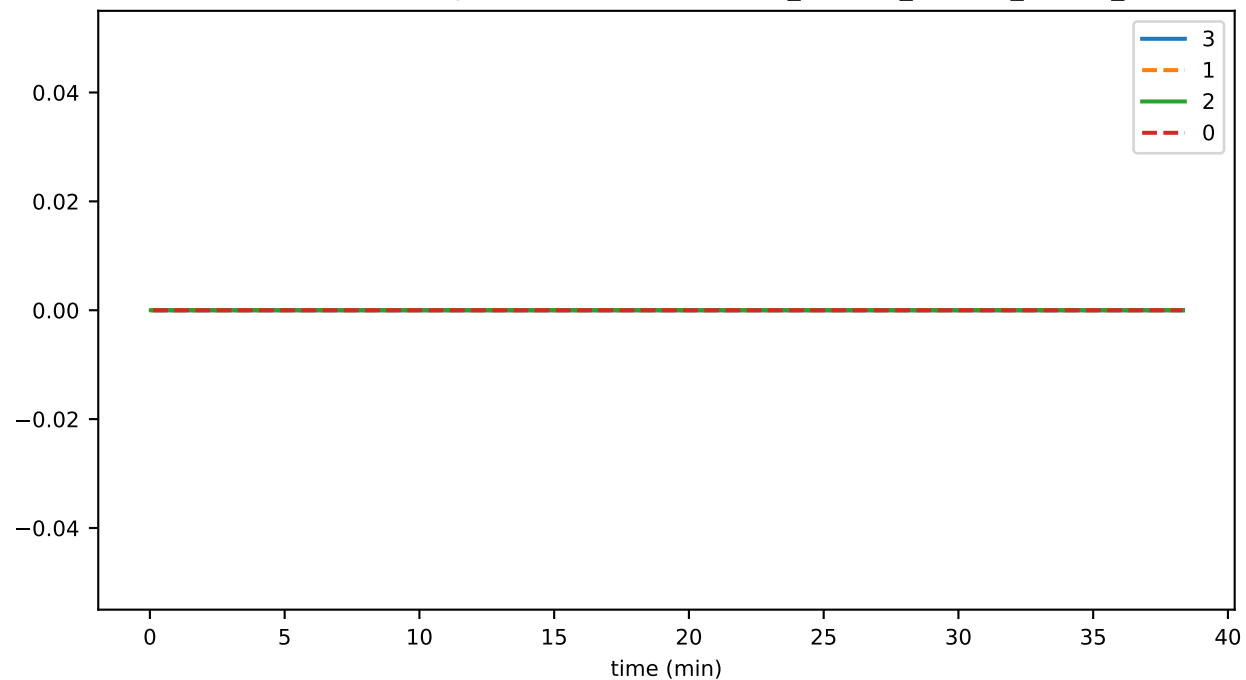
SmartContractService:SystemContractMethodCall_DIRECT_total
