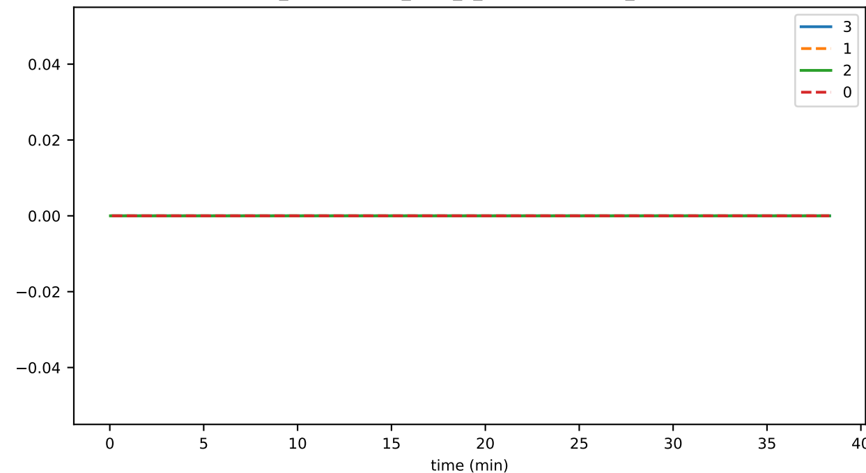
ds_compactions_level_0_leafKeysTimeMs_state
