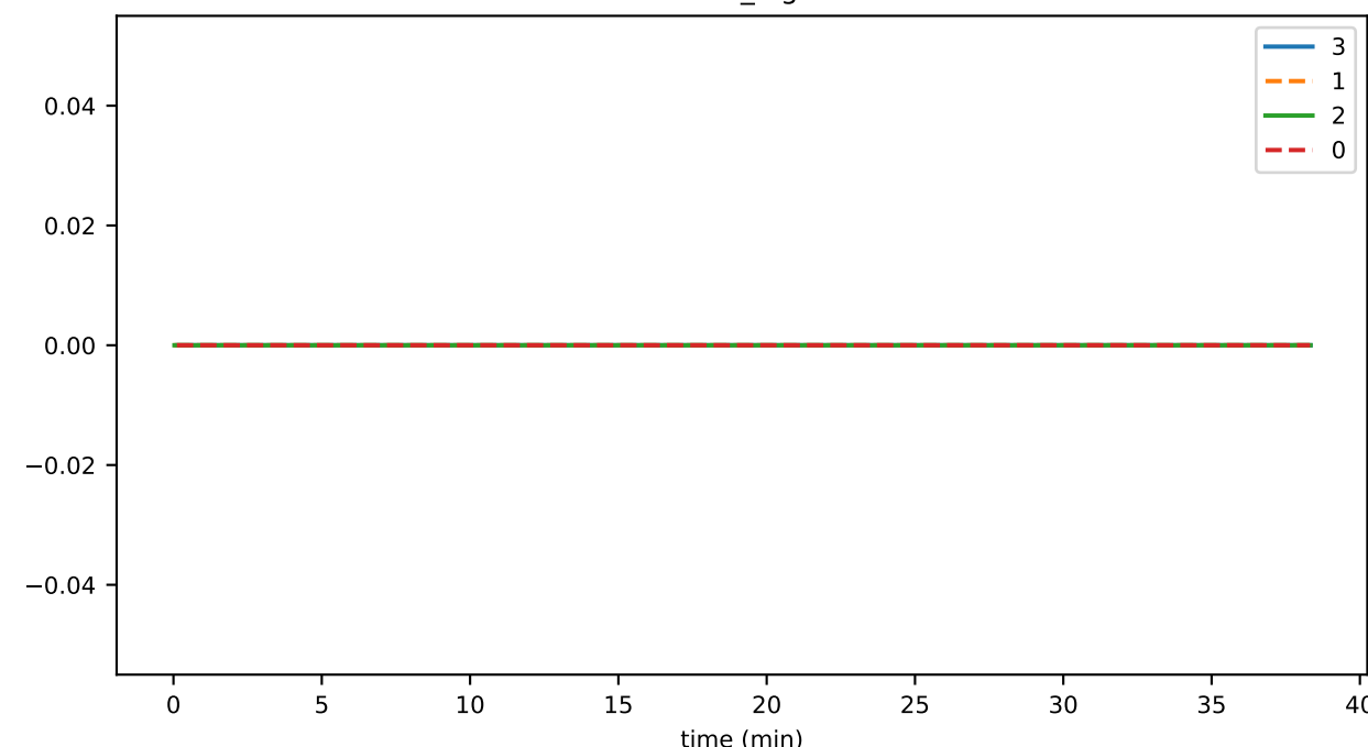
recordHashes_highestBlock
