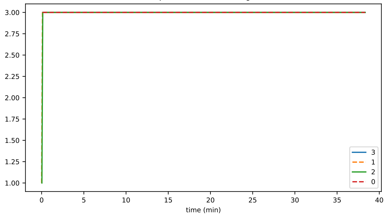
rpcWriteThreadRunning
