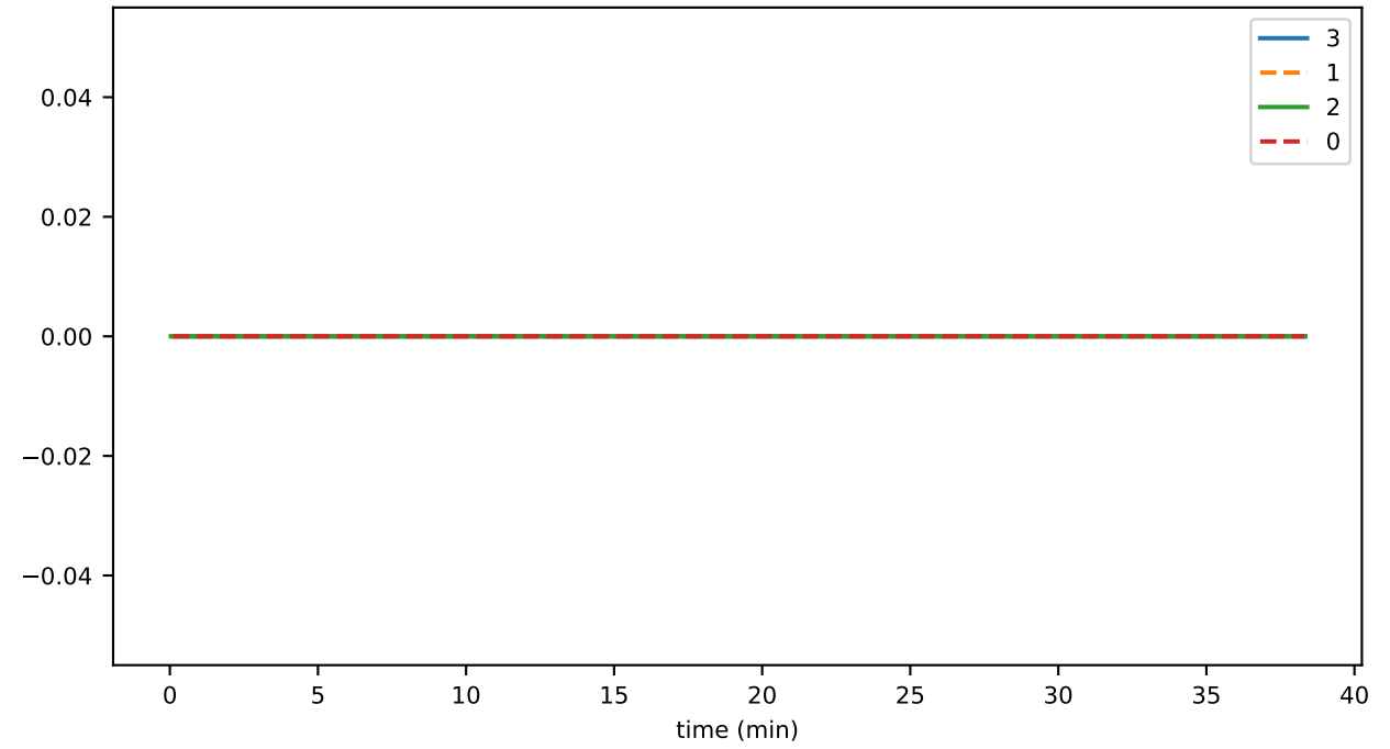
averageTimeToFullySignState
