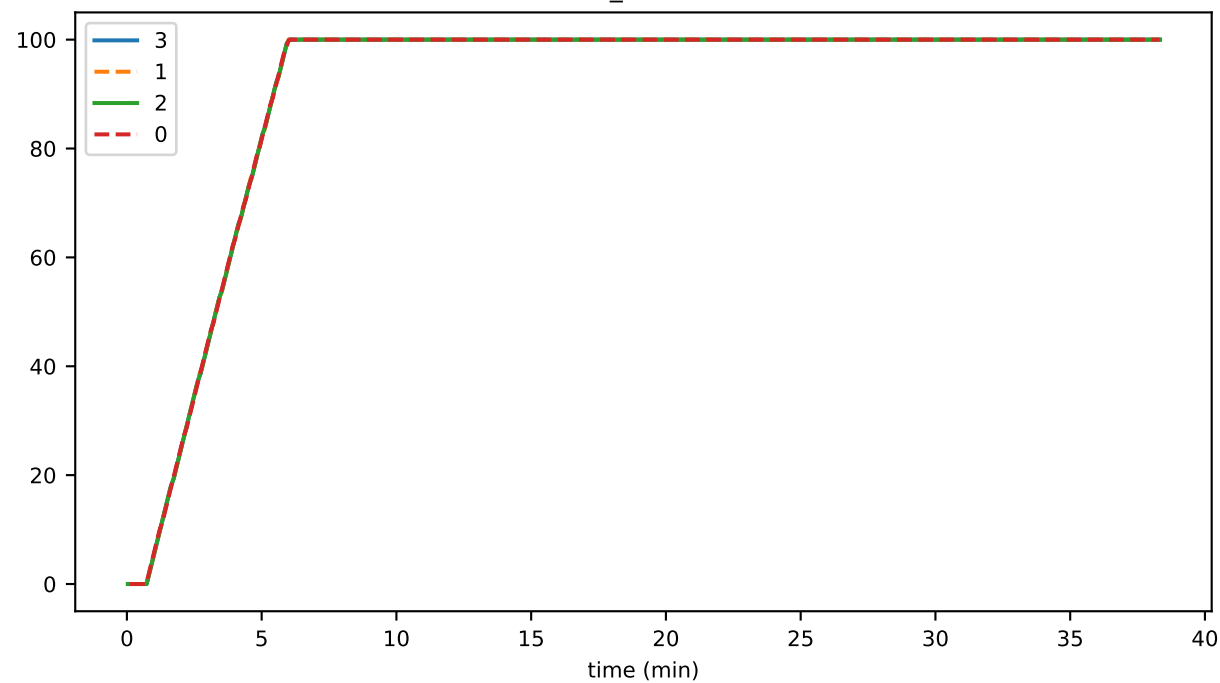
buffer_saturation
