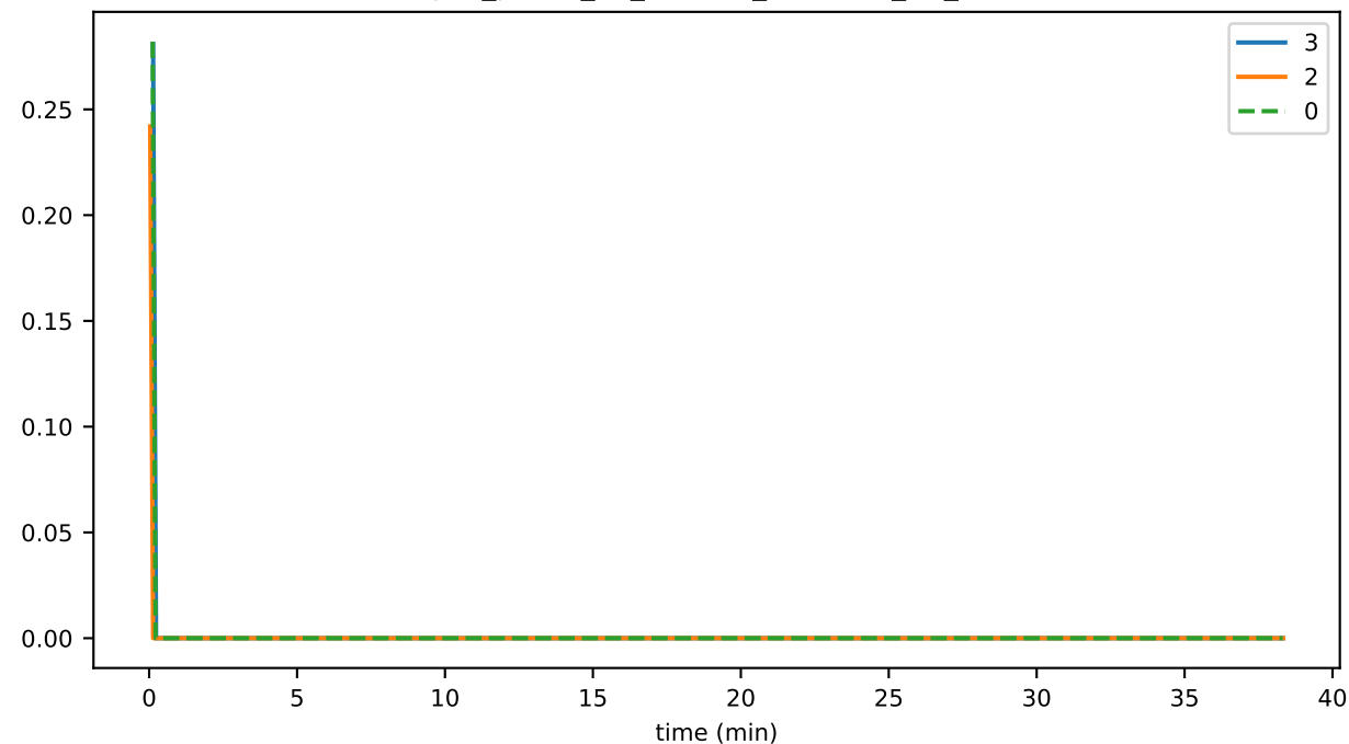
sync_phase_01_fraction_RECEIVING_EVENTS
