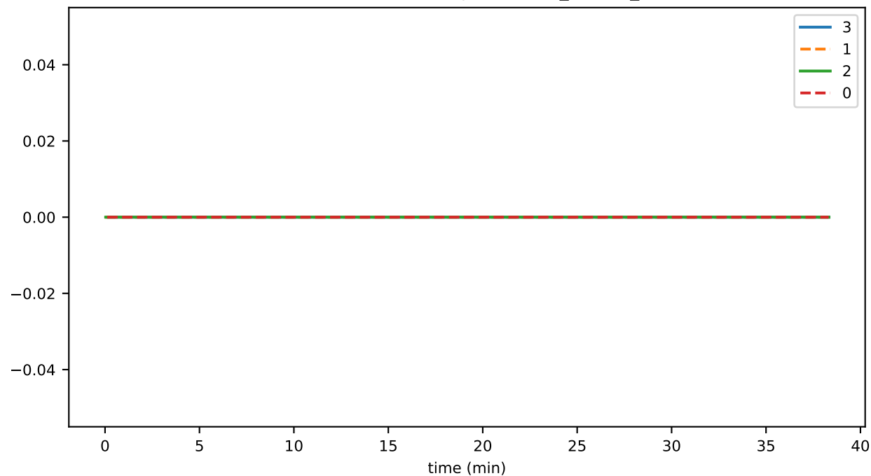
SmartContractService:OpsDuration_TxnsThrottled
