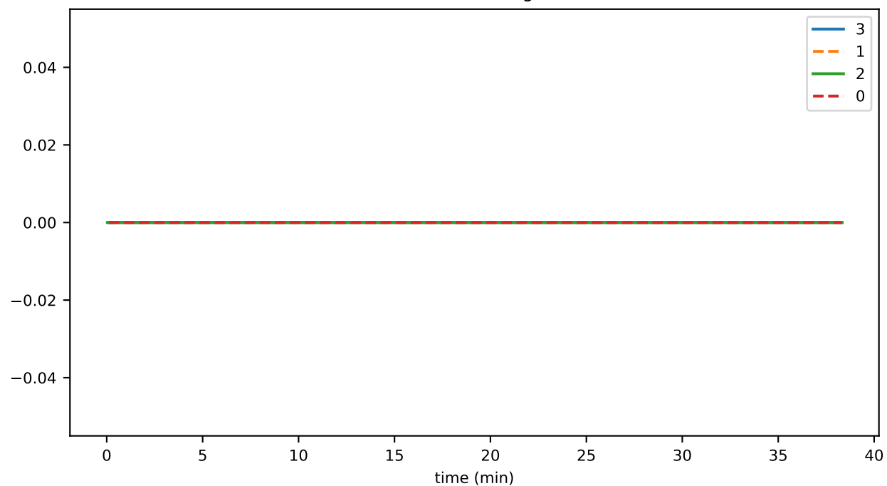
branchingEvents
