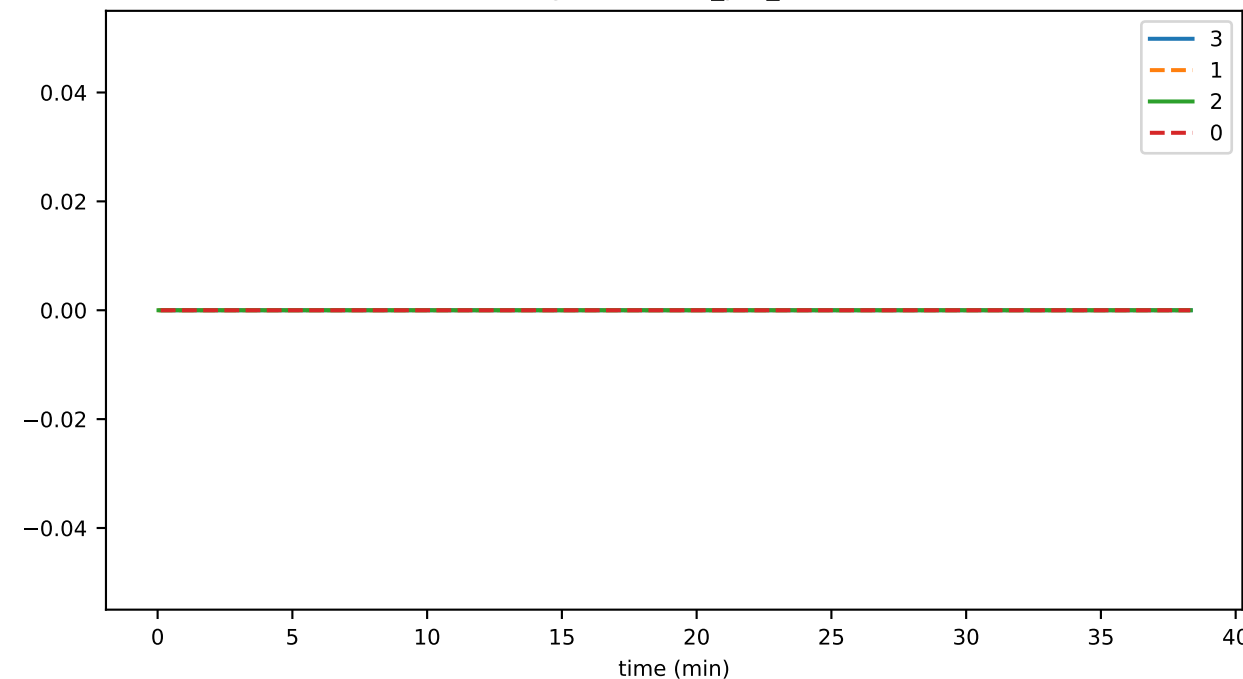
SigIntakeQueueDepth
