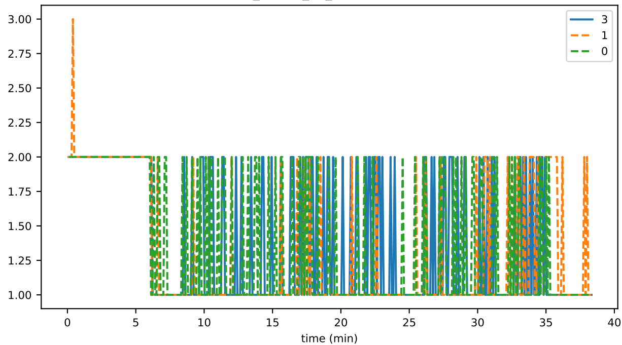
rpc_output_02_queueMaxSize
