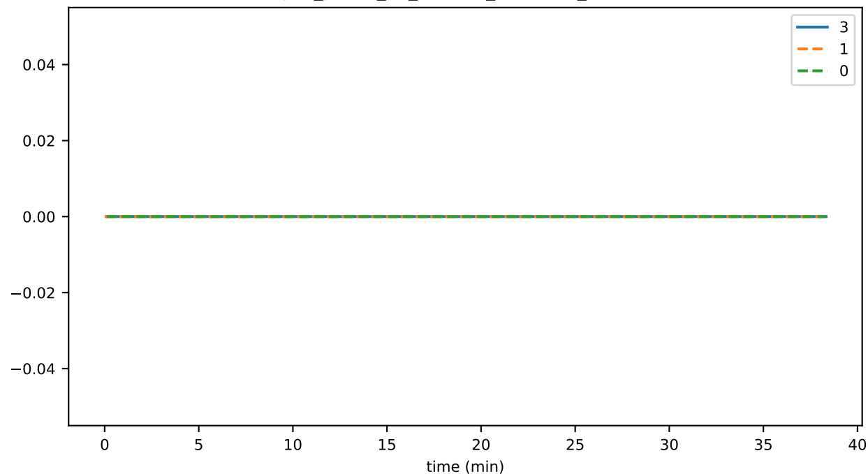
sync_phase_03_fraction_EXCHANGING_TIPS
