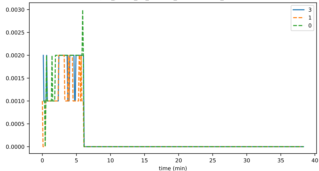
sync_phase_02_fraction_EXCHANGING_WINDOWS
