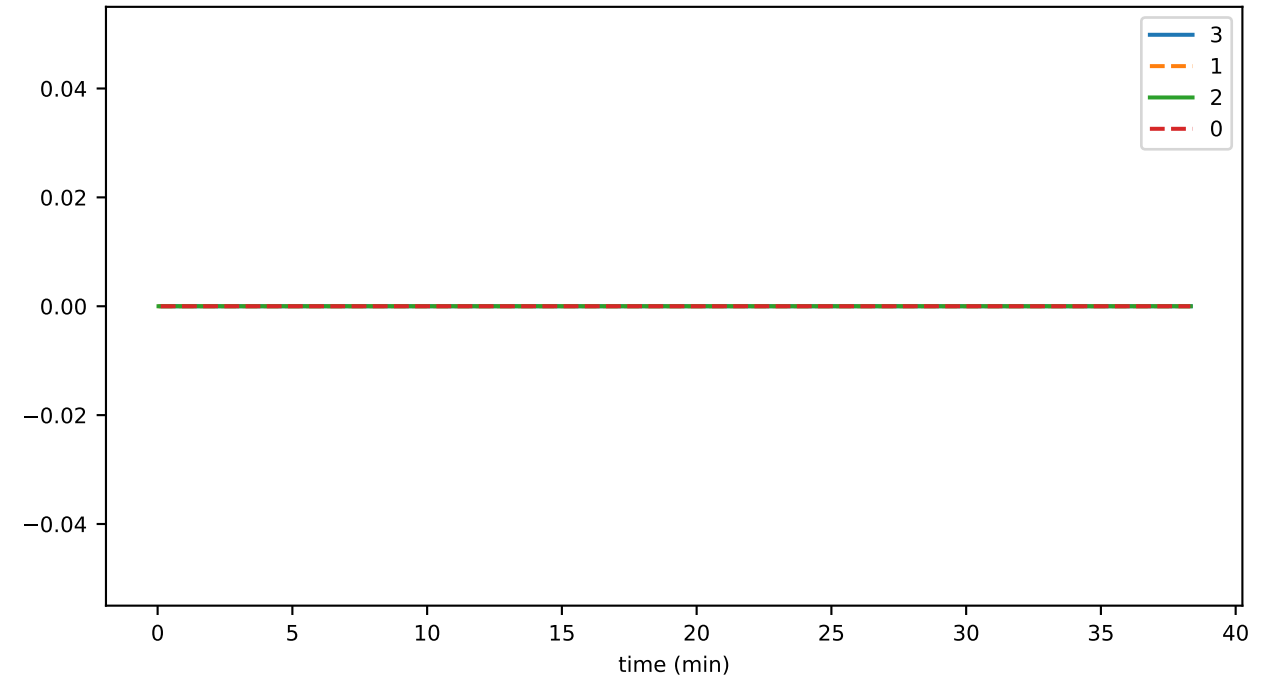
sstatesSigned_per_sec
