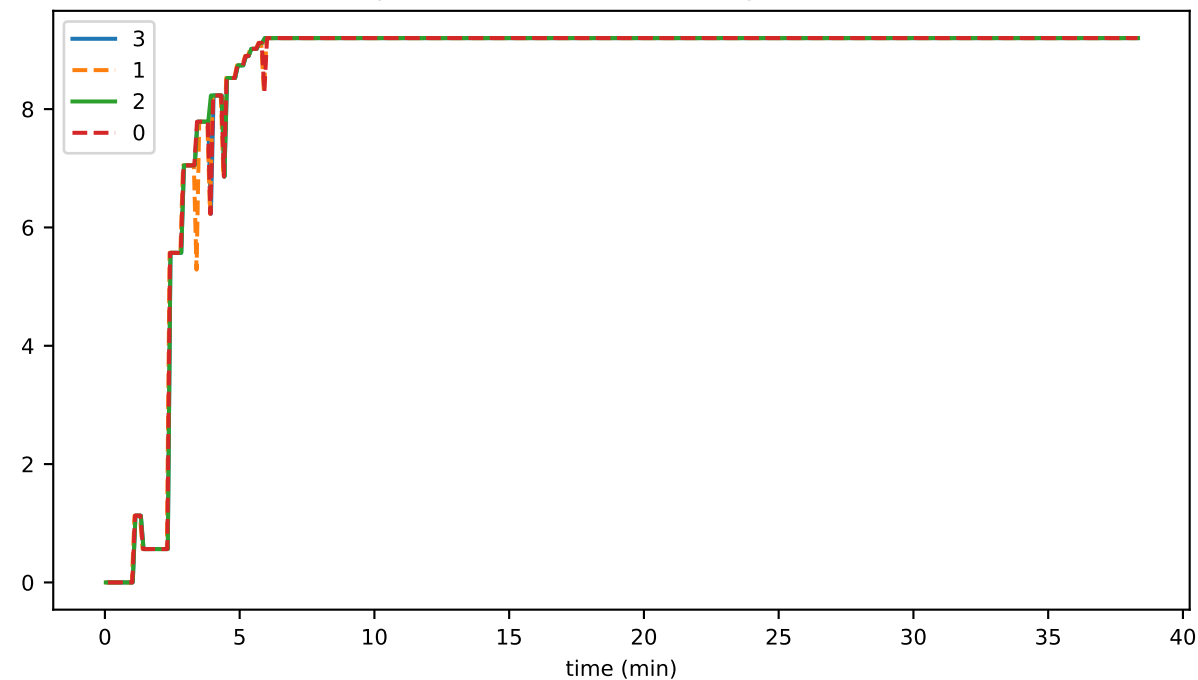
preconsensusEventFileOldestIdentifier
