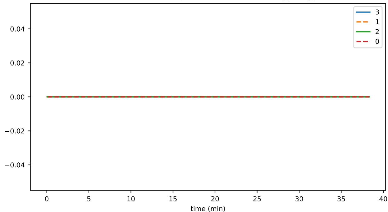
SmartContractService:TransactionDuration_count
