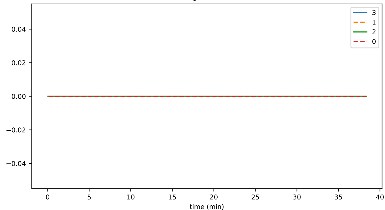
sync_per_secC
