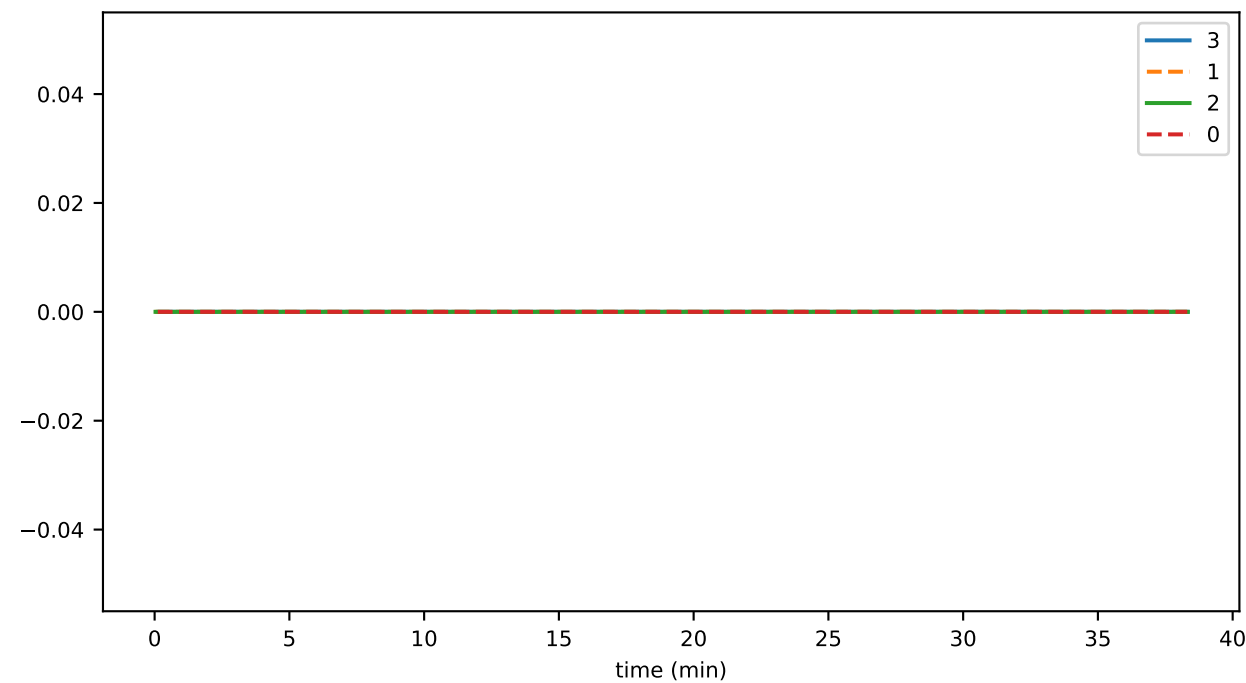
eventsWithNullFields
