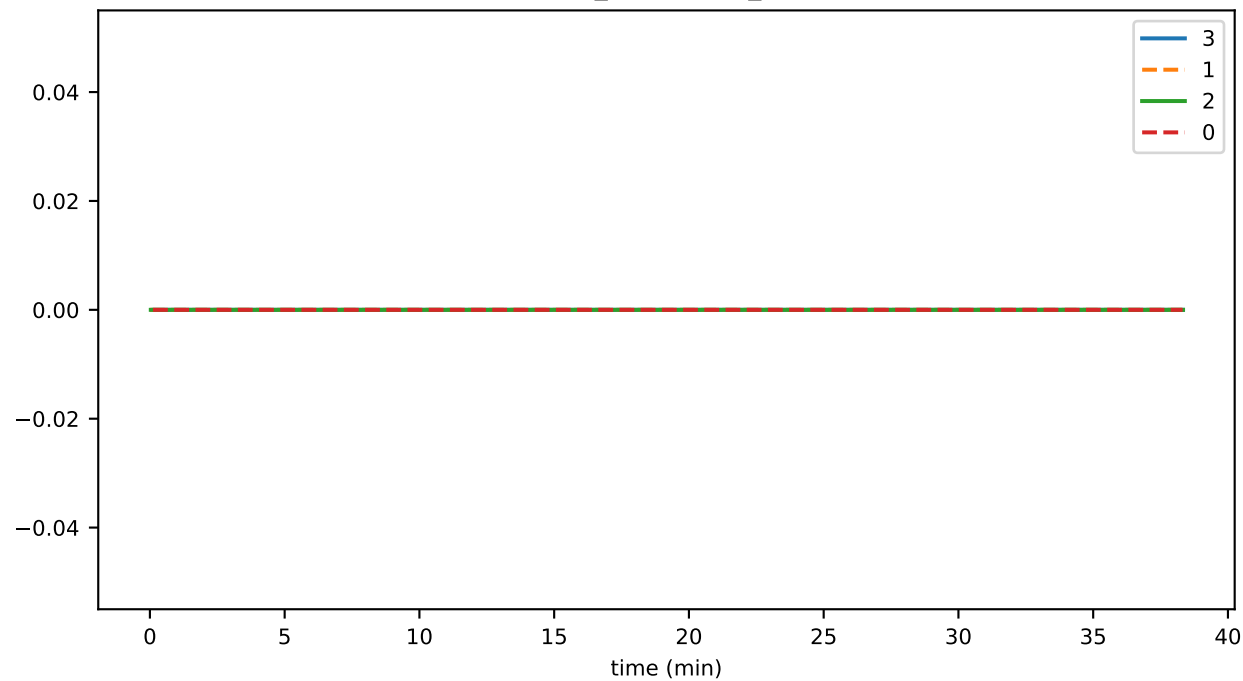
connRecv_endStream_timeout
