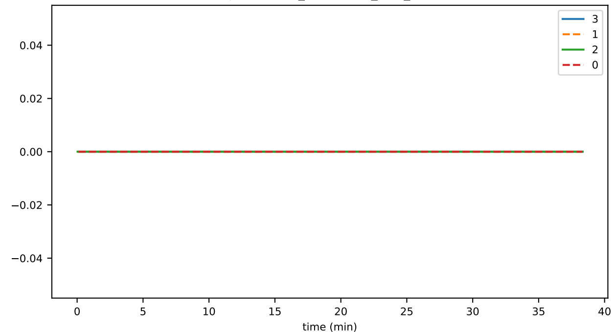
outgoingSyncRequests_per_sec
