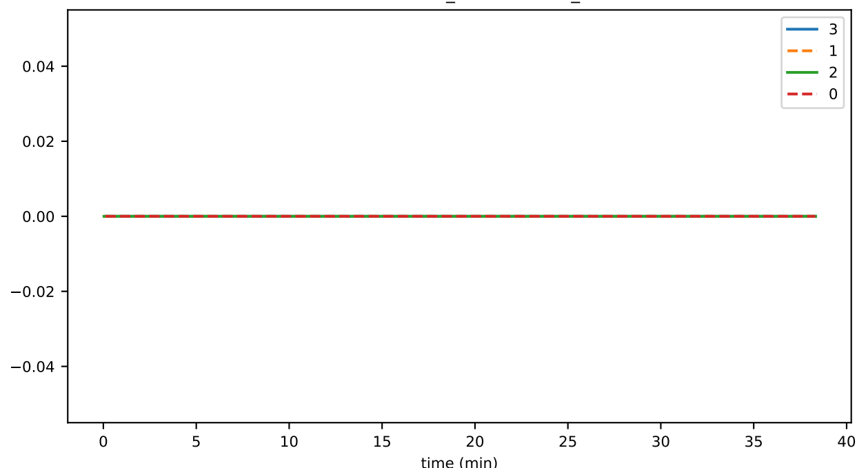
futureEventBuffer_eventCreator_count
