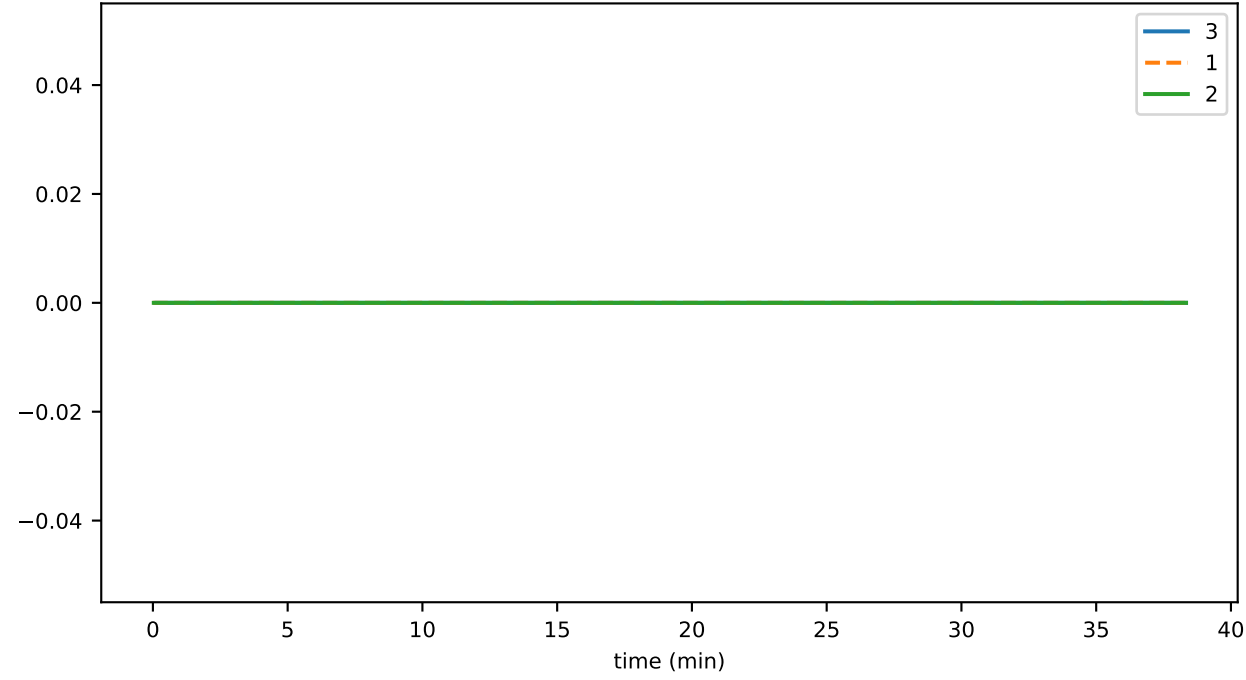
reconnectRejections_per_sec_00
