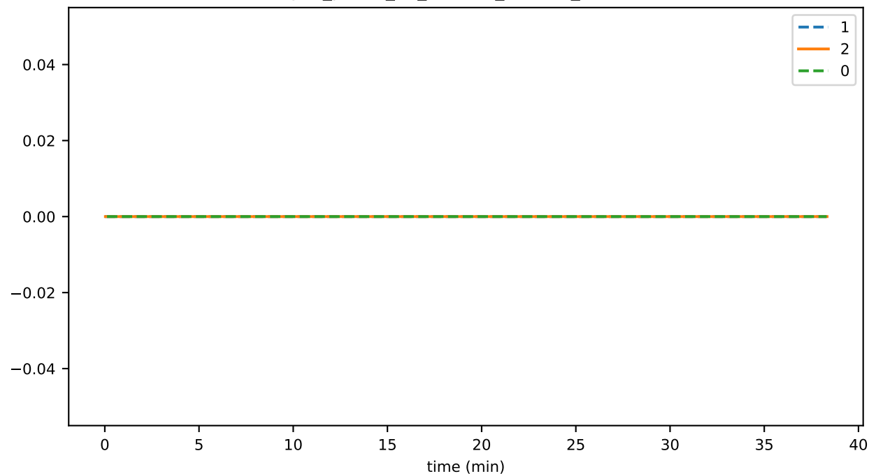
sync_phase_03_fraction_NO_PERMIT
