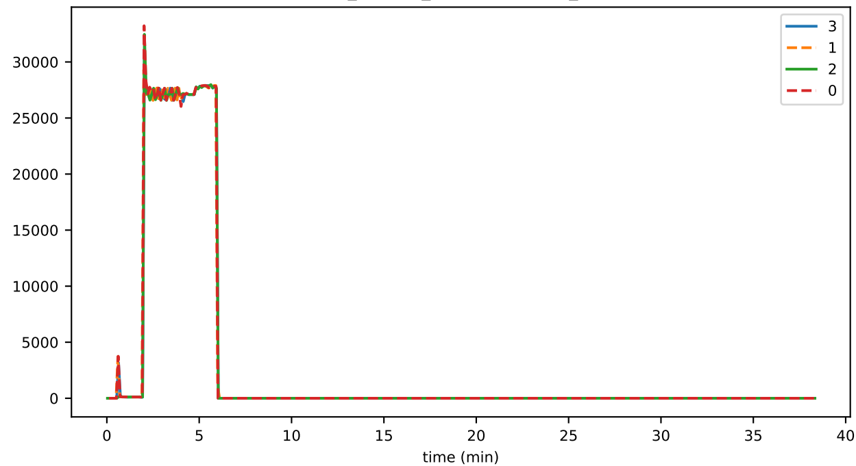
vmap_queries_updatedEntities_state
