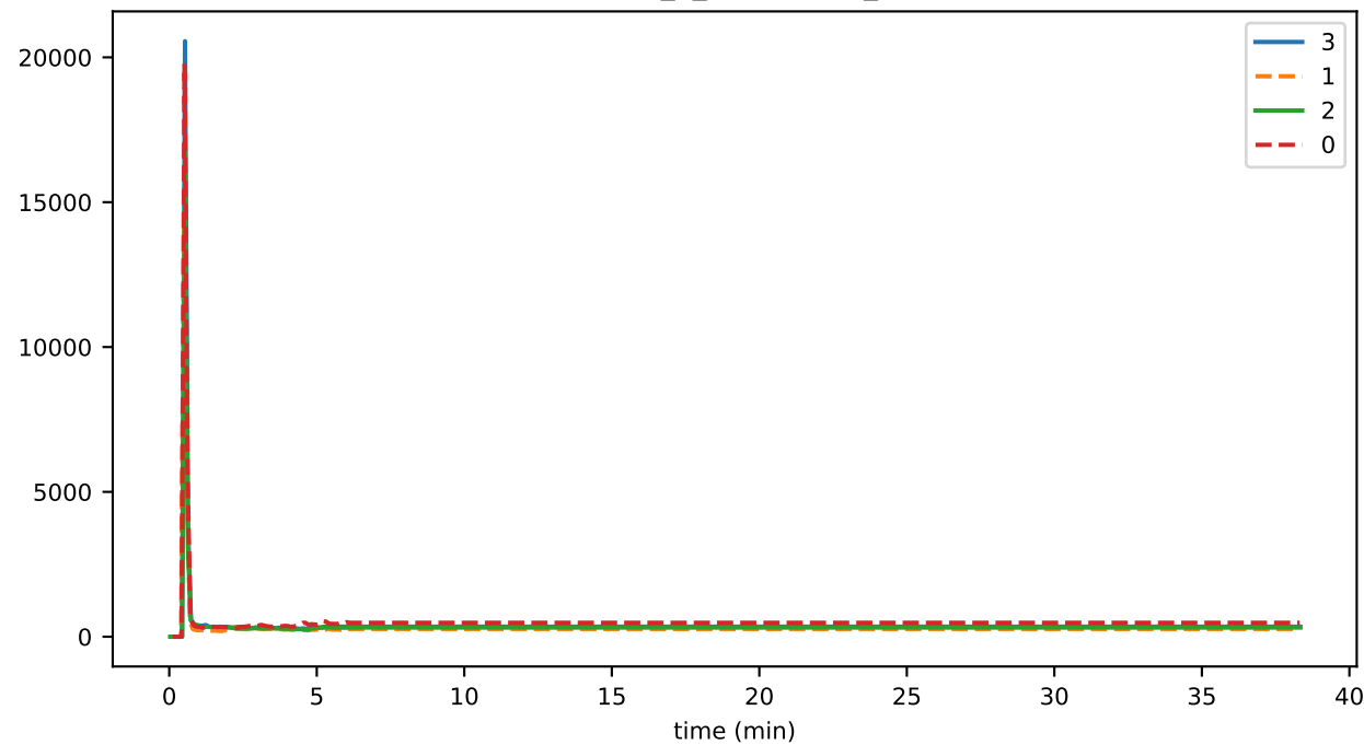
eventDelay_4_verification_gossip
