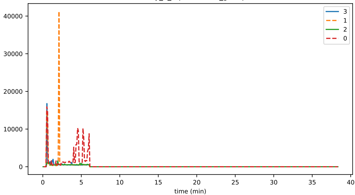
eventDelay_5_orphanBuffer_gossipMAX
