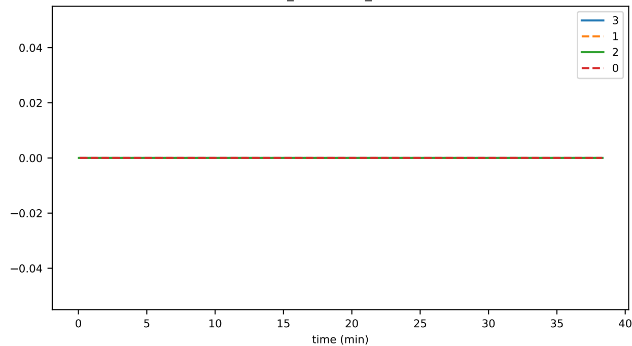
connSend_endStream_tooFarBehind
