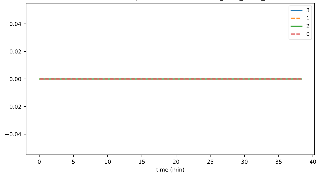
SmartContractService:SystemContractMethodCall_MINT_BURN_failed
