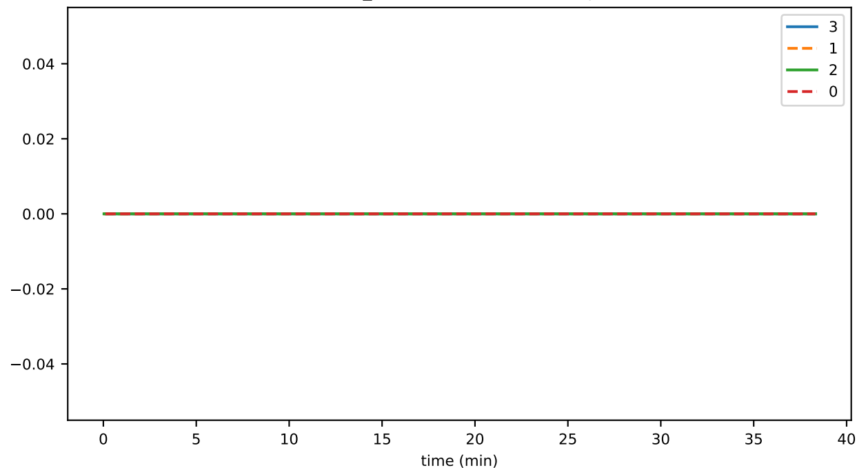
conn_closed
