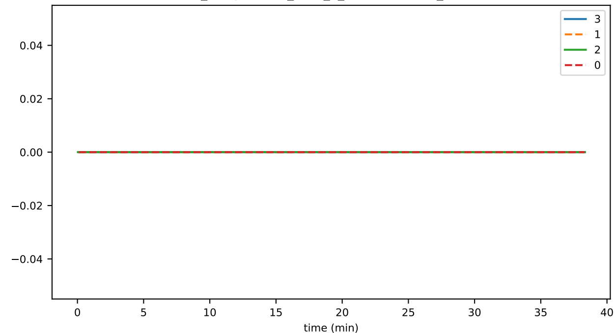
ds_compactions_level_3_leafKeysTimeMs_state
