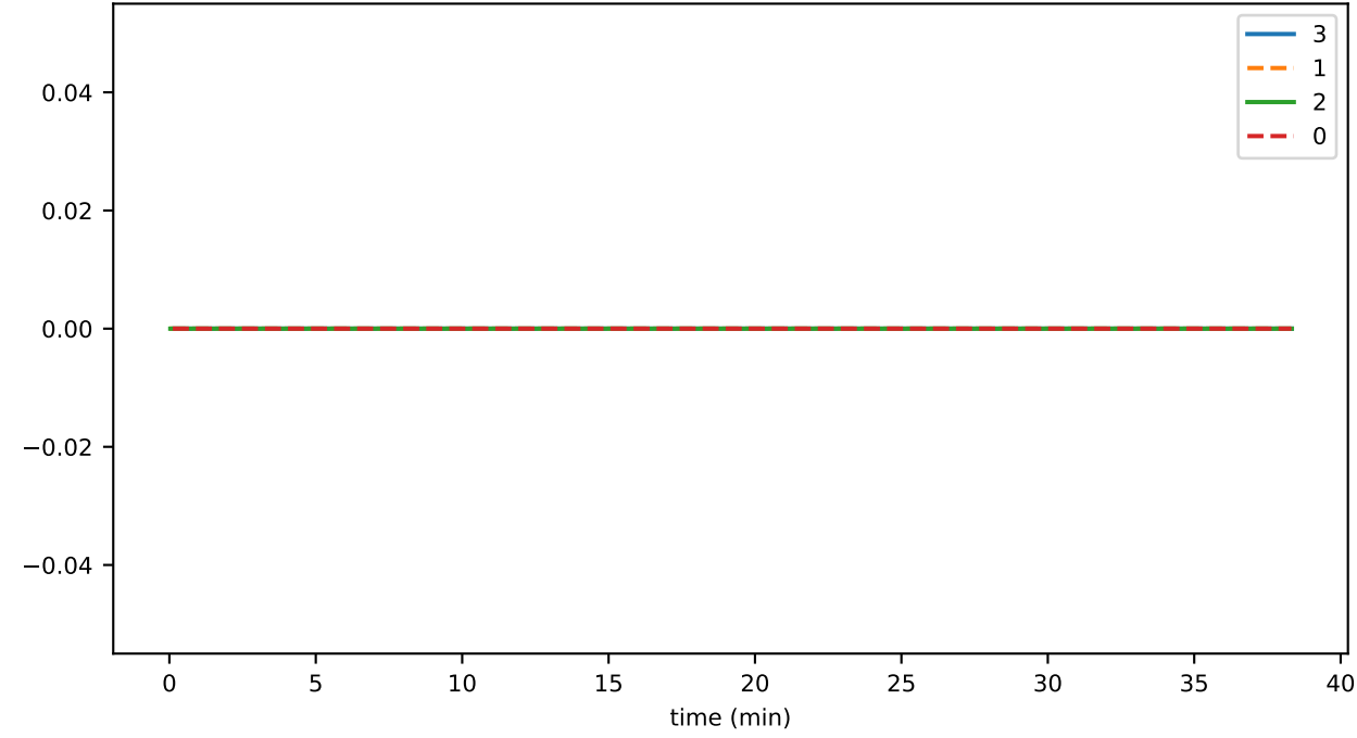
broadcastDisabledDueToLag
