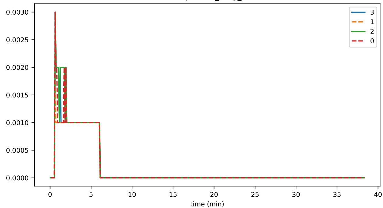
EventDeduplicator_busy_fraction
