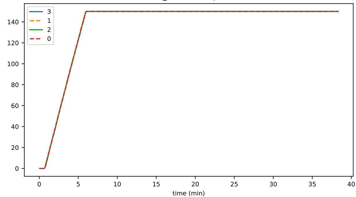
buffer_latestBlockOpened
