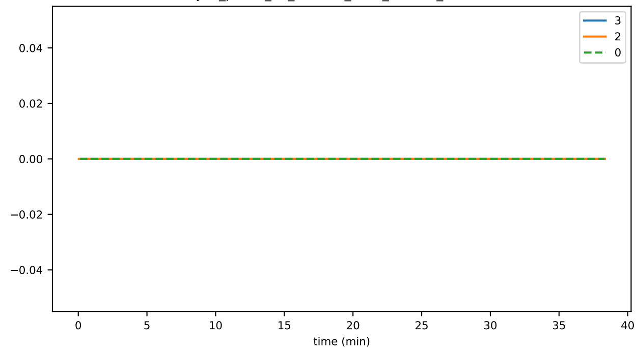
sync_phase_01_fraction_SELF_FALLEN_BEHIND
