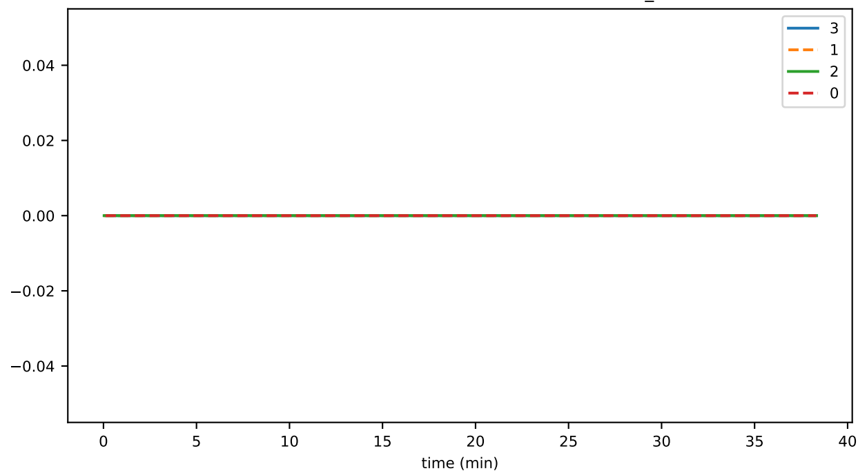
SmartContractService:LatestGasPrice
