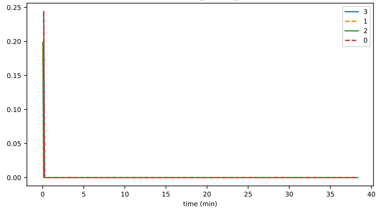
eventCreation_fraction_IDLE
