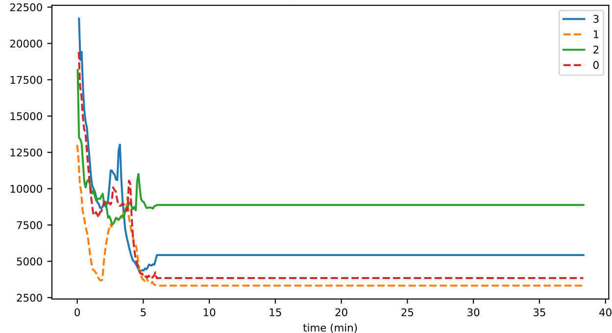
syncPermitsAvailable
