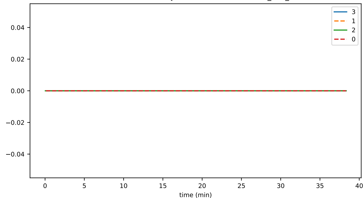
SmartContractService:SystemContractMethodCall_MINT_BURN_failed
