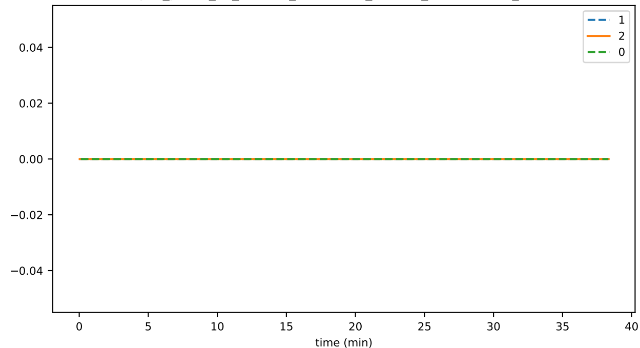
sync_phase_03_fraction_SELF_FALLEN_BEHIND
