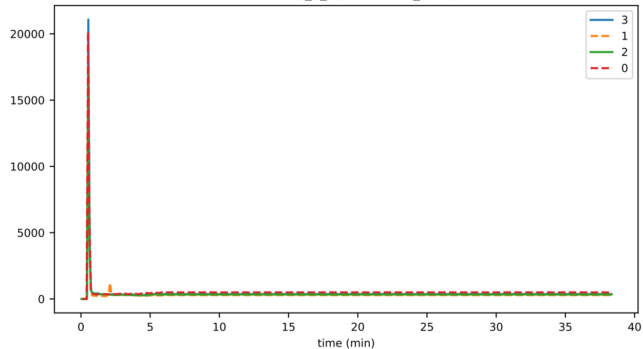
eventDelay_5_orphanBuffer_runtime
