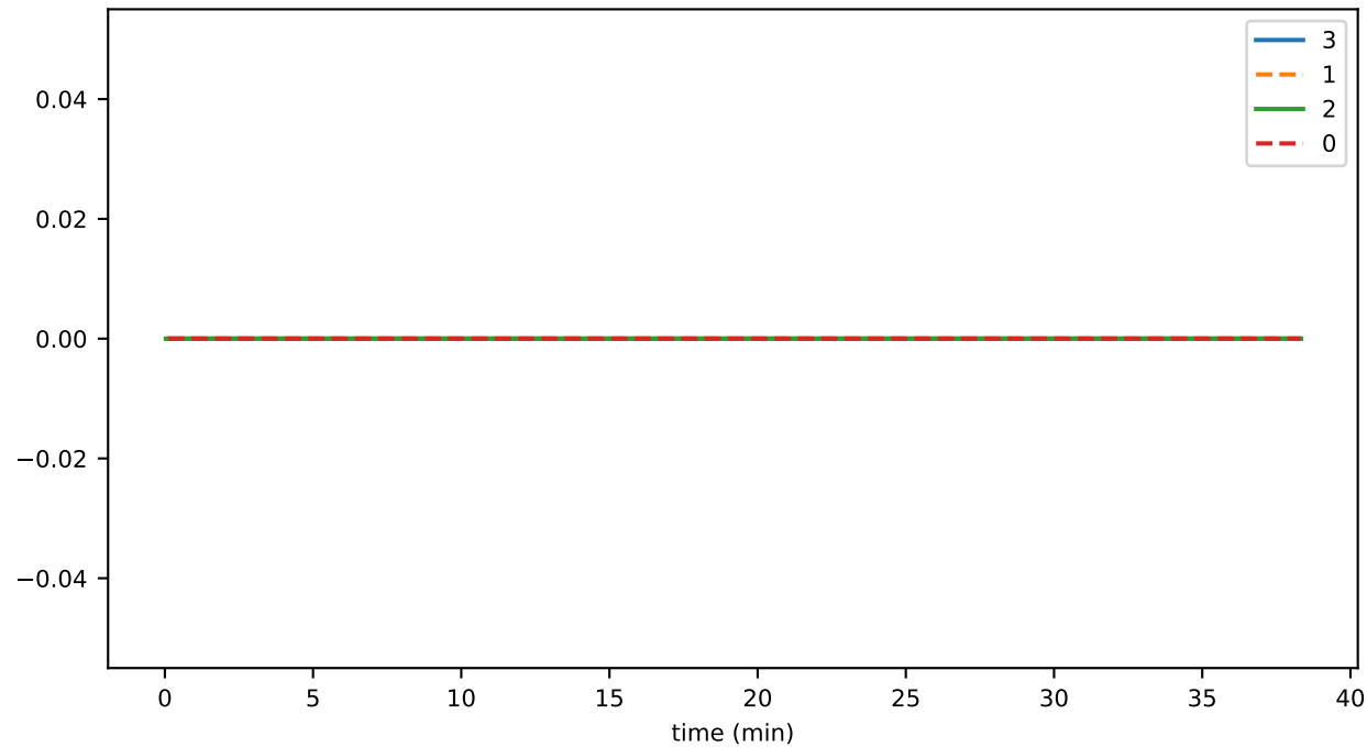
ds_compactions_level_6_hashesSavedSpaceMb_state
