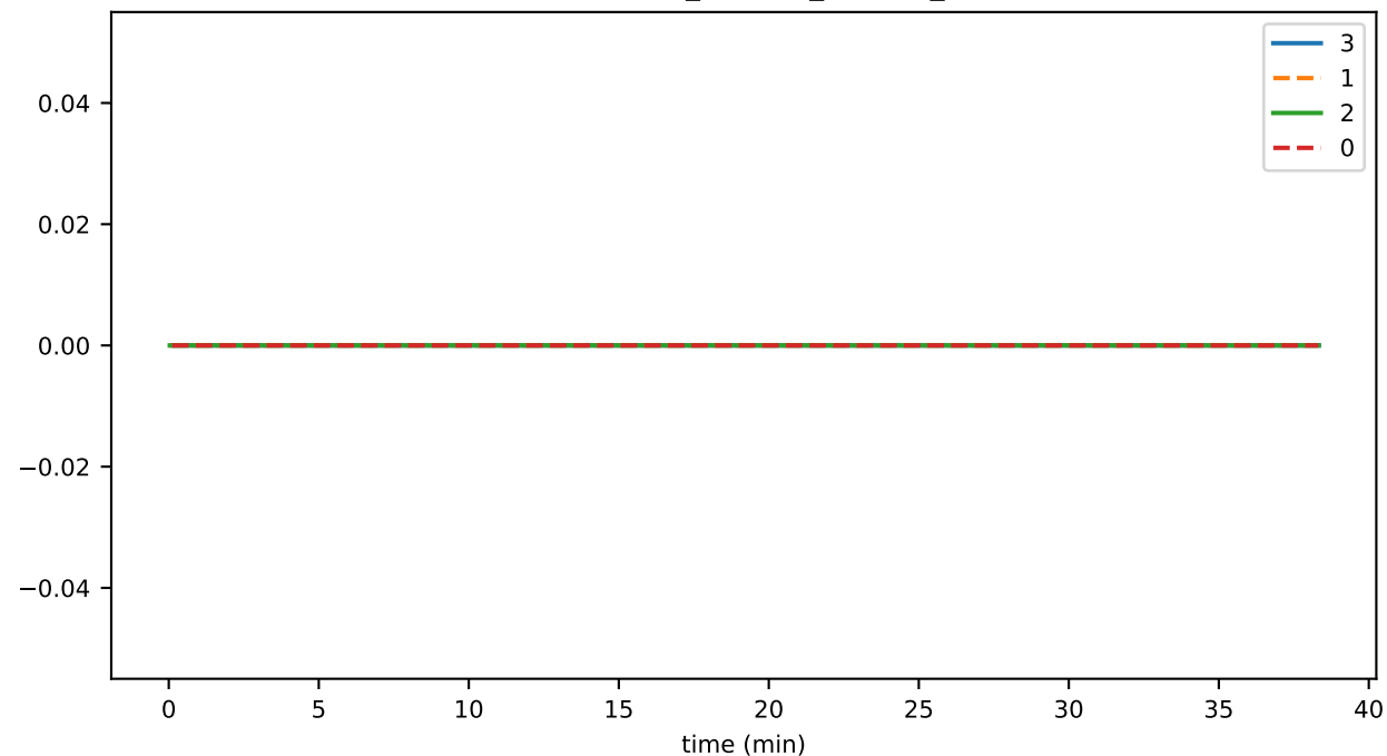
EventDeduplicator_busy_fraction
