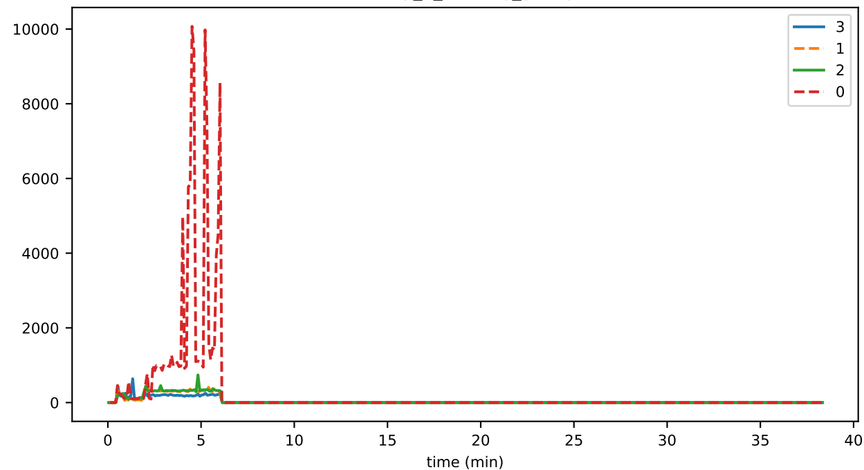
eventDelay_1_hashing_storageMAX
