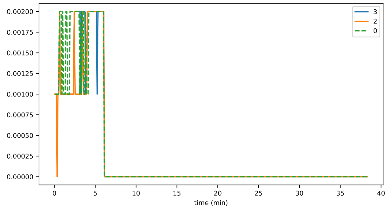
sync_phase_01_fraction_EXCHANGING_WINDOWS
