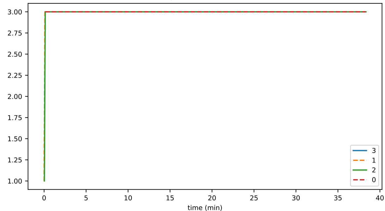
syncs_in_progress
