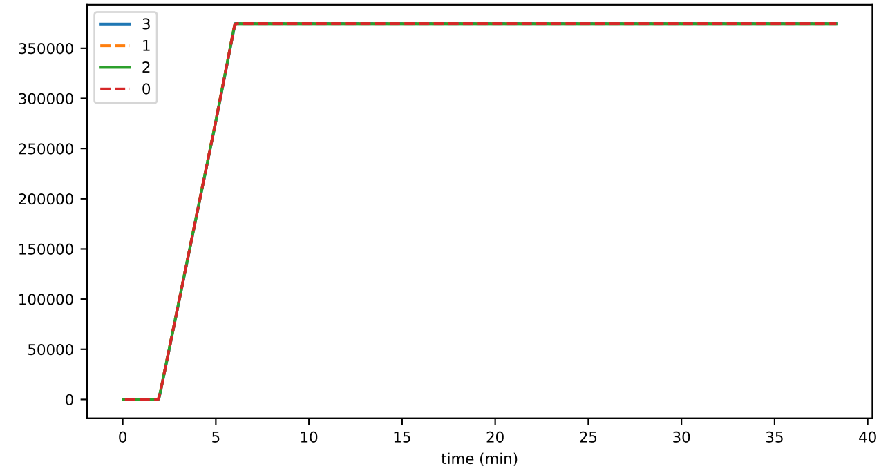
trans_per_sec
