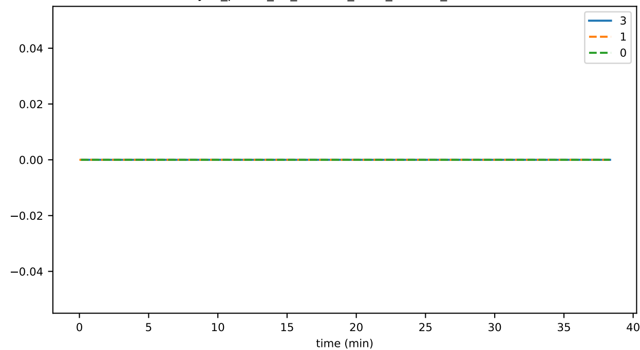
sync_phase_02_fraction_SELF_FALLEN_BEHIND
