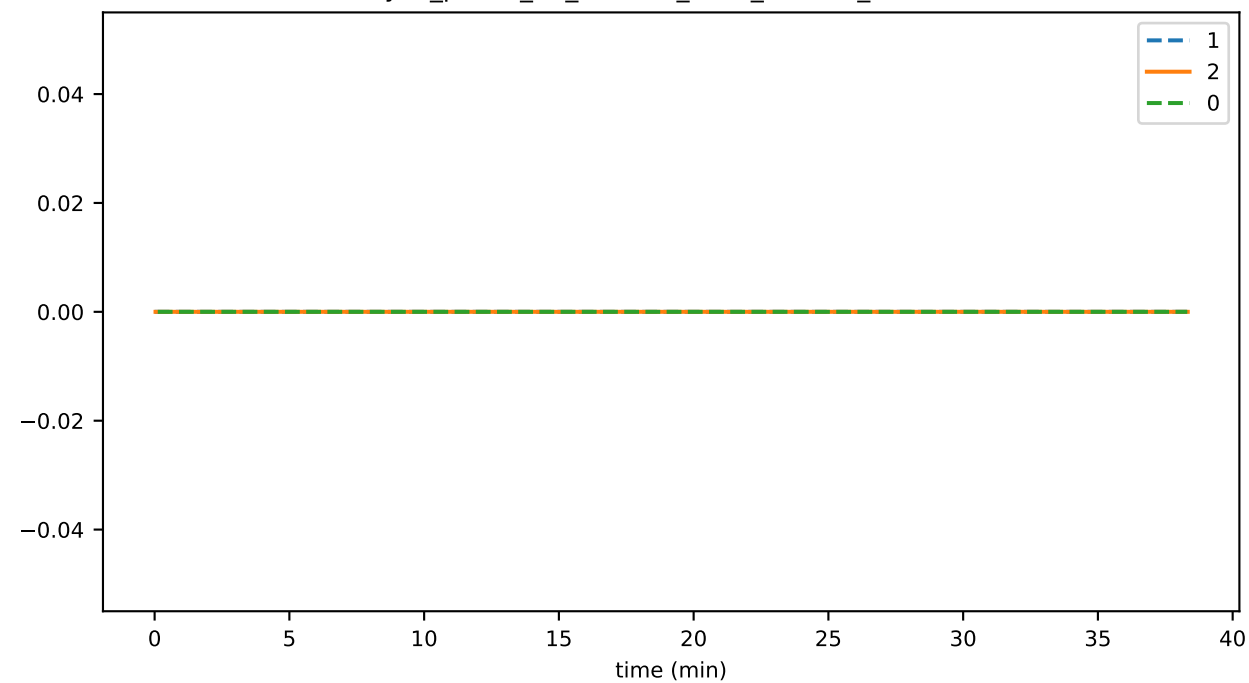
sync_phase_03_fraction_SELF_FALLEN_BEHIND
