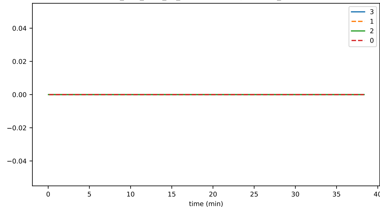
ds_files_level_1_leafKeysFileSizeByLevelMb_state
