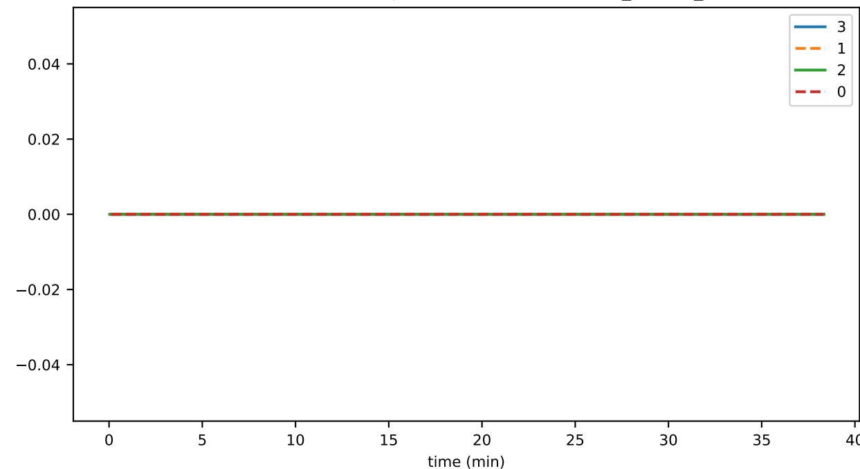
SmartContractService:SystemContractMethodCall_SCHEDULE_failed
