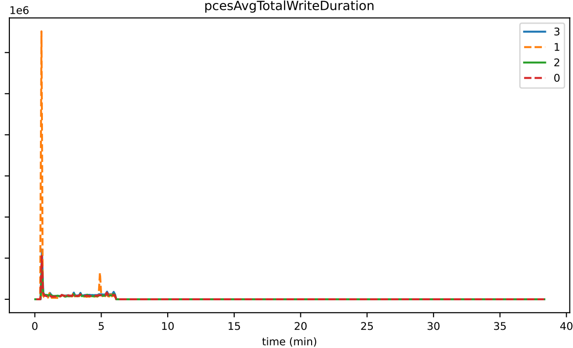
pcesAvgTotalWriteDuration
