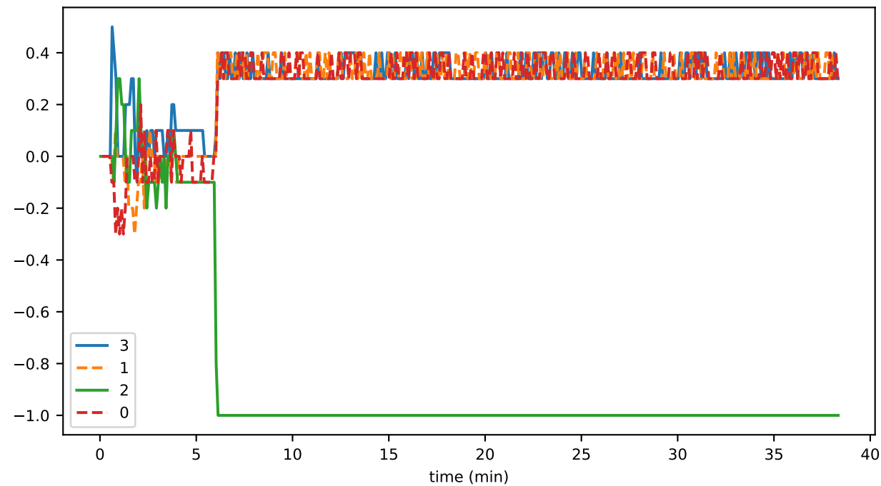
syncIndicatorDiff
