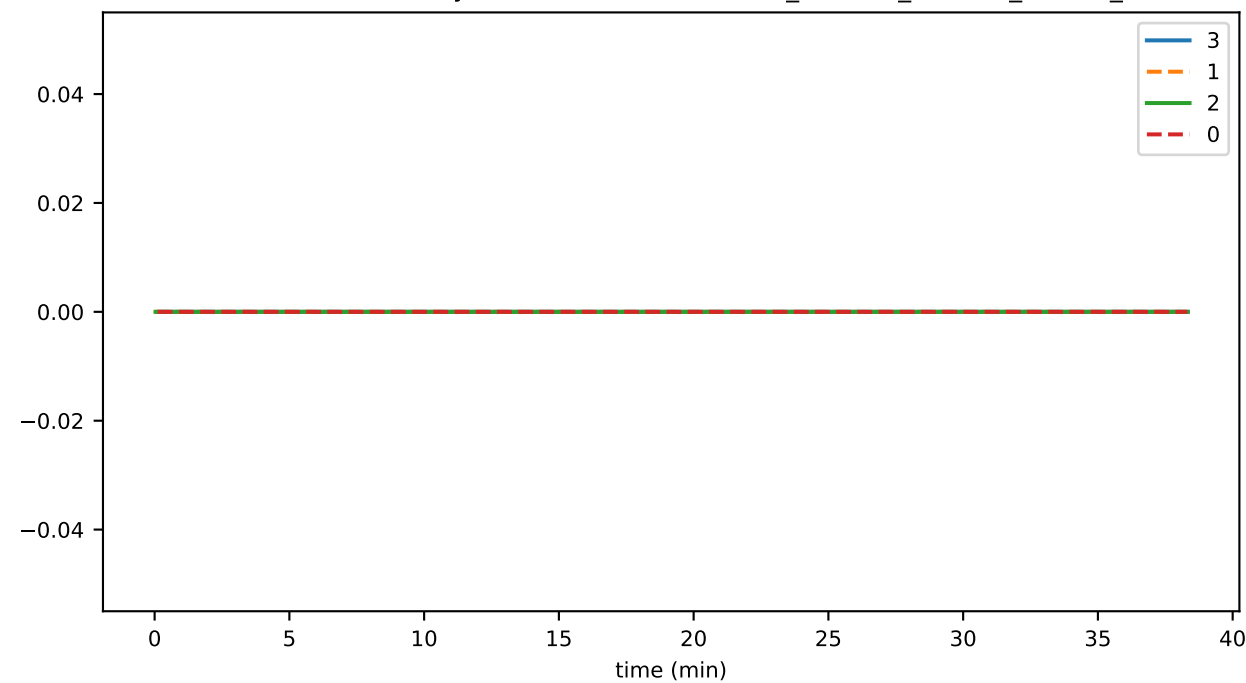
SmartContractService:SystemContractMethodCall_CREATE_DELETE_TOKEN_failed
