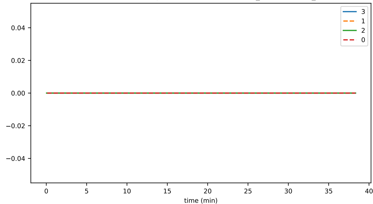
SmartContractService:SystemContractMethodCall_CREATE_DELETE_TOKEN_failed
