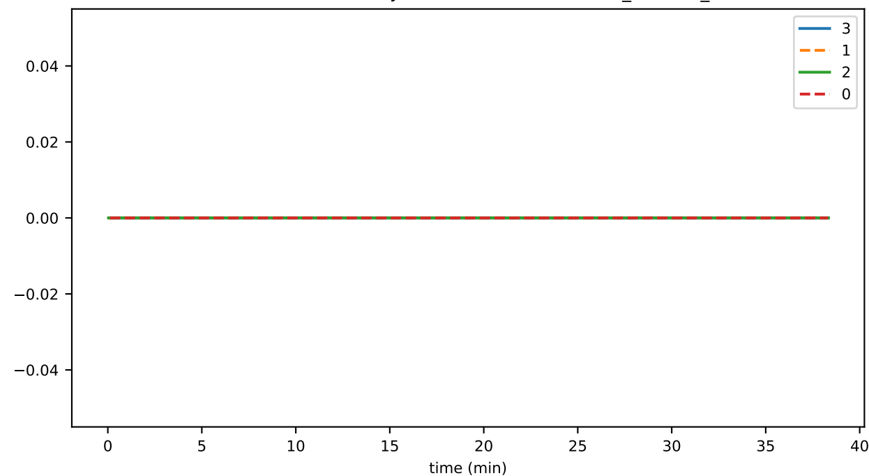
SmartContractService:SystemContractMethodCall_FREEZE_UNFREEZE_failed
