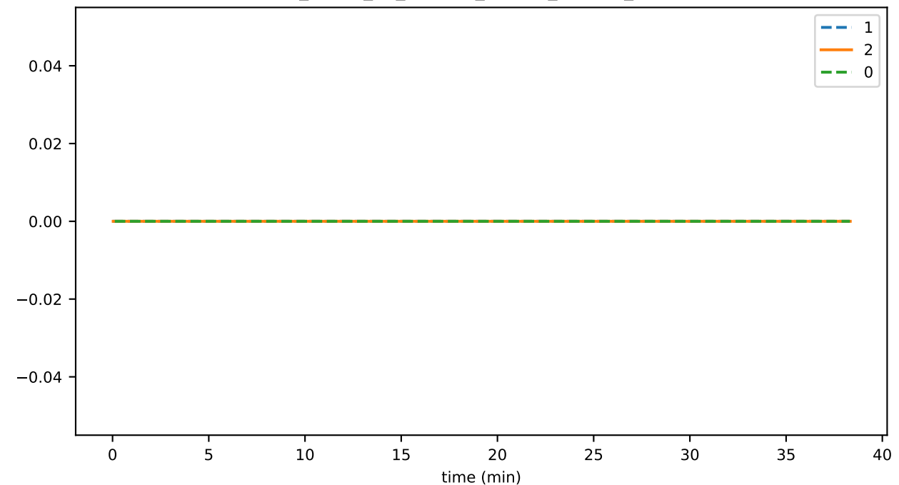
sync_phase_03_fraction_OTHER_FALLEN_BEHIND
