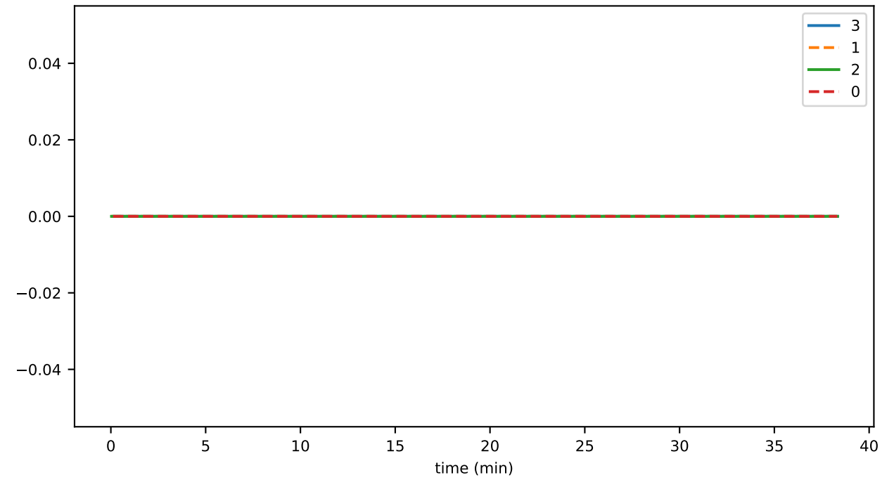
ds_files_level_6_leavesFileSizeByLevelMb_state
