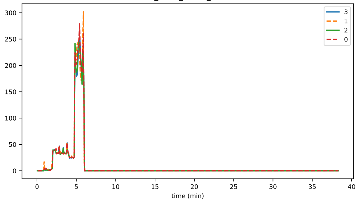
dupEvPercent
