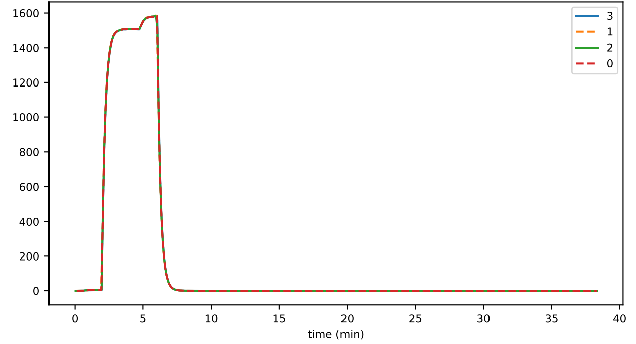
trans_per_sec
