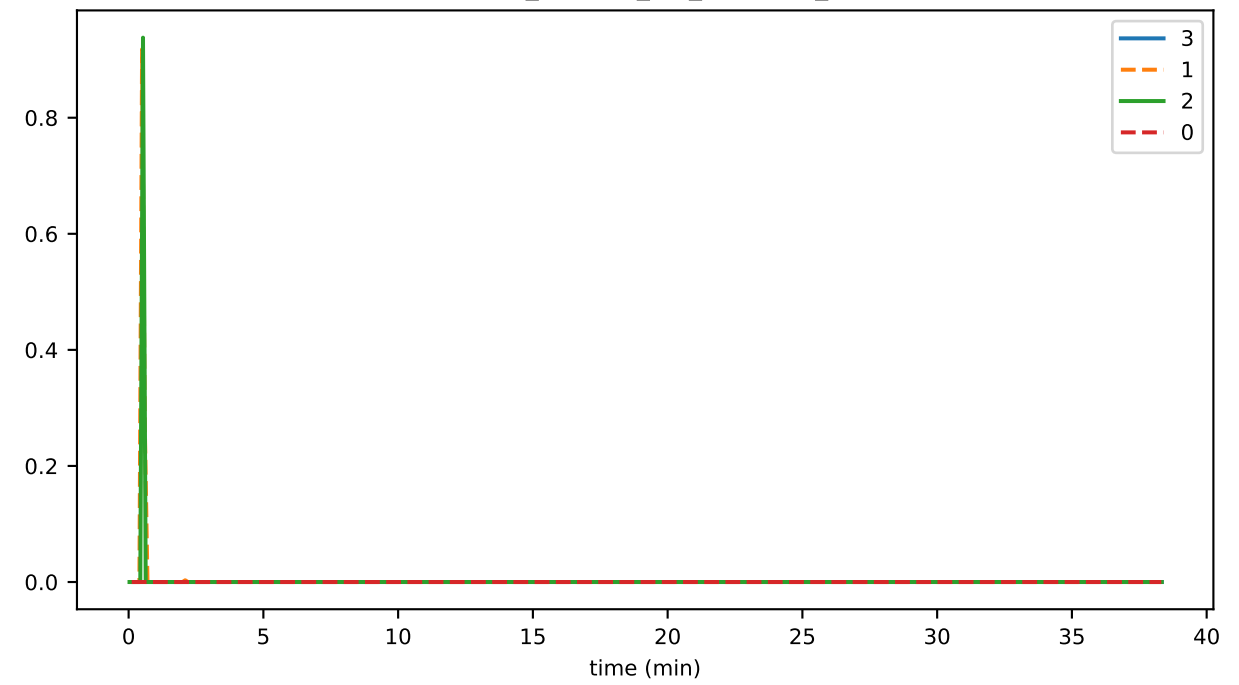
eventCreation_fraction_NO_ELIGIBLE_PARENTS
