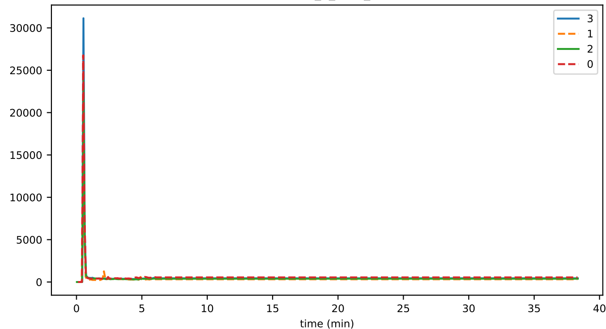
eventDelay_6_pces_gossip
