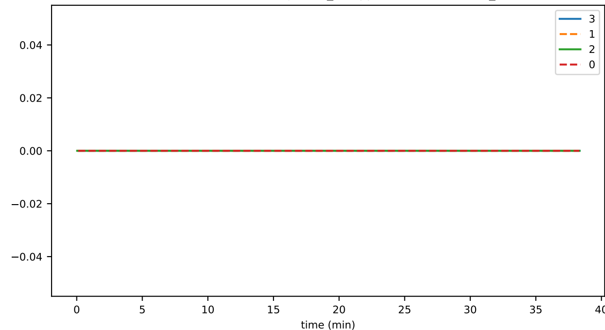
SmartContractService:SuccessfulTransactionDuration_count
