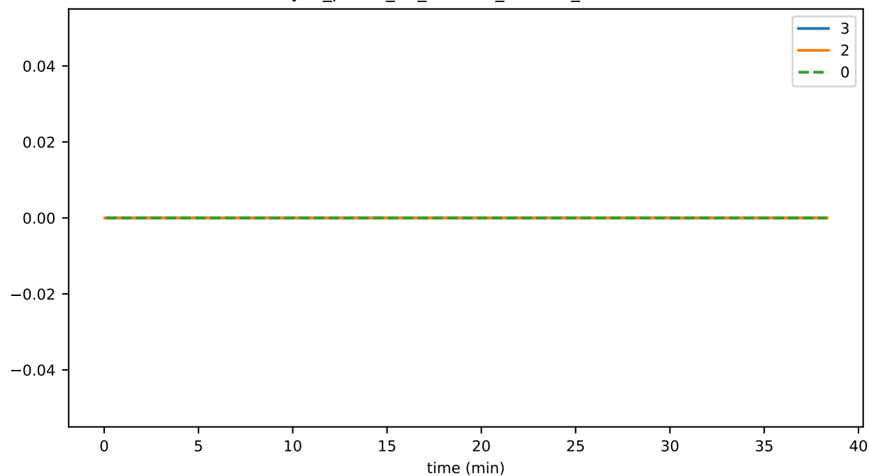
sync_phase_01_fraction_NO_PERMIT
