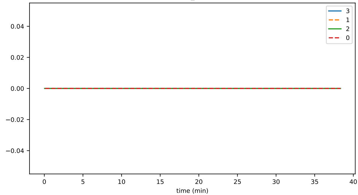
connRecv_skipBlock
