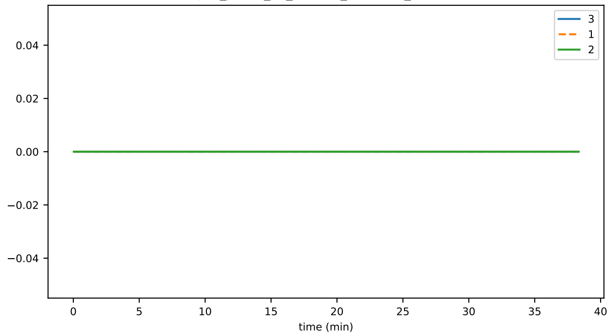
sync_phase_01_fraction_EXCHANGING_TIPS
