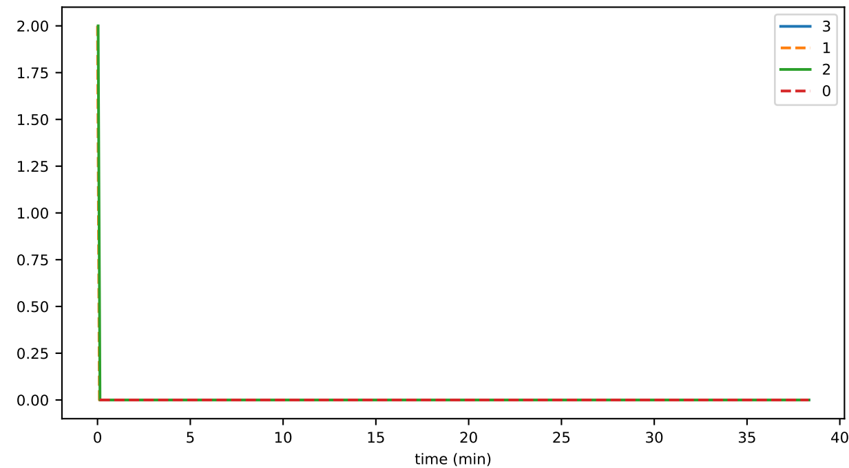
syncPermitsAvailable
