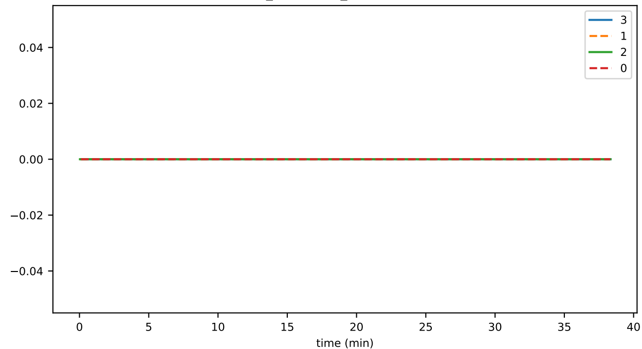
conn_connClose_connectionError
