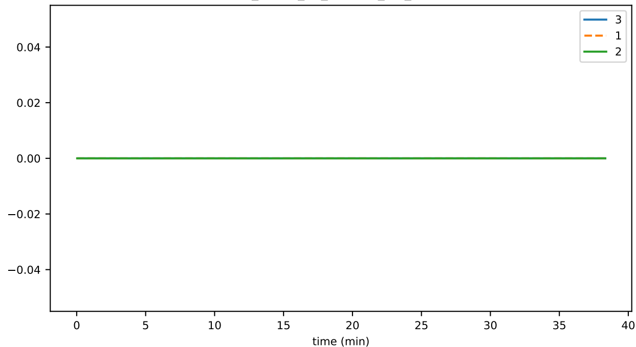
sync_phase_00_fraction_NO_PERMIT
