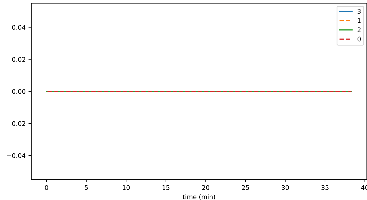
sigStateHash
