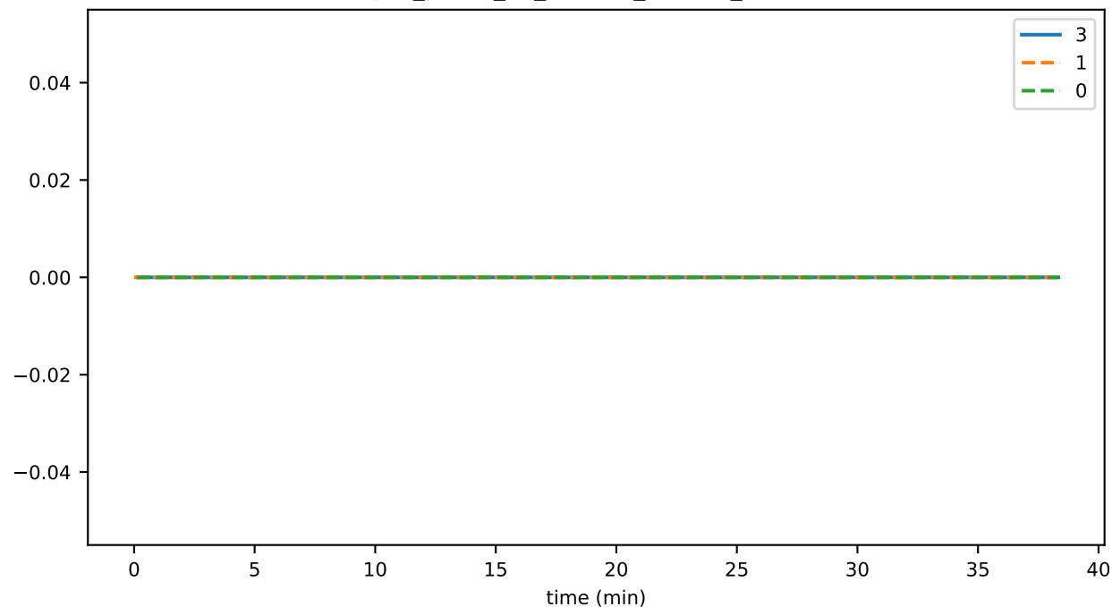
sync_phase_02_fraction_NO_PERMIT
