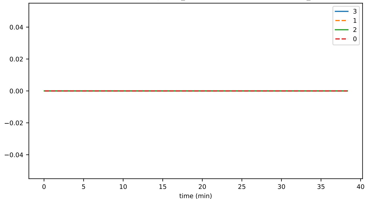
SmartContractService:Rejected_contractCreateTxDueToIntrinsicGas_total
