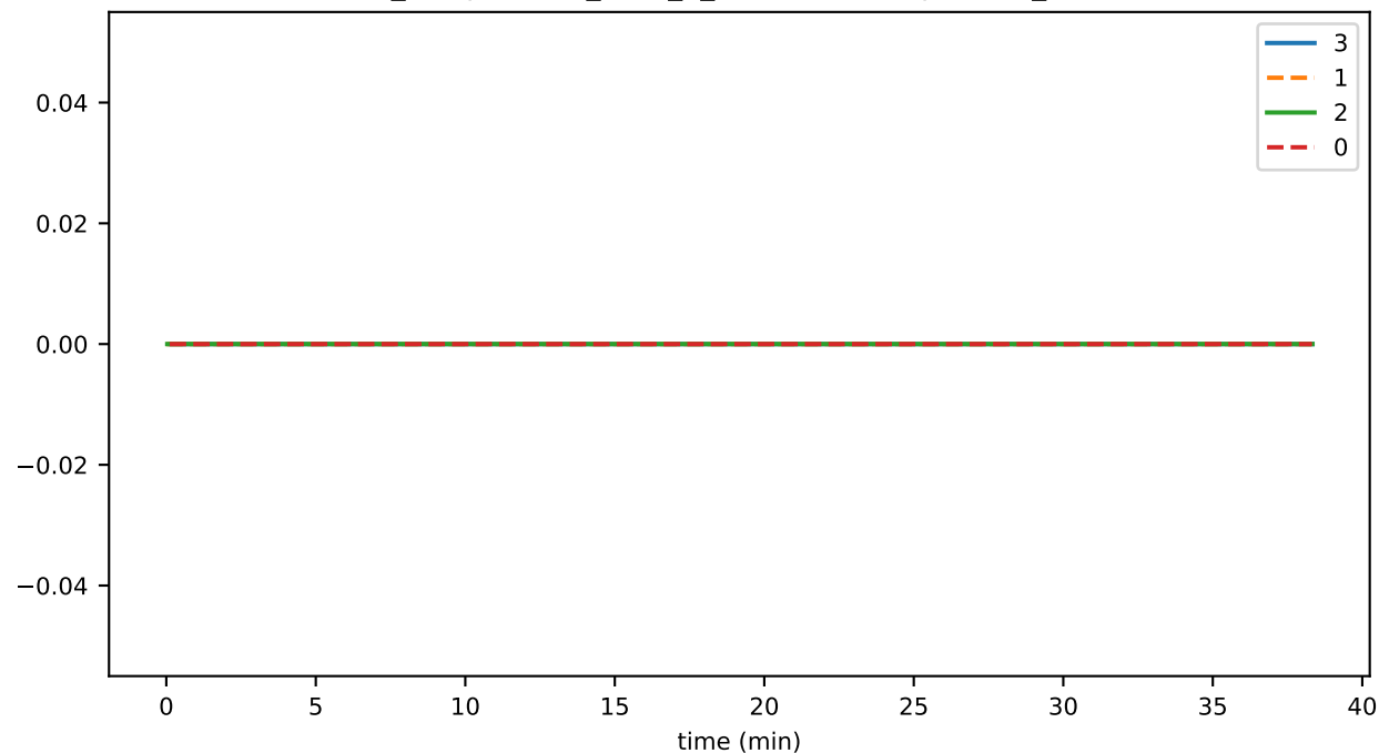
ds_compactions_level_7_leafKeysSavedSpaceMb_state
