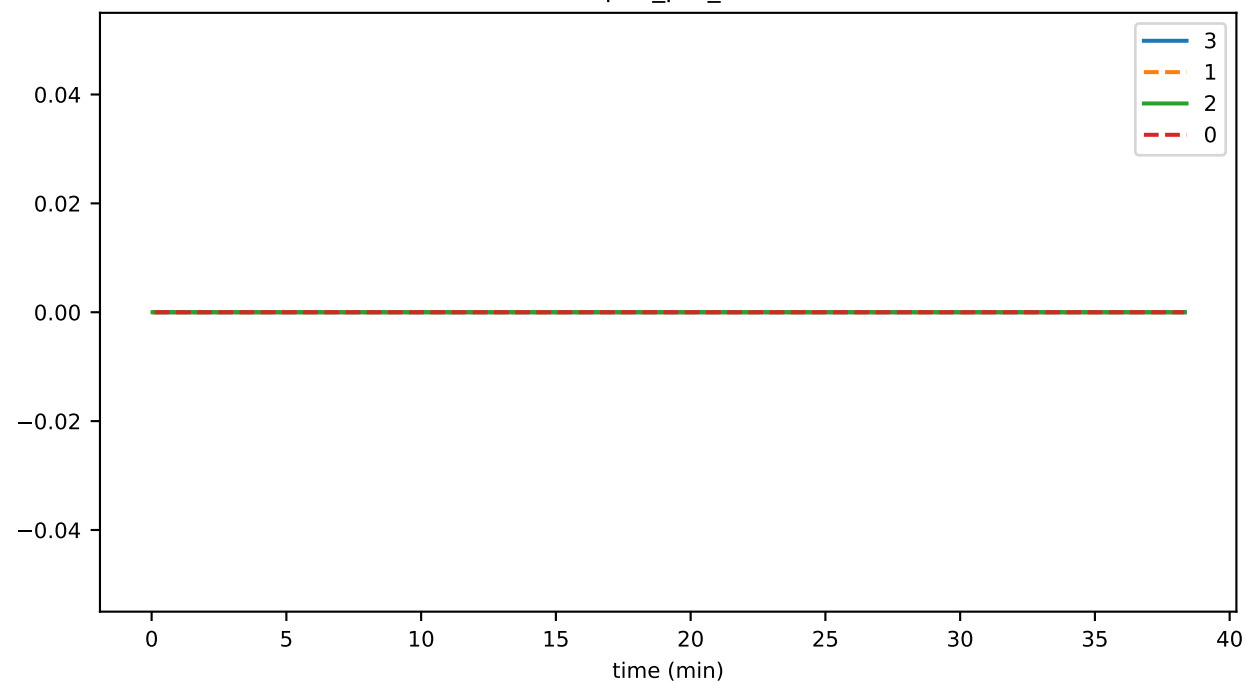
endsReconnectAsReceiver
