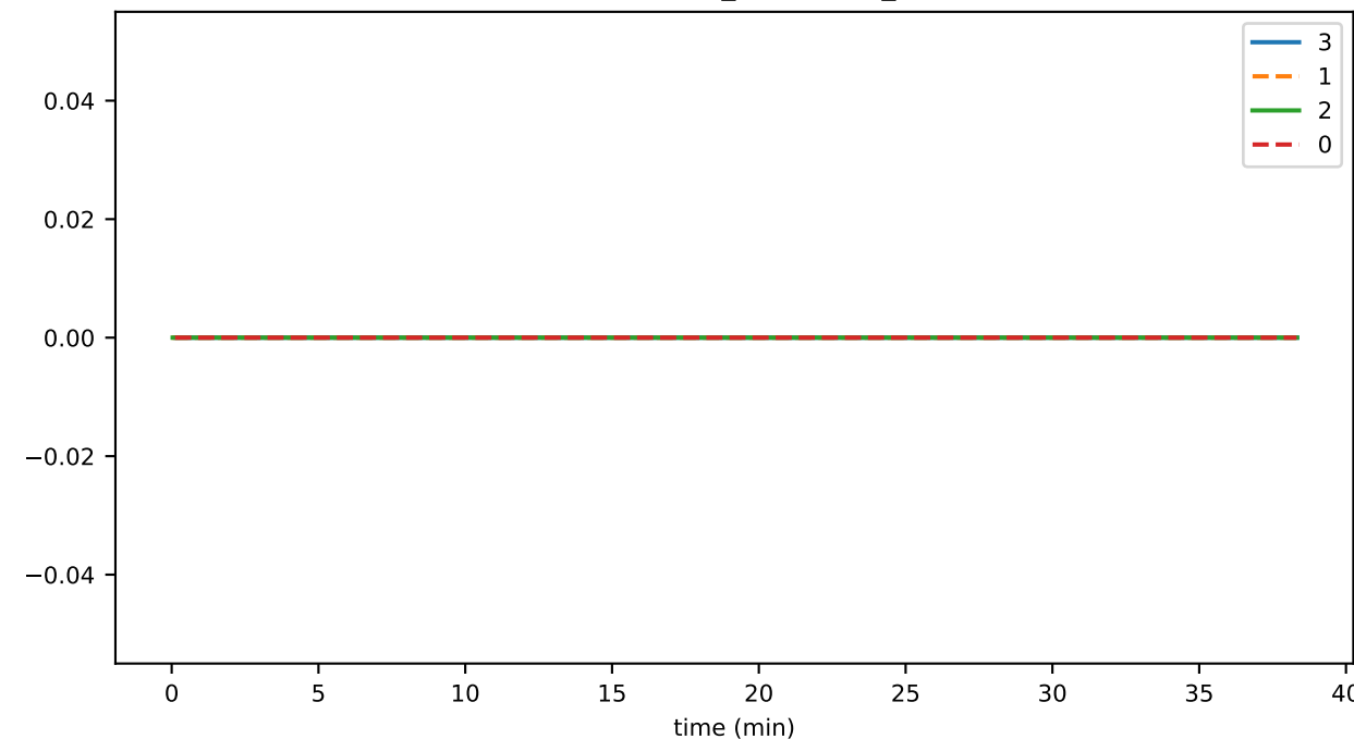
futureEventBuffer_eventCreator_maxBR
