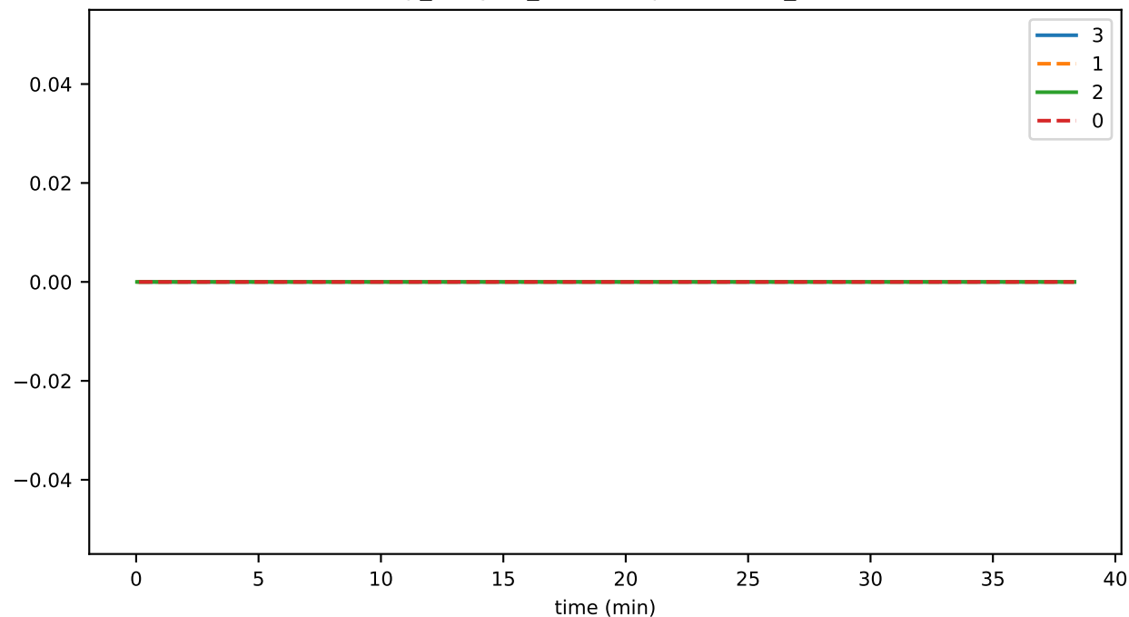
vmap_lifecycle_flushDurationMs_state
