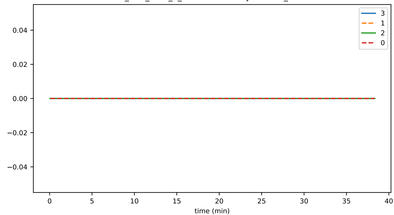
ds_files_level_4_hashesFileSizeByLevelMb_state
