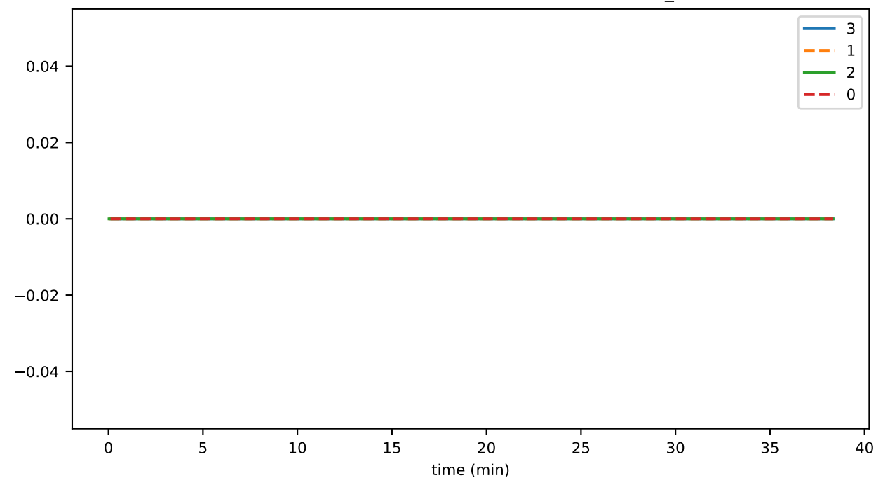
SmartContractService:OpsDuration_PerTxn_avg
