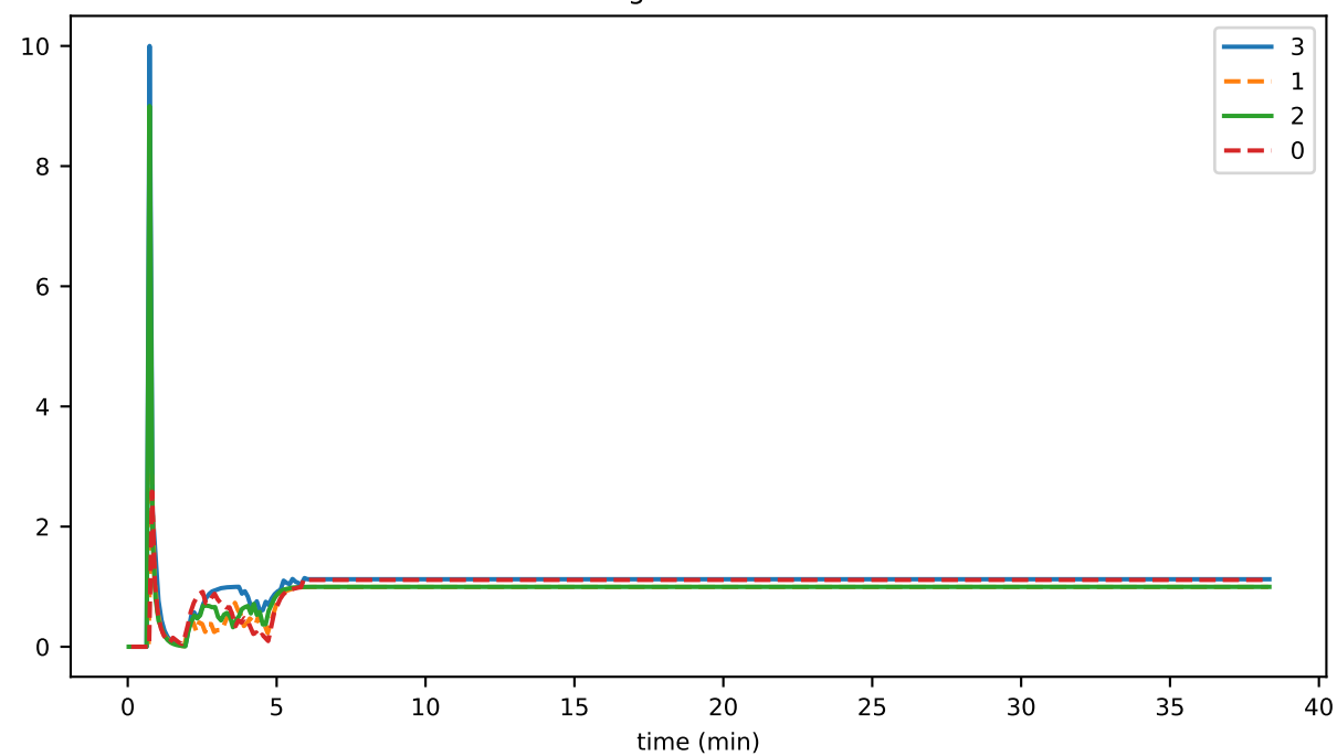
sigStateHash
