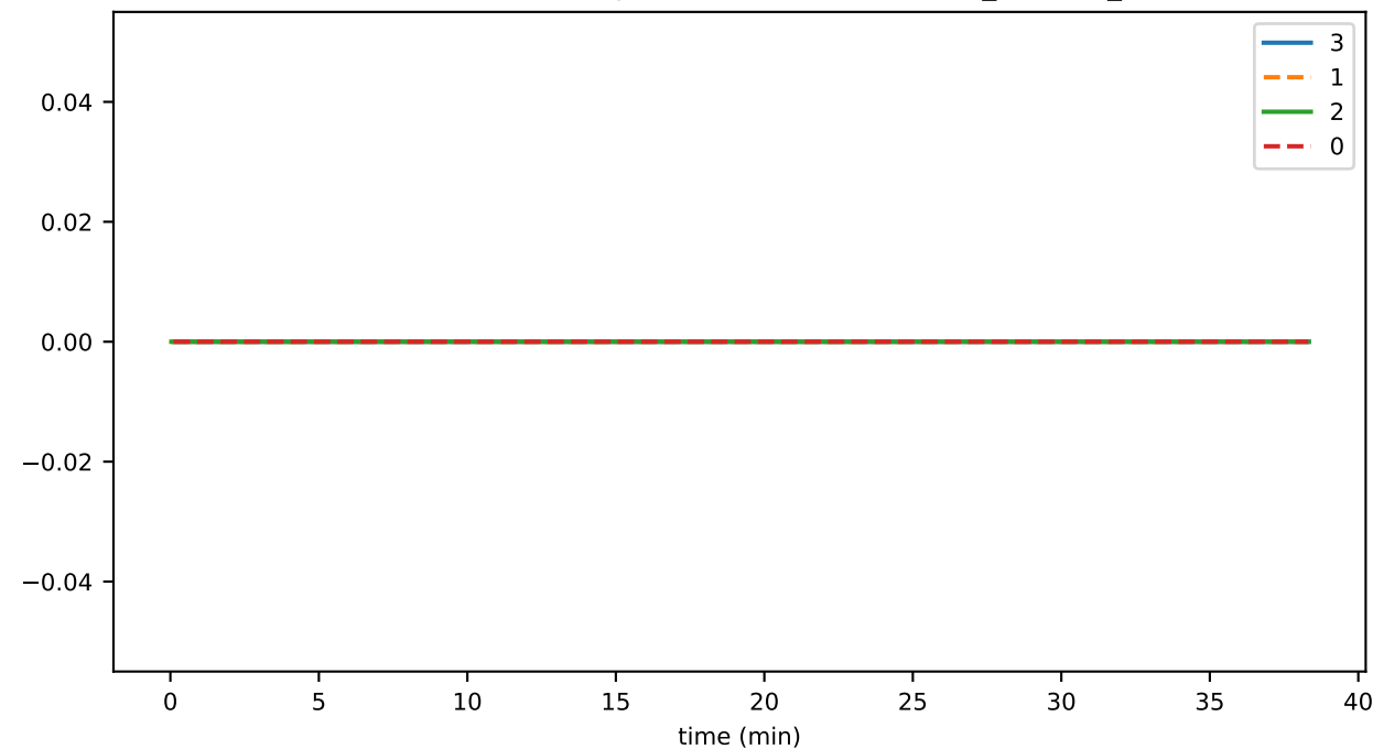
SmartContractService:SystemContractMethodCall_WIPE_failed
