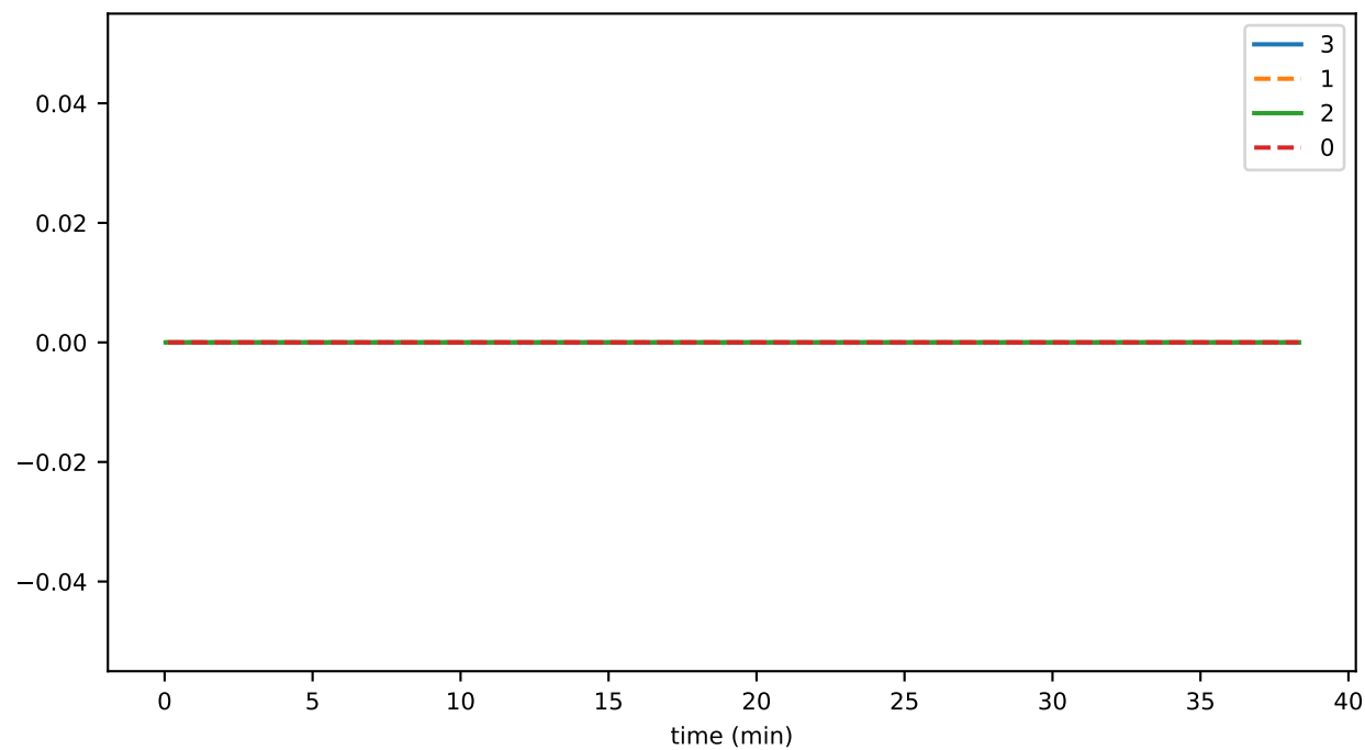
eventStreamQueueSize
