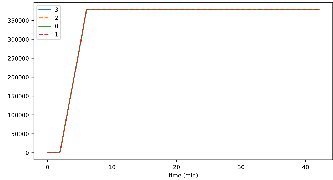
trans_per_sec
