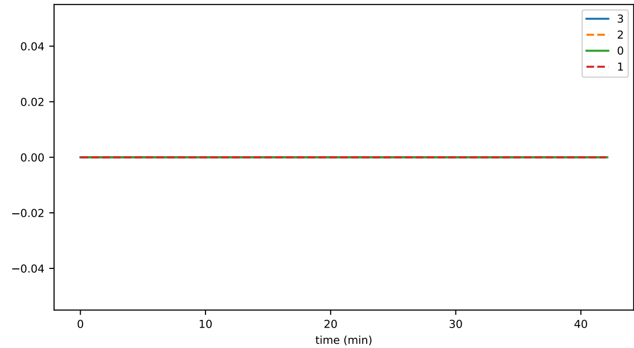
ds_files_hashesStoreFileSizeMb_state
