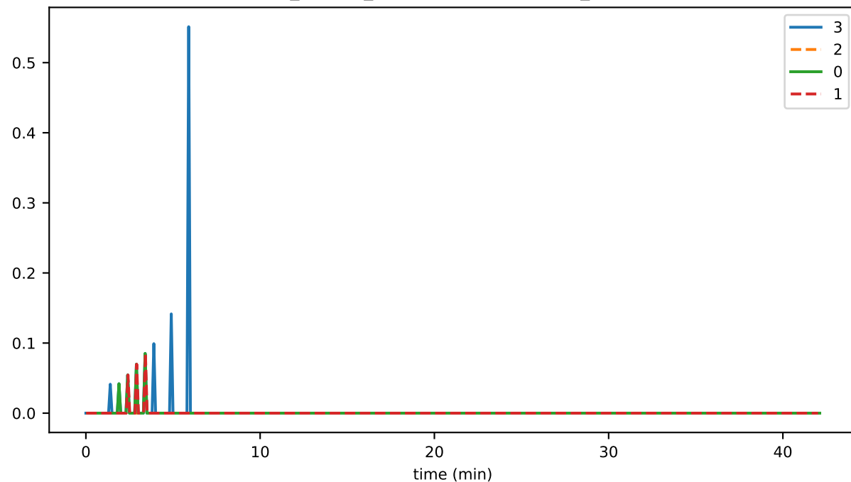
ds_flushes_hashesStoreFileSizeMb_state
