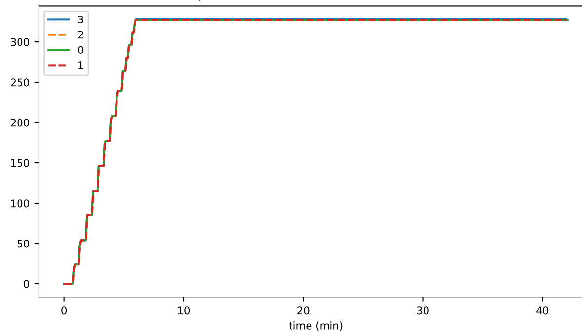
preconsensusEventFileOldestSeconds
