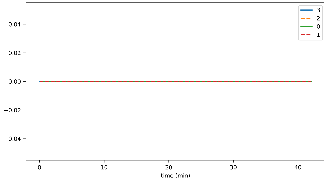
ds_compactions_level_2_hashesSavedSpaceMb_state
