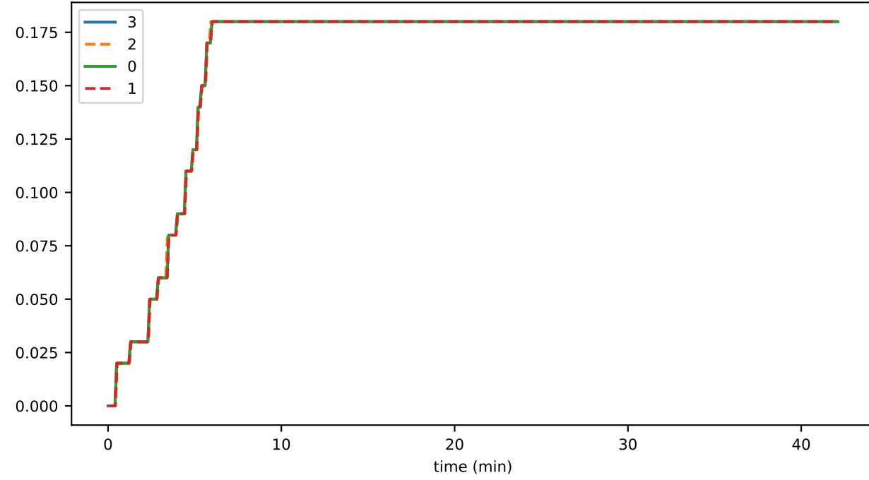
directMemPercent
