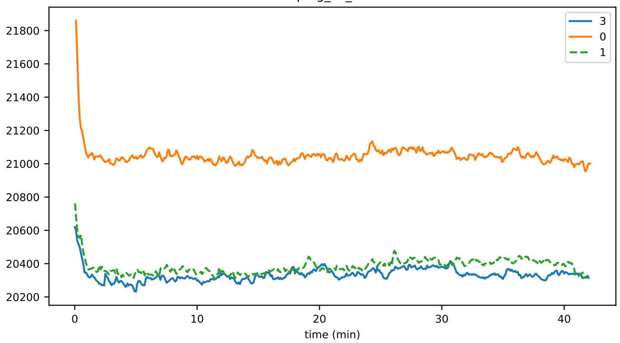
ping_us_02
