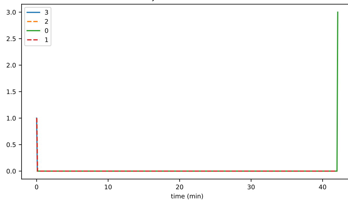
syncPermitsAvailable
