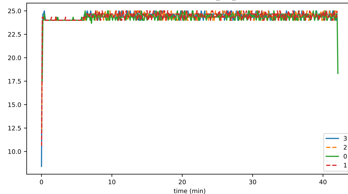
accountsPercentUsed
