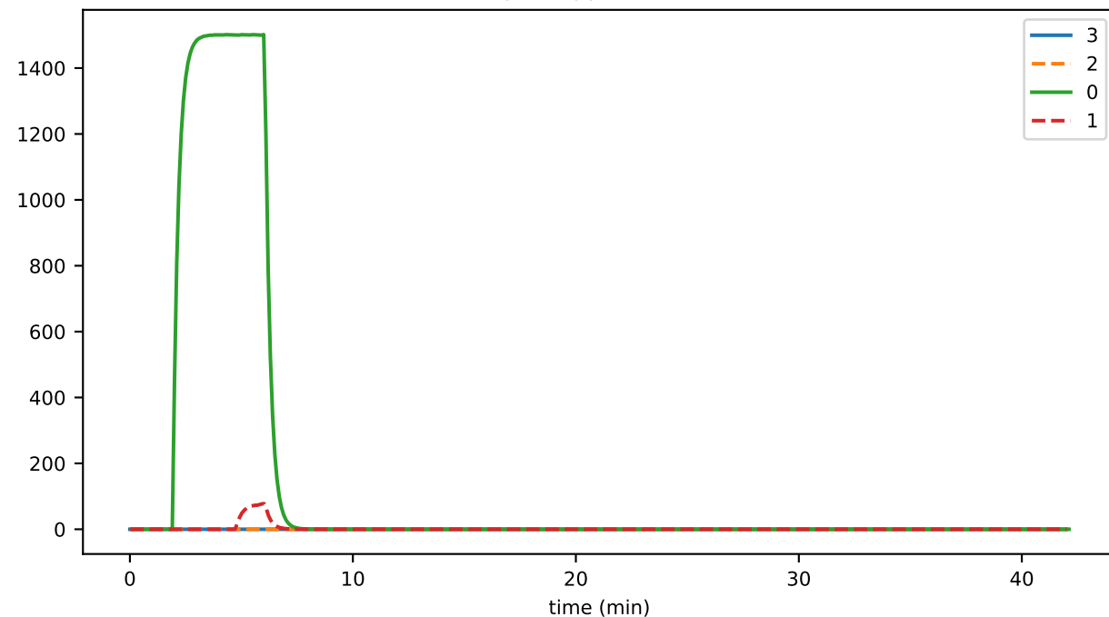
accountsMaxNumber
