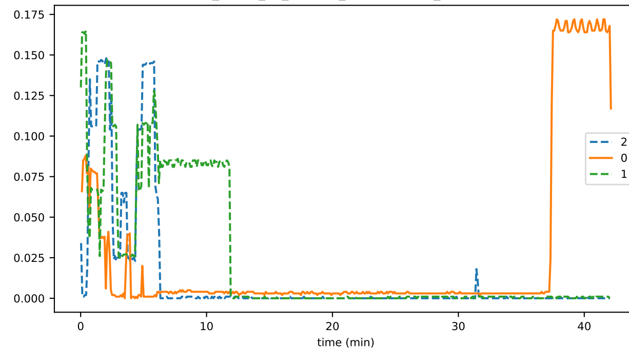
sync_phase_03_fraction_EXCHANGING_WINDOWS
