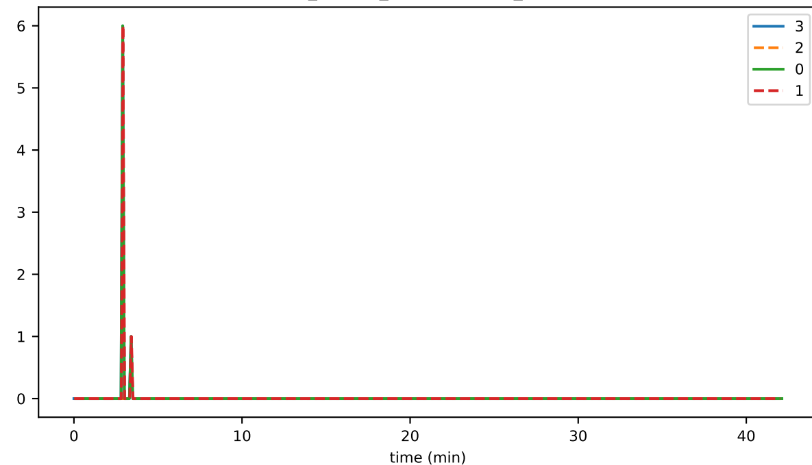
ds_flushes_leavesDeleted_state
