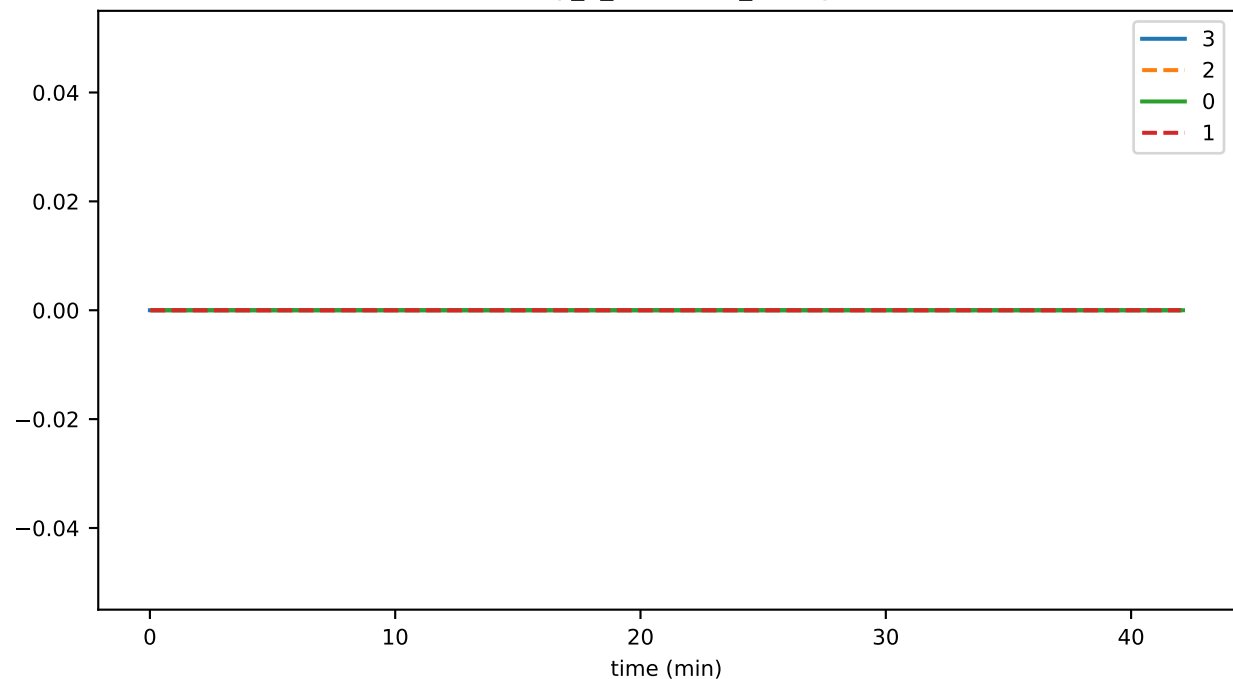
eventDelay_3_deduplication_gossipMAX
