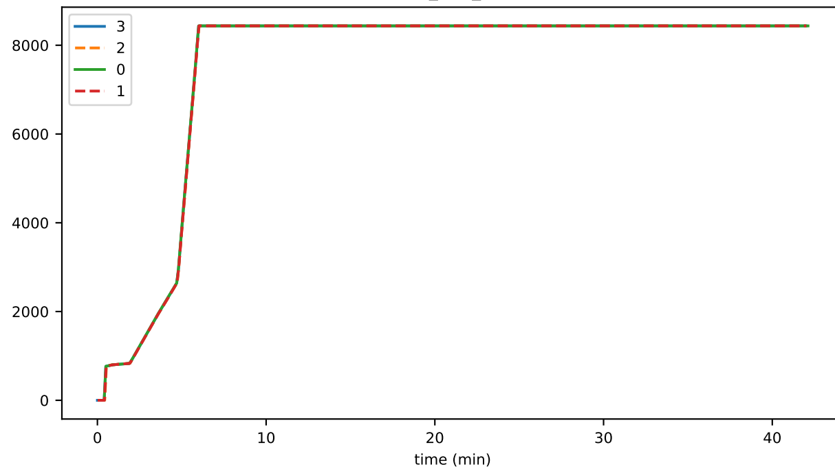
vmap_size_state
