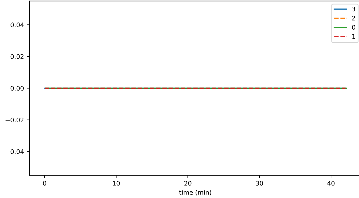
dupEvPercent
