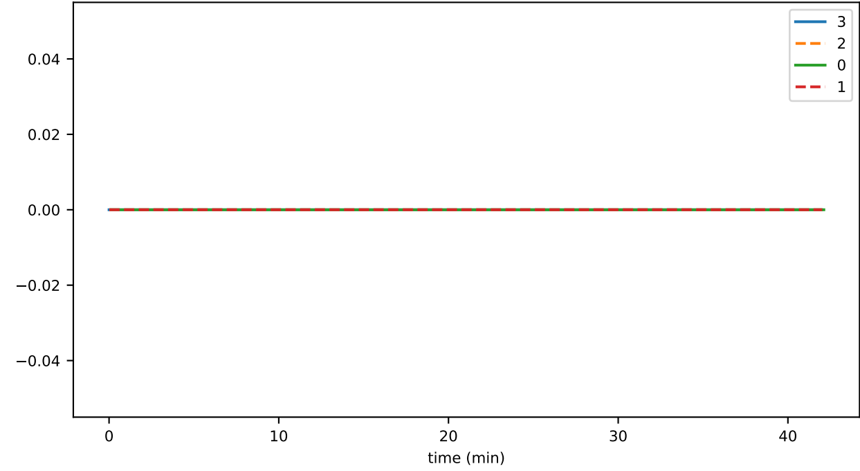
ds_files_level_2_leavesFileSizeByLevelMb_state
