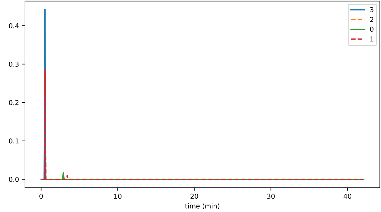
eventCreation_fraction_NO_ELIGIBLE_PARENTS
