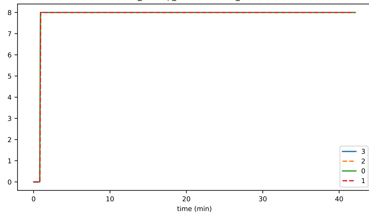
ds_reads_hashes_state
