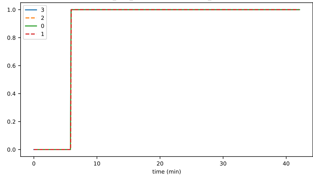
ds_files_hashesStoreFileSizeMb_state
