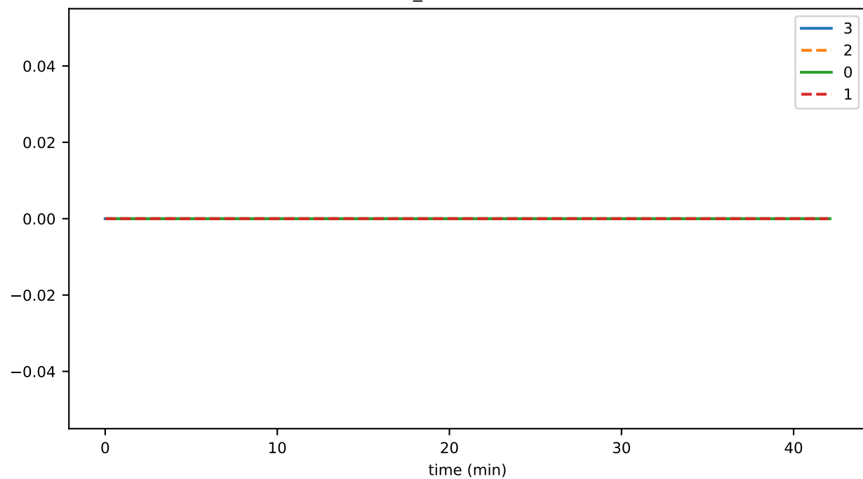
buffer_latestBlockAcked
