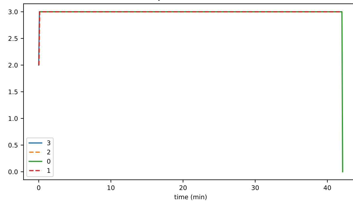
syncs_in_progress
