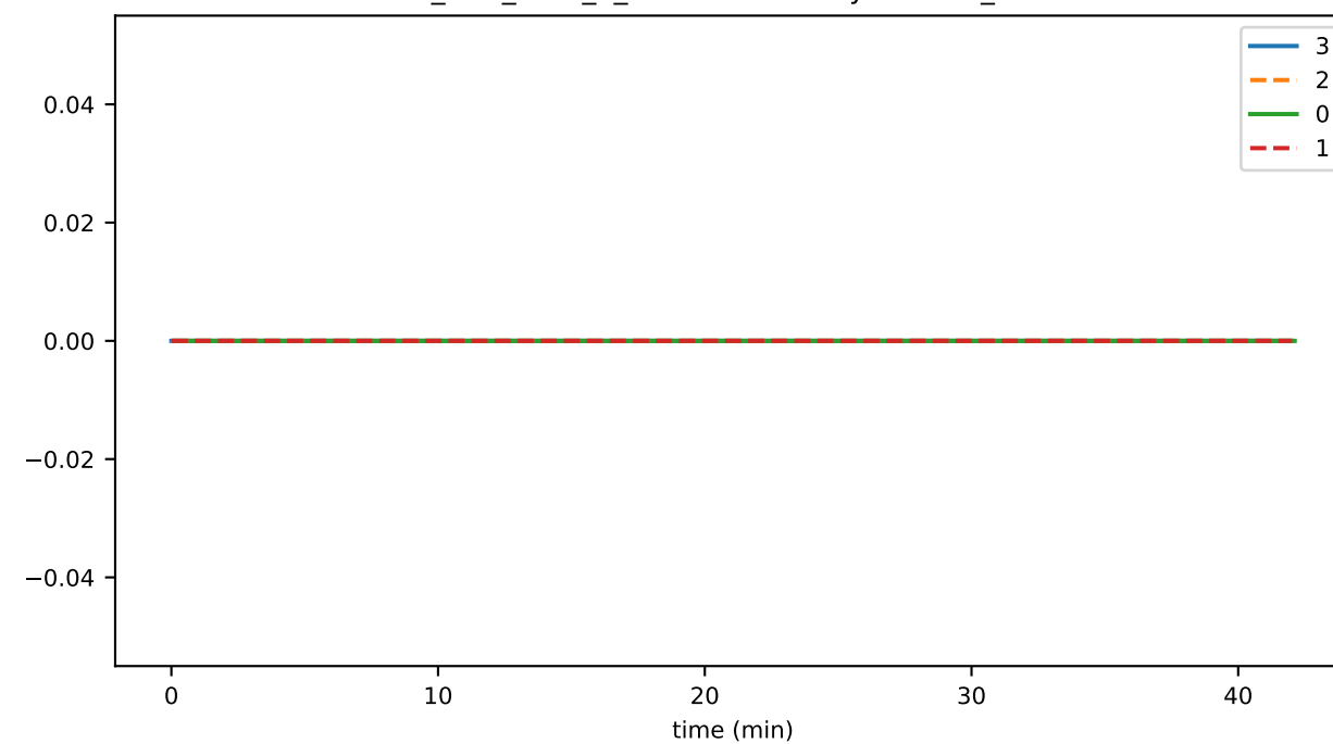
ds_files_level_8_hashesFileSizeByLevelMb_state
