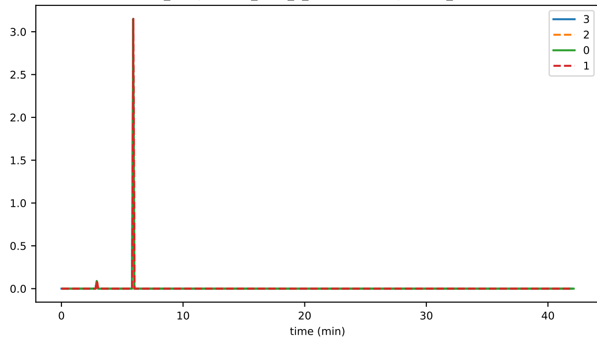
ds_compactions_level_2_hashesSavedSpaceMb_state
