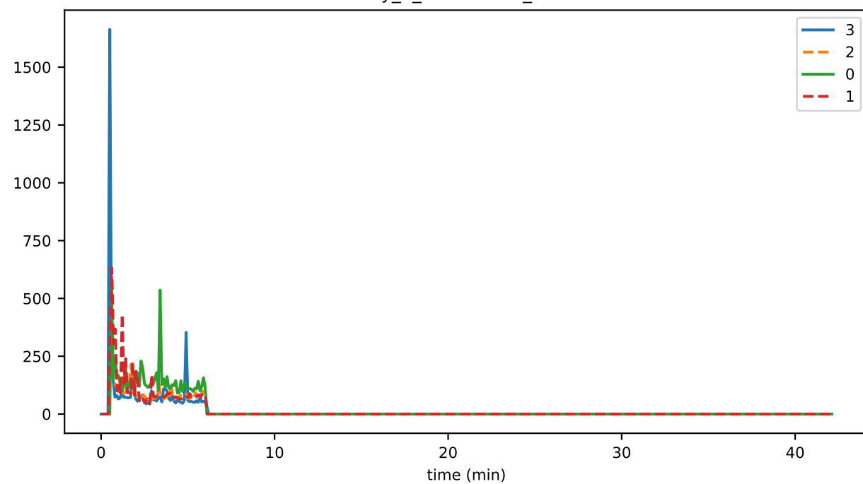
eventDelay_4_verification_runtimeMAX
