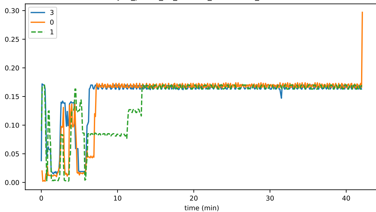
sync_phase_02_fraction_RECEIVING_EVENTS
