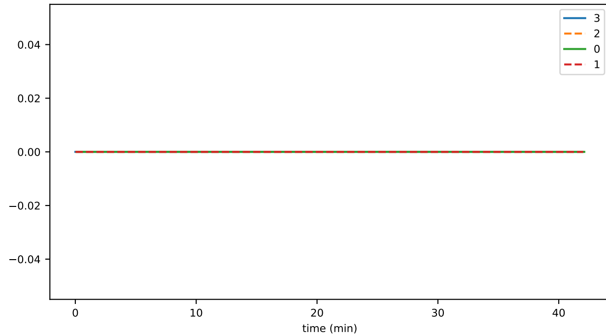
ds_files_hashesStoreFileCount_state
