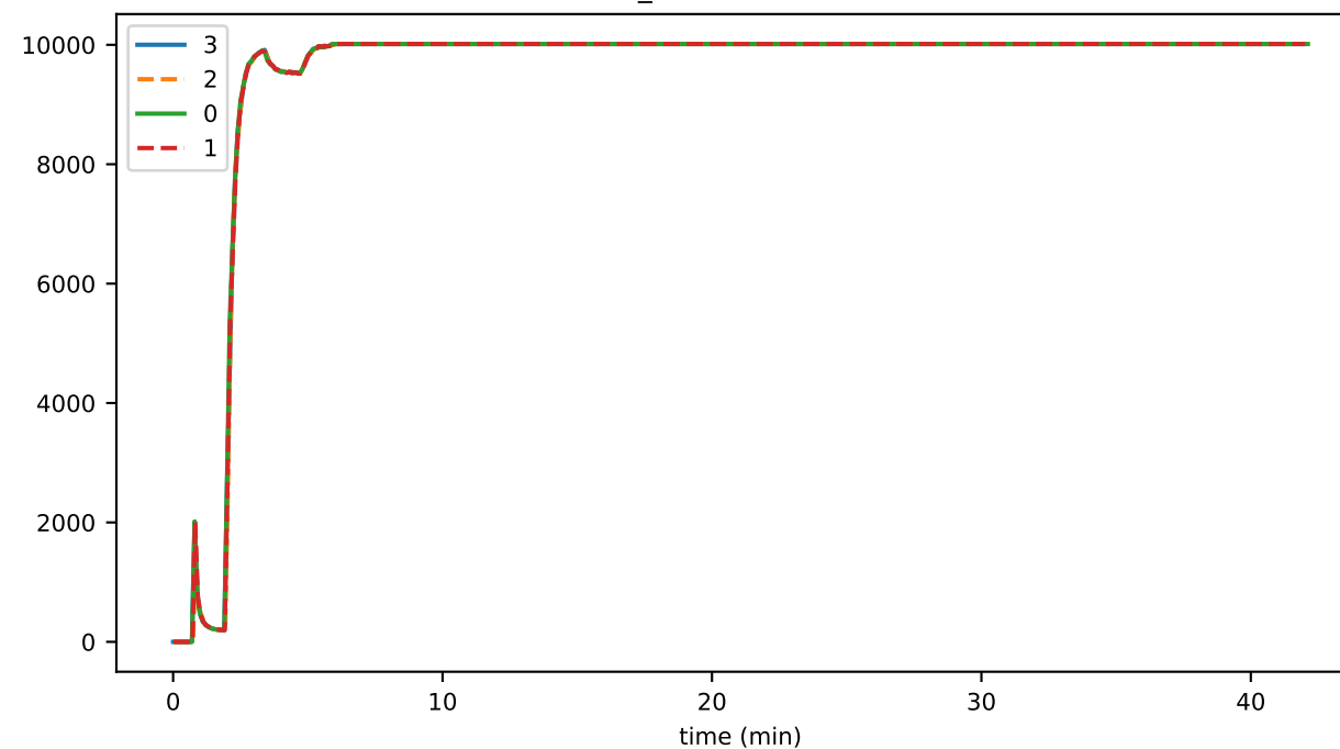
buffer_latestBlockOpened
