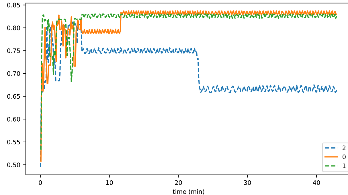
sync_phase_03_fraction_OTHER_FALLEN_BEHIND
