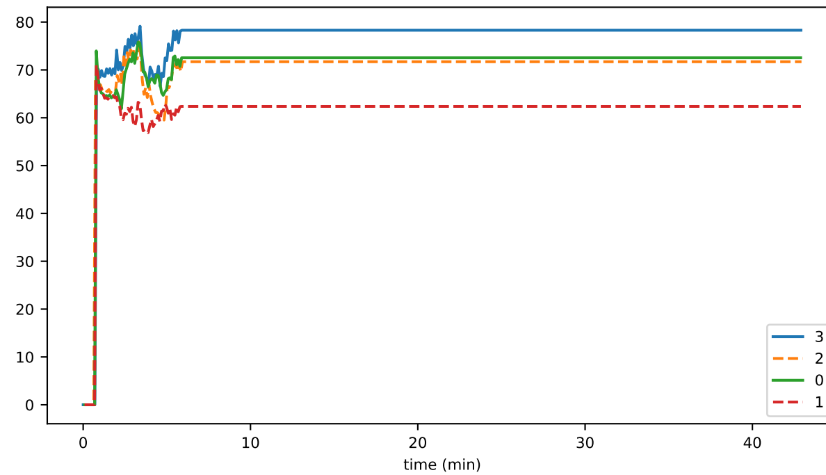
averageTimeToFullySignState
