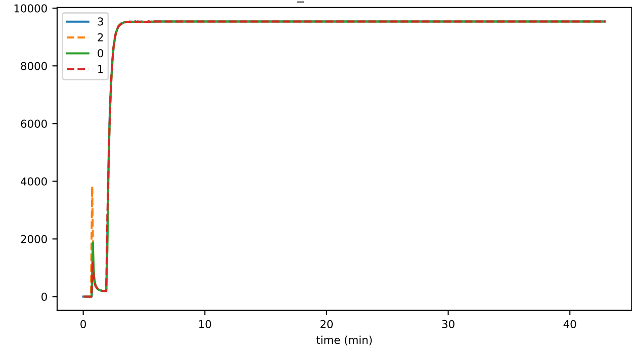
buffer_latestBlockOpened
