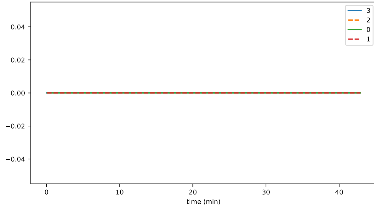
vmap_lifecycle_flushDurationMs_state
