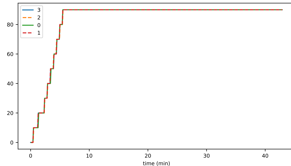
disconnects_per_sec_00
