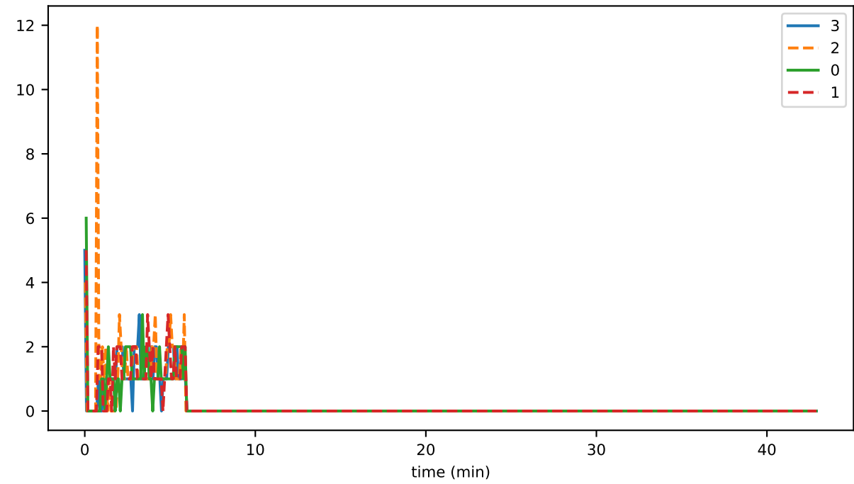
vmap_lifecycle_hashDurationMs_state
