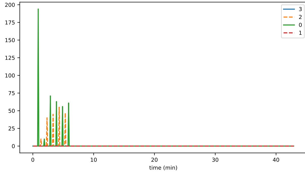
vmap_lifecycle_flushDurationMs_state
