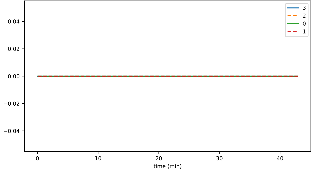
branchingNodeCount
