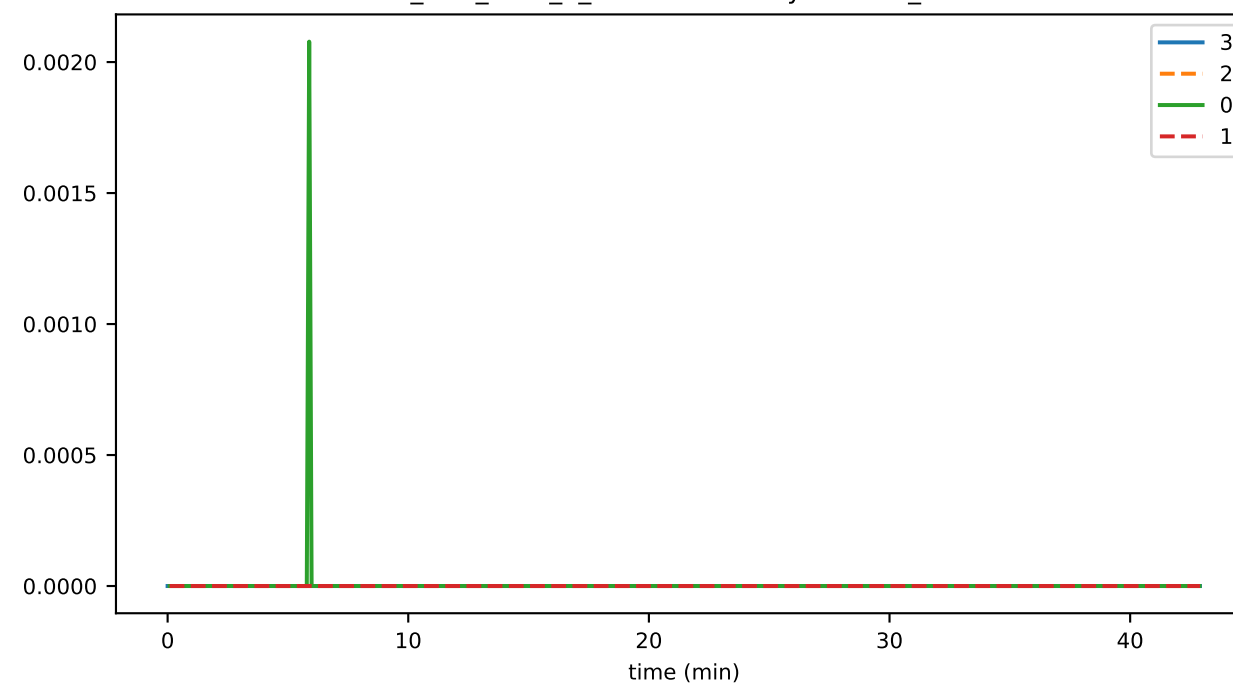
ds_files_level_2_leavesFileSizeByLevelMb_state
