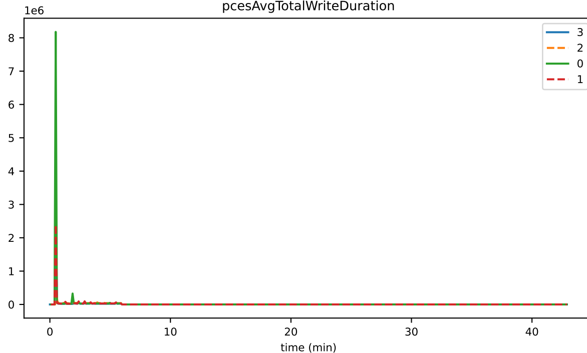
pcesAvgTotalWriteDuration
