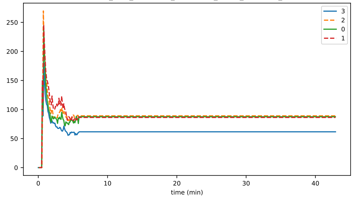
ConsensusEngine_busy_fraction
