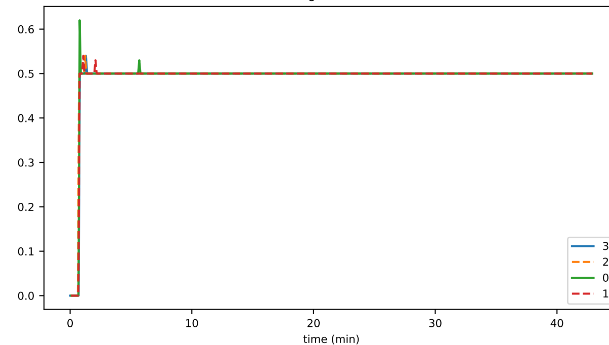
vmap_lifecycle_familySizeBackpressureMs_state
