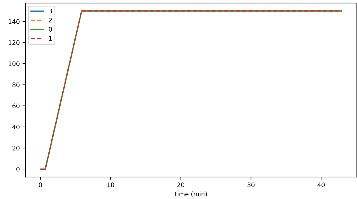
buffer_latestBlockOpened
