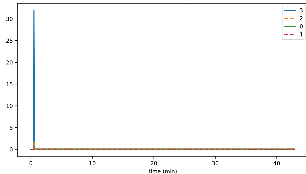
secR2C
