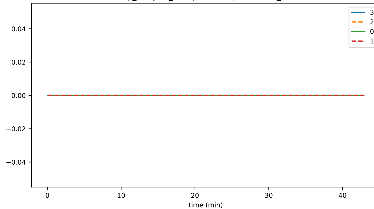
vmap_lifecycle_familySizeBackpressureMs_state
