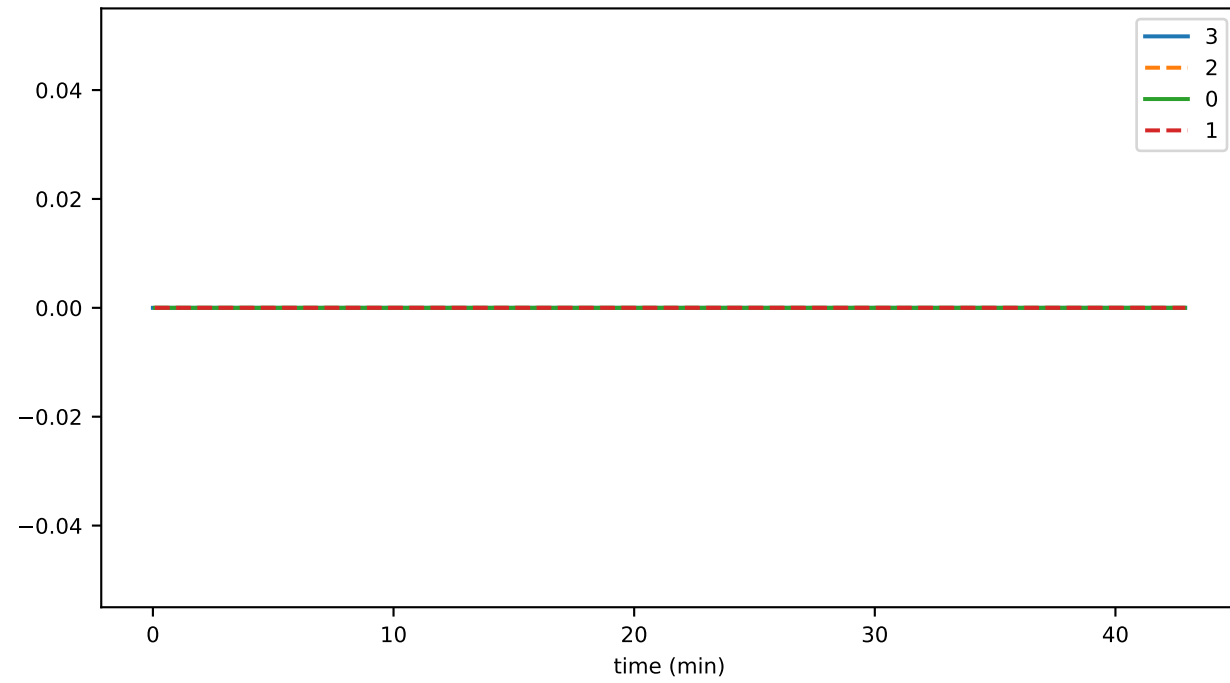
ds_compactions_level_2_hashesSavedSpaceMb_state
