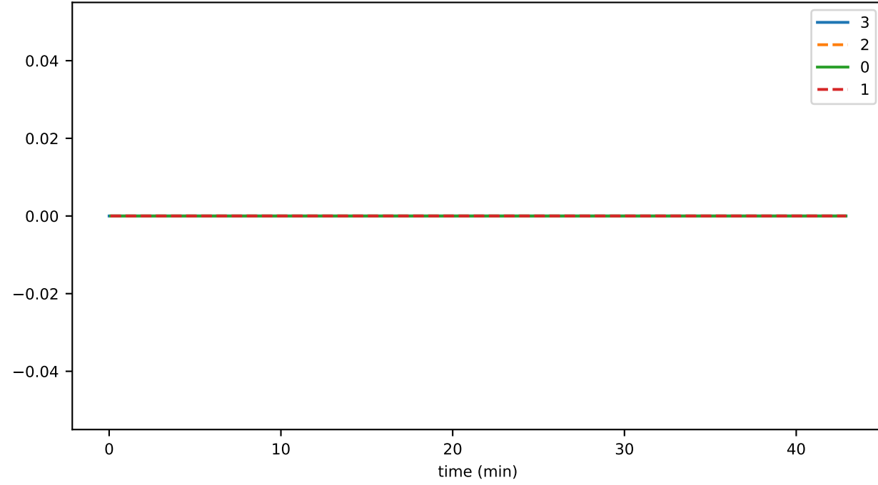
ds_compactions_level_6_hashesSavedSpaceMb_state
