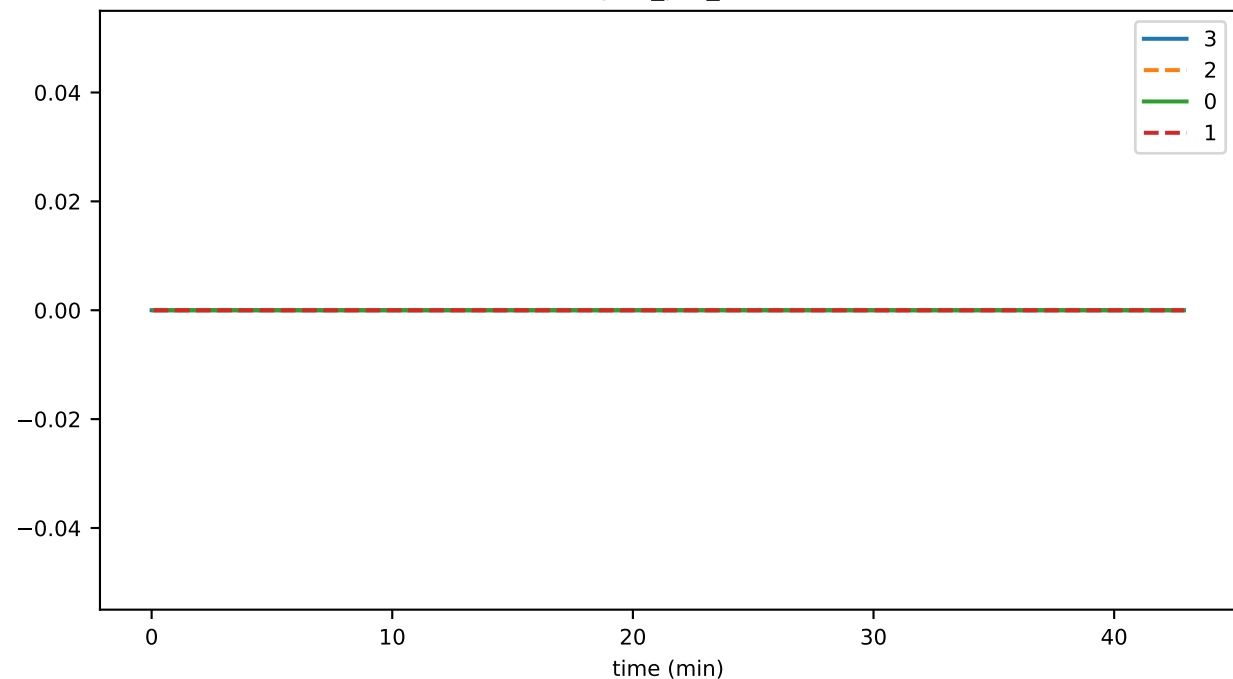
SmartContractService:FailedTransactionDuration_avg
