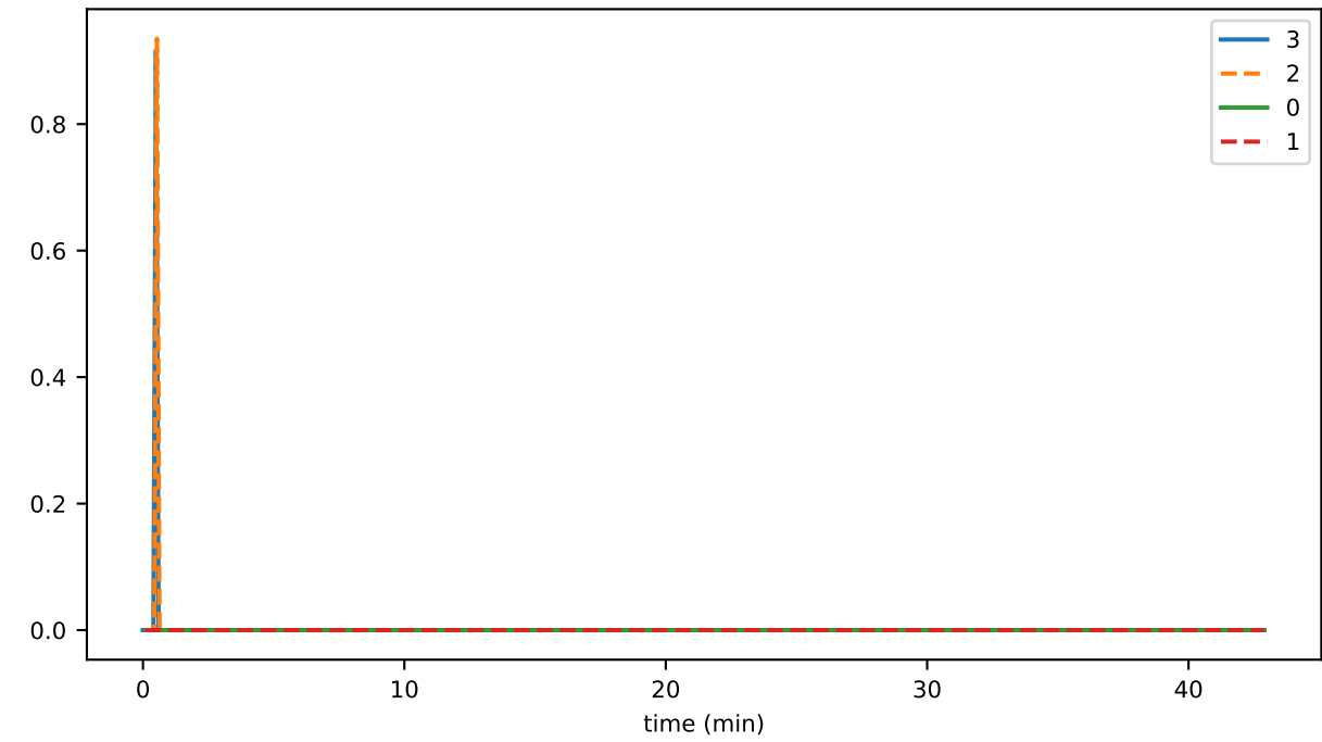
eventCreation_fraction_NO_ELIGIBLE_PARENTS
