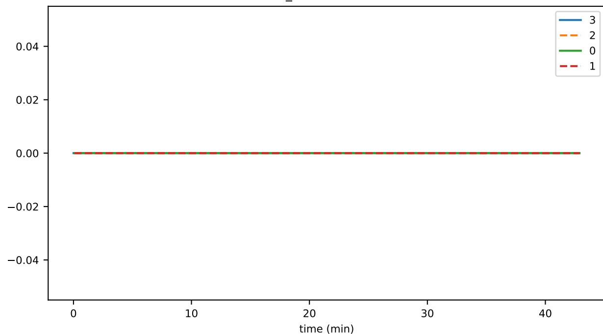
buffer_saturation
