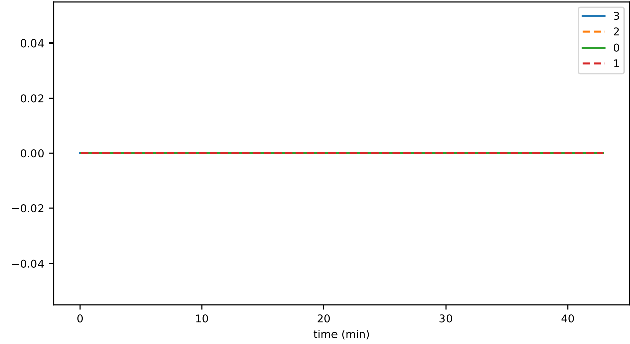
ds_files_level_9_leafKeysFileSizeByLevelMb_state
