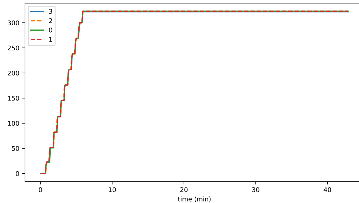
preconsensusEventFileOldestSeconds
