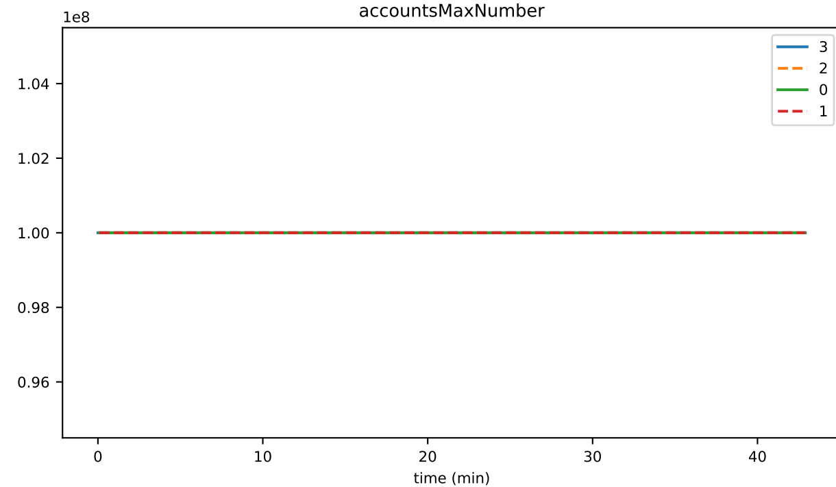
accountsMaxNumber
