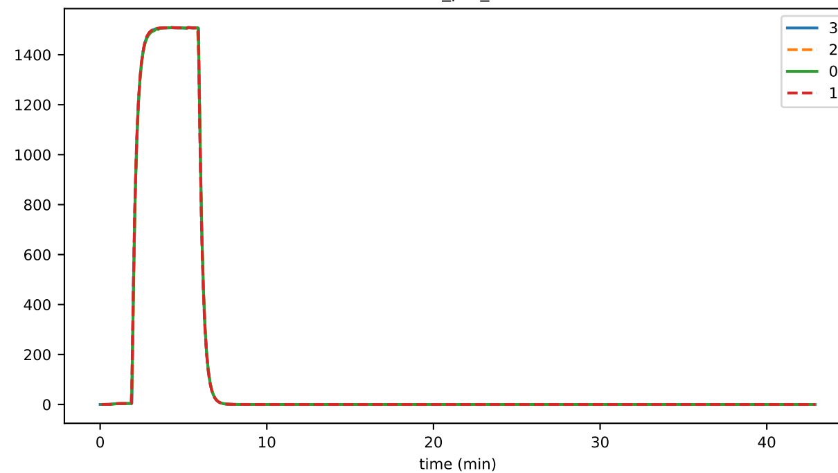
trans_per_sec
