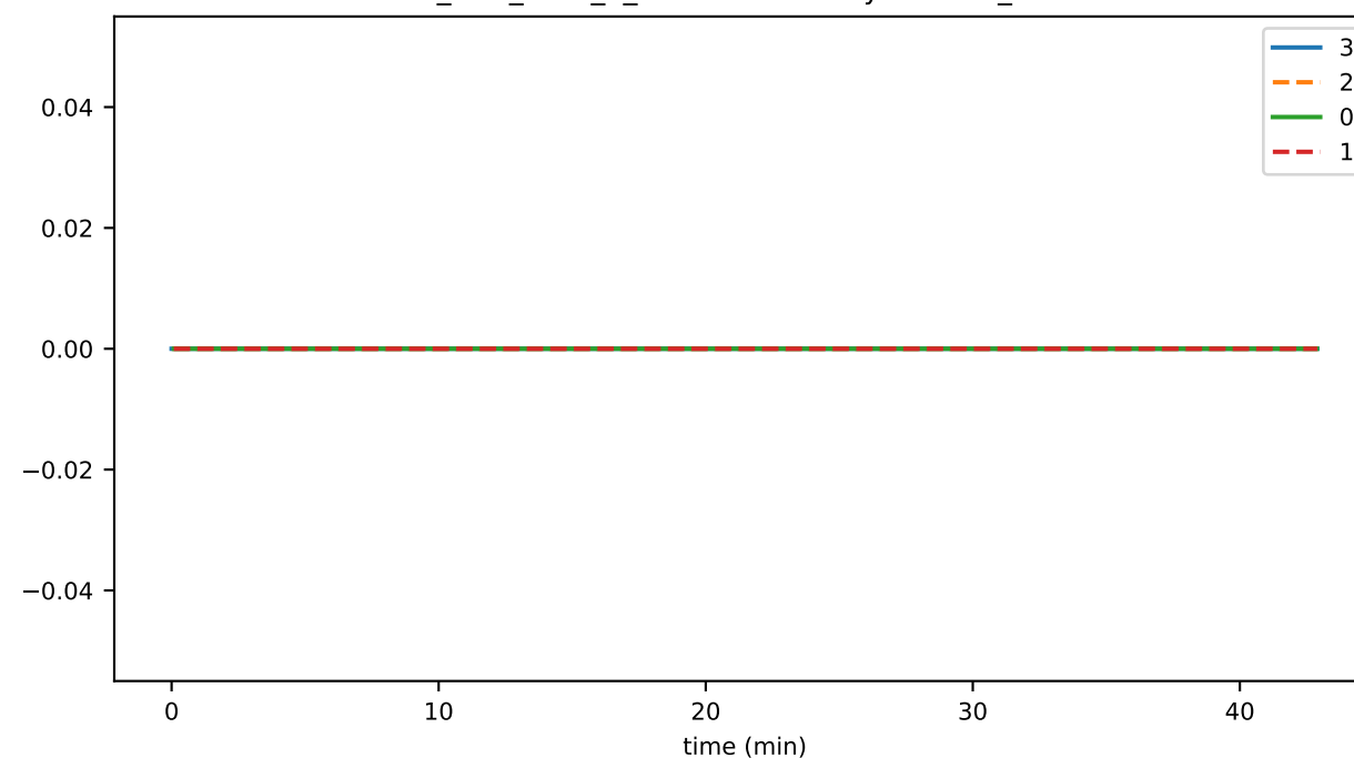
ds_files_level_2_leavesFileSizeByLevelMb_state
