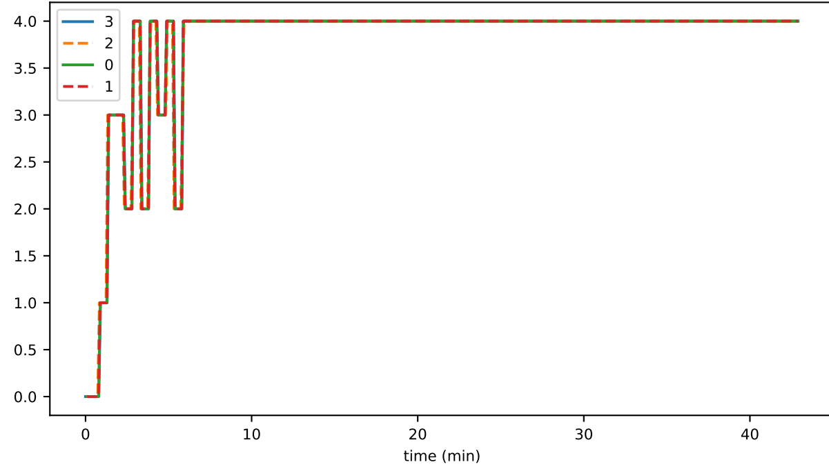
ds_files_hashesStoreFileCount_state
