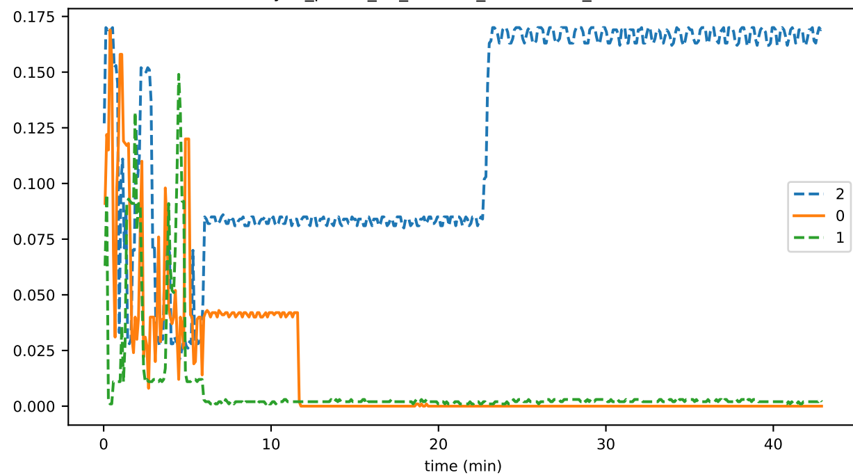
sync_phase_03_fraction_RECEIVING_EVENTS
