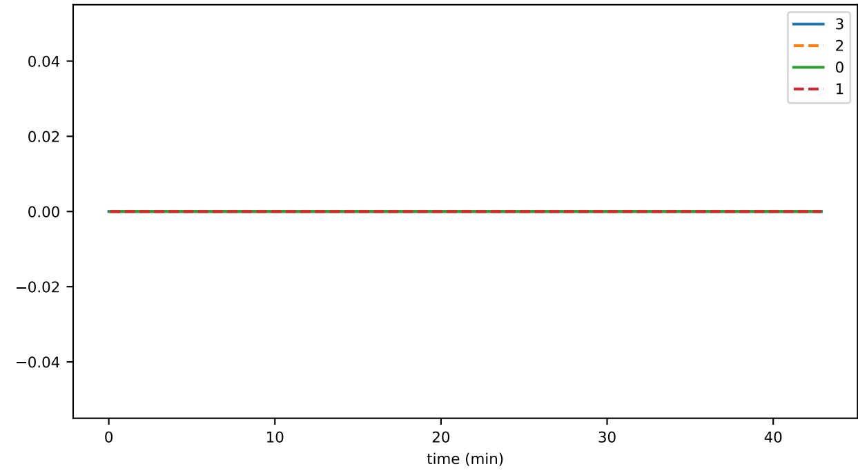
ds_files_level_9_leafKeysFileSizeByLevelMb_state
