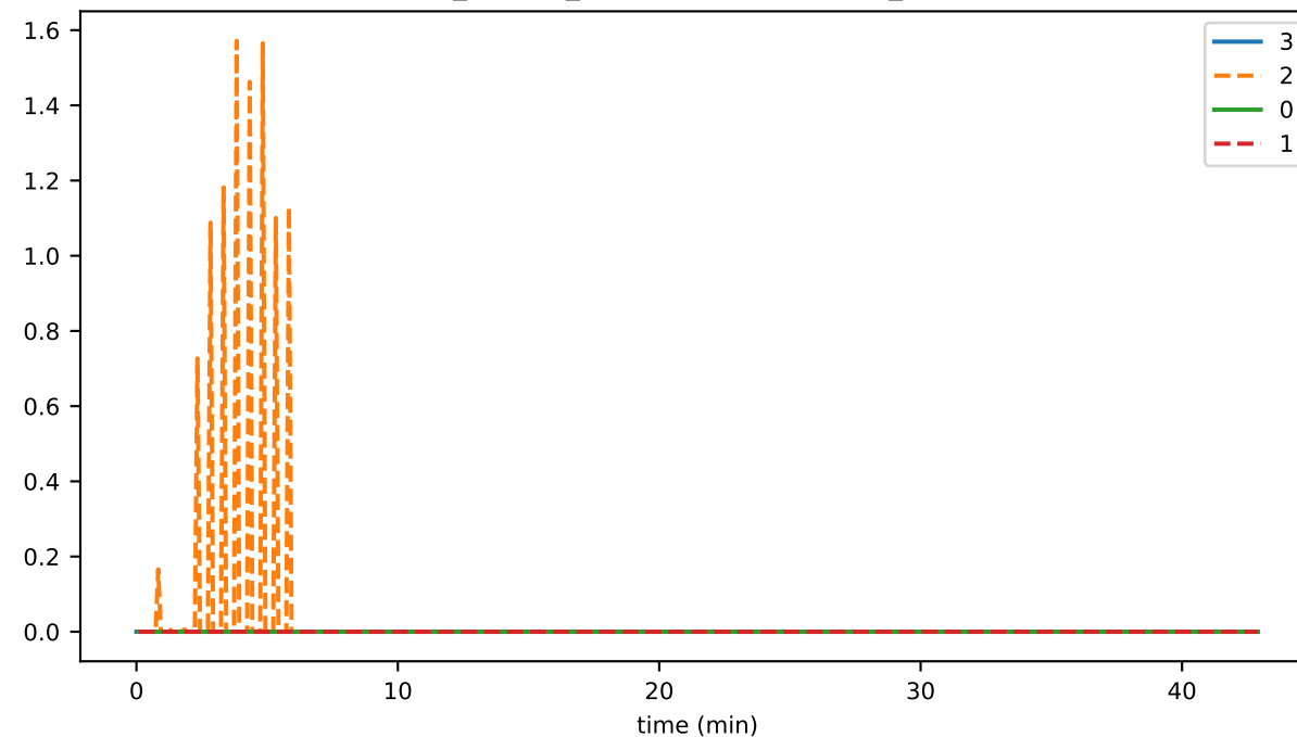
ds_flushes_leavesStoreFileSizeMb_state
