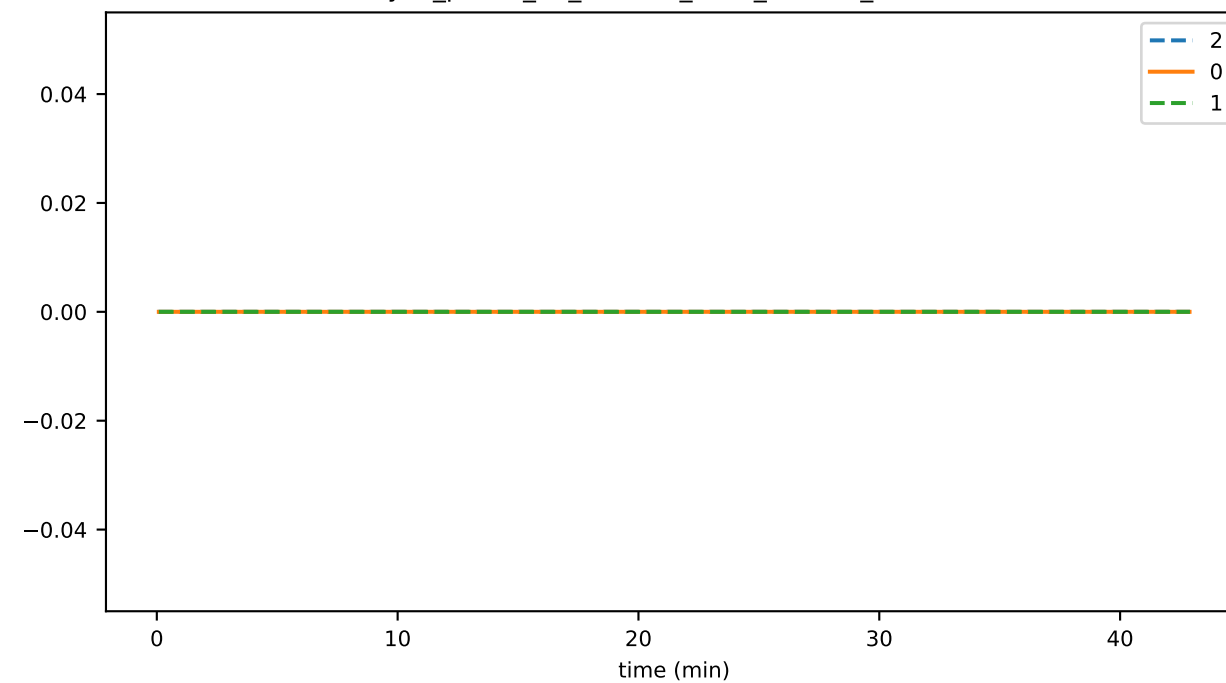
sync_phase_03_fraction_SELF_FALLEN_BEHIND
