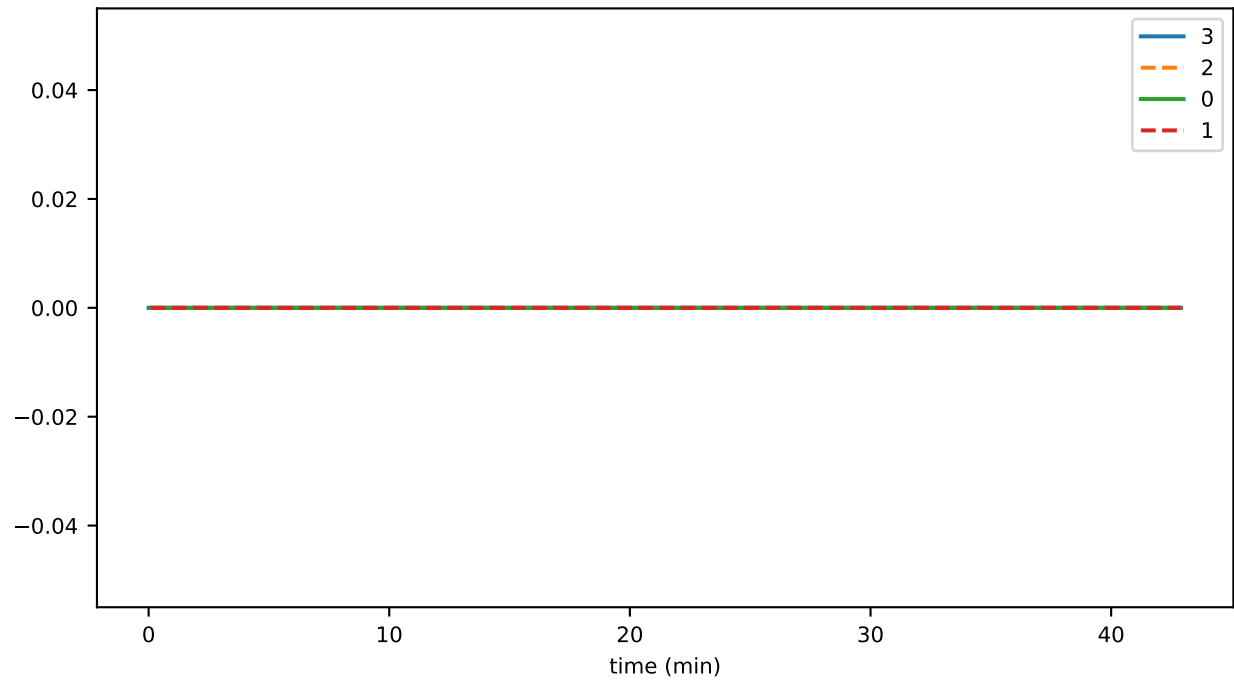
ds_compactions_level_2_hashesTimeMs_state
