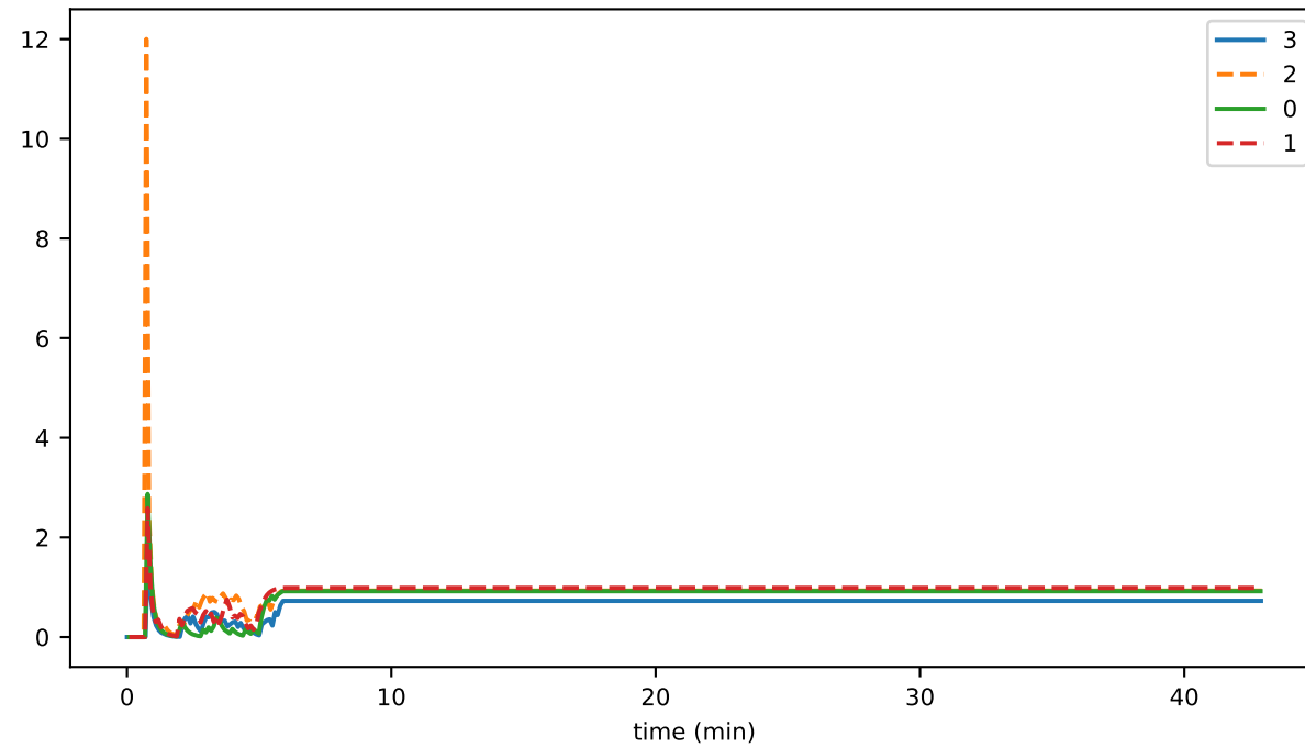
sigStateHash
