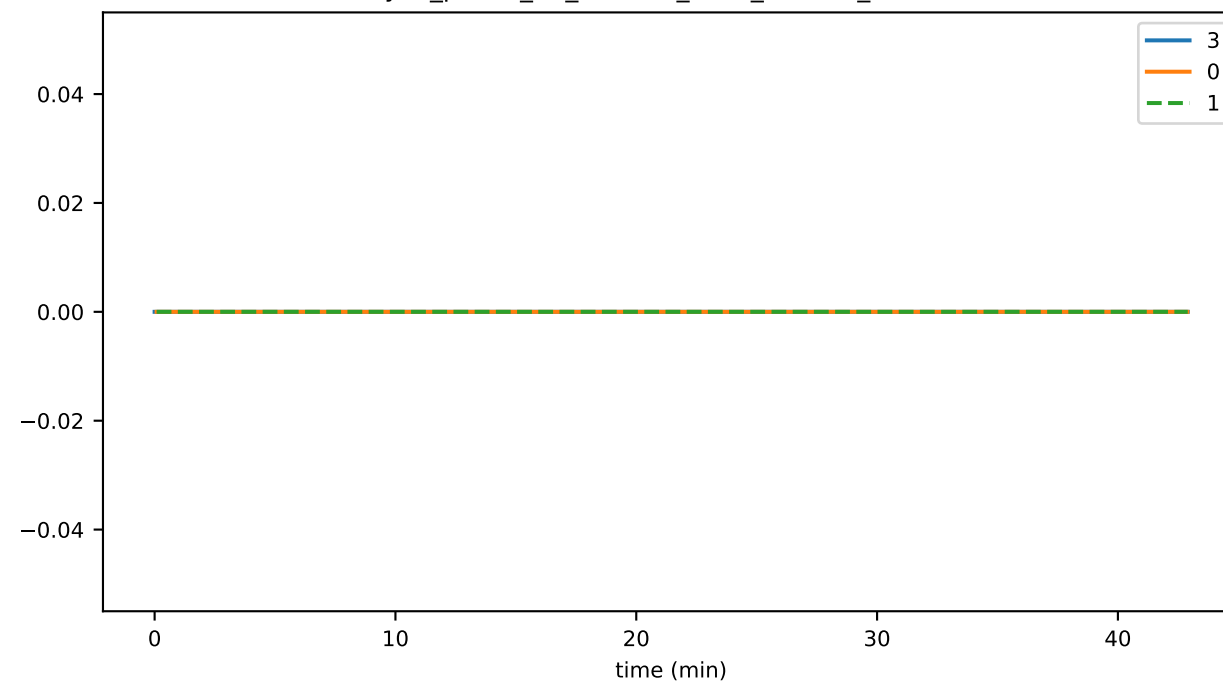
sync_phase_02_fraction_SELF_FALLEN_BEHIND
