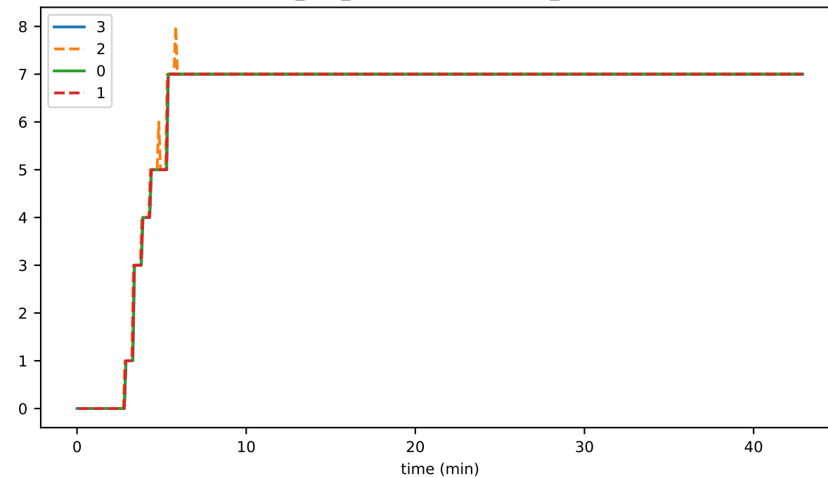
ds_files_leavesStoreFileSizeMb_state
