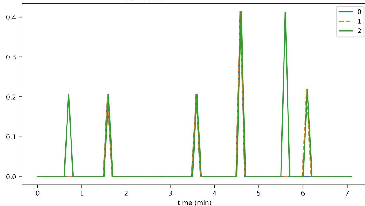
ds_files_level_2_hashesFileSizeByLevelMb_state
