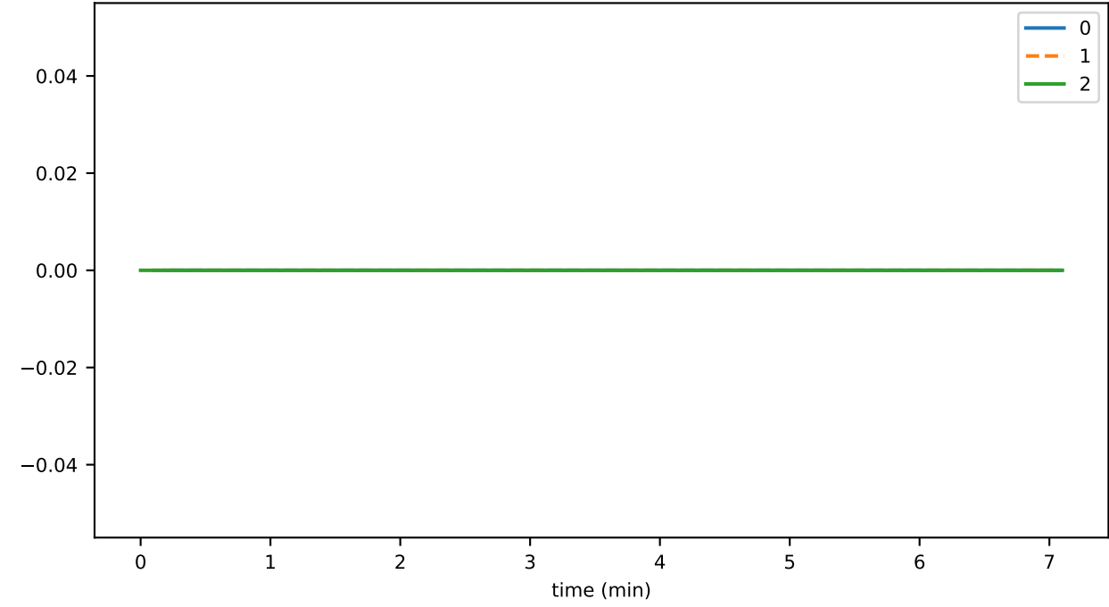
cryptoGetLiveHashDurationAvg
