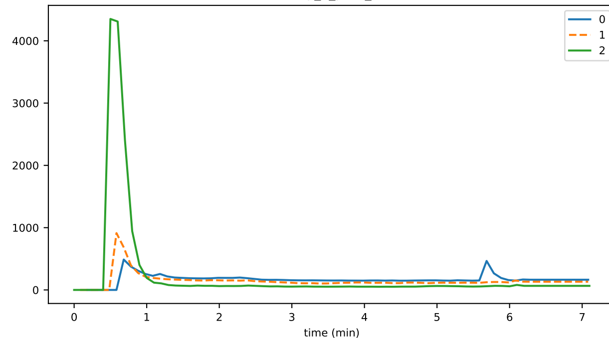
eventDelay_6_pces_storage
