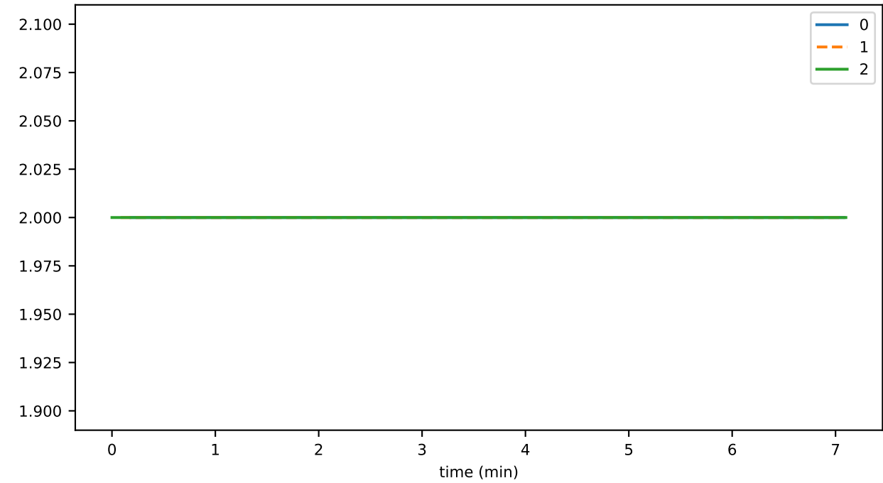
oldestSignedStateSeconds
