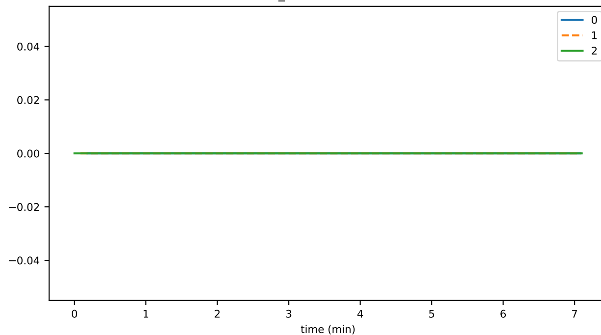
connRecv_latestBlockSkipBlock
