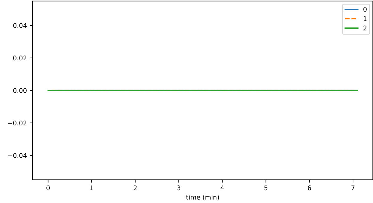
historyProofTransR1ToFailCnt
