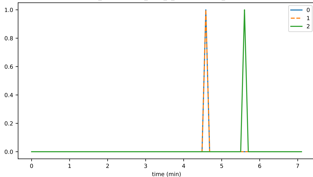
ds_compactions_level_3_leavesTimeMs_state
