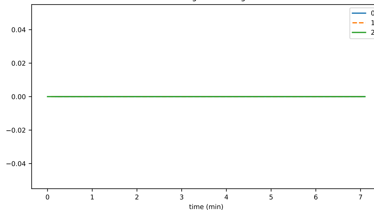
utilPrngThrottledTxns
