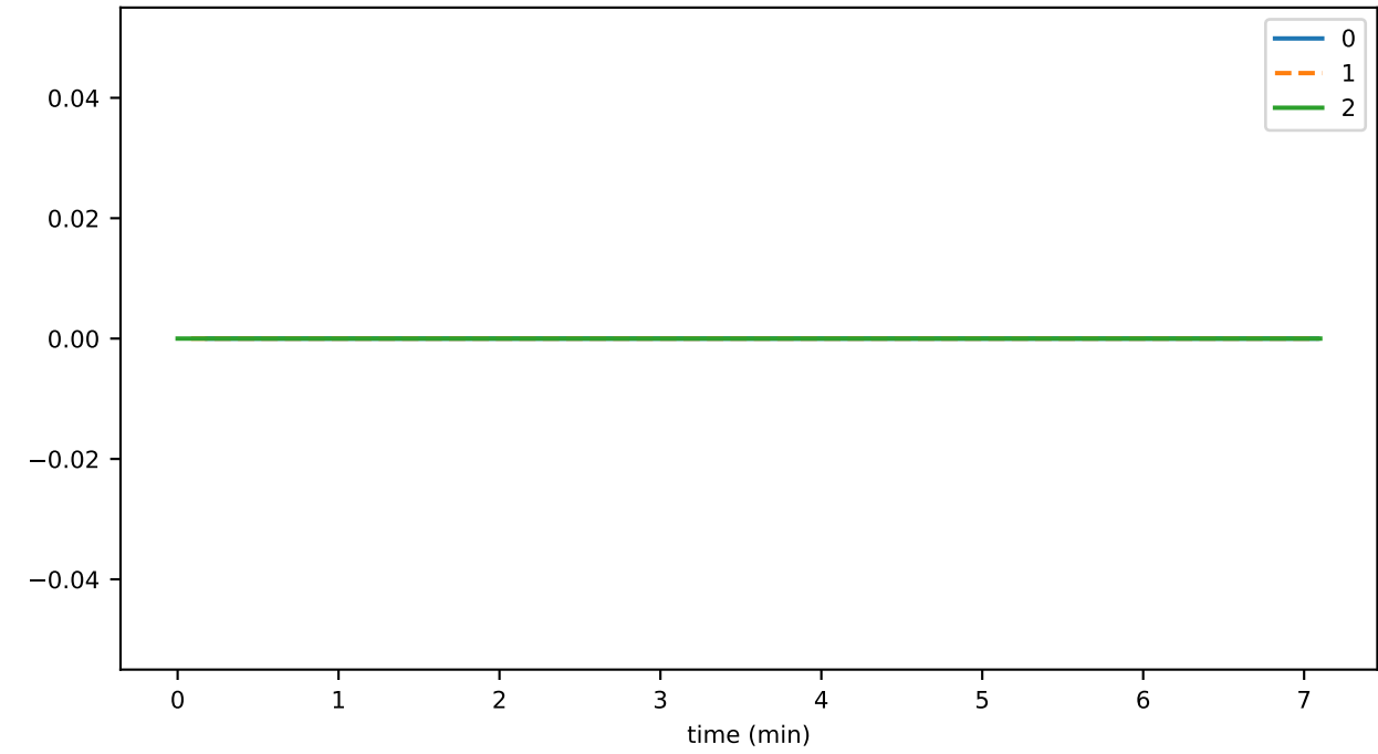
historyProofTransR1ToFailCnt
