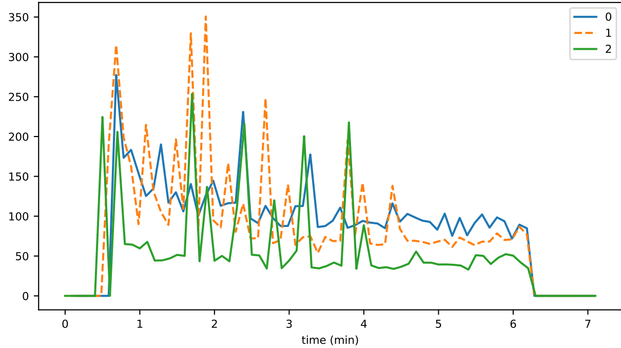
eventDelay_3_deduplication_storageMAX
