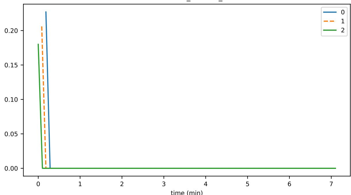
eventCreation_fraction_IDLE
