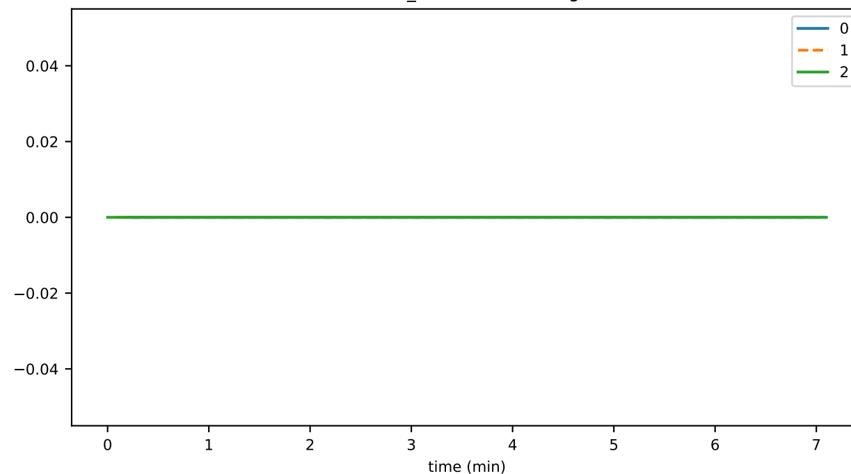
buffer_numBlocksPruned
