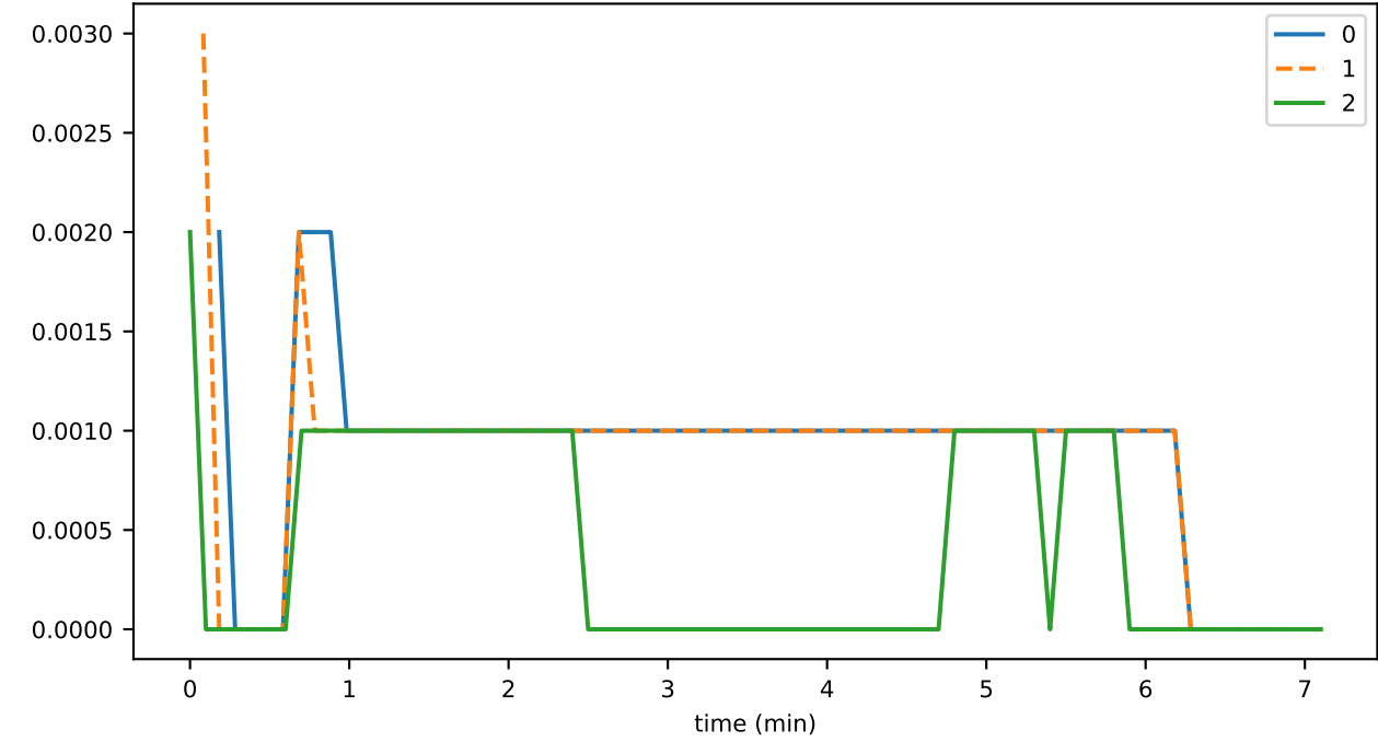
EventDeduplicator_busy_fraction
