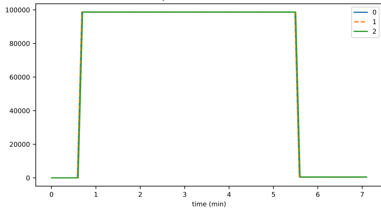
historyProofTransWMetaToWasmMs
