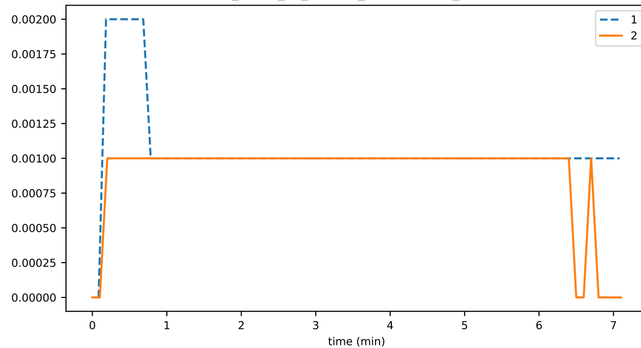
sync_phase_00_fraction_EXCHANGING_EVENTS
