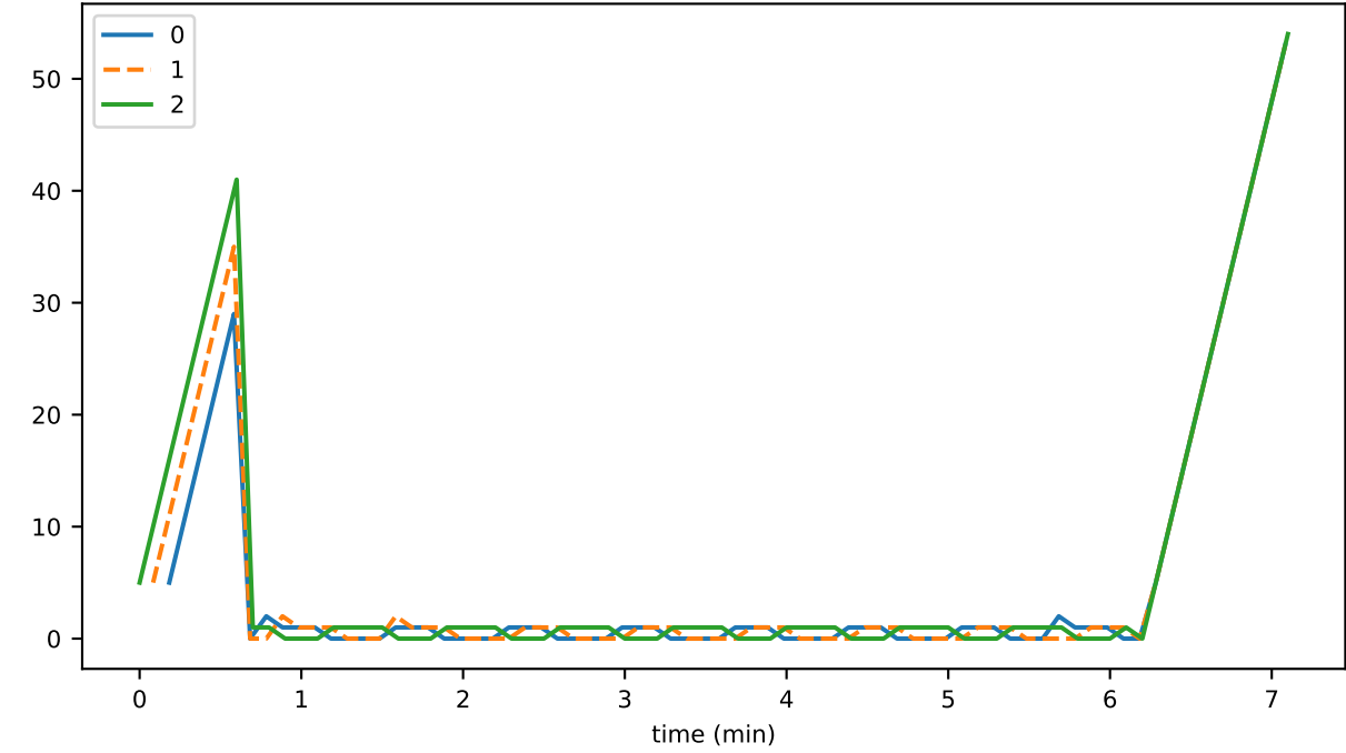
oldestSignedStateSeconds
