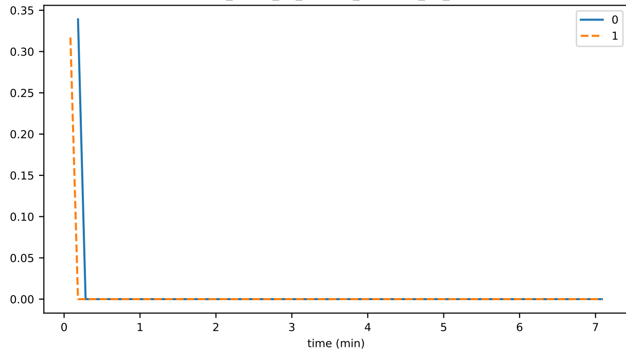
sync_phase_02_fraction_OUTSIDE_OF_RPC
