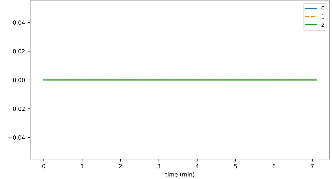
EventManager_unhandled_task_count
