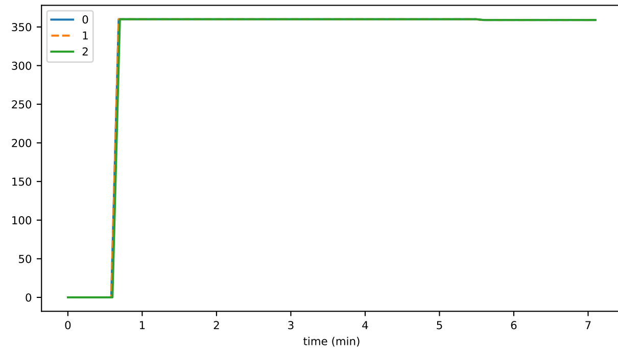
historyProofTransR2ToR3Ms
