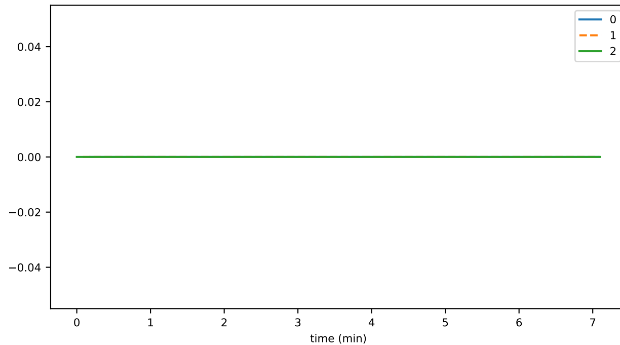
blockNodeRewardsEligibleCount
