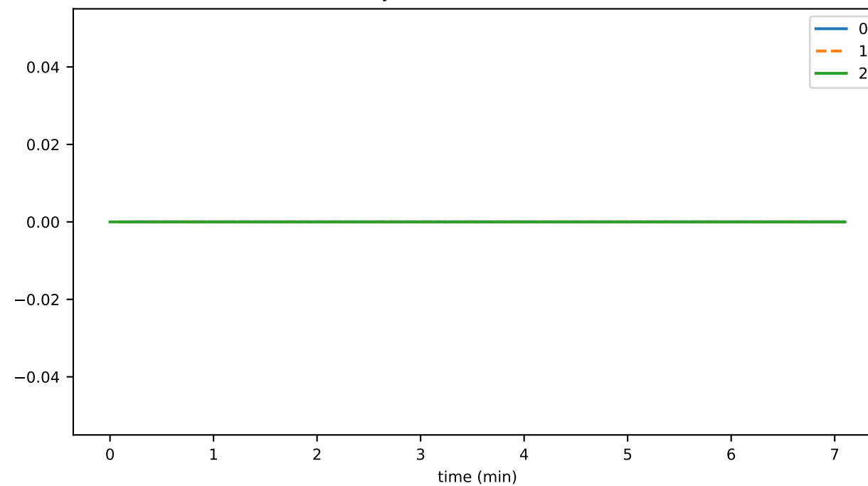
historyProofTransWasmToFailCnt
