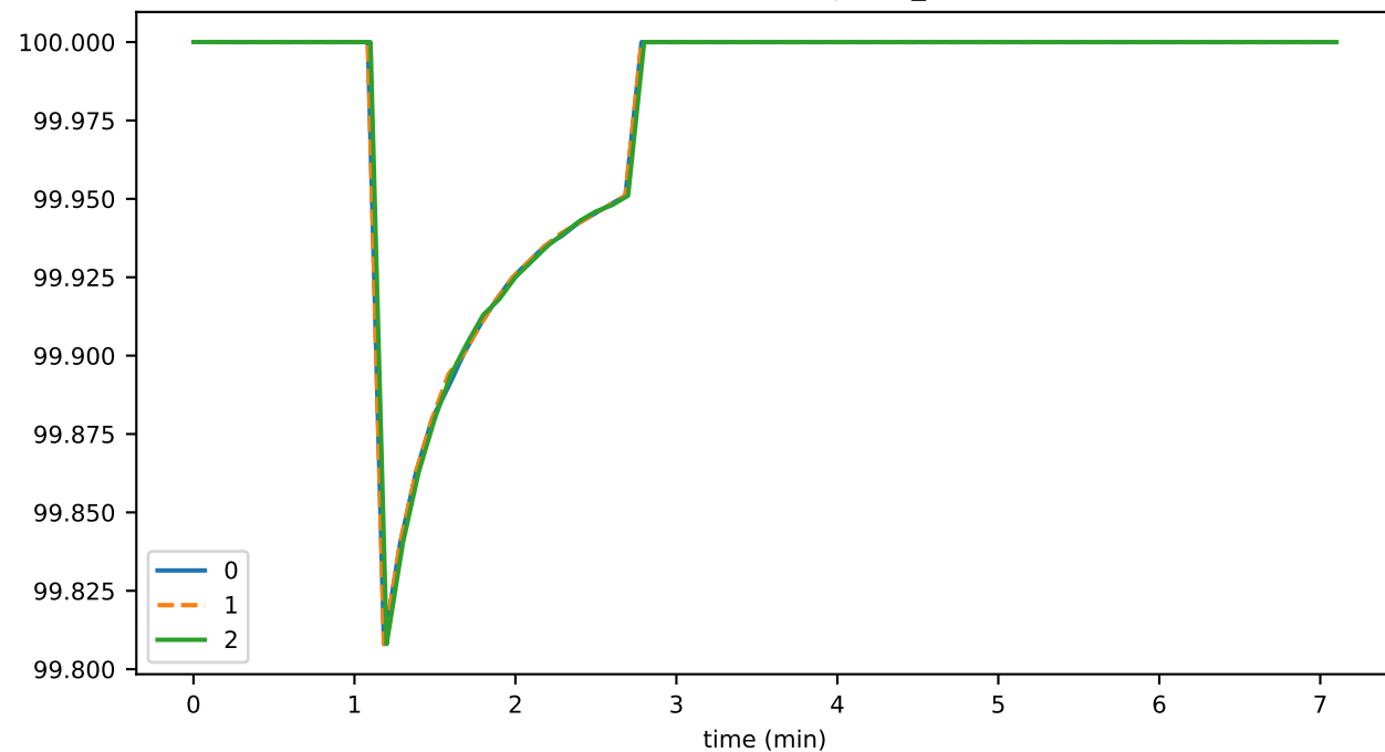
nodeCreateDurationAvg
