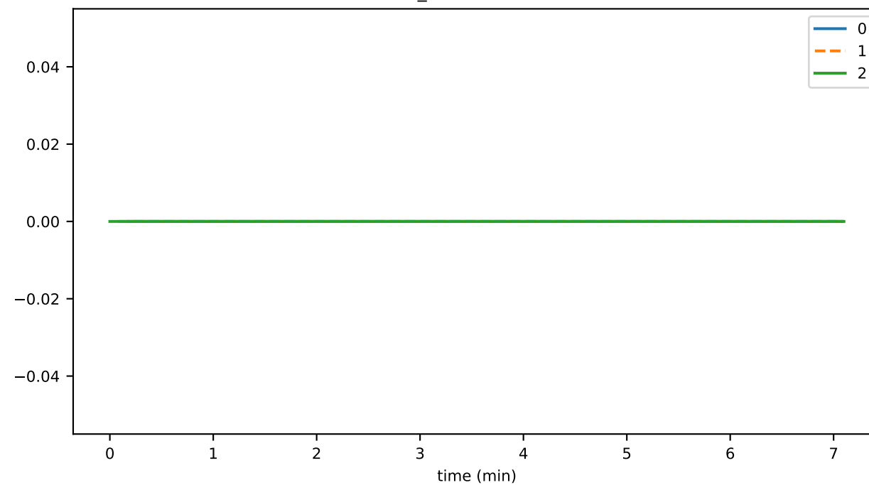
buffer_numBlocksPruned
