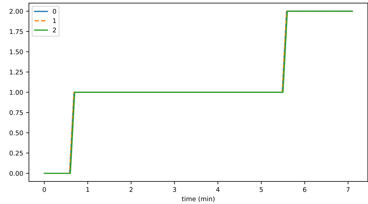
historyProofTransR3ToAggCnt
