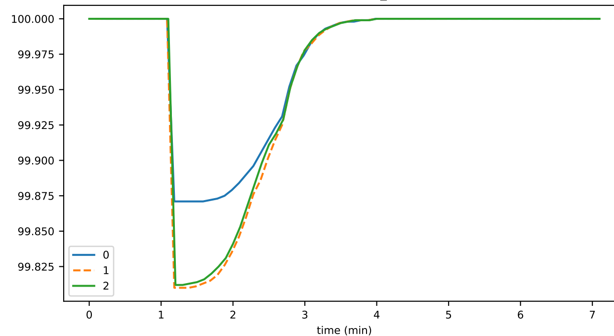
nodeActivePercentSnapshot_node0
