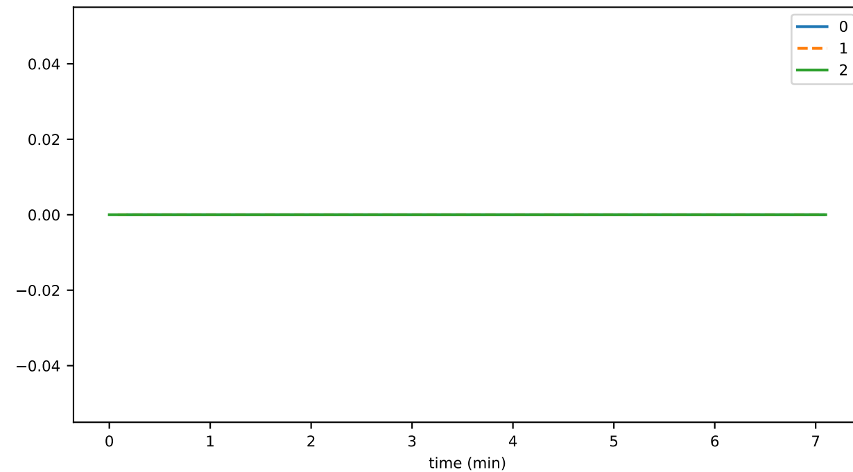
nodeCreateDurationMax
