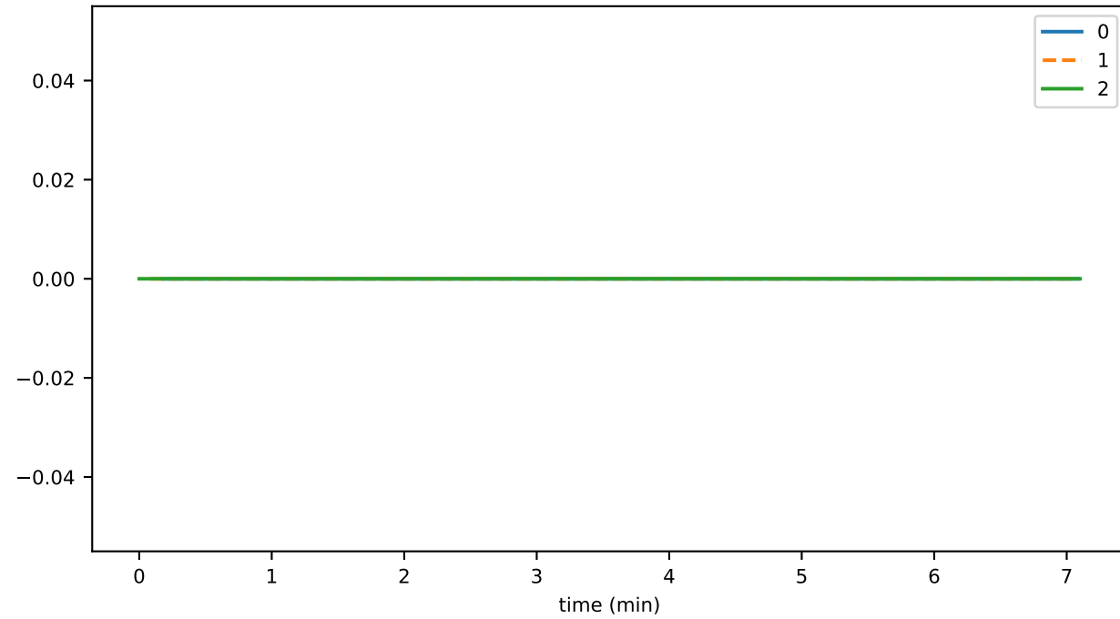
ds_compactions_level_6_leafKeysTimeMs_state
