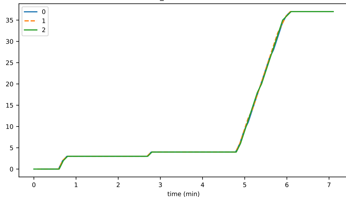
buffer_numBlocksOpened
