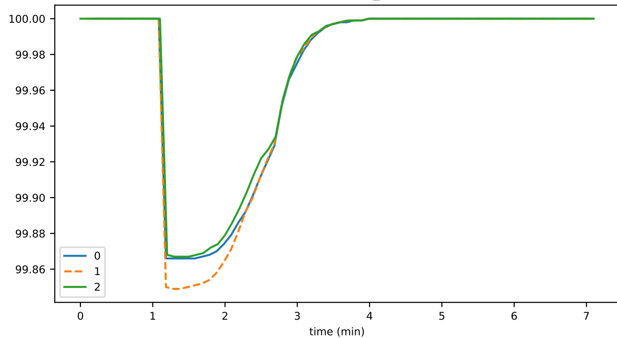
nodeActivePercent_node2
