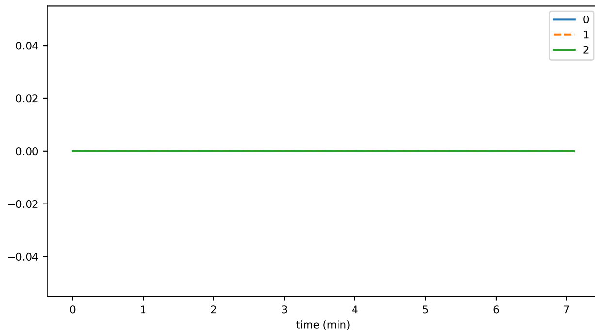
eventsWithInvalidParents
