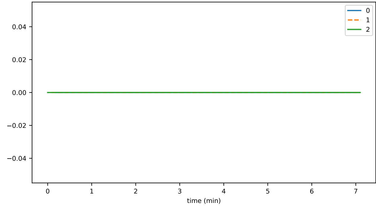
SmartContractService:SystemContractMethodCall_ALLOWANCE_failed
