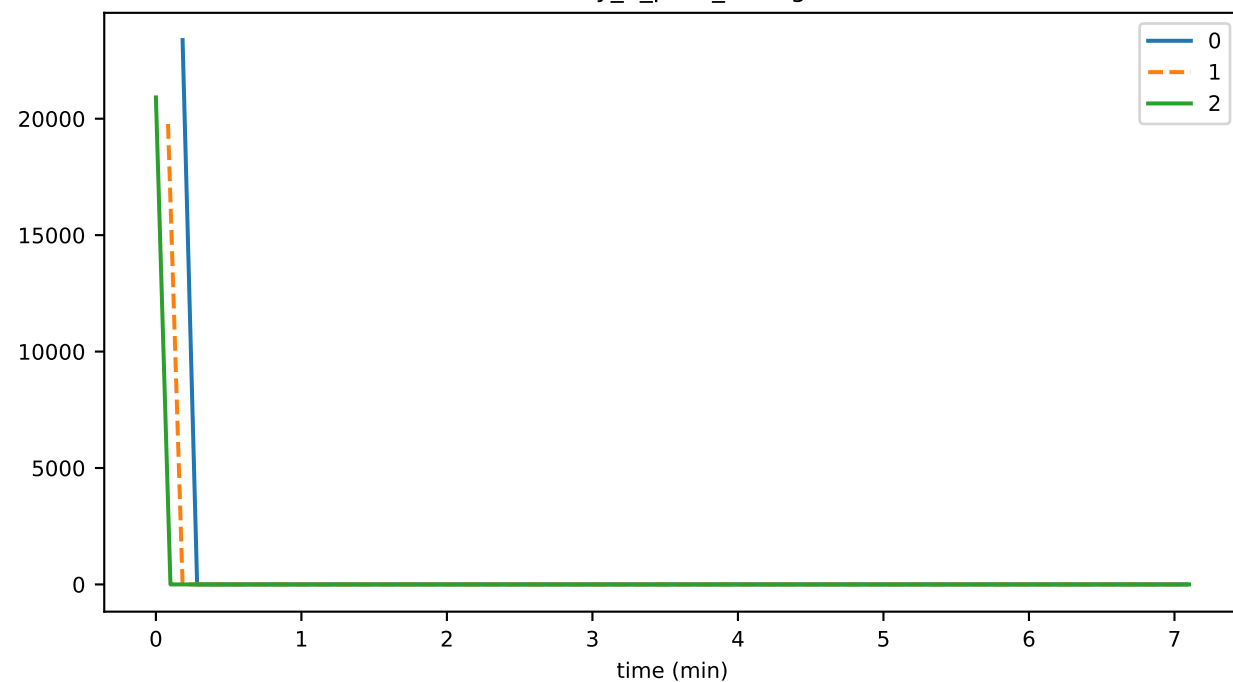
eventDelay_7_consensus_gossipMAX
