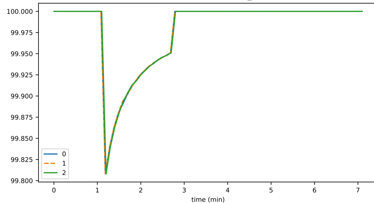
nodeCreateDurationMax
