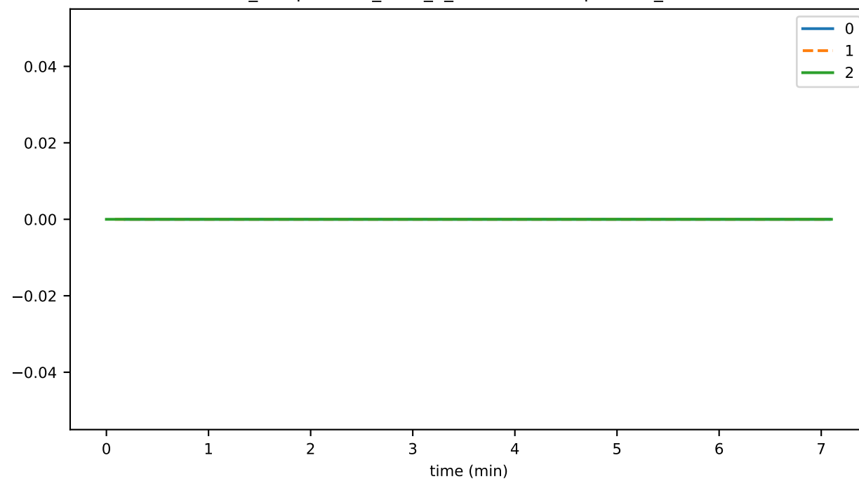
ds_compactions_level_0_leafKeysSavedSpaceMb_state
