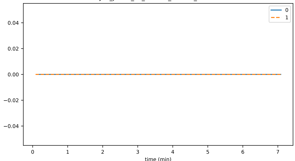
sync_phase_02_fraction_GOSSIP_HALTED
