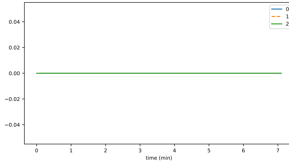
atomicBatchDurationAvg
