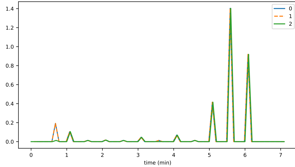
ds_offheap_dataSourceMb_state
