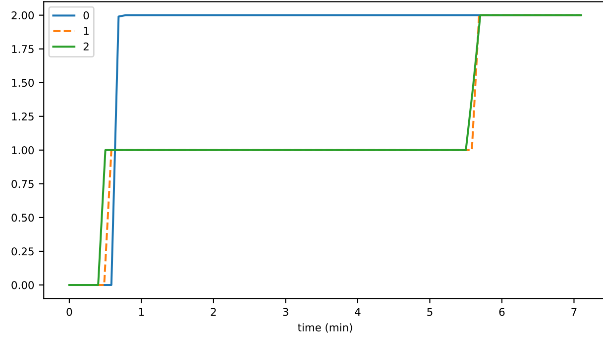
createdEventParents
