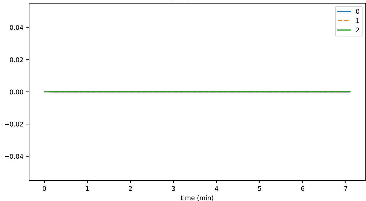
eventCreation_fraction_IDLE
