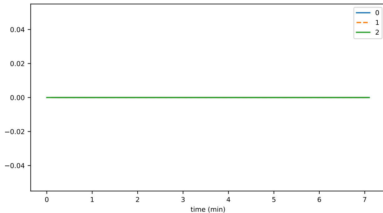
consThroughputLimitsPercentUsed
