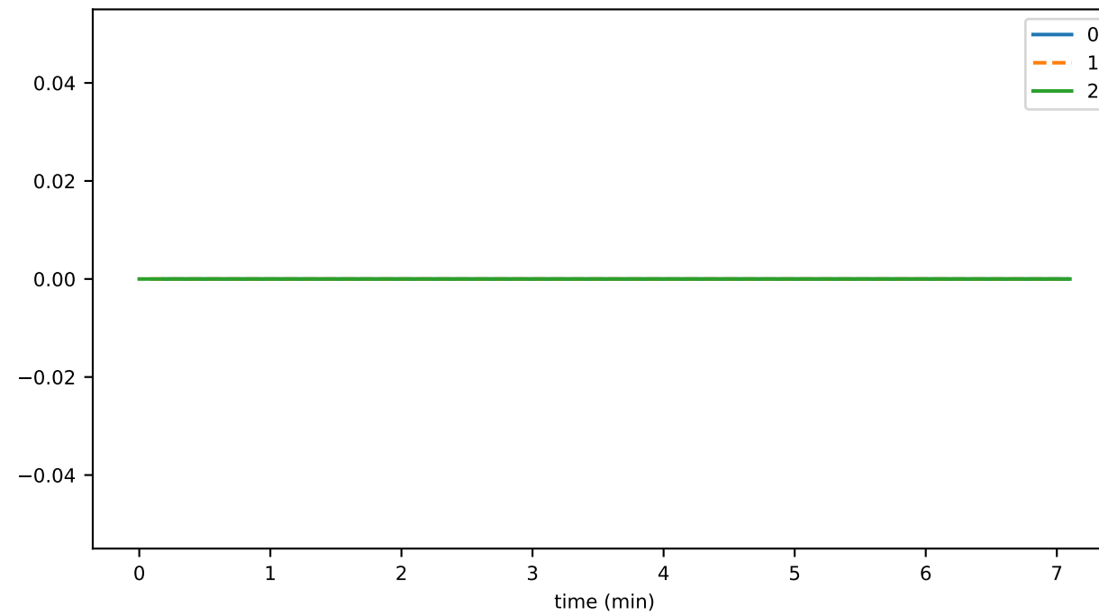
queriedAccountBalances
