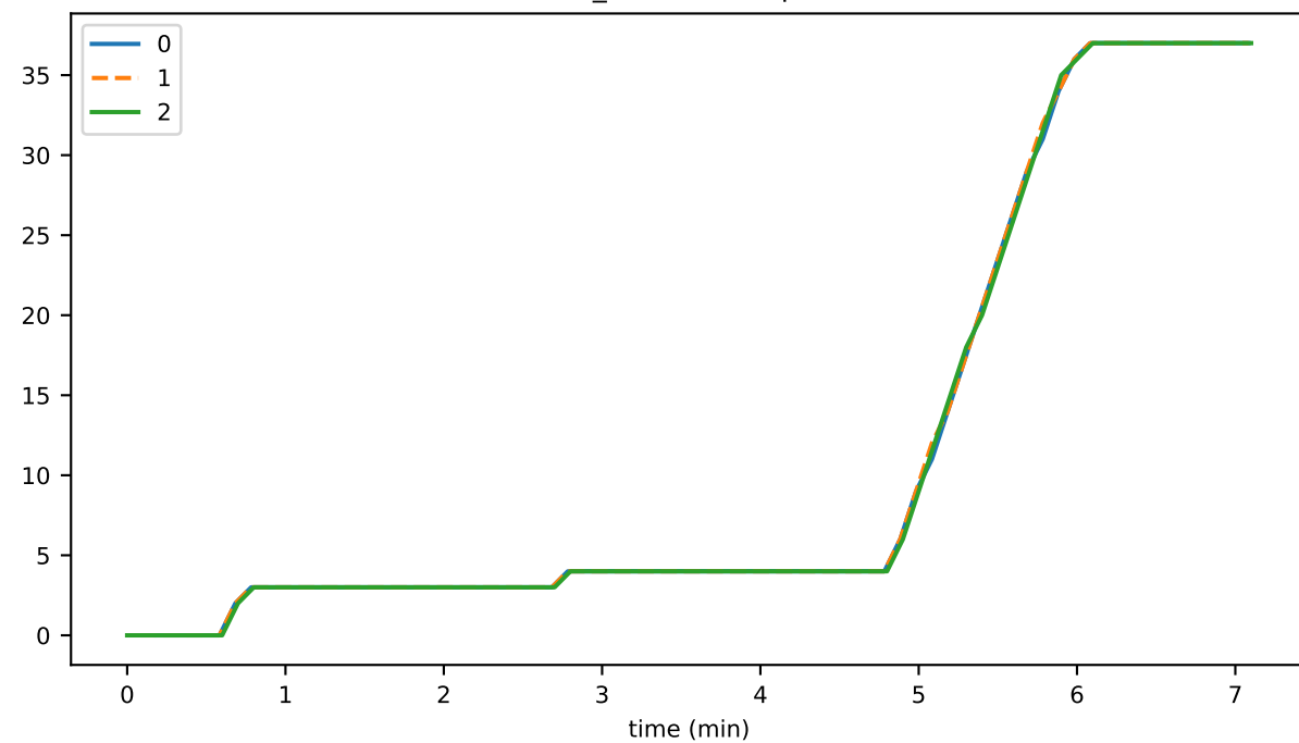
buffer_numBlocksOpened
