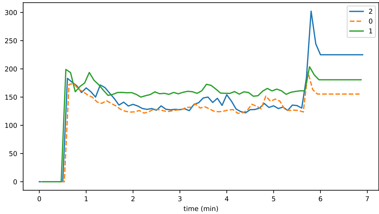
timeToDeleteState
