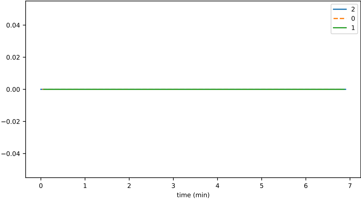
SmartContractService:SystemContractMethodCall_HAS_failed
