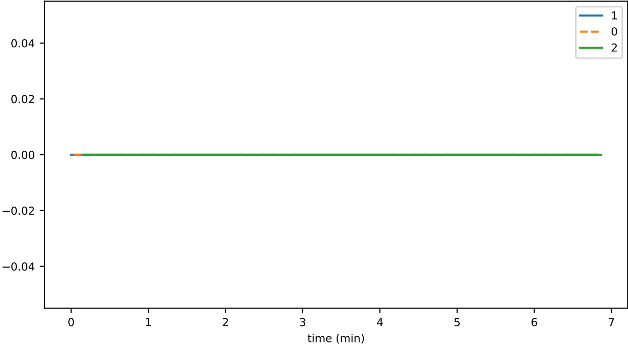
SmartContractService:SystemContractMethodCall_TRANSFER_total
