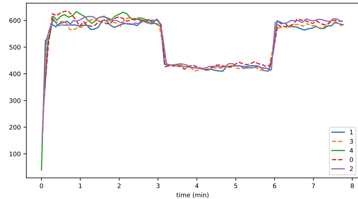
dupEvPercent
