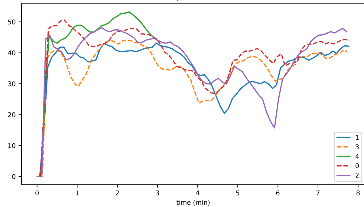
dupEvPercent
