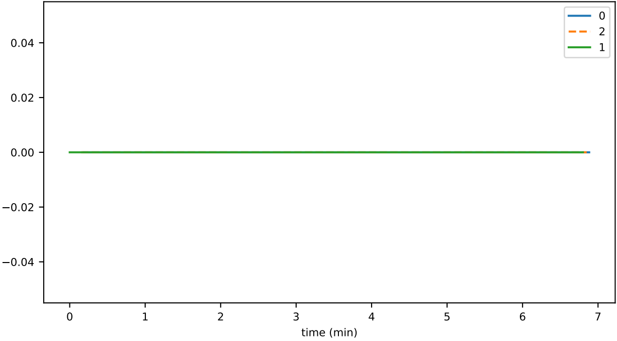
SmartContractService:SystemContractMethodCall_HSS_failed
