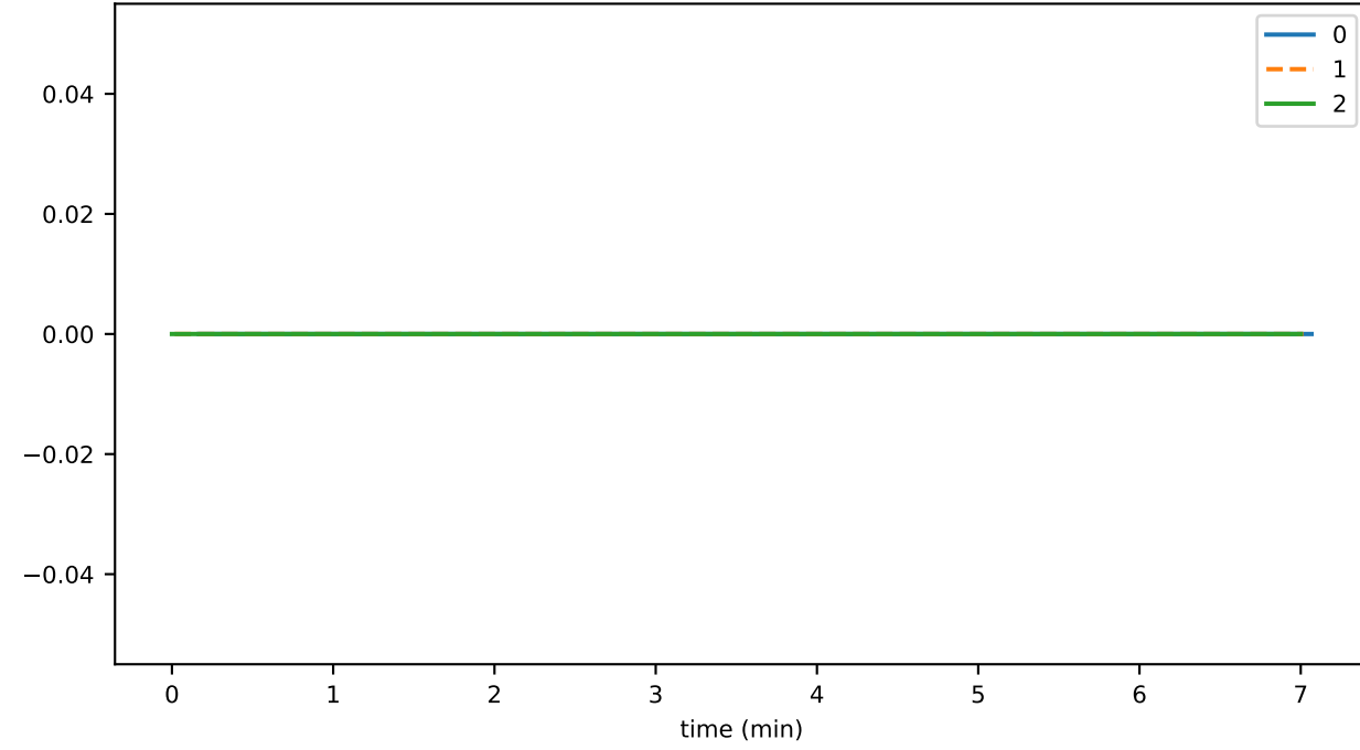
hookStoreDurationMax
