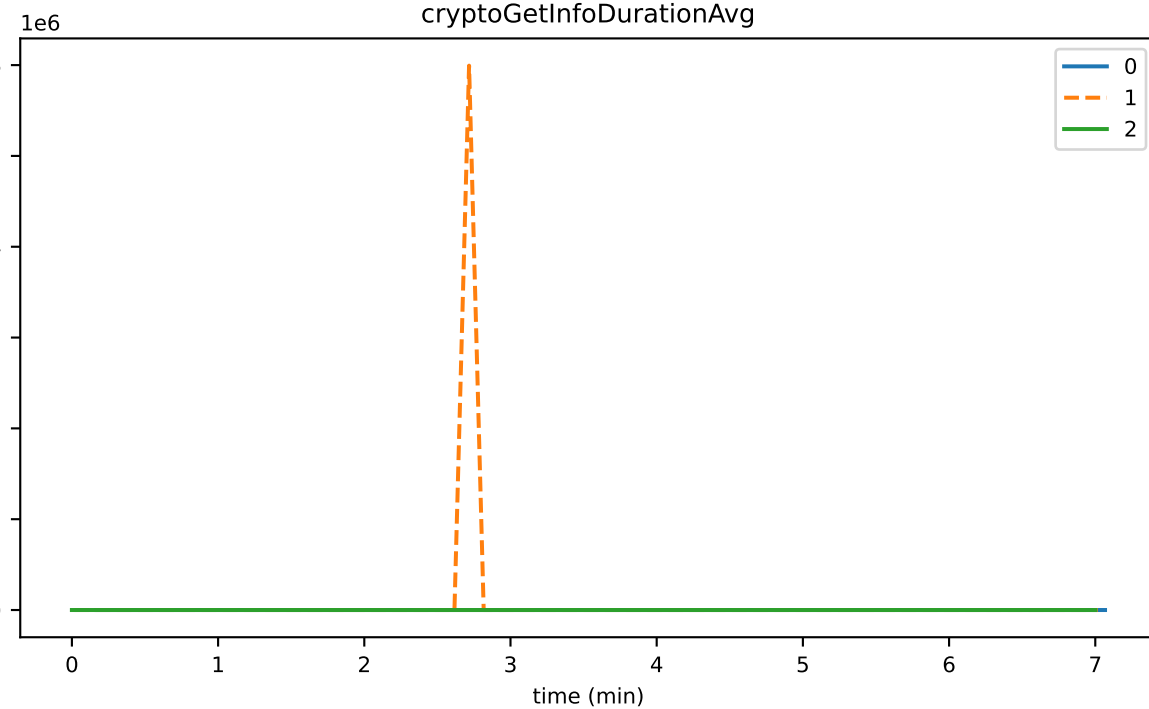
cryptoGetInfoDurationAvg
