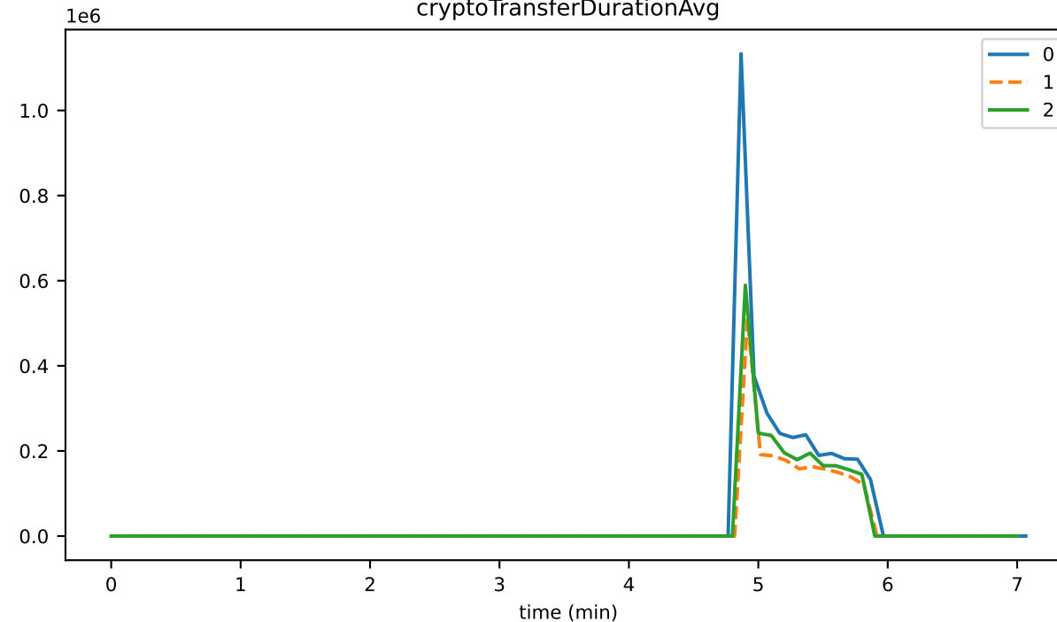
cryptoTransferDurationAvg
