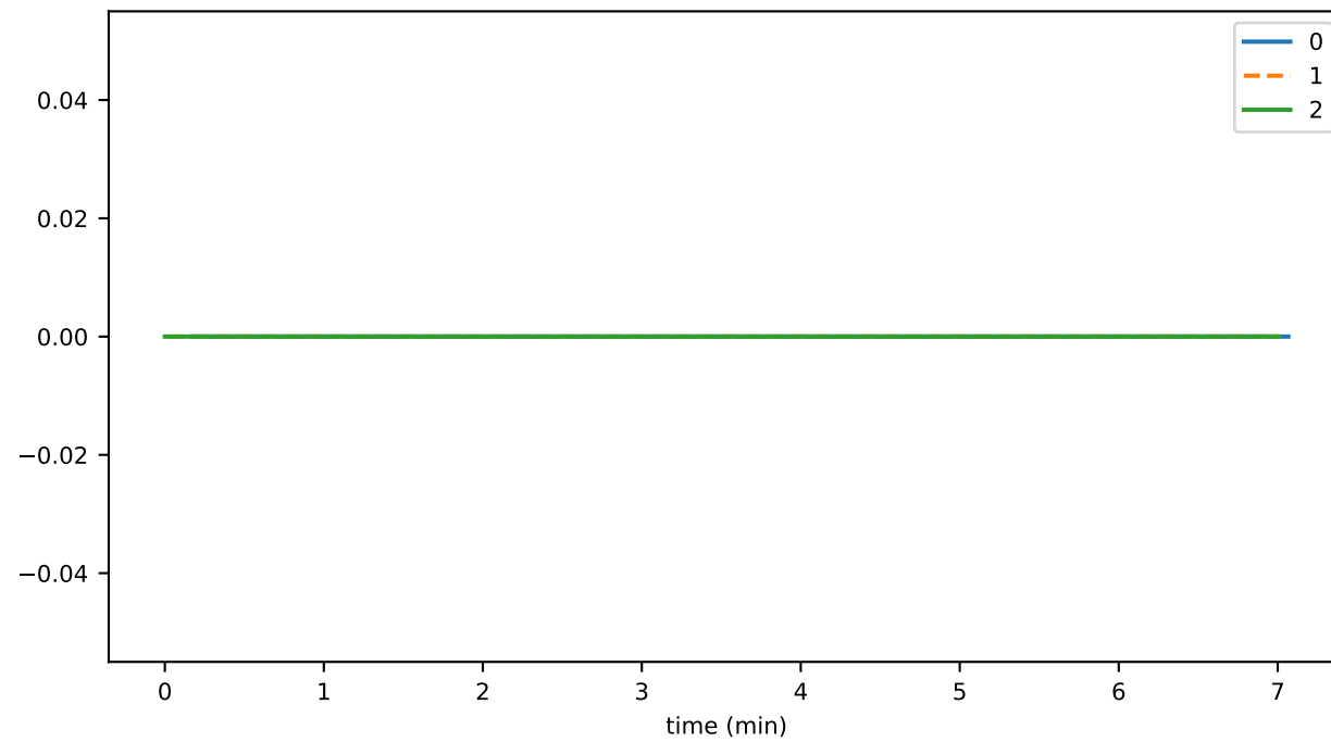
hasFallenBehind
