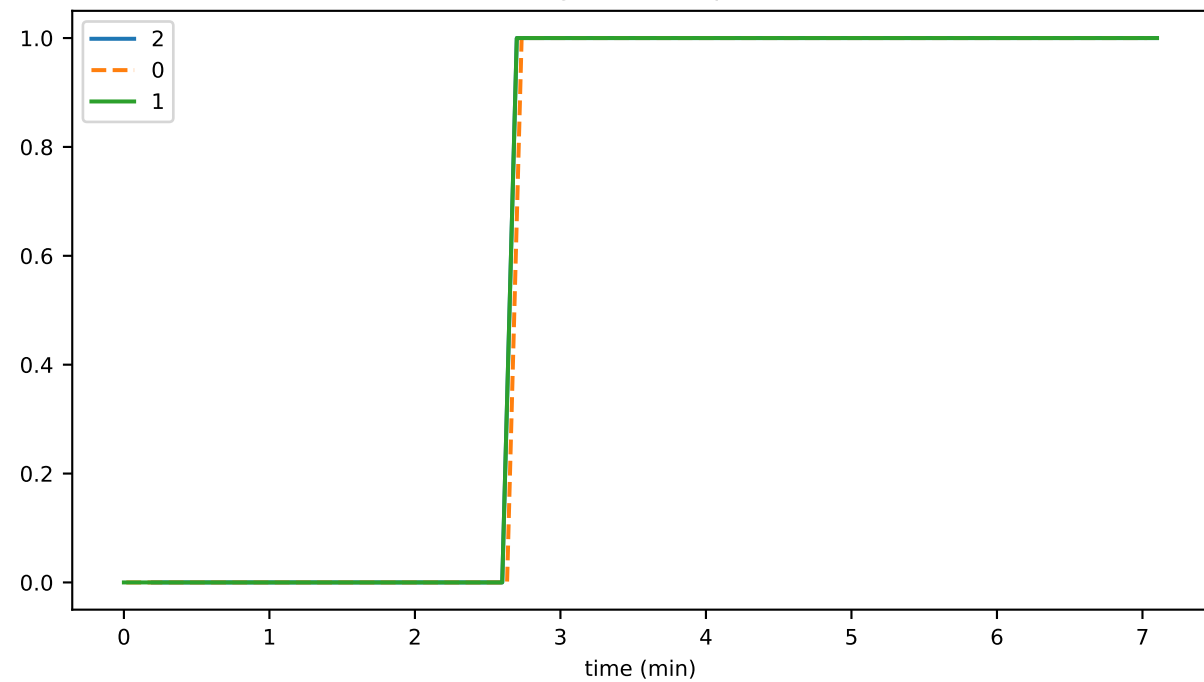
conn_activeConnlp
