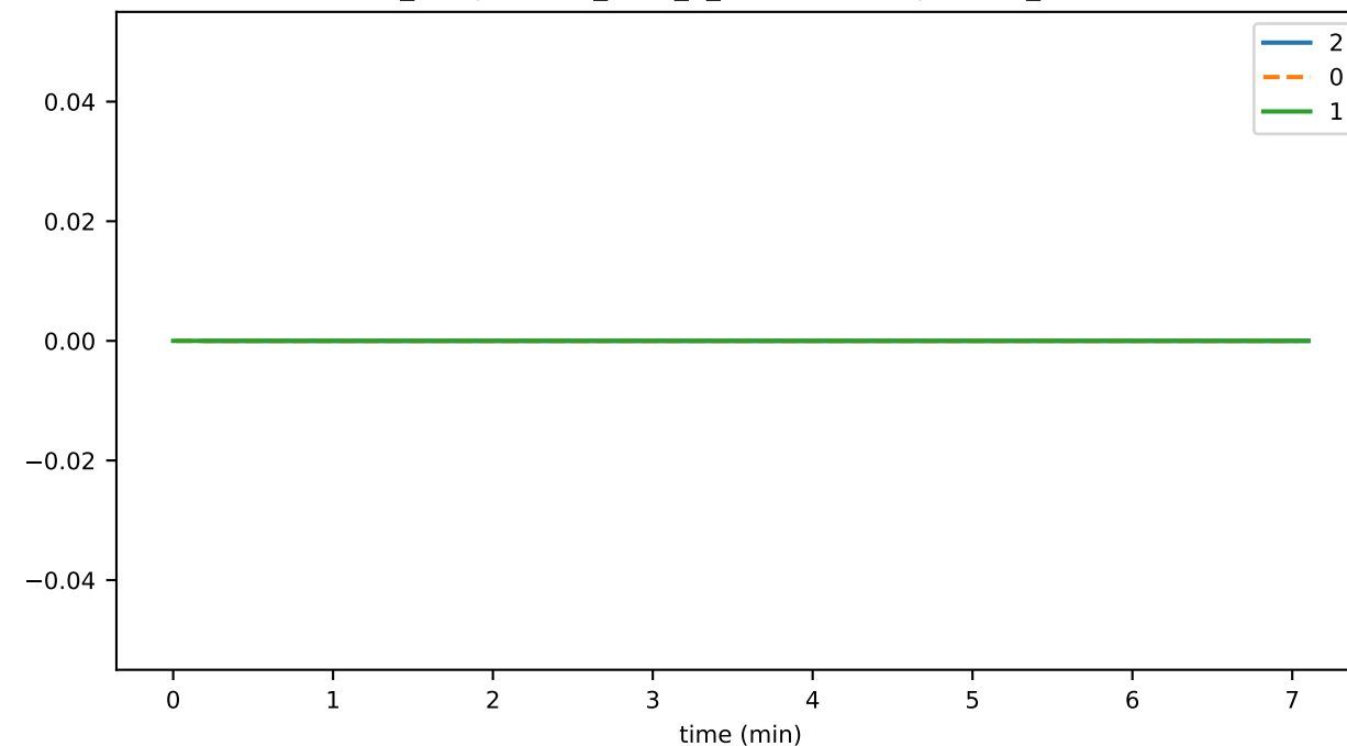
ds_compactions_level_3_hashesSavedSpaceMb_state
