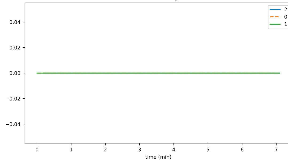
blockNodeRewardsEligibleCount
