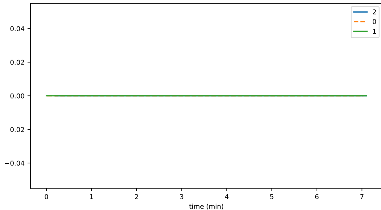
cryptoGetLiveHashDurationMax
