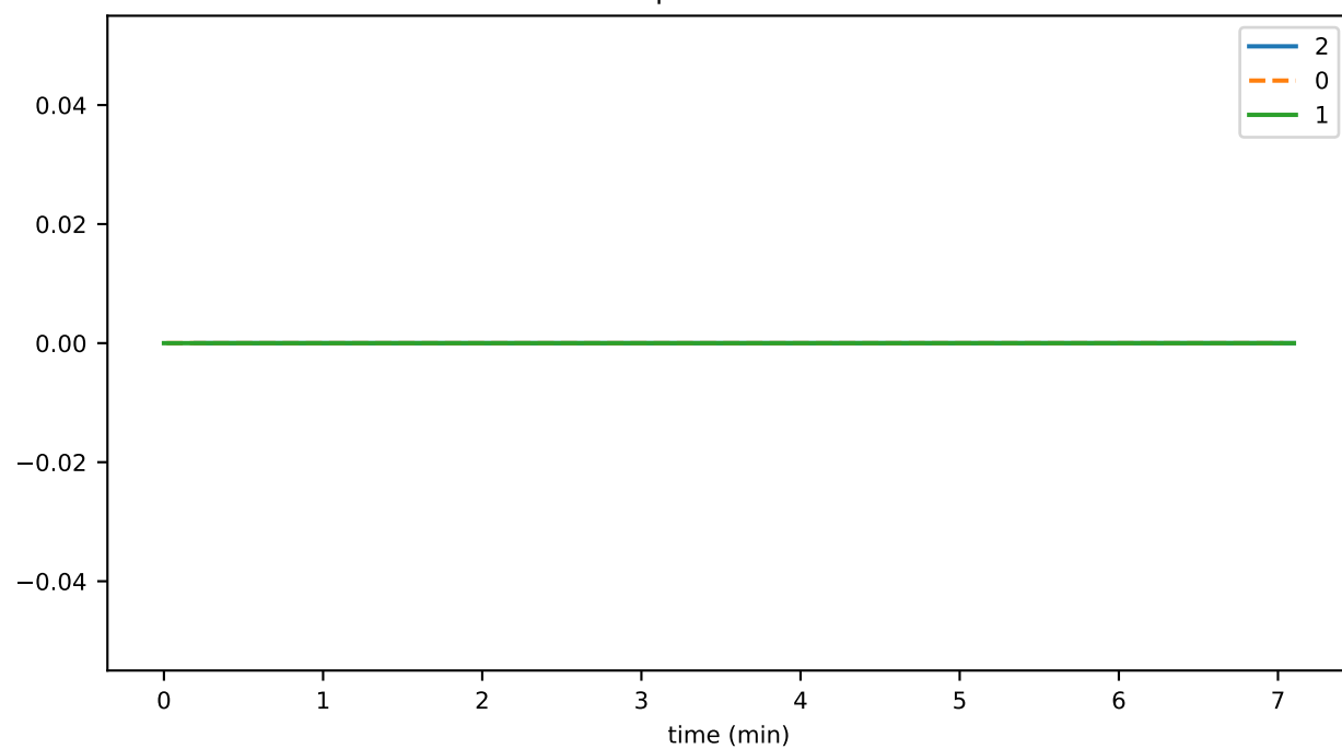
hookDispatchDurationMax
