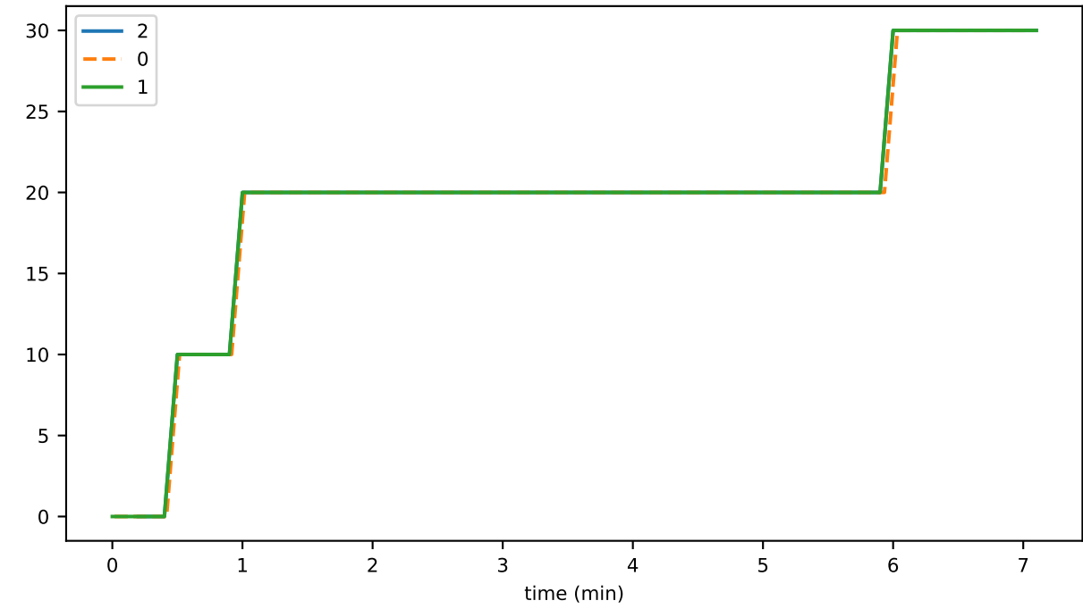
disconnects_per_sec_00
