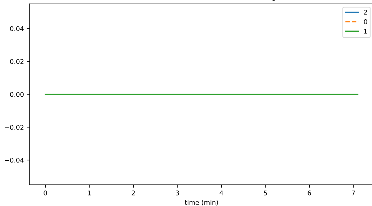
networkGetExecutionTimeThrottledTxns
