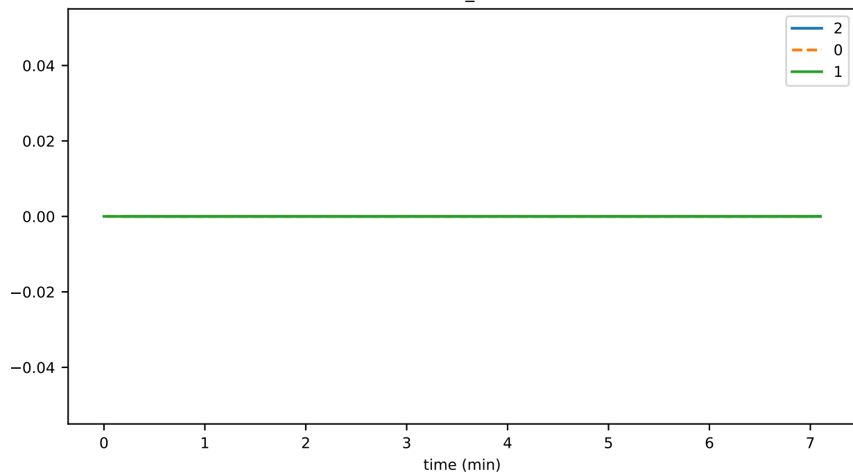
registeredNodeCreateDurationAvg
