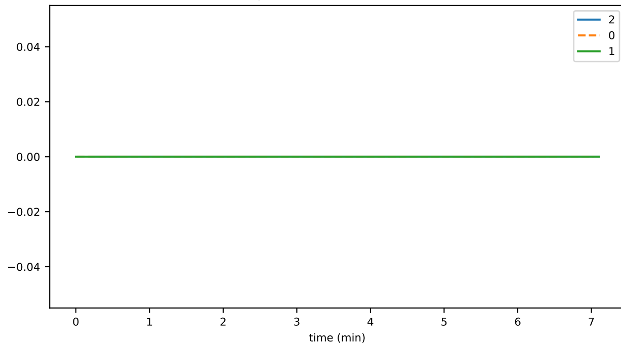
StateSigner_unhandled_task_count
