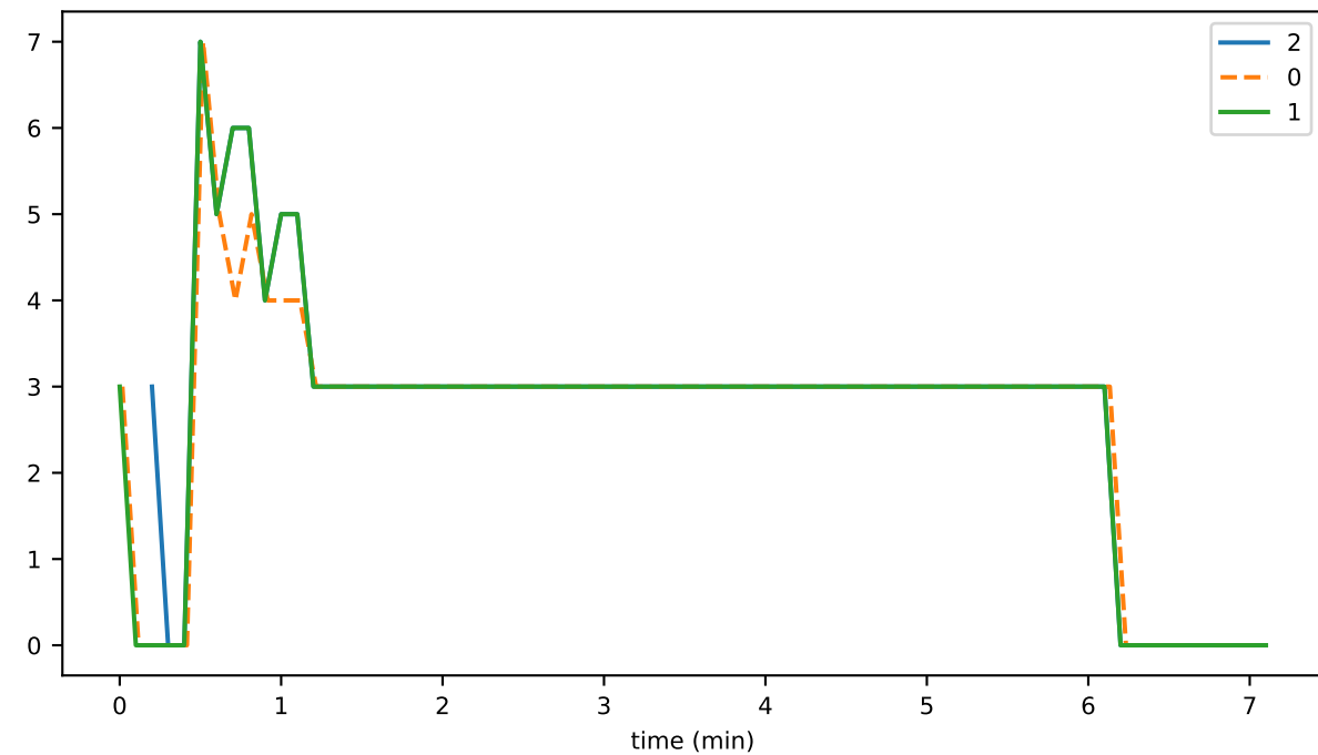
graphDepthUntilConsensusMAX
