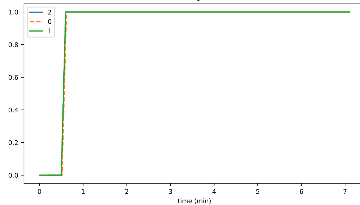
trans_per_event
