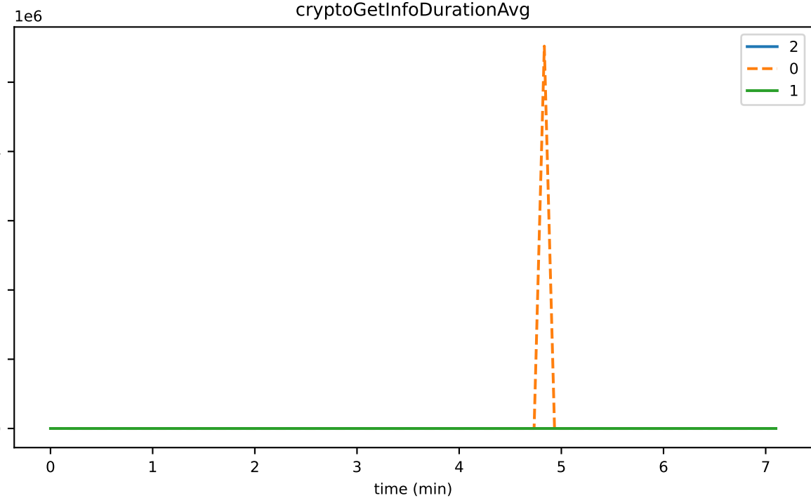
cryptoGetInfoDurationAvg
