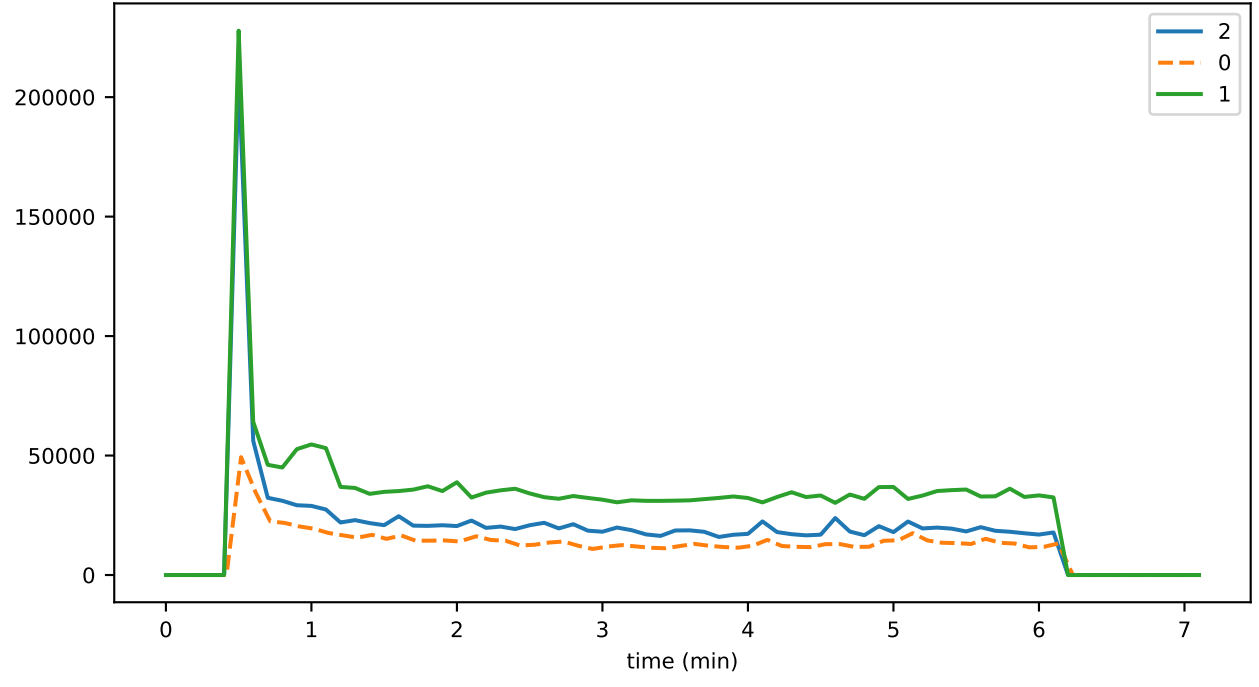
pcesAvgTotalWriteDuration
