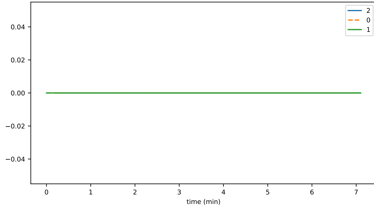
ds_offheap_hashesListMb_state
