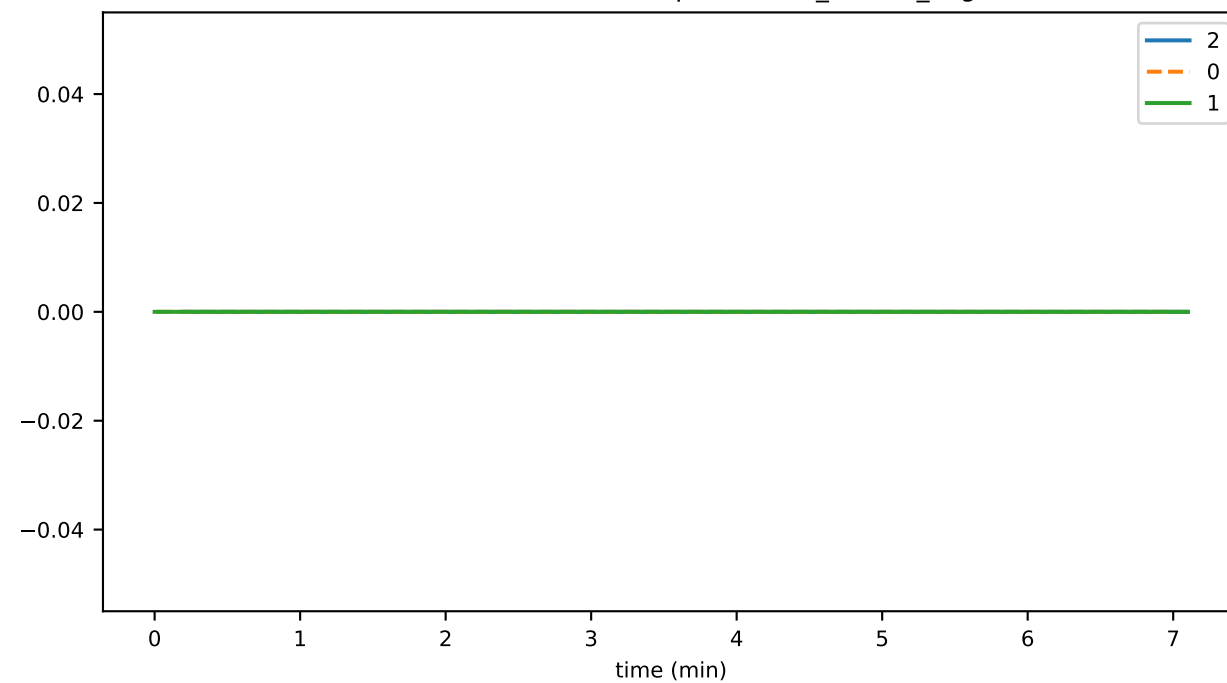
SmartContractService:OpsDuration_PerTxn_avg
