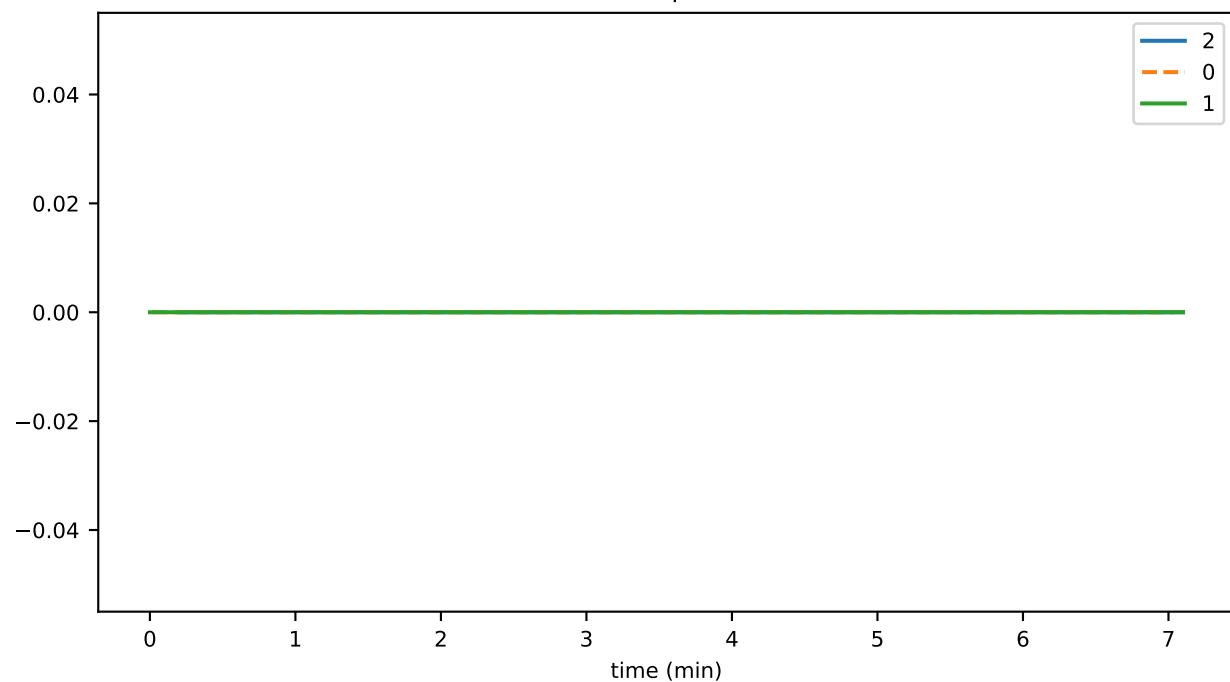
tokenAirdropDurationAvg
