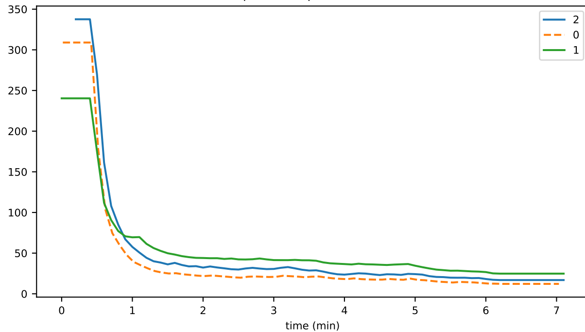
uptimeComputationTime
