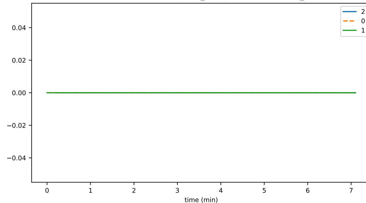
SmartContractService:SuccessfulTransactionDuration_count
