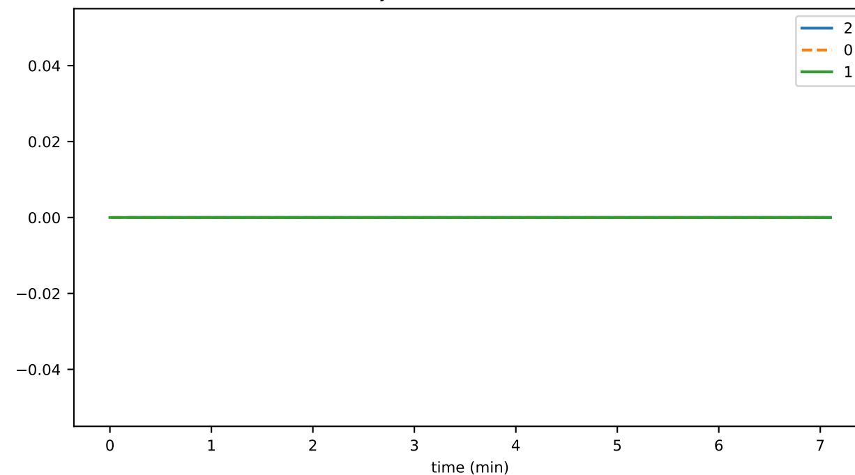
historyProofTransWAsmToR1Cnt
