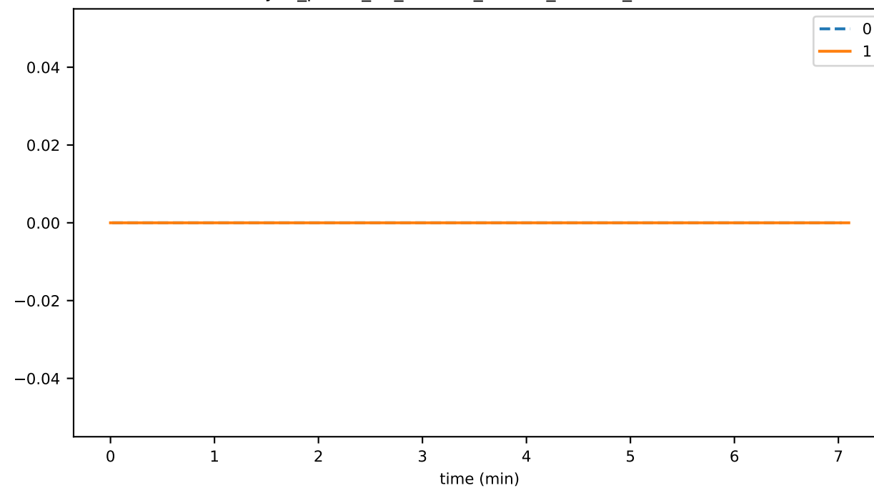
sync_phase_02_fraction_OTHER_FALLEN_BEHIND
