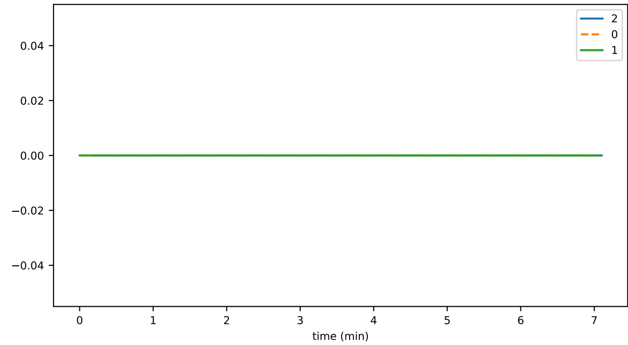
contractDeleteThrottledTxns
