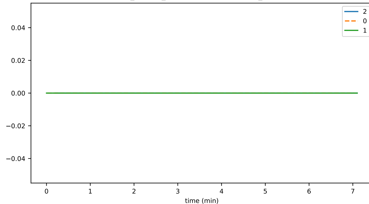
ds_flushes_leafKeysStoreFileSizeMb_state
