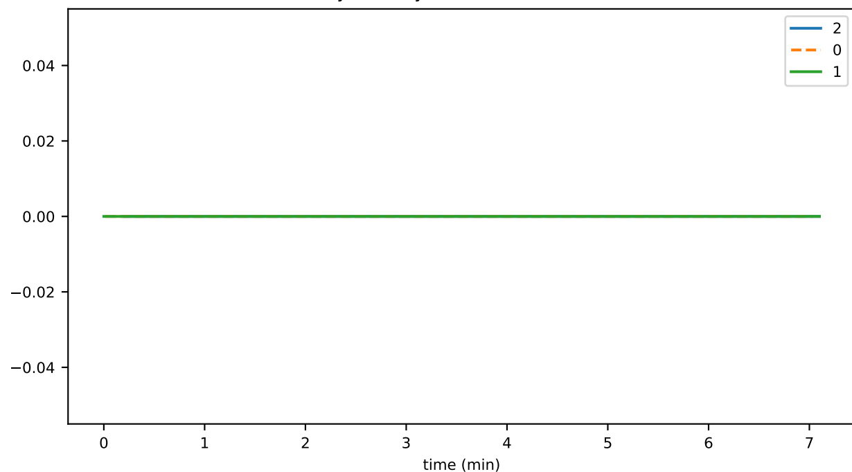
historyProofRetriesAvg
