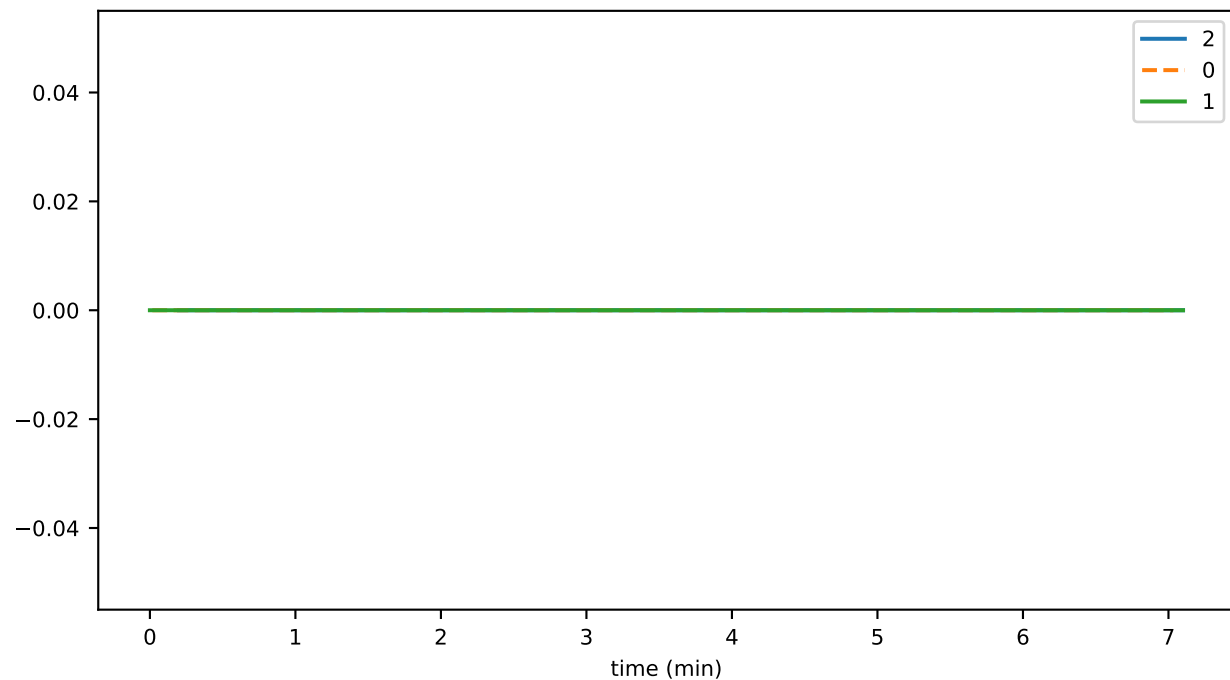
contractCreateDurationAvg
