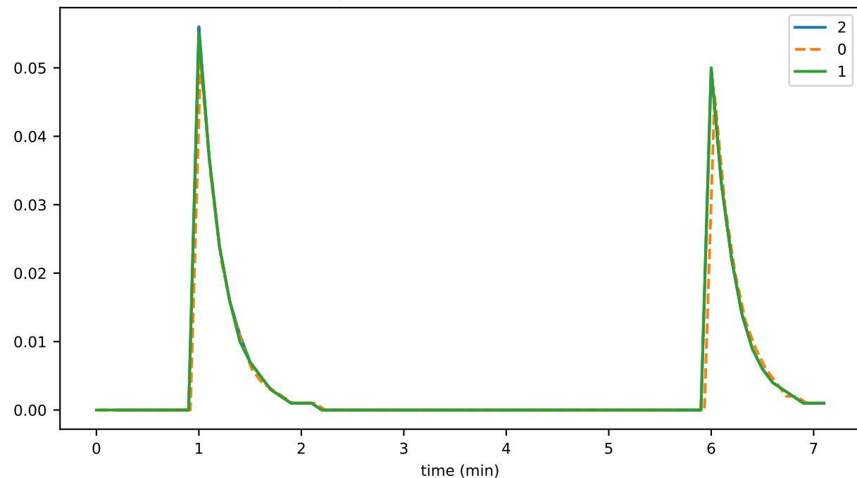
preconsensusEventFileYoungestIdentifier
