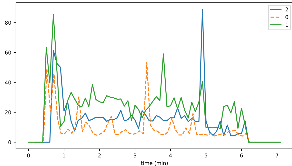
eventDelay_1_hashing_gossipMAX
