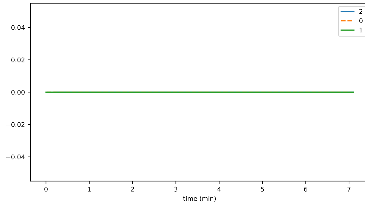
SmartContractService:SystemContractMethodCall_ERC20_failed
