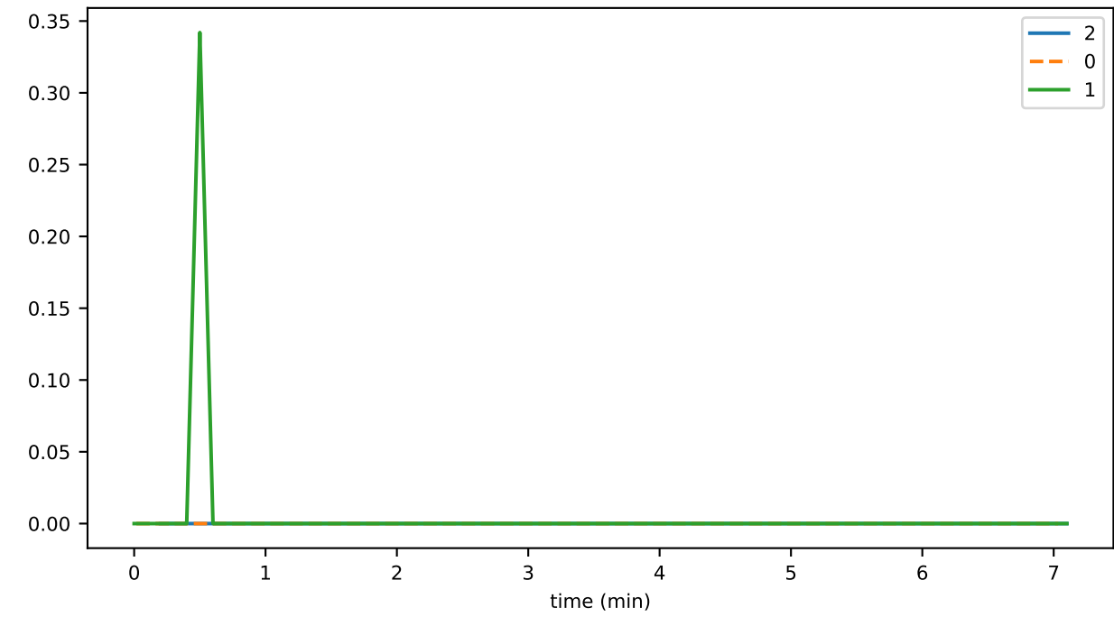
eventCreation_fraction_PIPELINE_INSERTION
