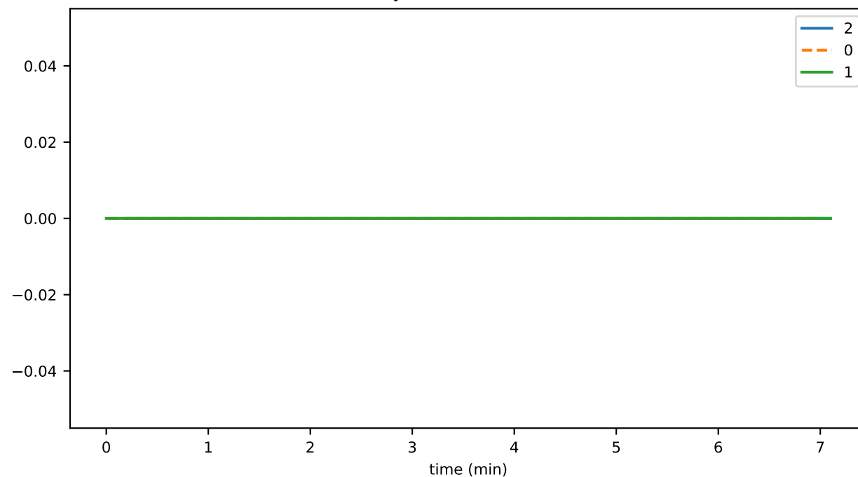
historyProofTransR1ToR2Cnt
