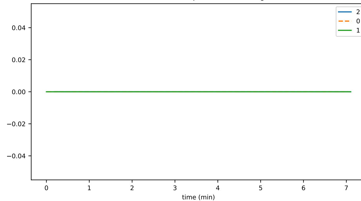
consensusGetTopicInfoDurationAvg
