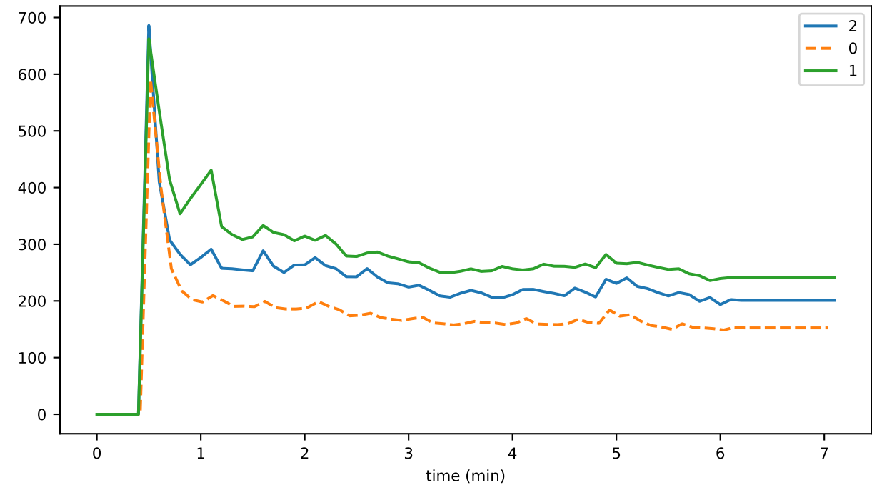
eventDelay_5_orphanBuffer_gossip
