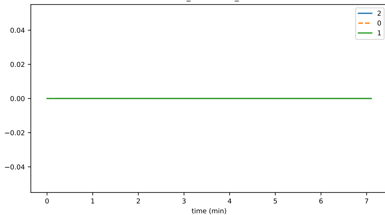
connRecv_endStream_success
