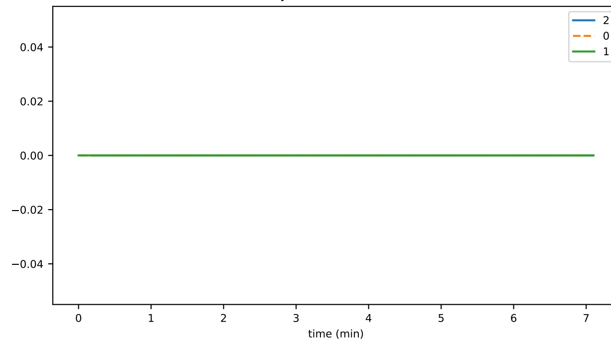
historyProofTransR2ToR3Cnt
