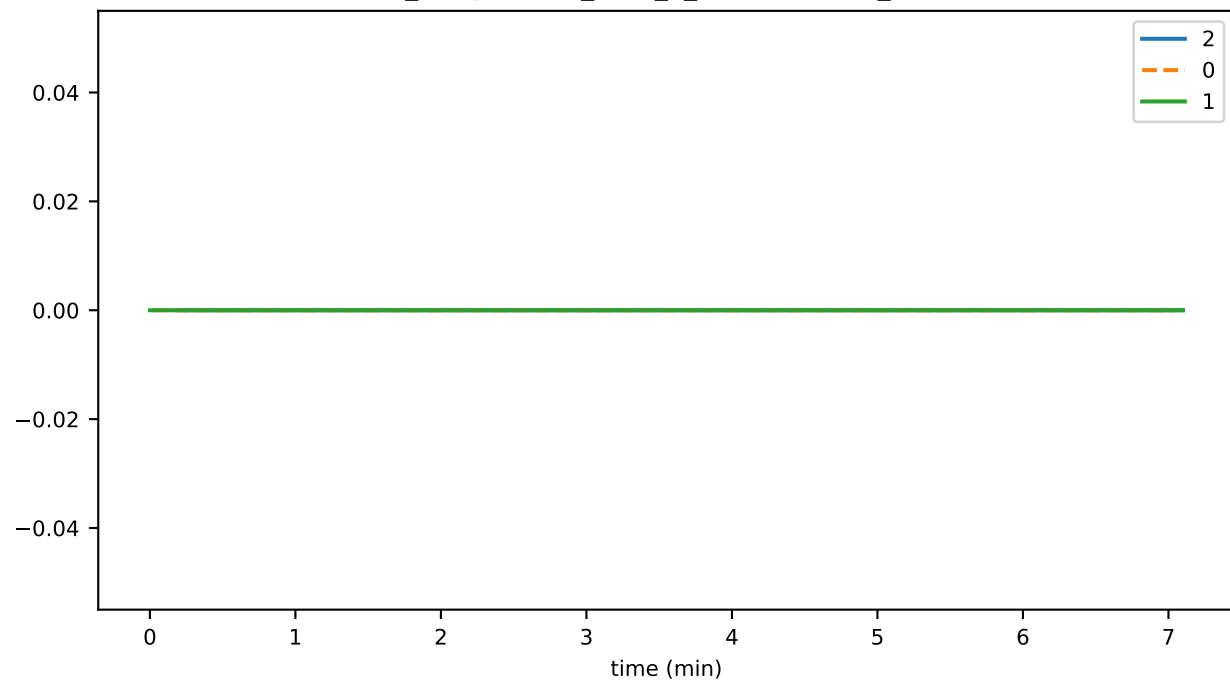
ds_files_hashesStoreFileSizeMb_state
