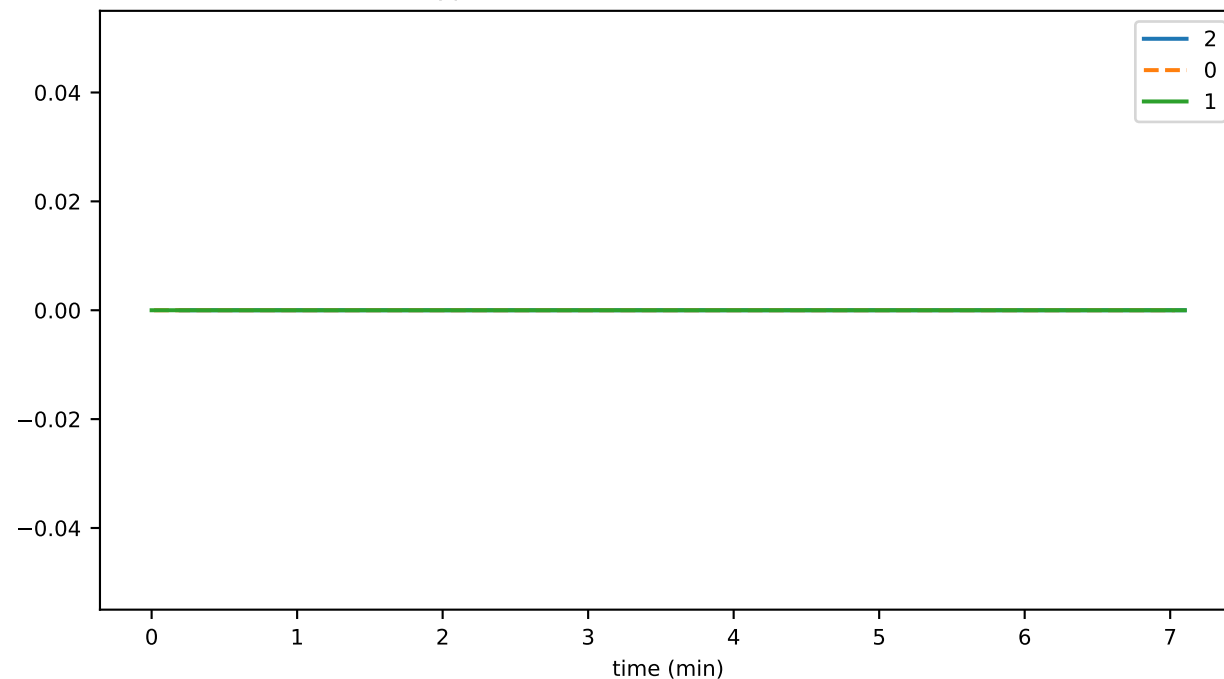
cryptoGetInfoDurationMax
