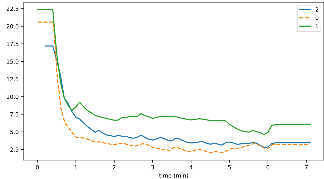
consensus_time_SETTING_EVENT_CONSENSUS_DATA
