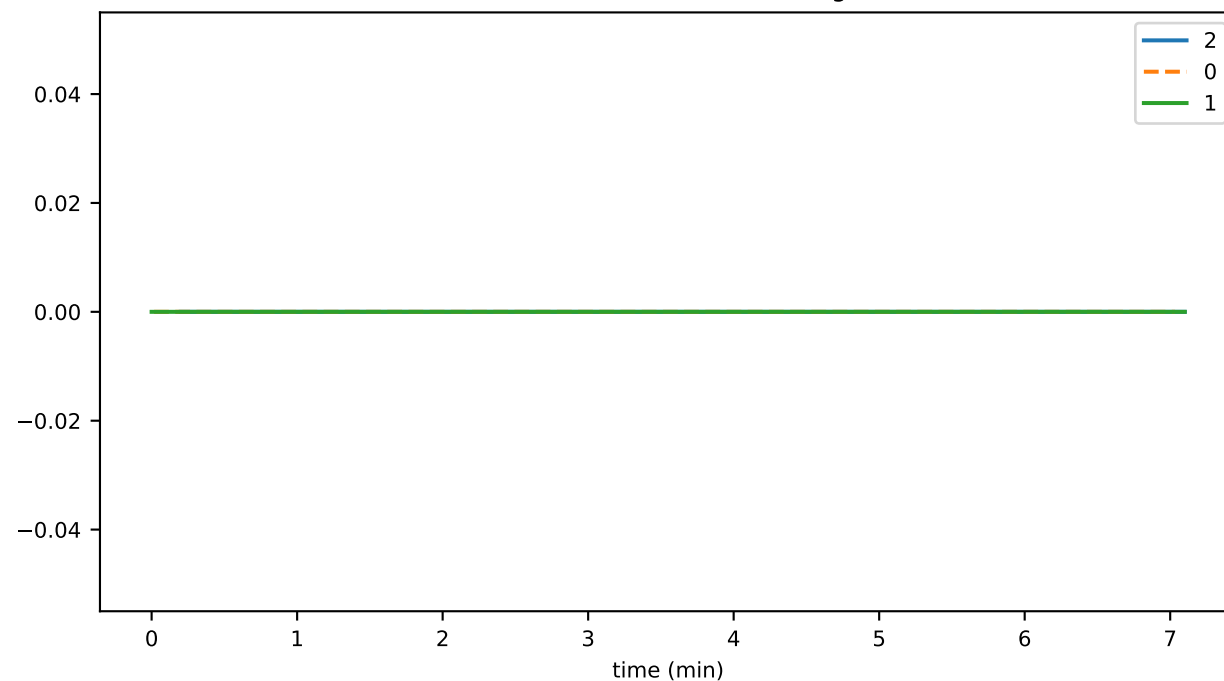
contractGetInfoDurationAvg
