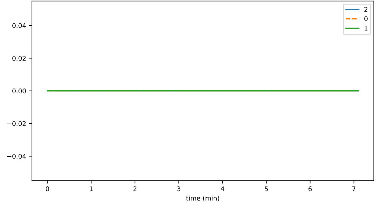
startsReconnectAsSender
