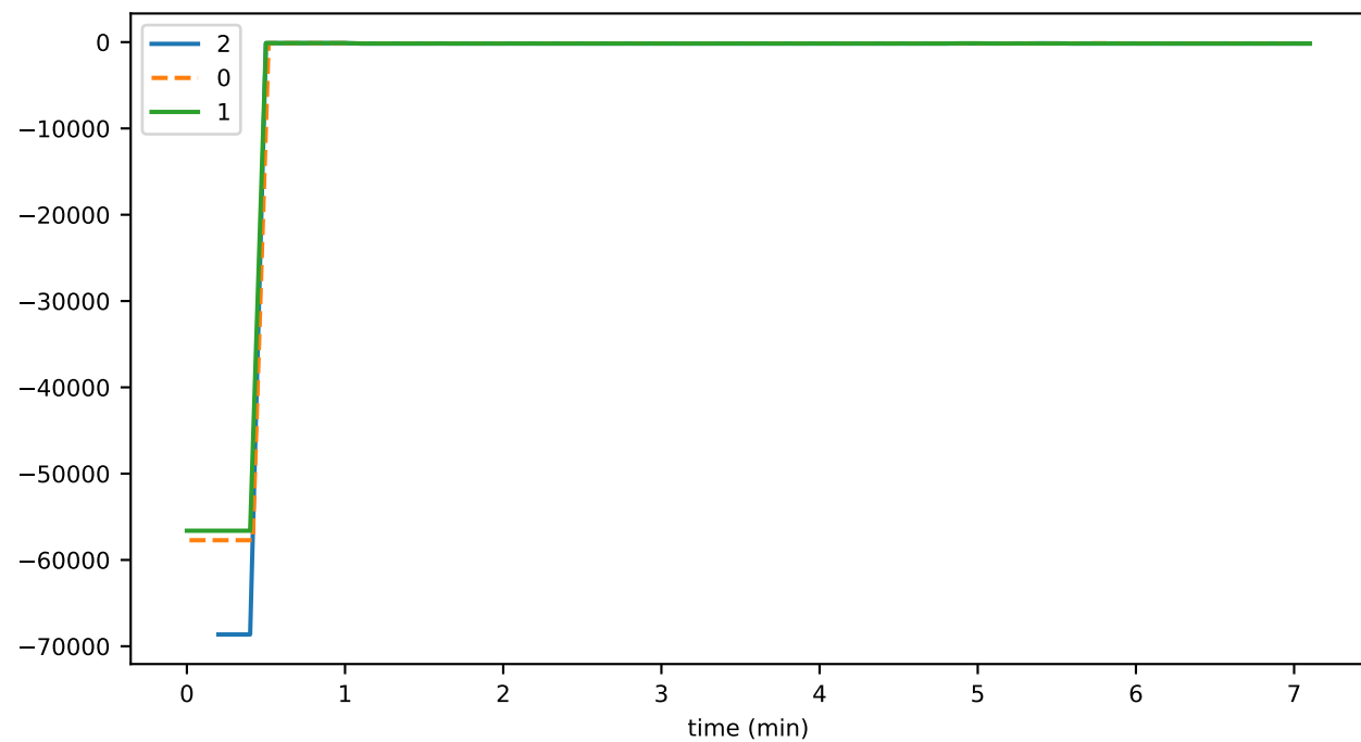
consensusTimeDeviation
