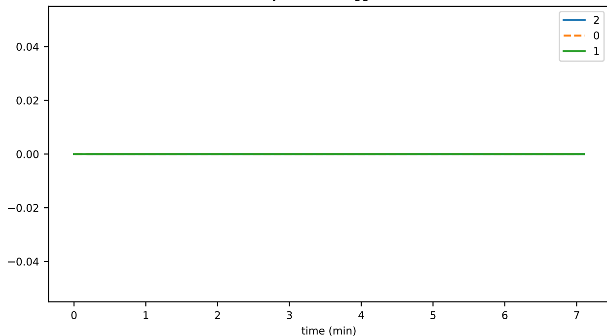
historyProofTransR1ToFailMs
