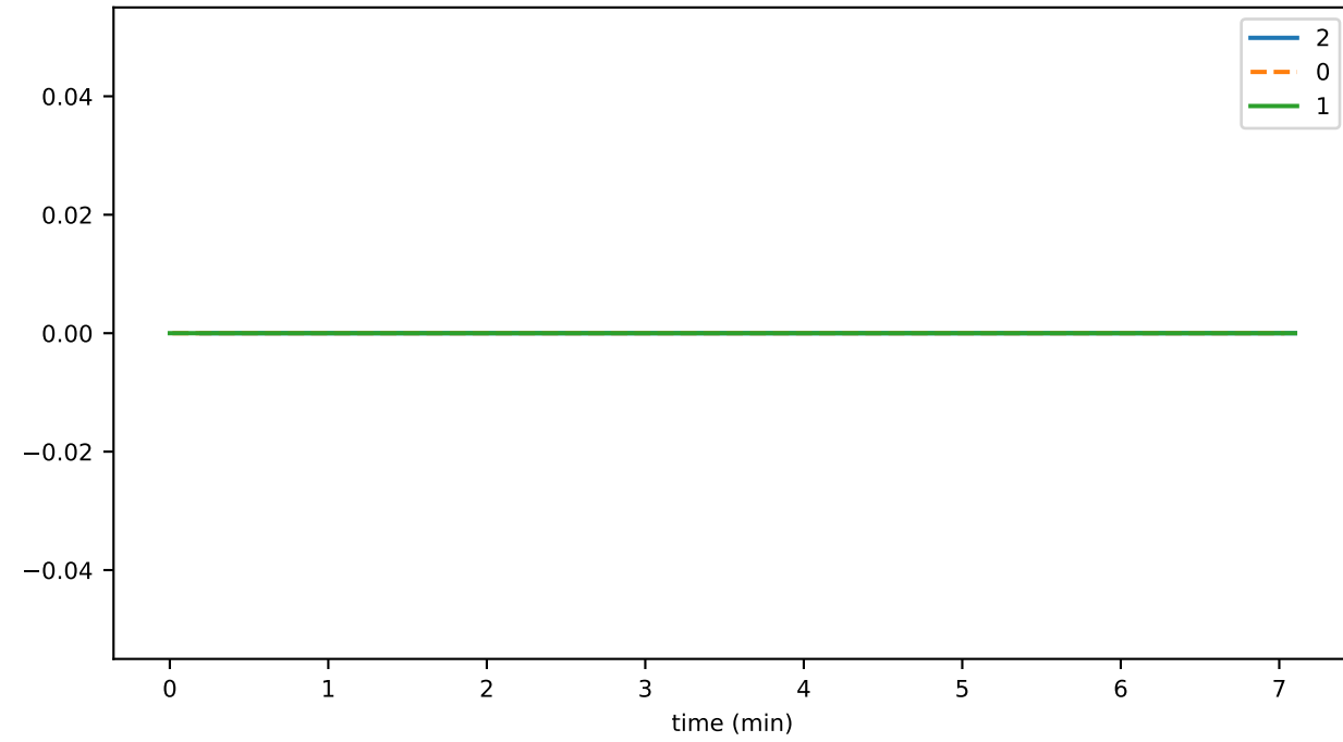
nodesUsed
