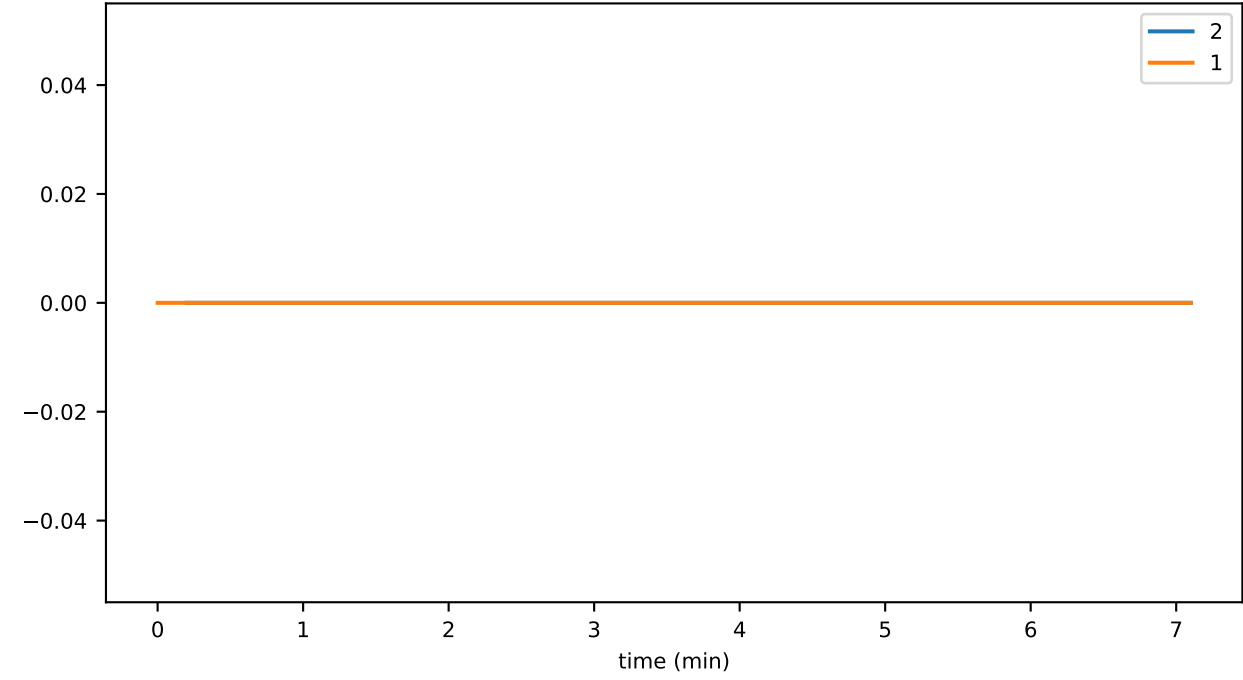
disconnects_per_sec_00
