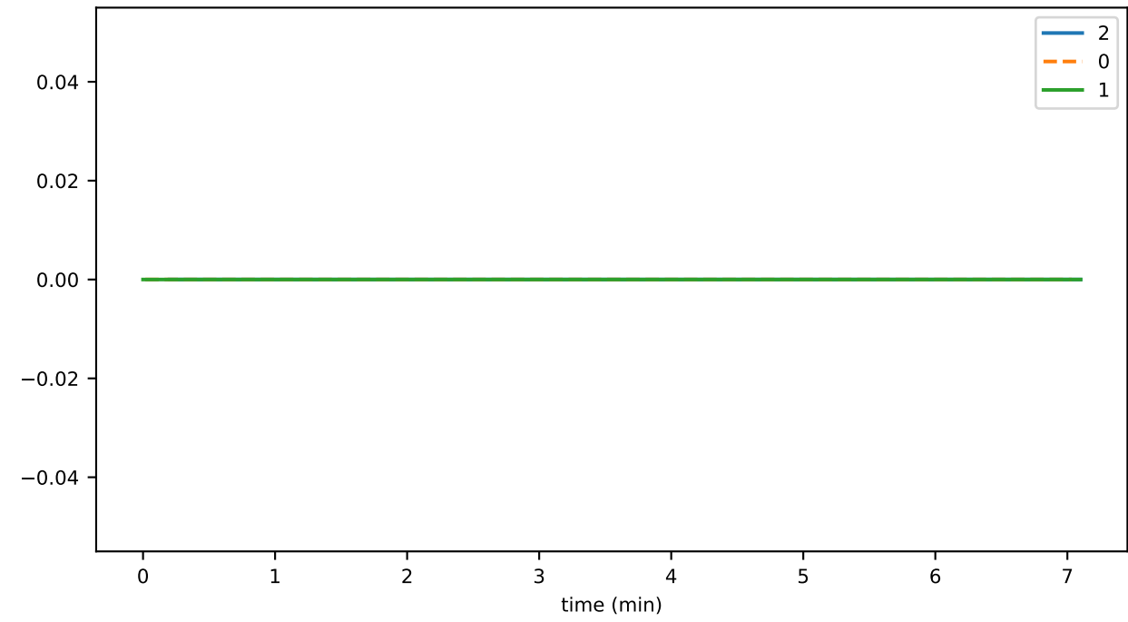
eventsWithInvalidFieldLength
