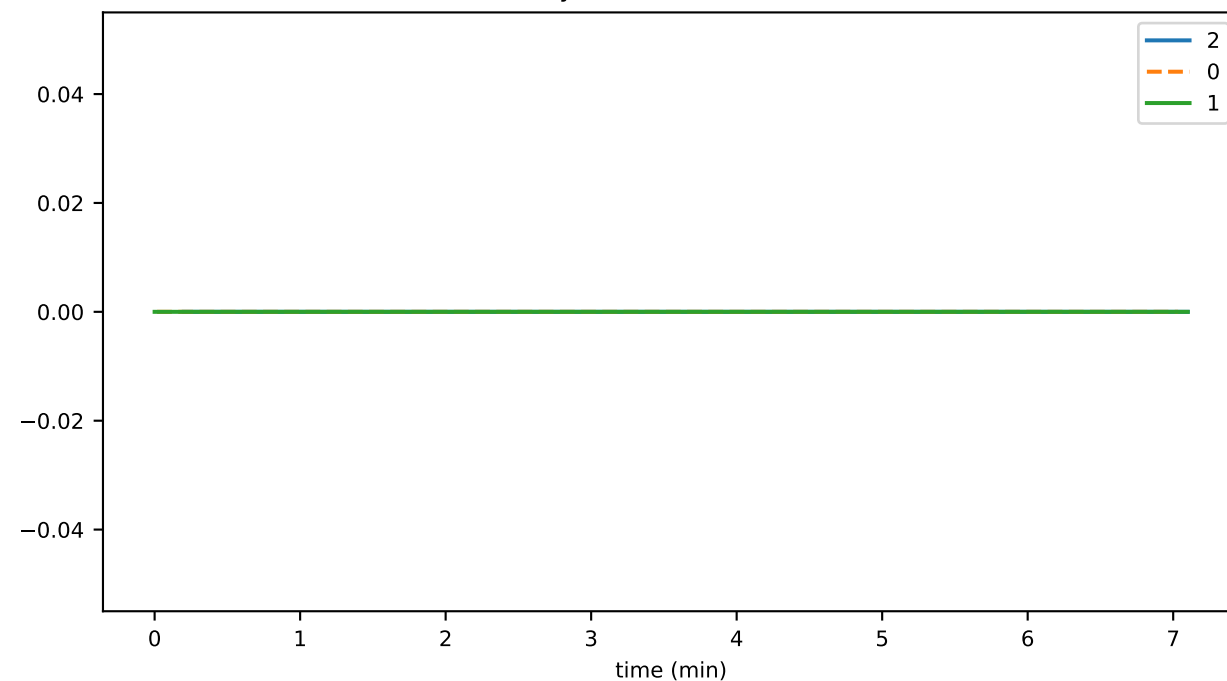
historyProofTransR3ToFailCnt
