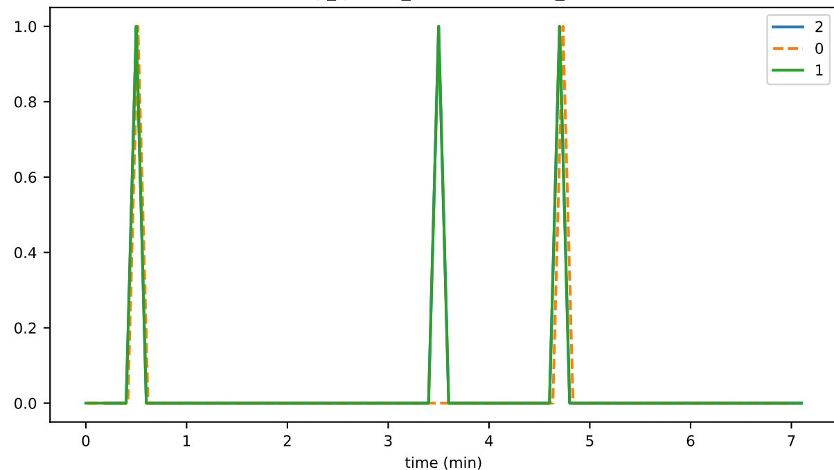
vmap_size_state
