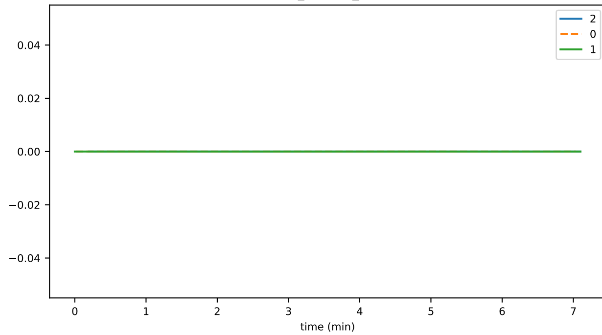
eventCreation_fraction_OVERLOADED
