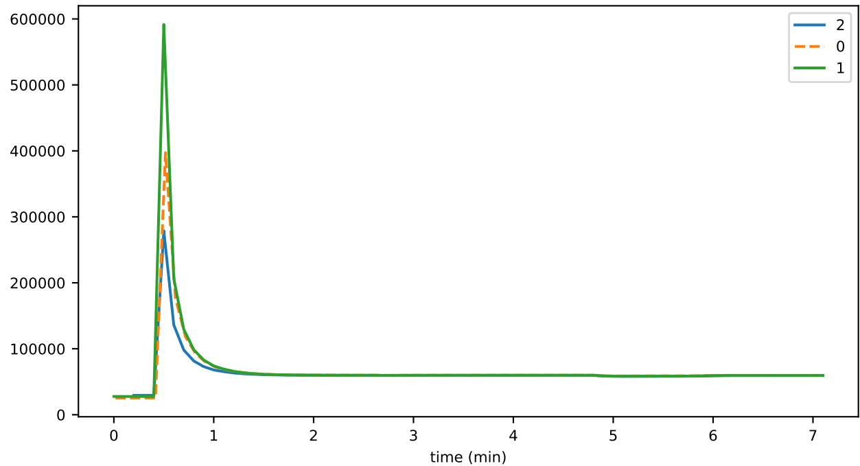
consensus_time_IDLE
