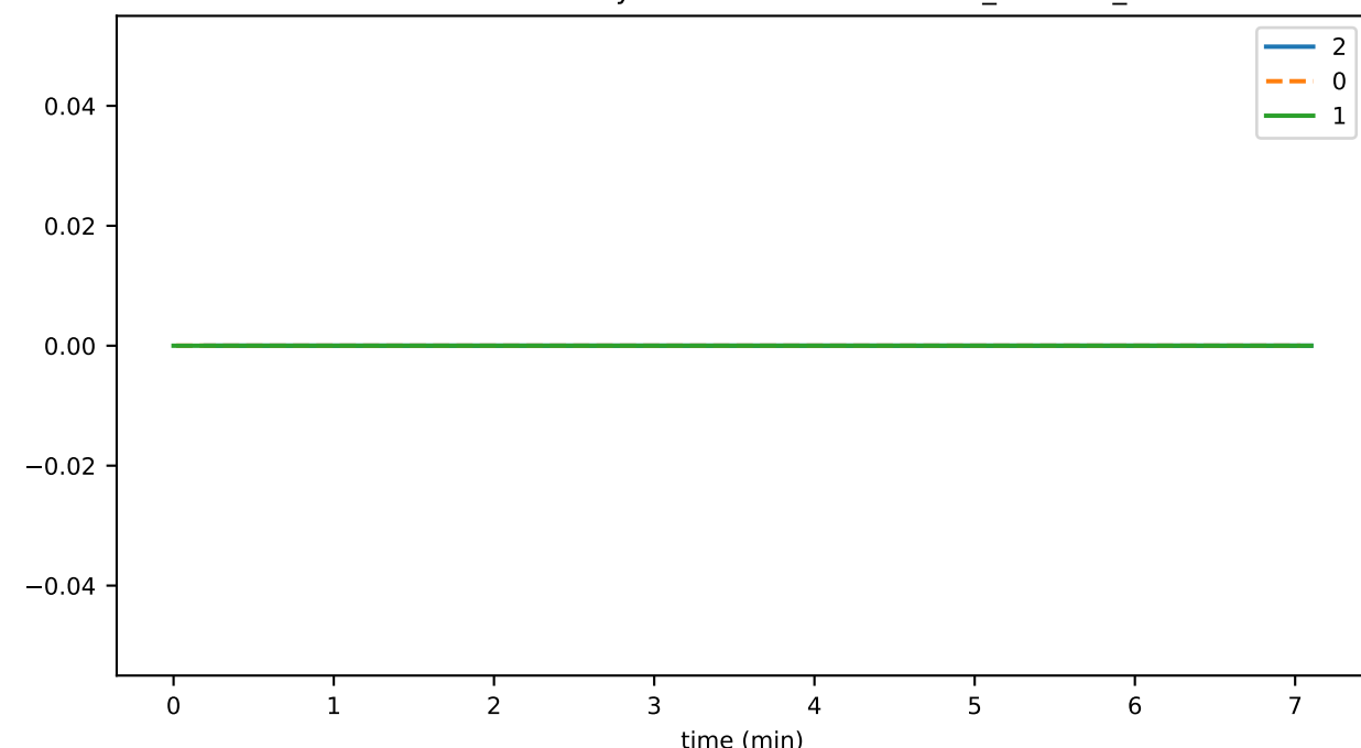
SmartContractService:SystemContractMethodCall_ALIASES_failed
