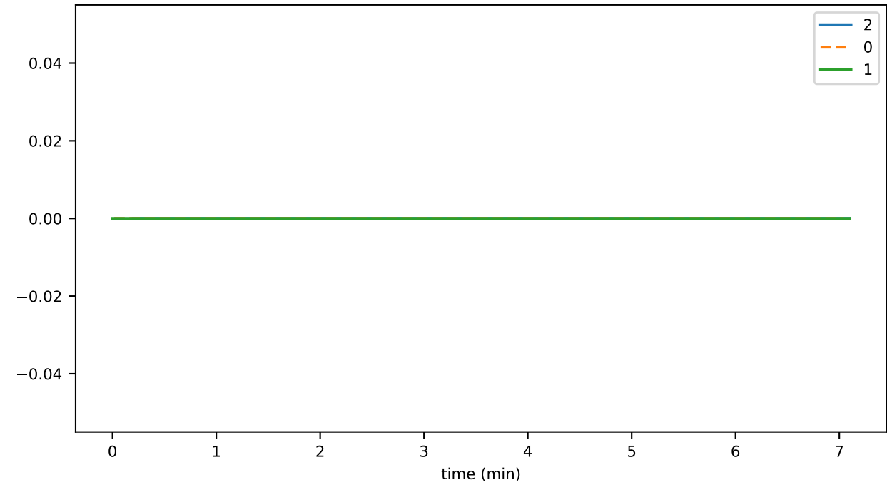
ds_compactions_level_9_hashesSavedSpaceMb_state
