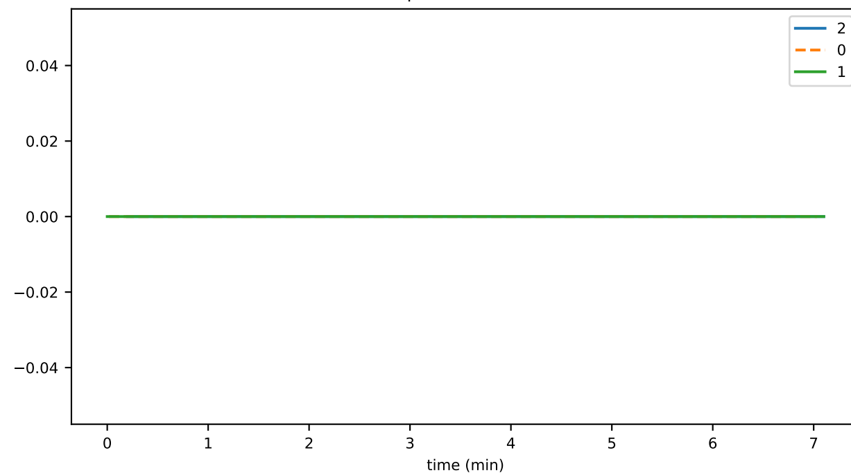
numEventsAddedUntilConsensus
