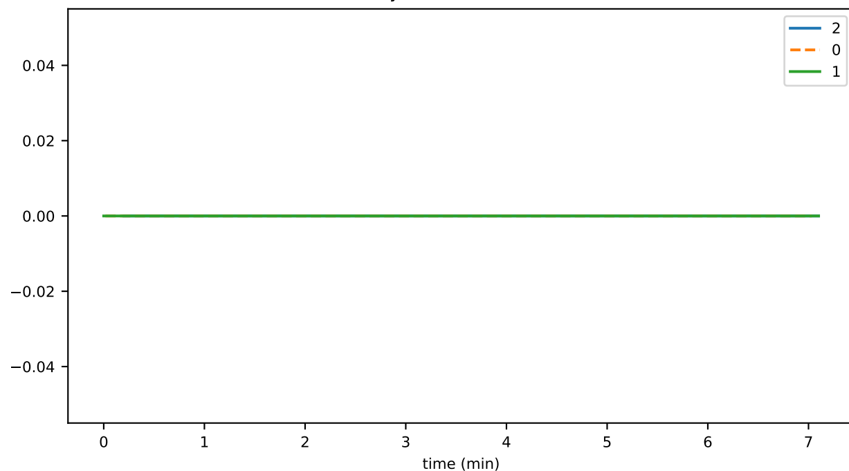
historyProofTransR2ToFailMs
