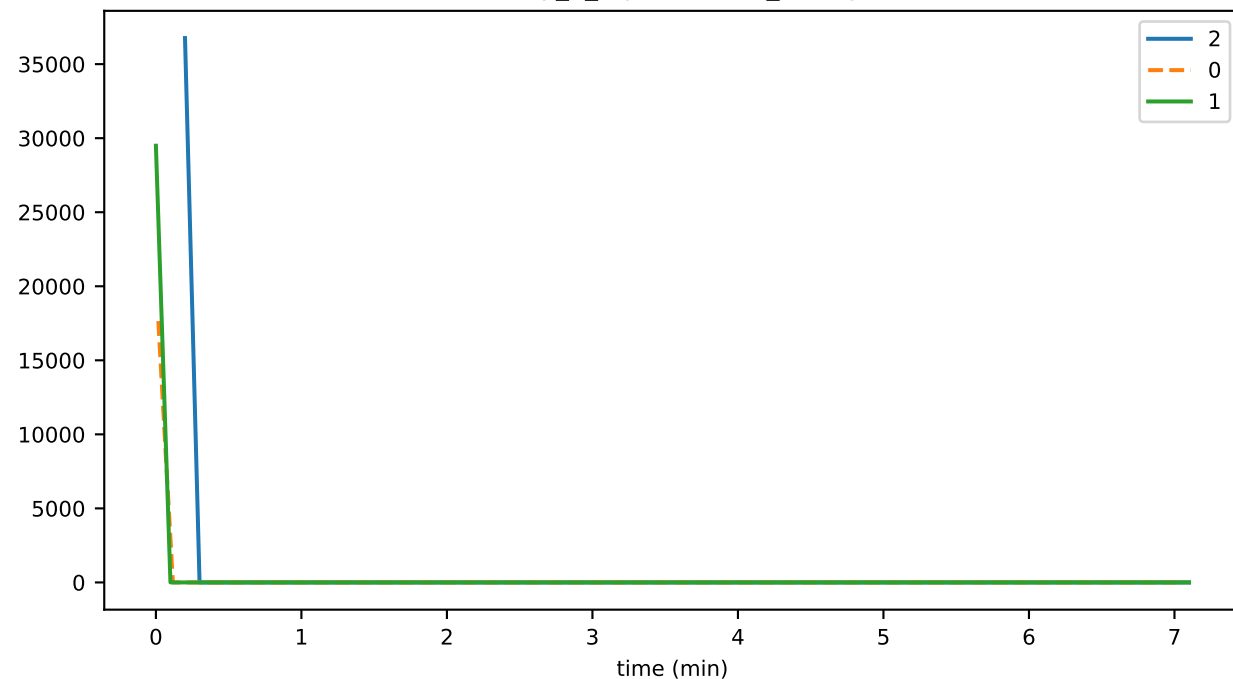
eventDelay_6_pces_gossipMAX
