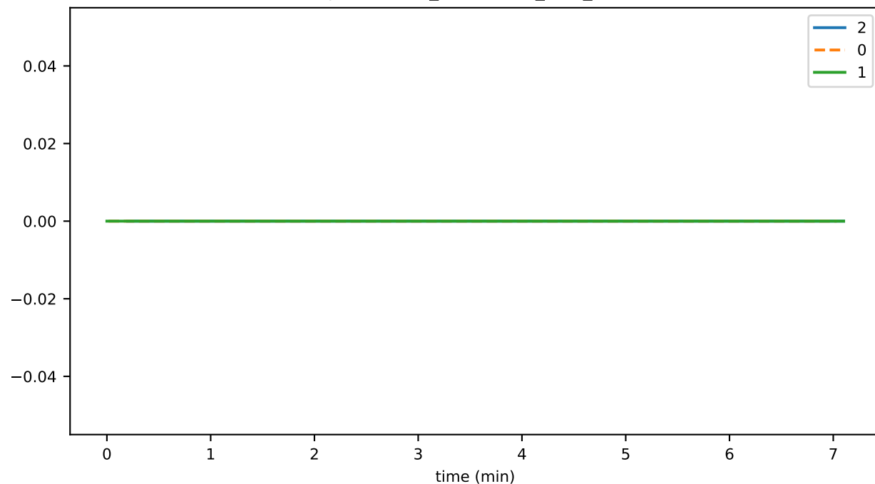
outgoingSyncRequests_per_sec
