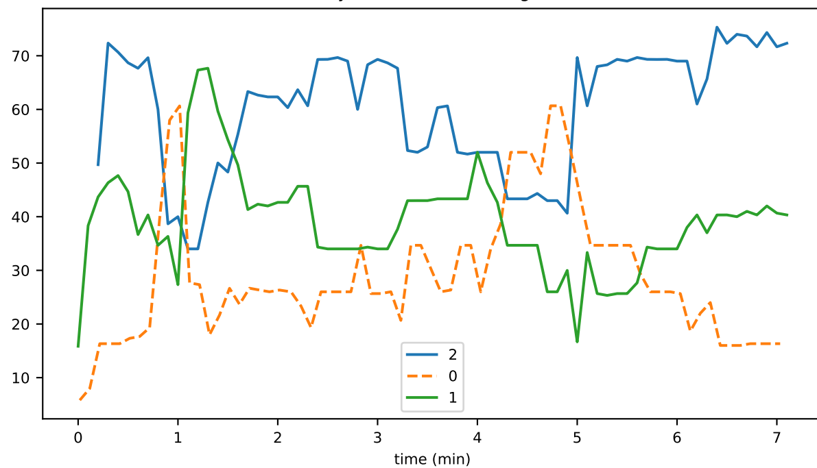
doNotSyncRemoteProcessingEvents
