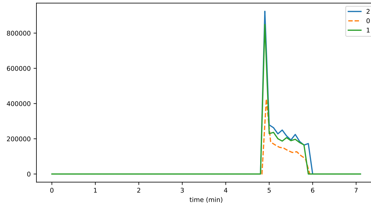
cryptoTransferDurationAvg
