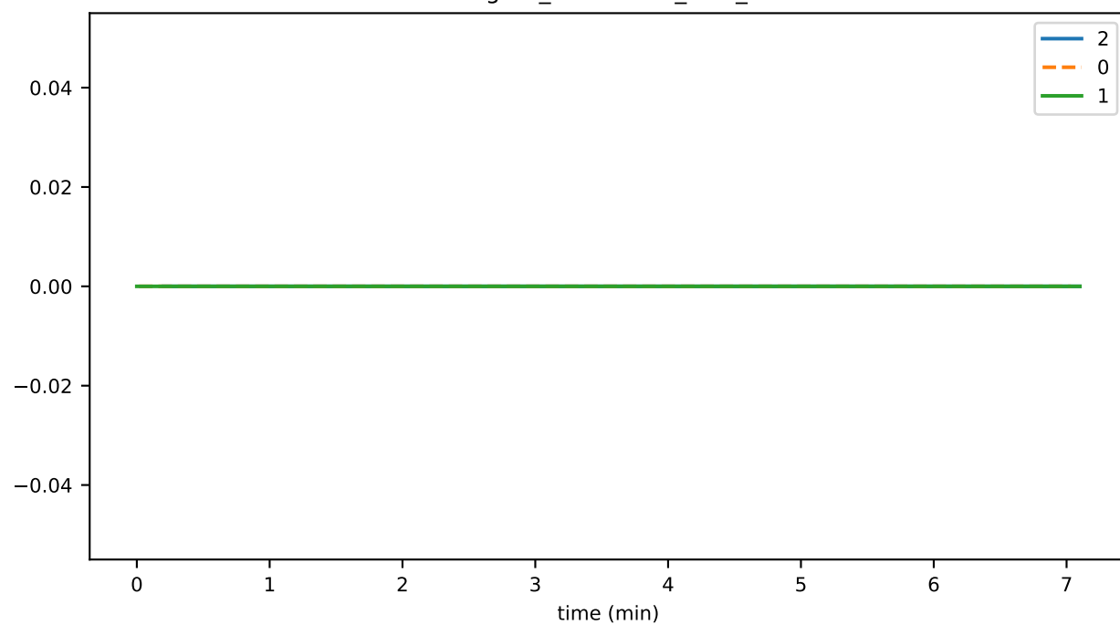
StateSigner_unhandled_task_count
