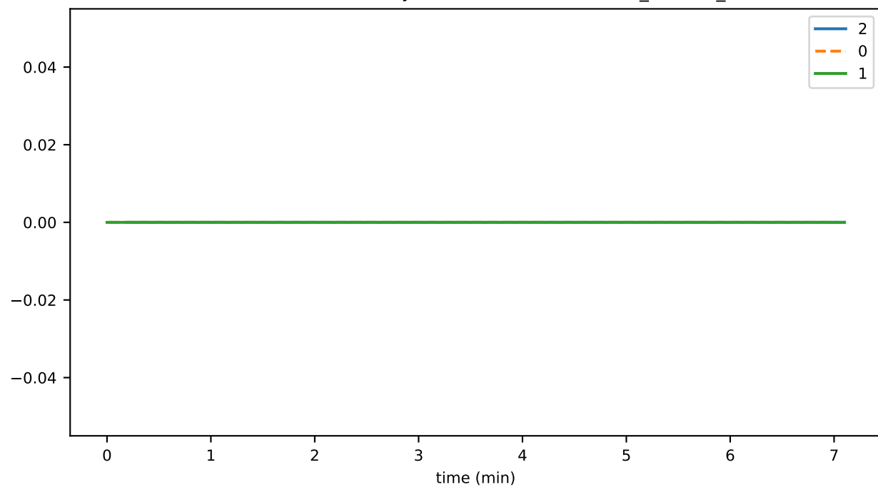
SmartContractService:SystemContractMethodCall_DIRECT_total
