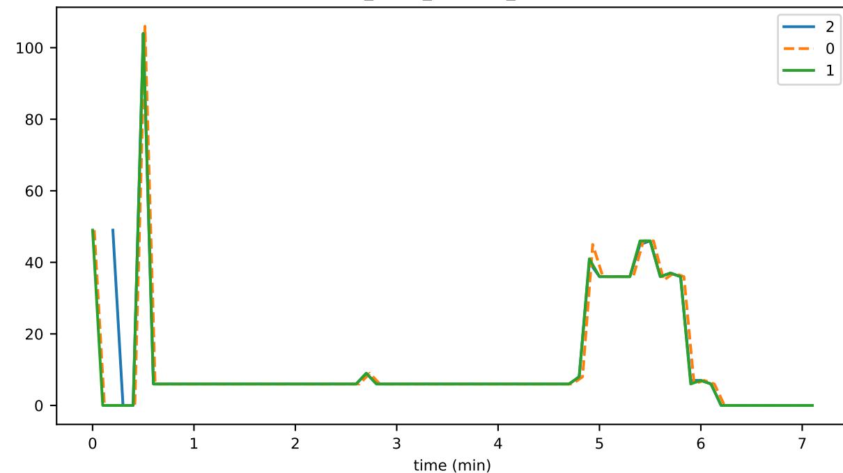
ds_reads_leafKeys_state
