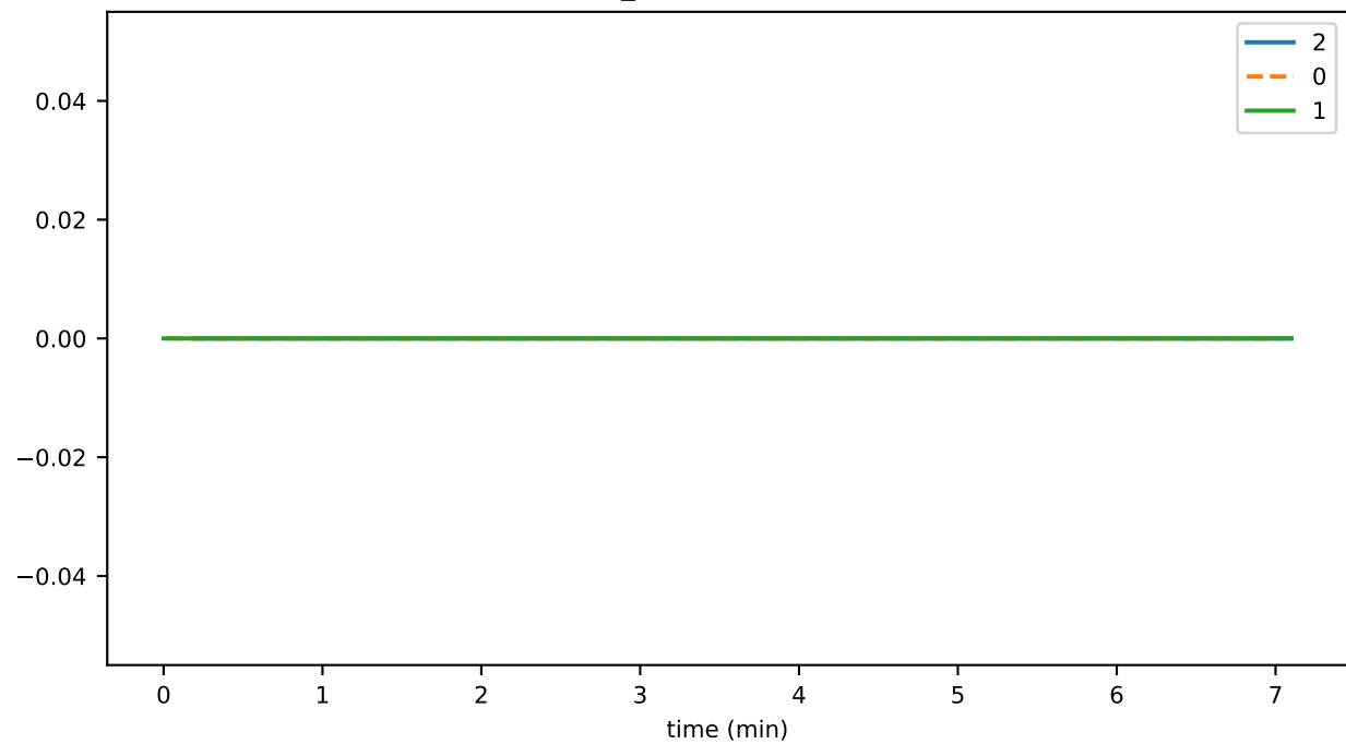
connRecv_nodeBehindPublisher
