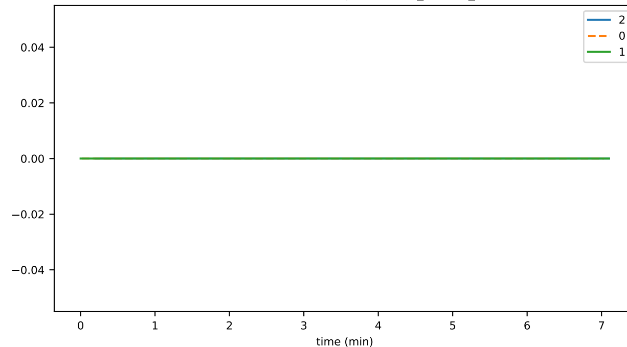
SmartContractService:Rejected_contractCallTx_total
