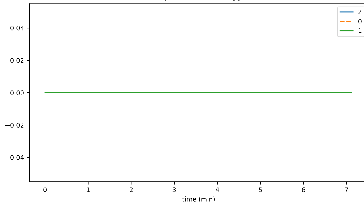
historyProofTransR3ToAggCnt
