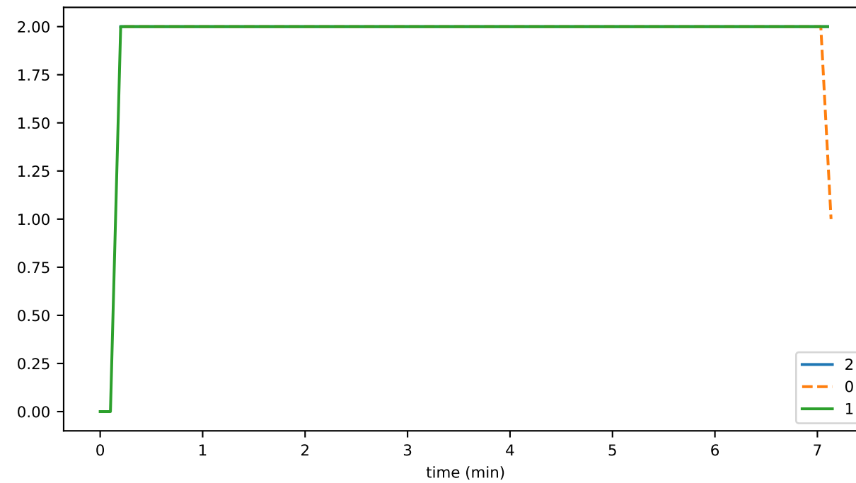
syncPermitsUtilized
