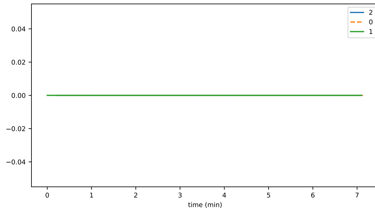
pcesAvgSyncDuration
