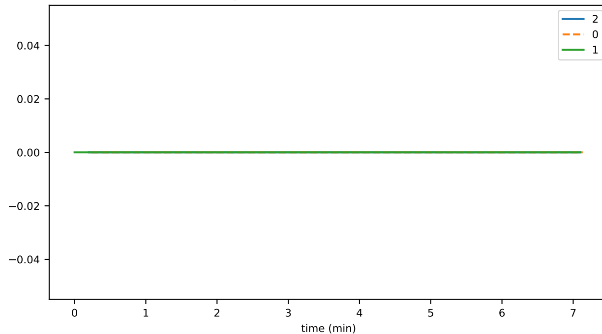
registeredNodeDeleteDurationAvg
