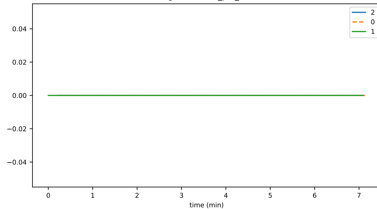
SigIntakePulse_per_sec
