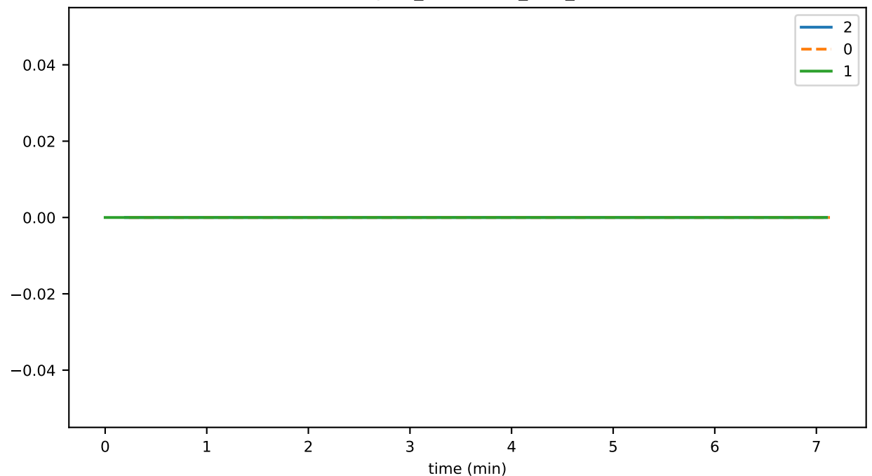
StateSnapshotManager_unhandled_task_count
