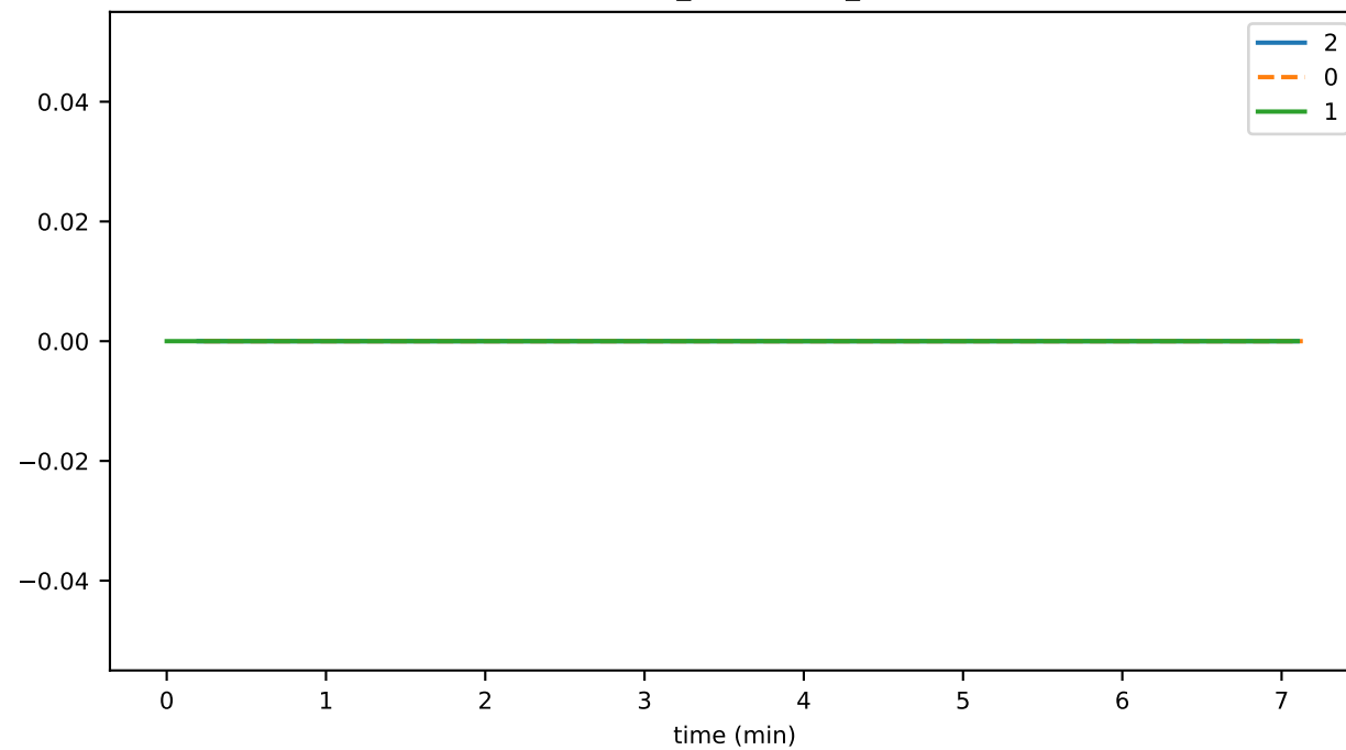
connRecv_endStream_persistenceFailed
