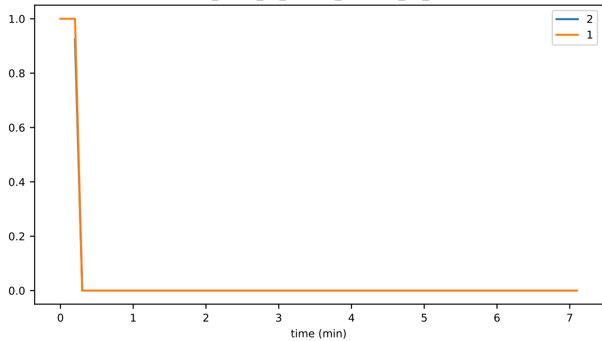
sync_phase_00_fraction_OUTSIDE_OF_RPC
