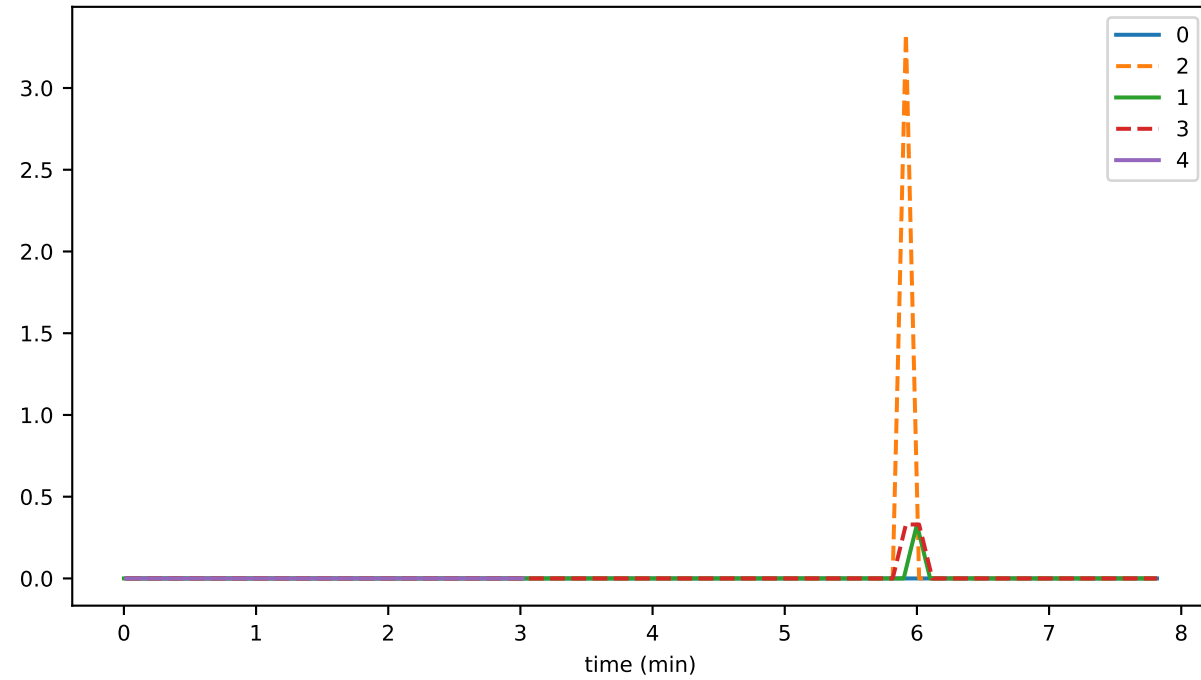
ds_compactions_level_0_hashesSavedSpaceMb_state
