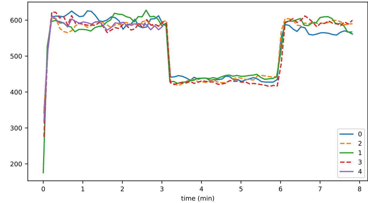
ds_compactions_level_0_hashesTimeMs_state
