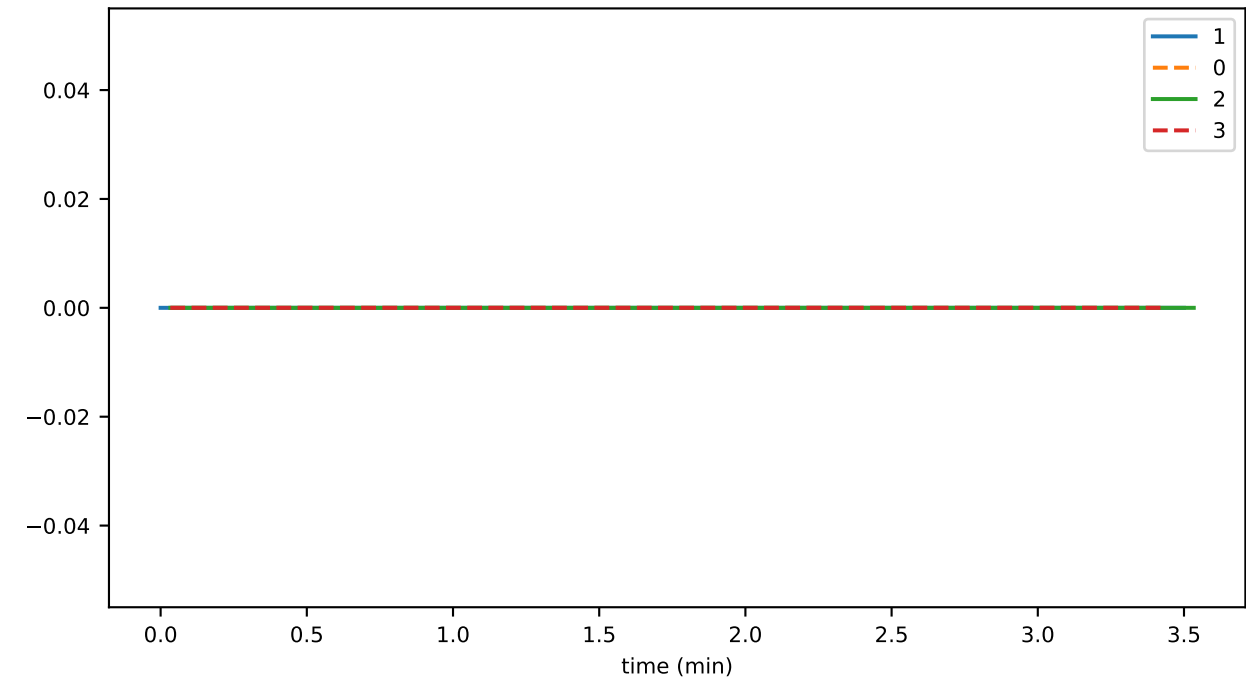
OrphanBuffer_unhandled_task_count
