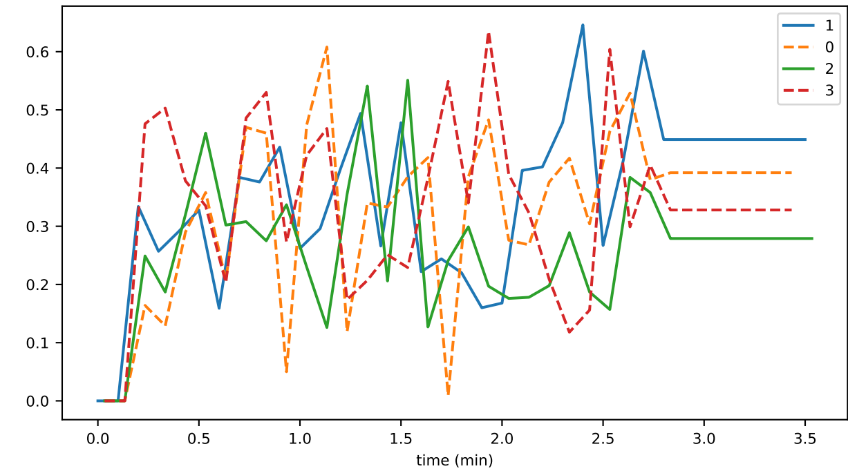
OrphanBuffer_unhandled_task_count
