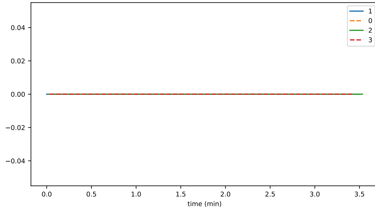
opportunitiesToInitiateSync_per_sec
