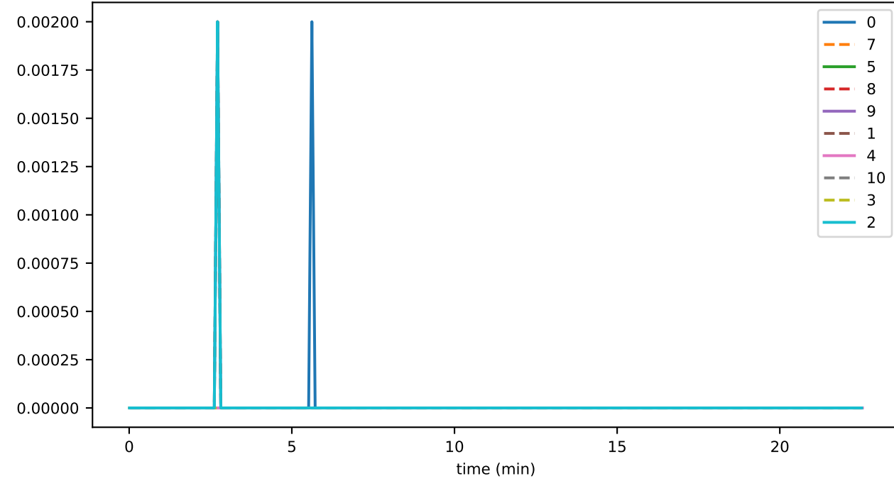
sync_phase_06_fraction_SELF_FALLEN_BEHIND
