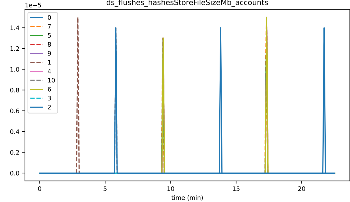
ds_flushes_hashesStoreFileSizeMb_accounts
