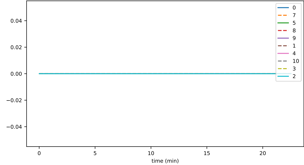
sync_phase_06_fraction_SENDING_EVENTS
