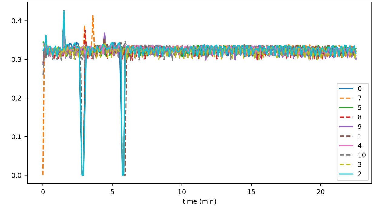
sync_phase_06_fraction_SENDING_EVENTS
