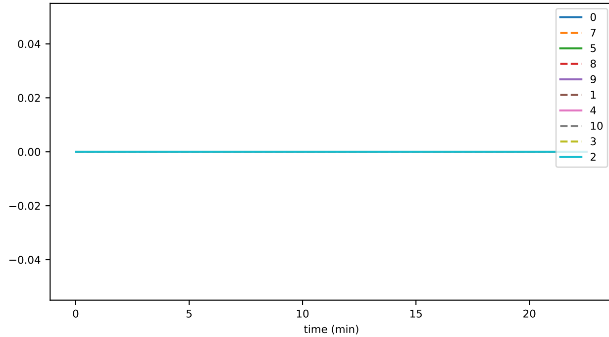
sync_phase_06_fraction_SELF_FALLEN_BEHIND
