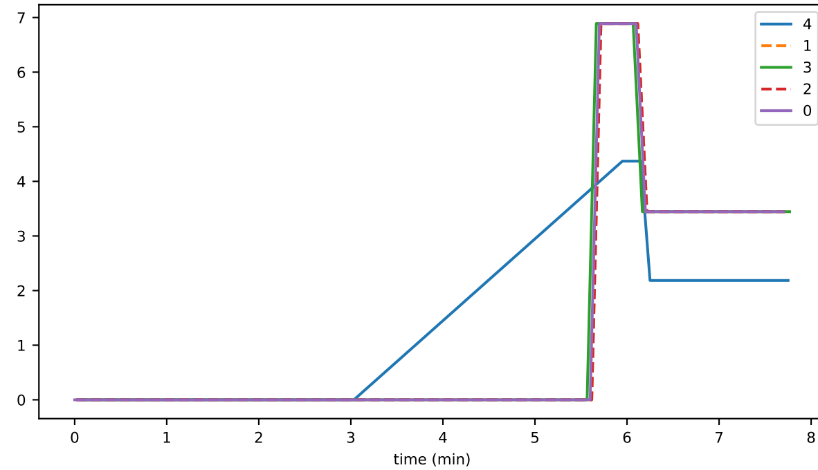
preconsensusEventFileOldestIdentifier
