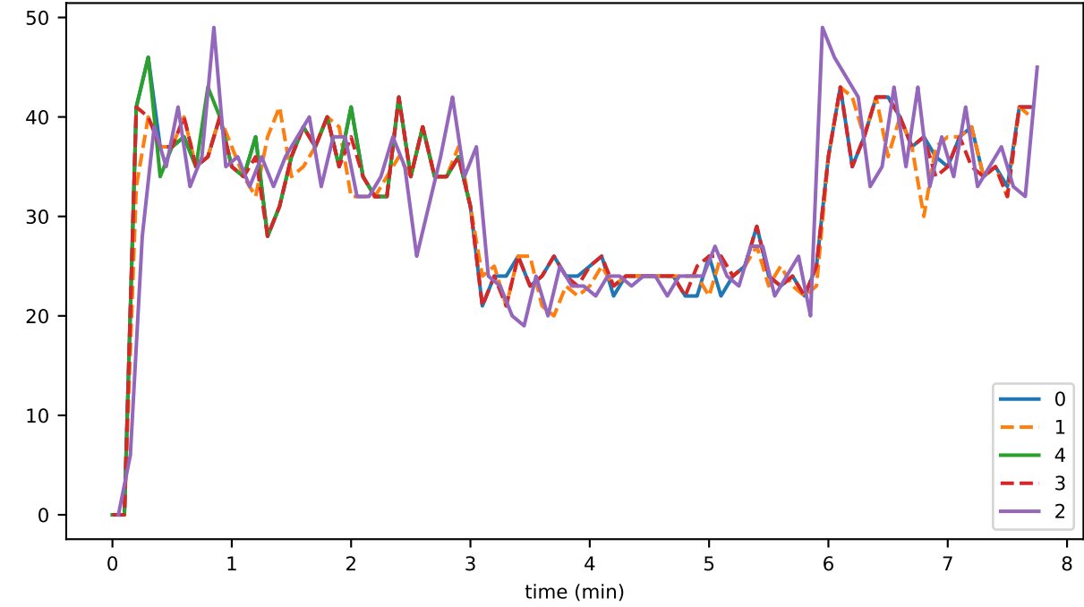
eventsPerRound
