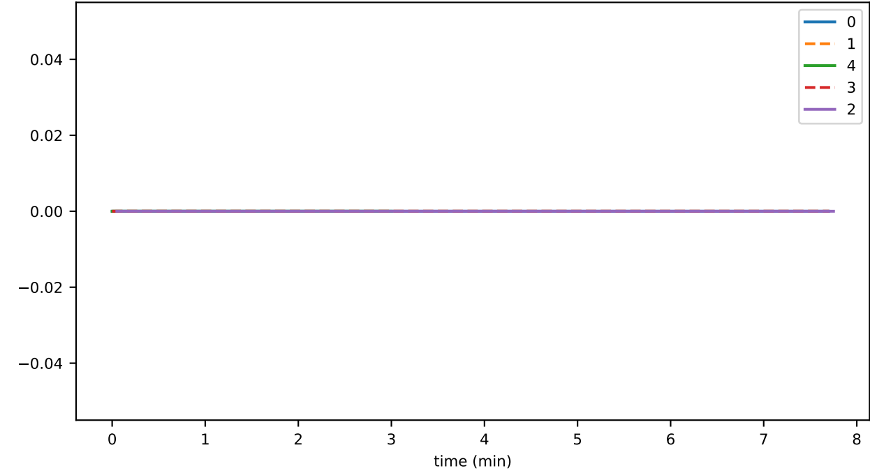
branchingEvents
