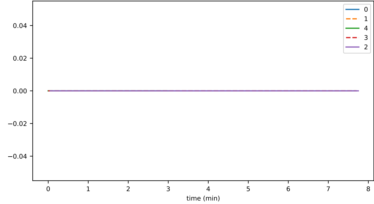
ds_compactions_level_0_hashesTimeMs_state
