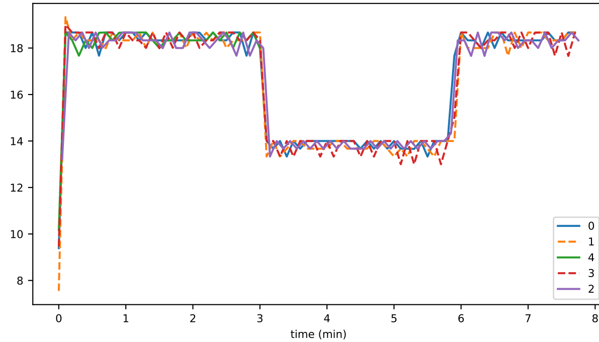
BranchDetector_unhandled_task_count
