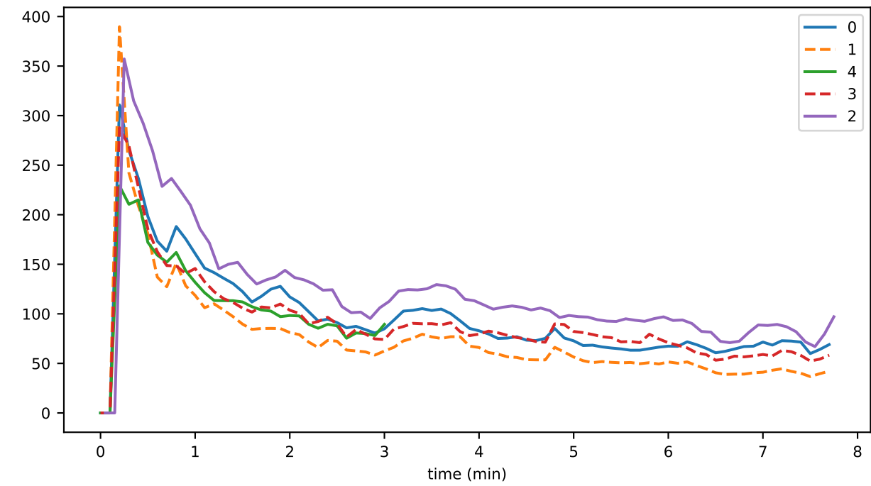
timeToDeleteState
