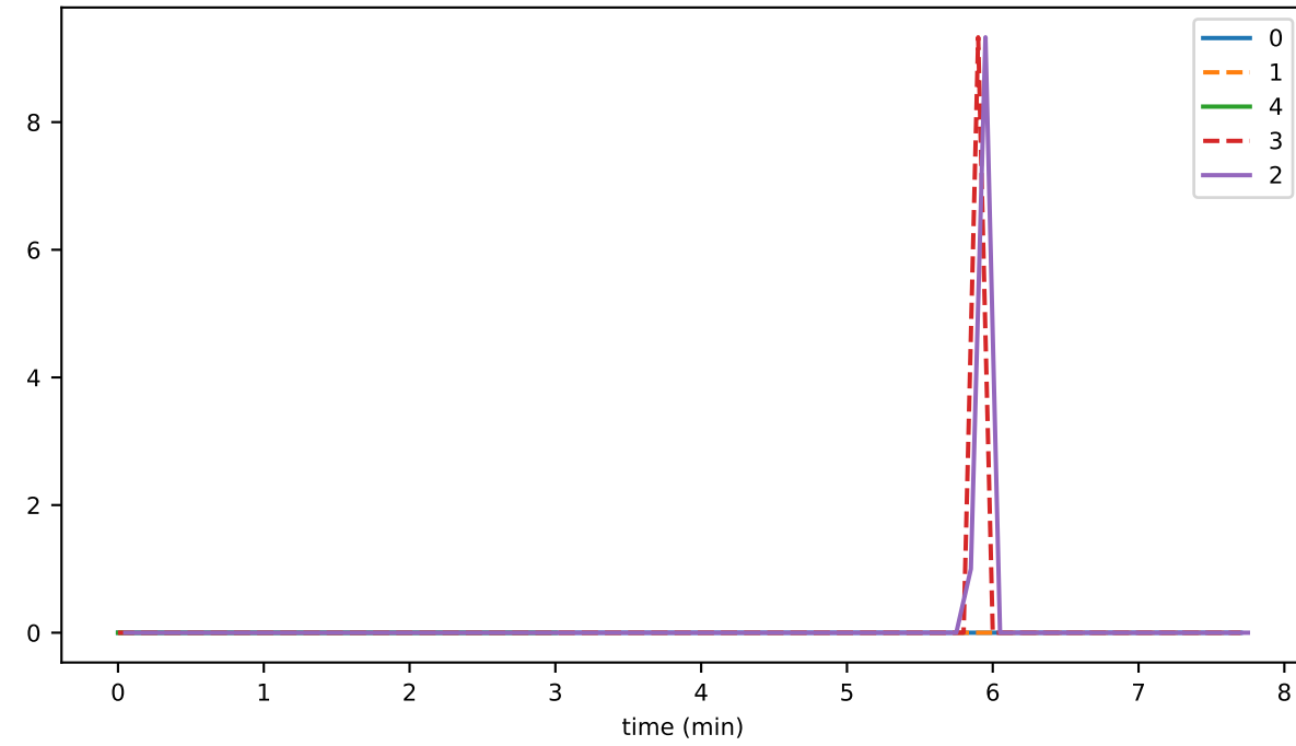
ds_compactions_level_0_hashesSavedSpaceMb_state
