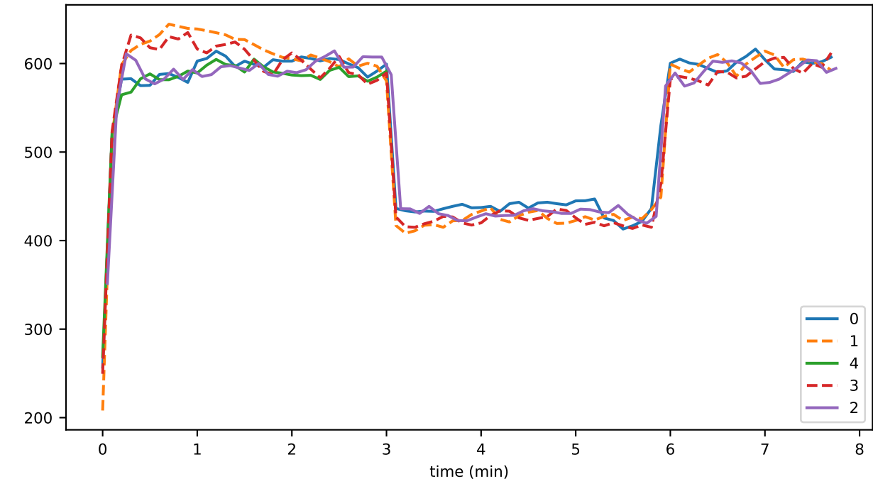
ds_compactions_level_0_hashesTimeMs_state
