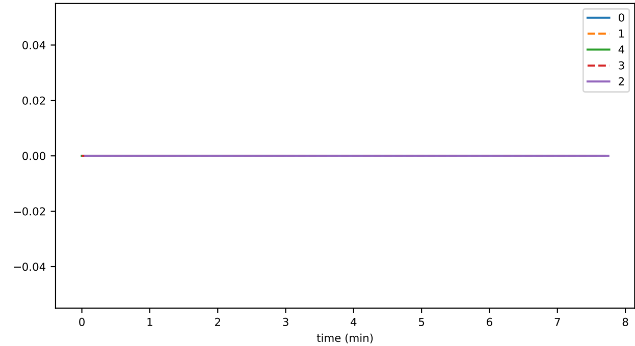
eventsPerRound
