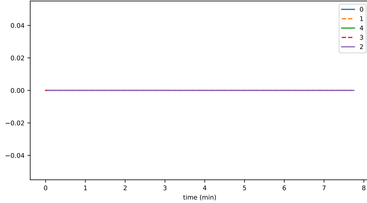
ds_compactions_level_0_hashesSavedSpaceMb_state
