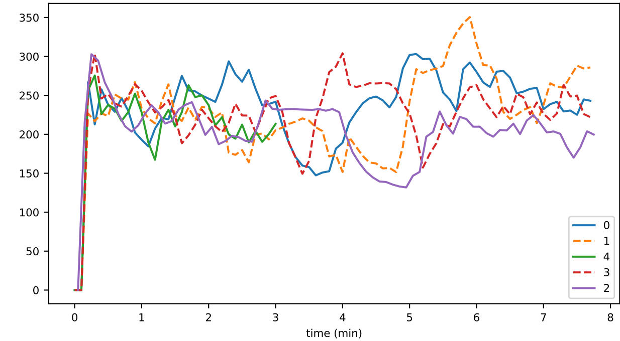
branchingEvents
